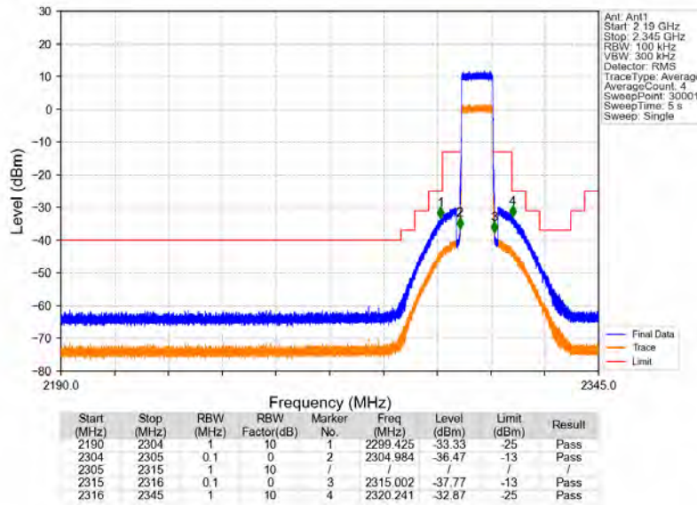
Band30_10MHz_64QAM_HCH_2310MHz_RB_50_0_NTNV
