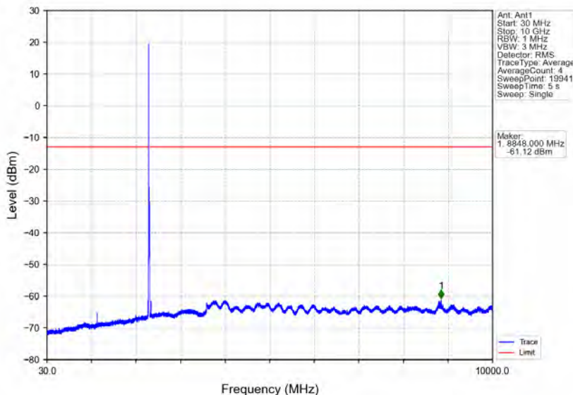
Band30_10MHz_64QAM_HCH_2310MHz_RB_1_0_NTV
