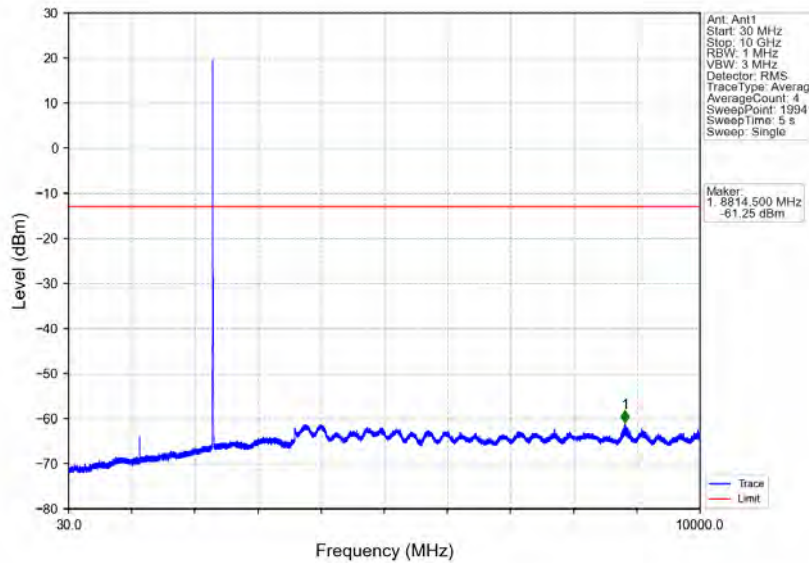
Band30_5MHz_64QAM_LCH_2307.5MHz_RB_1_0_NTNV
