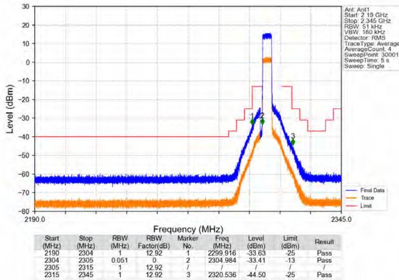
Band30_5MHz_16QAM_LCH_2307.5MHz_RB_25_0_NTNV
