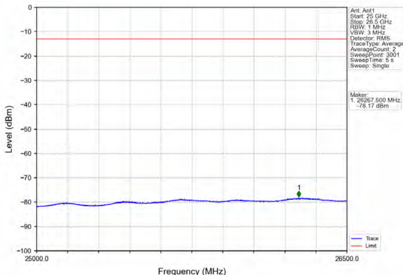
Band30_10MHz_64QAM_MCH_2310MHz_RB_1_0_NTNV
