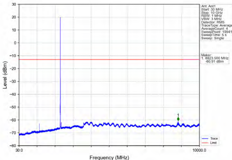
Band30_5MHz_64QAM_HCH_2312.5MHz_RB_1_0_NTNV
