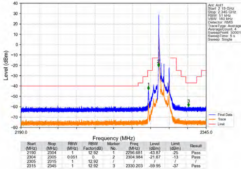
Band30_5MHz_64QAM_LCH_2307.5MHz_RB_1_0_NTNV
