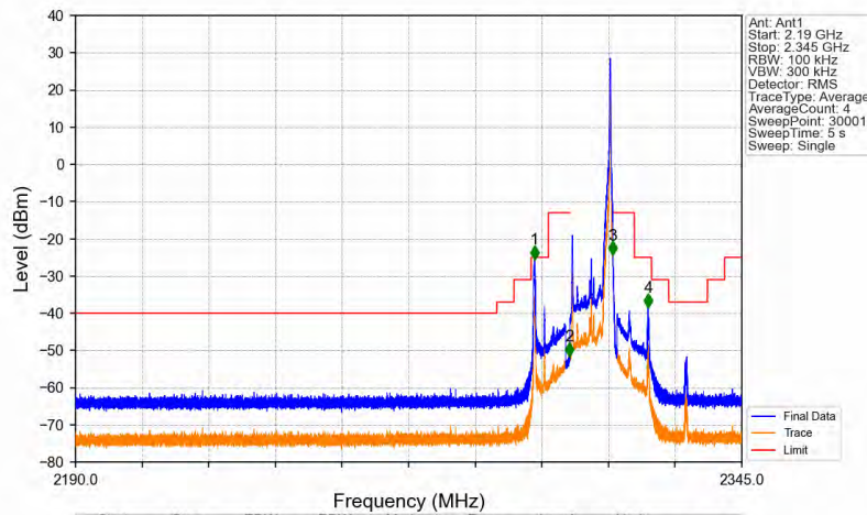
Band30_10MHz_64QAM_HCH_2310MHz_RB_1_49_NTNV
