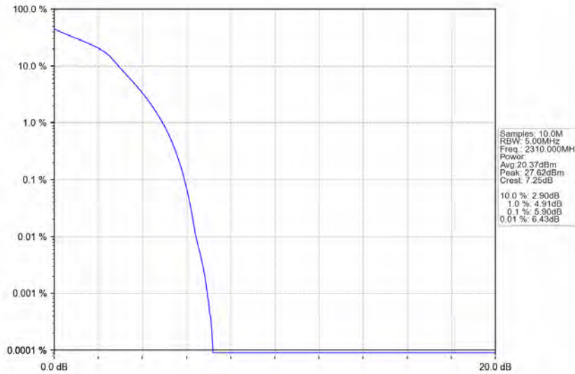
Band30_5MHz_16QAM_MCH_2310MHz_RB_25_0_NTNV
