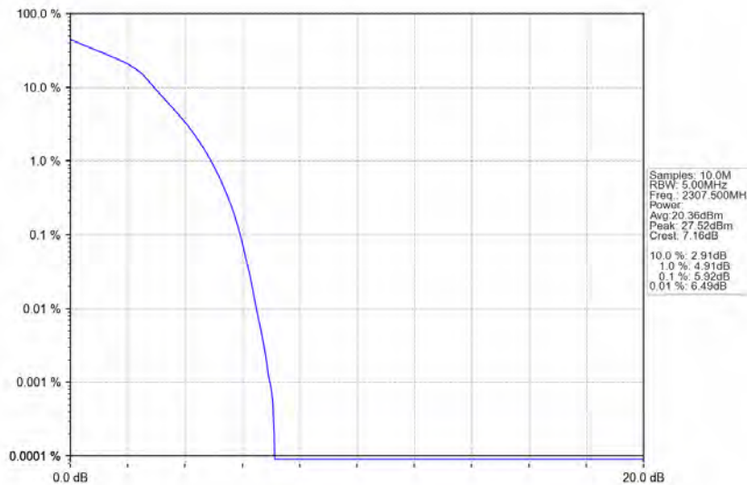
Band30_5MHz_16QAM_LCH_2307.5MHz_RB_25_0_NTNV
