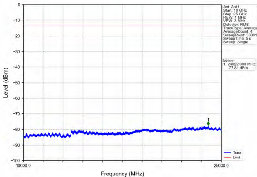
Band30_5MHz_64QAM_HCH_2312.5MHz_RB_1_0_NTNV
