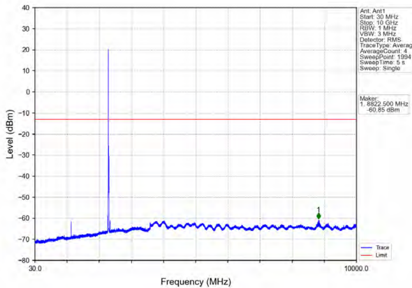
Band30_10MHz_64QAM_MCH_2310MHz_RB_1_0_NTNV
