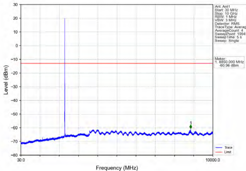
Band30_5MHz_64QAM_MCH_2310MHz_RB_1_0_NTNV
