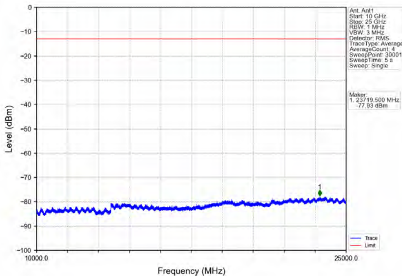
Band30_10MHz_64QAM_HCH_2310MHz_RB_1_0_NTV
