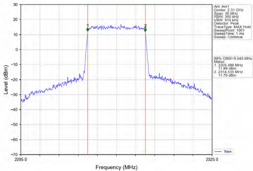
Band30_10MHz_64QAM_LCH_2310MHz_RB_50_0_NTNV
