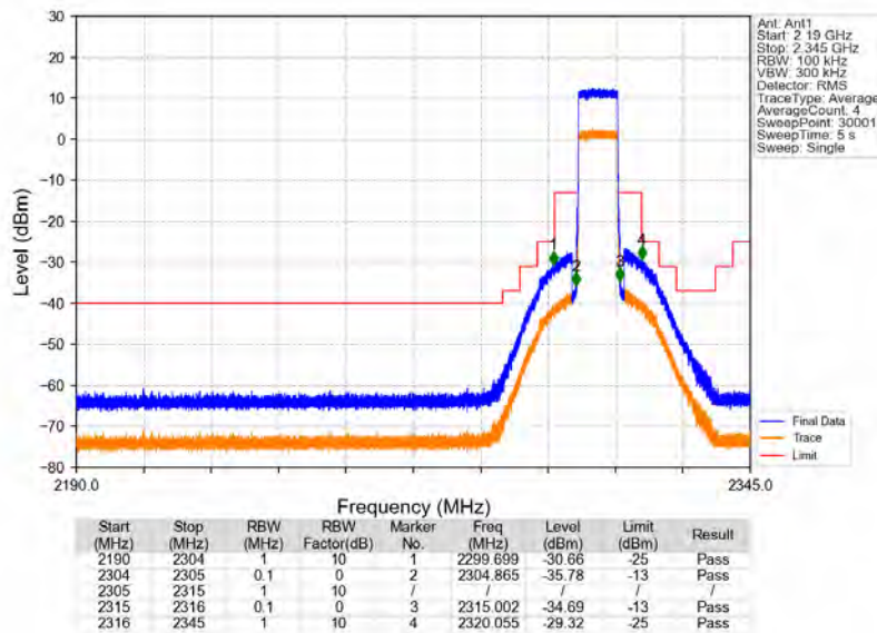
Band30_10MHz_16QAM_HCH_2310MHz_RB_50_0_NTNV
