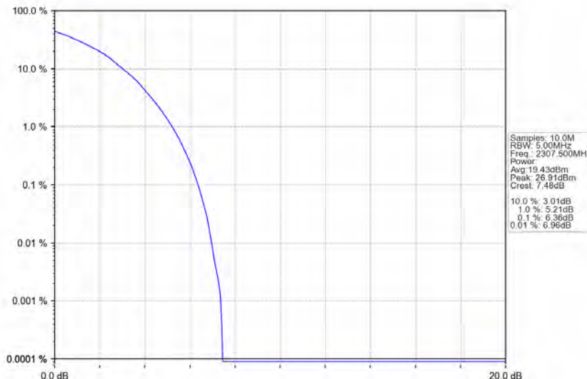
Band30_5MHz_64QAM_LCH_2307.5MHz_RB_25_0_NTNV
