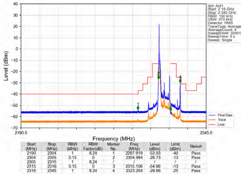
Band30_10MHz_64QAM_LCH_2310MHz_RB_1_0_NTNV
