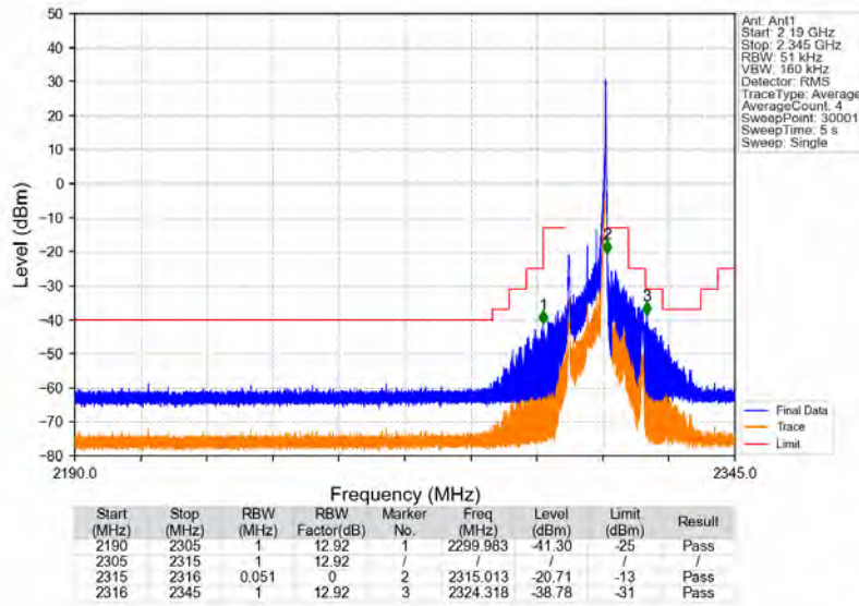
Band30_5MHz_QPSK_HCH_2312.5MHz_RB_1_24_NTNV
