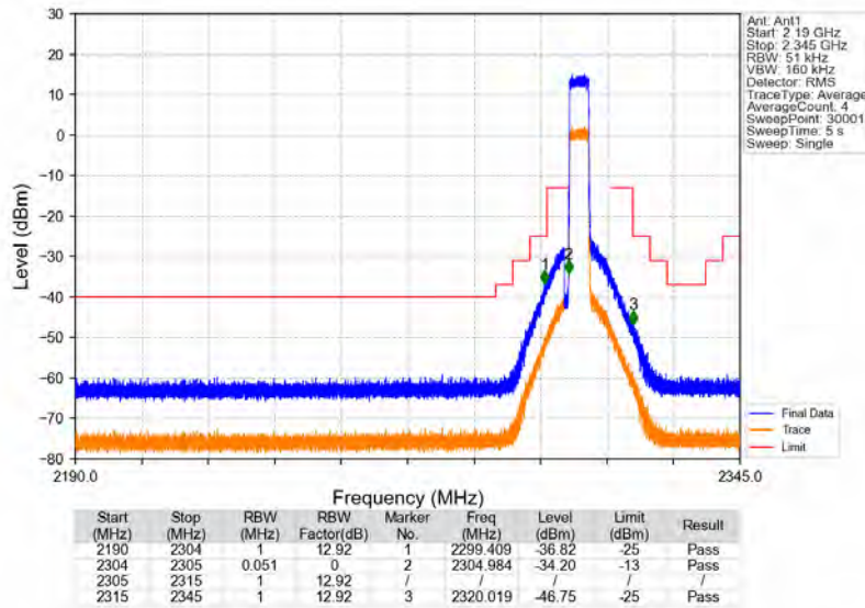
Band30_5MHz_64QAM_MCH_2310MHz_RB_1_0_NTNV
