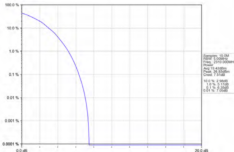
Band30_5MHz_64QAM_MCH_2310MHz_RB_25_0_NTNV
