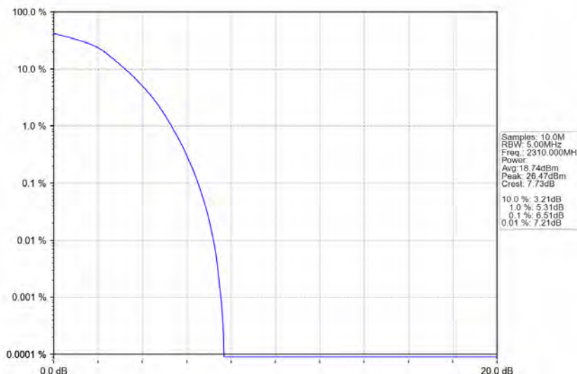
Band30_10MHz_16QAM_HCH_2310MHz_RB_50_0_NTNV
