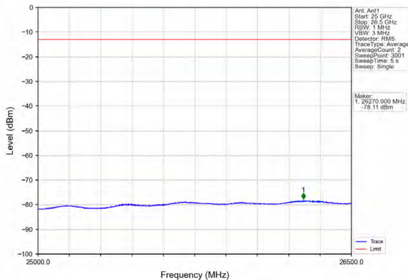
Band30_5MHz_16QAM_HCH_2312.5MHz_RB_1_0_NTNV
