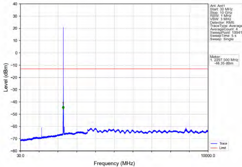
Band30_5MHz_16QAM_HCH_2312.5MHz_RB_1_0_NTNV
