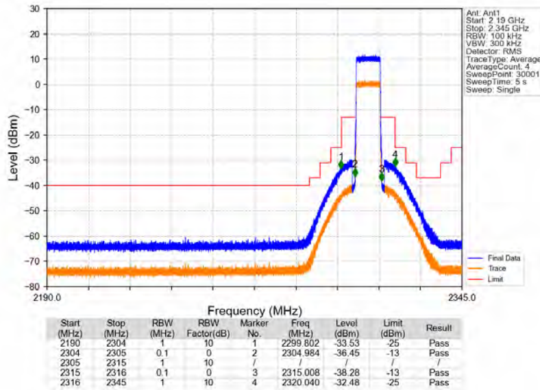
Band30_10MHz_64QAM_MCH_2310MHz_RB_1_0_NTNV
