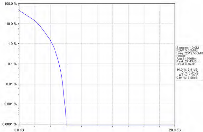
Band30_5MHz_QPSK_HCH_2312.5MHz_RB_25_0_NTNV
