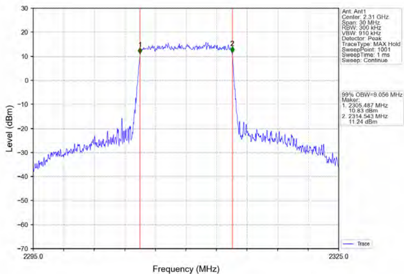
Band30_10MHz_64QAM_HCH_2310MHz_RB_50_0_NTNV
