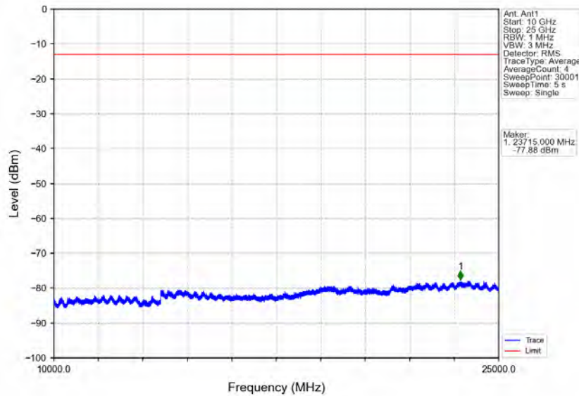
Band30_10MHz_16QAM_HCH_2310MHz_RB_1_0_NTV
