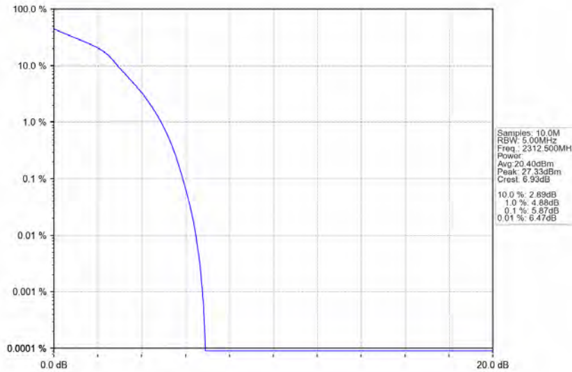
Band30_5MHz_16QAM_HCH_2312.5MHz_RB_25_0_NTNV
