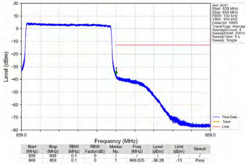
Band26b_10MHz_QPSK_HCH_844MHz_RB_50_0_NTNV
