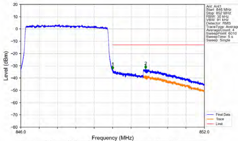
Band26b_3MHz_16QAM_HCH_847.5MHz_RB_15_0_NTNV
