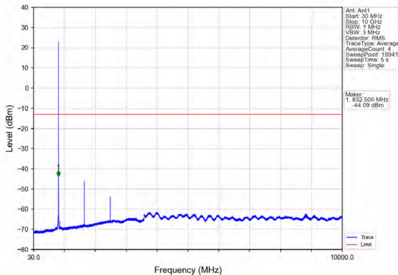
Band26b_1.4MHz_QPSK_MCH_836.5MHz_RB_1_0_NTNV
