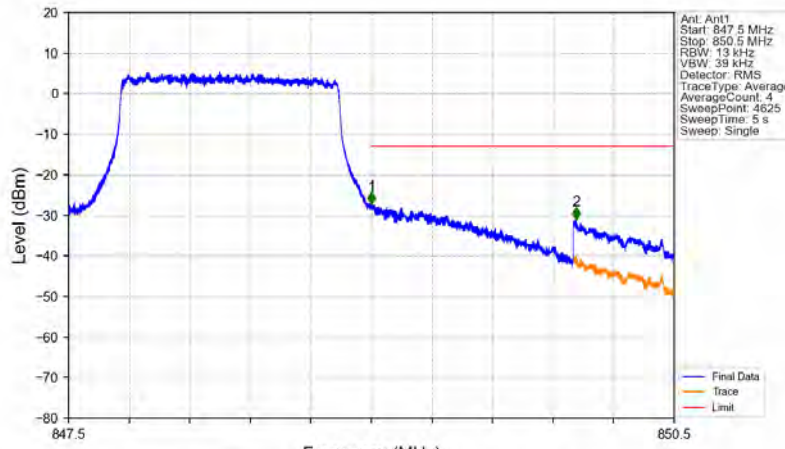
Band26b_1.4MHz_QPSK_HCH_848.3MHz_RB_6_0_NTNV
