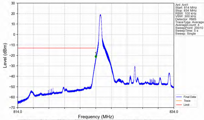
Band26b_10MHz_64QAM_LCH_829MHz_RB_1_0_NTNV
