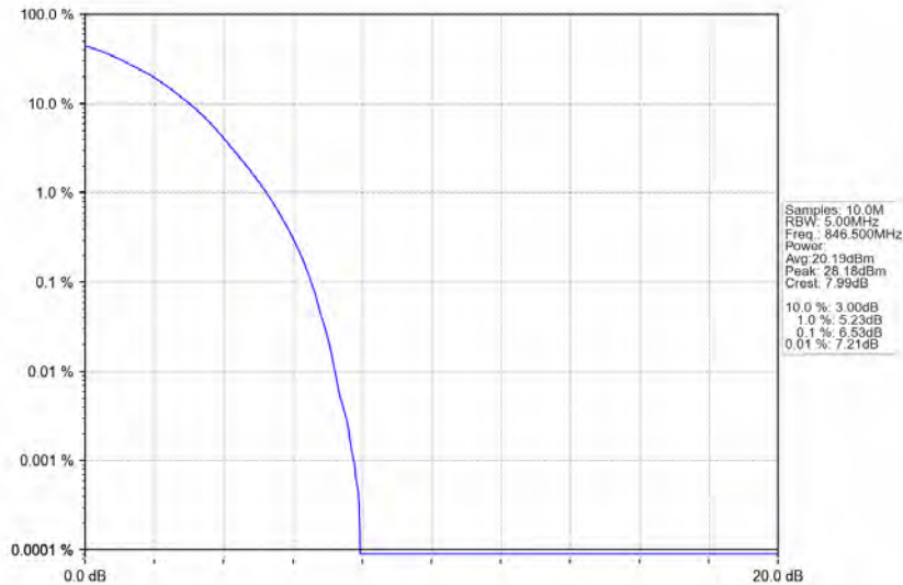
Band26b_5MHz_64QAM_HCH_846.5MHz_RB_25_0_NTNV
