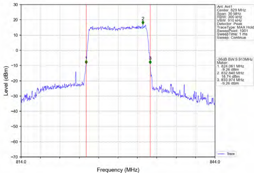
Band26b_10MHz_64QAM_LCH_829MHz_RB_50_0_NTNV
