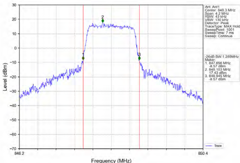
Band26b_1.4MHz_16QAM_HCH_848.3MHz_RB_6_0_NTNV
