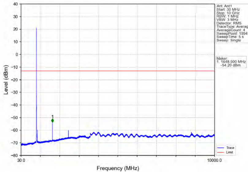
Band26b_5MHz_64QAM_LCH_826.5MHz_RB_1_0_NTNV
