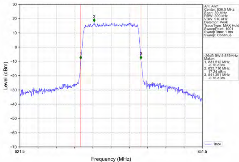
Band26b_10MHz_16QAM_MCH_836.5MHz_RB_50_0_NTNV
