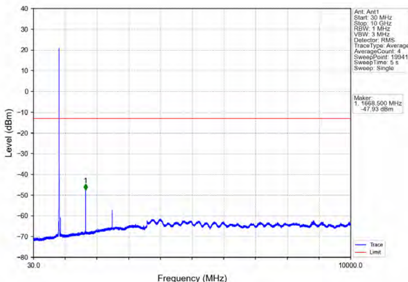
Band26b_5MHz_64QAM_MCH_836.5MHz_RB_1_0_NTNV
