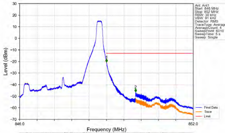
Band26b_3MHz_16QAM_HCH_847.5MHz_RB_1_14_NTNV
