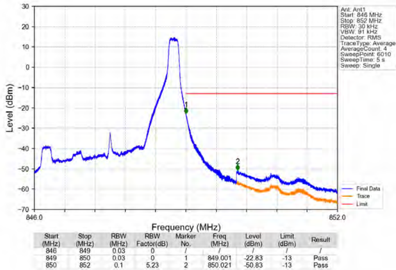
Band26b_3MHz_64QAM_HCH_847.5MHz_RB_1_14_NTNV
