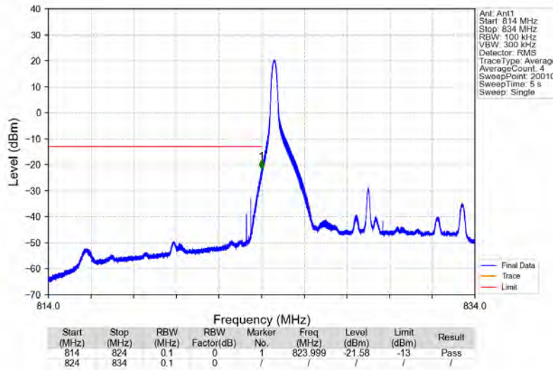
Band26b_10MHz_16QAM_LCH_829MHz_RB_1_0_NTNV
