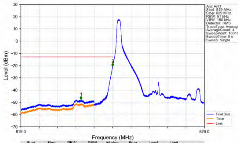
Band26b_5MHz_16QAM_LCH_826.5MHz_RB_1_0_NTNV
