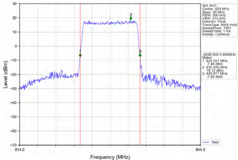
Band26b_10MHz_QPSK_LCH_829MHz_RB_50_0_NTNV
