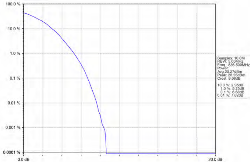
Band26b_5MHz_64QAM_MCH_836.5MHz_RB_25_0_NTNV
