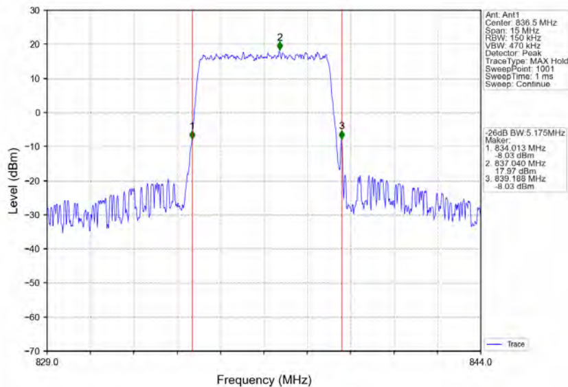
Band26b_5MHz_QPSK_MCH_836.5MHz_RB_25_0_NTNV
