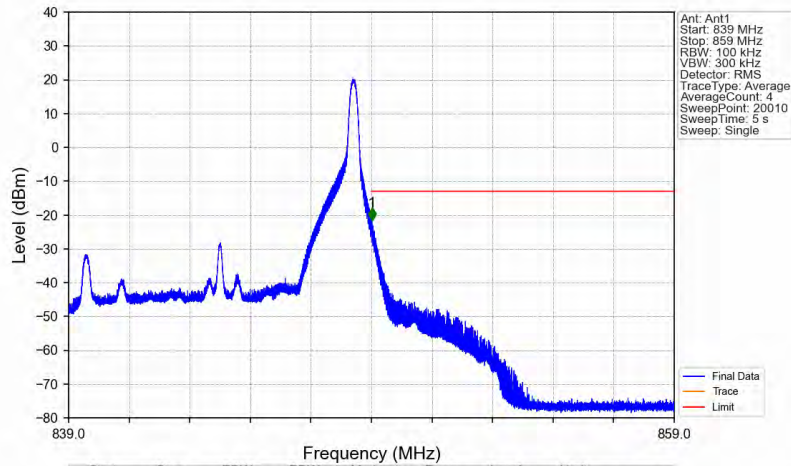
Band26b_10MHz_16QAM_HCH_844MHz_RB_1_49_NTNV
