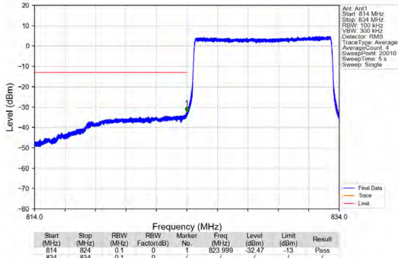
Band26b_10MHz_QPSK_LCH_829MHz_RB_50_0_NTNV
