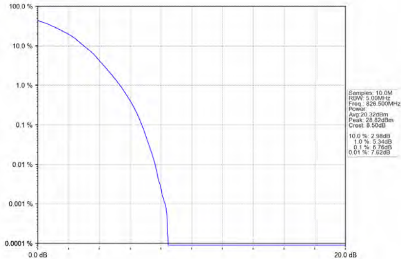
Band26b_5MHz_64QAM_LCH_826.5MHz_RB_25_0_NTNV
