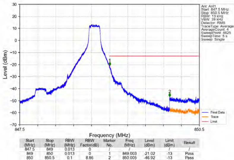
Band26b_1.4MHz_QPSK_HCH_848.3MHz_RB_1_5_NTNV
