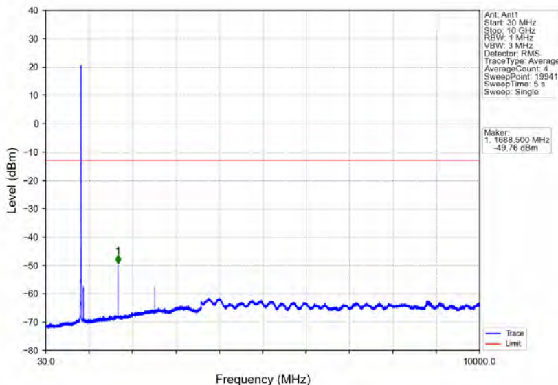
Band26b_5MHz_64QAM_HCH_846.5MHz_RB_1_24_NTNV
