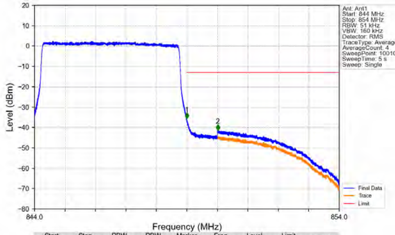
Band26b_5MHz_64QAM_HCH_846.5MHz_RB_25_0_NTNV
