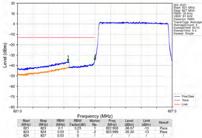
Band26b_3MHz_64QAM_LCH_825.5MHz_RB_15_0_NTNV
