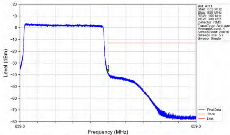
Band26b_10MHz_16QAM_HCH_844MHz_RB_50_0_NTNV
