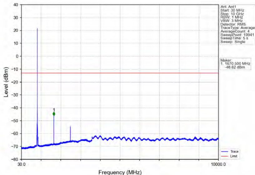
Band26b_3MHz_16QAM_HCH_847.5MHz_RB_1_0_NTNV
