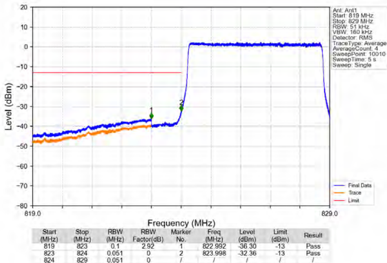
Band26b_5MHz_64QAM_LCH_826.5MHz_RB_25_0_NTNV
