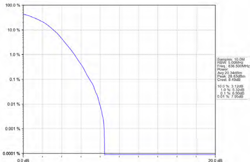
Band26b_1.4MHz_64QAM_MCH_836.5MHz_RB_6_0_NTNV
