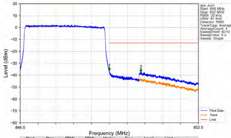
Band26b_3MHz_64QAM_HCH_847.5MHz_RB_15_0_NTNV
