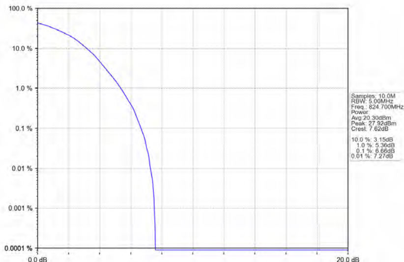
Band26b_1.4MHz_64QAM_LCH_824.7MHz_RB_6_0_NTNV
