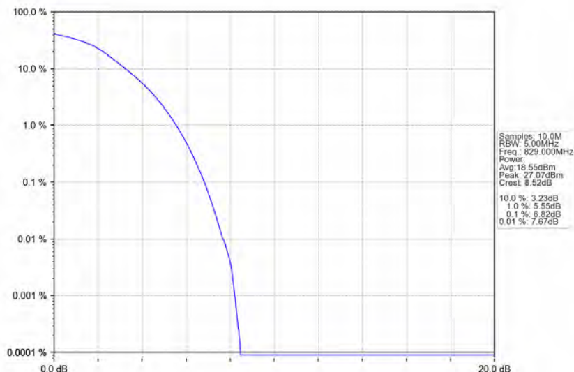
Band26b_10MHz_64QAM_LCH_829MHz_RB_50_0_NTNV
