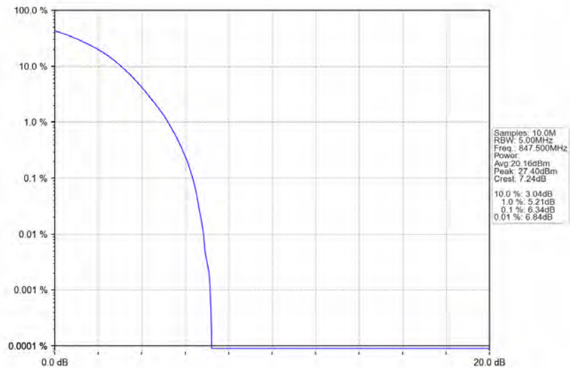
Band26b_3MHz_64QAM_HCH_847.5MHz_RB_15_0_NTNV
