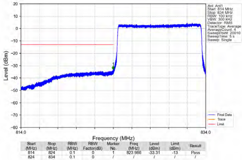
Band26b_10MHz_16QAM_LCH_829MHz_RB_50_0_NTNV
