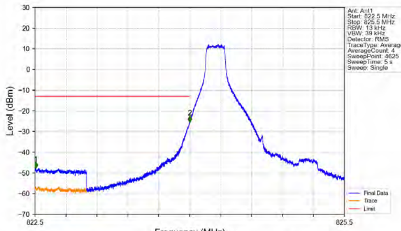
Band26b_1.4MHz_16QAM_LCH_824.7MHz_RB_1_0_NTNV
