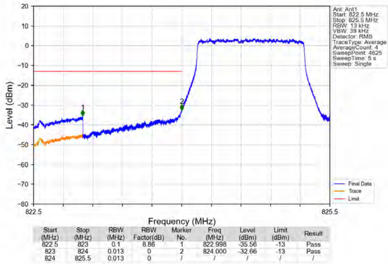
Band26b_1.4MHz_16QAM_LCH_824.7MHz_RB_6_0_NTNV
