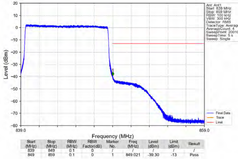
Band26b_10MHz_64QAM_HCH_844MHz_RB_50_0_NTNV
