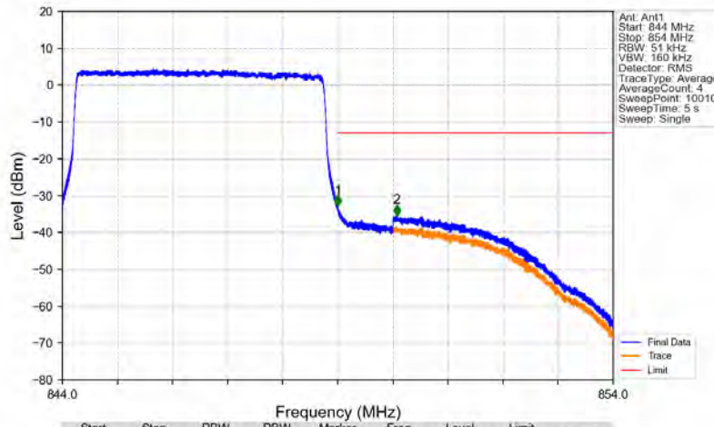
Band26b_5MHz_QPSK_HCH_846.5MHz_RB_25_0_NTNV
