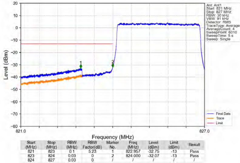
Band26b_3MHz_QPSK_LCH_825.5MHz_RB_15_0_NTNV
