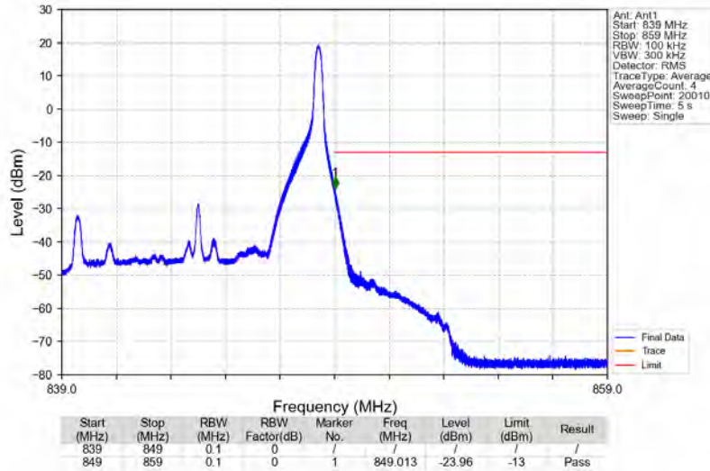
Band26b_10MHz_64QAM_HCH_844MHz_RB_1_49_NTNV
