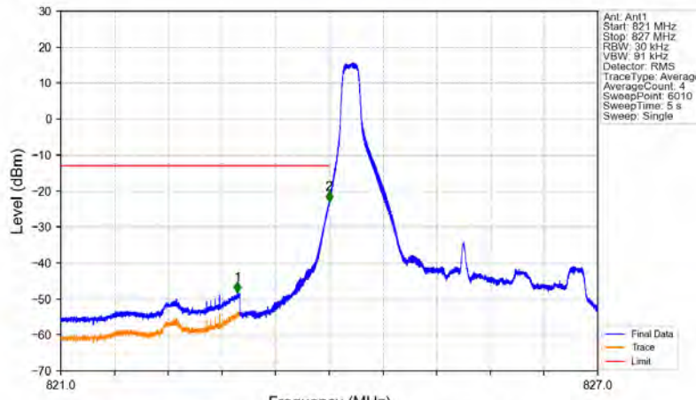
Band26b_3MHz_16QAM_LCH_825.5MHz_RB_1_0_NTNV
