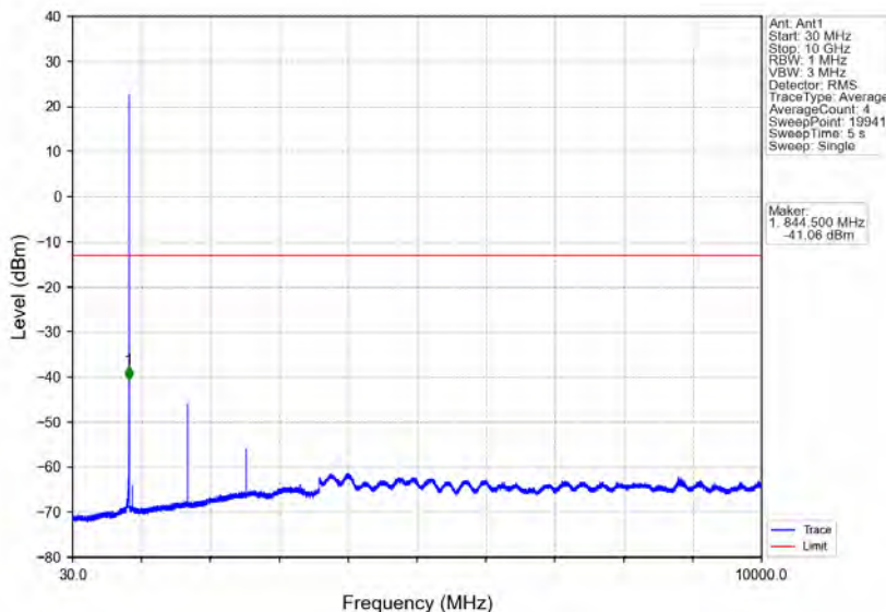
Band26b_1.4MHz_QPSK_HCH_848.3MHz_RB_1_5_NTNV
