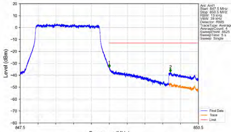
Band26b_1.4MHz_64QAM_HCH_848.3MHz_RB_6_0_NTNV
