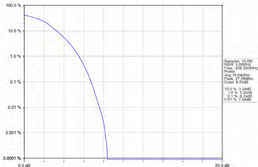
Band26b_10MHz_64QAM_MCH_836.5MHz_RB_50_0_NTNV
