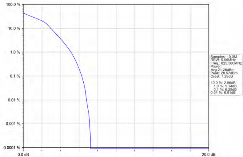
Band26b_3MHz_16QAM_LCH_825.5MHz_RB_15_0_NTNV
