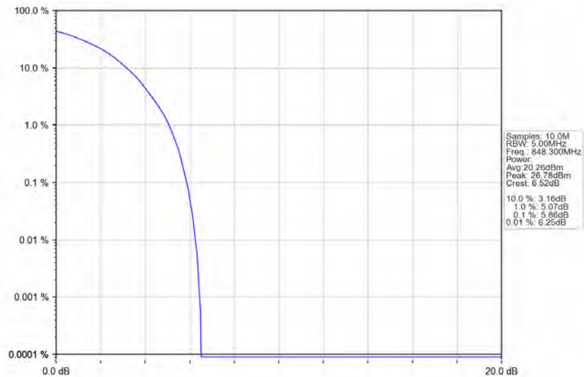
Band26b_1.4MHz_64QAM_HCH_848.3MHz_RB_6_0_NTNV
