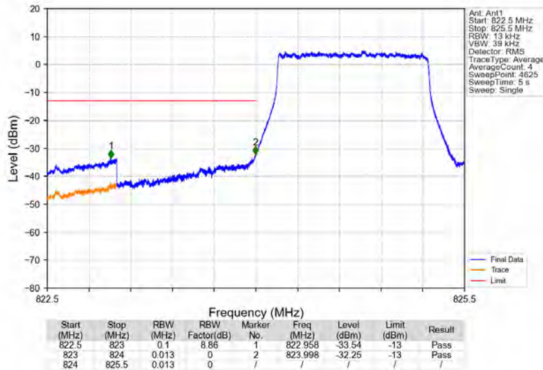
Band26b_1.4MHz_QPSK_LCH_824.7MHz_RB_6_0_NTNV
