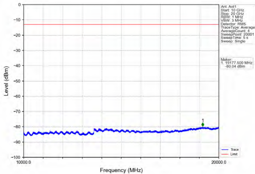
Band25_1.4MHz_64QAM_LCH_1850.7MHz_RB_6_0_NTNV
