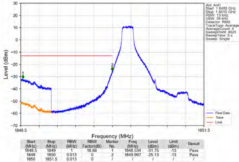
Band25_1.4MHz_16QAM_LCH_1850.7MHz_RB_1_0_NTNV
