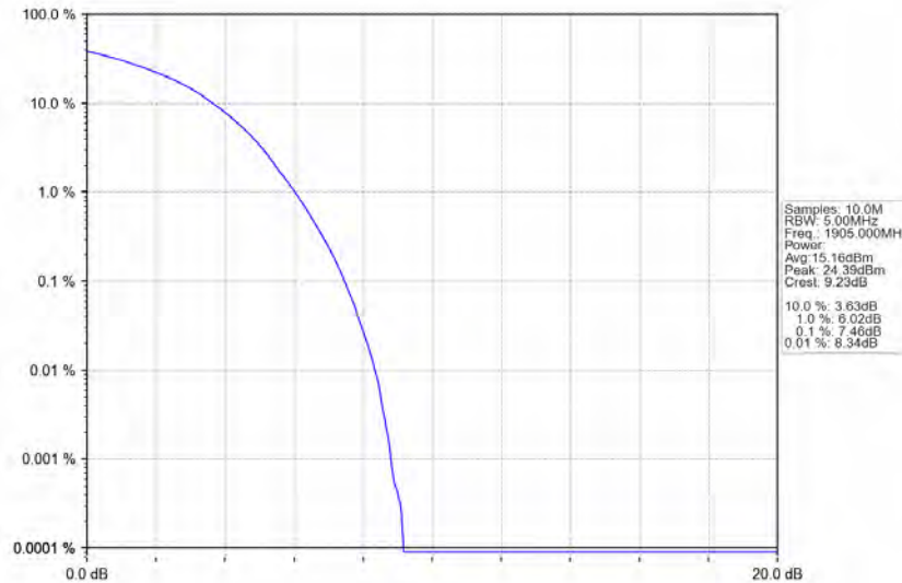
Band25_20MHz_64QAM_HCH_1905MHz_RB_100_0_NTNV
