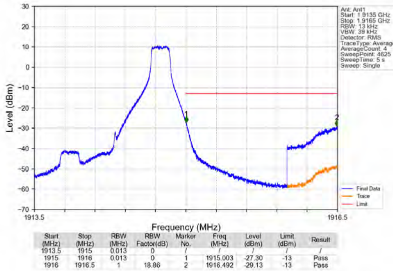
Band25_1.4MHz_64QAM_HCH_1914.3MHz_RB_1_5_NTNV
