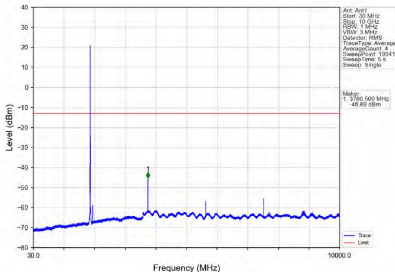
Band25_5MHz_16QAM_MCH_1882.5MHz_RB_1_0_NTNV
