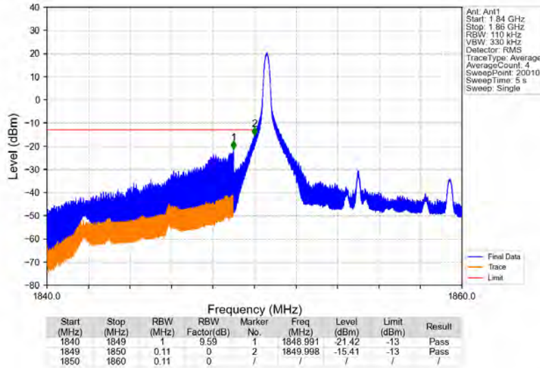
Band25_10MHz_16QAM_LCH_1855MHz_RB_1_0_NTNV
