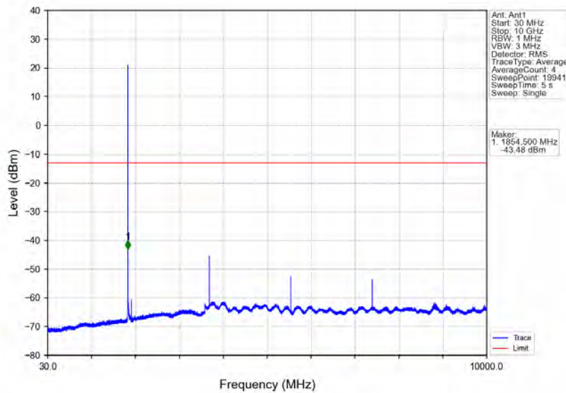
Band25_1.4MHz_16QAM_LCH_1850.7MHz_RB_1_0_NTNV
