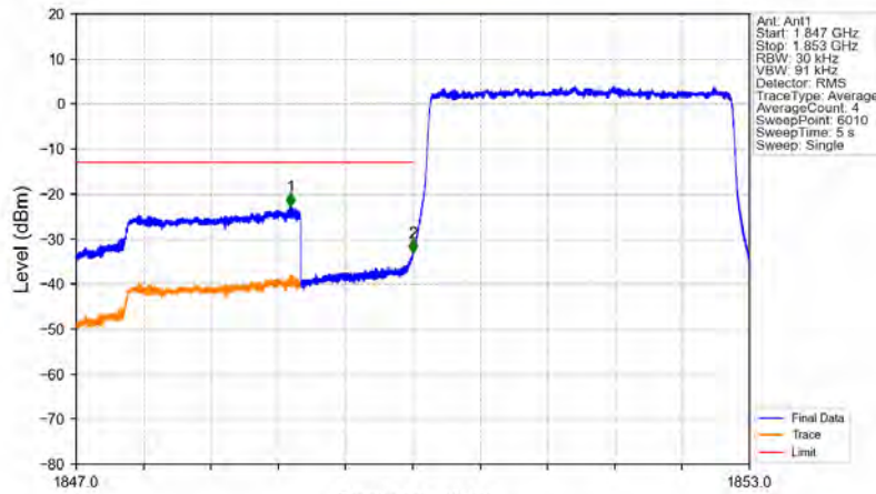
Band25_3MHz_QPSK_LCH_1851.5MHz_RB_15_0_NTNV
