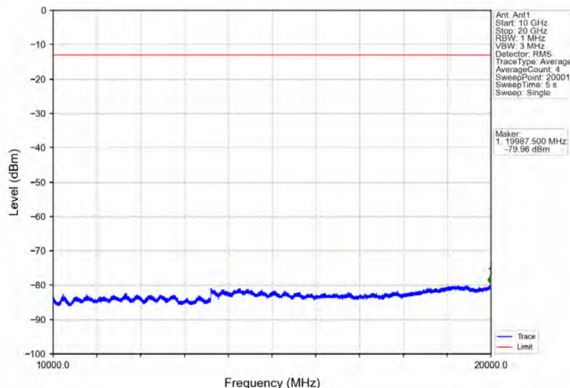
Band25_5MHz_16QAM_MCH_1882.5MHz_RB_1_0_NTNV
