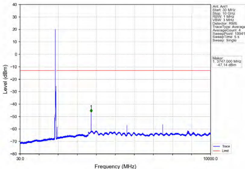
Band25_20MHz_64QAM_MCH_1882.5MHz_RB_1_0_NTNV
