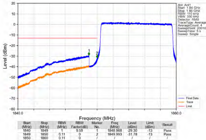
Band25_10MHz_64QAM_LCH_1855MHz_RB_50_0_NTNV
