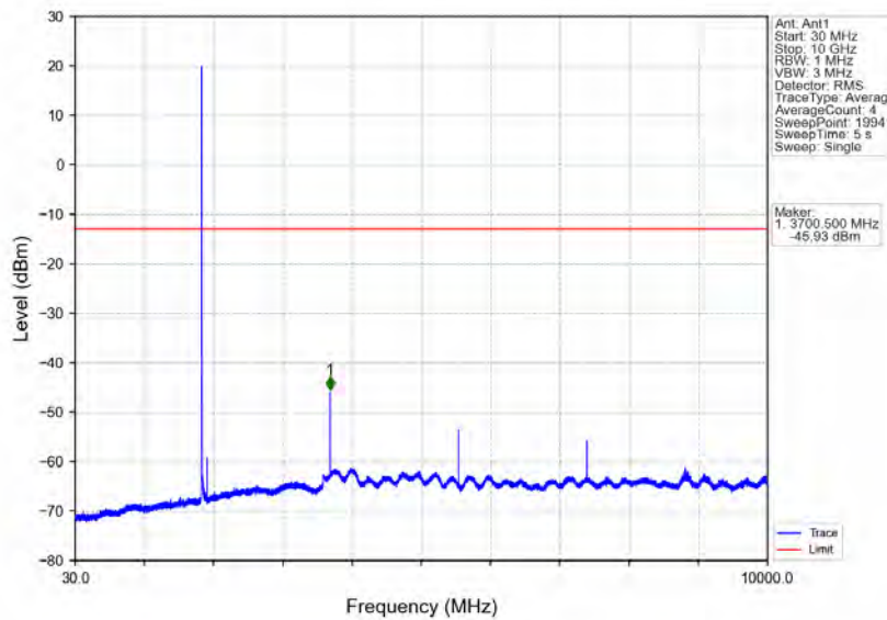
Band25_3MHz_64QAM_LCH_1851.5MHz_RB_1_0_NTNV
