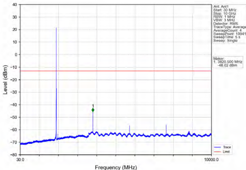
Band25_5MHz_16QAM_HCH_1912.5MHz_RB_1_0_NTNV
