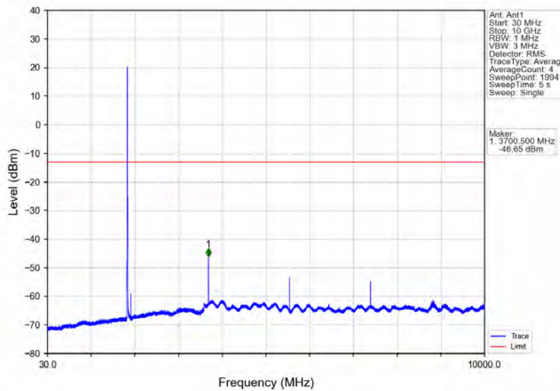
Band25_5MHz_64QAM_LCH_1852.5MHz_RB_1_0_NTNV
