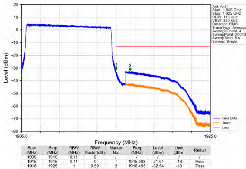
Band25_10MHz_QPSK_HCH_1910MHz_RB_50_0_NTV
