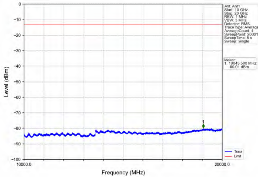
Band25_1.4MHz_16QAM_LCH_1850.7MHz_RB_6_0_NTNV
