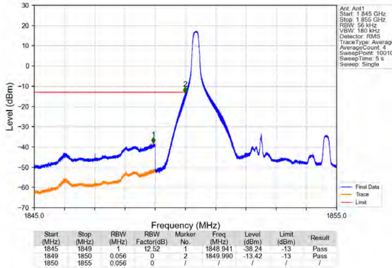
Band25_5MHz_16QAM_LCH_1852.5MHz_RB_1_0_NTNV
