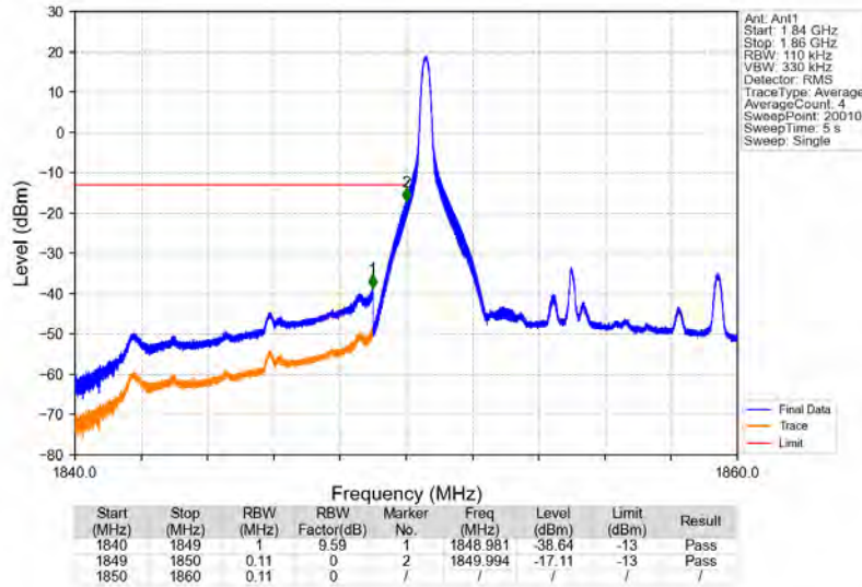
Band25_10MHz_64QAM_LCH_1855MHz_RB_1_0_NTNV
