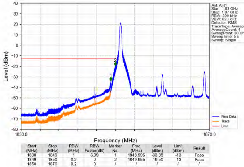
Band25_20MHz_16QAM_LCH_1860MHz_RB_1_0_NTNV
