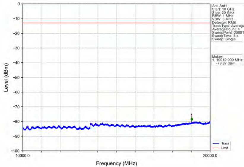
Band25_10MHz_64QAM_HCH_1910MHz_RB_1_0_NTV
