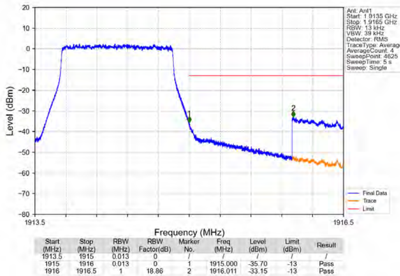
Band25_1.4MHz_64QAM_HCH_1914.3MHz_RB_6_0_NTNV
