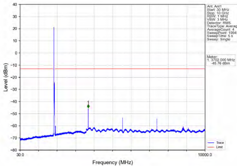
Band25_20MHz_16QAM_LCH_1860MHz_RB_1_0_NTNV
