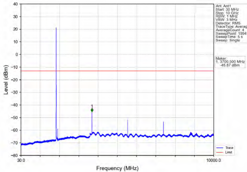
Band25_5MHz_16QAM_LCH_1852.5MHz_RB_1_0_NTNV
