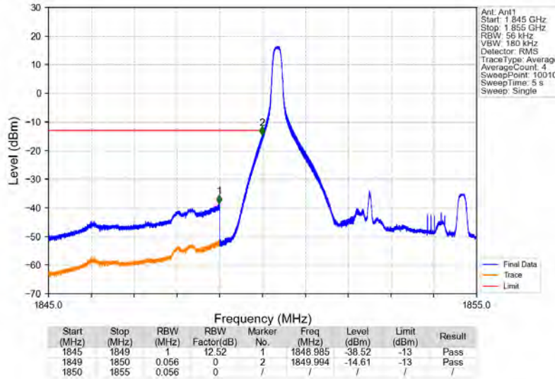
Band25_5MHz_64QAM_LCH_1852.5MHz_RB_1_0_NTNV
