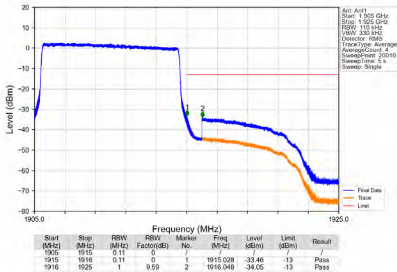
Band25_10MHz_64QAM_HCH_1910MHz_RB_50_0_NTNV
