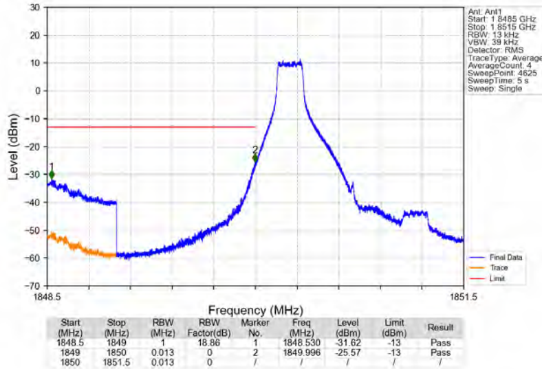
Band25_1.4MHz_64QAM_LCH_1850.7MHz_RB_1_0_NTNV
