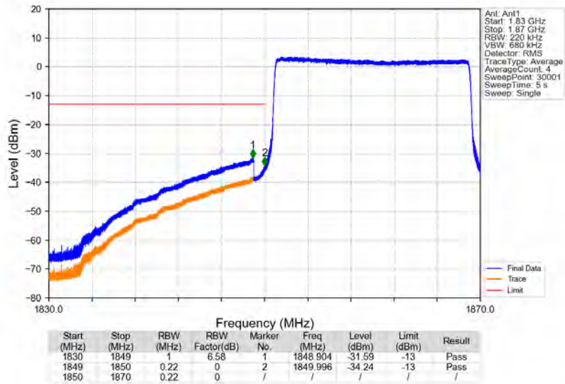
Band25_20MHz_16QAM_LCH_1860MHz_RB_100_0_NTNV
