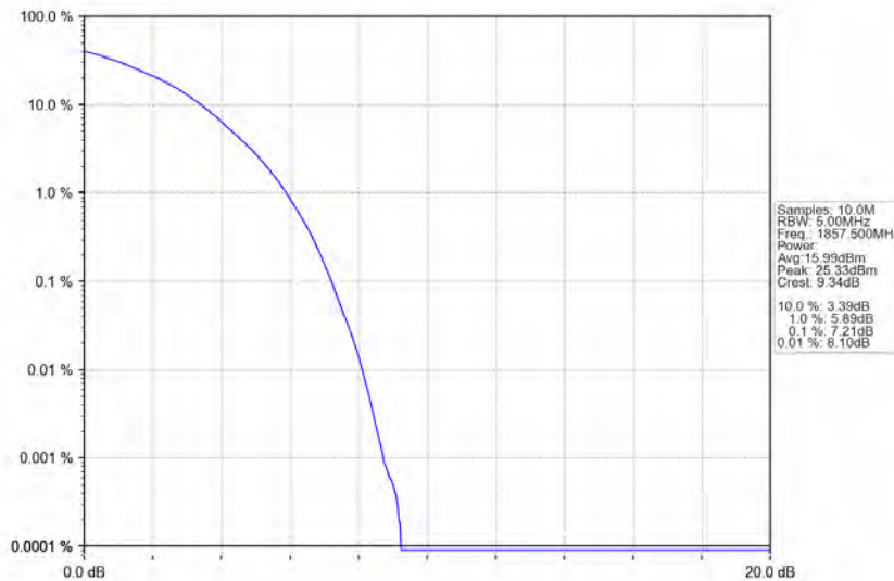
Band25_15MHz_64QAM_LCH_1857.5MHz_RB_75_0_NTNV
