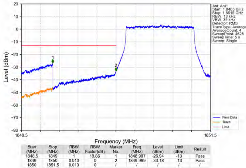
Band25_1.4MHz_16QAM_LCH_1850.7MHz_RB_6_0_NTNV
