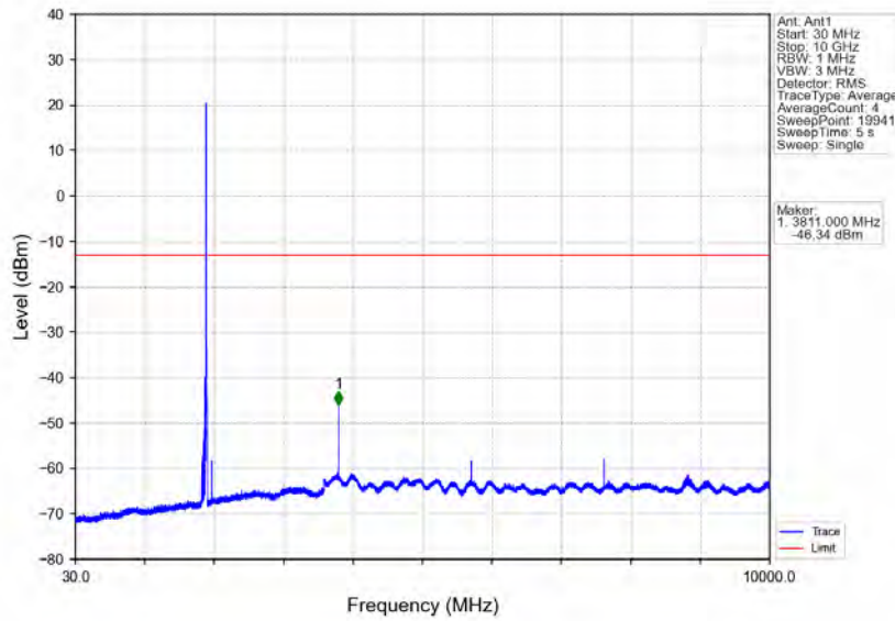
Band25_10MHz_64QAM_HCH_1910MHz_RB_1_0_NTV
