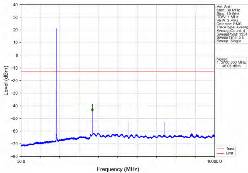
Band25_3MHz_16QAM_LCH_1851.5MHz_RB_1_0_NTNV
