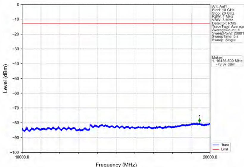
Band25_5MHz_16QAM_HCH_1912.5MHz_RB_1_0_NTNV
