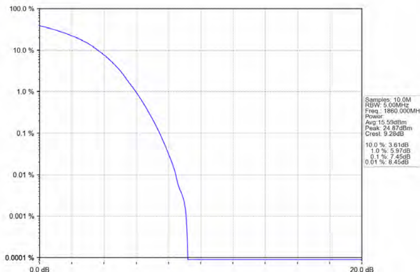
Band25_20MHz_16QAM_LCH_1860MHz_RB_100_0_NTNV
