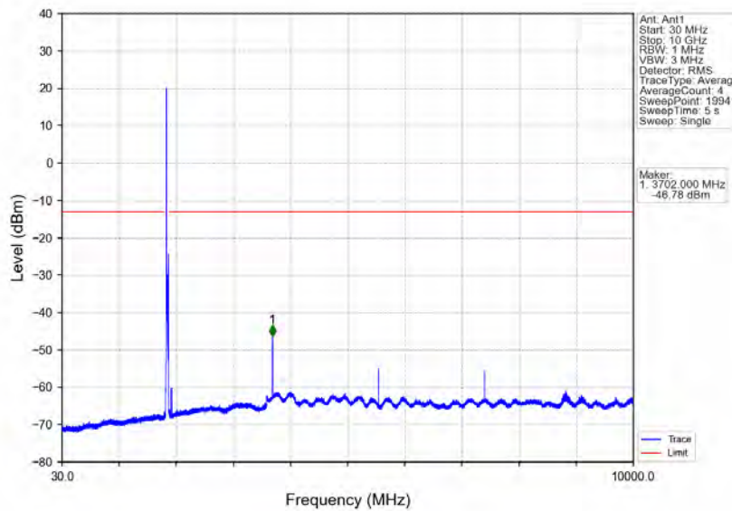
Band25_20MHz_64QAM_LCH_1860MHz_RB_1_0_NTNV
