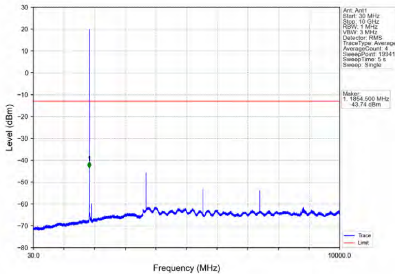
Band25_1.4MHz_64QAM_LCH_1850.7MHz_RB_1_0_NTNV
