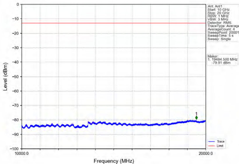
Band25_20MHz_64QAM_MCH_1882.5MHz_RB_1_0_NTNV
