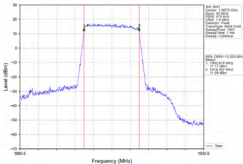
Band25_15MHz_16QAM_HCH_1907.5MHz_RB_75_0_NTNV
