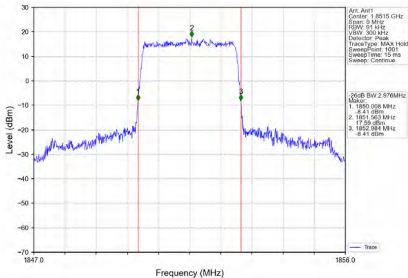
Band25_3MHz_QPSK_LCH_1851.5MHz_RB_15_0_NTNV
