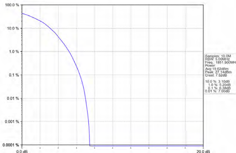
Band25_3MHz_64QAM_LCH_1851.5MHz_RB_15_0_NTNV
