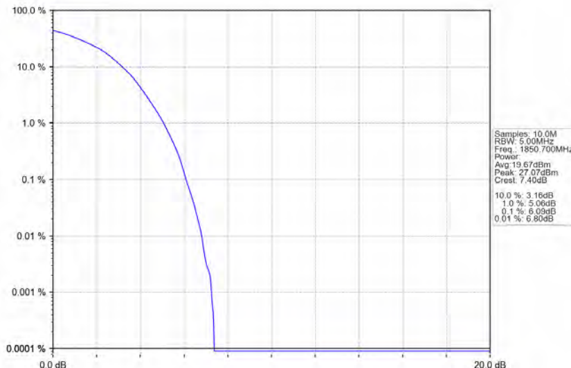
Band25_1.4MHz_64QAM_LCH_1850.7MHz_RB_6_0_NTNV
