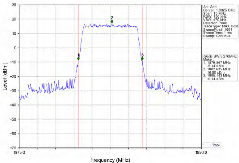
Band25_5MHz_QPSK_MCH_1882.5MHz_RB_25_0_NTNV
