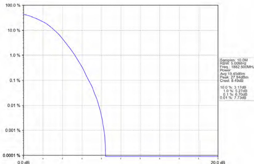
Band25_1.4MHz_64QAM_MCH_1882.5MHz_RB_6_0_NTNV
