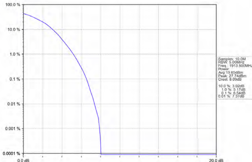
Band25_3MHz_64QAM_HCH_1913.5MHz_RB_15_0_NTNV
