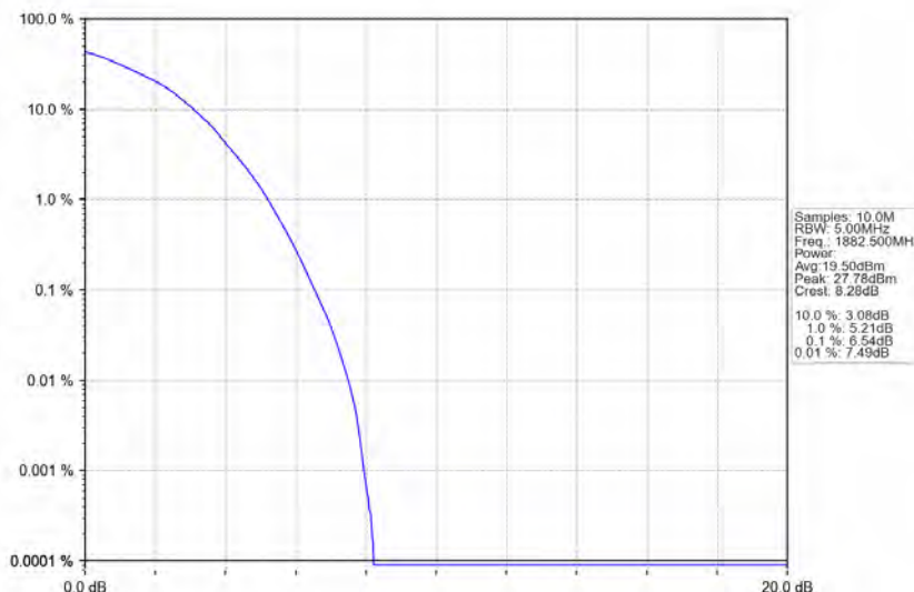
Band25_3MHz_64QAM_MCH_1882.5MHz_RB_15_0_NTNV
