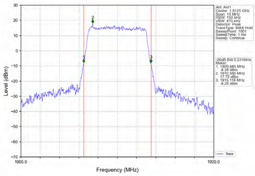
Band25_5MHz_16QAM_HCH_1912.5MHz_RB_25_0_NTNV
