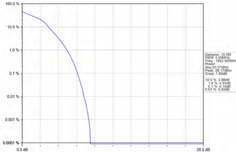
Band25_5MHz_16QAM_LCH_1852.5MHz_RB_25_0_NTNV
