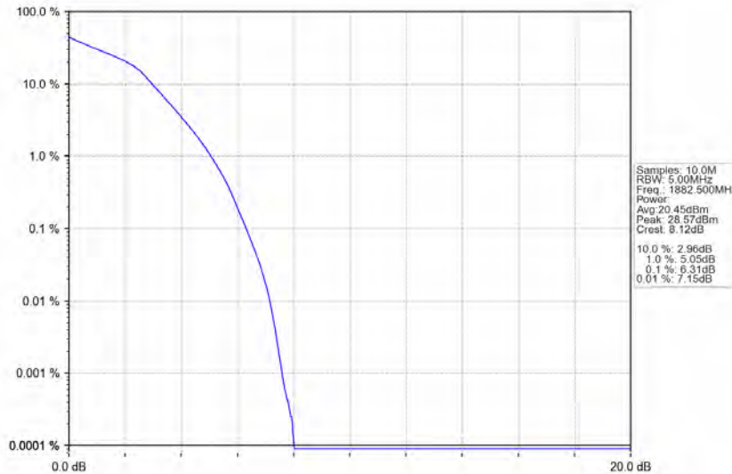
Band25_3MHz_16QAM_MCH_1882.5MHz_RB_15_0_NTNV
