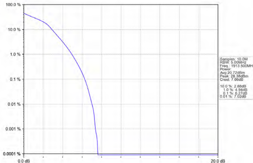
Band25_3MHz_16QAM_HCH_1913.5MHz_RB_15_0_NTNV
