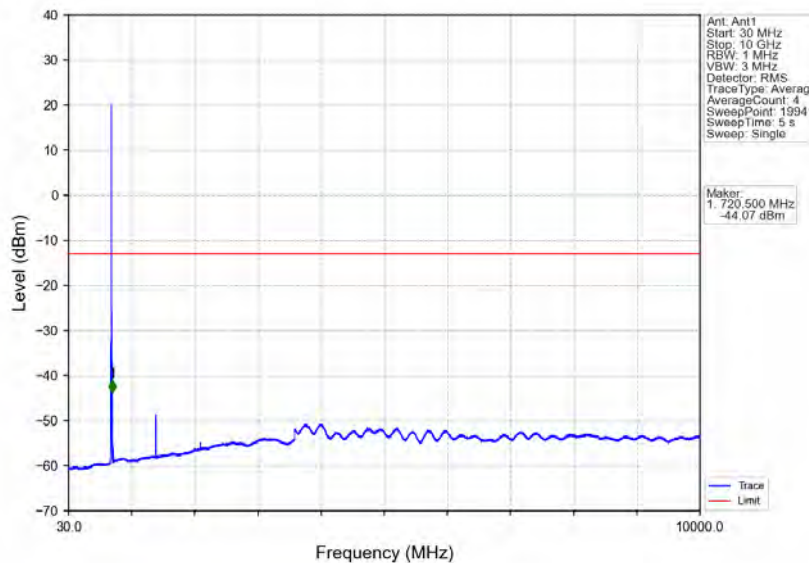
Band17_5MHz_64QAM_LCH_706.5MHz_RB_1_0_NTNV
