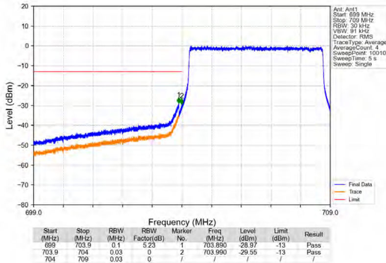
Band17_5MHz_64QAM_LCH_706.5MHz_RB_25_0_NTNV
