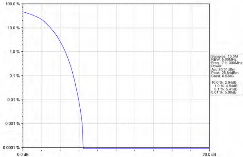
Band17_10MHz_QPSK_HCH_711MHz_RB_50_0_NTNV
