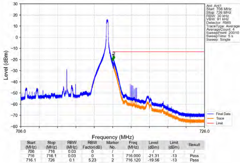
Band17_10MHz_QPSK_HCH_711MHz_RB_1_49_NTNV
