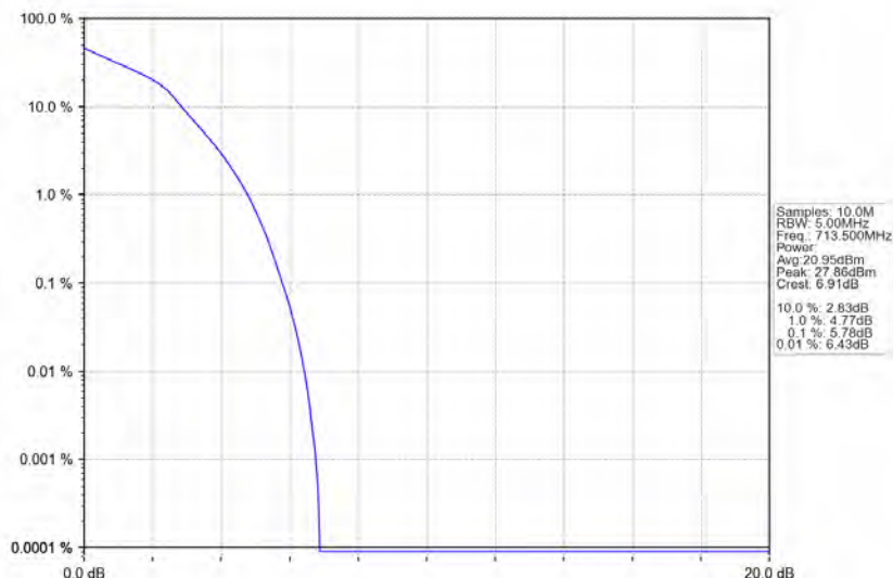
Band17_5MHz_16QAM_HCH_713.5MHz_RB_25_0_NTNV
