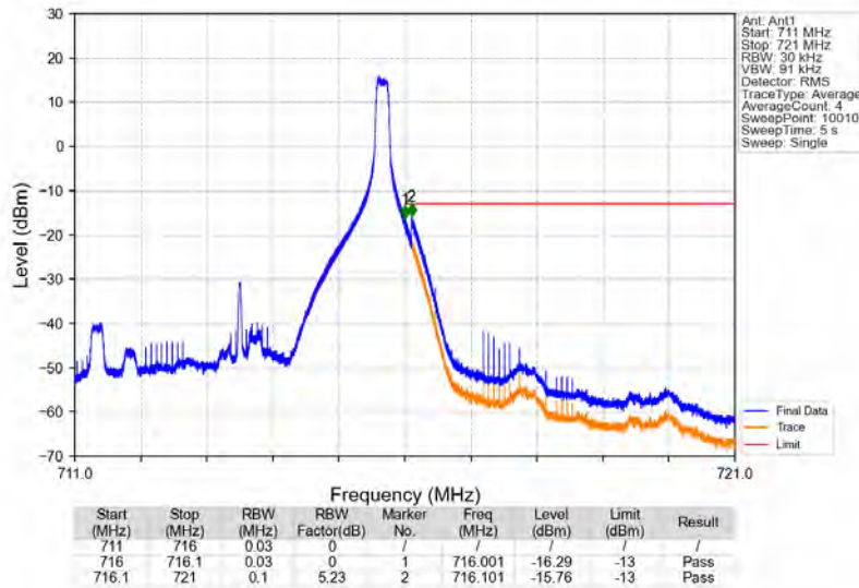
Band17_5MHz_QPSK_HCH_713.5MHz_RB_1_24_NTNV
