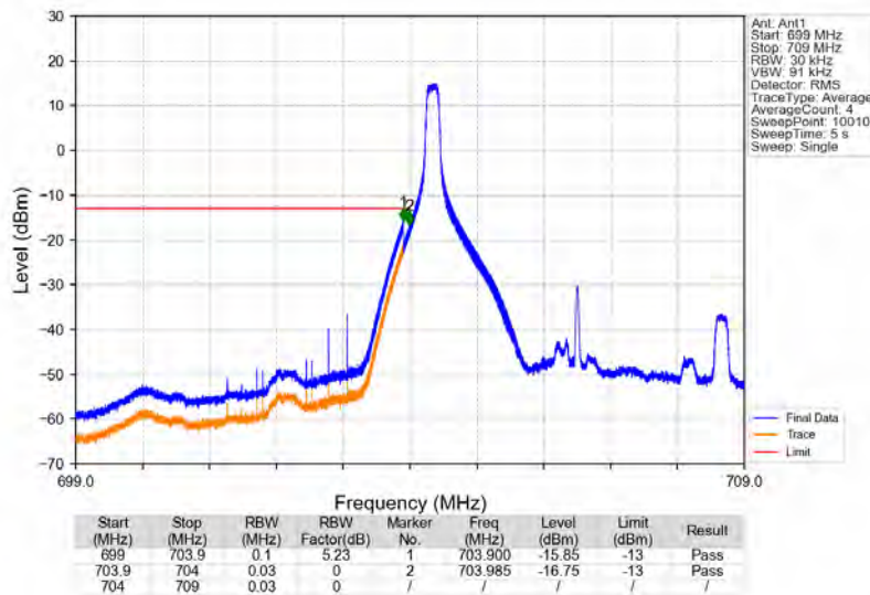
Band17_5MHz_16QAM_LCH_706.5MHz_RB_1_0_NTNV
