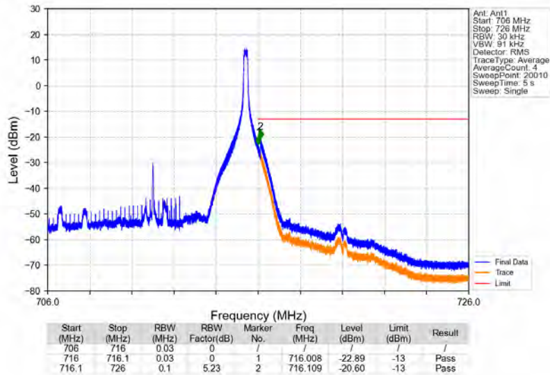
Band17_10MHz_64QAM_HCH_711MHz_RB_1_49_NTNV
