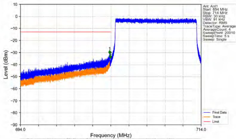
Band17_10MHz_16QAM_LCH_709MHz_RB_50_0_NTNV
