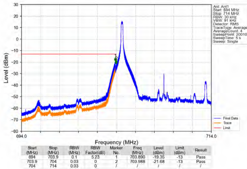
Band17_10MHz_16QAM_LCH_709MHz_RB_1_0_NTNV
