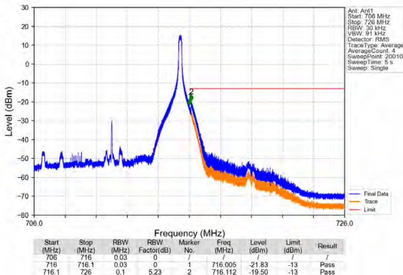
Band17_10MHz_16QAM_HCH_711MHz_RB_1_49_NTV
