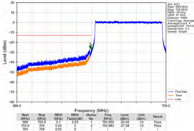
Band17_5MHz_QPSK_LCH_706.5MHz_RB_25_0_NTNV
