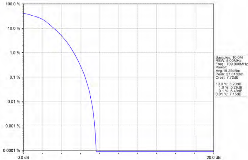
Band17_10MHz_16QAM_LCH_709MHz_RB_50_0_NTNV
