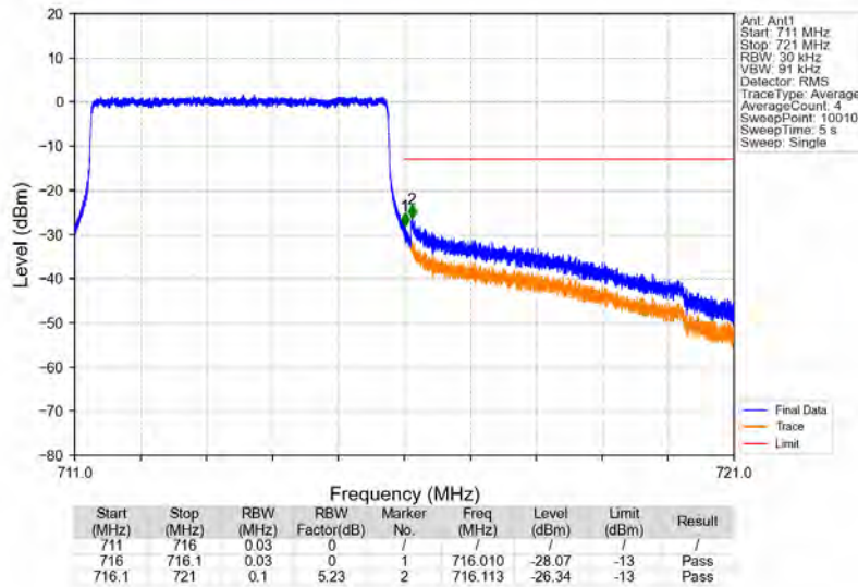
Band17_5MHz_QPSK_HCH_713.5MHz_RB_25_0_NTNV
