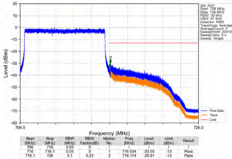
Band17_10MHz_QPSK_HCH_711MHz_RB_50_0_NTNV
