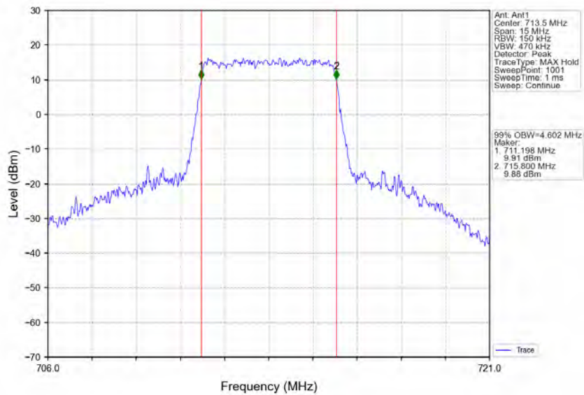
Band17_5MHz_16QAM_HCH_713.5MHz_RB_25_0_NTNV
