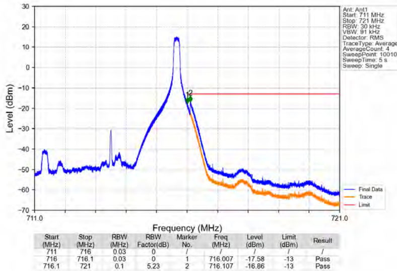
Band17_5MHz_16QAM_HCH_713.5MHz_RB_1_24_NTNV
