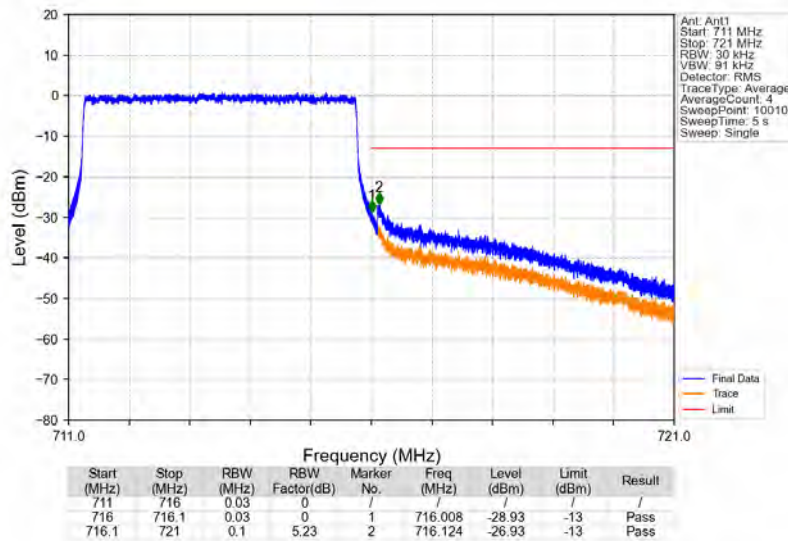
Band17_5MHz_16QAM_HCH_713.5MHz_RB_25_0_NTNV
