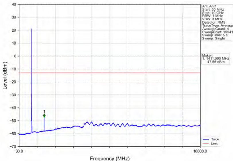
Band17_10MHz_16QAM_HCH_711MHz_RB_1_0_NTNV
