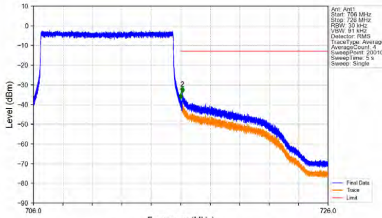
Band17_10MHz_64QAM_HCH_711MHz_RB_50_0_NTNV
