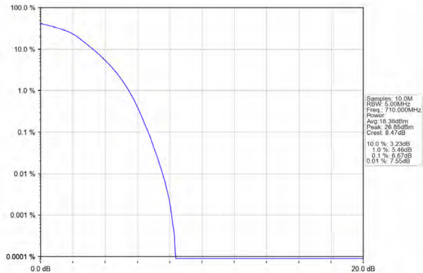
Band17_10MHz_64QAM_MCH_710MHz_RB_50_0_NTNV
