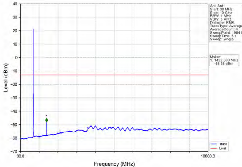
Band17_5MHz_16QAM_HCH_713.5MHz_RB_1_0_NTNV
