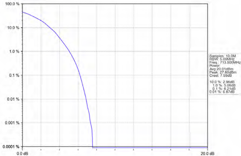
Band17_5MHz_64QAM_HCH_713.5MHz_RB_25_0_NTNV
