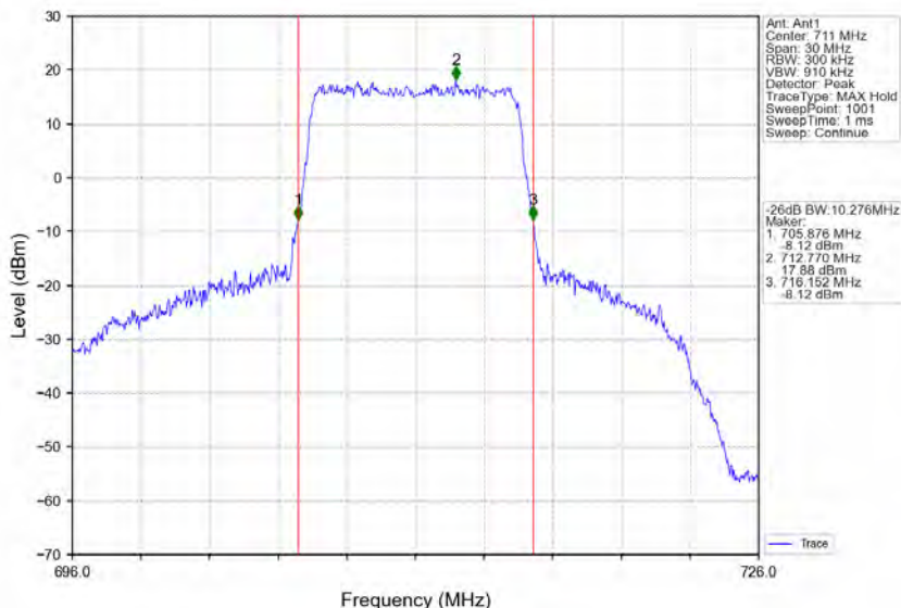
Band17_10MHz_QPSK_HCH_711MHz_RB_50_0_NTNV
