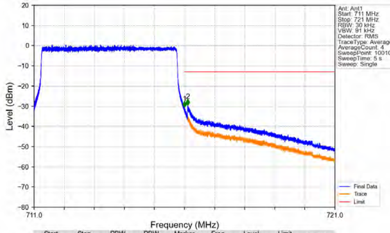
Band17_5MHz_64QAM_HCH_713.5MHz_RB_25_0_NTNV
