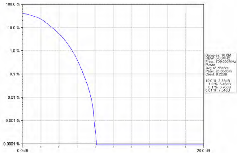
Band17_10MHz_64QAM_LCH_709MHz_RB_50_0_NTNV
