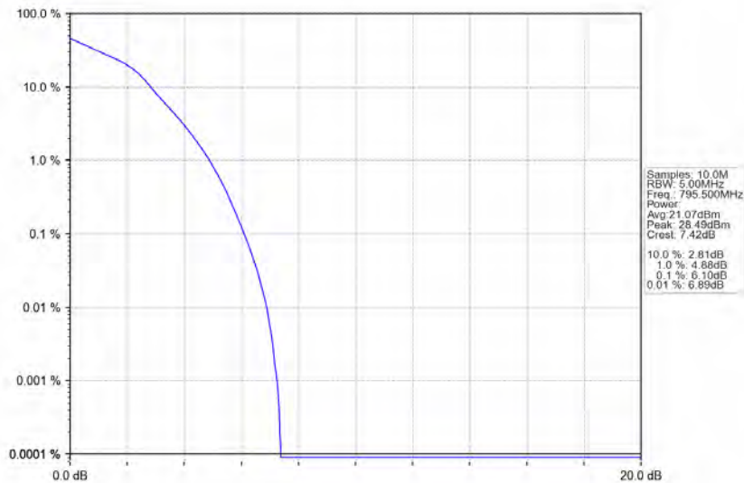
Band14_5MHz_16QAM_HCH_795.5MHz_RB_25_0_NTNV
