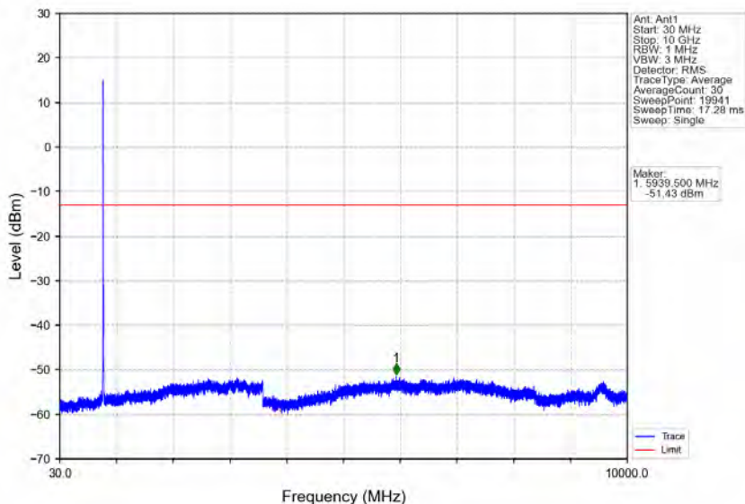
Band14_10MHz_16QAM_LCH_793MHz_RB_50_0_NTNV
