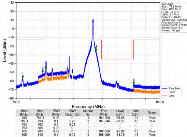
Band14_10MHz_16QAM_HCH_793MHz_RB_50_0_NTV
