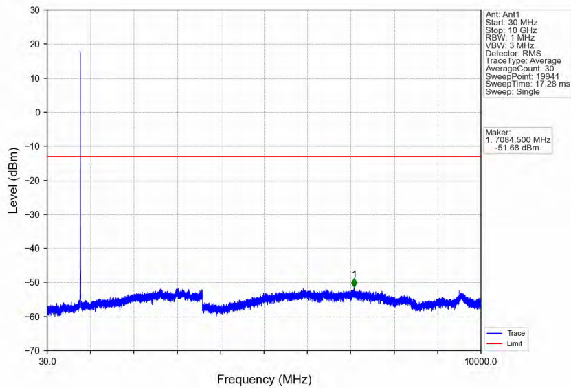
Band14_5MHz_QPSK_HCH_795.5MHz_RB_1_24_NTNV
