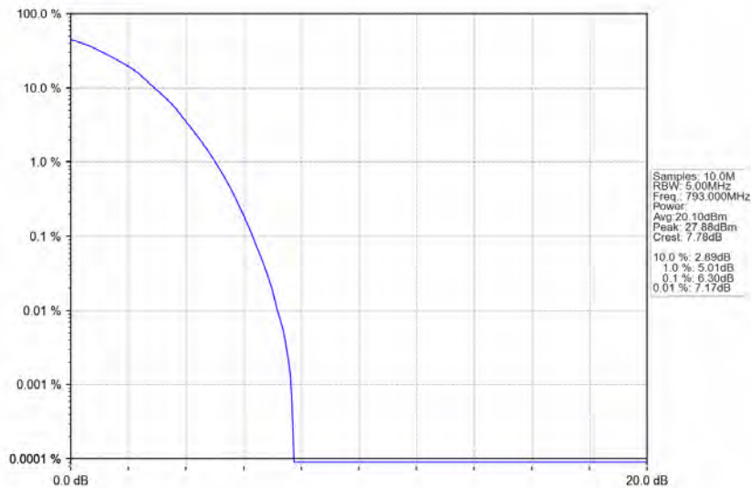
Band14_5MHz_64QAM_MCH_793MHz_RB_25_0_NTNV
