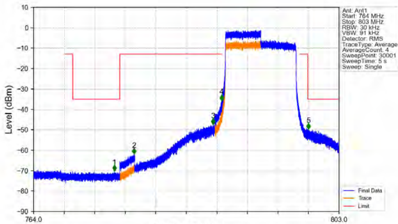
Band14_10MHz_16QAM_LCH_793MHz_RB_50_0_NTNV
