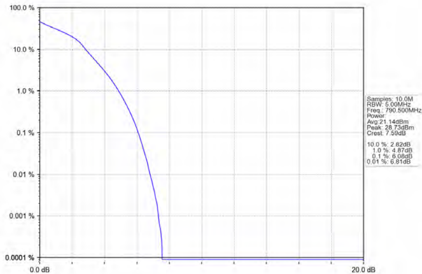
Band14_5MHz_16QAM_LCH_790.5MHz_RB_25_0_NTNV
