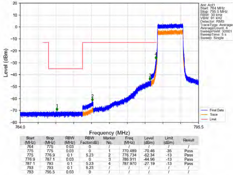
Band14_5MHz_QPSK_MCH_793MHz_RB_1_0_NTNV
