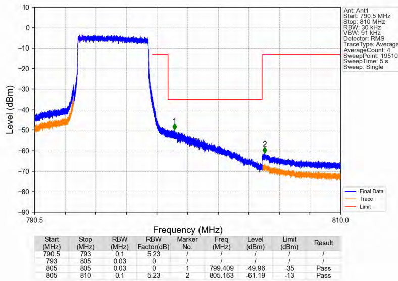
Band14_5MHz_16QAM_HCH_795.5MHz_RB_25_0_NTNV
