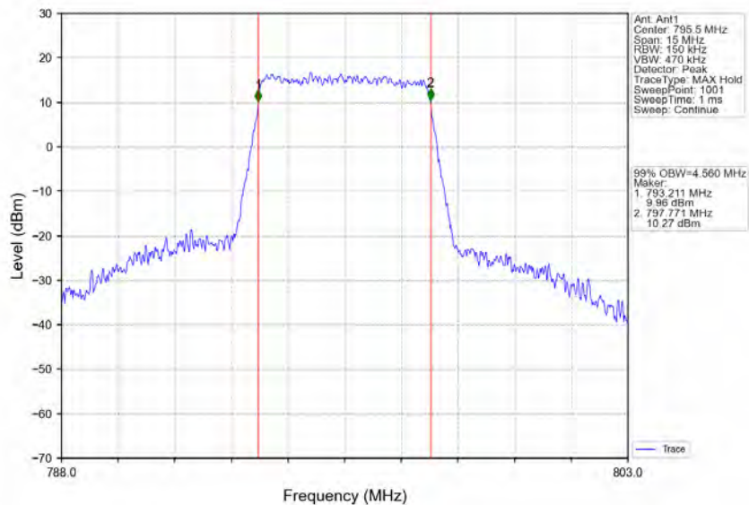
Band14_5MHz_16QAM_HCH_795.5MHz_RB_25_0_NTNV
