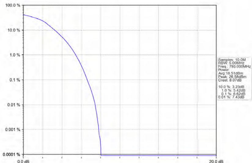
Band14_10MHz_64QAM_MCH_793MHz_RB_50_0_NTNV
