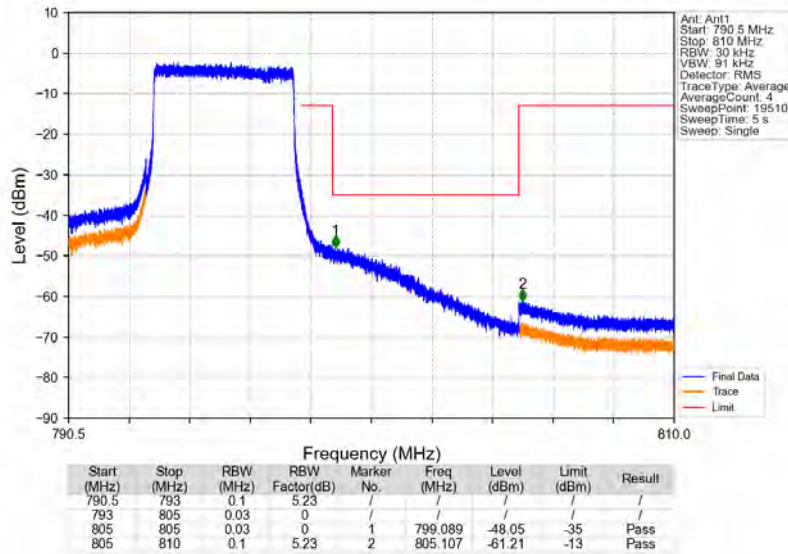
Band14_5MHz_16QAM_LCH_790.5MHz_RB_1_0_NTNV
