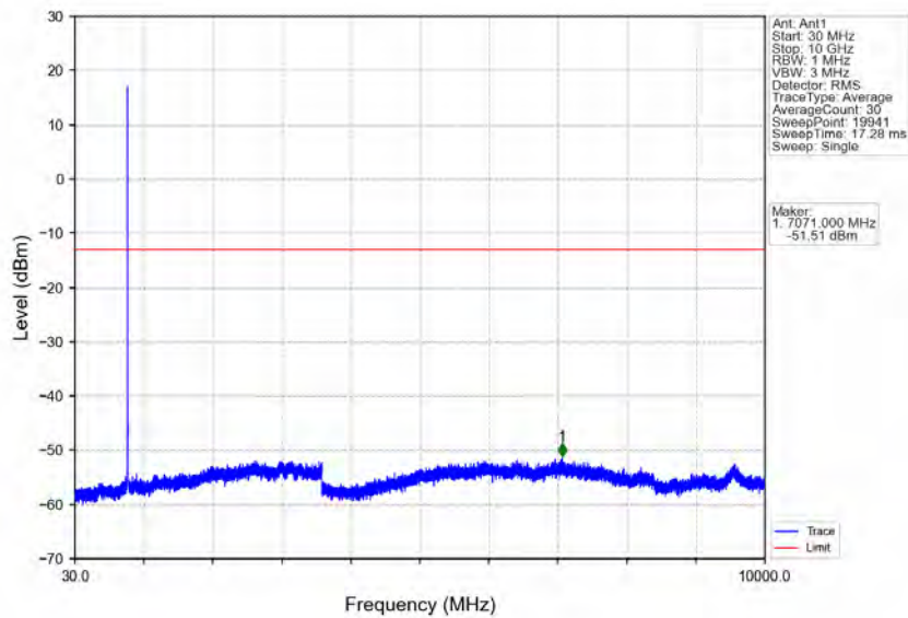
Band14_5MHz_16QAM_LCH_790.5MHz_RB_25_0_NTNV
