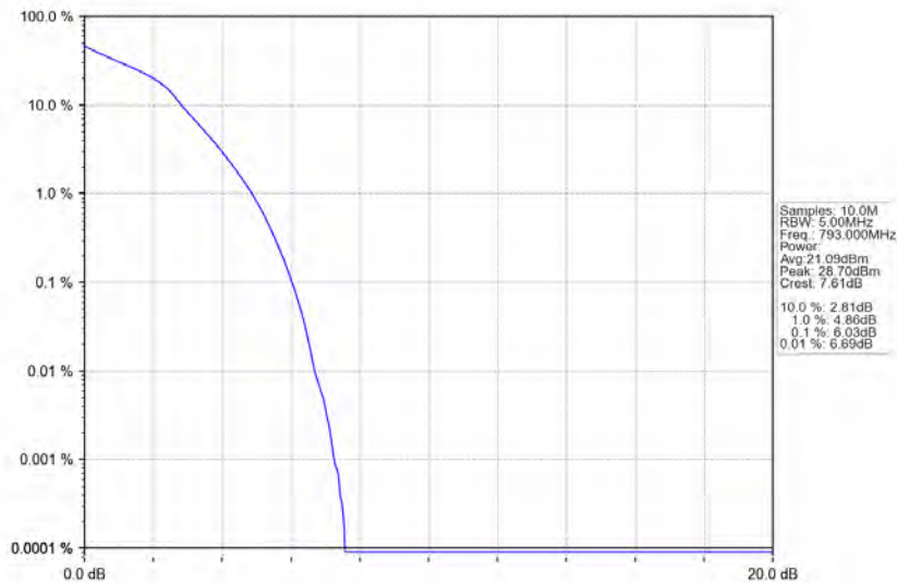
Band14_5MHz_16QAM_MCH_793MHz_RB_25_0_NTNV
