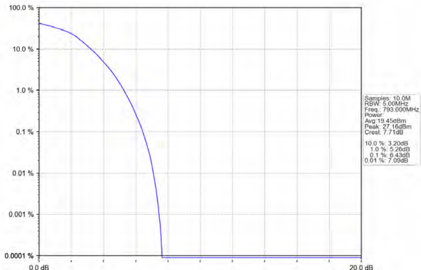
Band14_10MHz_16QAM_HCH_793MHz_RB_50_0_NTNV
