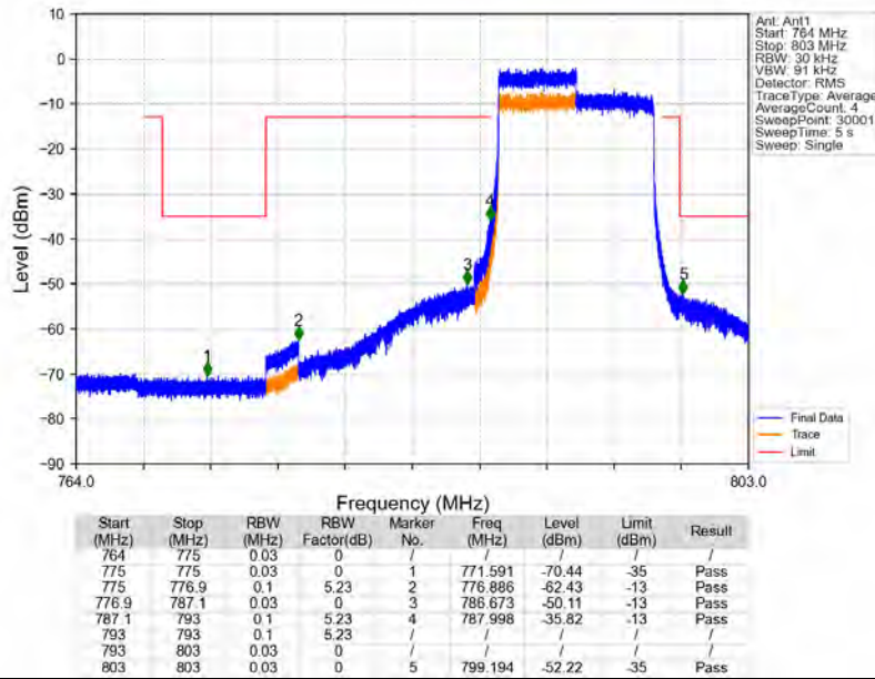
Band14_10MHz_64QAM_MCH_793MHz_RB_1_0_NTNV
