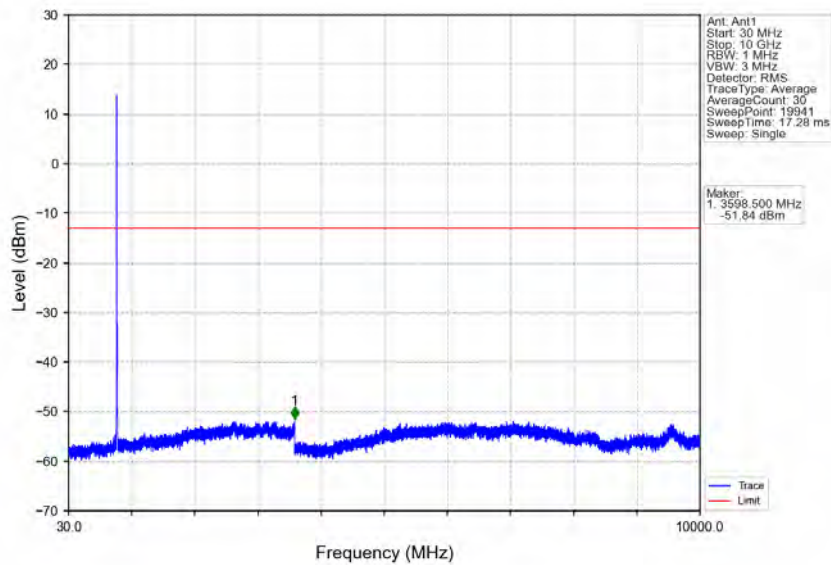
Band14_10MHz_64QAM_MCH_793MHz_RB_1_0_NTNV
