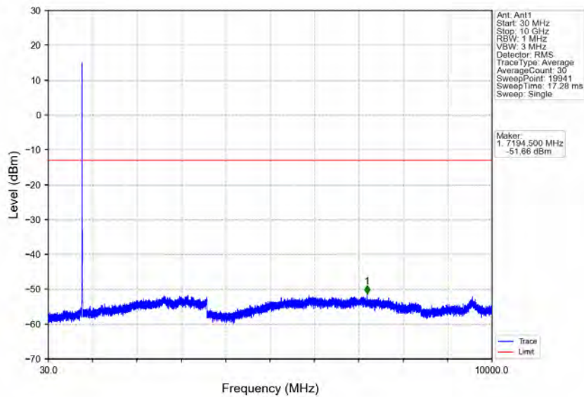
Band14_10MHz_64QAM_HCH_793MHz_RB_1_49_NTNV
