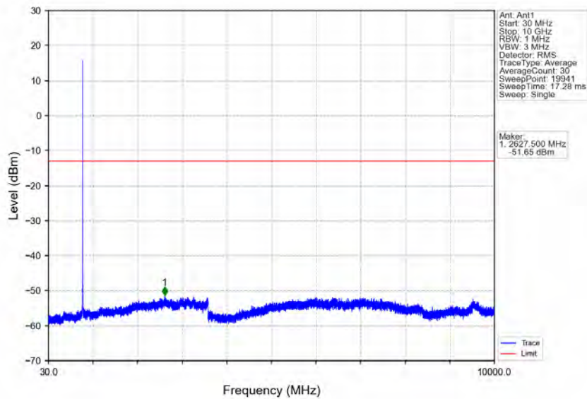
Band14_5MHz_64QAM_HCH_795.5MHz_RB_1_24_NTNV
