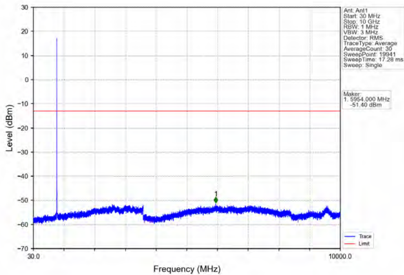
Band14_5MHz_16QAM_HCH_795.5MHz_RB_1_0_NTNV
