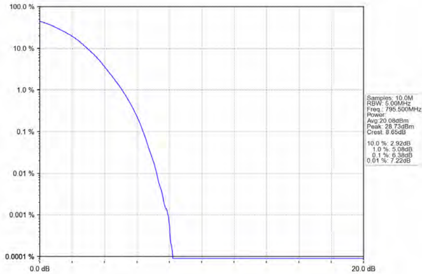
Band14_5MHz_64QAM_HCH_795.5MHz_RB_25_0_NTNV
