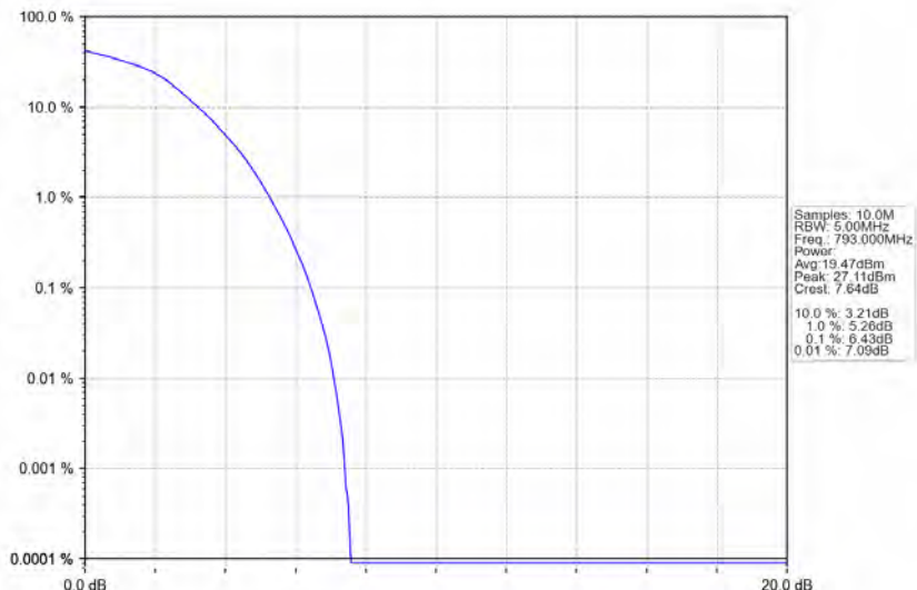
Band14_10MHz_16QAM_MCH_793MHz_RB_50_0_NTNV
