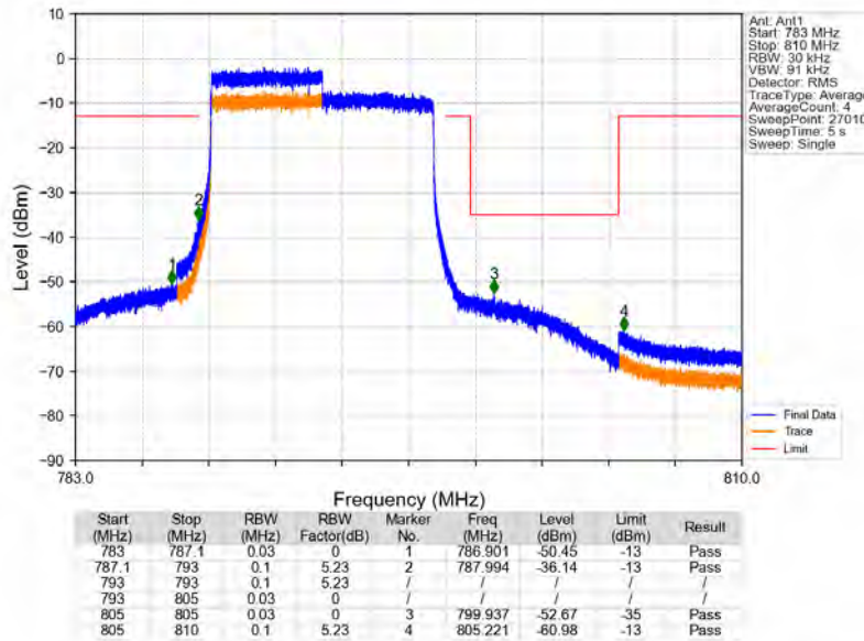
Band14_10MHz_64QAM_HCH_793MHz_RB_50_0_NTV
