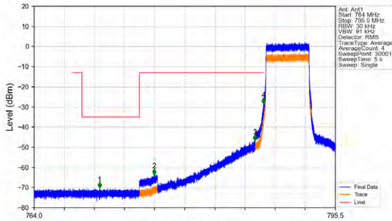
Band14_5MHz_16QAM_LCH_790.5MHz_RB_25_0_NTNV
