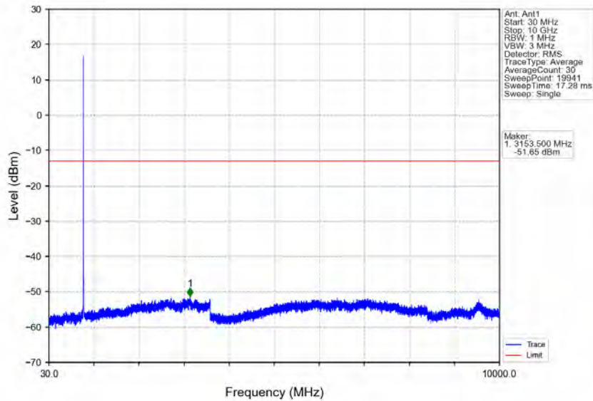
Band14_5MHz_QPSK_MCH_793MHz_RB_1_0_NTNV
