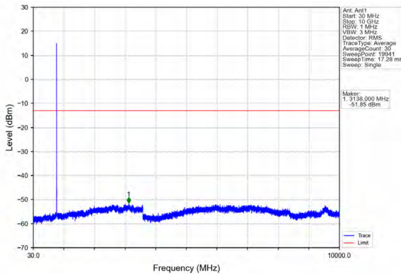
Band14_5MHz_64QAM_LCH_790.5MHz_RB_1_0_NTNV
