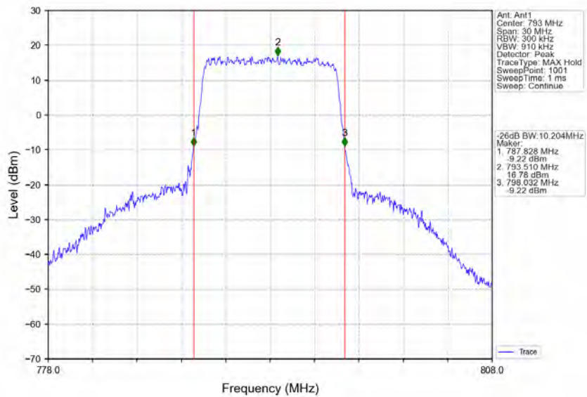
Band14_10MHz_64QAM_LCH_793MHz_RB_50_0_NTNV
