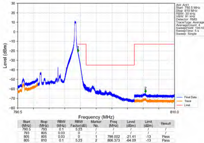
Band14_5MHz_QPSK_HCH_795.5MHz_RB_1_24_NTNV
