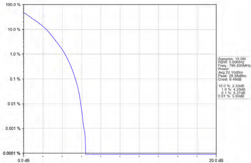
Band14_5MHz_QPSK_HCH_795.5MHz_RB_25_0_NTNV
