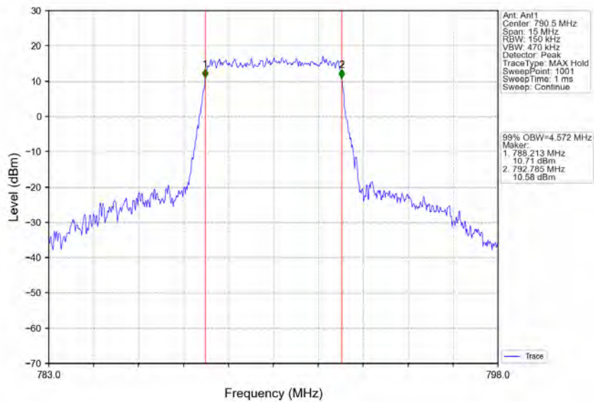
Band14_5MHz_16QAM_LCH_790.5MHz_RB_25_0_NTNV
