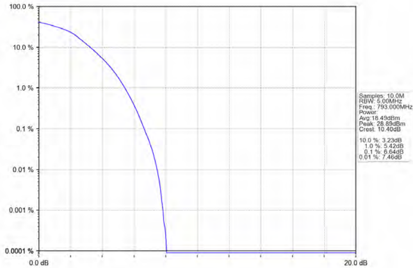
Band14_10MHz_64QAM_HCH_793MHz_RB_50_0_NTV
