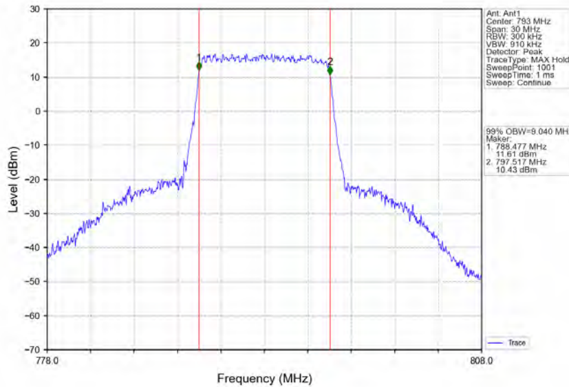
Band14_10MHz_64QAM_LCH_793MHz_RB_50_0_NTNV
