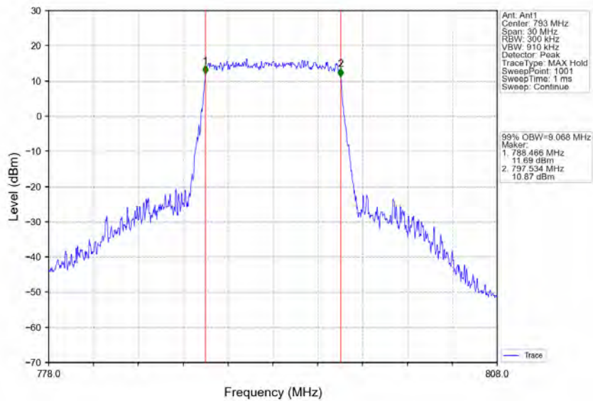
Band14_10MHz_64QAM_HCH_793MHz_RB_50_0_NTNV
