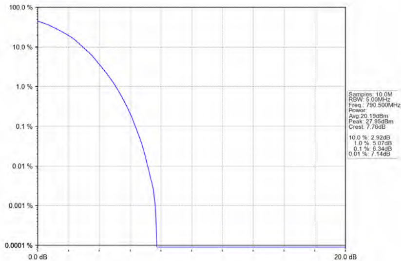
Band14_5MHz_64QAM_LCH_790.5MHz_RB_25_0_NTNV
