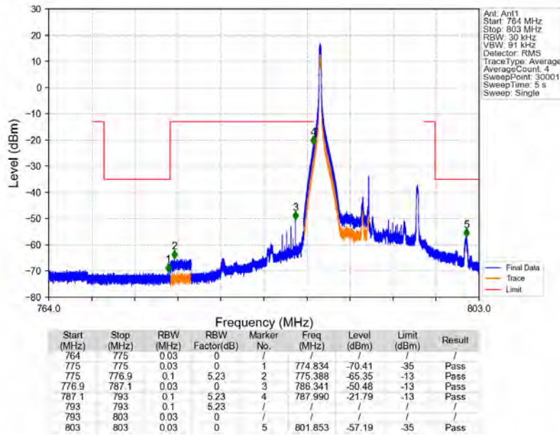
Band14_10MHz_16QAM_LCH_793MHz_RB_1_0_NTNV
