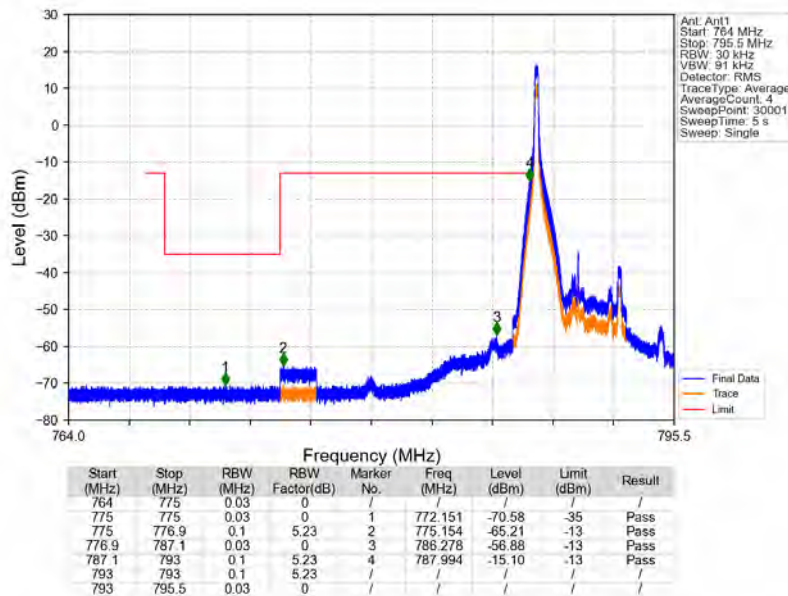
Band14_5MHz_16QAM_LCH_790.5MHz_RB_1_0_NTNV
