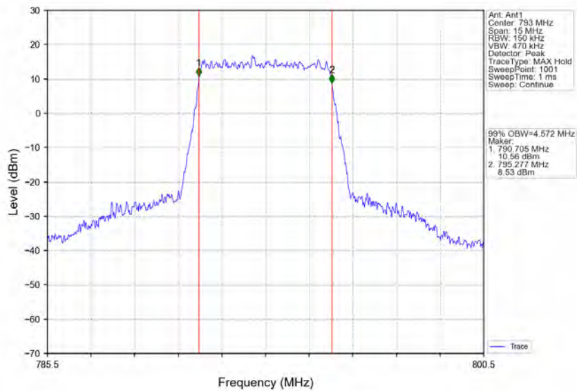
Band14_5MHz_64QAM_MCH_793MHz_RB_25_0_NTNV
