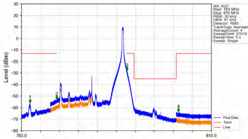
Band14_10MHz_64QAM_HCH_793MHz_RB_1_49_NTNV
