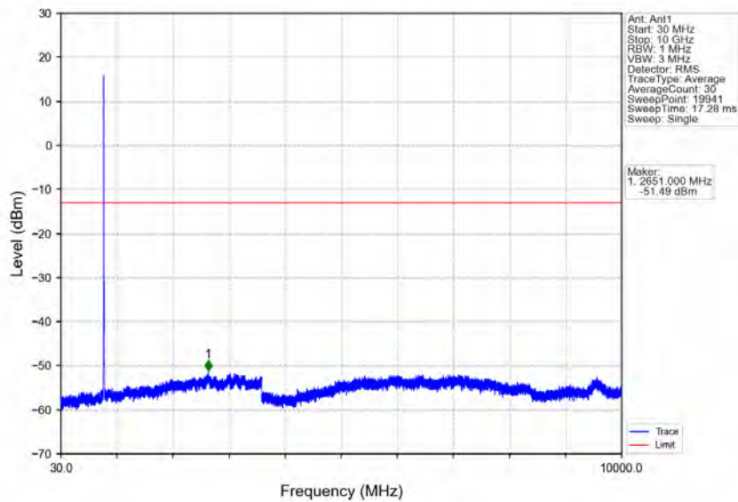
Band14_10MHz_16QAM_HCH_793MHz_RB_1_0_NTNV
