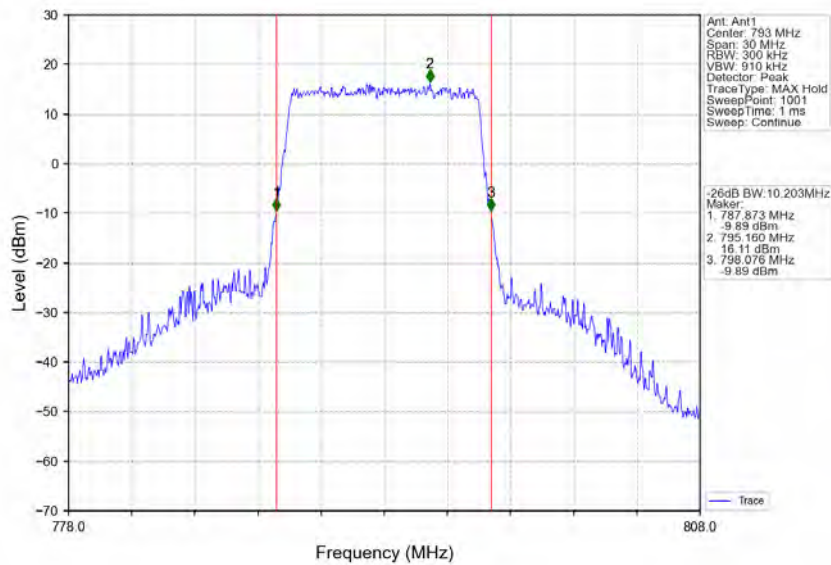
Band14_10MHz_64QAM_HCH_793MHz_RB_50_0_NTNV
