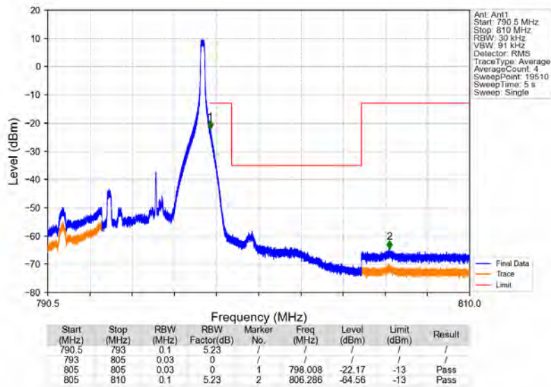
Band14_5MHz_64QAM_HCH_795.5MHz_RB_1_24_NTNV
