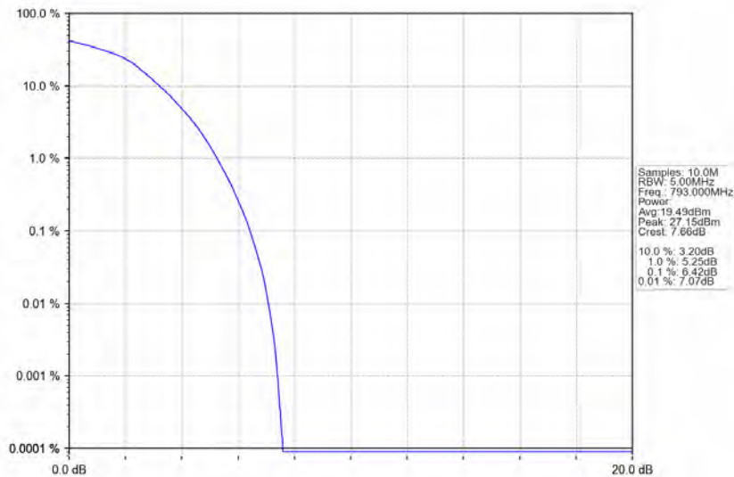
Band14_10MHz_16QAM_LCH_793MHz_RB_50_0_NTNV
