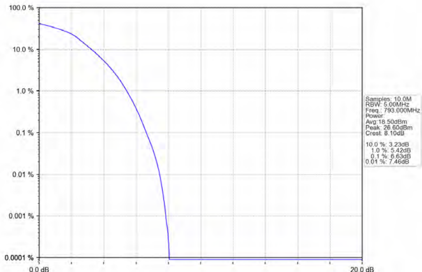
Band14_10MHz_64QAM_LCH_793MHz_RB_50_0_NTNV
