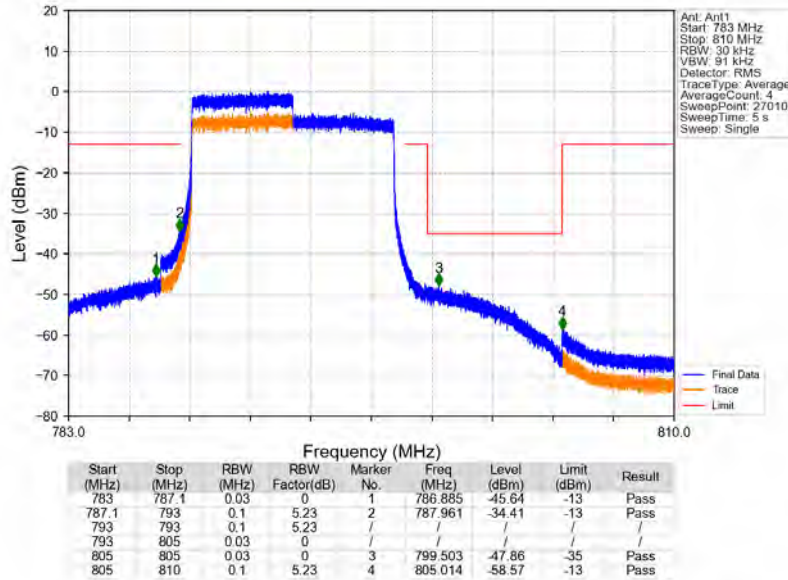
Band14_10MHz_16QAM_LCH_793MHz_RB_1_0_NTNV
