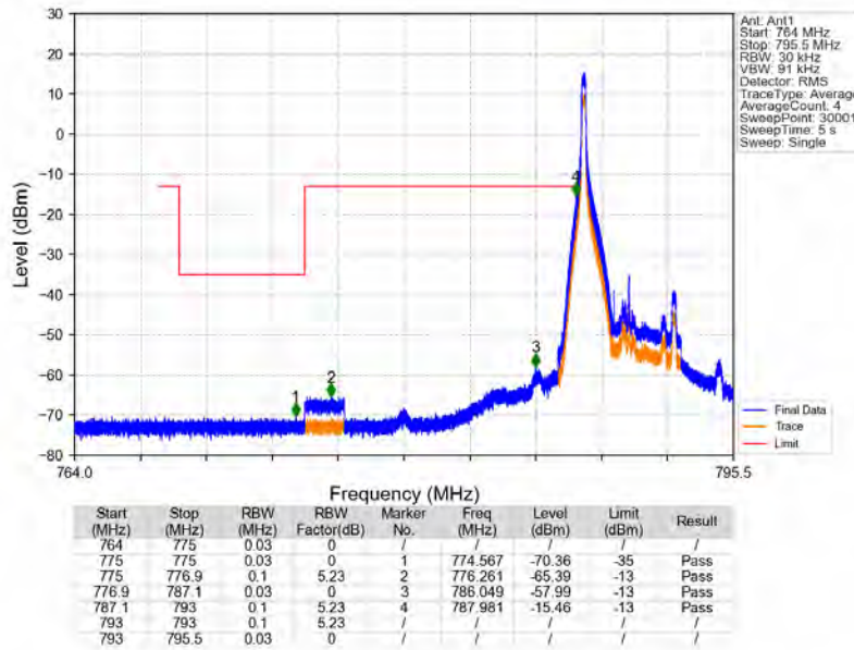
Band14_5MHz_64QAM_LCH_790.5MHz_RB_1_0_NTNV
