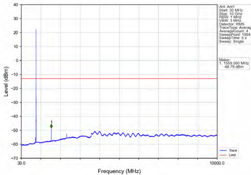
Band13_5MHz_QPSK_MCH_782MHz_RB_1_0_NTNV
