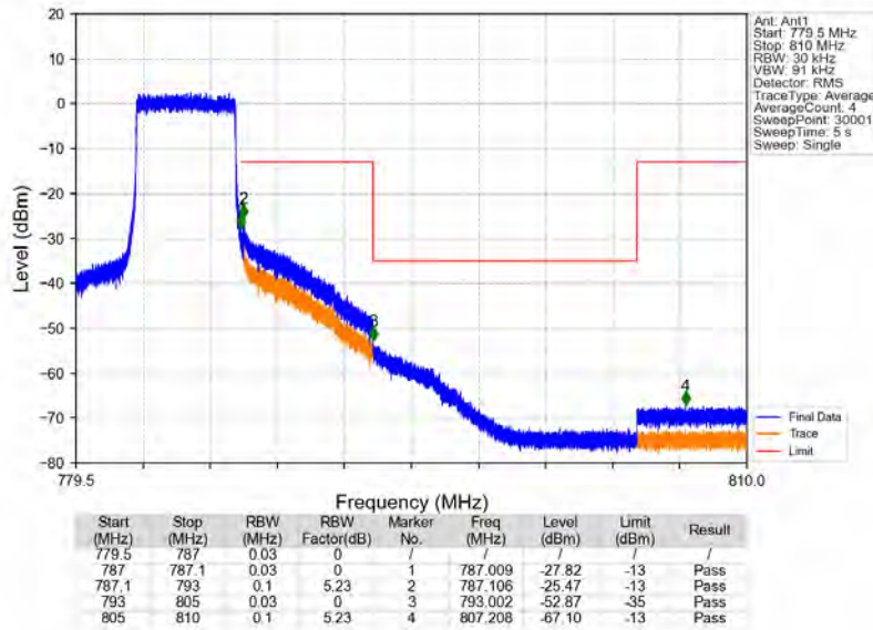
Band13_5MHz_16QAM_LCH_779.5MHz_RB_1_0_NTNV
