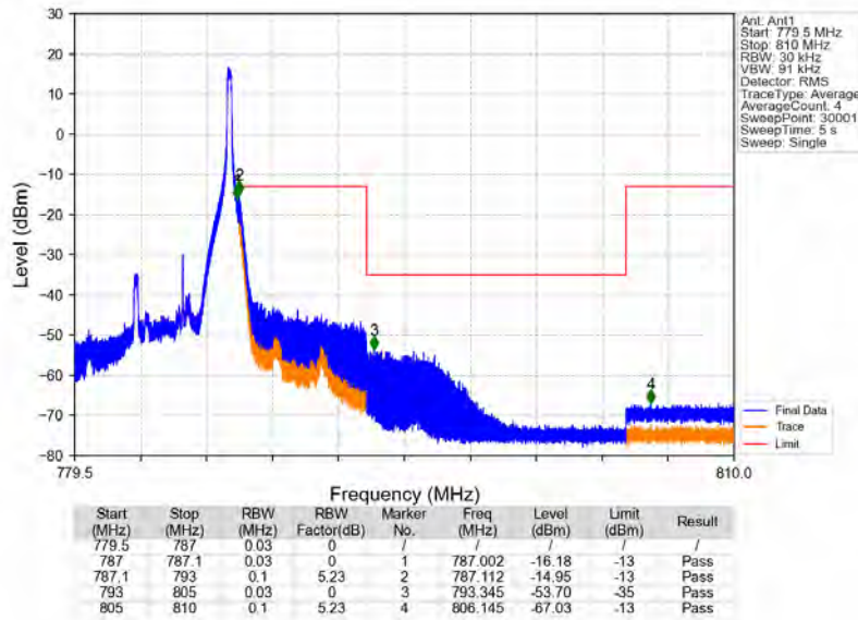
Band13_5MHz_QPSK_HCH_784.5MHz_RB_1_24_NTNV
