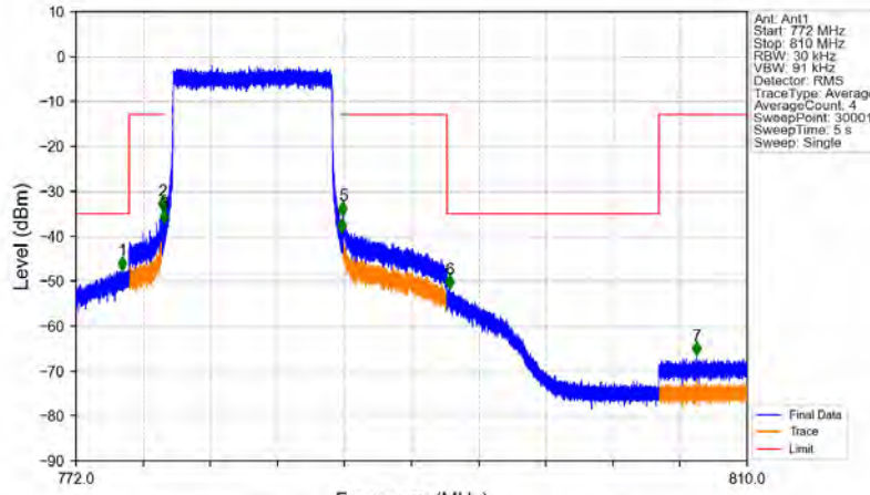
Band13_10MHz_64QAM_HCH_782MHz_RB_50_0_NTNV
