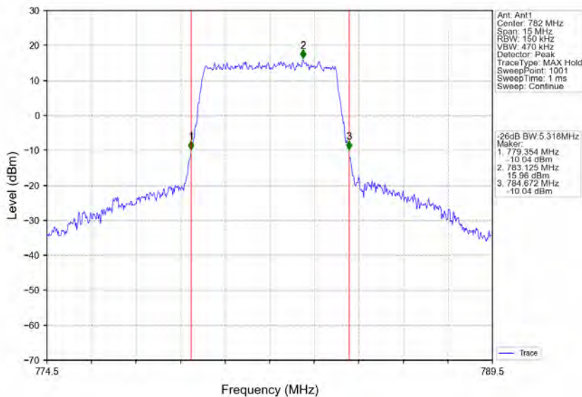
Band13_5MHz_64QAM_MCH_782MHz_RB_25_0_NTNV
