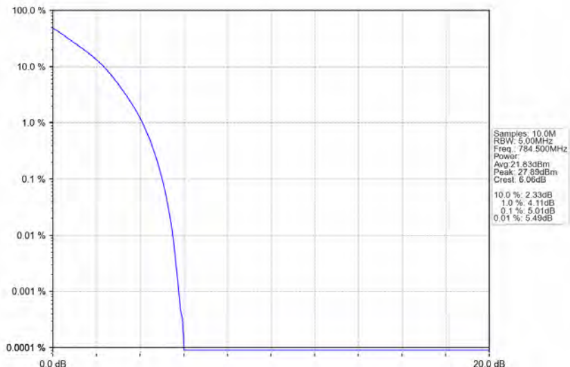
Band13_5MHz_QPSK_HCH_784.5MHz_RB_25_0_NTNV
