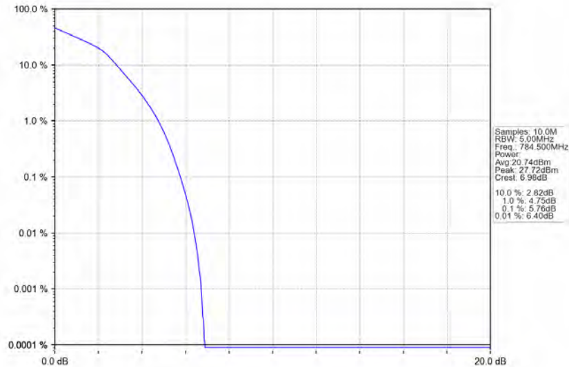
Band13_5MHz_16QAM_HCH_784.5MHz_RB_25_0_NTNV
