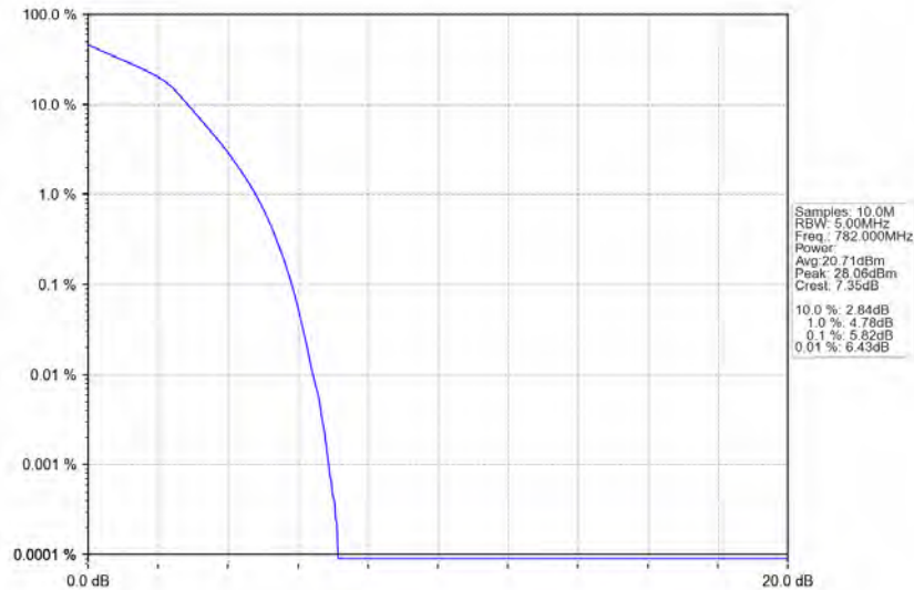
Band13_5MHz_16QAM_MCH_782MHz_RB_25_0_NTNV
