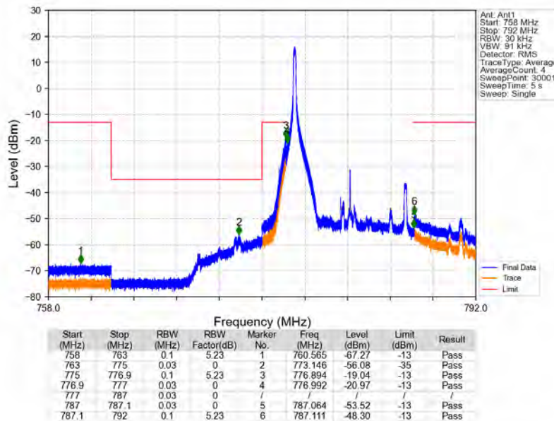
Band13_10MHz_16QAM_LCH_782MHz_RB_1_0_NTNV
