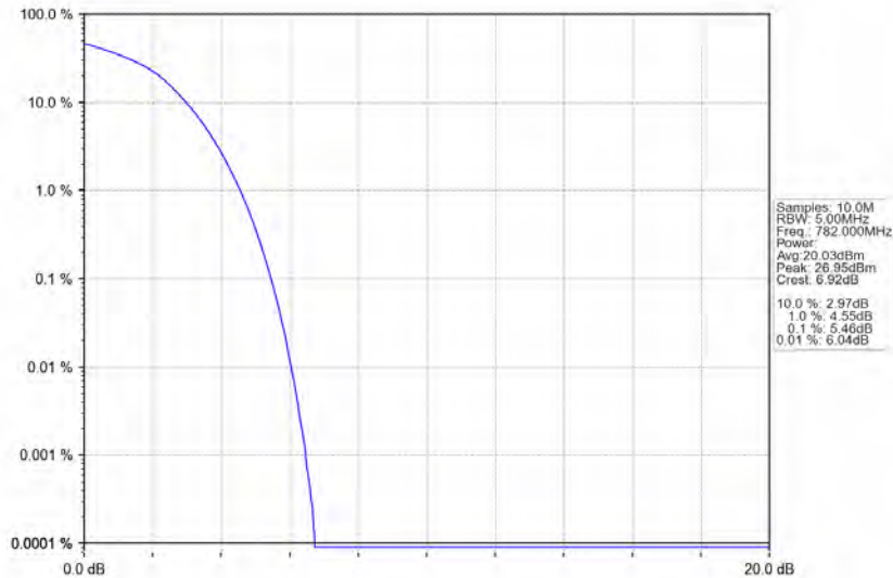
Band13_10MHz_QPSK_HCH_782MHz_RB_50_0_NTNV
