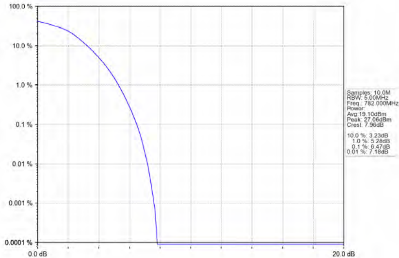
Band13_10MHz_16QAM_LCH_782MHz_RB_50_0_NTNV
