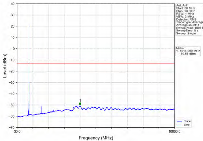
Band13_10MHz_64QAM_LCH_782MHz_RB_1_0_NTV
