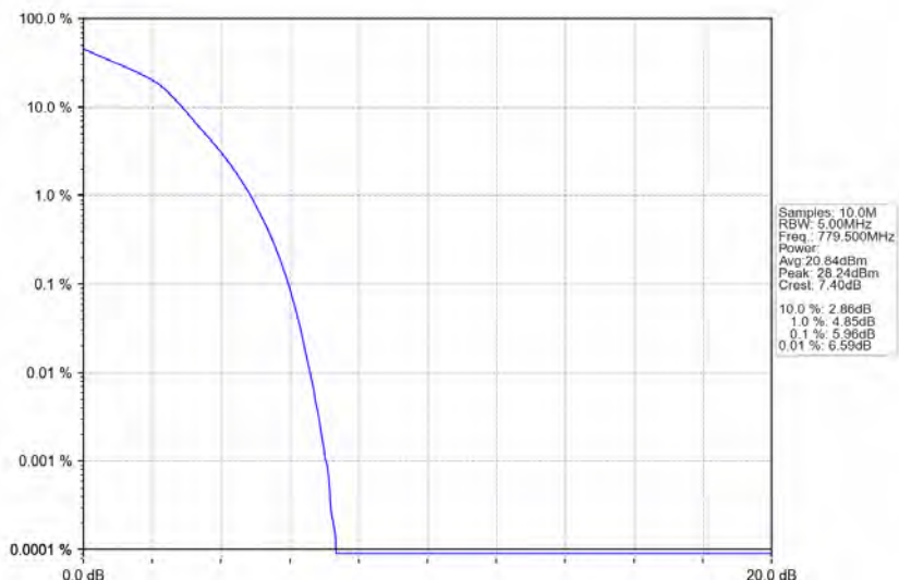
Band13_5MHz_16QAM_LCH_779.5MHz_RB_25_0_NTNV
