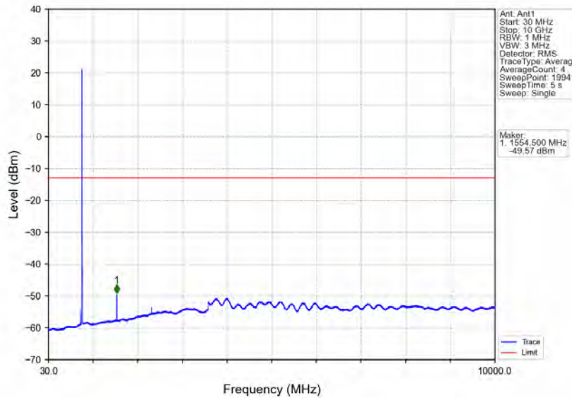
Band13_5MHz_16QAM_LCH_779.5MHz_RB_25_0_NTNV
