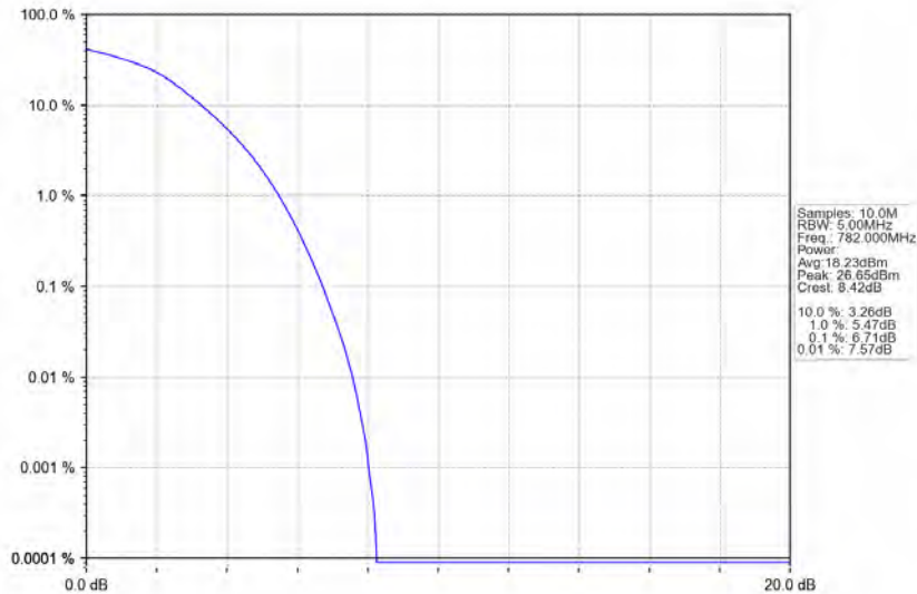
Band13_10MHz_64QAM_MCH_782MHz_RB_50_0_NTNV
