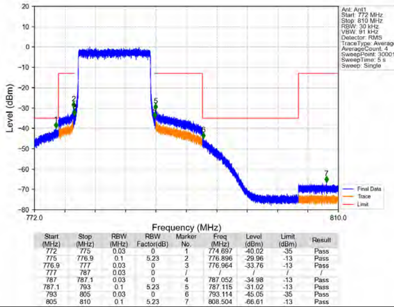
Band13_10MHz_16QAM_LCH_782MHz_RB_1_0_NTNV
