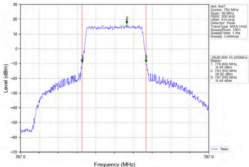
Band13_10MHz_64QAM_HCH_782MHz_RB_50_0_NTNV
