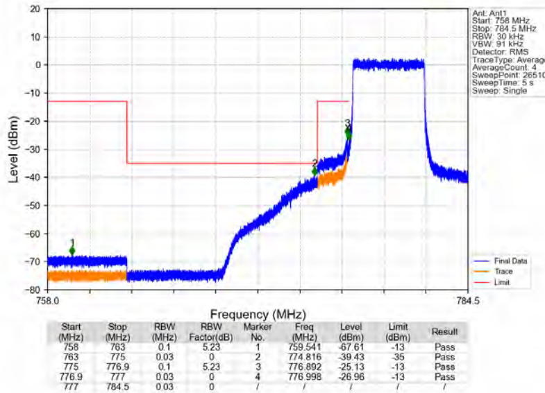
Band13_5MHz_QPSK_MCH_782MHz_RB_1_0_NTNV
