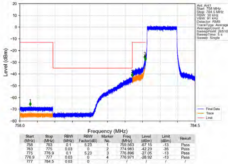
Band13_5MHz_16QAM_LCH_779.5MHz_RB_25_0_NTNV
