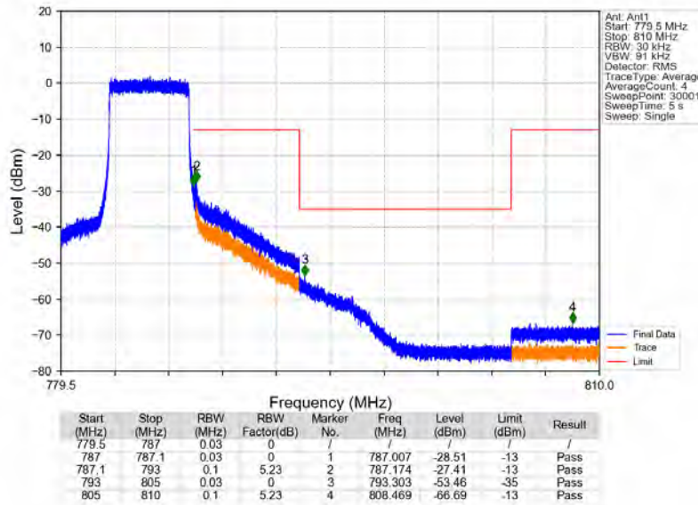
Band13_5MHz_16QAM_HCH_784.5MHz_RB_25_0_NTNV
