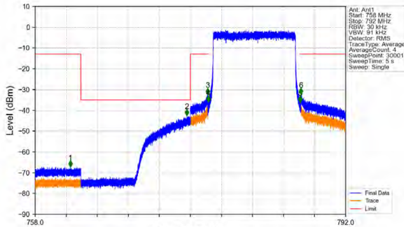
Band13_10MHz_16QAM_LCH_782MHz_RB_50_0_NTNV
