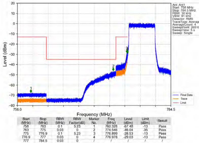
Band13_5MHz_64QAM_MCH_782MHz_RB_1_0_NTNV
