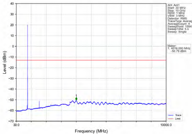
Band13_5MHz_64QAM_MCH_782MHz_RB_1_0_NTNV
