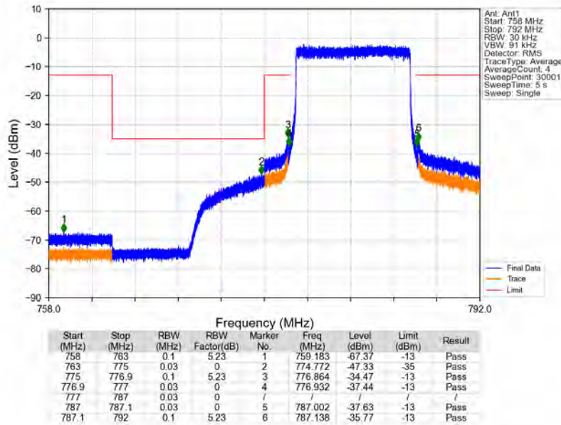
Band13_10MHz_64QAM_MCH_782MHz_RB_1_0_NTNV
