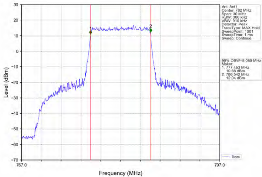
Band13_10MHz_64QAM_LCH_782MHz_RB_50_0_NTNV
