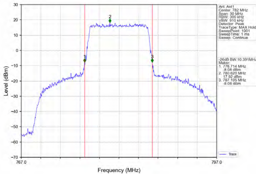
Band13_10MHz_QPSK_LCH_782MHz_RB_50_0_NTNV
