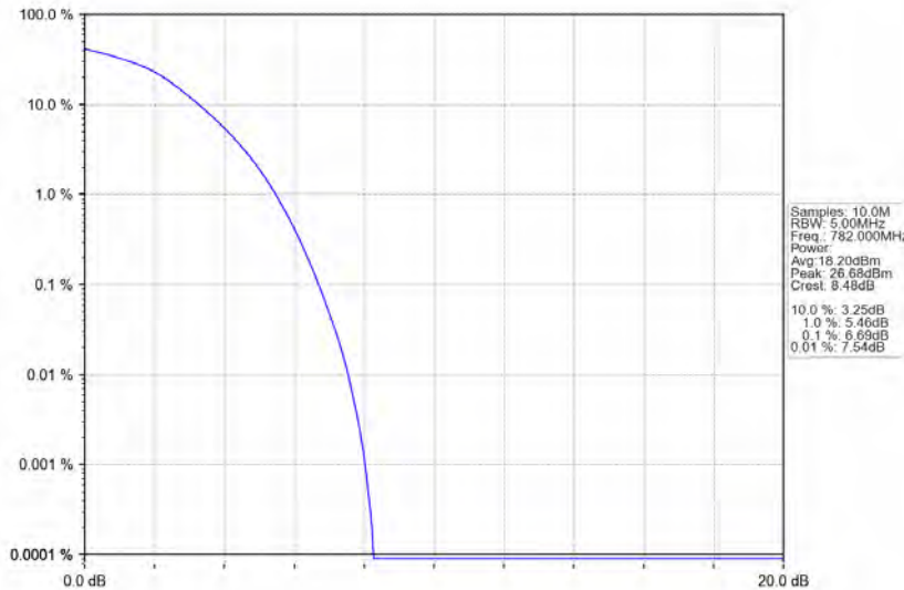
Band13_10MHz_64QAM_HCH_782MHz_RB_50_0_NTV
