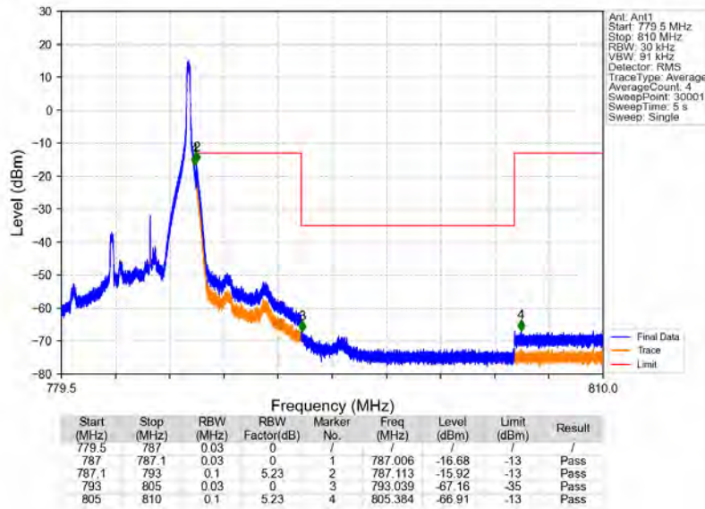
Band13_5MHz_64QAM_HCH_784.5MHz_RB_1_24_NTNV
