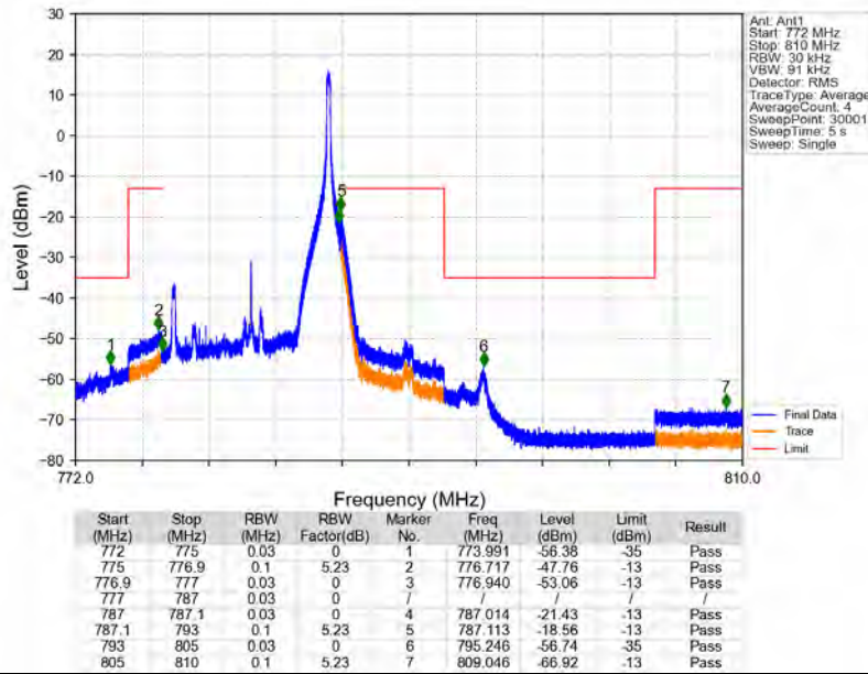
Band13_10MHz_16QAM_HCH_782MHz_RB_50_0_NTV
