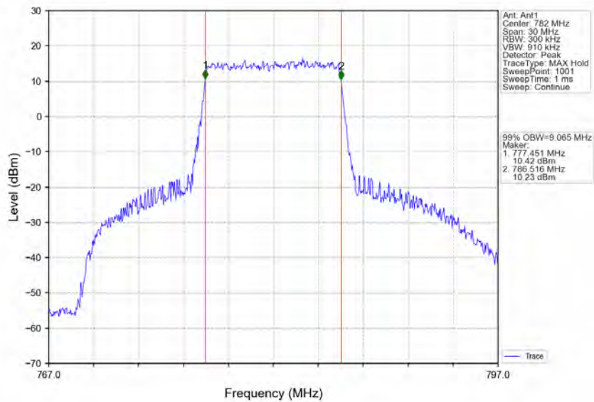
Band13_10MHz_64QAM_HCH_782MHz_RB_50_0_NTNV
