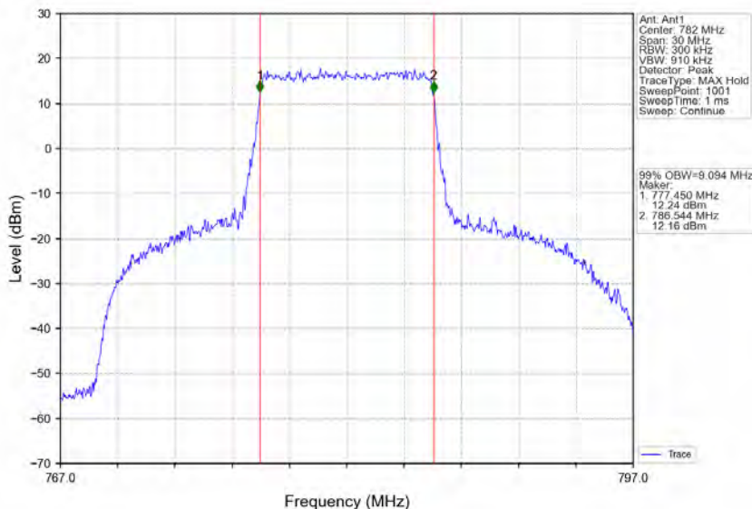
Band13_10MHz_QPSK_HCH_782MHz_RB_50_0_NTNV
