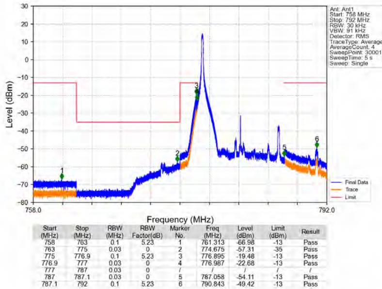
Band13_10MHz_64QAM_LCH_782MHz_RB_1_0_NTV
