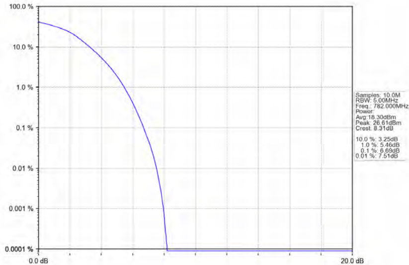
Band13_10MHz_64QAM_LCH_782MHz_RB_50_0_NTNV
