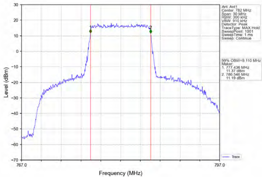
Band13_10MHz_QPSK_LCH_782MHz_RB_50_0_NTNV
