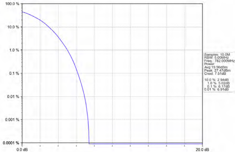
Band13_5MHz_64QAM_MCH_782MHz_RB_25_0_NTNV
