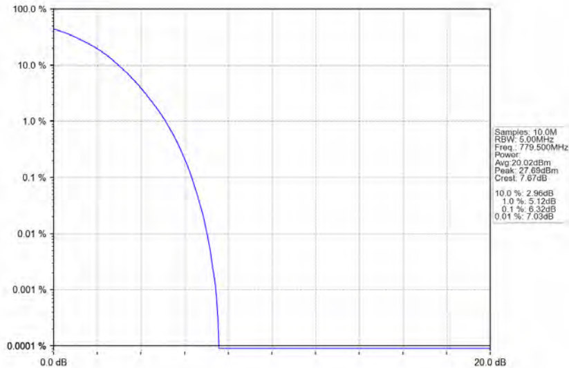
Band13_5MHz_64QAM_LCH_779.5MHz_RB_25_0_NTNV
