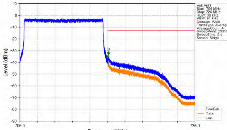
Band12_10MHz_64QAM_HCH_711MHz_RB_50_0_NTV
