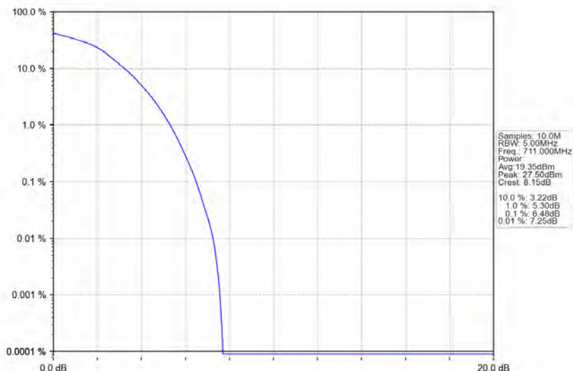
Band12_10MHz_16QAM_HCH_711MHz_RB_50_0_NTNV
