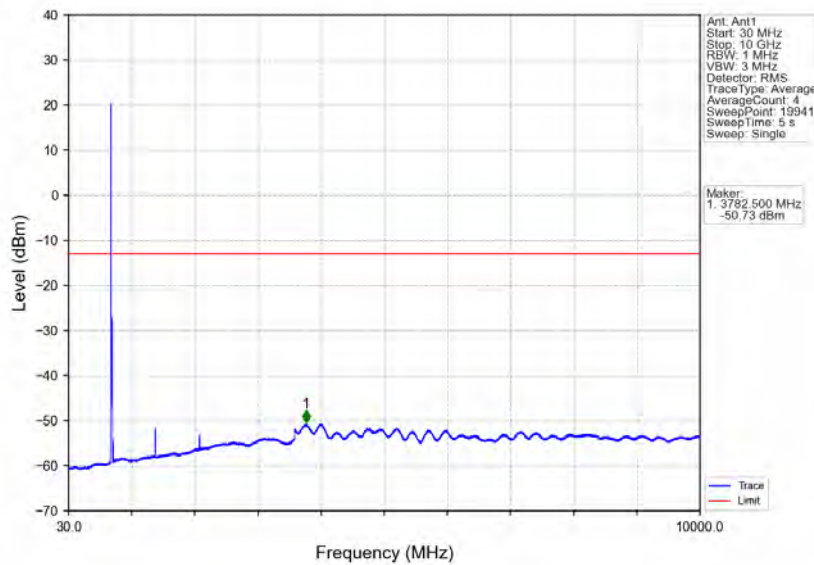
Band12_10MHz_64QAM_LCH_704MHz_RB_1_0_NTV
