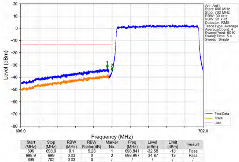
Band12_3MHz_16QAM_LCH_700.5MHz_RB_15_0_NTNV
