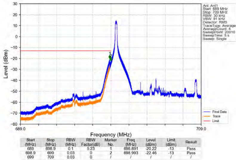
Band12_10MHz_64QAM_LCH_704MHz_RB_1_0_NTV
