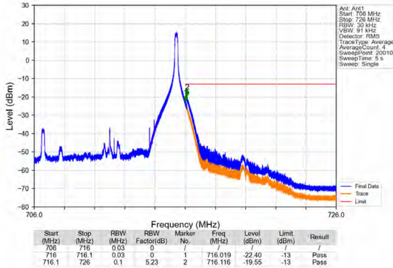
Band12_10MHz_16QAM_HCH_711MHz_RB_1_49_NTV
