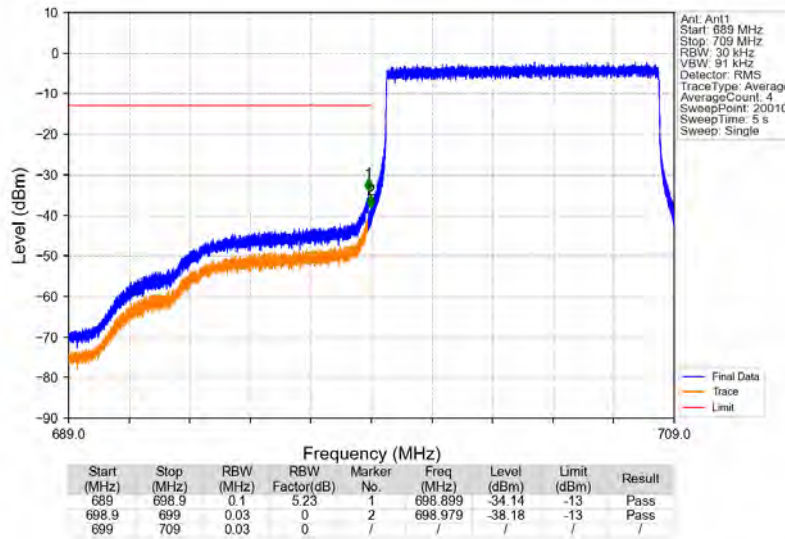
Band12_10MHz_64QAM_LCH_704MHz_RB_50_0_NTNV
