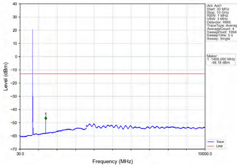
Band12_10MHz_64QAM_MCH_707.5MHz_RB_1_0_NTNV
