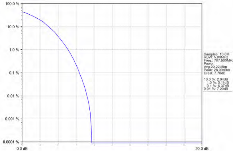
Band12_5MHz_64QAM_MCH_707.5MHz_RB_25_0_NTNV
