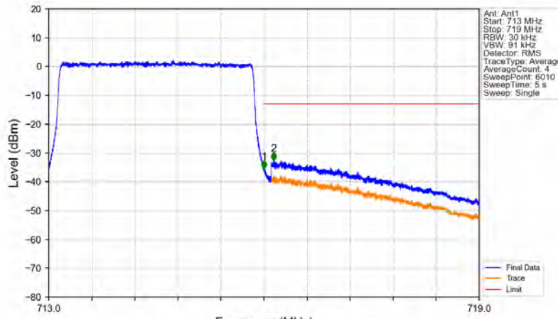
Band12_3MHz_64QAM_HCH_714.5MHz_RB_15_0_NTNV
