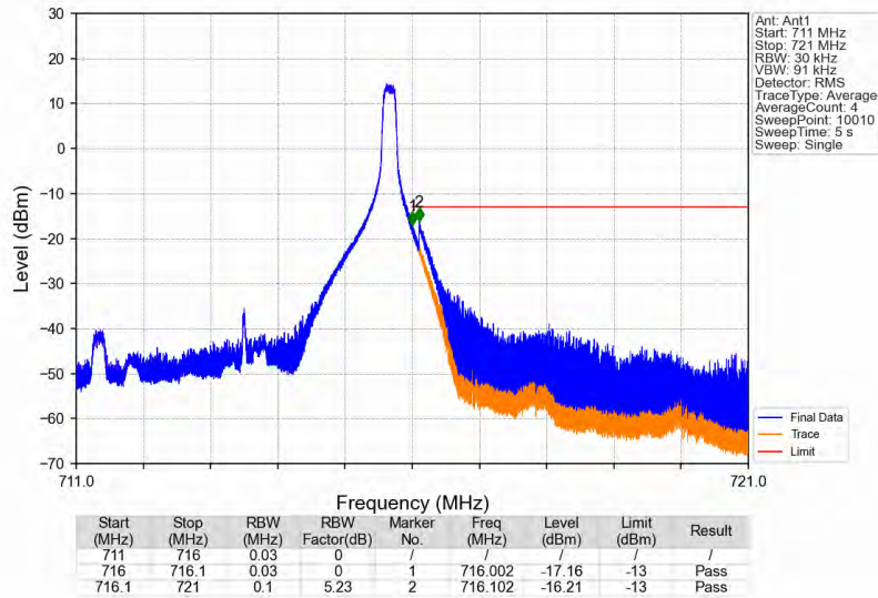
Band12_5MHz_64QAM_HCH_713.5MHz_RB_1_24_NTNV
