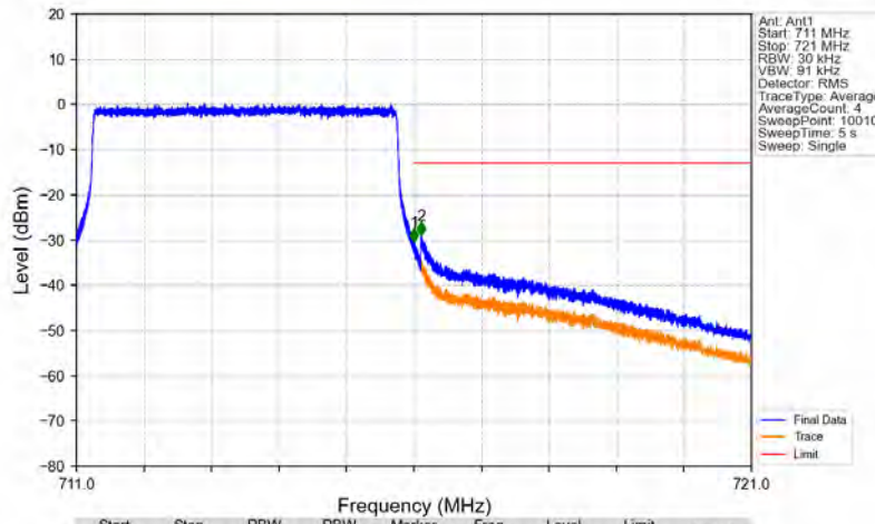
Band12_5MHz_64QAM_HCH_713.5MHz_RB_25_0_NTNV
