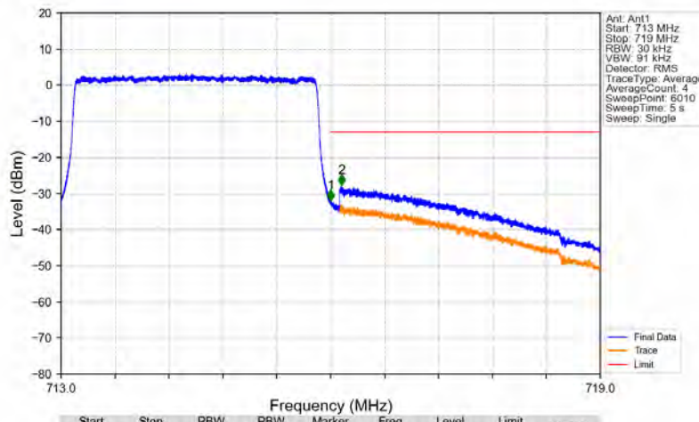
Band12_3MHz_16QAM_HCH_714.5MHz_RB_15_0_NTNV
