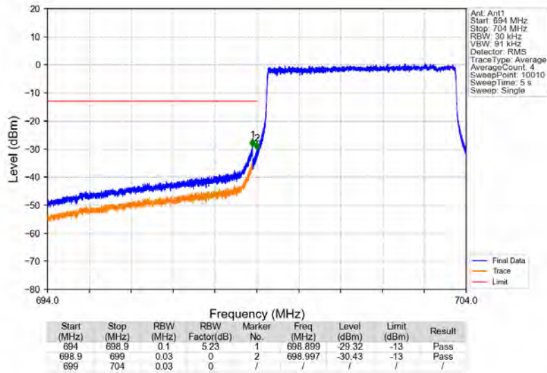
Band12_5MHz_64QAM_LCH_701.5MHz_RB_25_0_NTNV
