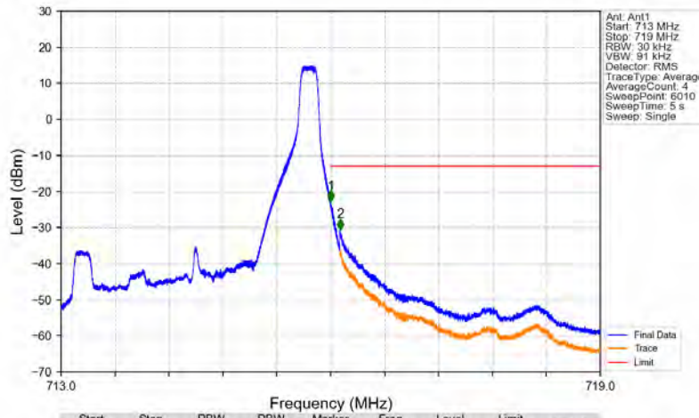
Band12_3MHz_16QAM_HCH_714.5MHz_RB_1_14_NTNV
