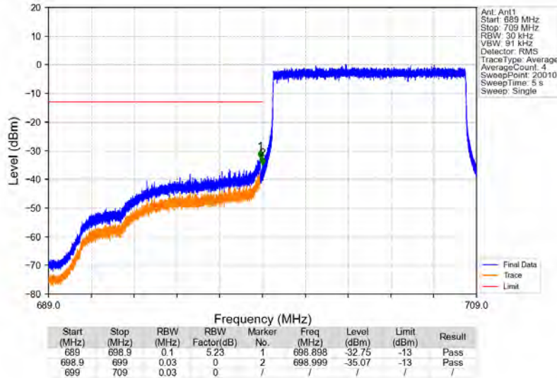
Band12_10MHz_QPSK_LCH_704MHz_RB_50_0_NTNV
