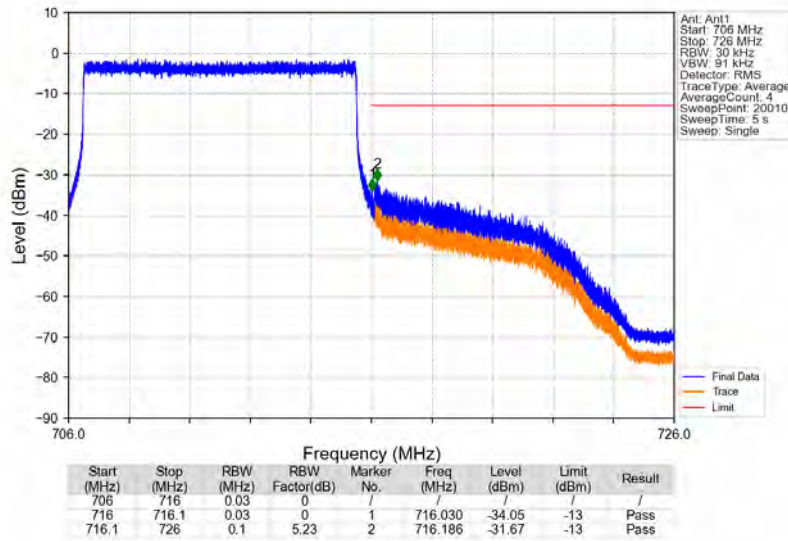
Band12_10MHz_16QAM_HCH_711MHz_RB_50_0_NTV
