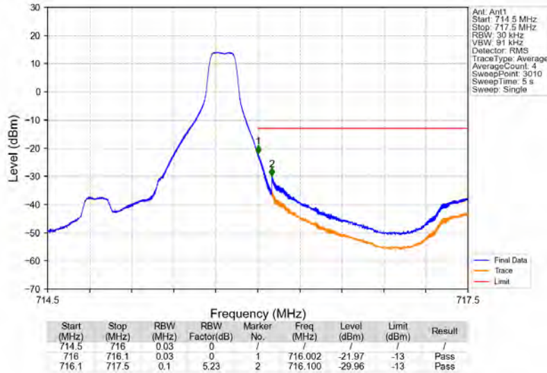
Band12_1.4MHz_16QAM_HCH_715.3MHz_RB_1_5_NTNV
