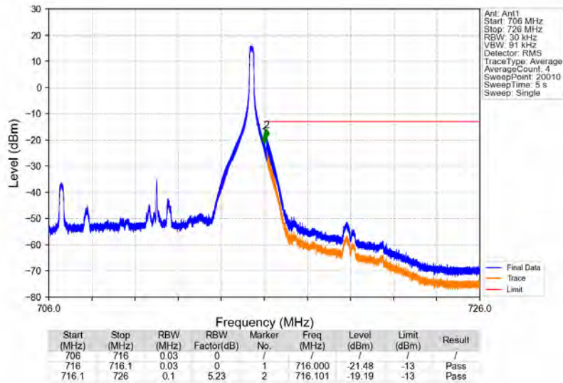
Band12_10MHz_QPSK_HCH_711MHz_RB_1_49_NTNV
