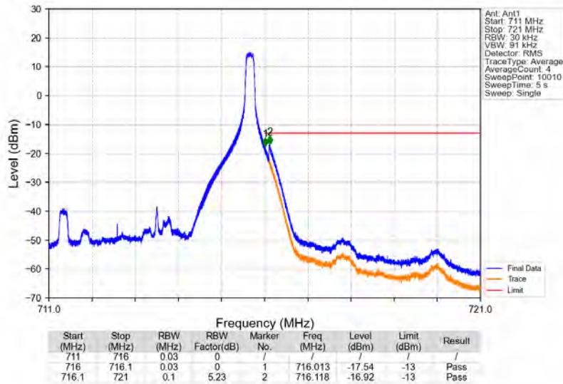
Band12_5MHz_16QAM_HCH_713.5MHz_RB_1_24_NTNV
