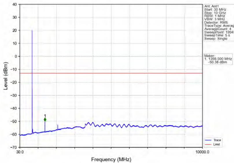
Band12_3MHz_64QAM_LCH_700.5MHz_RB_1_0_NTNV
