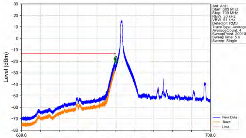
Band12_10MHz_16QAM_LCH_704MHz_RB_1_0_NTNV
