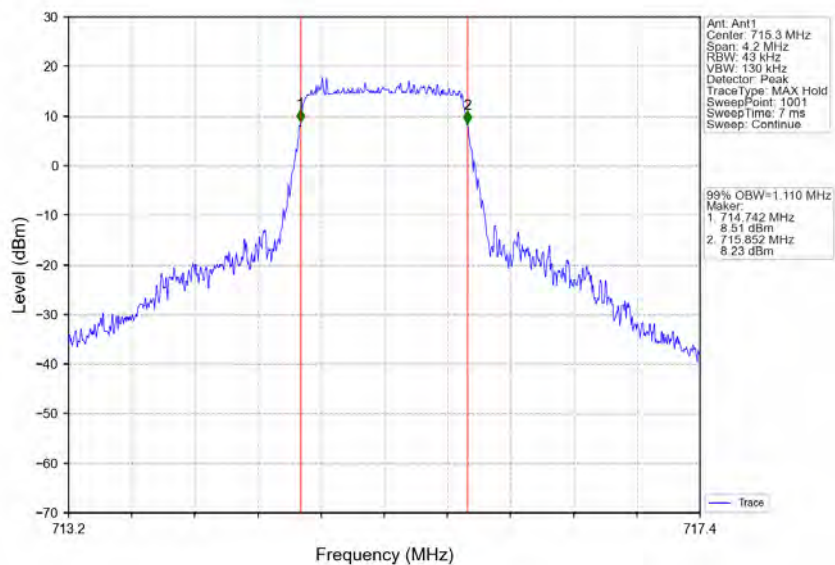
Band12_1.4MHz_16QAM_HCH_715.3MHz_RB_6_0_NTNV
