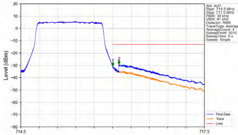
Band12_1.4MHz_64QAM_HCH_715.3MHz_RB_6_0_NTNV
