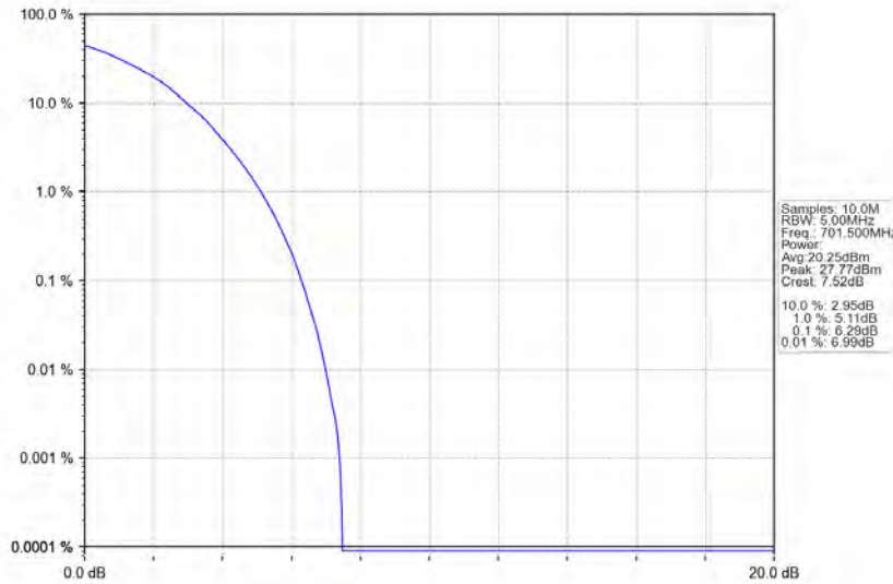
Band12_5MHz_64QAM_LCH_701.5MHz_RB_25_0_NTNV
