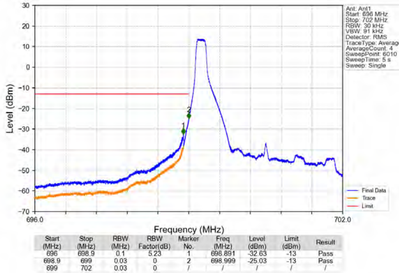
Band12_3MHz_64QAM_LCH_700.5MHz_RB_1_0_NTNV
