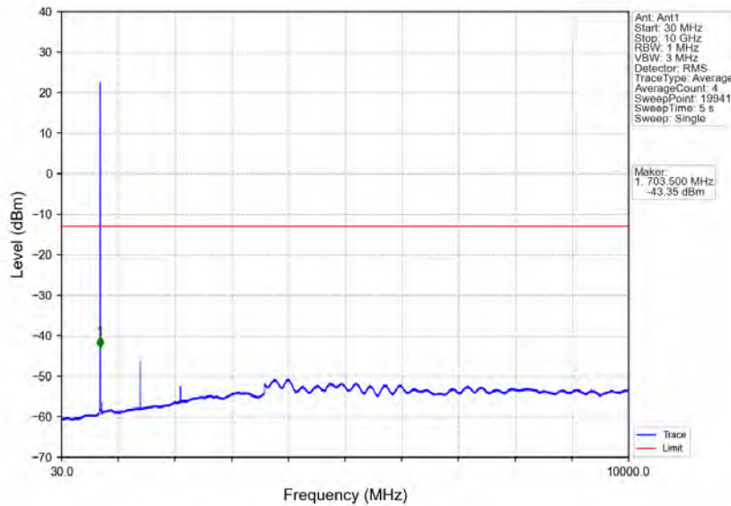
Band12_1.4MHz_QPSK_MCH_707.5MHz_RB_1_0_NTV
