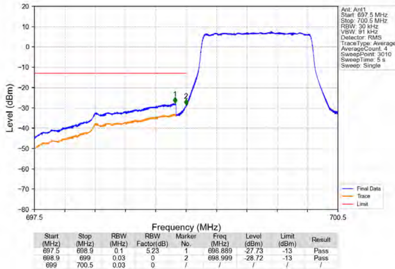
Band12_1.4MHz_QPSK_LCH_699.7MHz_RB_6_0_NTV
