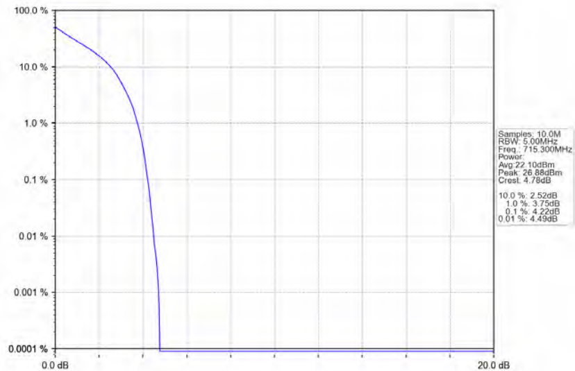
Band12_1.4MHz_QPSK_HCH_715.3MHz_RB_6_0_NTNV
