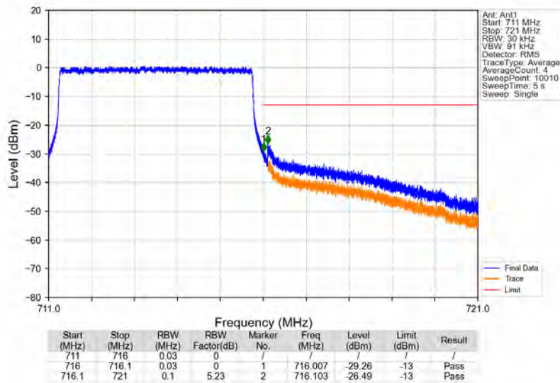
Band12_5MHz_16QAM_HCH_713.5MHz_RB_25_0_NTNV
