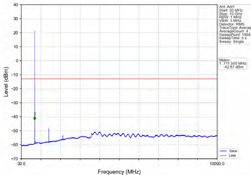
Band12_1.4MHz_16QAM_HCH_715.3MHz_RB_1_0_NTNV
