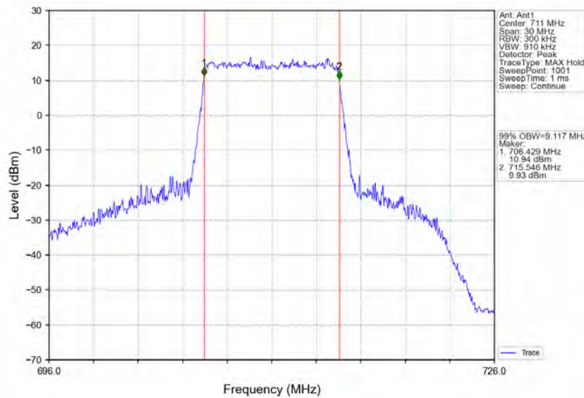
Band12_10MHz_64QAM_HCH_711MHz_RB_50_0_NTNV
