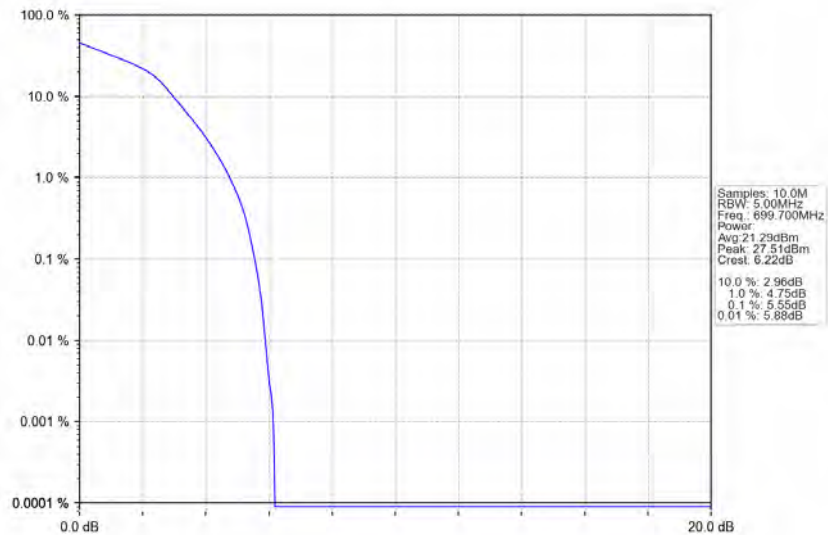
Band12_1.4MHz_16QAM_LCH_699.7MHz_RB_6_0_NTNV
