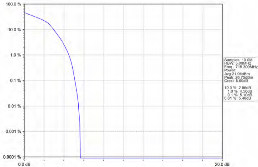
Band12_1.4MHz_16QAM_HCH_715.3MHz_RB_6_0_NTNV
