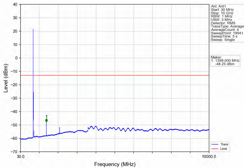
Band12_10MHz_16QAM_LCH_704MHz_RB_50_0_NTNV
