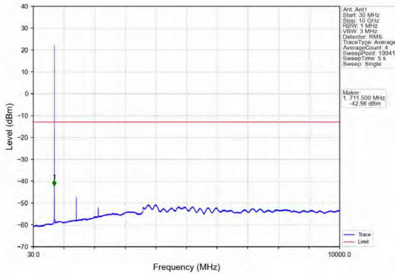
Band12_1.4MHz_QPSK_HCH_715.3MHz_RB_1_5_NTV
