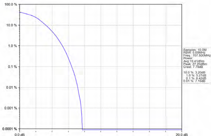
Band12_10MHz_16QAM_MCH_707.5MHz_RB_50_0_NTNV
