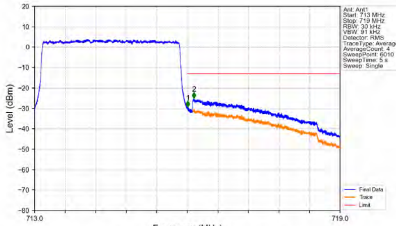
Band12_3MHz_QPSK_HCH_714.5MHz_RB_15_0_NTNV
