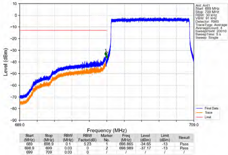
Band12_10MHz_16QAM_LCH_704MHz_RB_50_0_NTNV
