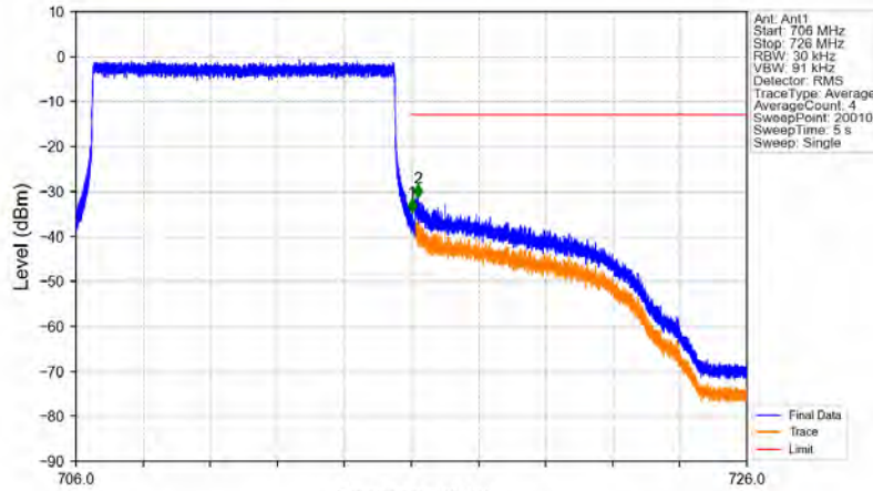
Band12_10MHz_QPSK_HCH_711MHz_RB_50_0_NTNV
