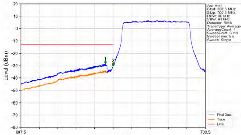
Band12_1.4MHz_16QAM_LCH_699.7MHz_RB_6_0_NTNV
