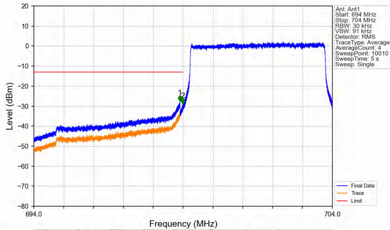
Band12_5MHz_QPSK_LCH_701.5MHz_RB_25_0_NTNV
