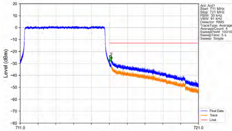
Band12_5MHz_QPSK_HCH_713.5MHz_RB_25_0_NTNV
