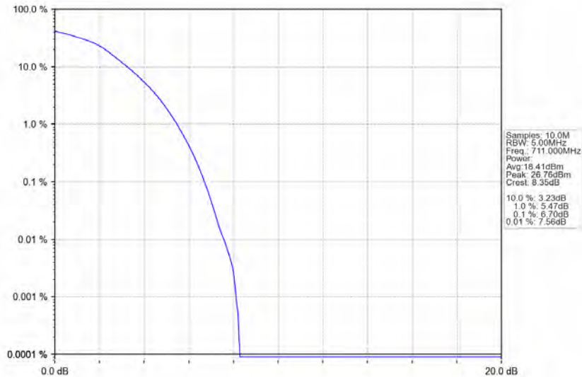
Band12_10MHz_64QAM_HCH_711MHz_RB_50_0_NTV
