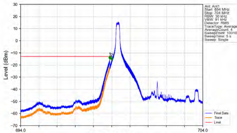
Band12_5MHz_16QAM_LCH_701.5MHz_RB_1_0_NTNV
