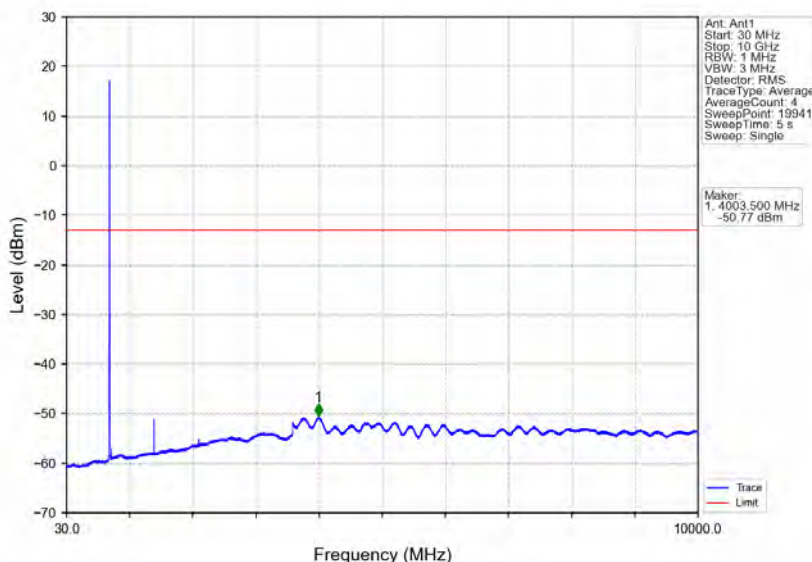
Band12_3MHz_64QAM_MCH_707.5MHz_RB_1_0_NTNV
