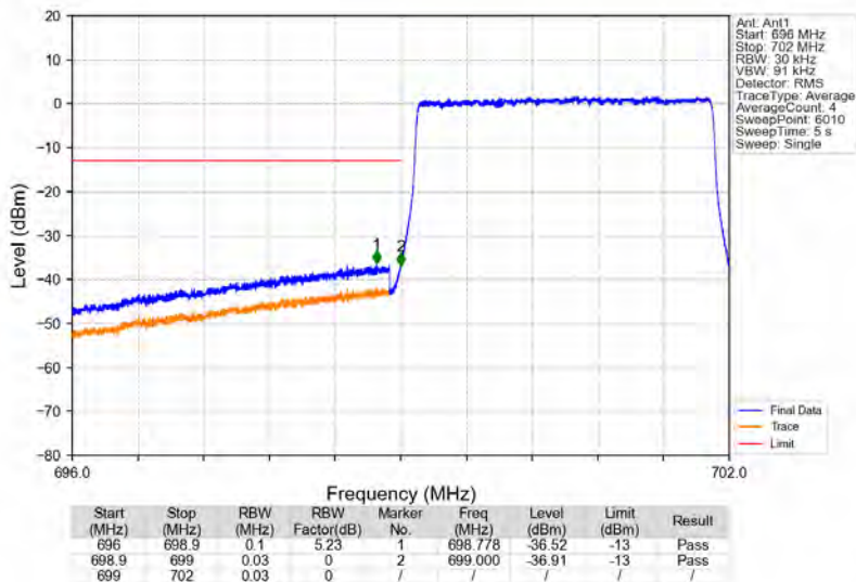
Band12_3MHz_64QAM_LCH_700.5MHz_RB_15_0_NTNV
