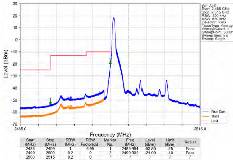
Band7_10MHz_64QAM_LCH_2505MHz_RB_1_0_NTNV
