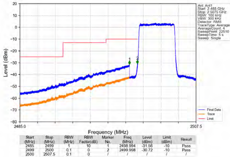
Band7_5MHz_64QAM_LCH_2502.5MHz_RB_25_0_NTNV
