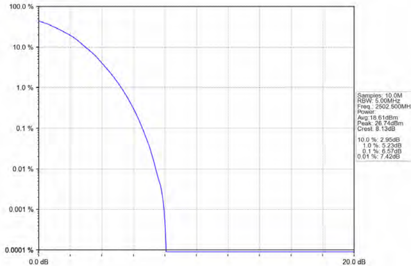
Band7_5MHz_64QAM_LCH_2502.5MHz_RB_25_0_NTNV
