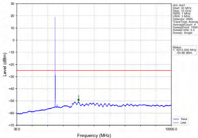
Band7_10MHz_64QAM_LCH_2505MHz_RB_1_0_NTNV
