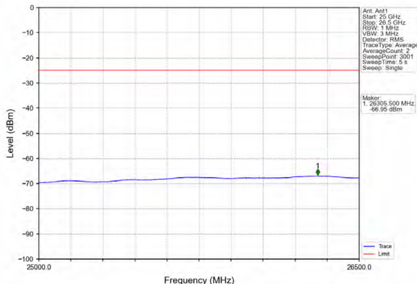
Band7_15MHz_QPSK_MCH_2535MHz_RB_1_0_NTNV
