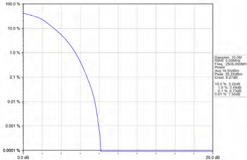
Band7_10MHz_64QAM_LCH_2505MHz_RB_50_0_NTNV
