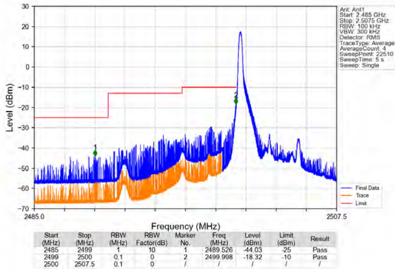
Band7_5MHz_64QAM_LCH_2502.5MHz_RB_1_0_NTNV
