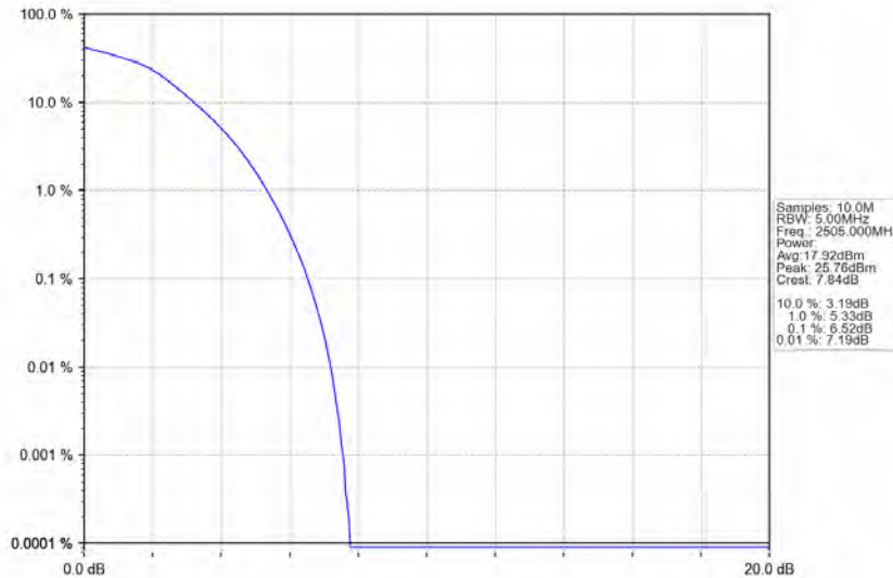
Band7_10MHz_16QAM_LCH_2505MHz_RB_50_0_NTNV
