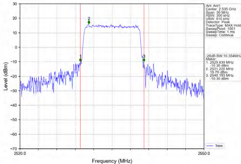
Band7_10MHz_16QAM_MCH_2535MHz_RB_50_0_NTNV
