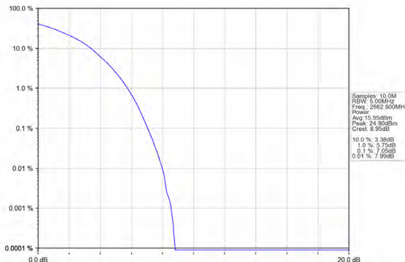
Band7_15MHz_16QAM_HCH_2562.5MHz_RB_75_0_NTNV
