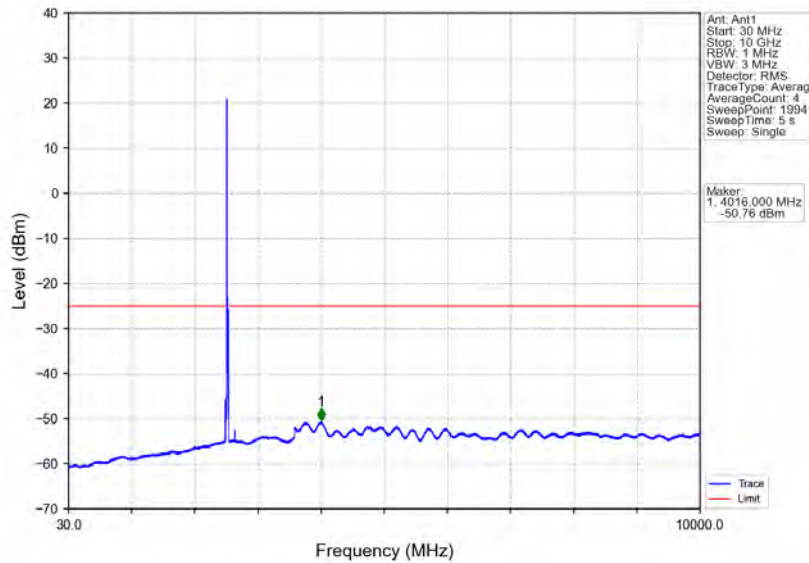
Band7_15MHz_QPSK_MCH_2535MHz_RB_1_0_NTNV
