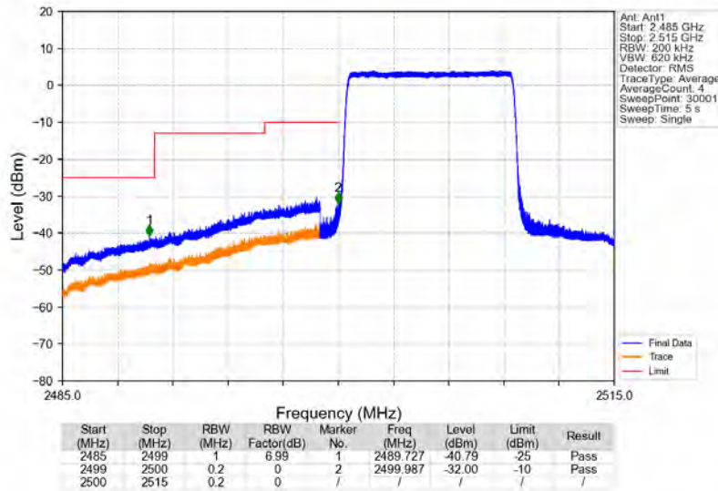
Band7_10MHz_16QAM_LCH_2505MHz_RB_50_0_NTV
