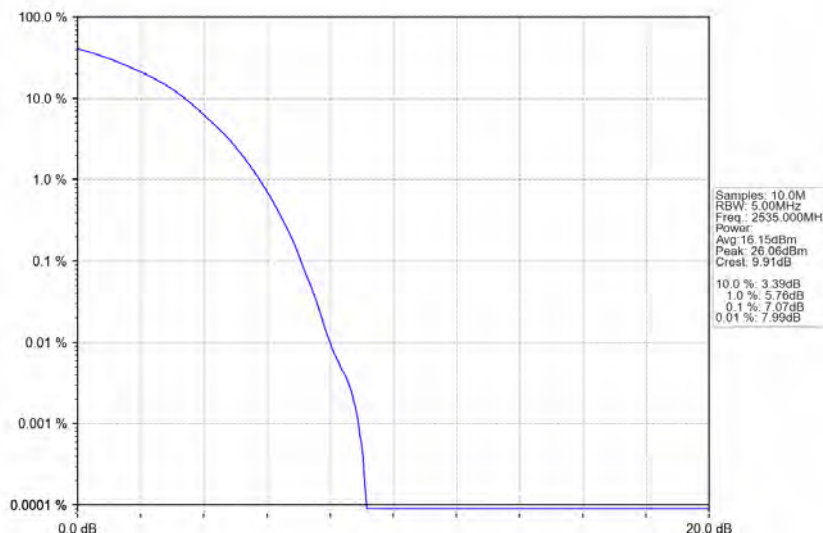
Band7_15MHz_16QAM_MCH_2535MHz_RB_75_0_NTNV
