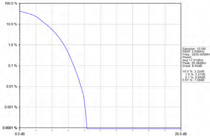
Band7_10MHz_64QAM_MCH_2535MHz_RB_50_0_NTNV
