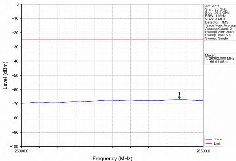
Band7_15MHz_16QAM_LCH_2507.5MHz_RB_75_0_NTNV
