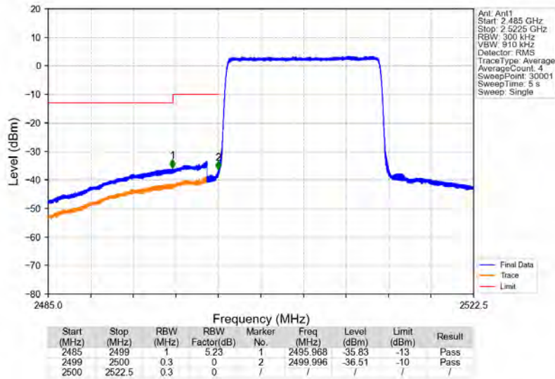
Band7_15MHz_64QAM_LCH_2507.5MHz_RB_75_0_NTNV
