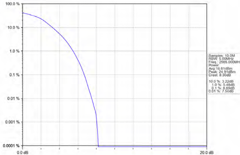
Band7_10MHz_64QAM_HCH_2565MHz_RB_50_0_NTV
