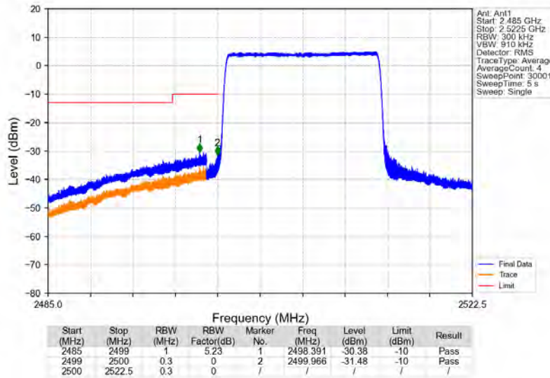
Band7_15MHz_QPSK_LCH_2507.5MHz_RB_75_0_NTNV
