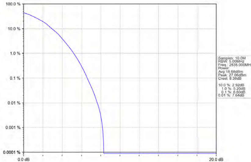
Band7_5MHz_64QAM_MCH_2535MHz_RB_25_0_NTNV
