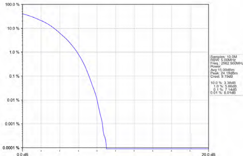
Band7_15MHz_64QAM_HCH_2562.5MHz_RB_75_0_NTNV
