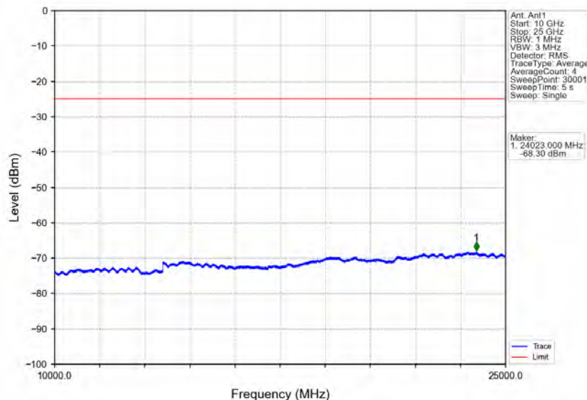
Band7_5MHz_64QAM_MCH_2535MHz_RB_1_0_NTNV
