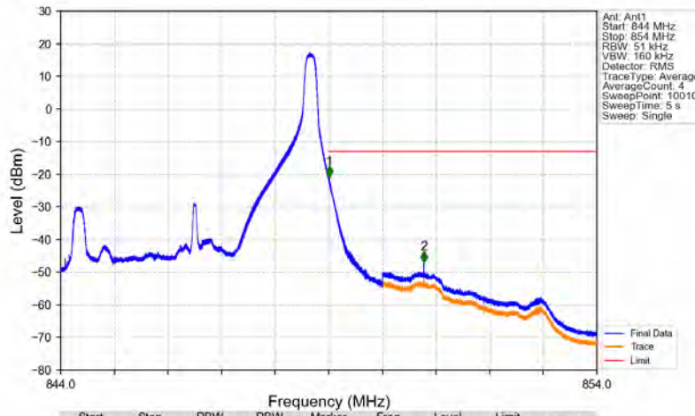
Band5_5MHz_16QAM_HCH_846.5MHz_RB_1_24_NTNV
