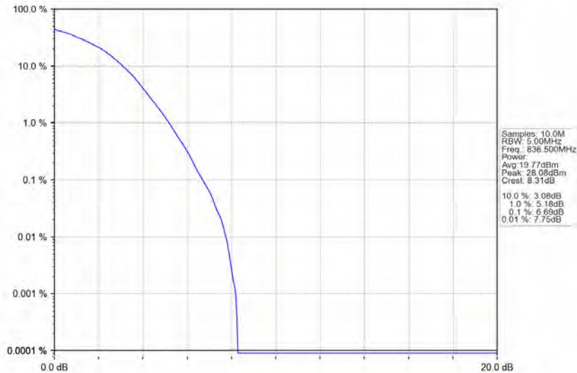
Band5_1.4MHz_64QAM_MCH_836.5MHz_RB_6_0_NTNV
