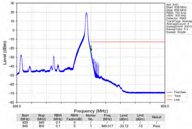
Band5_10MHz_16QAM_HCH_844MHz_RB_1_49_NTNV
