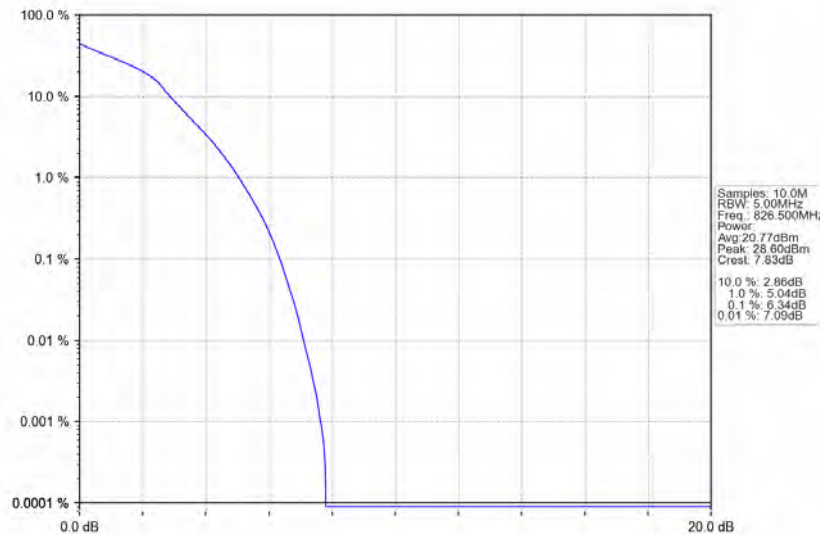
Band5_5MHz_16QAM_LCH_826.5MHz_RB_25_0_NTNV
