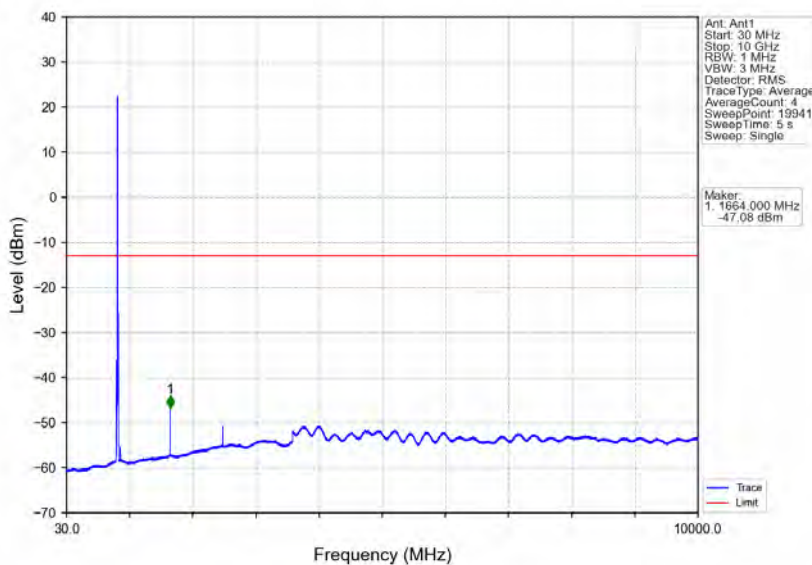
Band5_10MHz_QPSK_MCH_836.5MHz_RB_1_0_NTNV
