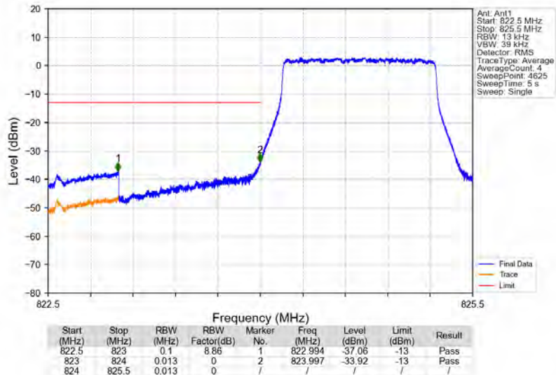
Band5_1.4MHz_16QAM_LCH_824.7MHz_RB_6_0_NTV
