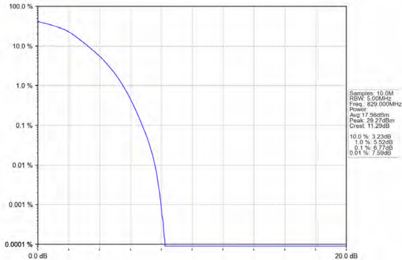
Band5_10MHz_64QAM_LCH_829MHz_RB_50_0_NTNV
