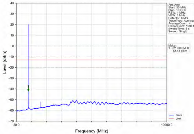
Band5_1.4MHz_64QAM_LCH_824.7MHz_RB_1_0_NTNV
