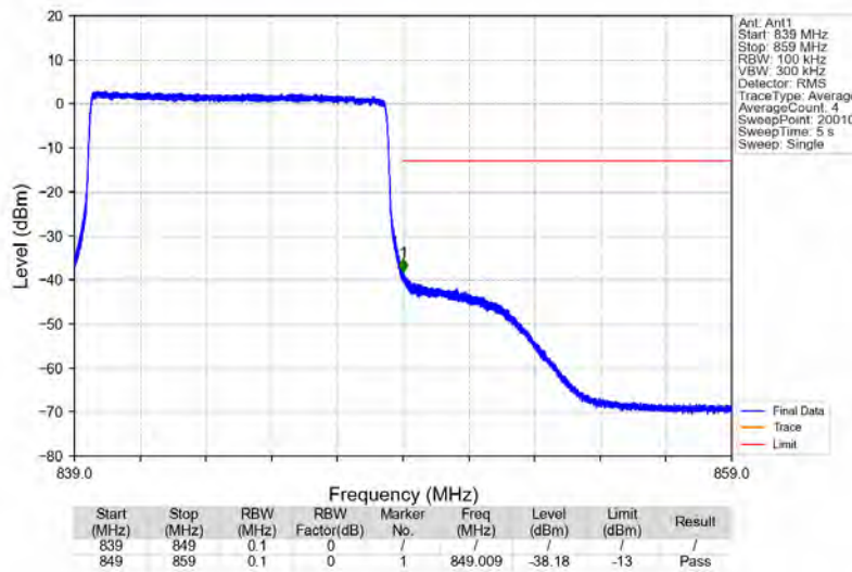
Band5_10MHz_16QAM_HCH_844MHz_RB_50_0_NTNV
