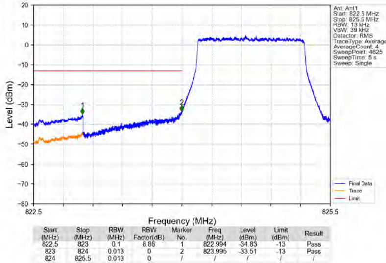
Band5_1.4MHz_QPSK_LCH_824.7MHz_RB_6_0_NTNV
