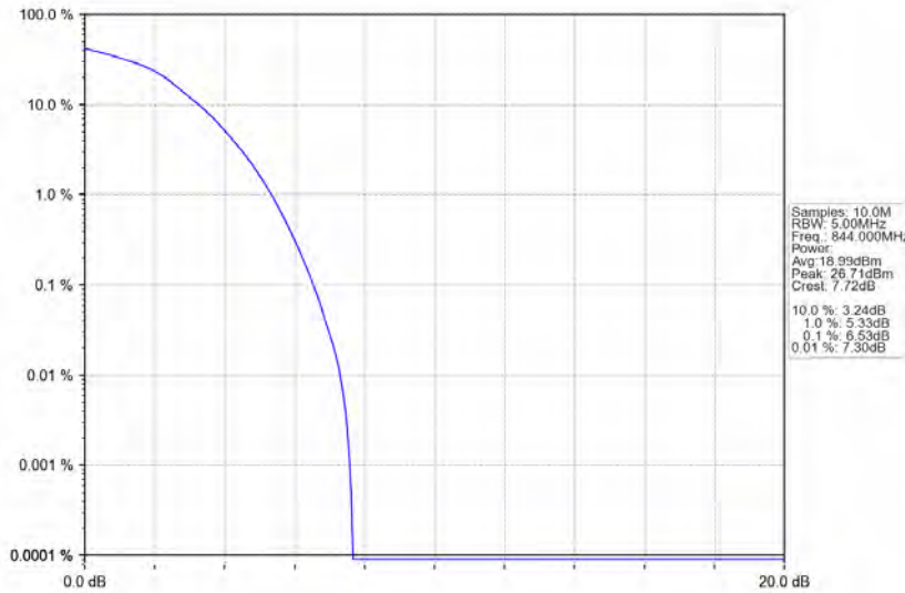
Band5_10MHz_16QAM_HCH_844MHz_RB_50_0_NTNV
