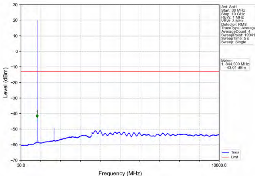
Band5_1.4MHz_64QAM_HCH_848.3MHz_RB_1_5_NTV
