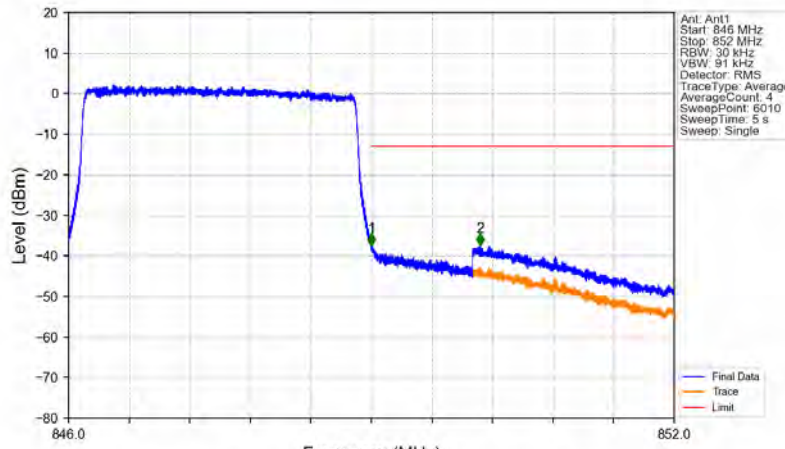
Band5_3MHz_64QAM_HCH_847.5MHz_RB_15_0_NTNV
