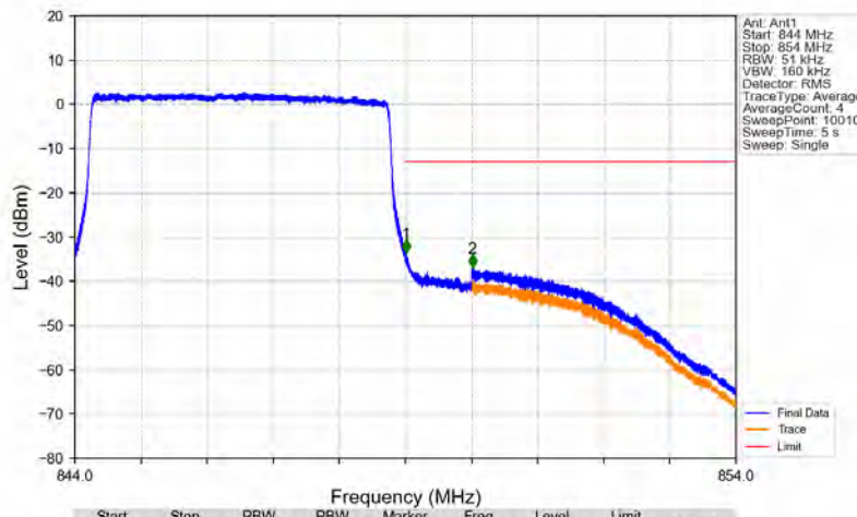
Band5_5MHz_16QAM_HCH_846.5MHz_RB_25_0_NTNV
