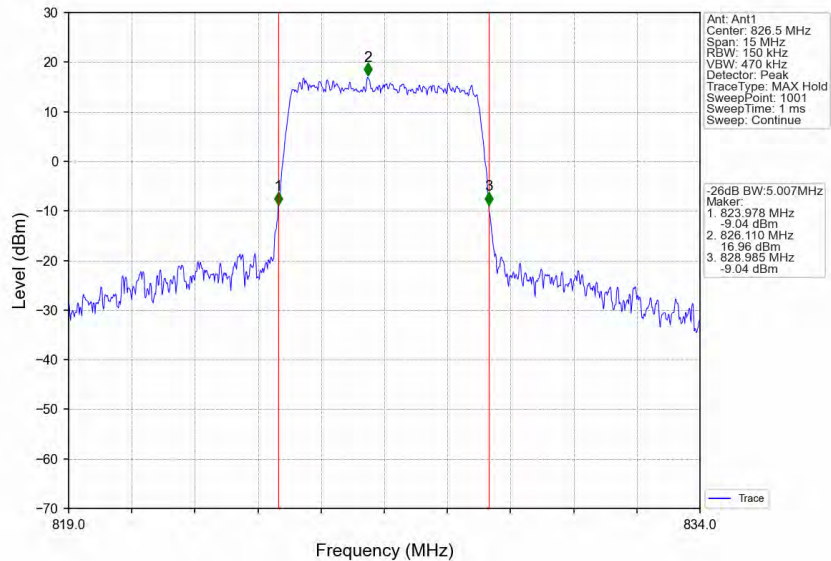
Band5_5MHz_16QAM_LCH_826.5MHz_RB_25_0_NTNV
