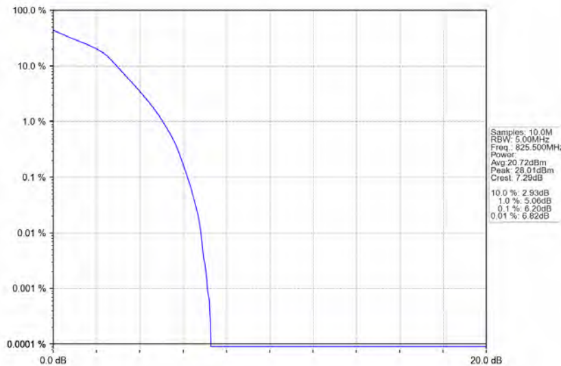
Band5_3MHz_16QAM_LCH_825.5MHz_RB_15_0_NTNV
