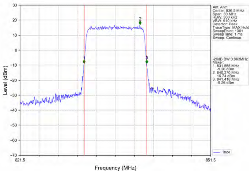
Band5_10MHz_16QAM_MCH_836.5MHz_RB_50_0_NTNV
