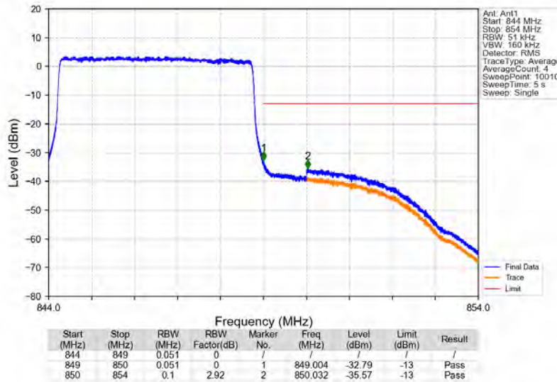
Band5_5MHz_QPSK_HCH_846.5MHz_RB_25_0_NTNV
