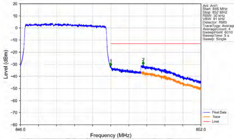
Band5_3MHz_QPSK_HCH_847.5MHz_RB_15_0_NTNV
