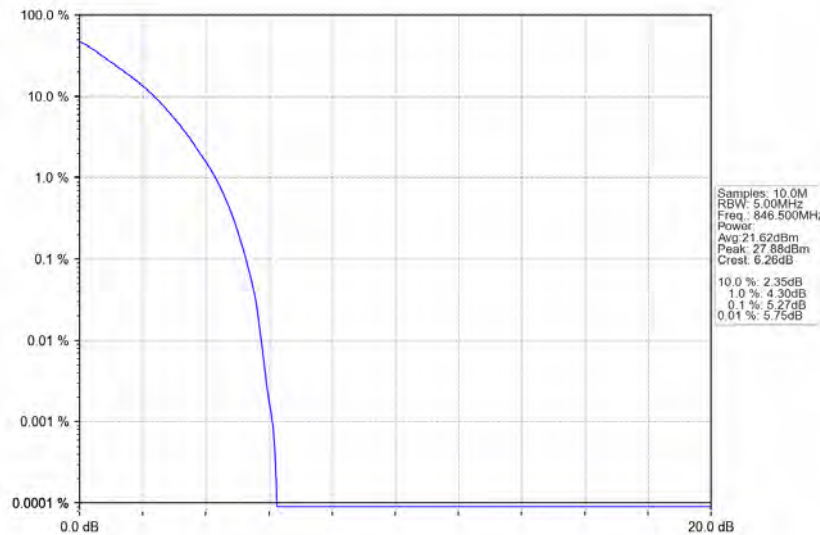
Band5_5MHz_QPSK_HCH_846.5MHz_RB_25_0_NTNV
