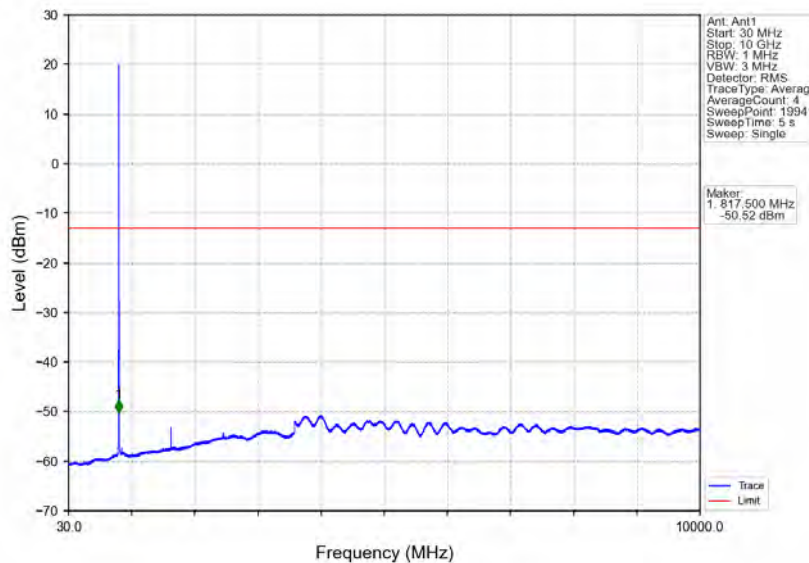
Band5_3MHz_64QAM_LCH_825.5MHz_RB_1_0_NTNV
