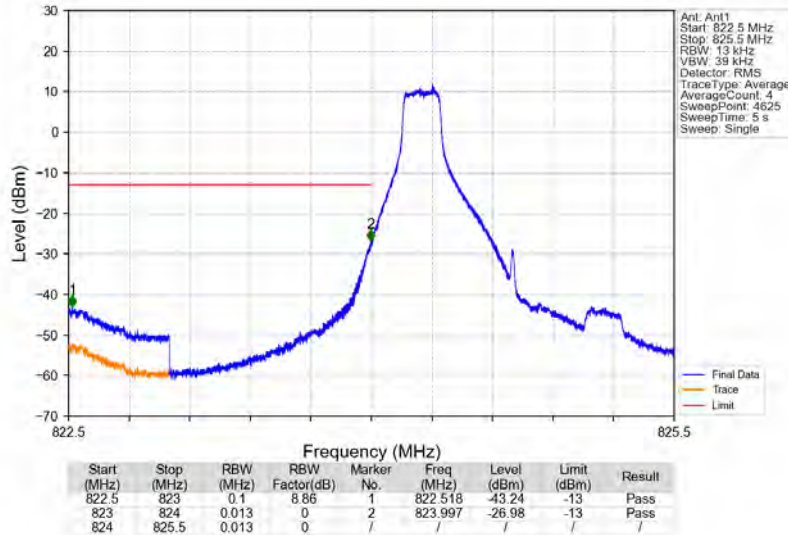
Band5_1.4MHz_64QAM_LCH_824.7MHz_RB_1_0_NTNV
