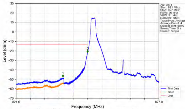
Band5_3MHz_16QAM_LCH_825.5MHz_RB_1_0_NTNV
