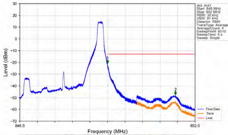
Band5_3MHz_16QAM_HCH_847.5MHz_RB_1_14_NTNV
