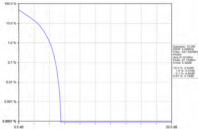
Band5_3MHz_QPSK_HCH_847.5MHz_RB_15_0_NTNV
