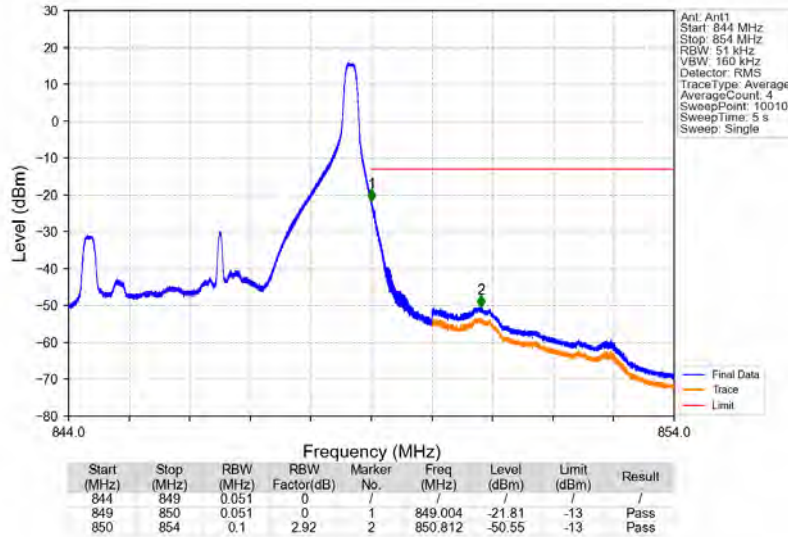
Band5_5MHz_64QAM_HCH_846.5MHz_RB_1_24_NTNV
