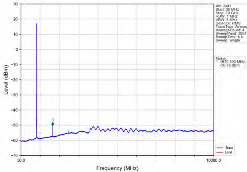
Band5_3MHz_64QAM_MCH_836.5MHz_RB_1_0_NTNV
