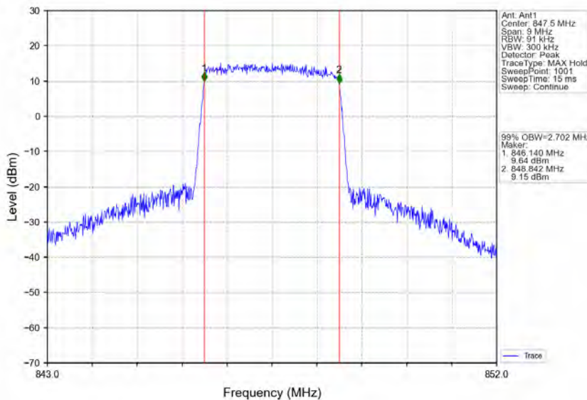
Band5_3MHz_64QAM_HCH_847.5MHz_RB_15_0_NTNV
