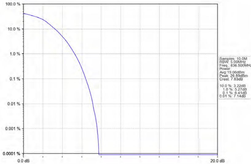
Band5_10MHz_16QAM_MCH_836.5MHz_RB_50_0_NTNV
