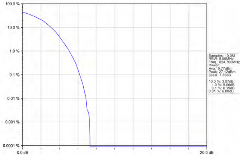
Band5_1.4MHz_64QAM_LCH_824.7MHz_RB_6_0_NTNV
