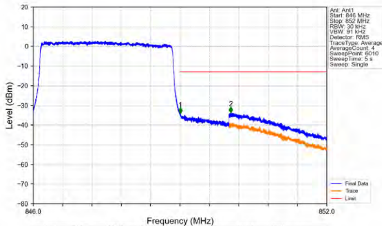
Band5_3MHz_16QAM_HCH_847.5MHz_RB_15_0_NTNV
