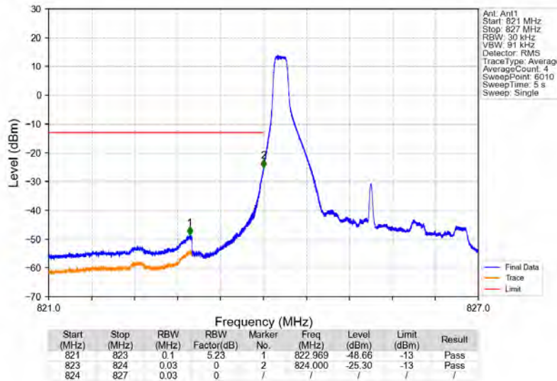
Band5_3MHz_64QAM_LCH_825.5MHz_RB_1_0_NTNV
