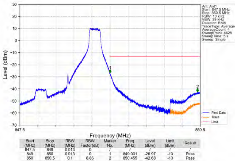
Band5_1.4MHz_64QAM_HCH_848.3MHz_RB_1_5_NTV
