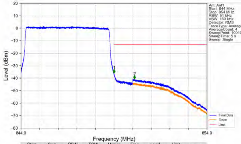
Band5_5MHz_64QAM_HCH_846.5MHz_RB_25_0_NTNV
