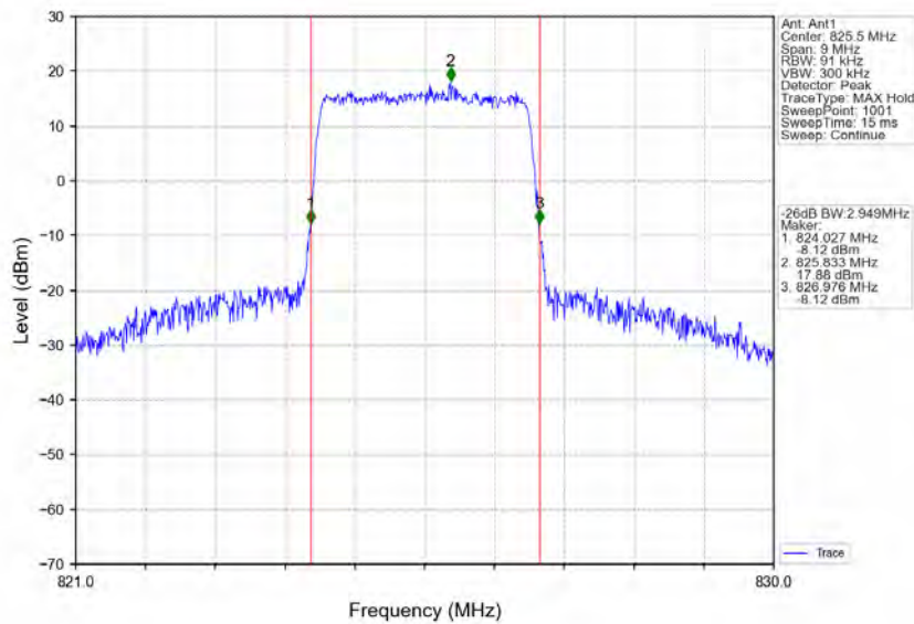
Band5_3MHz_QPSK_LCH_825.5MHz_RB_15_0_NTNV
