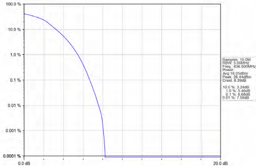
Band5_10MHz_64QAM_MCH_836.5MHz_RB_50_0_NTNV
