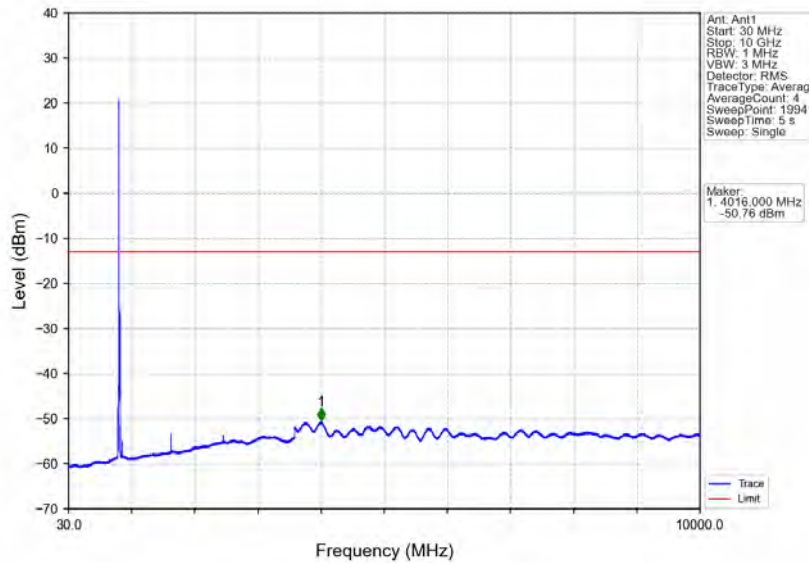
Band5_10MHz_64QAM_LCH_829MHz_RB_1_0_NTNV
