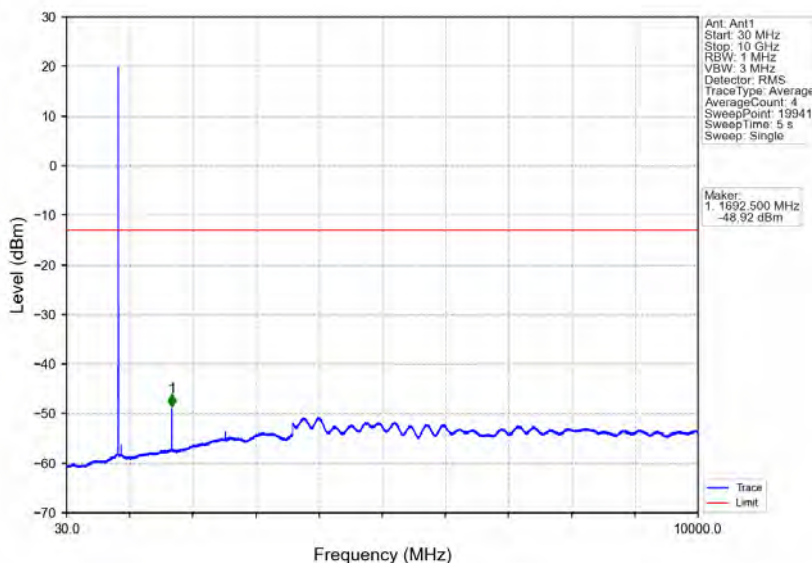
Band5_3MHz_64QAM_HCH_847.5MHz_RB_1_14_NTNV
