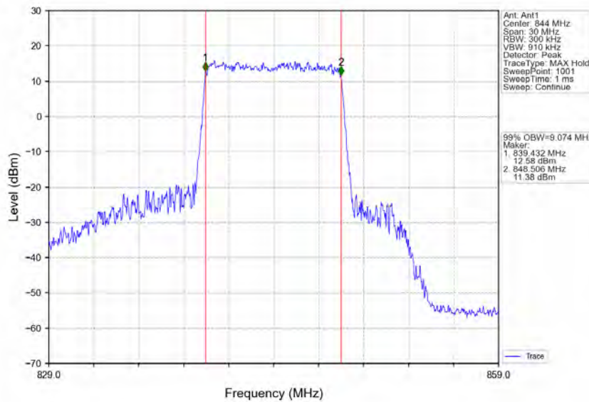
Band5_10MHz_64QAM_HCH_844MHz_RB_50_0_NTNV
