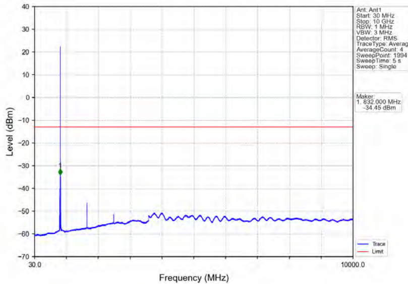
Band5_1.4MHz_QPSK_MCH_836.5MHz_RB_1_0_NTNV
