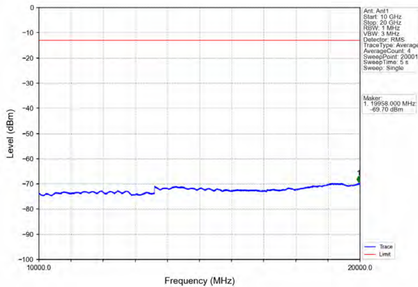
Band4_10MHz_64QAM_LCH_1715MHz_RB_50_0_NTV
