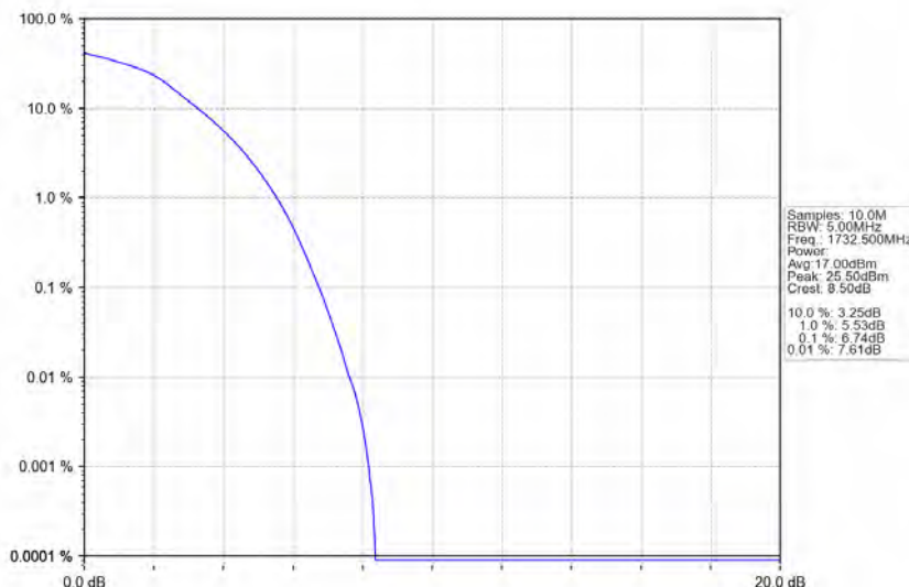
Band4_10MHz_64QAM_MCH_1732.5MHz_RB_50_0_NTNV
