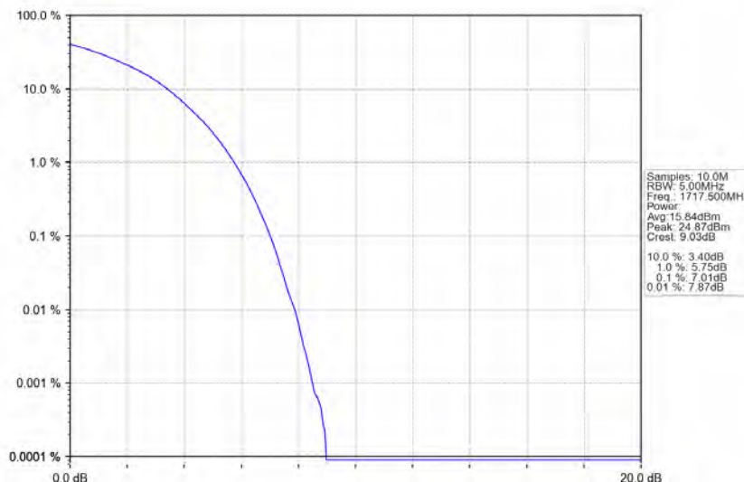
Band4_15MHz_16QAM_LCH_1717.5MHz_RB_75_0_NTNV
