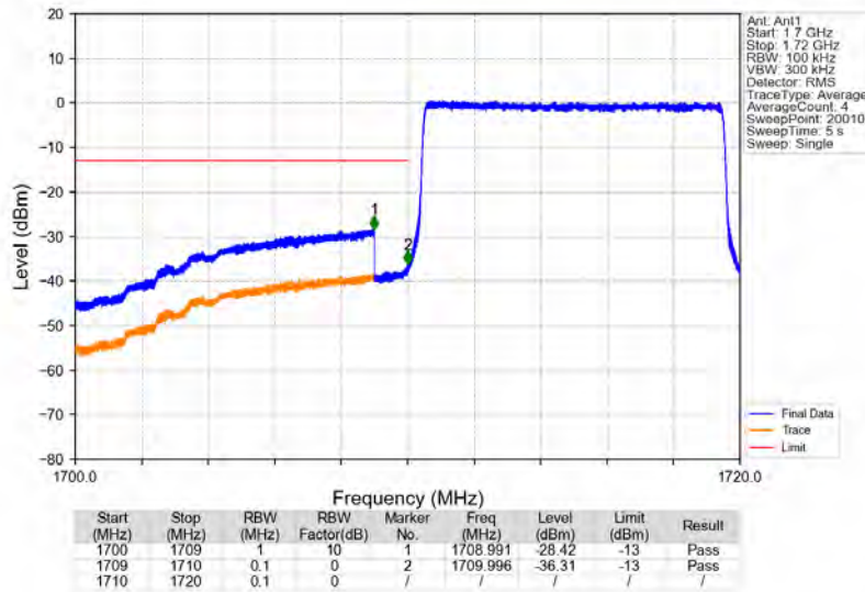
Band4_10MHz_64QAM_LCH_1715MHz_RB_50_0_NTV
