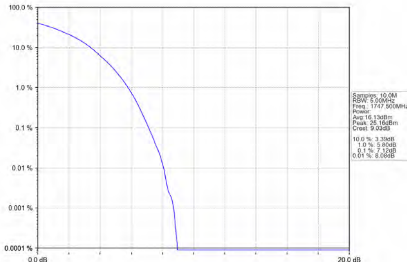
Band4_15MHz_16QAM_HCH_1747.5MHz_RB_75_0_NTNV
