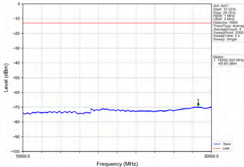
Band4_3MHz_QPSK_HCH_1753.5MHz_RB_1_0_NTNV
