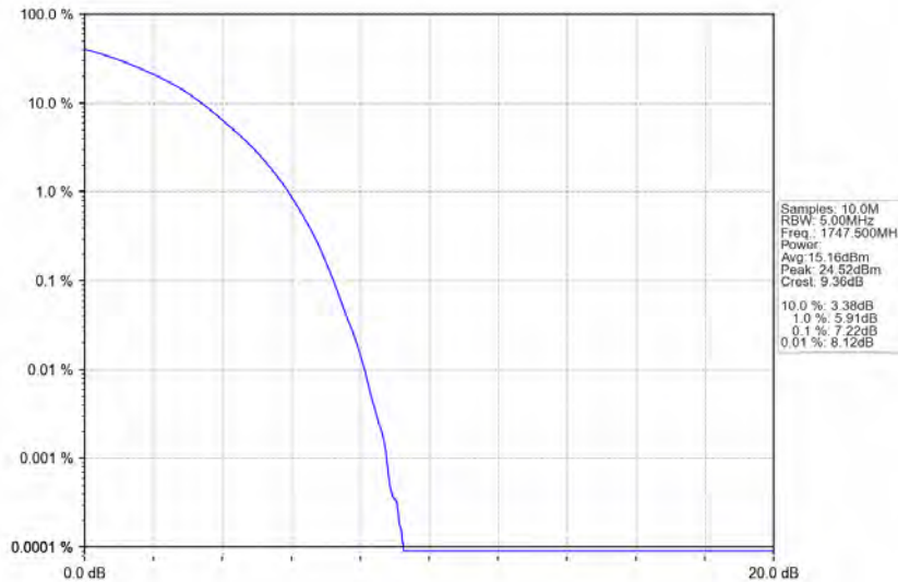
Band4_15MHz_64QAM_HCH_1747.5MHz_RB_75_0_NTNV
