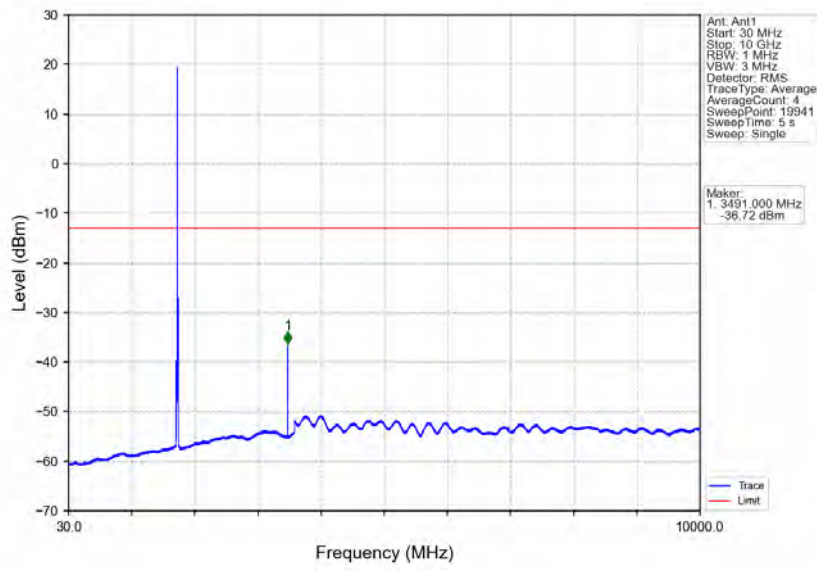
Band4_10MHz_64QAM_HCH_1750MHz_RB_1_0_NTNV
