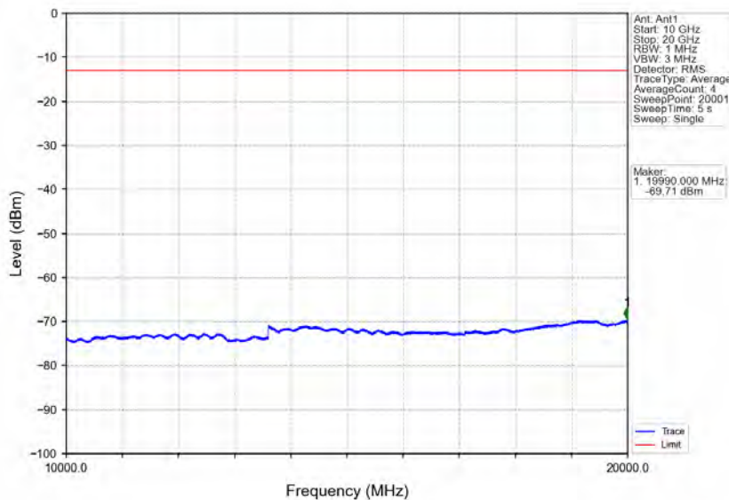
Band4_1.4MHz_64QAM_MCH_1732.5MHz_RB_1_0_NTNV
