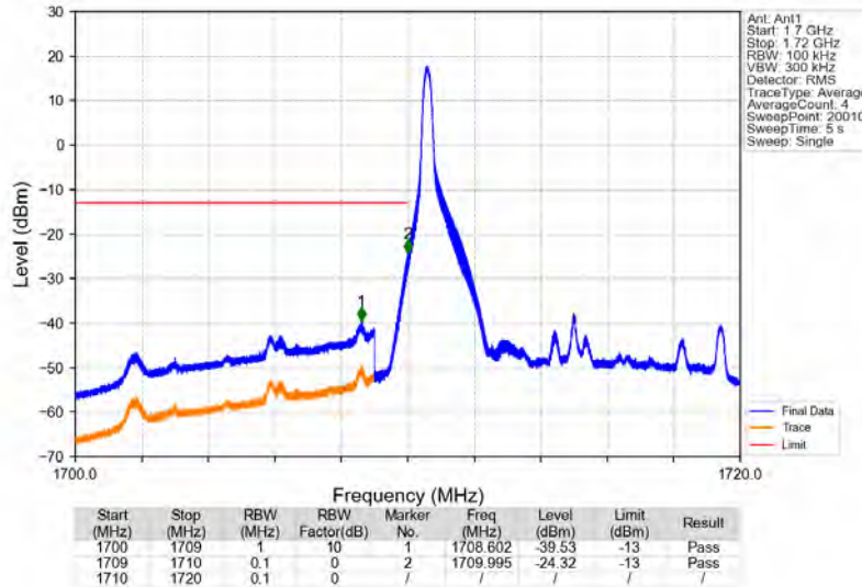
Band4_10MHz_64QAM_LCH_1715MHz_RB_1_0_NTNV
