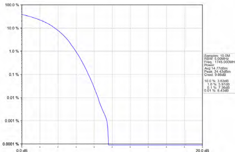
Band4_20MHz_16QAM_HCH_1745MHz_RB_100_0_NTNV
