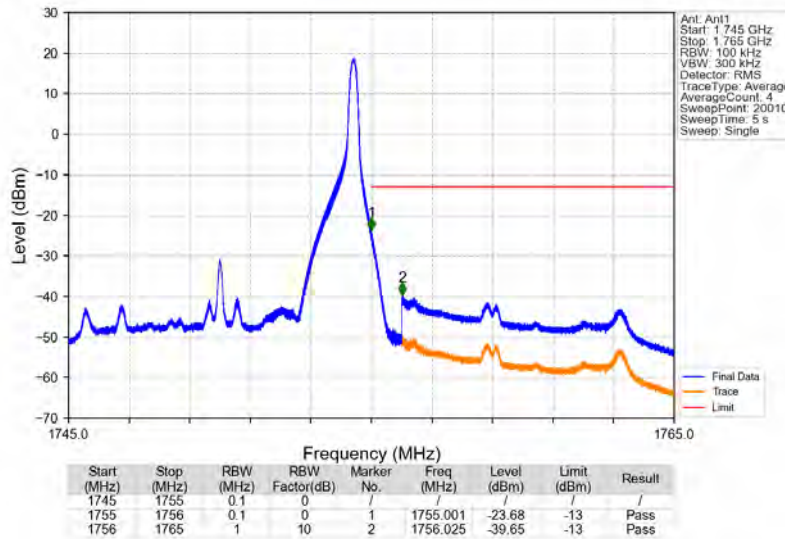
Band4_10MHz_16QAM_HCH_1750MHz_RB_1_49_NTV
