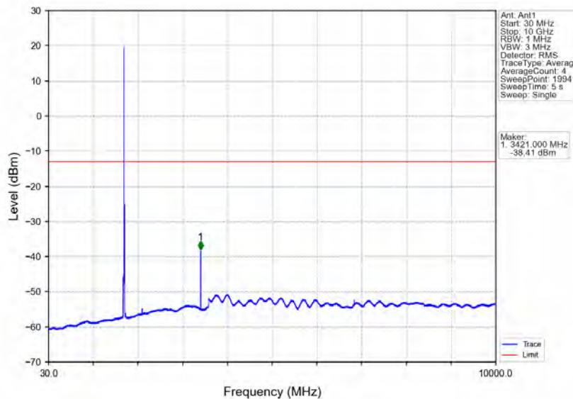
Band4_10MHz_64QAM_LCH_1715MHz_RB_1_0_NTNV
