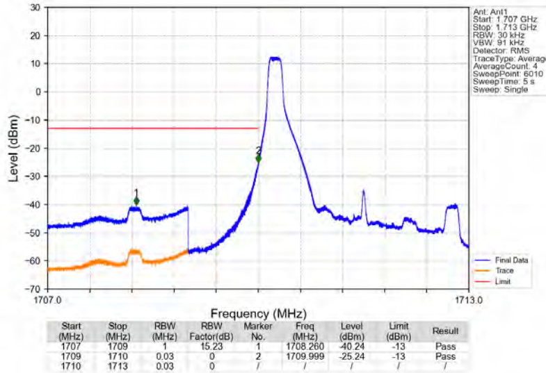
Band4_3MHz_64QAM_LCH_1711.5MHz_RB_1_0_NTNV
