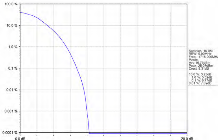
Band4_10MHz_64QAM_LCH_1715MHz_RB_50_0_NTNV
