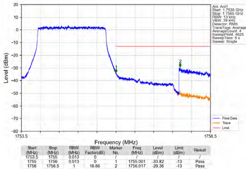
Band4_1.4MHz_QPSK_HCH_1754.3MHz_RB_6_0_NTV
