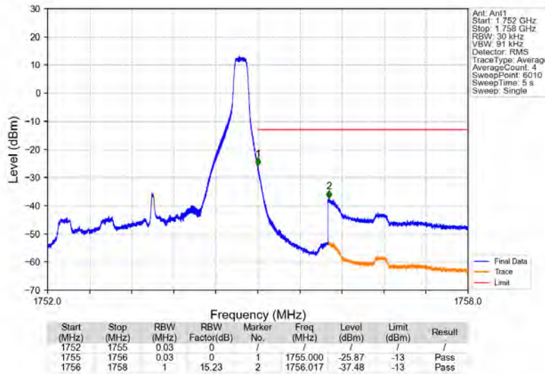
Band4_3MHz_64QAM_HCH_1753.5MHz_RB_1_14_NTNV
