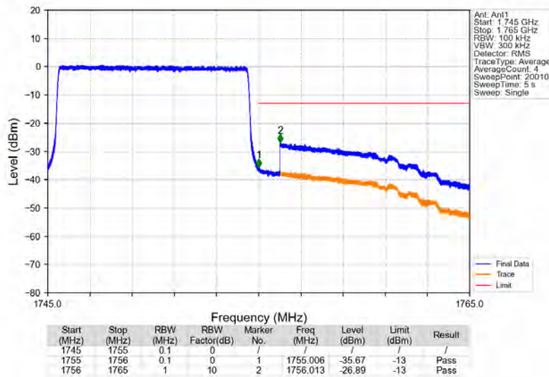
Band4_10MHz_64QAM_HCH_1750MHz_RB_50_0_NTV
