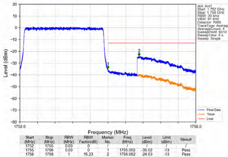
Band4_3MHz_64QAM_HCH_1753.5MHz_RB_15_0_NTNV
