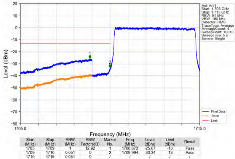
Band4_5MHz_64QAM_LCH_1712.5MHz_RB_25_0_NTNV
