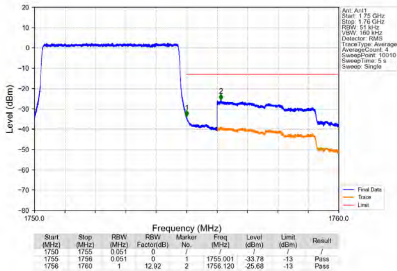
Band4_5MHz_QPSK_HCH_1752.5MHz_RB_25_0_NTNV
