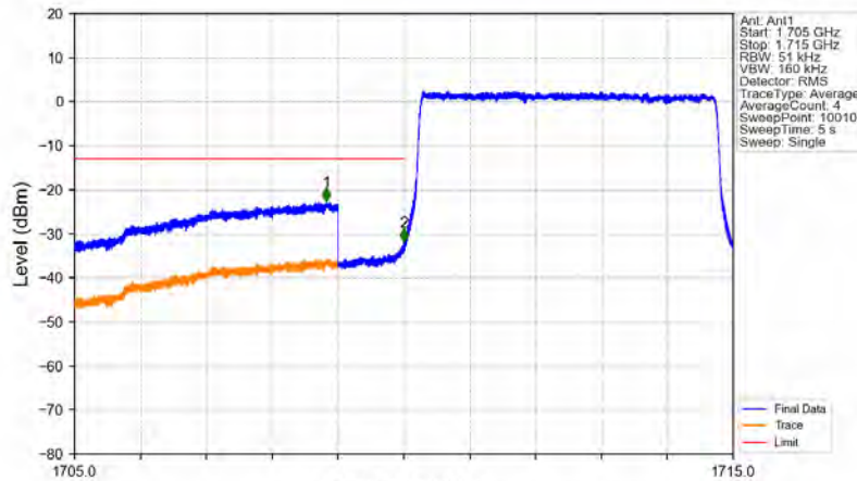
Band4_5MHz_QPSK_LCH_1712.5MHz_RB_25_0_NTNV
