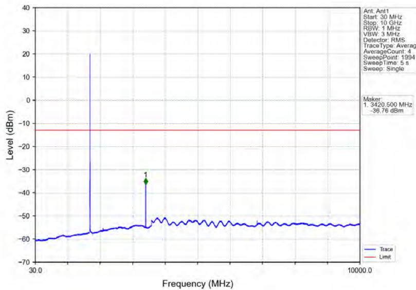
Band4_3MHz_16QAM_LCH_1711.5MHz_RB_1_0_NTNV
