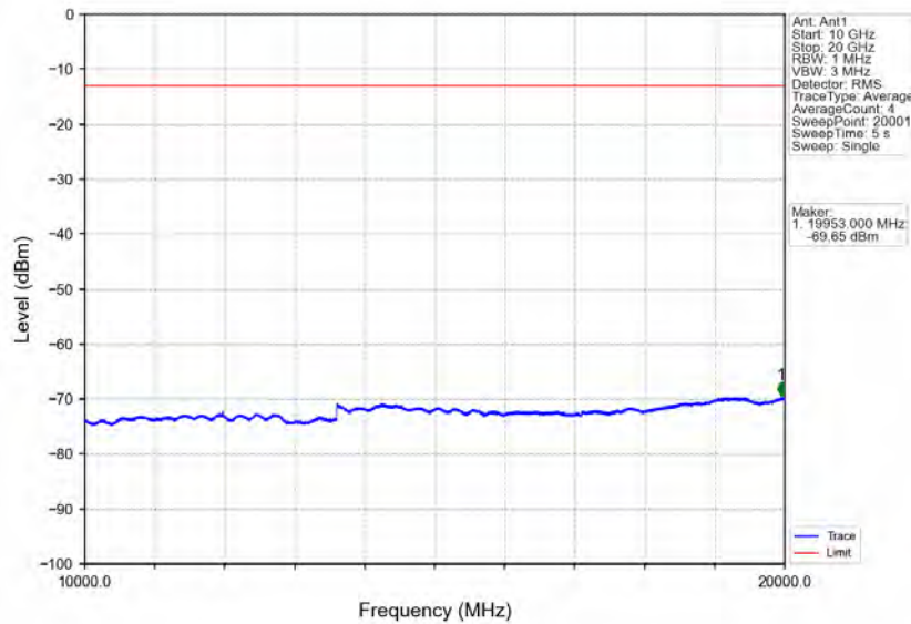
Band4_10MHz_16QAM_LCH_1715MHz_RB_50_0_NTV
