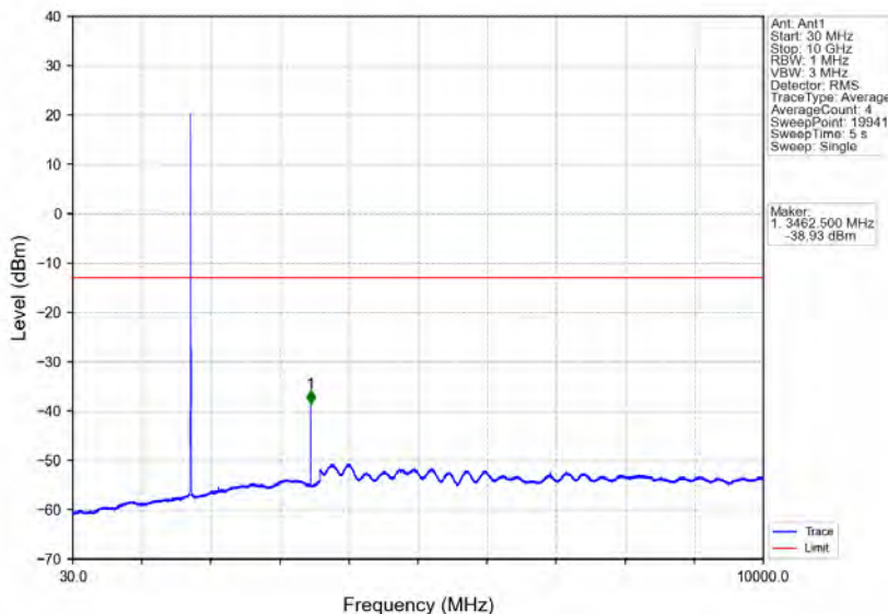
Band4_3MHz_16QAM_MCH_1732.5MHz_RB_1_0_NTNV
