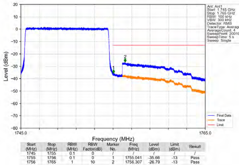
Band4_10MHz_16QAM_HCH_1750MHz_RB_50_0_NTV
