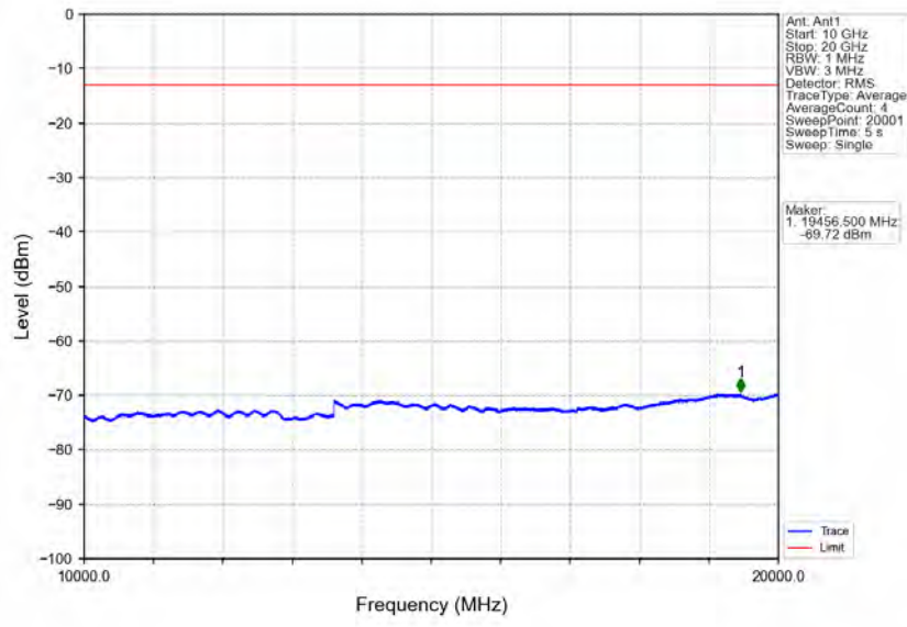
Band4_3MHz_16QAM_HCH_1753.5MHz_RB_1_0_NTNV
