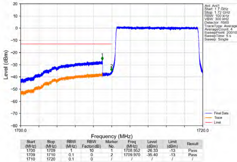
Band4_10MHz_16QAM_LCH_1715MHz_RB_50_0_NTV
