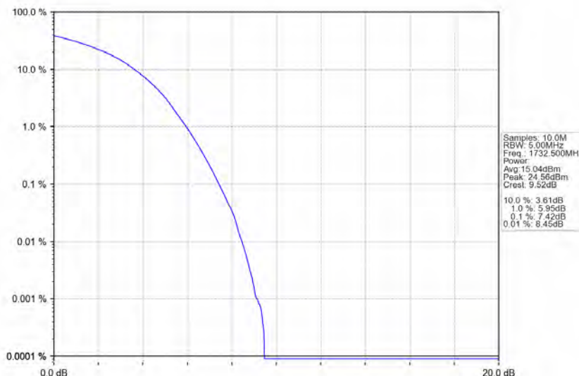
Band4_20MHz_16QAM_MCH_1732.5MHz_RB_100_0_NTNV
