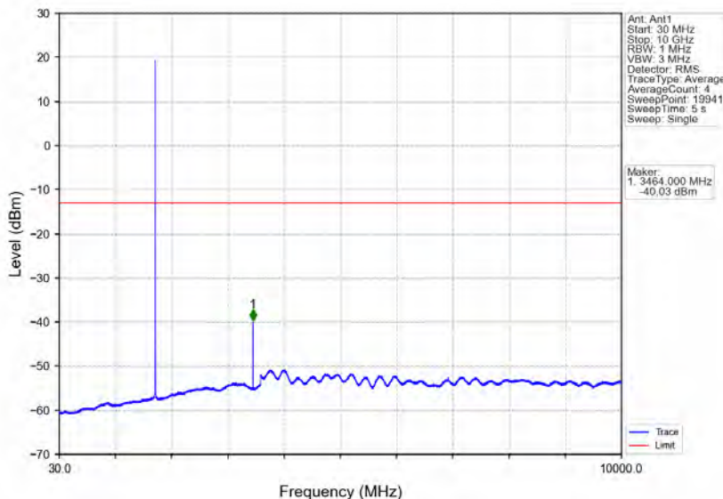
Band4_1.4MHz_64QAM_MCH_1732.5MHz_RB_1_0_NTNV
