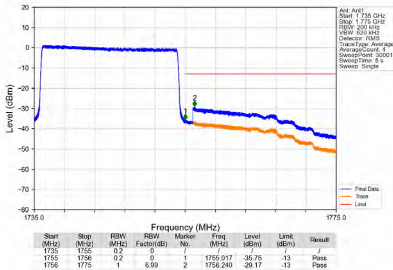
Band4_20MHz_64QAM_HCH_1745MHz_RB_100_0_NTNV
