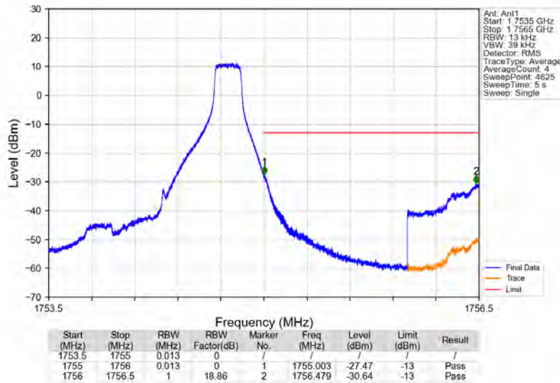
Band4_1.4MHz_QPSK_HCH_1754.3MHz_RB_1_5_NTV
