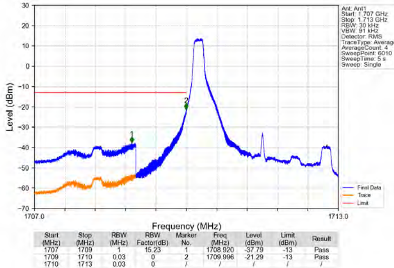
Band4_3MHz_16QAM_LCH_1711.5MHz_RB_1_0_NTNV
