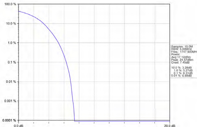
Band4_15MHz_QPSK_HCH_1747.5MHz_RB_75_0_NTNV
