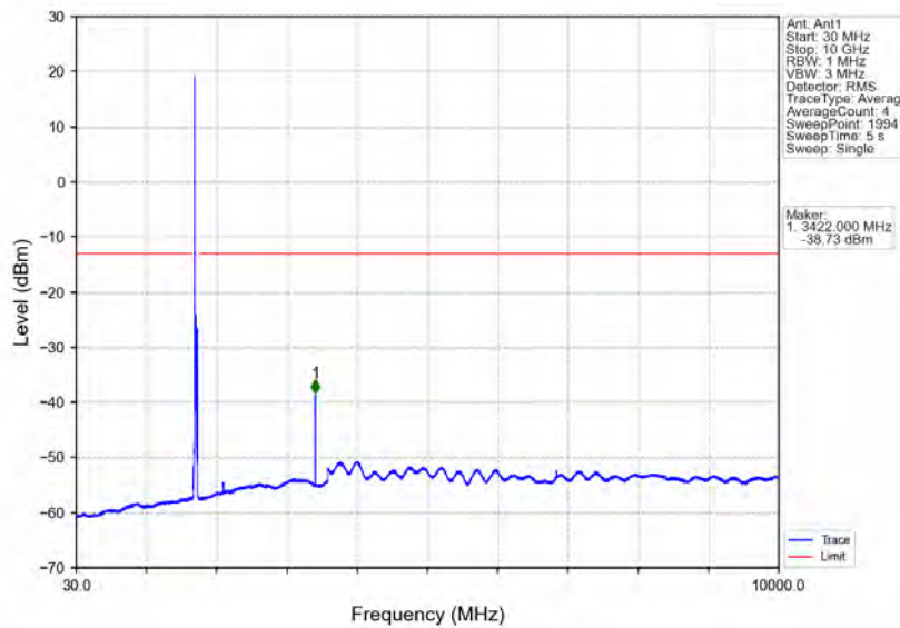
Band4_20MHz_64QAM_LCH_1720MHz_RB_1_0_NTNV
