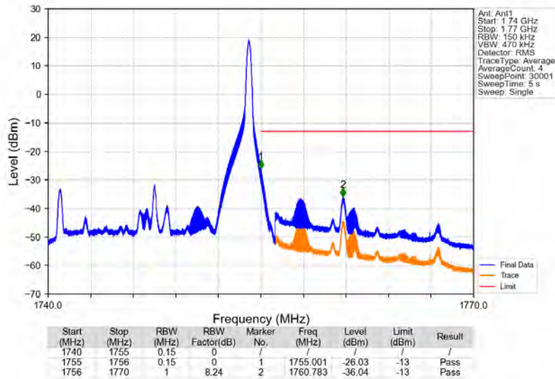
Band4_15MHz_64QAM_HCH_1747.5MHz_RB_1_74_NTNV
