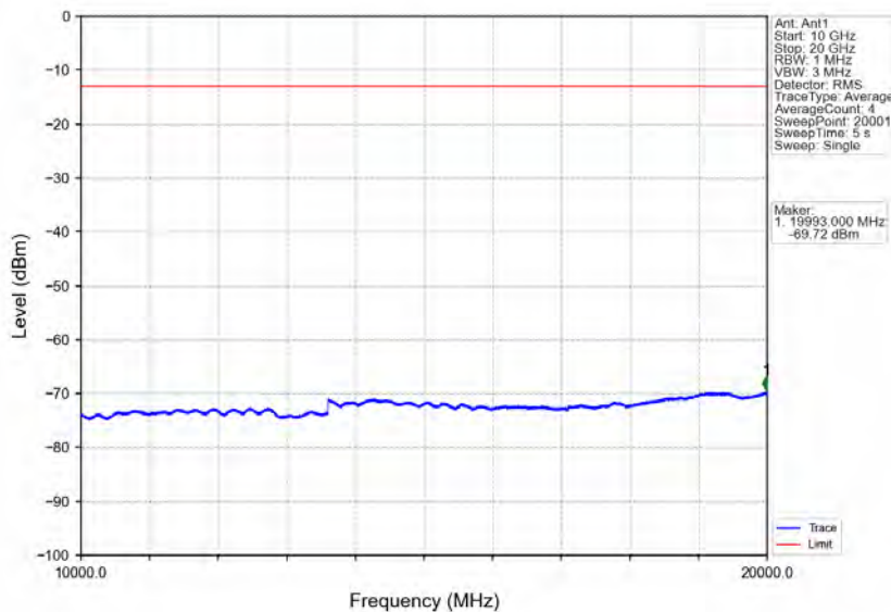
Band4_3MHz_16QAM_MCH_1732.5MHz_RB_1_0_NTNV
