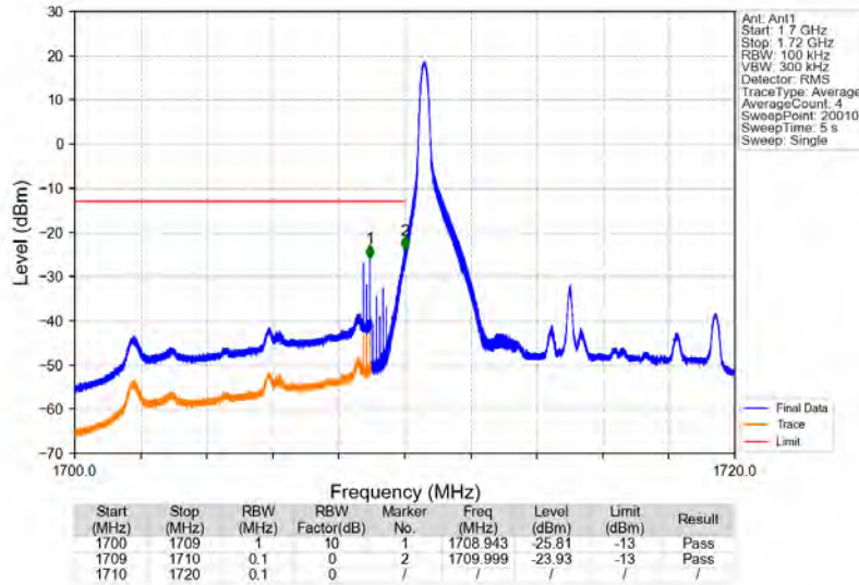
Band4_10MHz_16QAM_LCH_1715MHz_RB_1_0_NTNV
