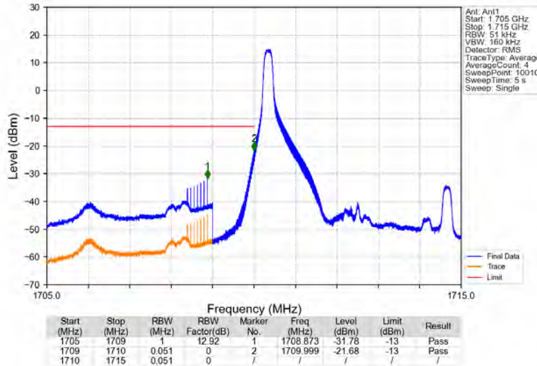
Band4_5MHz_64QAM_LCH_1712.5MHz_RB_1_0_NTNV
