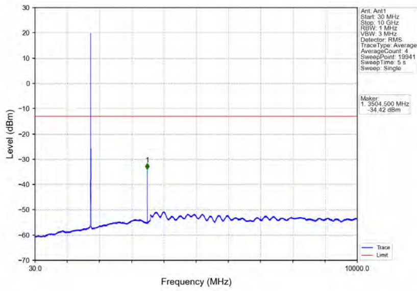
Band4_3MHz_16QAM_HCH_1753.5MHz_RB_1_0_NTNV
