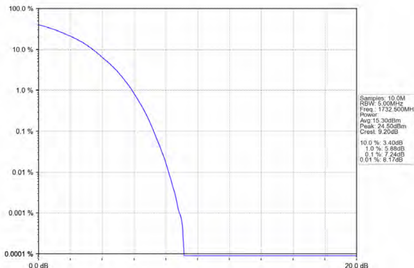
Band4_15MHz_64QAM_MCH_1732.5MHz_RB_75_0_NTNV
