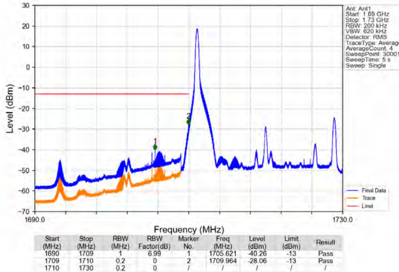
Band4_20MHz_64QAM_LCH_1720MHz_RB_1_0_NTNV
