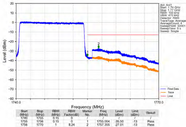
Band4_15MHz_64QAM_HCH_1747.5MHz_RB_75_0_NTNV
