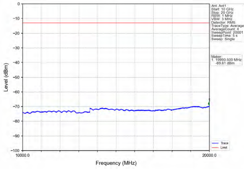
Band4_10MHz_64QAM_HCH_1750MHz_RB_1_0_NTNV
