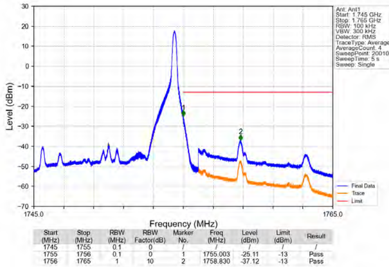
Band4_10MHz_64QAM_HCH_1750MHz_RB_1_49_NTV
