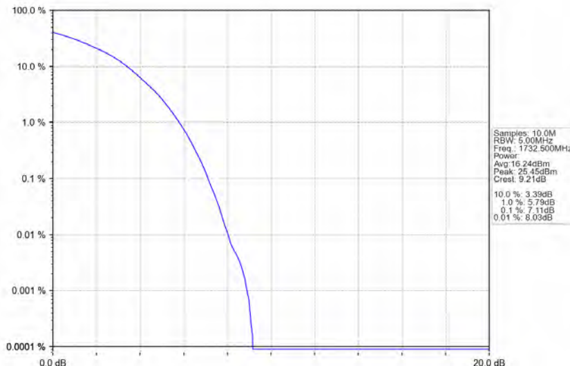
Band4_15MHz_16QAM_MCH_1732.5MHz_RB_75_0_NTNV
