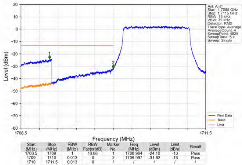
Band4_1.4MHz_QPSK_LCH_1710.7MHz_RB_6_0_NTV
