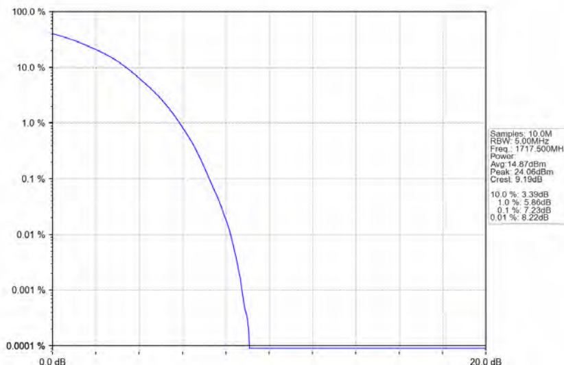
Band4_15MHz_64QAM_LCH_1717.5MHz_RB_75_0_NTNV
