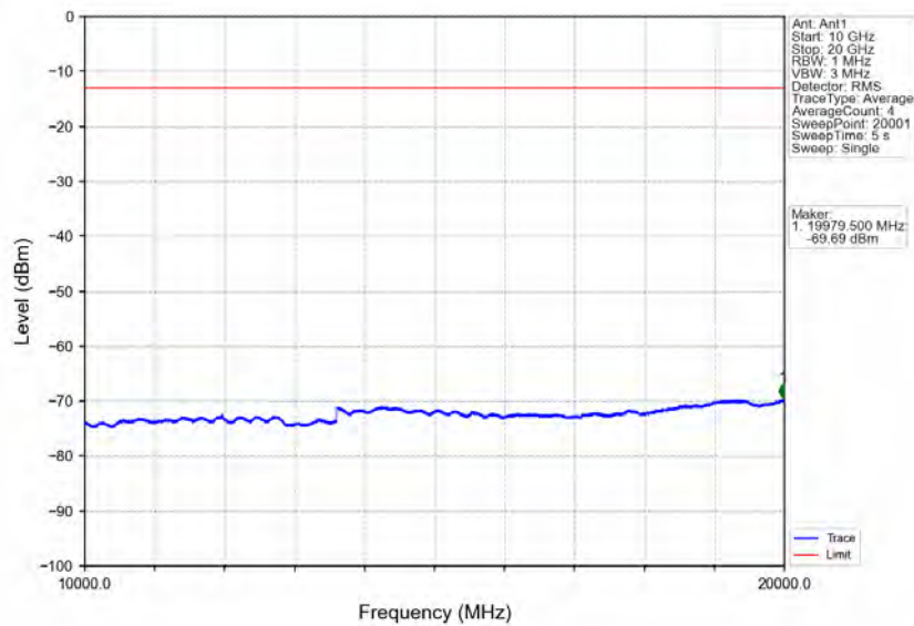
Band4_1.4MHz_QPSK_LCH_1710.7MHz_RB_6_0_NTV
