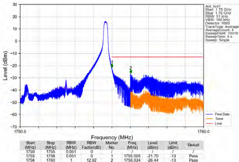
Band4_5MHz_16QAM_HCH_1752.5MHz_RB_1_24_NTNV
