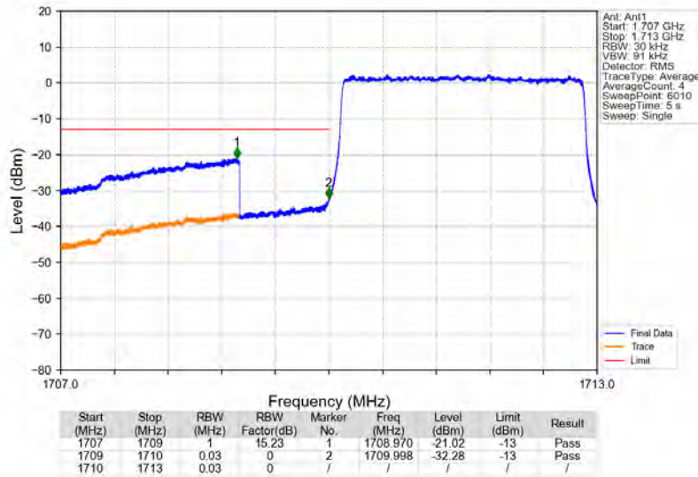
Band4_3MHz_QPSK_LCH_1711.5MHz_RB_15_0_NTNV
