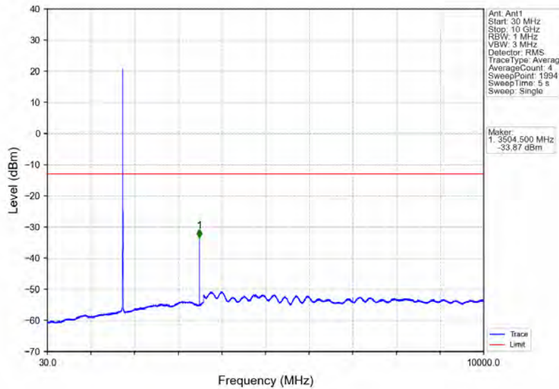
Band4_3MHz_QPSK_HCH_1753.5MHz_RB_1_0_NTNV
