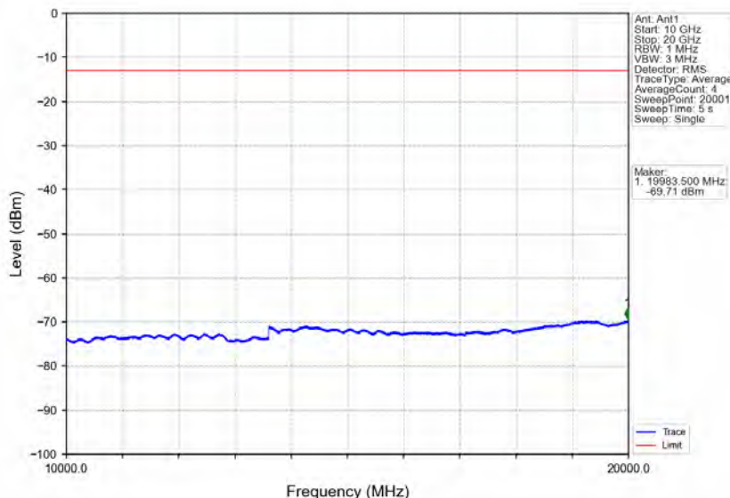
Band2_5MHz_16QAM_MCH_1880MHz_RB_1_0_NTNV
