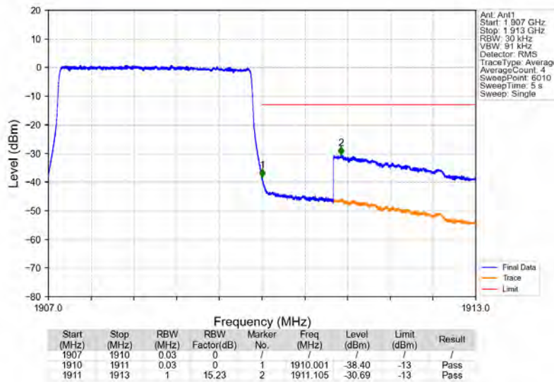
Band2_3MHz_64QAM_HCH_1908.5MHz_RB_15_0_NTNV
