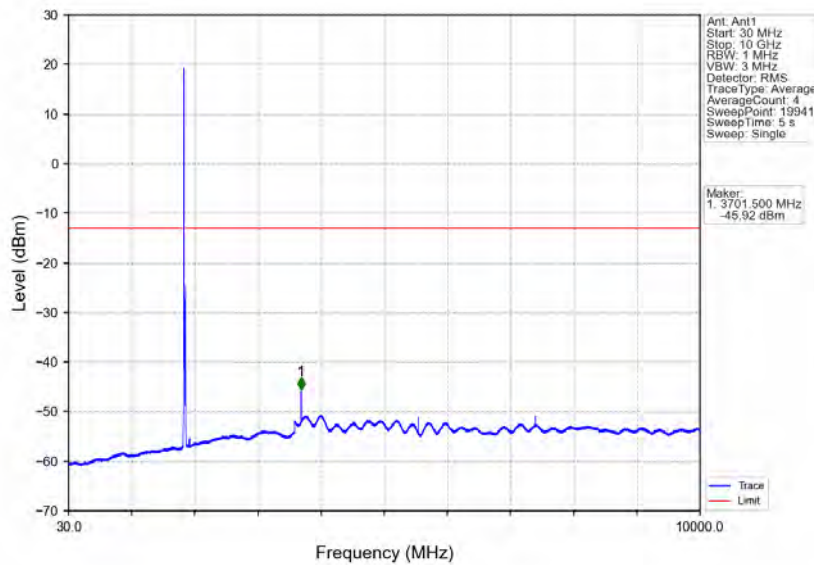
Band2_15MHz_64QAM_LCH_1857.5MHz_RB_1_0_NTV
