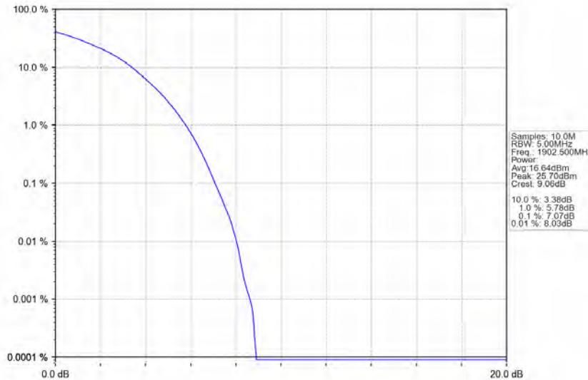
Band2_15MHz_16QAM_HCH_1902.5MHz_RB_75_0_NTNV
