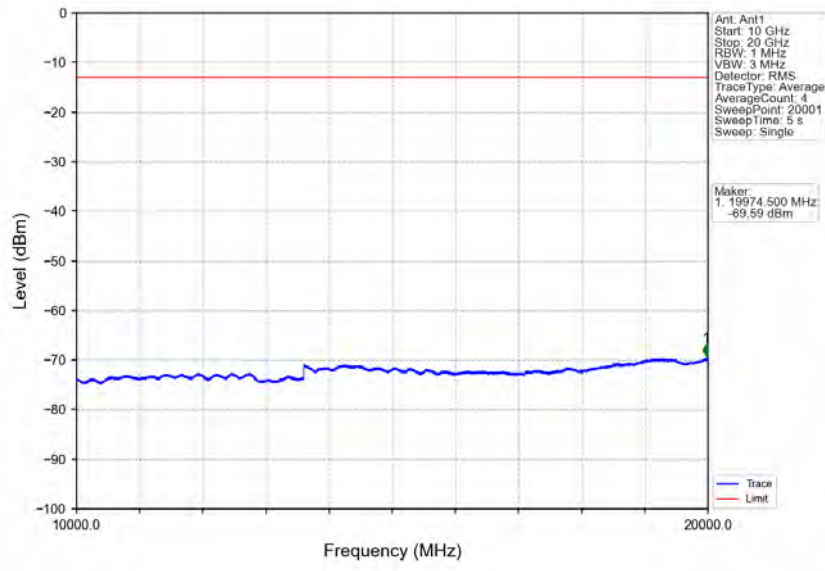
Band2_1.4MHz_64QAM_HCH_1909.3MHz_RB_1_0_NTNV
