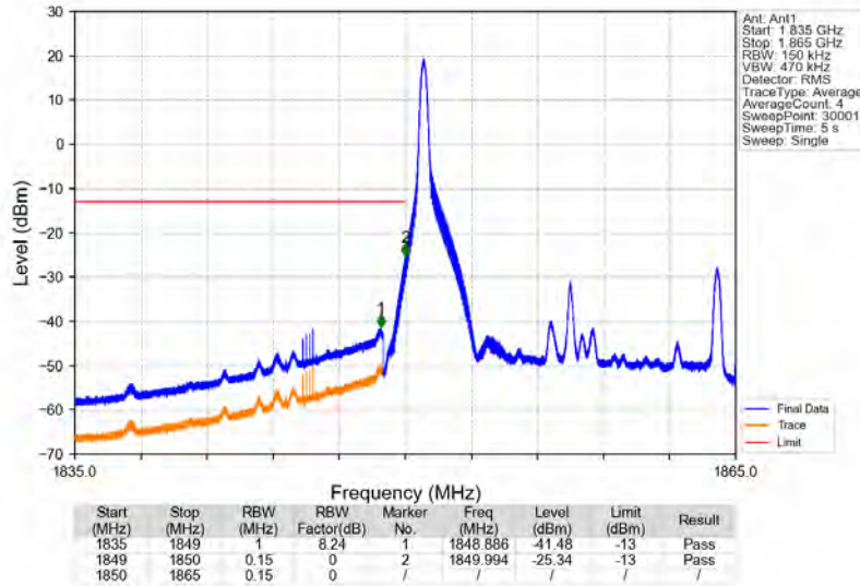
Band2_15MHz_64QAM_LCH_1857.5MHz_RB_1_0_NTV
