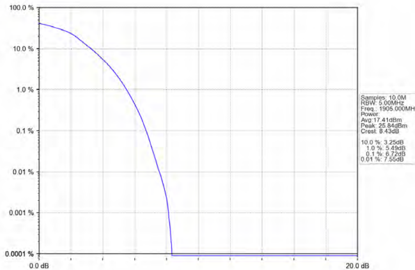
Band2_10MHz_64QAM_HCH_1905MHz_RB_50_0_NTV
