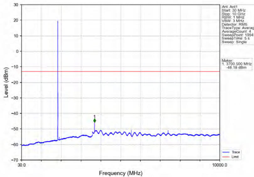
Band2_5MHz_64QAM_LCH_1852.5MHz_RB_1_0_NTNV
