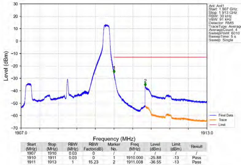
Band2_3MHz_64QAM_HCH_1908.5MHz_RB_1_14_NTNV
