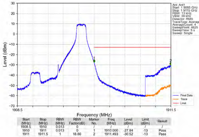
Band2_1.4MHz_64QAM_HCH_1909.3MHz_RB_1_5_NTNV
