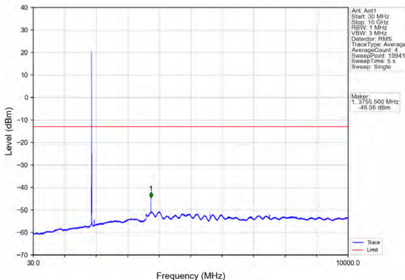
Band2_5MHz_16QAM_MCH_1880MHz_RB_1_0_NTNV
