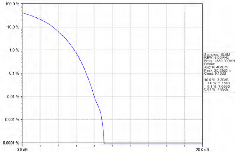
Band2_15MHz_16QAM_MCH_1880MHz_RB_75_0_NTNV
