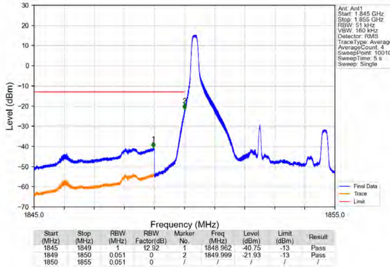
Band2_5MHz_64QAM_LCH_1852.5MHz_RB_1_0_NTNV
