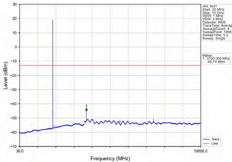
Band2_3MHz_64QAM_LCH_1851.5MHz_RB_1_0_NTNV
