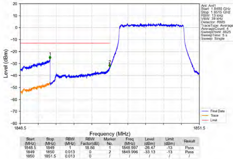
Band2_1.4MHz_QPSK_LCH_1850.7MHz_RB_6_0_NTV
