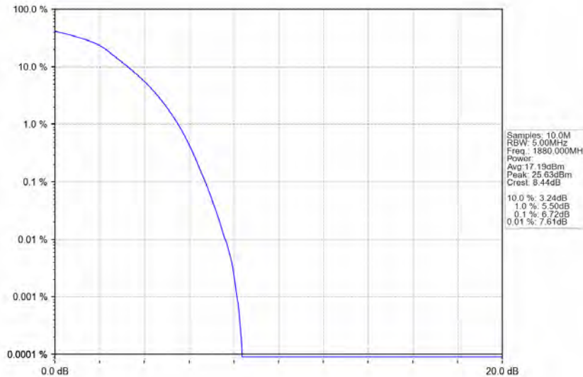
Band2_10MHz_64QAM_MCH_1880MHz_RB_50_0_NTNV
