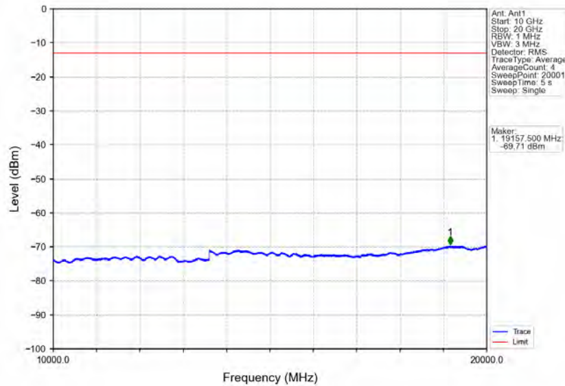
Band2_5MHz_16QAM_LCH_1852.5MHz_RB_25_0_NTNV
