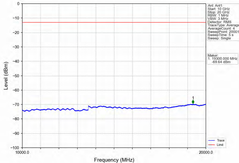
Band2_1.4MHz_16QAM_HCH_1909.3MHz_RB_1_0_NTNV
