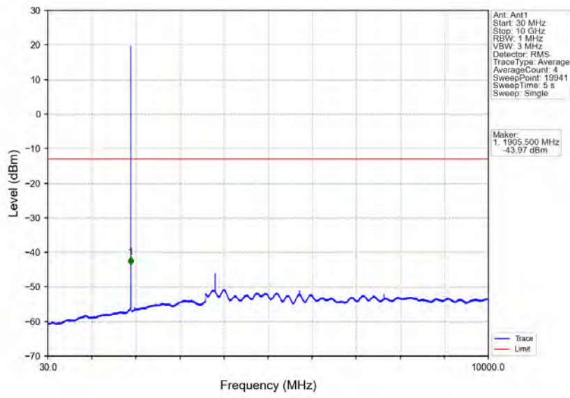
Band2_1.4MHz_64QAM_HCH_1909.3MHz_RB_1_0_NTNV
