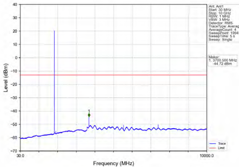
Band2_3MHz_16QAM_LCH_1851.5MHz_RB_1_0_NTNV
