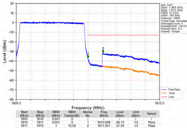
Band2_5MHz_64QAM_HCH_1907.5MHz_RB_25_0_NTNV
