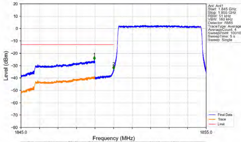
Band2_5MHz_QPSK_LCH_1852.5MHz_RB_25_0_NTNV
