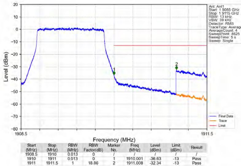
Band2_1.4MHz_64QAM_HCH_1909.3MHz_RB_6_0_NTNV
