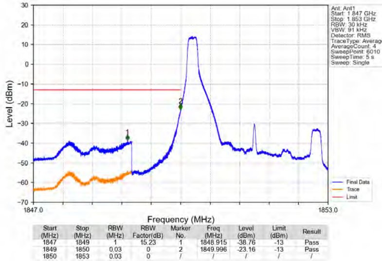
Band2_3MHz_16QAM_LCH_1851.5MHz_RB_1_0_NTNV
