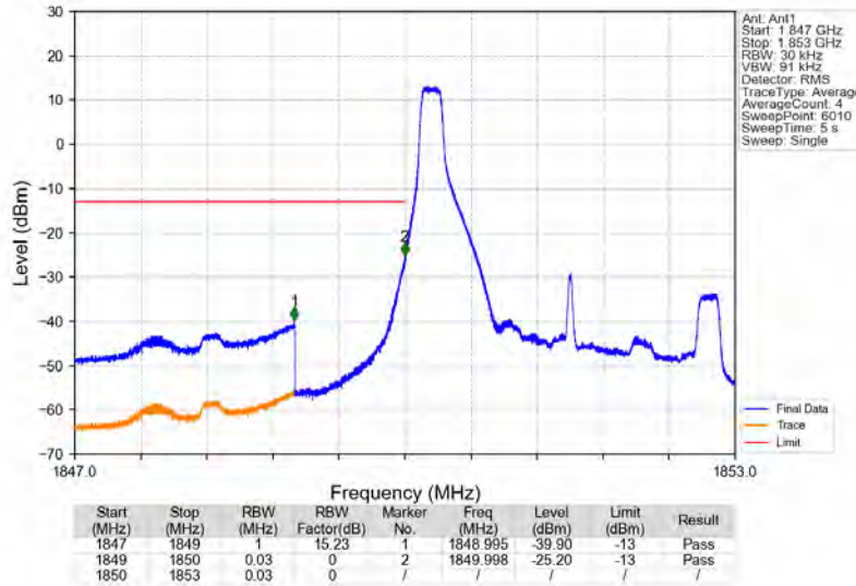
Band2_3MHz_64QAM_LCH_1851.5MHz_RB_1_0_NTNV
