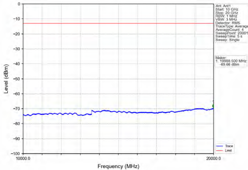
Band2_1.4MHz_QPSK_LCH_1850.7MHz_RB_6_0_NTV
