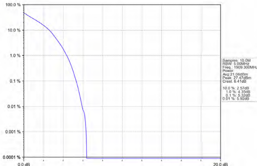
Band2_1.4MHz_QPSK_HCH_1909.3MHz_RB_6_0_NTNV
