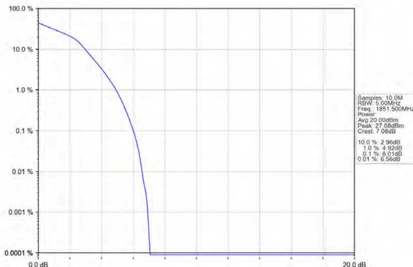
Band2_3MHz_16QAM_LCH_1851.5MHz_RB_15_0_NTNV
