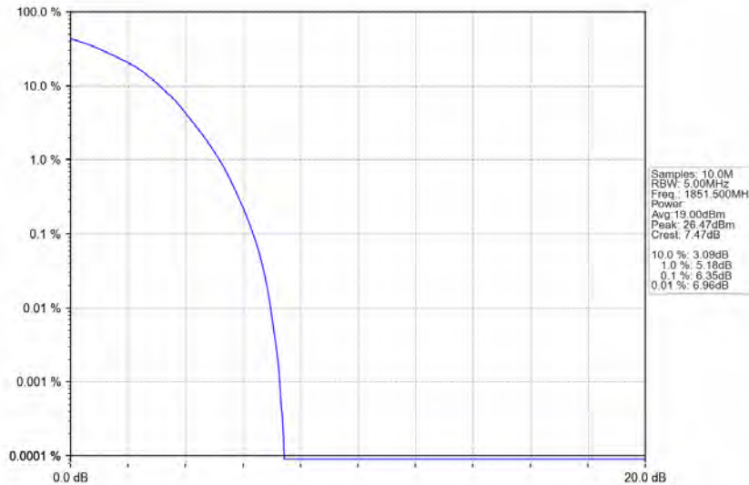
Band2_3MHz_64QAM_LCH_1851.5MHz_RB_15_0_NTNV
