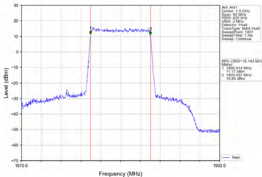
Band2_20MHz_64QAM_HCH_1900MHz_RB_100_0_NTNV
