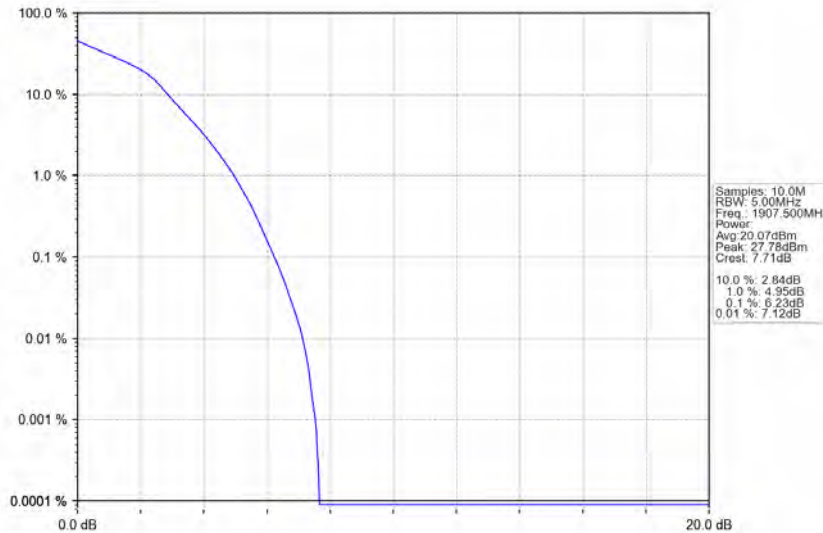
Band2_5MHz_16QAM_HCH_1907.5MHz_RB_25_0_NTNV
