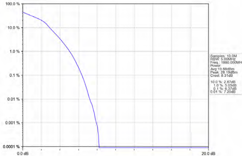
Band2_5MHz_16QAM_MCH_1880MHz_RB_25_0_NTNV
