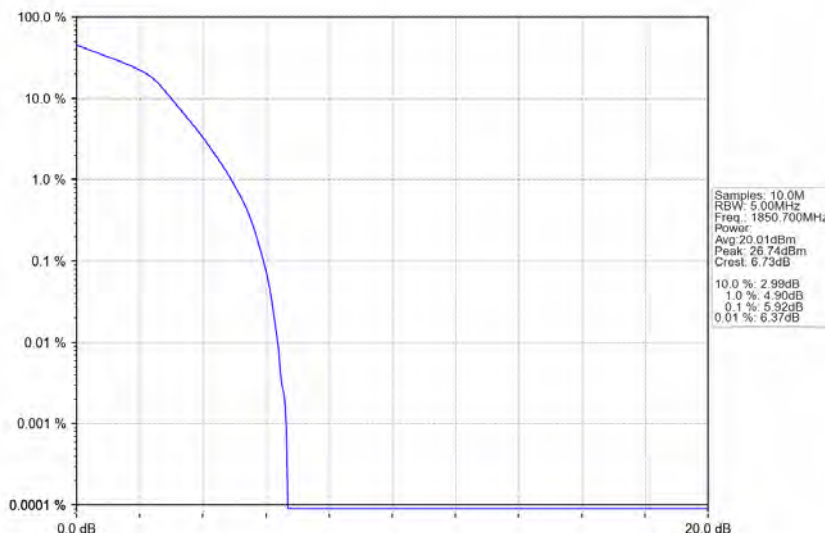
Band2_1.4MHz_16QAM_LCH_1850.7MHz_RB_6_0_NTNV
