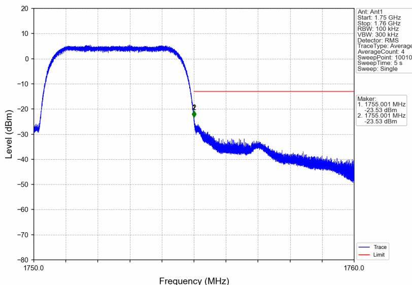
Band4_HSUPA_HCH_1752.6MHz_Subtest 1_NTNV
