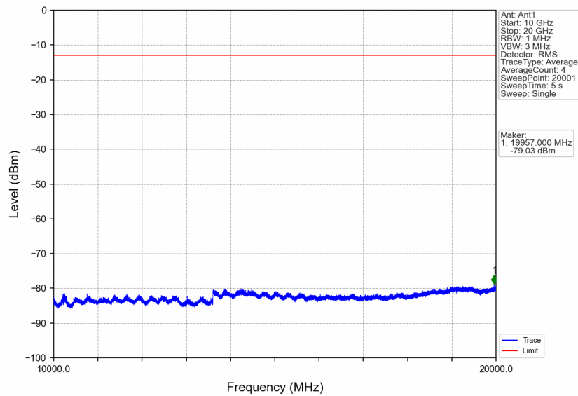
Band4_HSUPA_HCH_1752.6MHz_Subtest 1_NTNV
