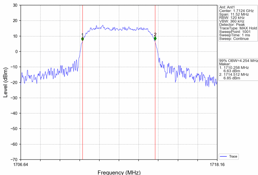
Band4_HSDPA_LCH_1712.4MHz_Subtest 1_NTNV
