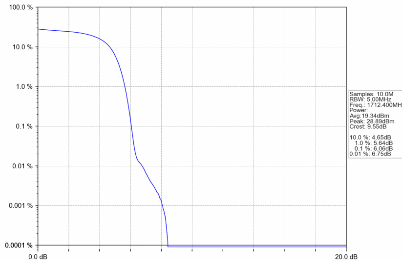
Band4_HSDPA_LCH_1712.4MHz_Subtest 1_NTNV
