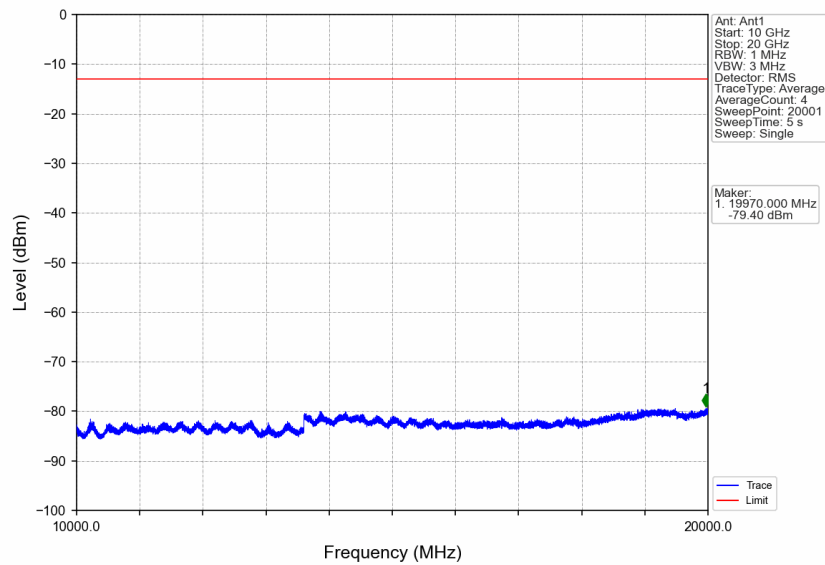
Band4_RMC_HCH_1752.6MHz_12.2kbps RMC_NTNV
