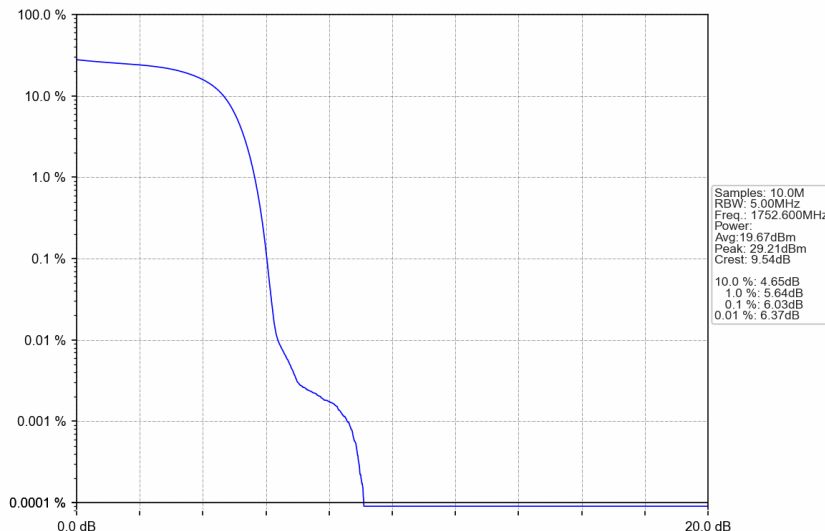
Band4_HSUPA_HCH_1752.6MHz_Subtest 1_NTNV
