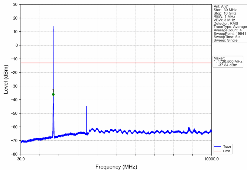
Band4_HSUPA_MCH_1732.6MHz_Subtest 1_NTNV
