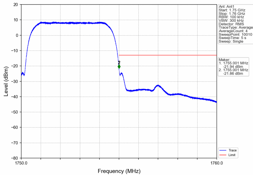
Band4_RMC_HCH_1752.6MHz_12.2kbps RMC_NTNV
