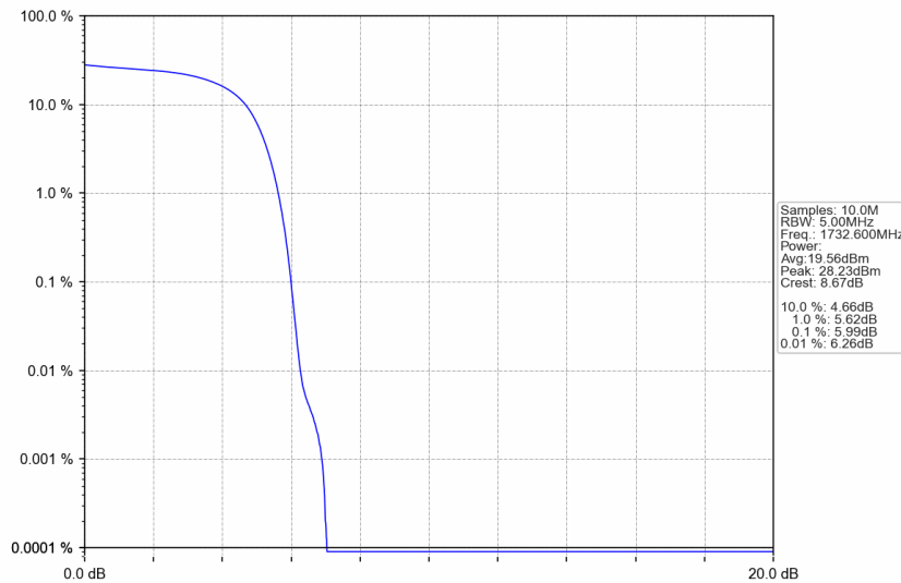
Band4_HSDPA_MCH_1732.6MHz_Subtest 1_NTV
