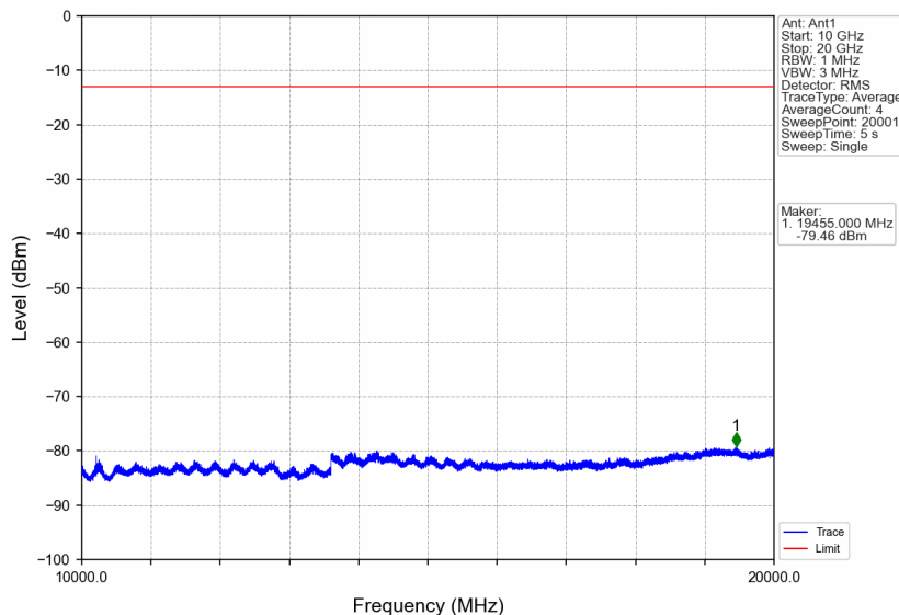
Band4_HSUPA_HCH_1752.6MHz_Subtest 1_NTNV
