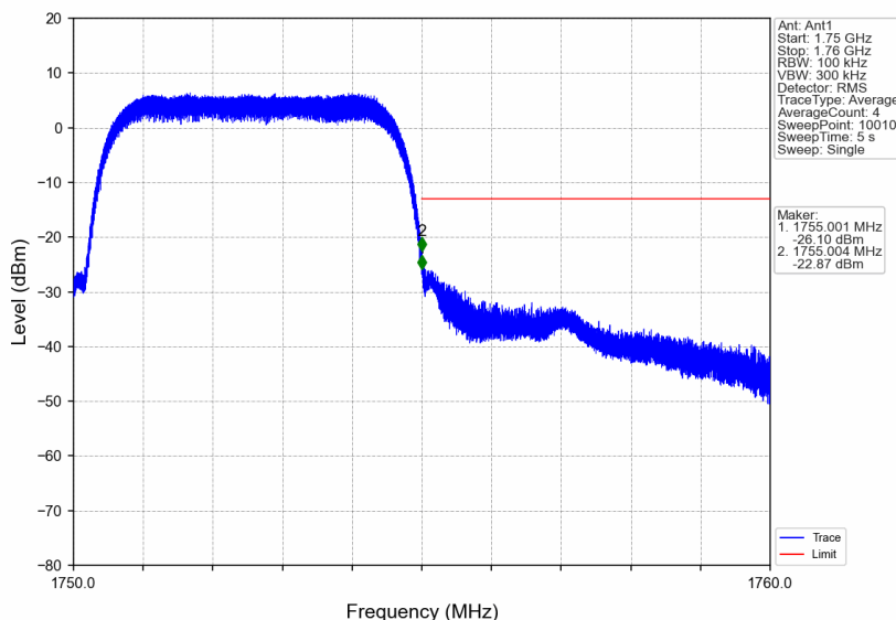
Band4_HSDPA_HCH_1752.6MHz_Subtest 1_NTNV
