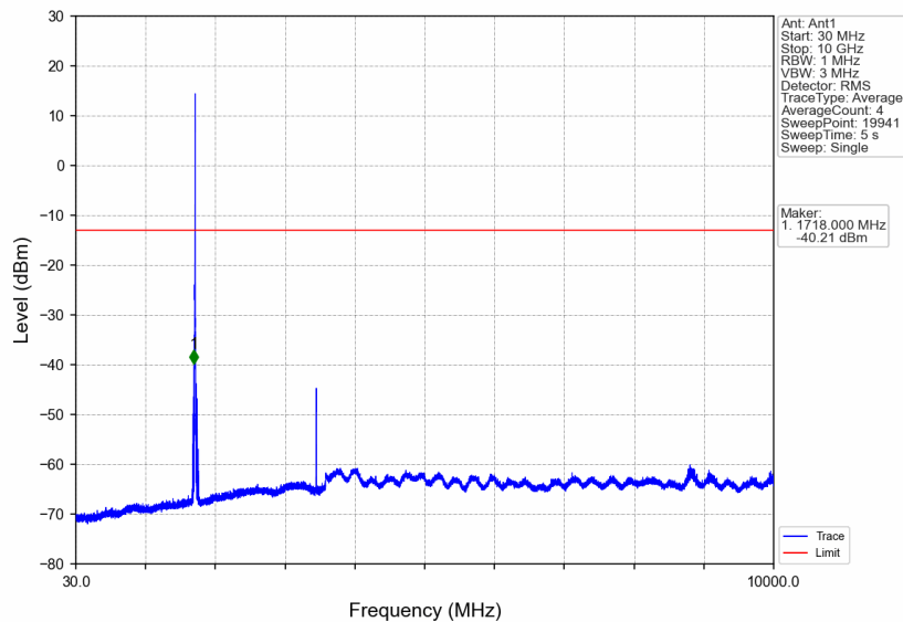
Band4_HSDPA_MCH_1732.6MHz_Subtest 1_NTNV
