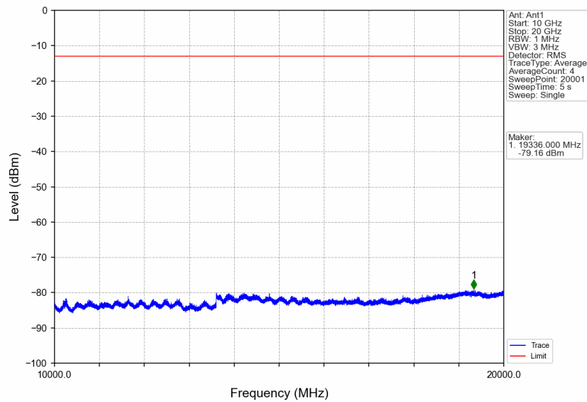
Band4_HSUPA_MCH_1732.6MHz_Subtest 1_NTNV
