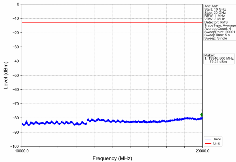
Band4_HSDPA_MCH_1732.6MHz_Subtest 1_NTNV
