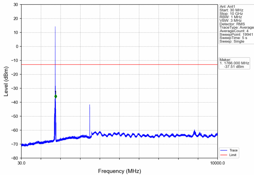
Band4_HSUPA_HCH_1752.6MHz_Subtest 1_NTNV
