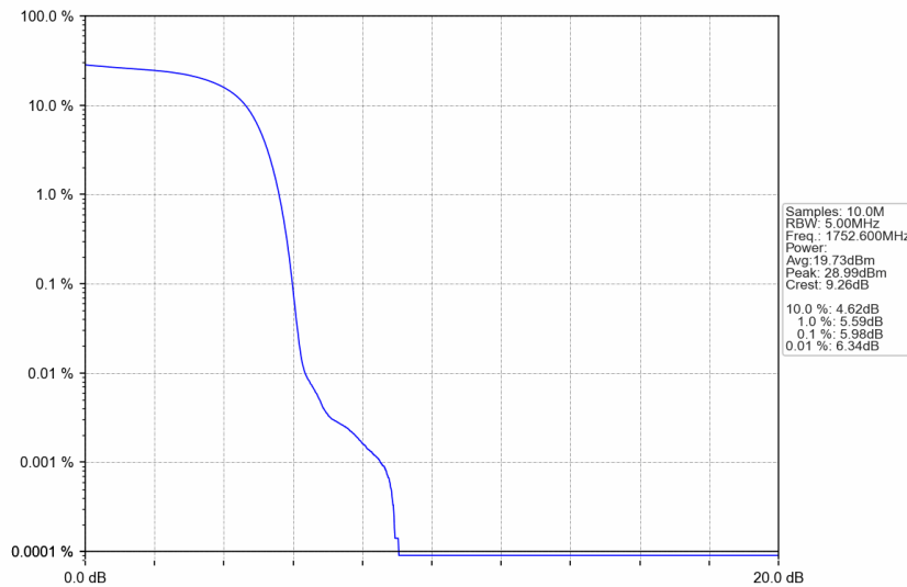
Band4_HSDPA_HCH_1752.6MHz_Subtest 1_NTV
