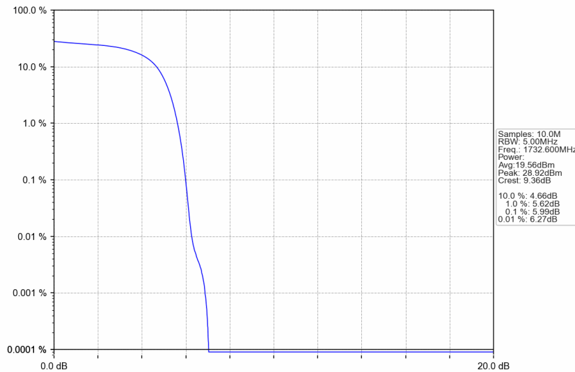
Band4_HSUPA_MCH_1732.6MHz_Subtest 1_NTNV
