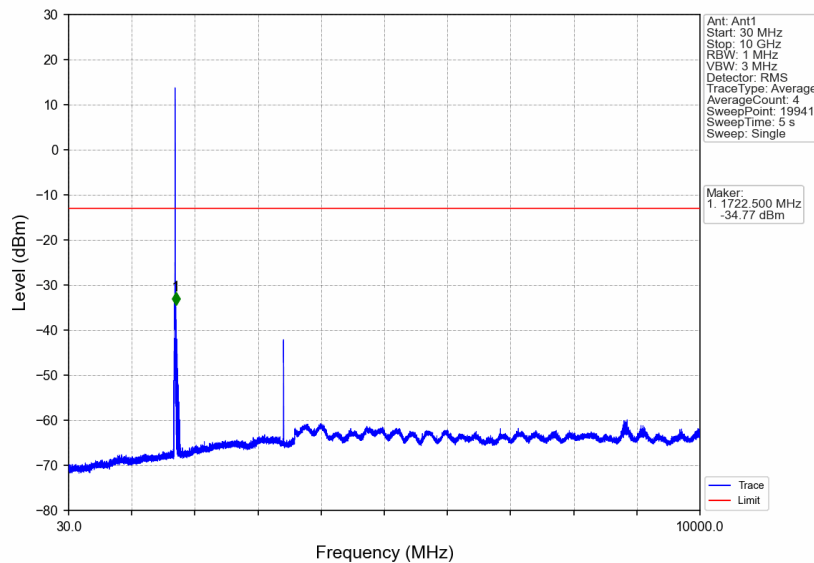
Band4_HSDPA_LCH_1712.4MHz_Subtest 1_NTNV
