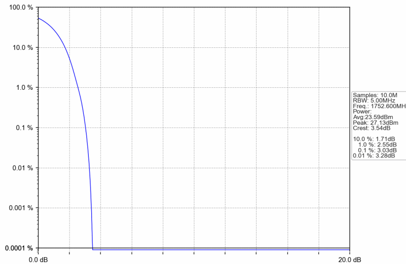
Band4_RMC_HCH_1752.6MHz_12.2kbps RMC_NTNV
