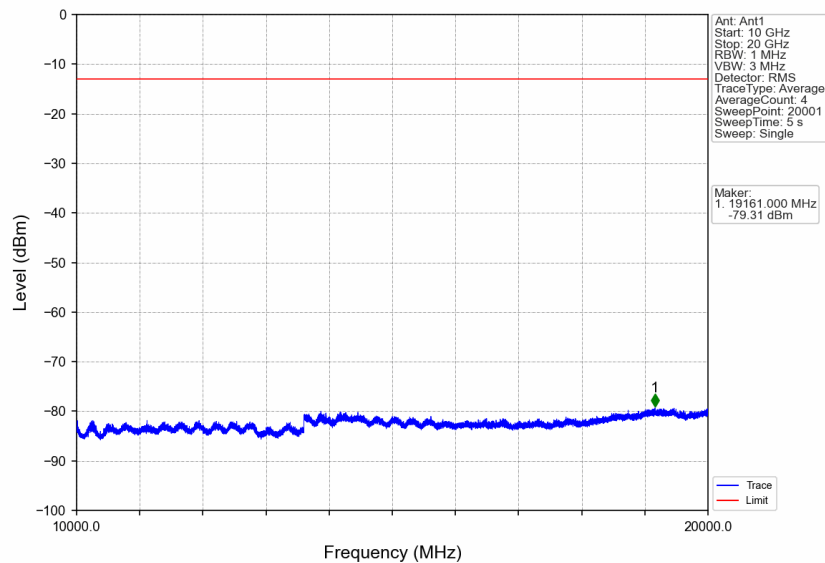
Band4_HSDPA_HCH_1752.6MHz_Subtest 1_NTNV
