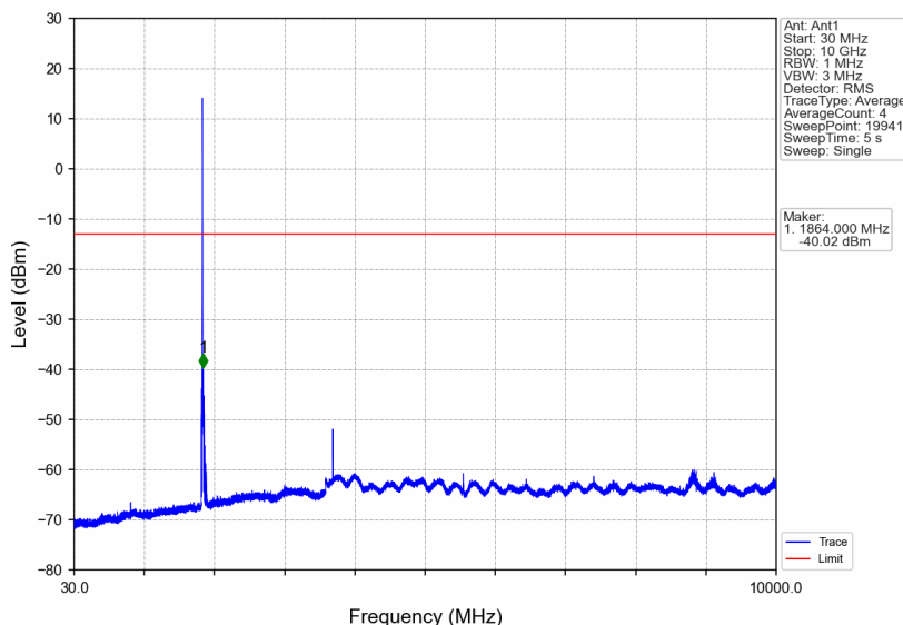
Band2_HSUPA_LCH_1852.4MHz_Subtest 1_NTNV
