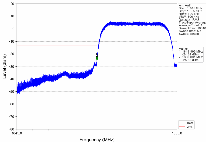
Band2_HSUPA_LCH_1852.4MHz_Subtest 1_NTNV
