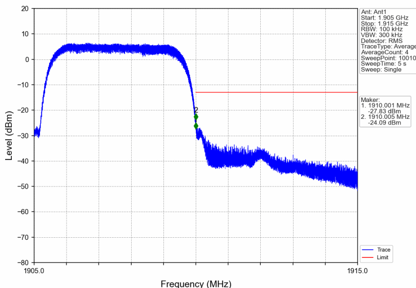
Band2_HSDPA_HCH_1907.6MHz_Subtest 1_NTNV
