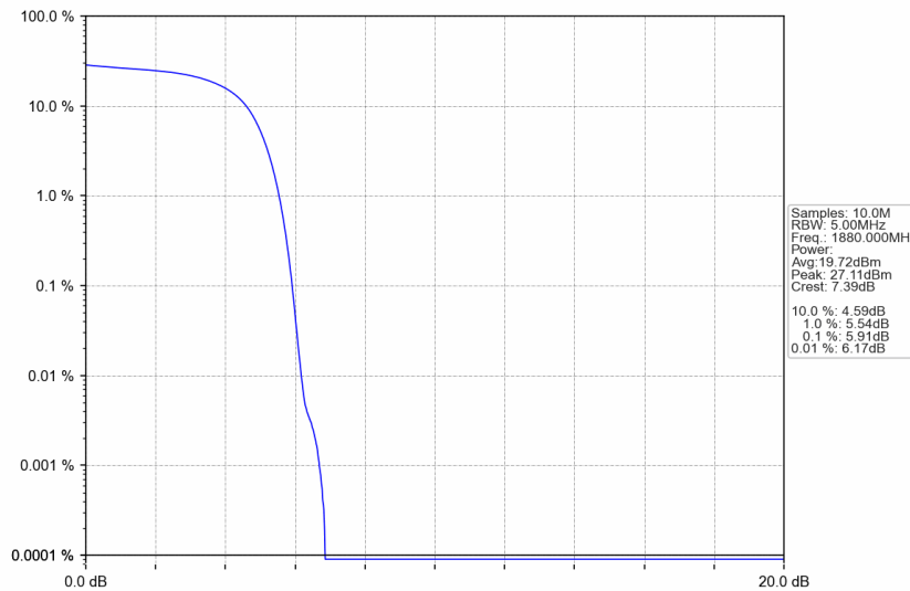
Band2_HSDPA_MCH_1880MHz_Subtest 1_NTNV
