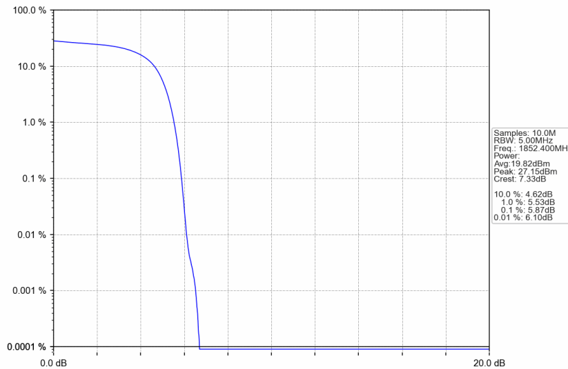
Band2_HSDPA_LCH_1852.4MHz_Subtest 1_NTNV
