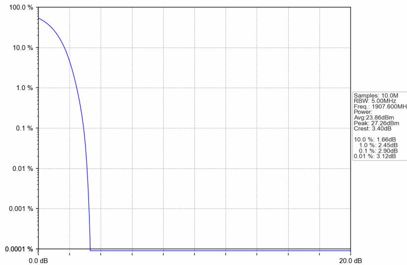
Band2_RMC_HCH_1907.6MHz_12.2kbps RMC_NTNV
