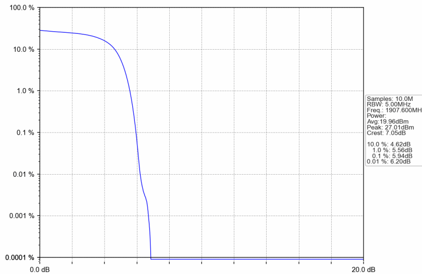
Band2_HSDPA_HCH_1907.6MHz_Subtest 1_NTNV
