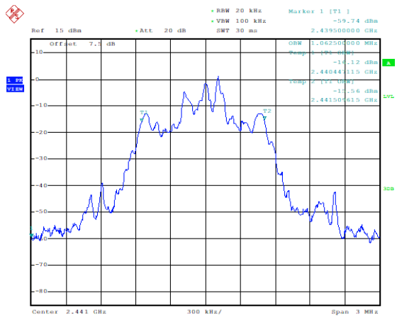
99% Bandwidth: DQPSK, Ch39
