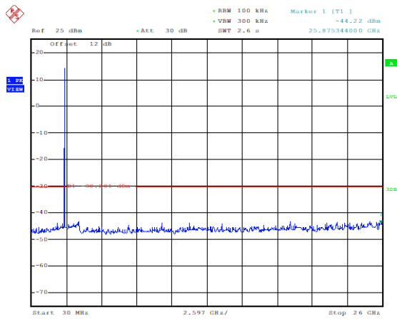
Conducted spurious emission: GFSK, Ch78, 30MHz~26GHz
