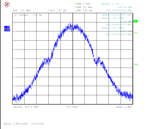
Channel 189-Occupied Bandwidth (99%)
