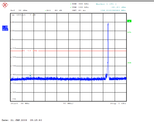
Channel 4175: 30MHz~1GHz
