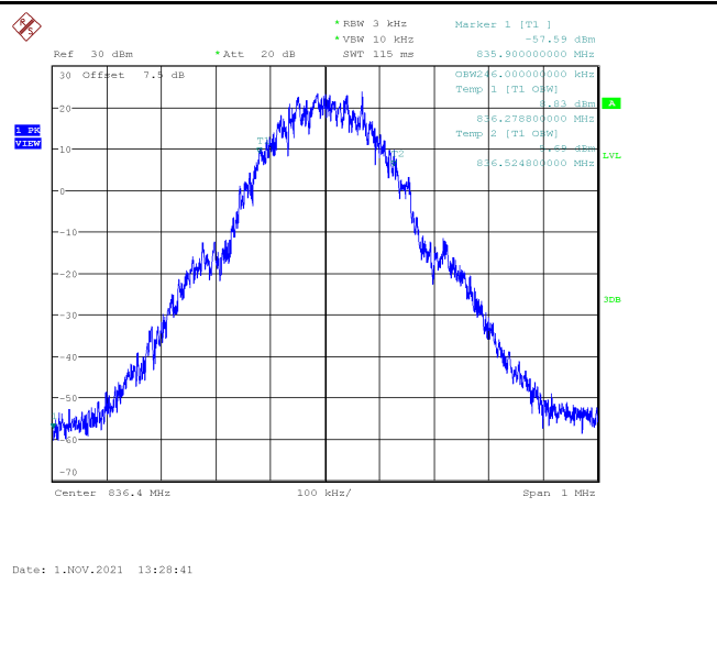
Channel 189-Occupied Bandwidth (99%)
