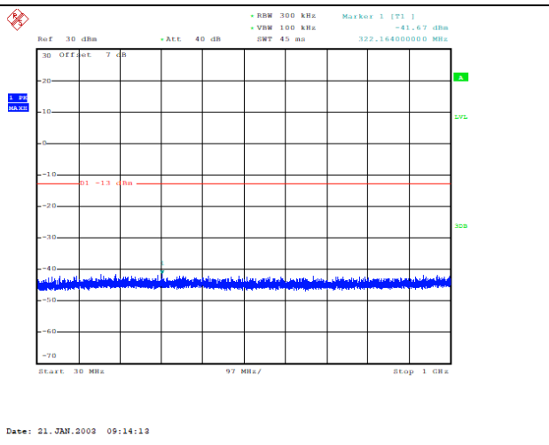
Channel 1450: 30MHz~1GHz
