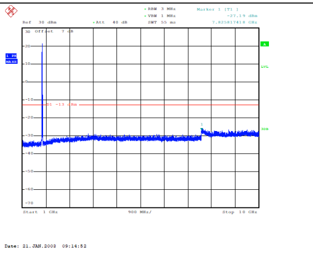
Channel 1450: 1GHz~10GHz
