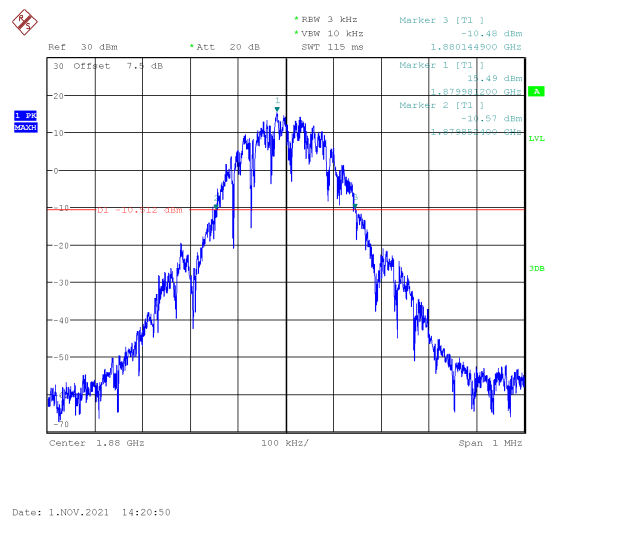
Channel 881- Emission Bandwidth (-26dBc BW)
