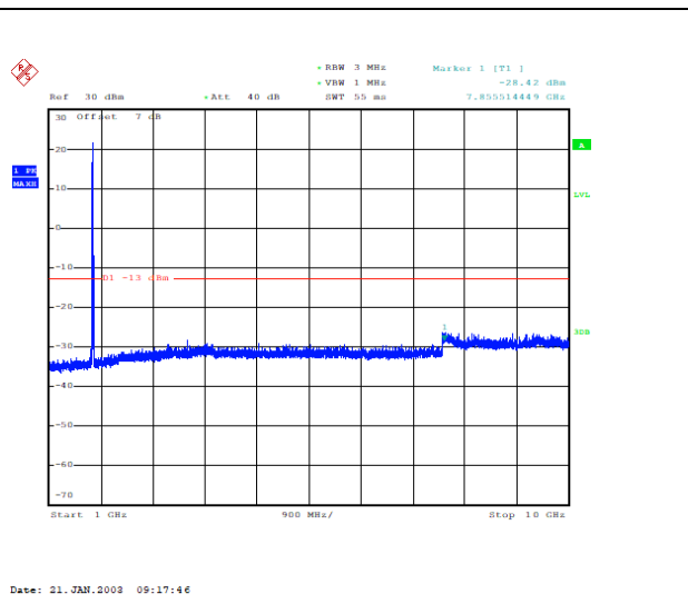
Channel 1512: 1GHz~10GHz
