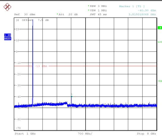
Channel 810: 1GHz~8GHz
