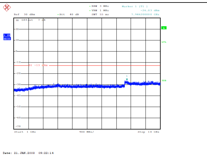
Channel 4232: 1GHz~10GHz
