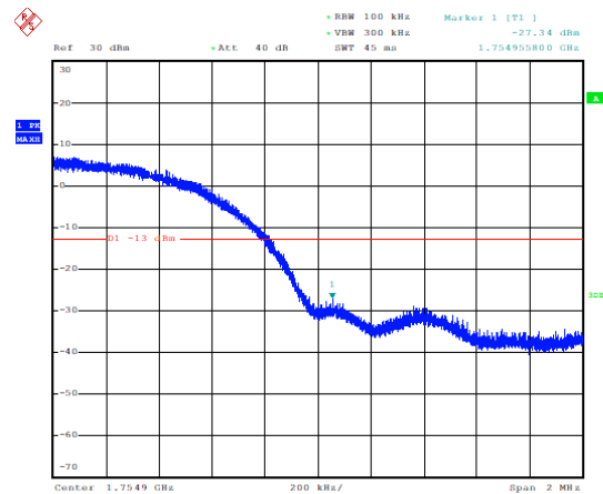
Channel 1512- HIGH BAND EDGE BLOCK
