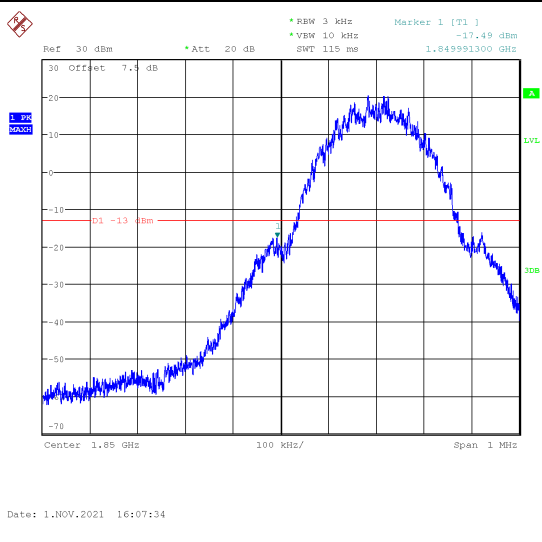
Channel 512- LOW BAND EDGE BLOCK
