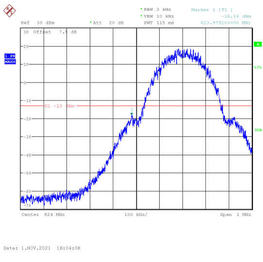
Channel 128- LOW BAND EDGE BLOCK
