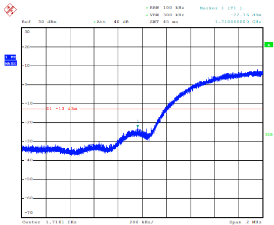
Channel 1313- LOW BAND EDGE BLOCK
