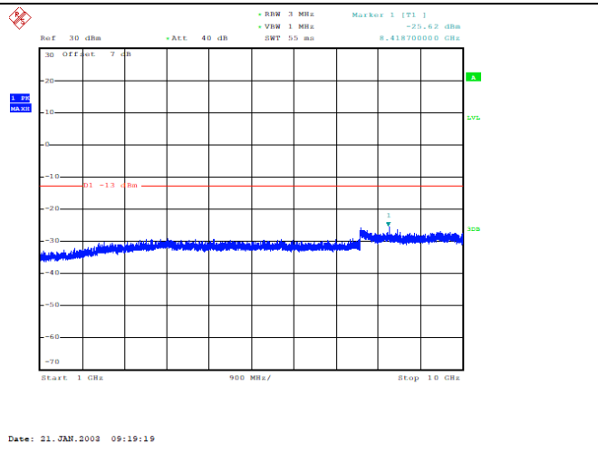
Channel 4175: 1GHz~10GHz
