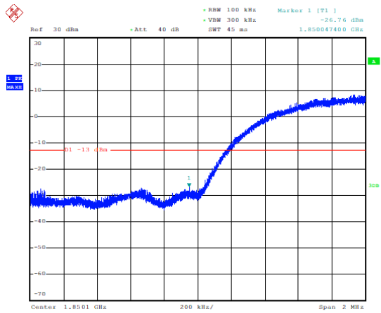
Channel 9263- LOW BAND EDGE BLOCK
