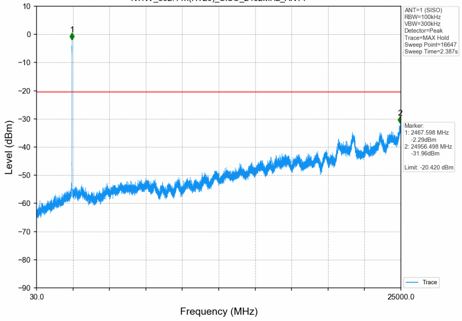
Unwanted Emissions in Non-restricted Frequency Bands NTNV_802.11n(HT20)_SISO_2462MHz_ANT1
