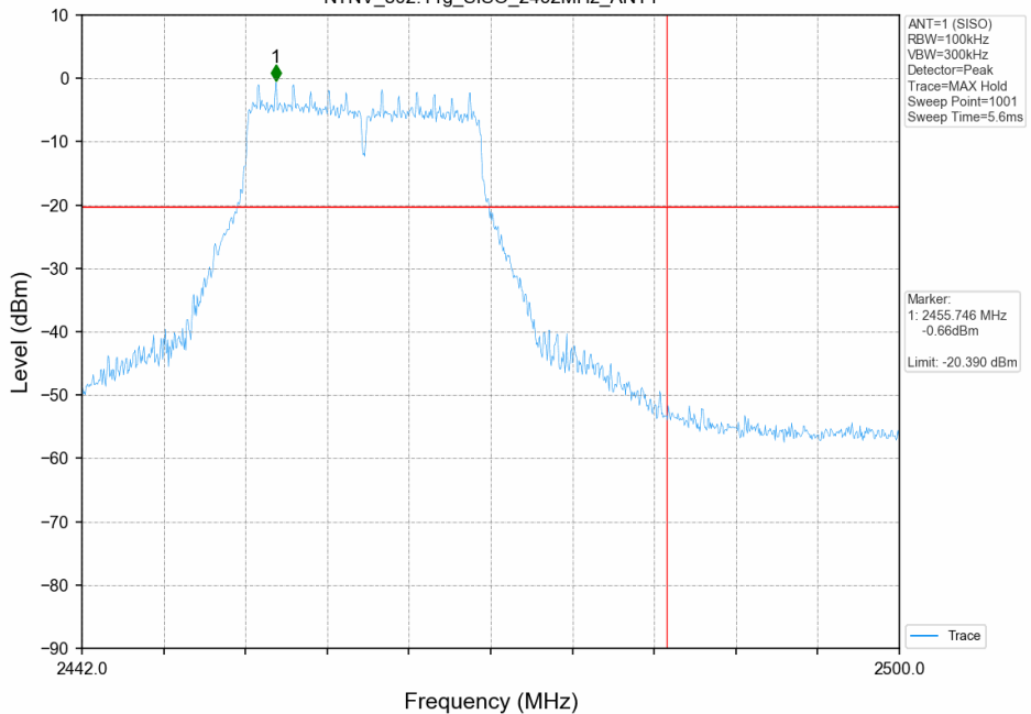
Unwanted Emissions in Non-restricted Frequency Bands NTNV_802.11g_SISO_2462MHz_ANT1
