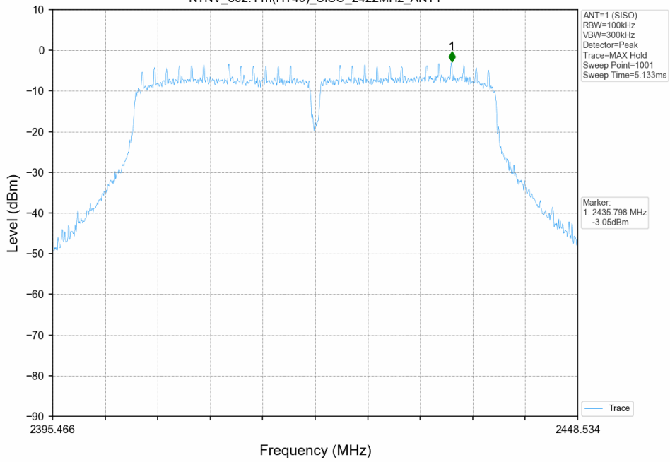
Unwanted Emissions in Non-restricted Frequency Bands NTNV_802.11n(HT40)_SISO_2422MHz_ANT1
