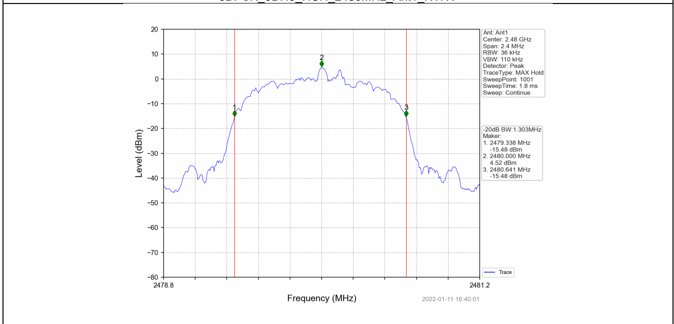
8DPSK_3DH5_HCH_2480MHz_Ant1_NTNV
