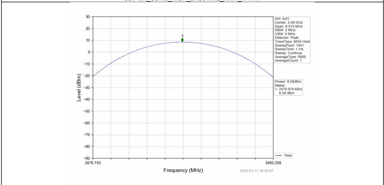
8DPSK_3DH5_HCH_2480MHz_Ant1_NTNV
