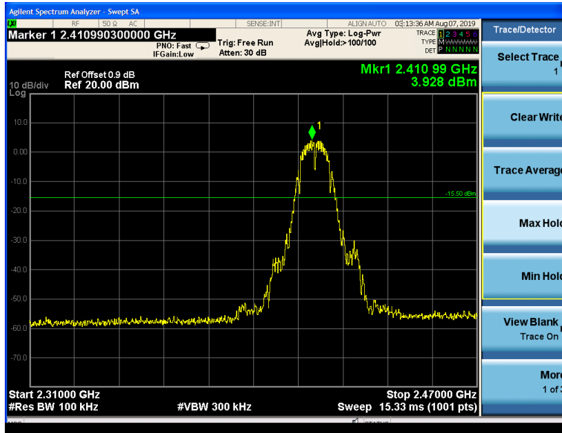
Fig 25. Band Edges (802.11b, Ch1)
