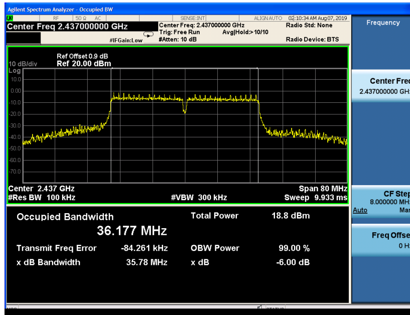
Fig 23. Occupied 6dB Bandwidth (802.11n-40MHz, Ch6)
