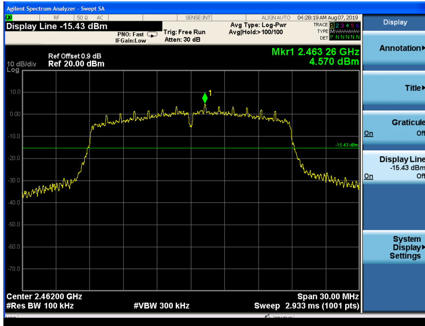
Fig 49. Conducted Spurious Emission (802.11n-20MHz, Ch11)
