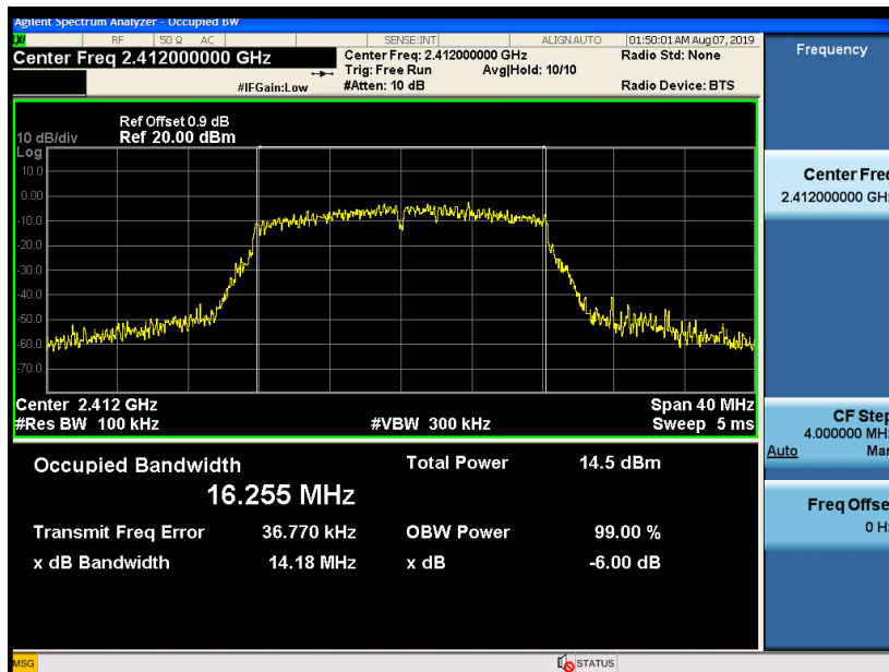
Fig 16. Occupied 6dB Bandwidth (802.11g, Ch1)
