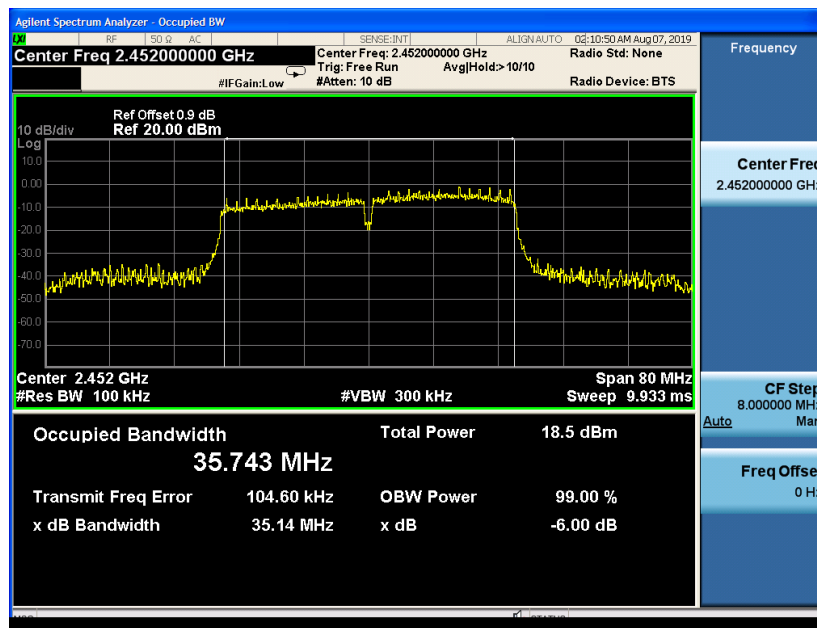
Fig 24. Occupied 6dB Bandwidth (802.11n-40MHz, Ch9)
