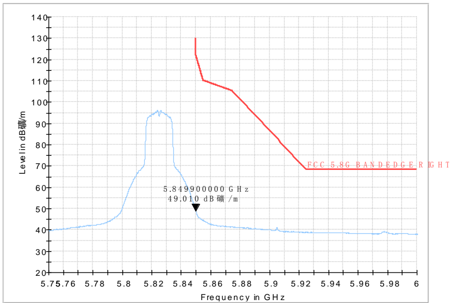
Average Fig. 45 Band Edges (802.11n-HT20, 5825MHz)
