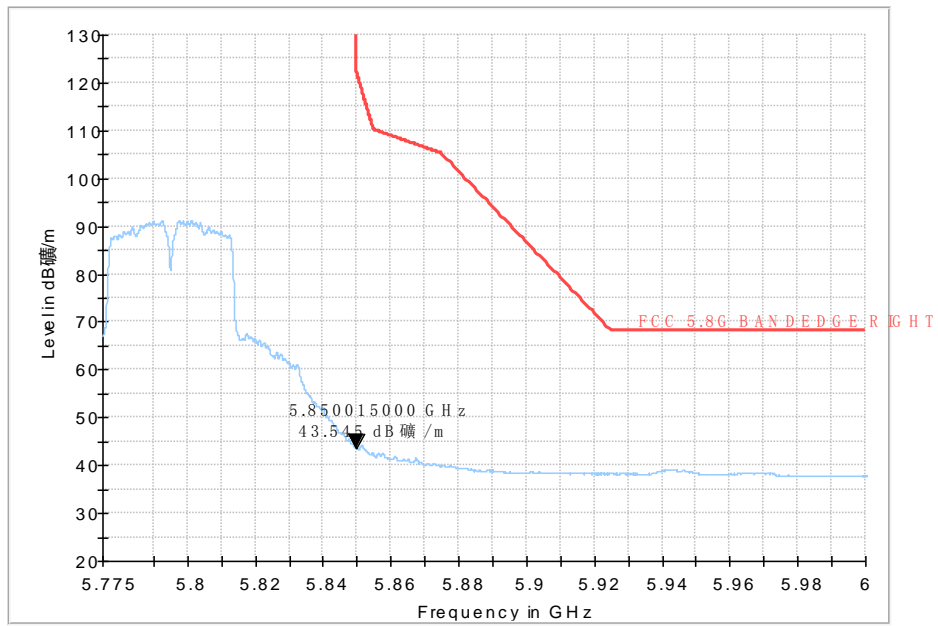
Average Fig. 47 Band Edges (802.11n-HT40, 5795MHz)
