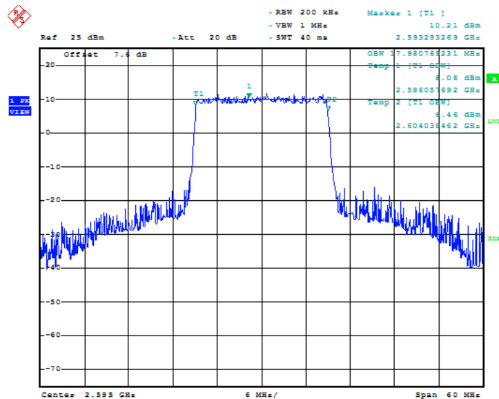
Fig.51 LTE band 41, 20MHz Bandwidth, QPSK (99% BW)
