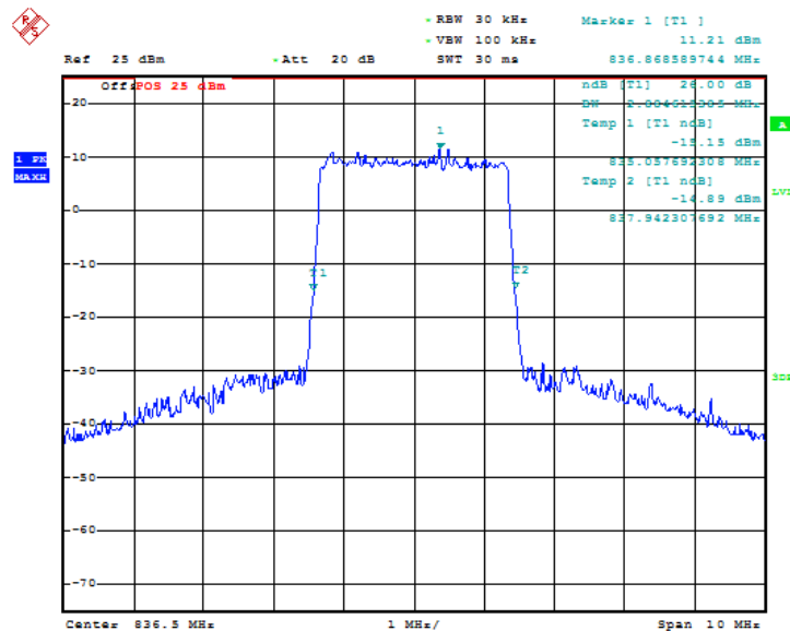
Fig.79 LTE band 5, 3MHz Bandwidth, QPSK (-26dBc BW)
