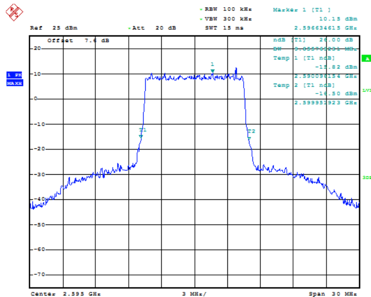
Fig.99 LTE band 41, 10MHz Bandwidth, QPSK (-26dBc BW)
