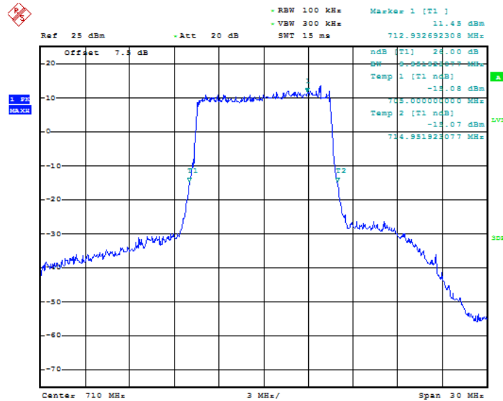
Fig.95 LTE band 17, 10MHz Bandwidth, QPSK (-26dBc BW)
