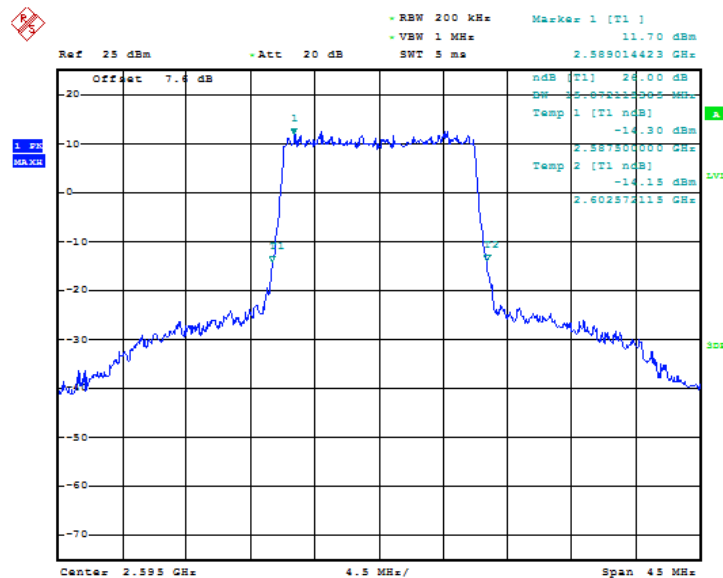
Fig.101 LTE band 41, 15MHz Bandwidth, QPSK (-26dBc BW)
