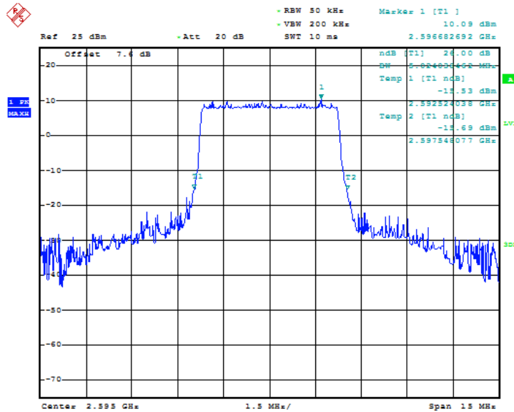
Fig.97 LTE band 41, 5MHz Bandwidth, QPSK (-26dBc BW)
