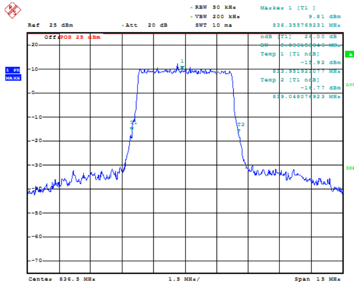
Fig.81 LTE band 5, 5MHz Bandwidth, QPSK (-26dBc BW)
