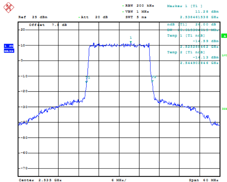
Fig.91 LTE band 7, 20MHz Bandwidth, QPSK (-26dBc BW)
