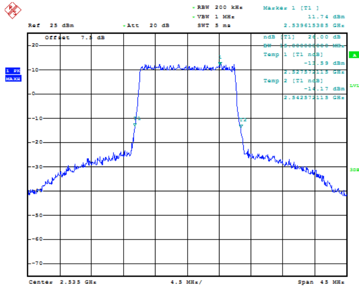
Fig.89 LTE band 7, 15MHz Bandwidth, QPSK (-26dBc BW)
