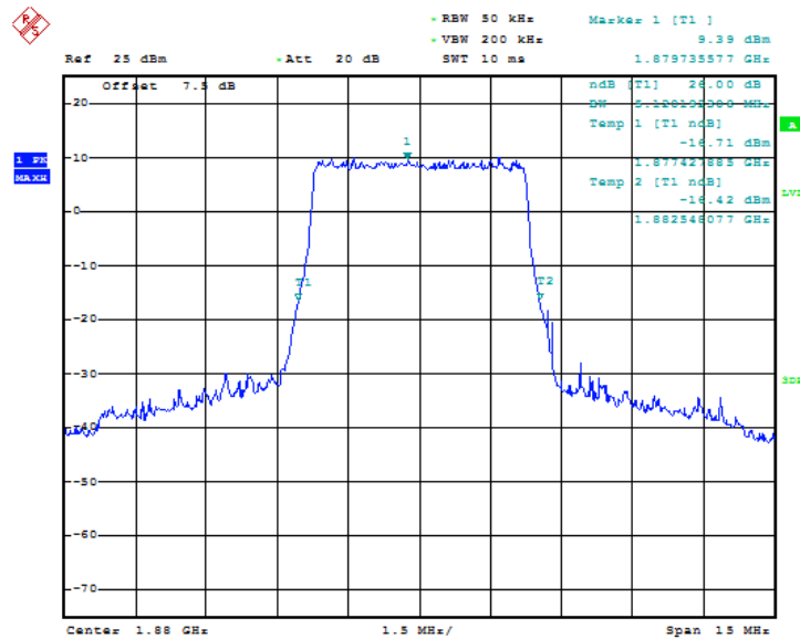
Fig.57 LTE band 2, 5MHz Bandwidth, QPSK (-26dBc BW)
