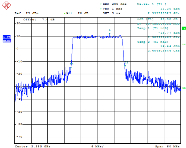
Fig.103 LTE band 41, 20MHz Bandwidth, QPSK (-26dBc BW)
