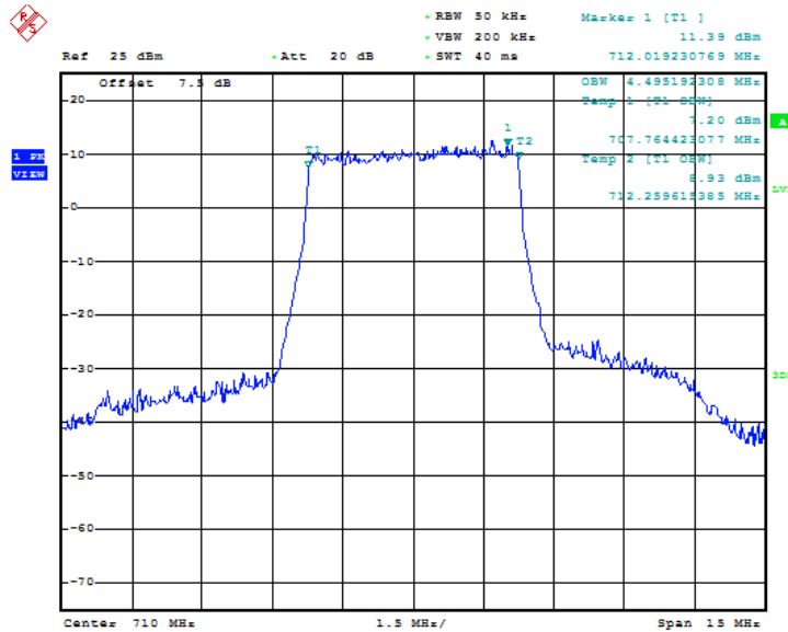
Fig.41 LTE band 17, 5MHz Bandwidth, QPSK (99% BW)
