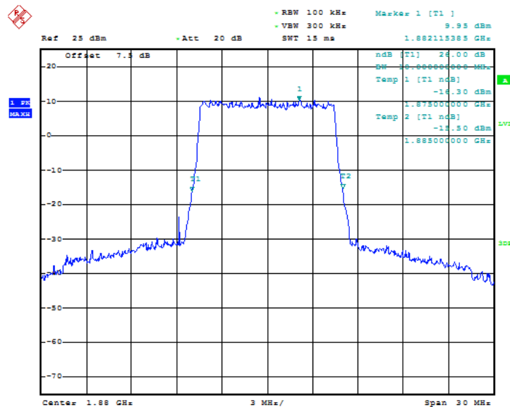
Fig.59 LTE band 2, 10MHz Bandwidth, QPSK (-26dBc BW)
