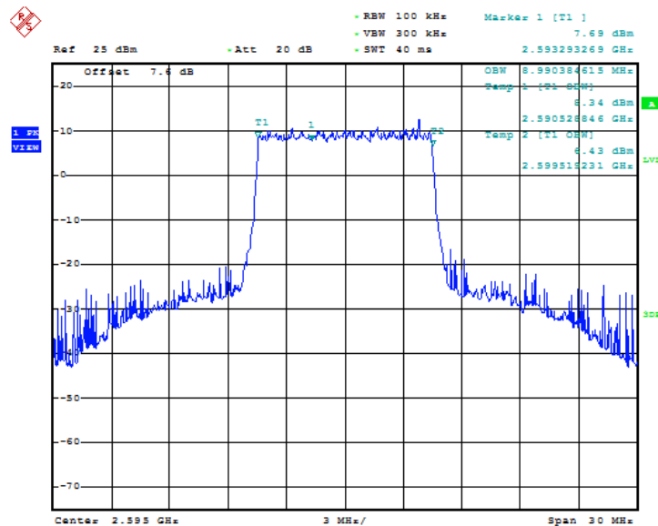
Fig.47 LTE band 41, 10MHz Bandwidth, QPSK (99% BW)
