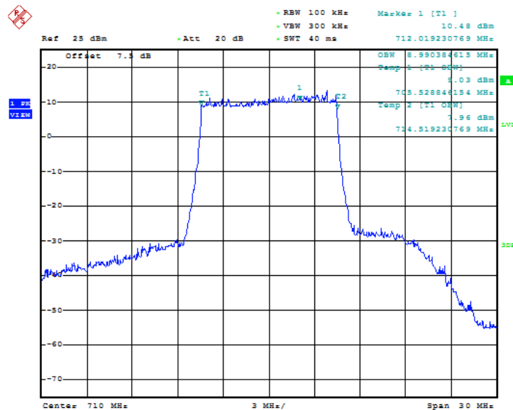
Fig.43 LTE band 17, 10MHz Bandwidth, QPSK (99% BW)
