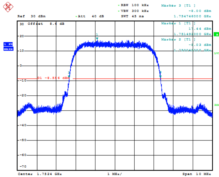
Fig.38 Channel 1312- Emission Bandwidth (-26dBc BW)
