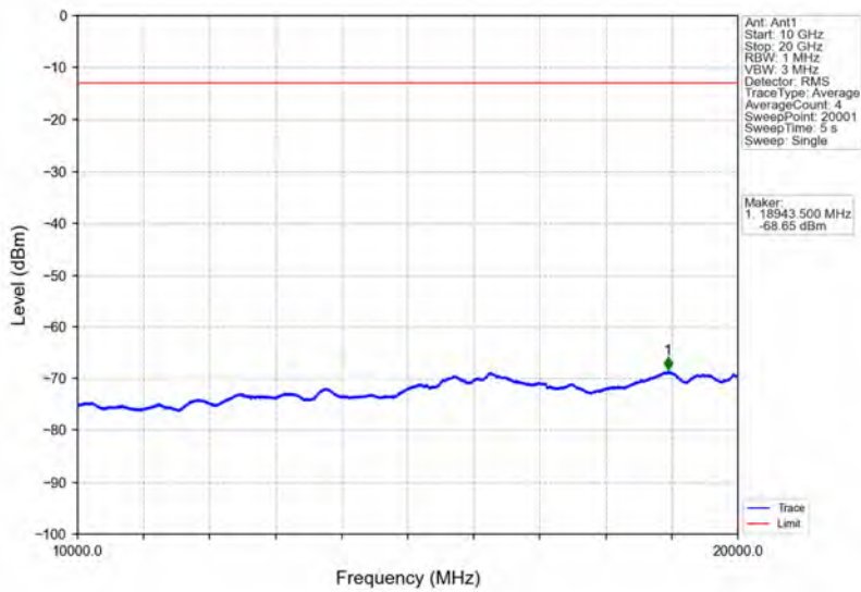
Band66_15MHz_16QAM_LCH_1717.5MHz_RB_75_0_NTNV
