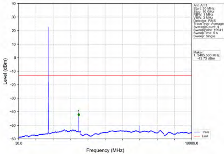
Band66_5MHz_QPSK_MCH_1745MHz_RB_1_0_NTNV
