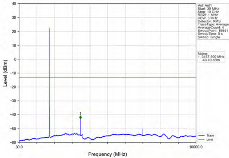
Band66_3MHz_QPSK_MCH_1745MHz_RB_1_0_NTNV
