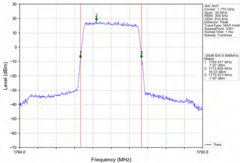
Band66_10MHz_QPSK_HCH_1775MHz_RB_50_0_NTNV
