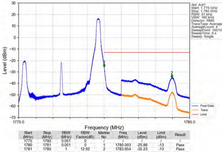
Band66_5MHz_16QAM_HCH_1777.5MHz_RB_1_24_NTNV
