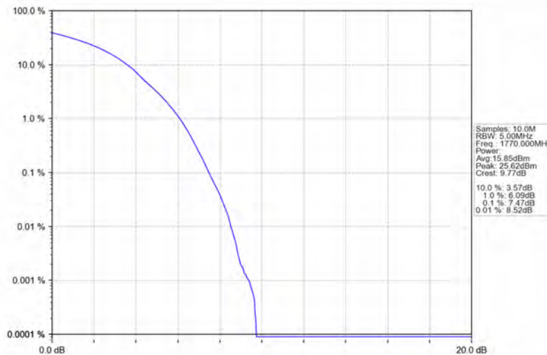
Band66_20MHz_16QAM_HCH_1770MHz_RB_100_0_NTNV
