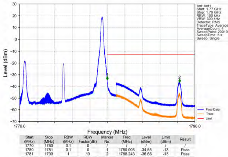
Band66_10MHz_16QAM_HCH_1775MHz_RB_1_49_NTNV
