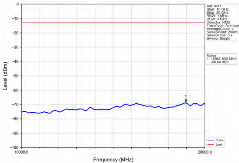
Band66_10MHz_64QAM_HCH_1775MHz_RB_1_0_NTNV
