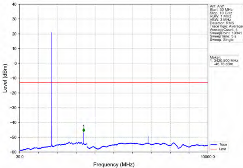
Band66_3MHz_16QAM_LCH_1711.5MHz_RB_1_0_NTNV
