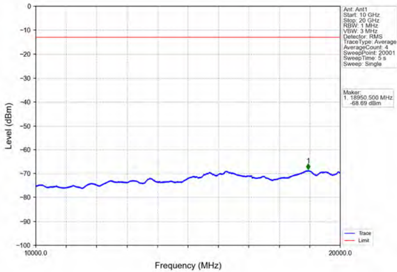
Band66_20MHz_64QAM_LCH_1720MHz_RB_100_0_NTNV
