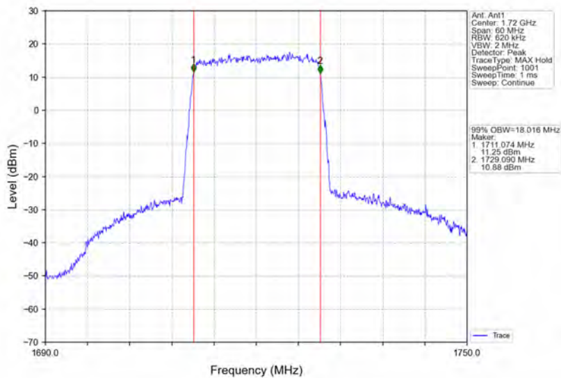
Band66_20MHz_64QAM_LCH_1720MHz_RB_100_0_NTNV
