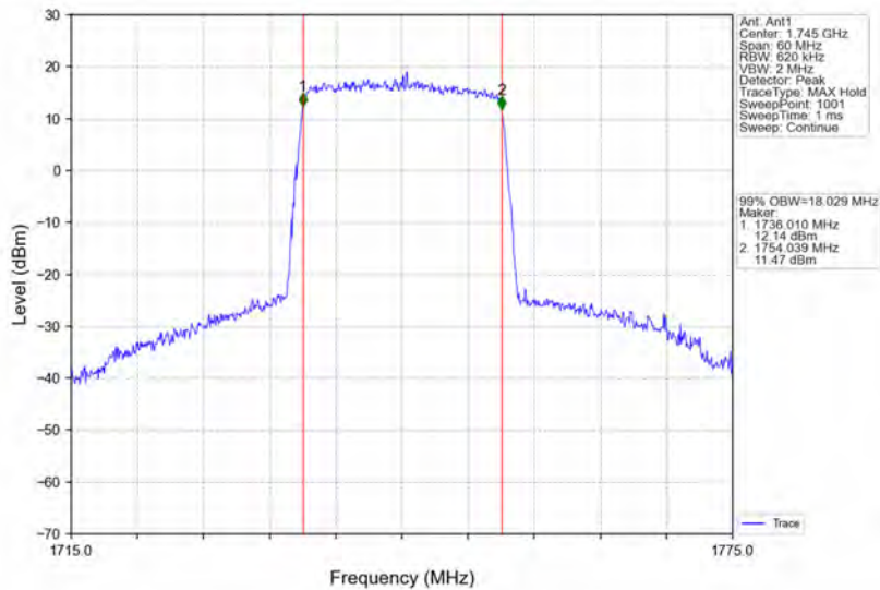
Band66_20MHz_16QAM_MCH_1745MHz_RB_100_0_NTNV
