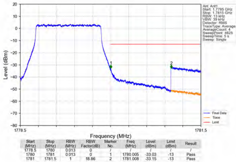
Band66_1.4MHz_16QAM_HCH_1779.3MHz_RB_6_0_NTNV
