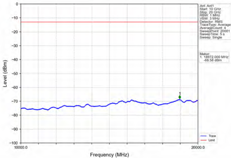
Band66_3MHz_QPSK_MCH_1745MHz_RB_1_0_NTNV
