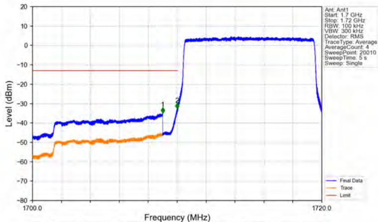
Band66_10MHz_QPSK_LCH_1715MHz_RB_50_0_NTNV
