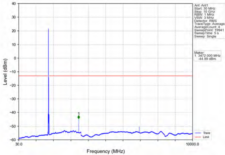
Band66_20MHz_64QAM_MCH_1745MHz_RB_1_0_NTNV
