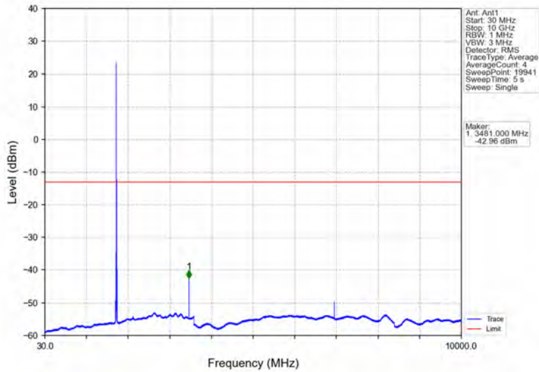
Band66_10MHz_QPSK_MCH_1745MHz_RB_1_0_NTNV
