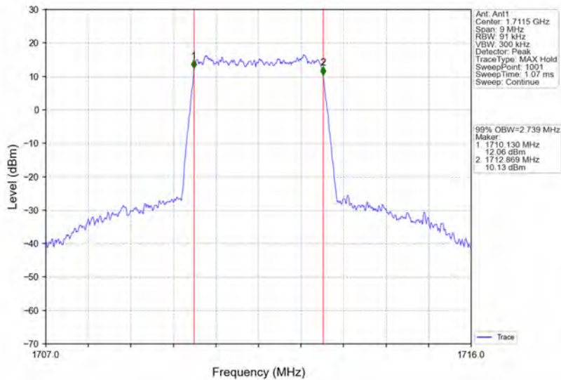
Band66_3MHz_64QAM_LCH_1711.5MHz_RB_15_0_NTNV
