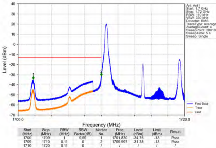
Band66_10MHz_16QAM_LCH_1715MHz_RB_1_0_NTNV
