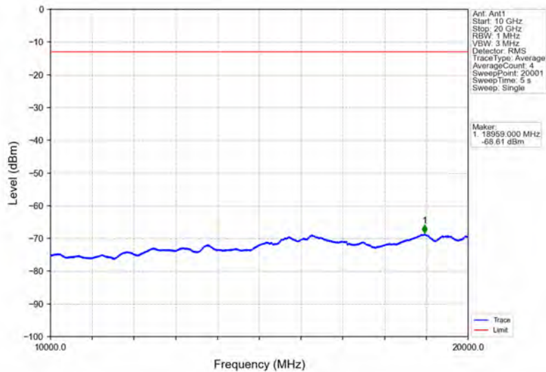
Band66_1.4MHz_16QAM_HCH_1779.3MHz_RB_1_0_NTNV
