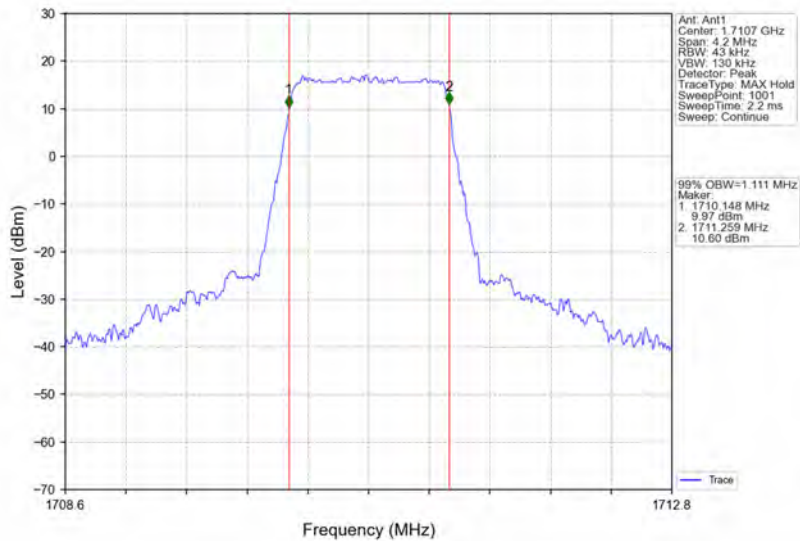
Band66_1.4MHz_16QAM_LCH_1710.7MHz_RB_6_0_NTNV
