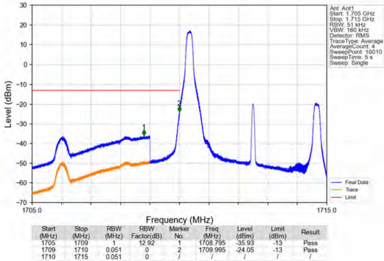
Band66_5MHz_16QAM_LCH_1712.5MHz_RB_1_0_NTNV
