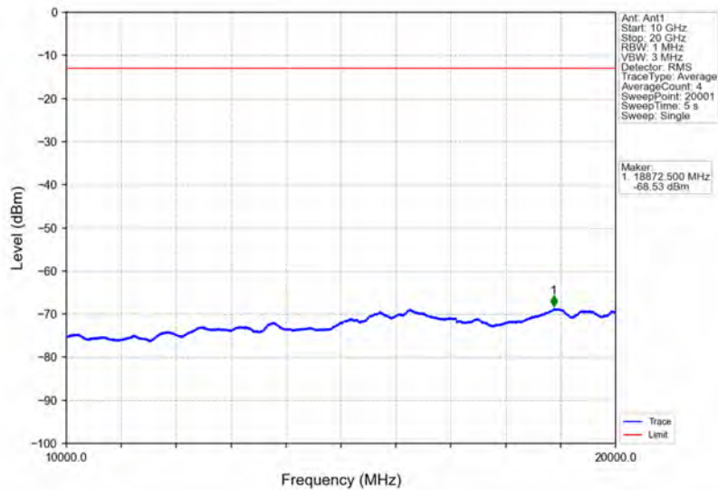
Band66_5MHz_QPSK_HCH_1777.5MHz_RB_1_0_NTNV
