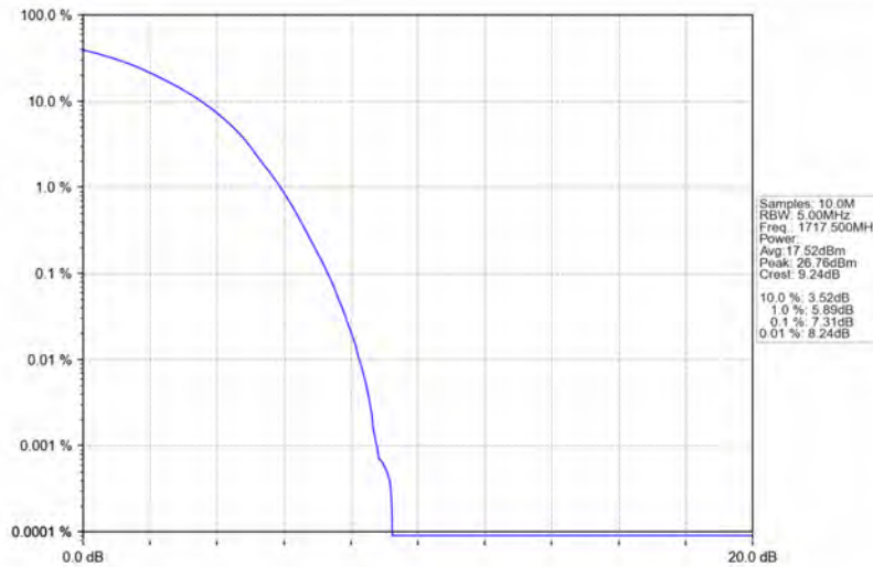
Band66_15MHz_16QAM_LCH_1717.5MHz_RB_75_0_NTNV
