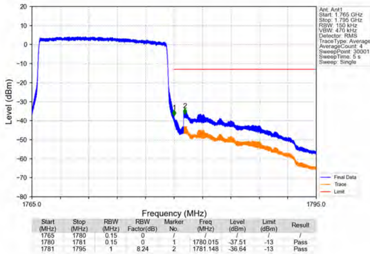
Band66_15MHz_QPSK_HCH_1772.5MHz_RB_75_0_NTNV
