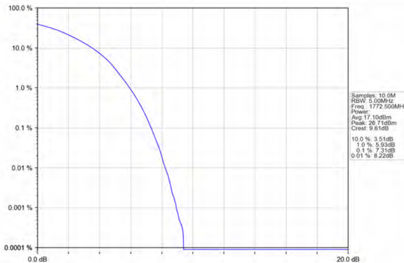
Band66_15MHz_16QAM_HCH_1772.5MHz_RB_75_0_NTNV
