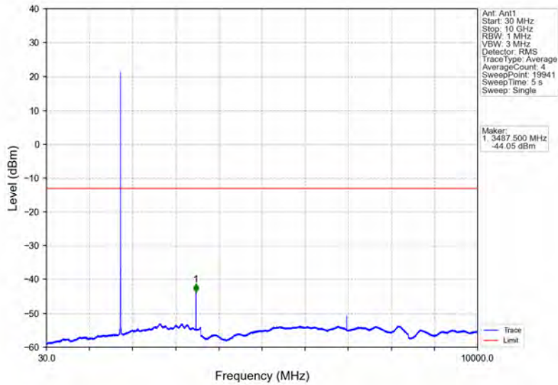
Band66_3MHz_16QAM_MCH_1745MHz_RB_1_0_NTNV
