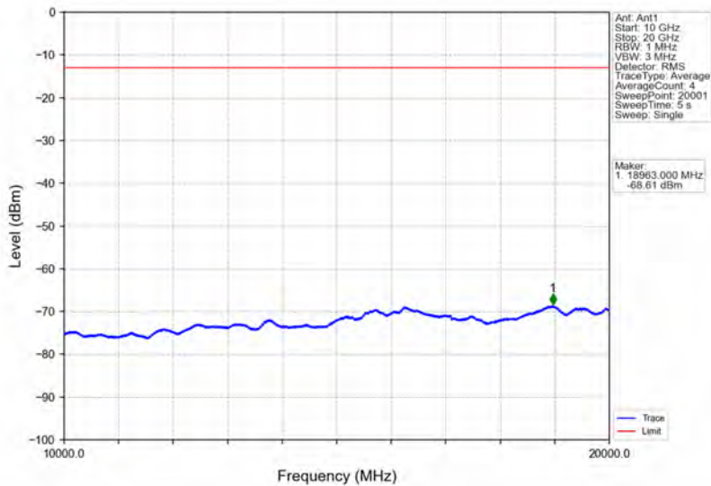
Band66_1.4MHz_QPSK_HCH_1779.3MHz_RB_1_0_NTNV
