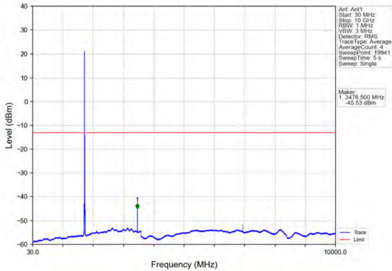
Band66_15MHz_64QAM_MCH_1745MHz_RB_1_0_NTNV
