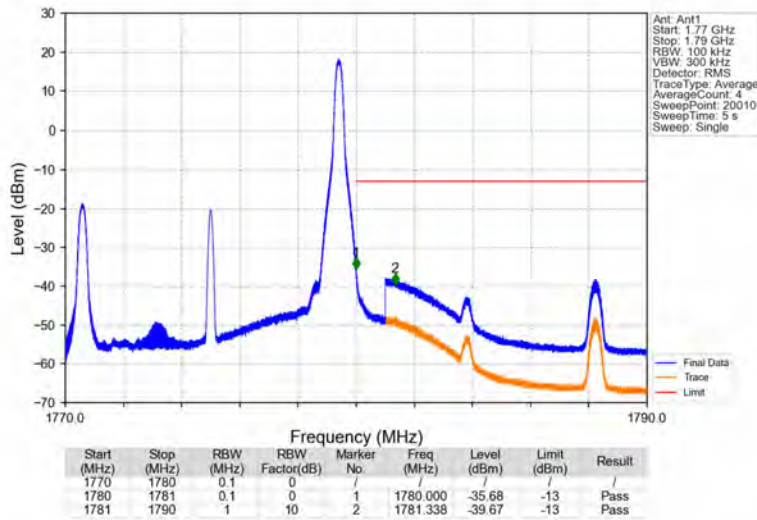
Band66_10MHz_64QAM_HCH_1775MHz_RB_1_49_NTNV
