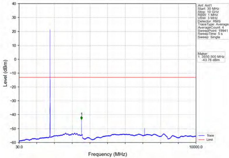
Band66_5MHz_16QAM_HCH_1777.5MHz_RB_1_0_NTNV
