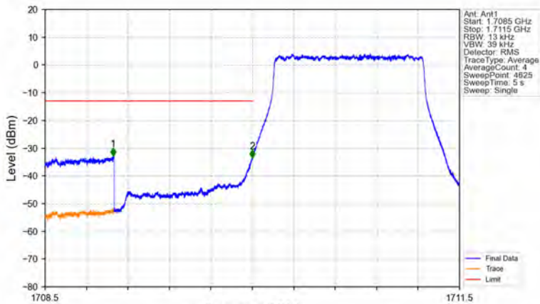
Band66_1.4MHz_QPSK_LCH_1710.7MHz_RB_6_0_NTNV
