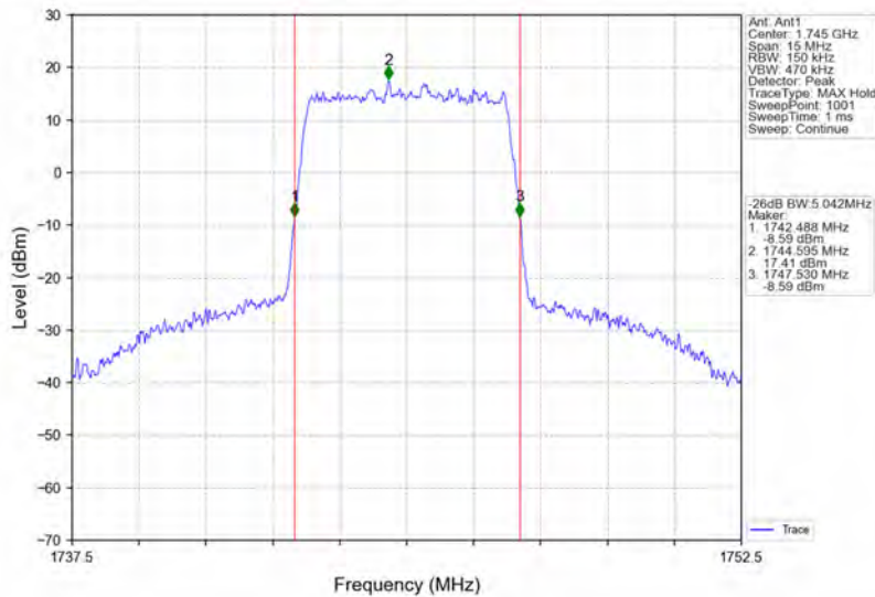
Band66_5MHz_64QAM_MCH_1745MHz_RB_25_0_NTNV
