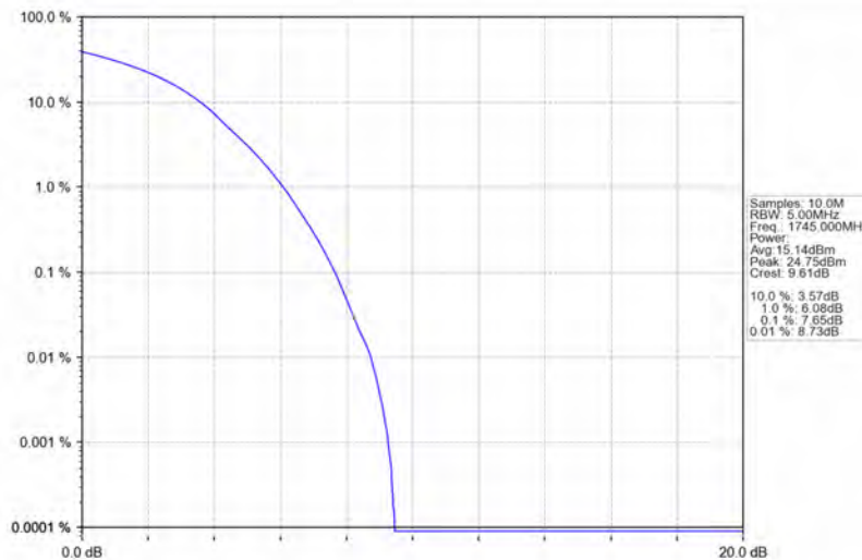
Band66_20MHz_64QAM_MCH_1745MHz_RB_100_0_NTNV
