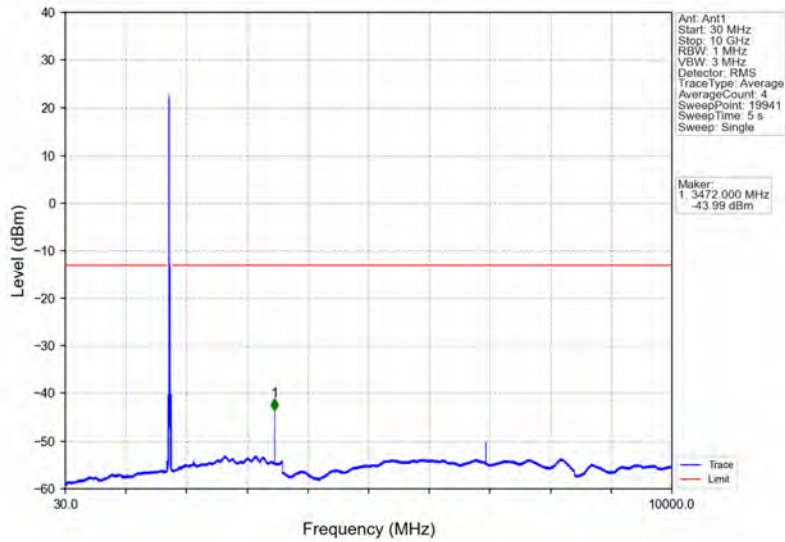
Band66_20MHz_16QAM_MCH_1745MHz_RB_1_0_NTNV
