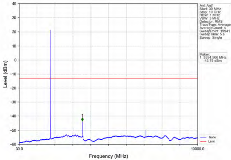
Band66_3MHz_16QAM_HCH_1778.5MHz_RB_1_0_NTNV
