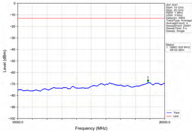
Band66_1.4MHz_QPSK_MCH_1745MHz_RB_1_0_NTNV
