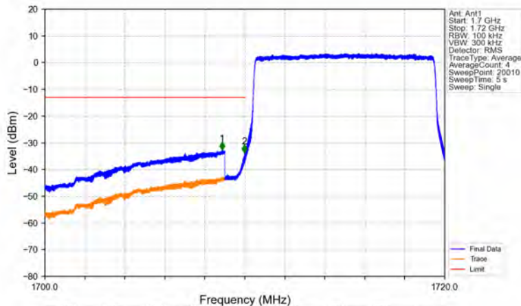
Band66_10MHz_16QAM_LCH_1715MHz_RB_50_0_NTNV
