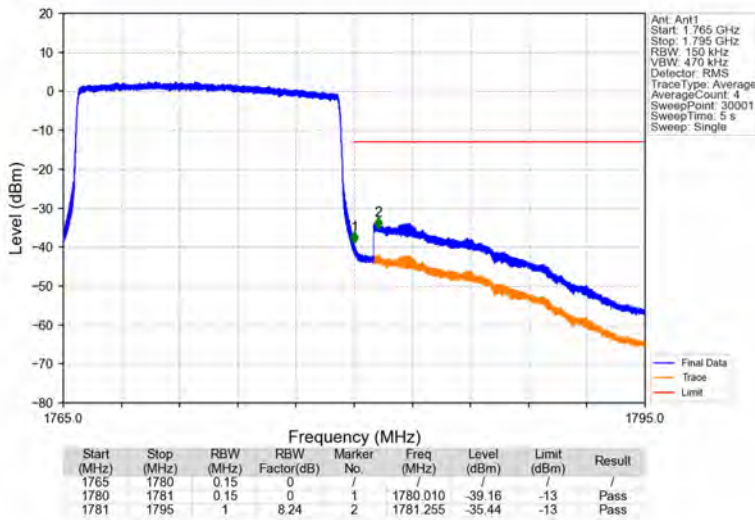
Band66_15MHz_64QAM_HCH_1772.5MHz_RB_75_0_NTNV
