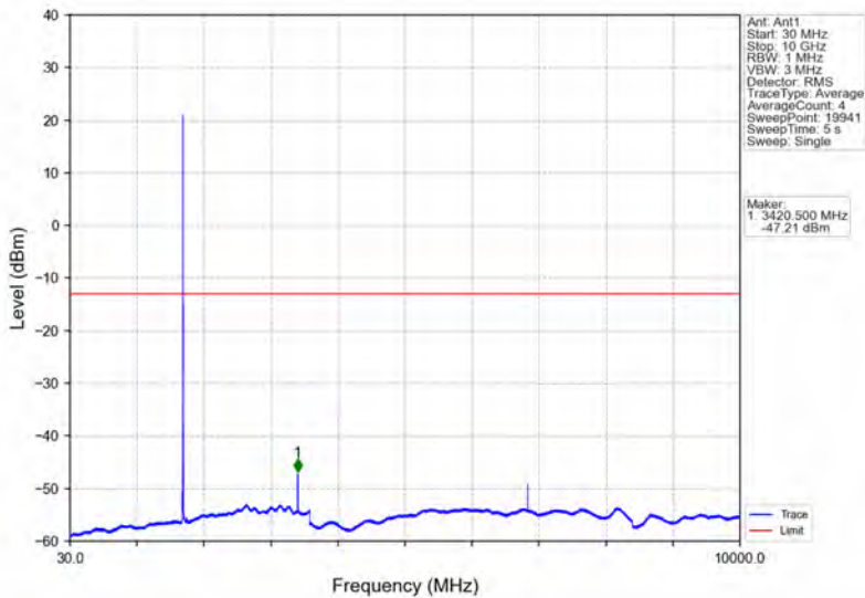
Band66_5MHz_16QAM_LCH_1712.5MHz_RB_1_0_NTNV
