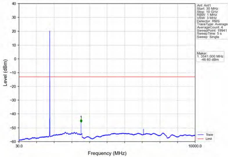
Band66_10MHz_64QAM_HCH_1775MHz_RB_1_0_NTNV
