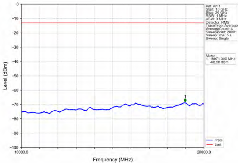
Band66_15MHz_16QAM_HCH_1772.5MHz_RB_1_0_NTNV
