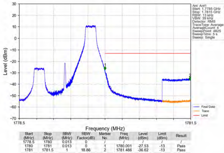
Band66_1.4MHz_16QAM_HCH_1779.3MHz_RB_1_5_NTNV
