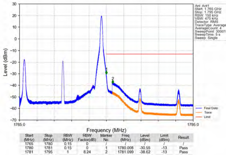
Band66_15MHz_16QAM_HCH_1772.5MHz_RB_1_74_NTNV
