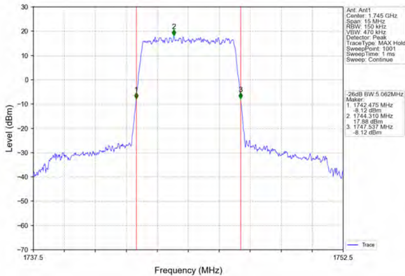
Band66_5MHz_QPSK_MCH_1745MHz_RB_25_0_NTNV
