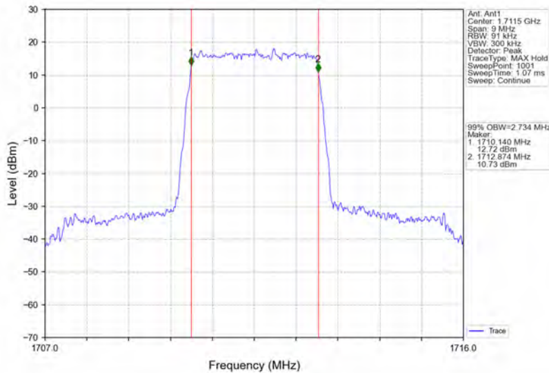
Band66_3MHz_QPSK_LCH_1711.5MHz_RB_15_0_NTNV
