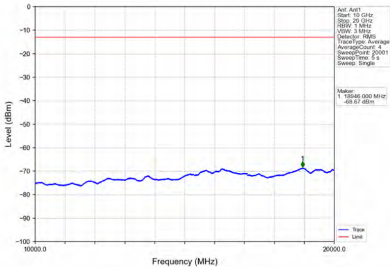
Band66_1.4MHz_64QAM_HCH_1779.3MHz_RB_1_0_NTNV
