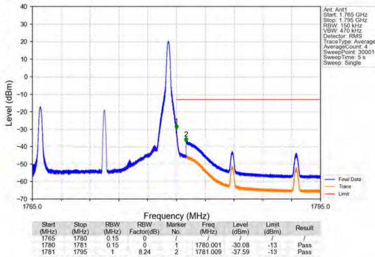
Band66_15MHz_QPSK_HCH_1772.5MHz_RB_1_74_NTNV
