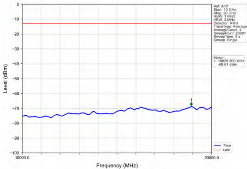
Band66_20MHz_16QAM_HCH_1770MHz_RB_1_0_NTNV
