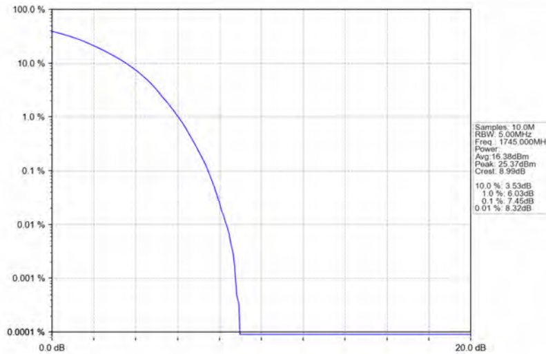
Band66_15MHz_64QAM_MCH_1745MHz_RB_75_0_NTNV
