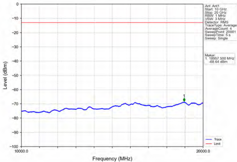
Band66_20MHz_16QAM_MCH_1745MHz_RB_1_0_NTNV
