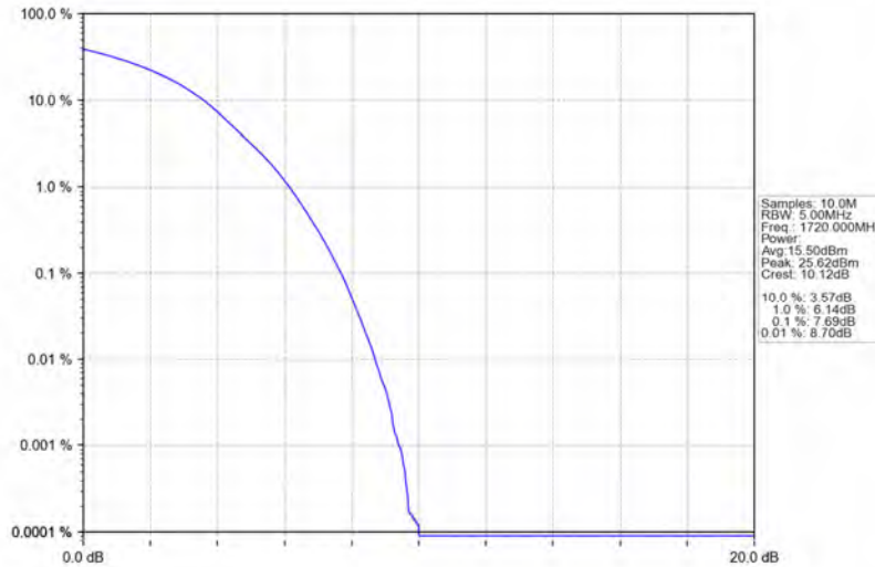
Band66_20MHz_64QAM_LCH_1720MHz_RB_100_0_NTNV
