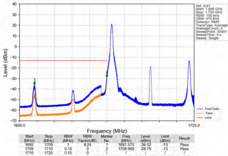
Band66_15MHz_16QAM_LCH_1717.5MHz_RB_1_0_NTNV
