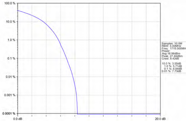
Band66_10MHz_16QAM_LCH_1715MHz_RB_50_0_NTNV
