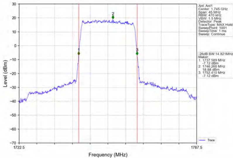
Band66_15MHz_QPSK_MCH_1745MHz_RB_75_0_NTNV
