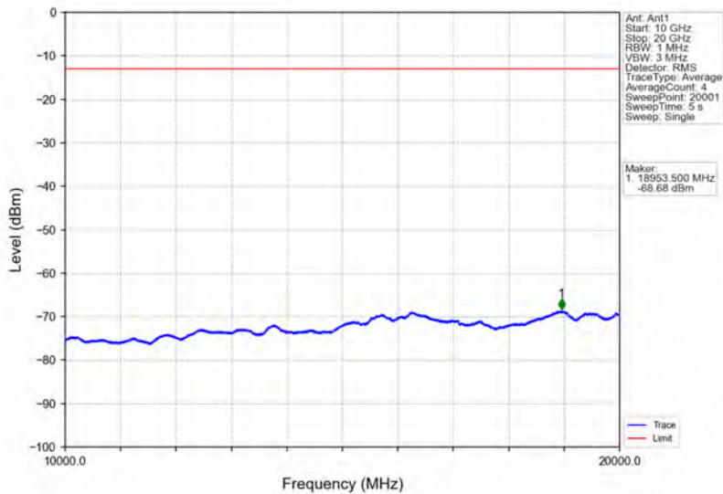
Band66_1.4MHz_16QAM_MCH_1745MHz_RB_1_0_NTNV
