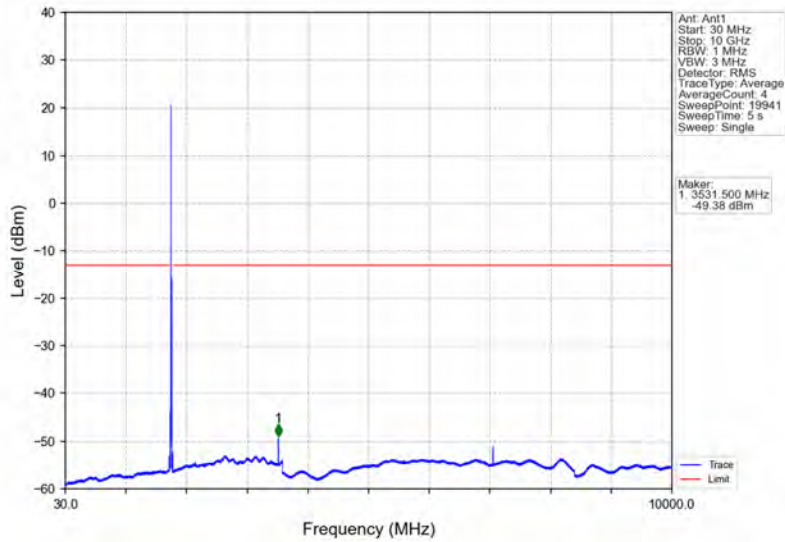
Band66_15MHz_64QAM_HCH_1772.5MHz_RB_1_0_NTNV
