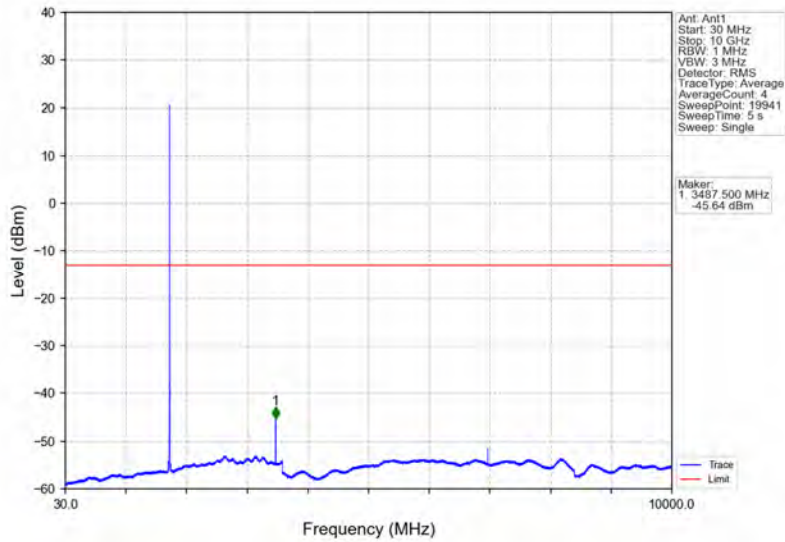
Band66_3MHz_64QAM_MCH_1745MHz_RB_1_0_NTNV
