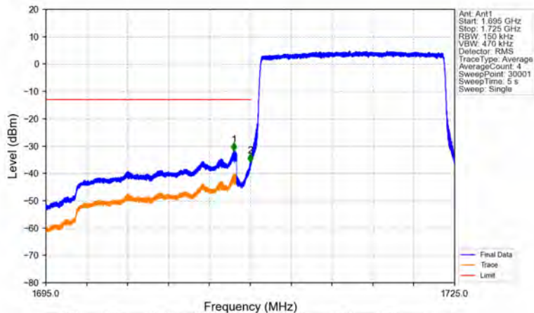
Band66_15MHz_QPSK_LCH_1717.5MHz_RB_75_0_NTNV
