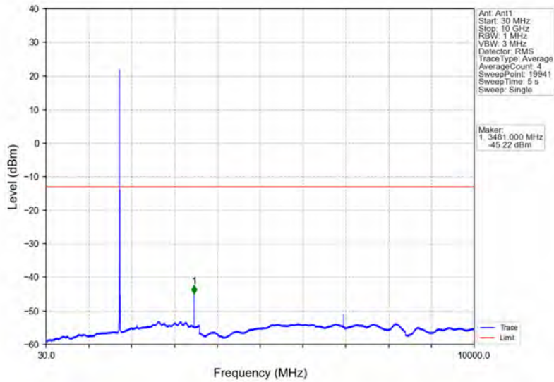
Band66_10MHz_64QAM_MCH_1745MHz_RB_1_0_NTNV
