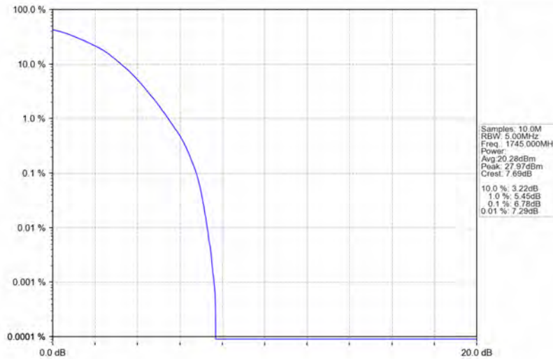
Band66_1.4MHz_64QAM_MCH_1745MHz_RB_6_0_NTNV
