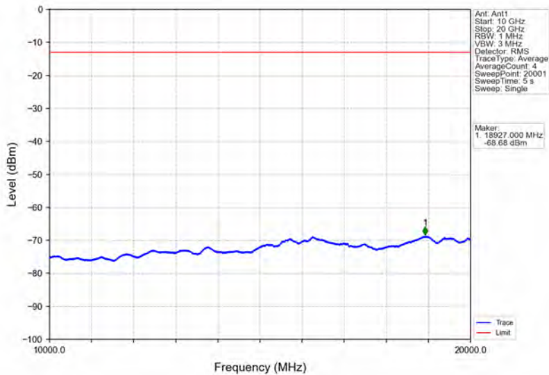
Band66_10MHz_QPSK_HCH_1775MHz_RB_1_0_NTNV
