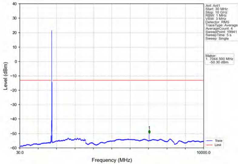
Band66_20MHz_16QAM_HCH_1770MHz_RB_1_0_NTNV
