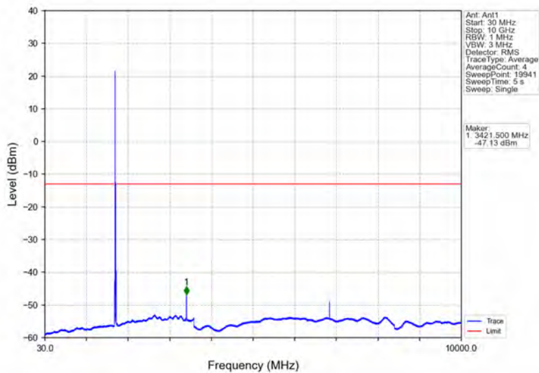
Band66_15MHz_16QAM_LCH_1717.5MHz_RB_1_0_NTNV
