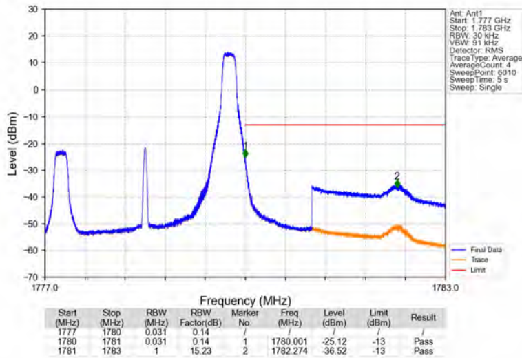
Band66_3MHz_64QAM_HCH_1778.5MHz_RB_1_14_NTNV
