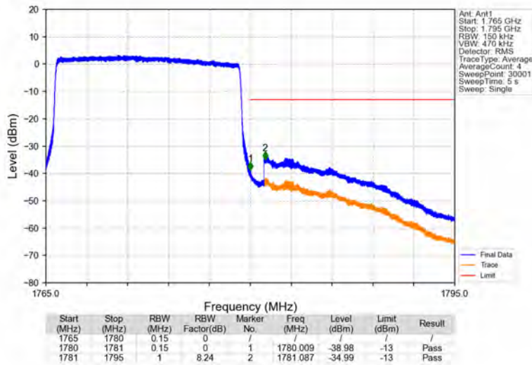
Band66_15MHz_16QAM_HCH_1772.5MHz_RB_75_0_NTNV
