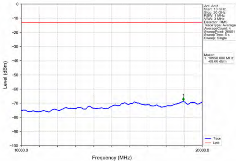
Band66_3MHz_16QAM_HCH_1778.5MHz_RB_1_0_NTNV
