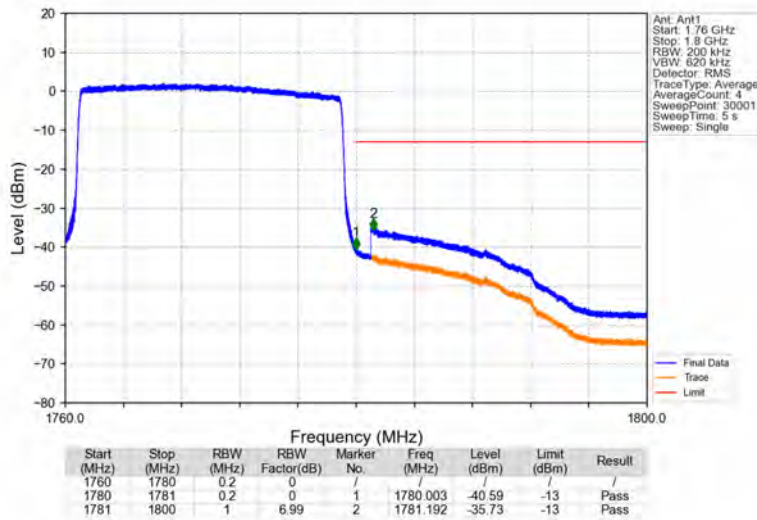
Band66_20MHz_64QAM_HCH_1770MHz_RB_100_0_NTNV
