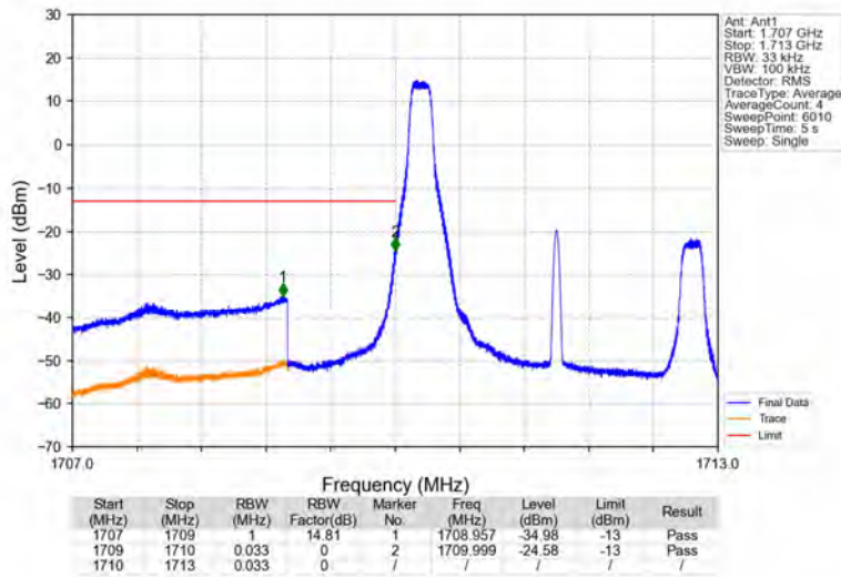
Band66_3MHz_64QAM_LCH_1711.5MHz_RB_1_0_NTNV
