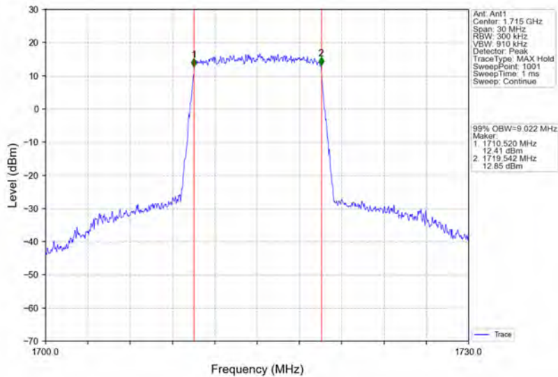
Band66_10MHz_64QAM_LCH_1715MHz_RB_50_0_NTNV
