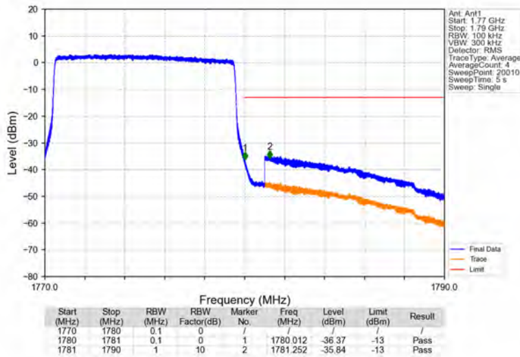
Band66_10MHz_16QAM_HCH_1775MHz_RB_50_0_NTNV
