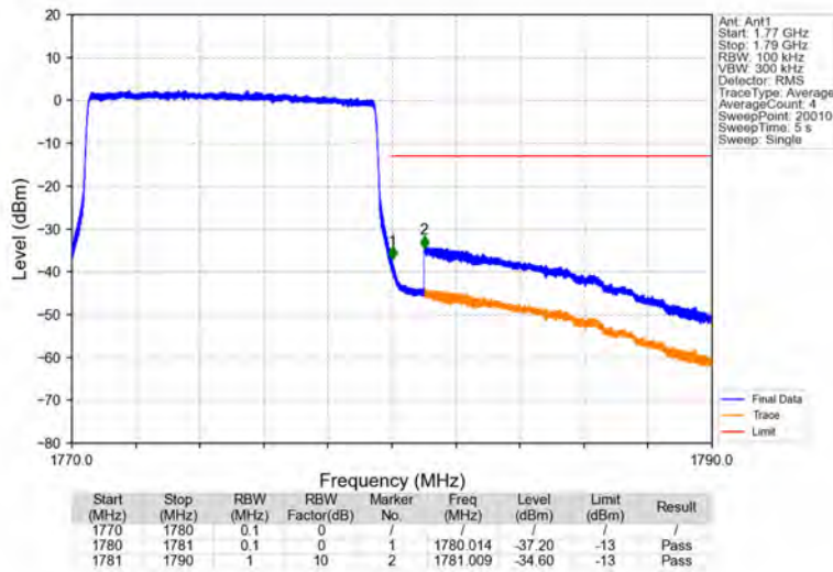
Band66_10MHz_64QAM_HCH_1775MHz_RB_50_0_NTNV
