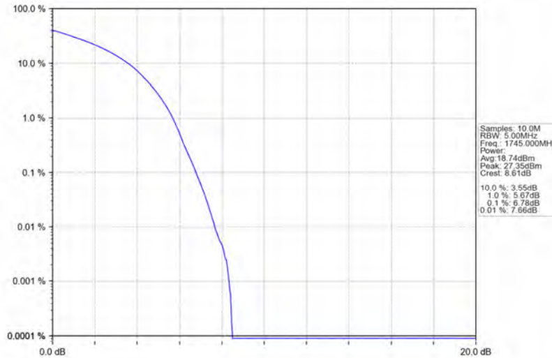
Band66_10MHz_16QAM_MCH_1745MHz_RB_50_0_NTNV
