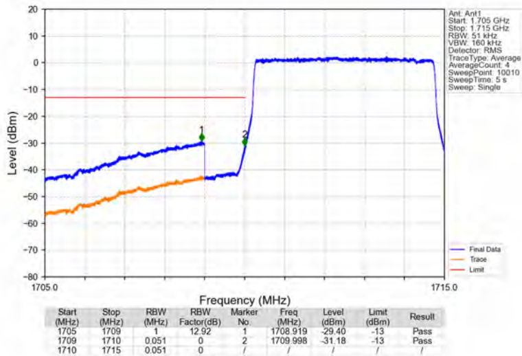
Band66_5MHz_64QAM_LCH_1712.5MHz_RB_25_0_NTNV
