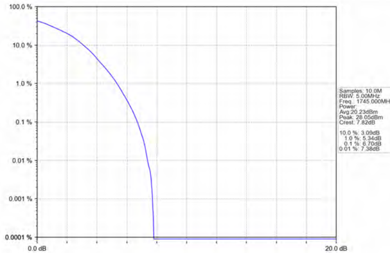
Band66_3MHz_64QAM_MCH_1745MHz_RB_15_0_NTNV
