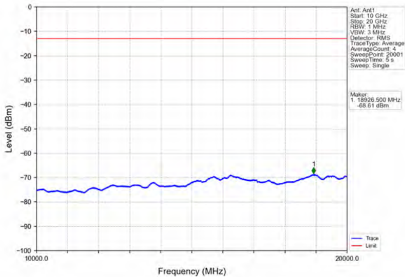
Band66_5MHz_QPSK_MCH_1745MHz_RB_1_0_NTNV
