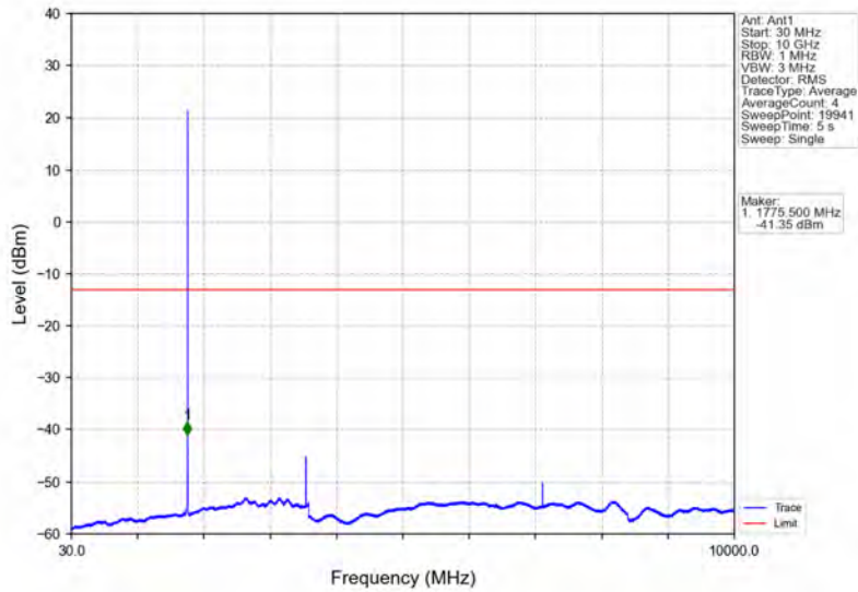
Band66_1.4MHz_16QAM_HCH_1779.3MHz_RB_1_0_NTNV
