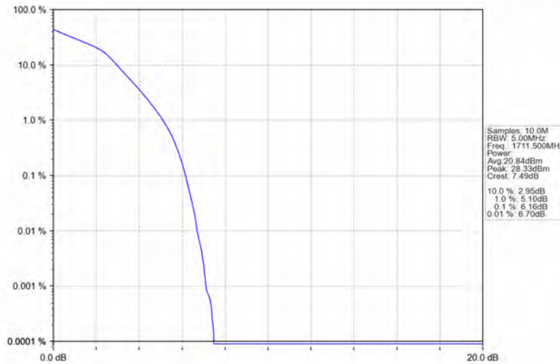
Band66_3MHz_16QAM_LCH_1711.5MHz_RB_15_0_NTNV
