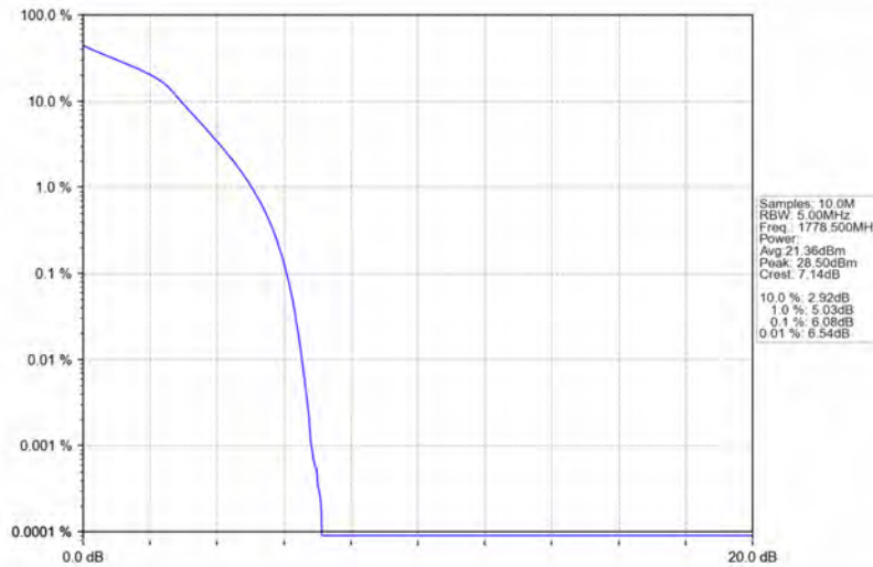
Band66_3MHz_16QAM_HCH_1778.5MHz_RB_15_0_NTNV
