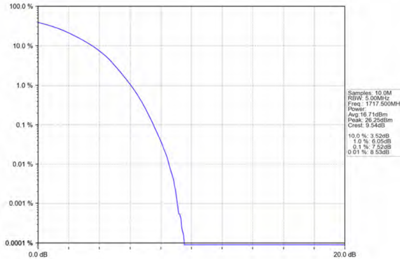
Band66_15MHz_64QAM_LCH_1717.5MHz_RB_75_0_NTNV
