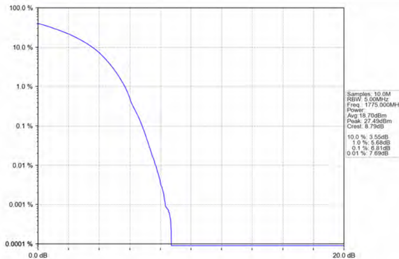
Band66_10MHz_16QAM_HCH_1775MHz_RB_50_0_NTNV
