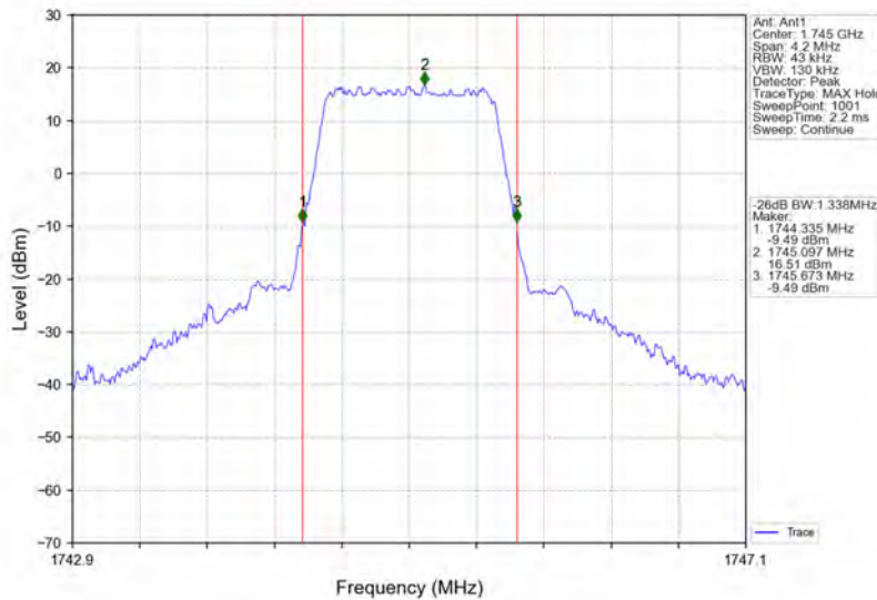
Band66_1.4MHz_64QAM_MCH_1745MHz_RB_6_0_NTNV
