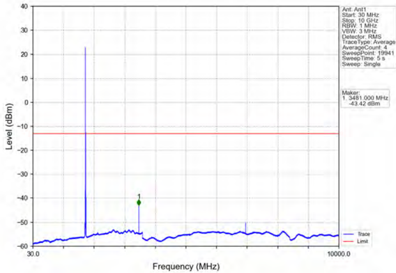
Band66_10MHz_16QAM_MCH_1745MHz_RB_1_0_NTNV
