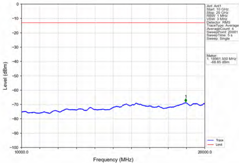
Band66_3MHz_64QAM_HCH_1778.5MHz_RB_1_0_NTNV
