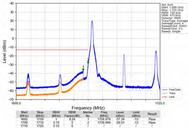
Band66_15MHz_64QAM_LCH_1717.5MHz_RB_1_0_NTNV
