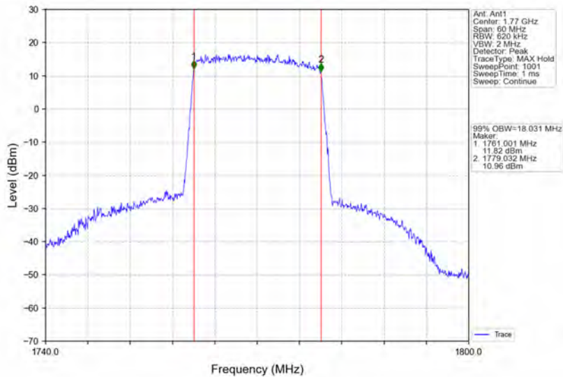
Band66_20MHz_64QAM_HCH_1770MHz_RB_100_0_NTNV
