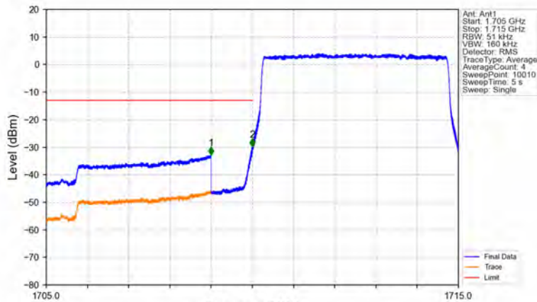
Band66_5MHz_QPSK_LCH_1712.5MHz_RB_25_0_NTNV
