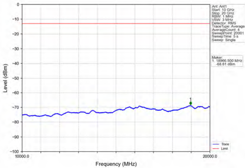
Band66_5MHz_64QAM_LCH_1712.5MHz_RB_25_0_NTNV
