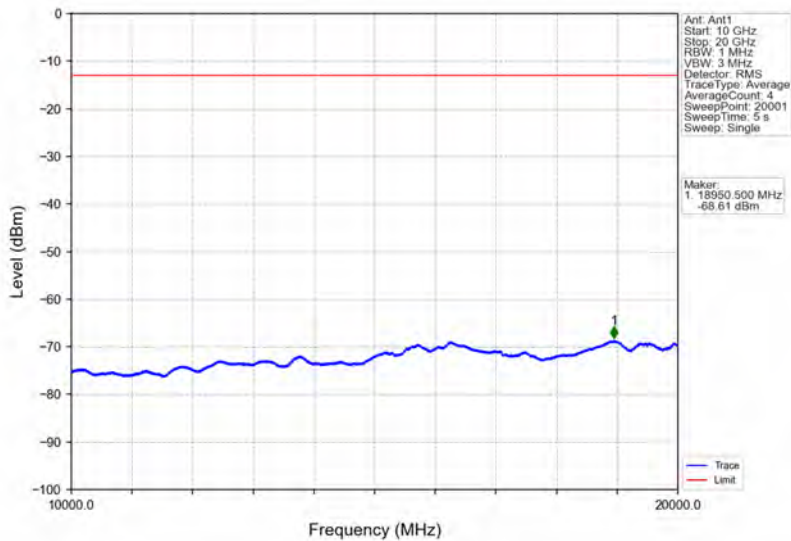
Band66_5MHz_16QAM_MCH_1745MHz_RB_1_0_NTNV
