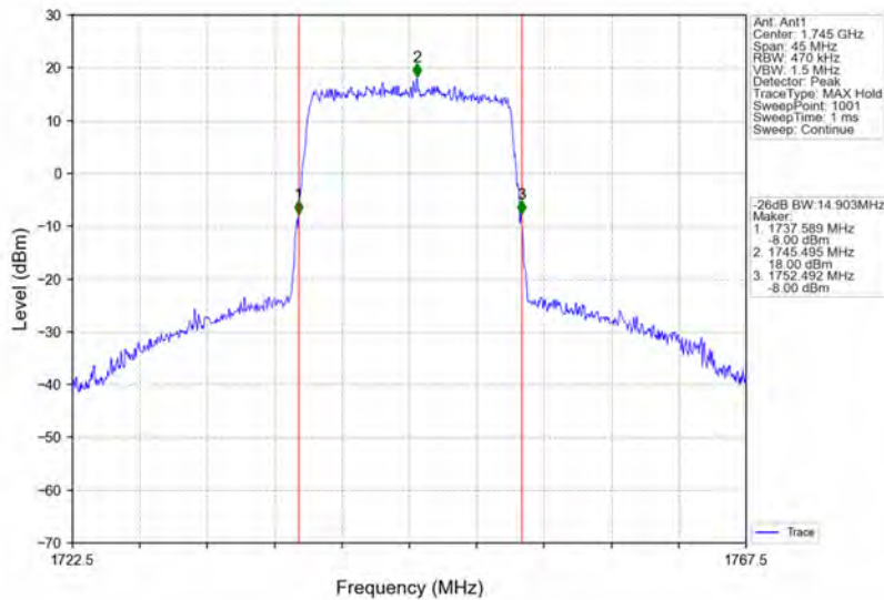
Band66_15MHz_64QAM_MCH_1745MHz_RB_75_0_NTNV
