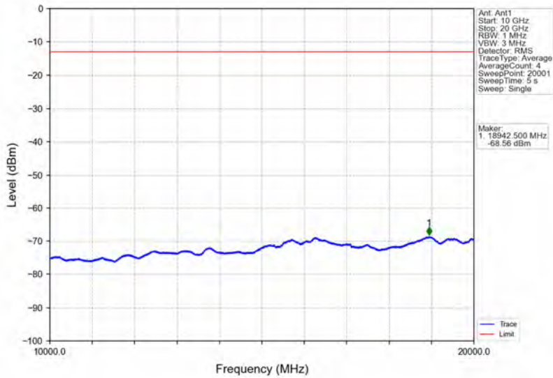
Band66_1.4MHz_QPSK_LCH_1710.7MHz_RB_6_0_NTNV
