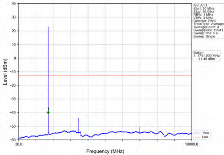
Band66_1.4MHz_QPSK_MCH_1745MHz_RB_1_0_NTNV
