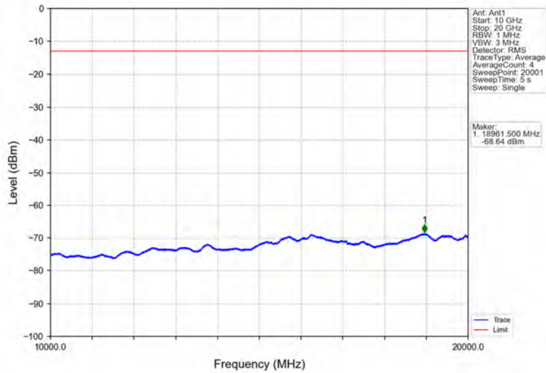
Band66_15MHz_64QAM_LCH_1717.5MHz_RB_75_0_NTNV
