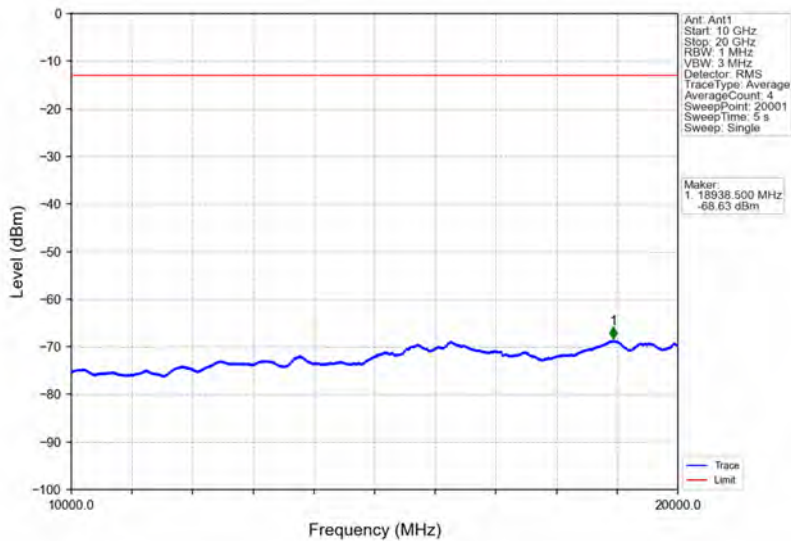
Band66_3MHz_16QAM_MCH_1745MHz_RB_1_0_NTNV
