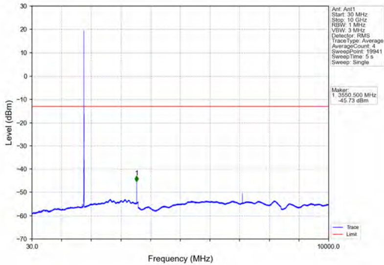
Band66_5MHz_64QAM_HCH_1777.5MHz_RB_1_0_NTNV
