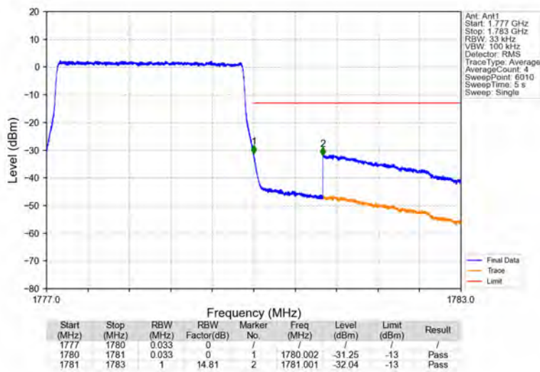
Band66_3MHz_64QAM_HCH_1778.5MHz_RB_15_0_NTNV
