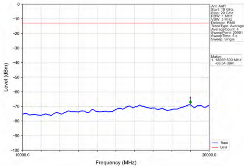
Band66_10MHz_QPSK_MCH_1745MHz_RB_1_0_NTNV
