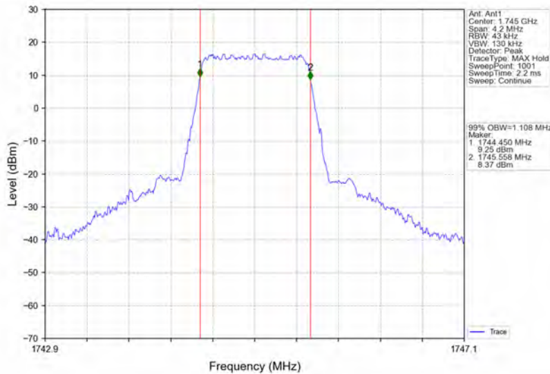
Band66_1.4MHz_64QAM_MCH_1745MHz_RB_6_0_NTNV
