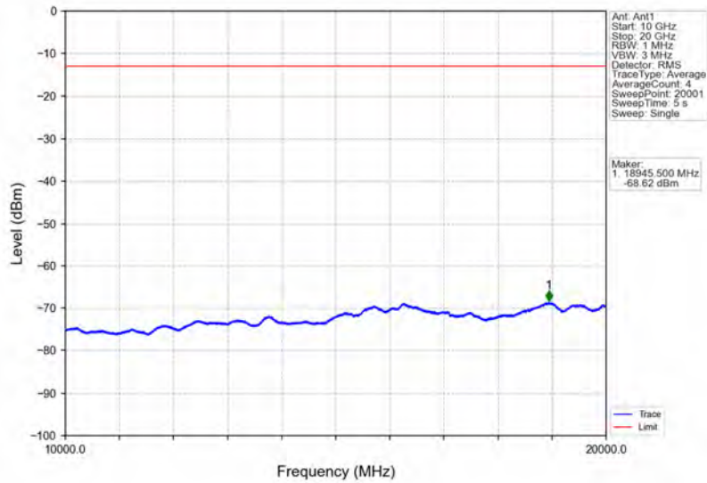
Band66_5MHz_QPSK_LCH_1712.5MHz_RB_25_0_NTNV
