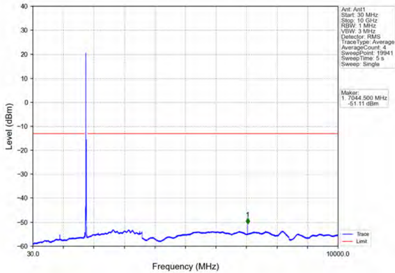
Band66_20MHz_64QAM_HCH_1770MHz_RB_1_0_NTNV
