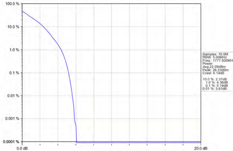
Band66_5MHz_QPSK_HCH_1777.5MHz_RB_25_0_NTNV
