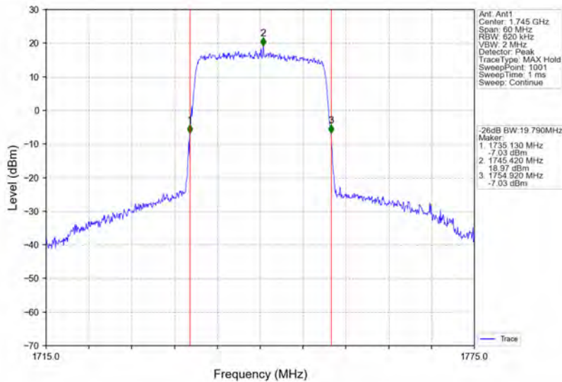
Band66_20MHz_16QAM_MCH_1745MHz_RB_100_0_NTNV
