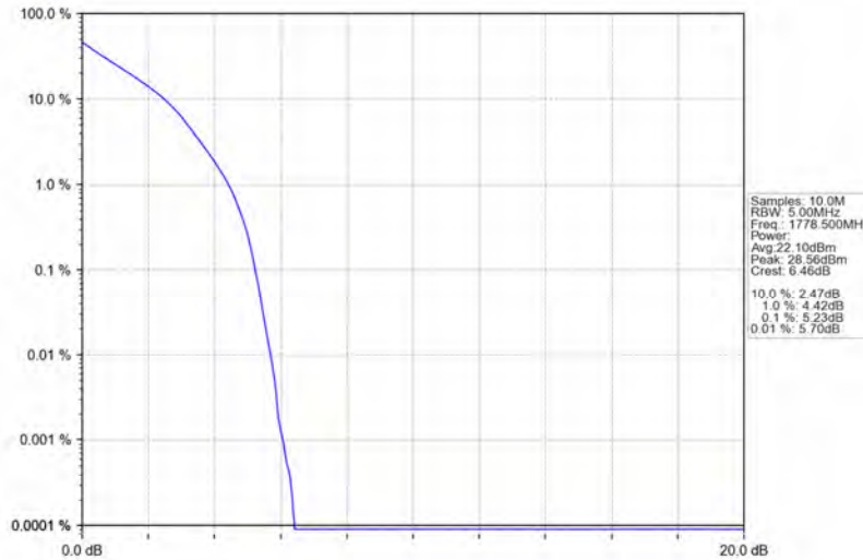
Band66_3MHz_QPSK_HCH_1778.5MHz_RB_15_0_NTNV
