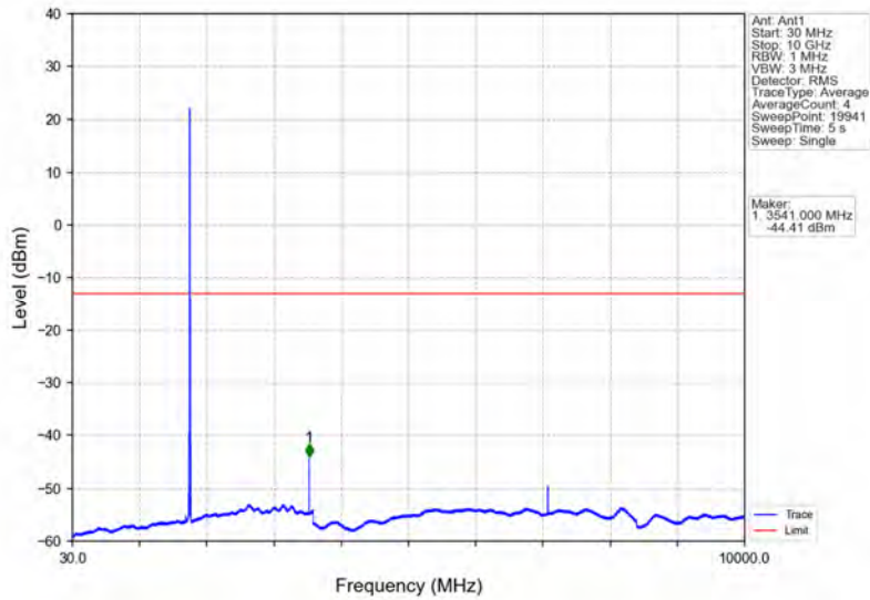
Band66_10MHz_QPSK_HCH_1775MHz_RB_1_0_NTNV
