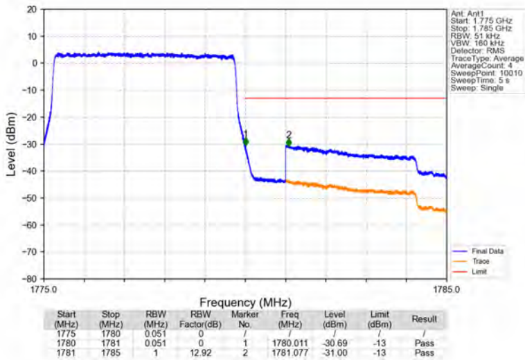
Band66_5MHz_QPSK_HCH_1777.5MHz_RB_25_0_NTNV
