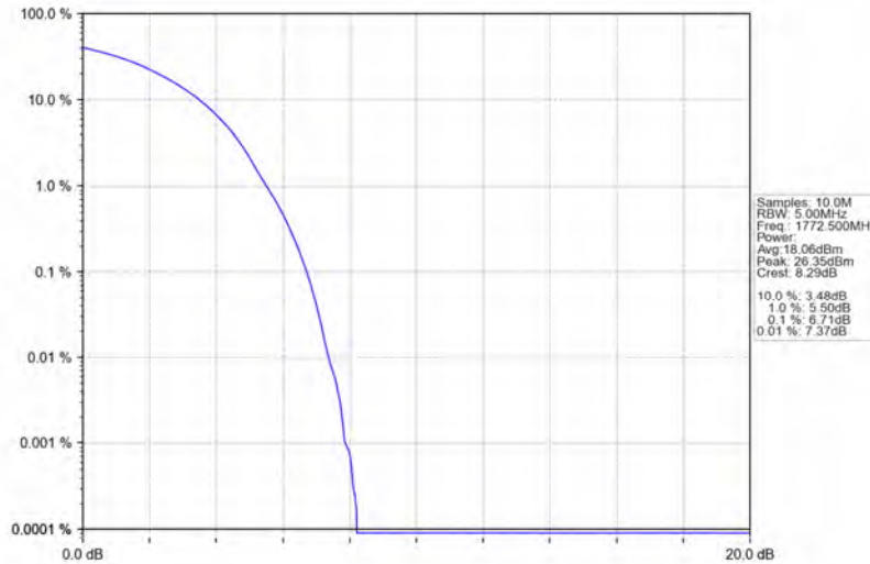
Band66_15MHz_QPSK_HCH_1772.5MHz_RB_75_0_NTNV
