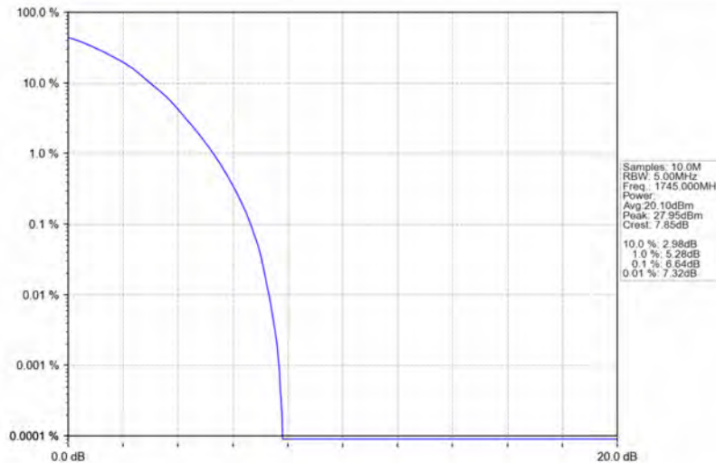
Band66_5MHz_64QAM_MCH_1745MHz_RB_25_0_NTNV
