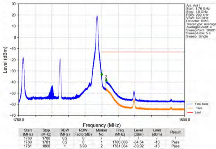
Band66_20MHz_64QAM_HCH_1770MHz_RB_1_99_NTNV
