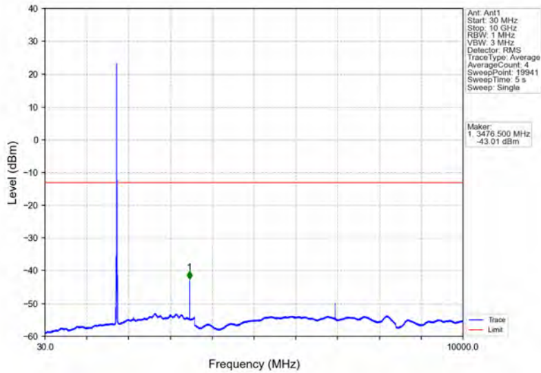
Band66_15MHz_QPSK_MCH_1745MHz_RB_1_0_NTNV
