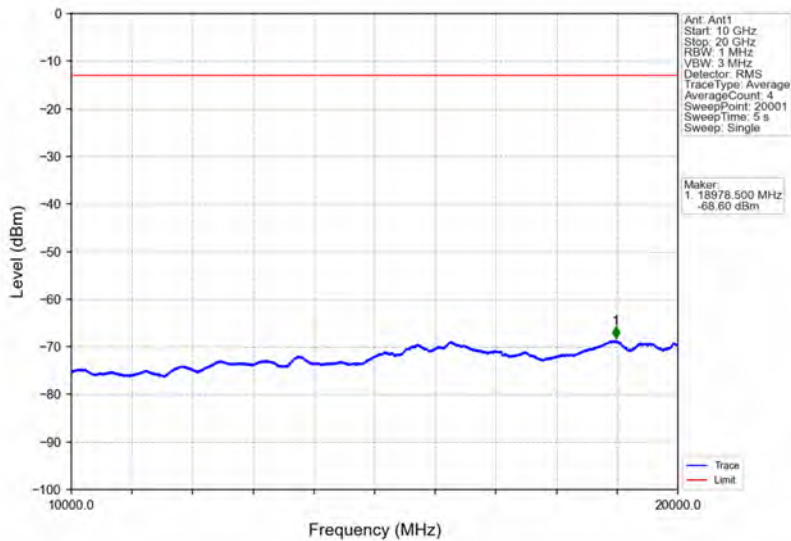
Band66_10MHz_16QAM_MCH_1745MHz_RB_1_0_NTNV
