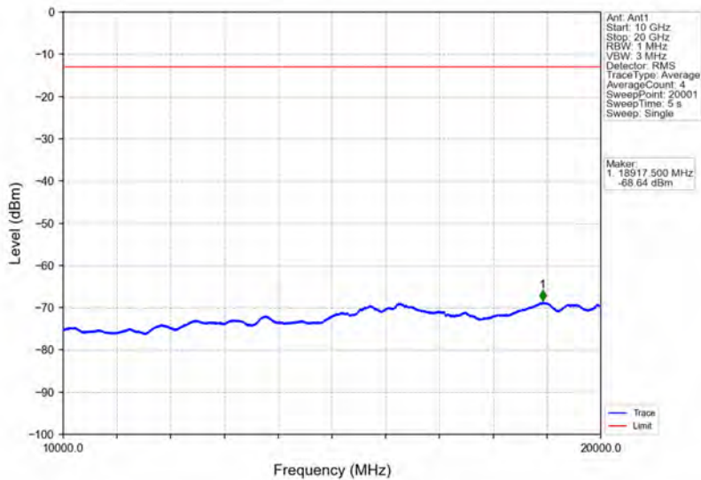
Band66_20MHz_64QAM_HCH_1770MHz_RB_1_0_NTNV
