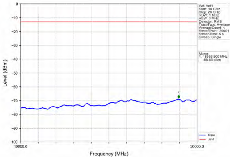
Band66_15MHz_16QAM_MCH_1745MHz_RB_1_0_NTNV
