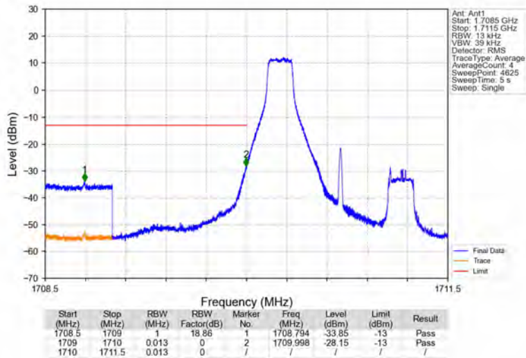
Band66_1.4MHz_16QAM_LCH_1710.7MHz_RB_1_0_NTNV
