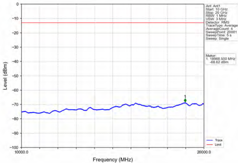
Band66_15MHz_QPSK_HCH_1772.5MHz_RB_1_0_NTNV
