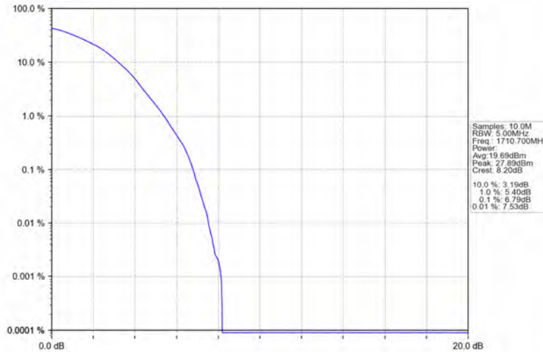
Band66_1.4MHz_64QAM_LCH_1710.7MHz_RB_6_0_NTNV
