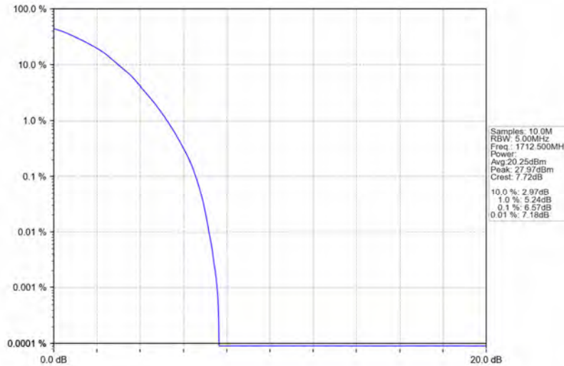
Band66_5MHz_64QAM_LCH_1712.5MHz_RB_25_0_NTNV
