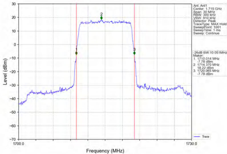
Band66_10MHz_QPSK_LCH_1715MHz_RB_50_0_NTNV
