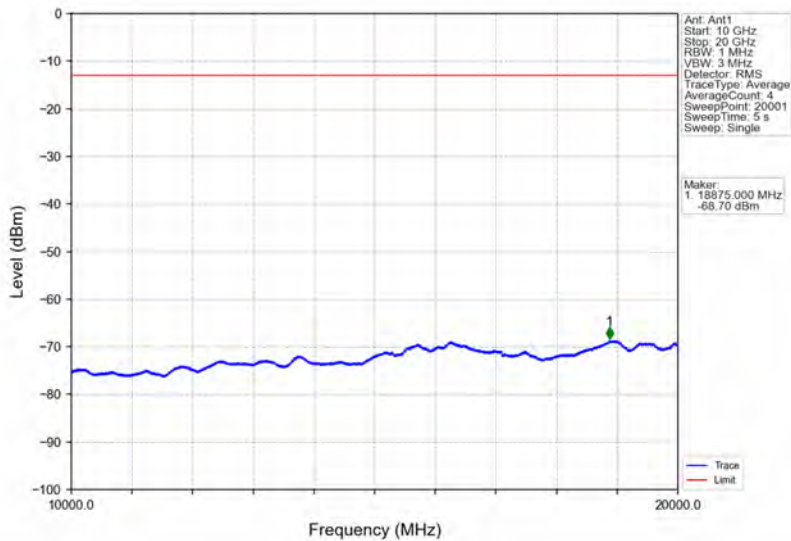
Band66_5MHz_64QAM_MCH_1745MHz_RB_1_0_NTNV
