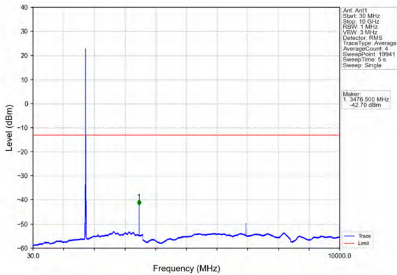
Band66_15MHz_16QAM_MCH_1745MHz_RB_1_0_NTNV
