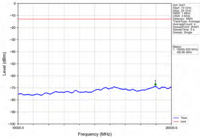
Band66_5MHz_64QAM_HCH_1777.5MHz_RB_1_0_NTNV
