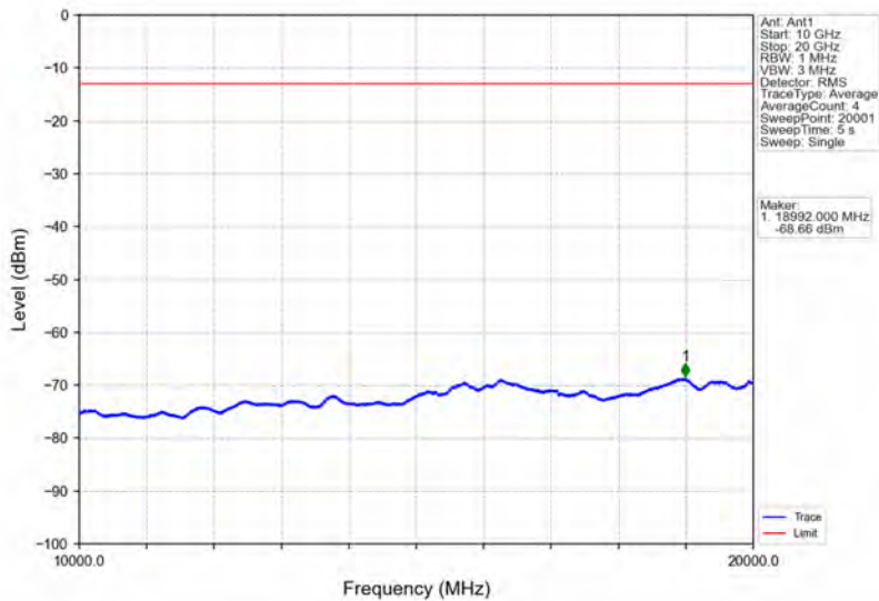
Band66_5MHz_16QAM_HCH_1777.5MHz_RB_1_0_NTNV
