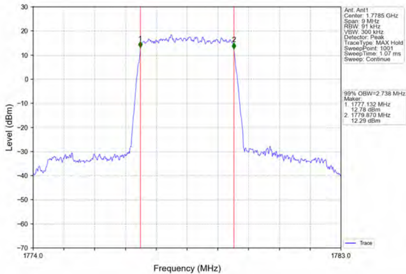
Band66_3MHz_QPSK_HCH_1778.5MHz_RB_15_0_NTNV
