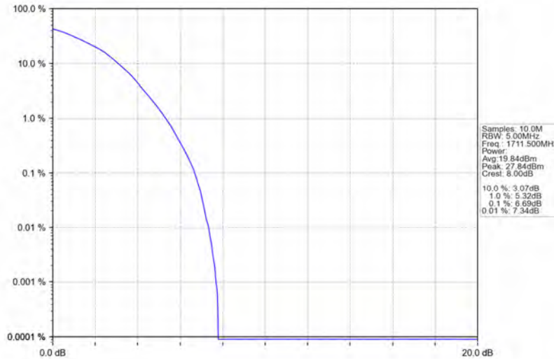
Band66_3MHz_64QAM_LCH_1711.5MHz_RB_15_0_NTNV
