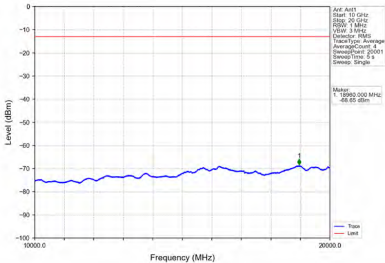
Band66_10MHz_16QAM_HCH_1775MHz_RB_1_0_NTNV
