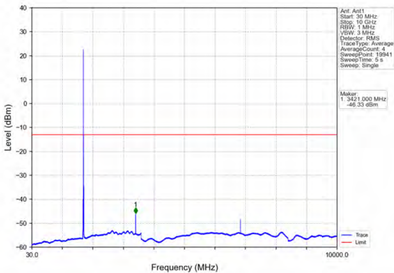
Band66_10MHz_16QAM_LCH_1715MHz_RB_1_0_NTNV
