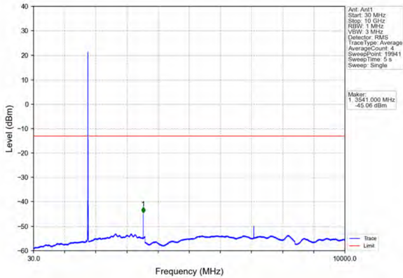
Band66_10MHz_16QAM_HCH_1775MHz_RB_1_0_NTNV
