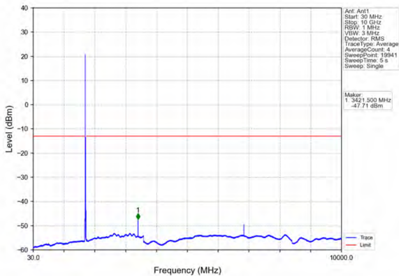
Band66_15MHz_64QAM_LCH_1717.5MHz_RB_1_0_NTNV
