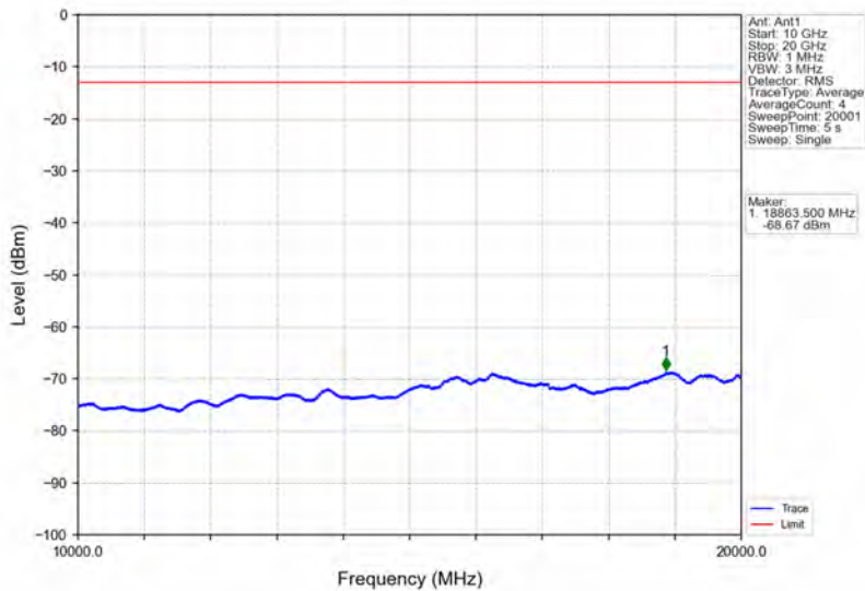
Band66_15MHz_64QAM_MCH_1745MHz_RB_1_0_NTNV
