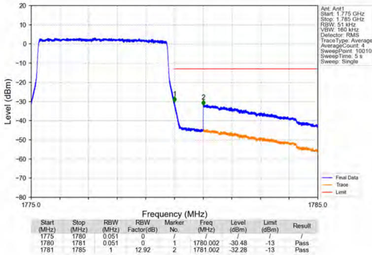
Band66_5MHz_16QAM_HCH_1777.5MHz_RB_25_0_NTNV
