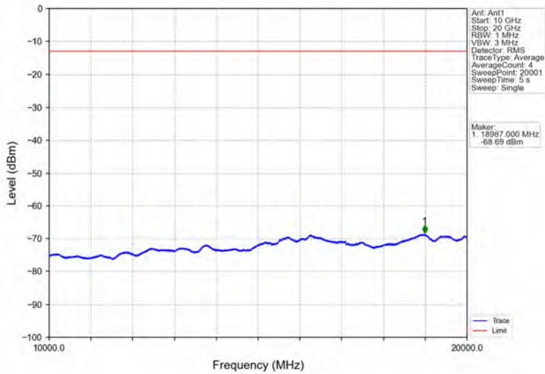
Band66_1.4MHz_64QAM_LCH_1710.7MHz_RB_6_0_NTNV
