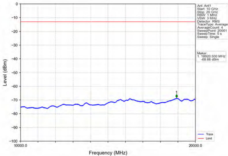
Band66_3MHz_64QAM_MCH_1745MHz_RB_1_0_NTNV
