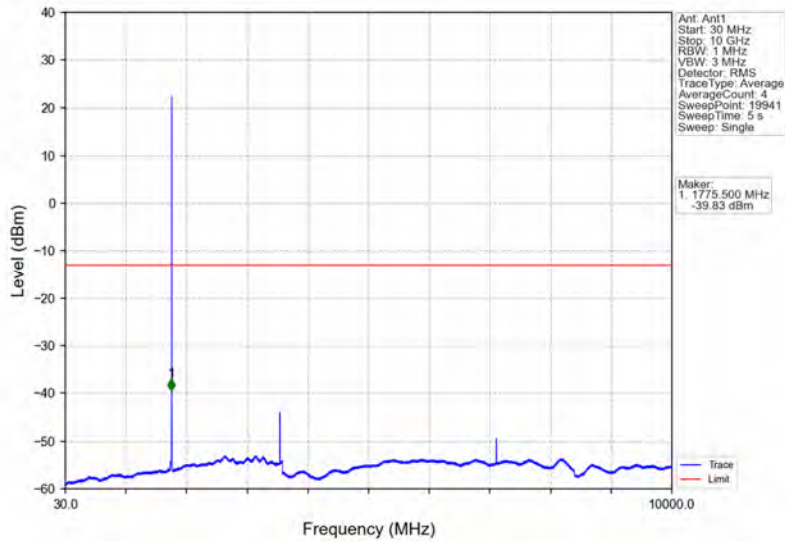
Band66_1.4MHz_QPSK_HCH_1779.3MHz_RB_1_0_NTNV
