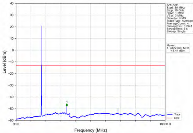
Band66_20MHz_64QAM_LCH_1720MHz_RB_1_0_NTNV
