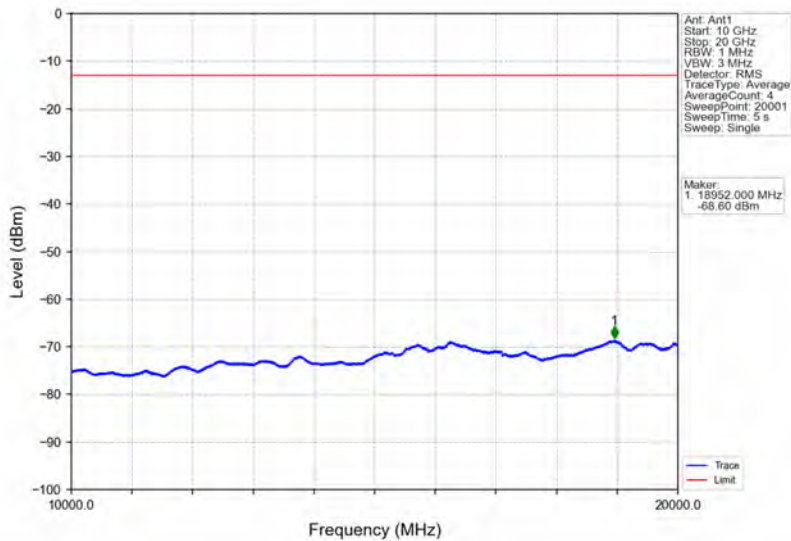
Band66_3MHz_QPSK_HCH_1778.5MHz_RB_1_0_NTNV
