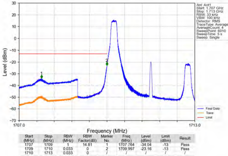
Band66_3MHz_16QAM_LCH_1711.5MHz_RB_1_0_NTNV
