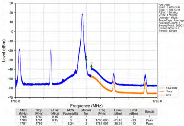
Band66_15MHz_64QAM_HCH_1772.5MHz_RB_1_74_NTNV
