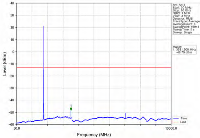
Band66_15MHz_16QAM_HCH_1772.5MHz_RB_1_0_NTNV
