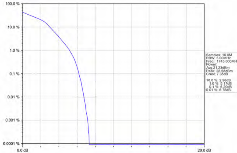
Band66_3MHz_16QAM_MCH_1745MHz_RB_15_0_NTNV
