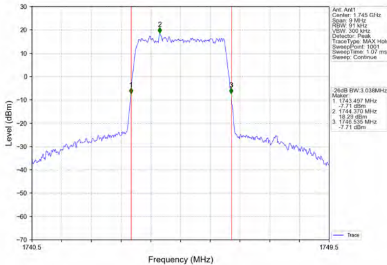
Band66_3MHz_16QAM_MCH_1745MHz_RB_15_0_NTNV
