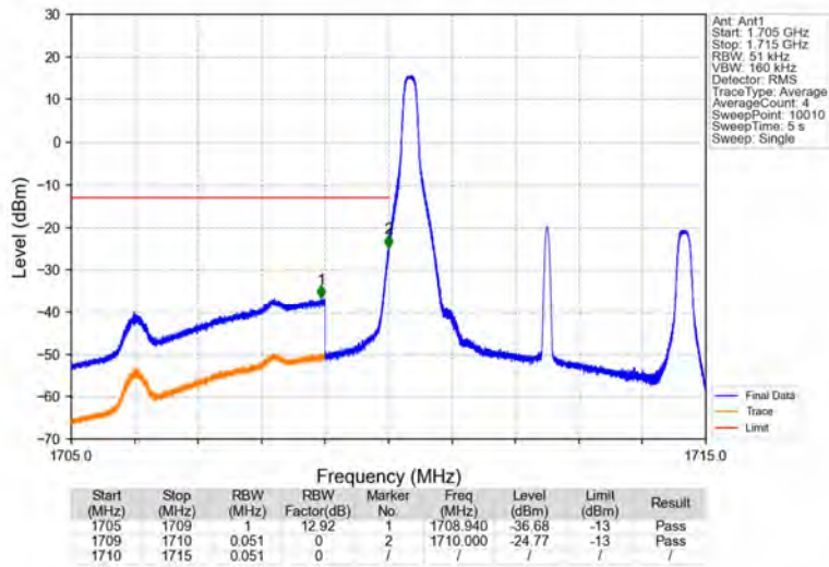
Band66_5MHz_64QAM_LCH_1712.5MHz_RB_1_0_NTNV
