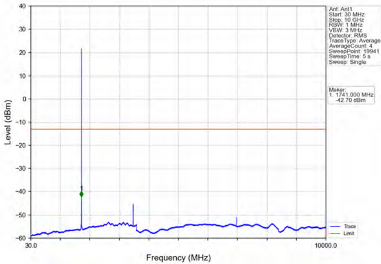
Band66_1.4MHz_16QAM_MCH_1745MHz_RB_1_0_NTNV
