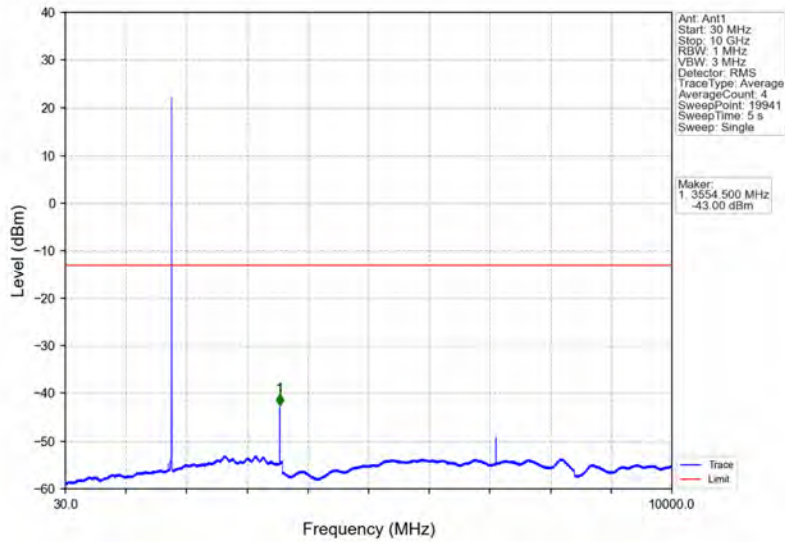
Band66_3MHz_QPSK_HCH_1778.5MHz_RB_1_0_NTNV
