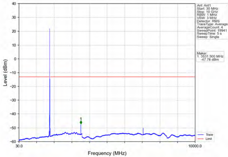
Band66_15MHz_QPSK_HCH_1772.5MHz_RB_1_0_NTNV
