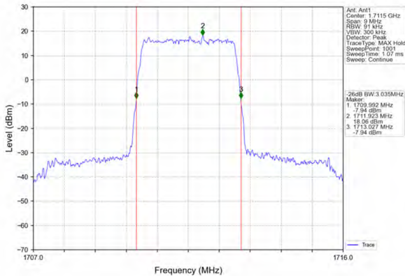
Band66_3MHz_QPSK_LCH_1711.5MHz_RB_15_0_NTNV
