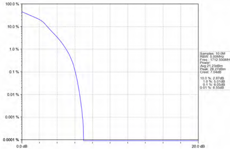
Band66_5MHz_16QAM_LCH_1712.5MHz_RB_25_0_NTNV
