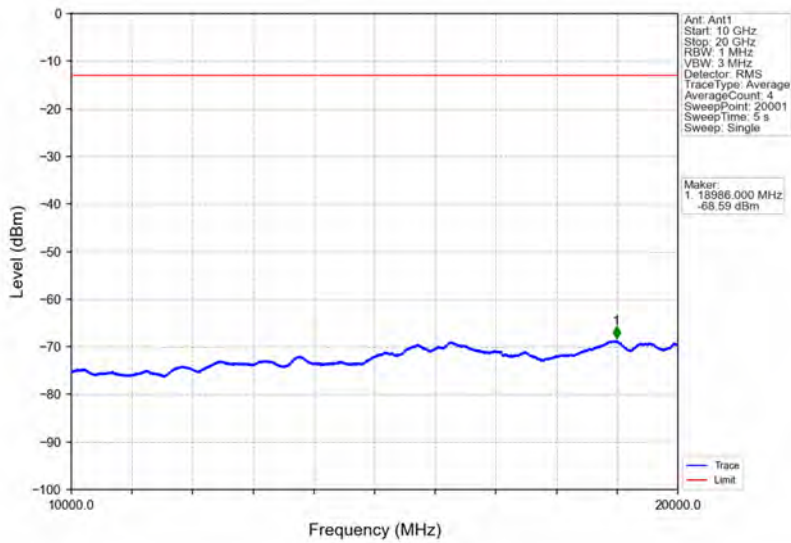
Band66_15MHz_64QAM_HCH_1772.5MHz_RB_1_0_NTNV
