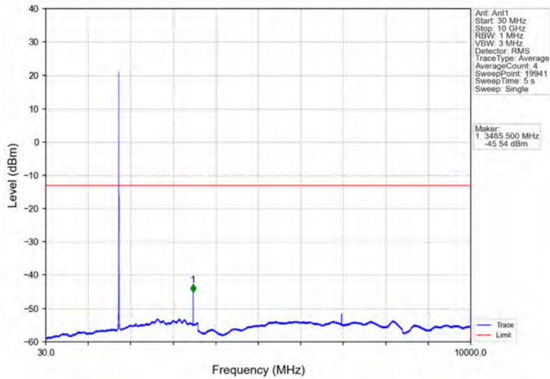
Band66_5MHz_64QAM_MCH_1745MHz_RB_1_0_NTNV
