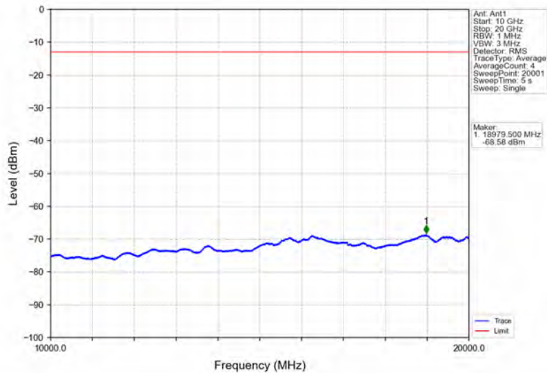
Band66_15MHz_QPSK_MCH_1745MHz_RB_1_0_NTNV
