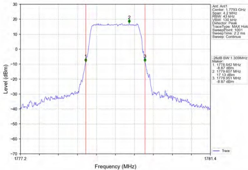
Band66_1.4MHz_16QAM_HCH_1779.3MHz_RB_6_0_NTNV
