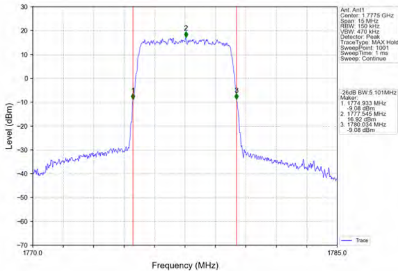
Band66_5MHz_16QAM_HCH_1777.5MHz_RB_25_0_NTNV
