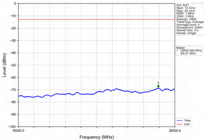
Band66_10MHz_64QAM_MCH_1745MHz_RB_1_0_NTNV
