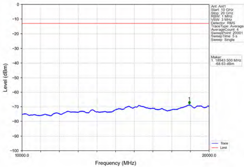
Band66_10MHz_16QAM_LCH_1715MHz_RB_50_0_NTNV
