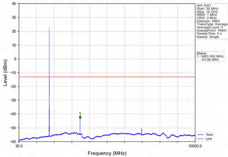
Band66_5MHz_16QAM_MCH_1745MHz_RB_1_0_NTNV
