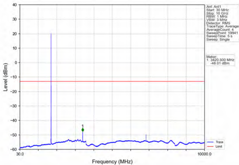
Band66_5MHz_64QAM_LCH_1712.5MHz_RB_1_0_NTNV
