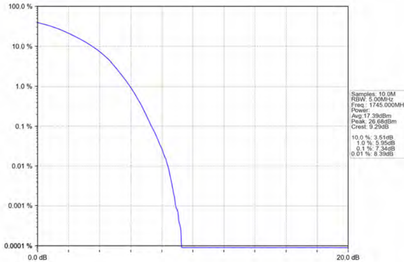
Band66_15MHz_16QAM_MCH_1745MHz_RB_75_0_NTNV
