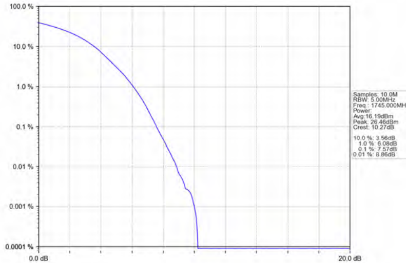
Band66_20MHz_16QAM_MCH_1745MHz_RB_100_0_NTNV
