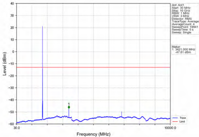
Band66_10MHz_64QAM_LCH_1715MHz_RB_1_0_NTNV
