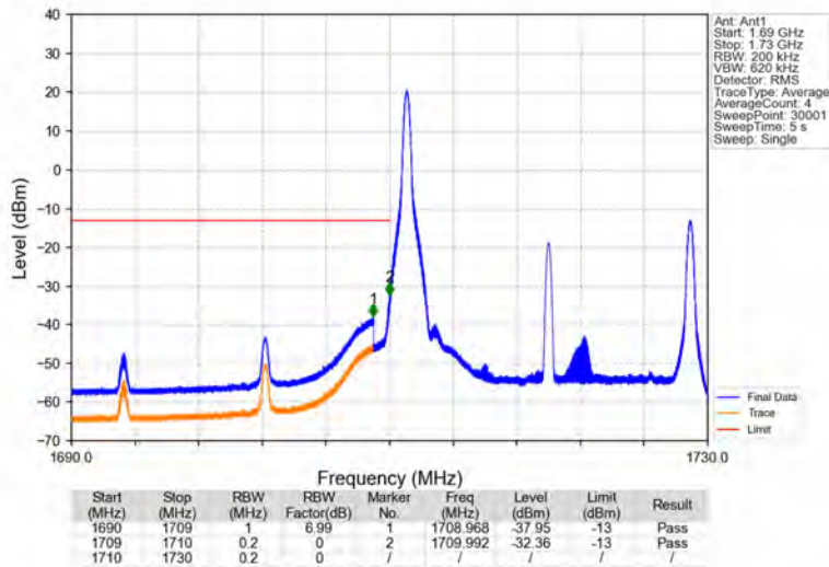
Band66_20MHz_64QAM_LCH_1720MHz_RB_1_0_NTNV
