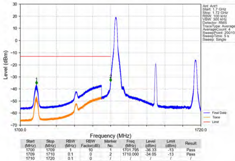
Band66_10MHz_64QAM_LCH_1715MHz_RB_1_0_NTNV
