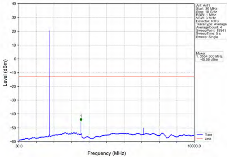
Band66_3MHz_64QAM_HCH_1778.5MHz_RB_1_0_NTNV
