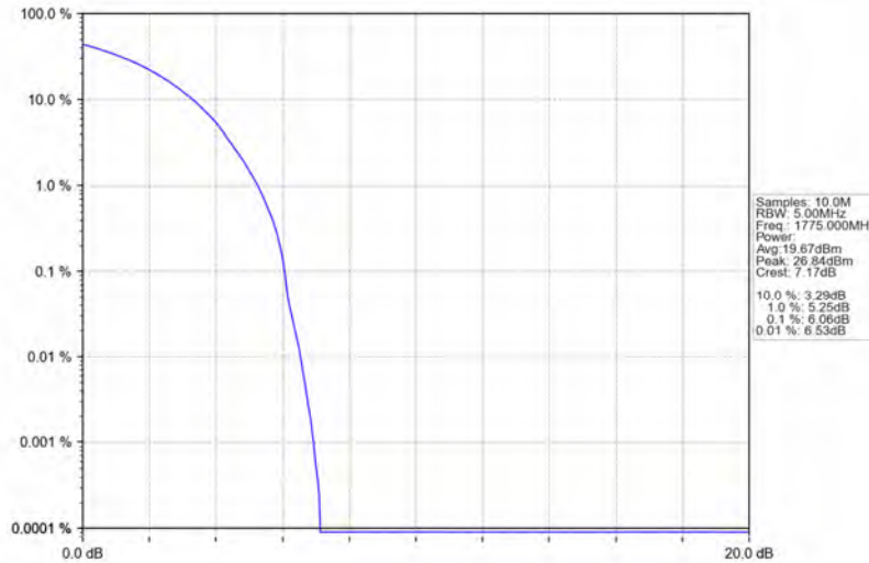
Band66_10MHz_QPSK_HCH_1775MHz_RB_50_0_NTNV
