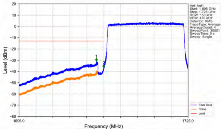
Band66_15MHz_16QAM_LCH_1717.5MHz_RB_75_0_NTNV
