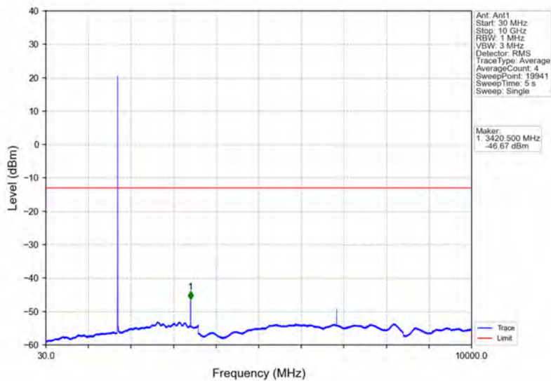
Band66_3MHz_64QAM_LCH_1711.5MHz_RB_1_0_NTNV
