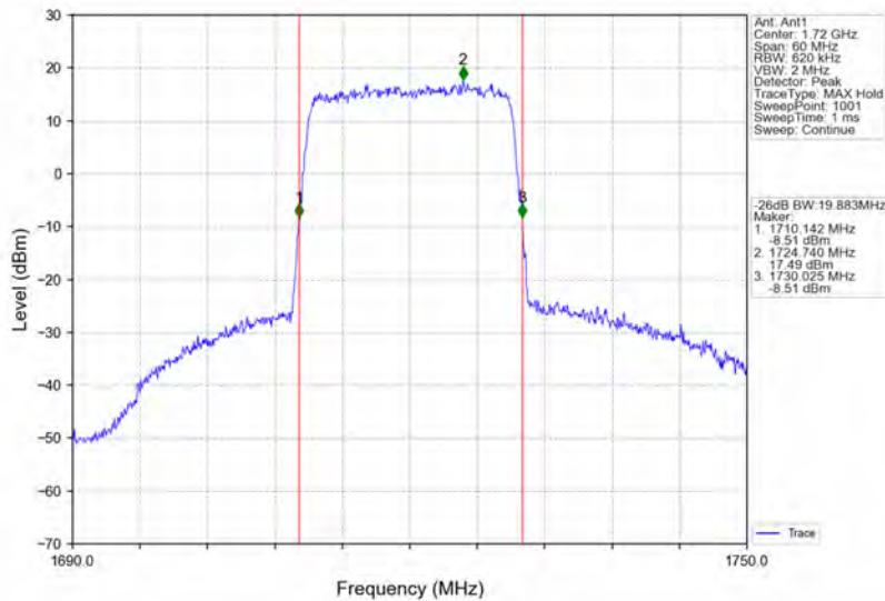
Band66_20MHz_64QAM_LCH_1720MHz_RB_100_0_NTNV
