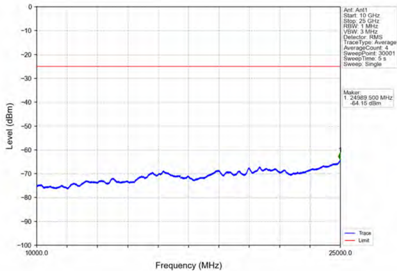
Band41_5MHz_16QAM_MCH_2593MHz_RB_1_0_NTNV
