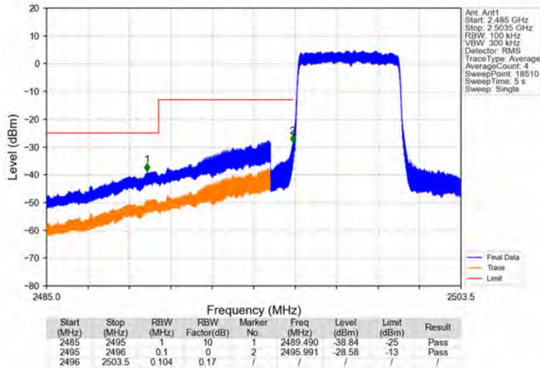
Band41_5MHz_16QAM_LCH_2498.5MHz_RB_25_0_NTNV
