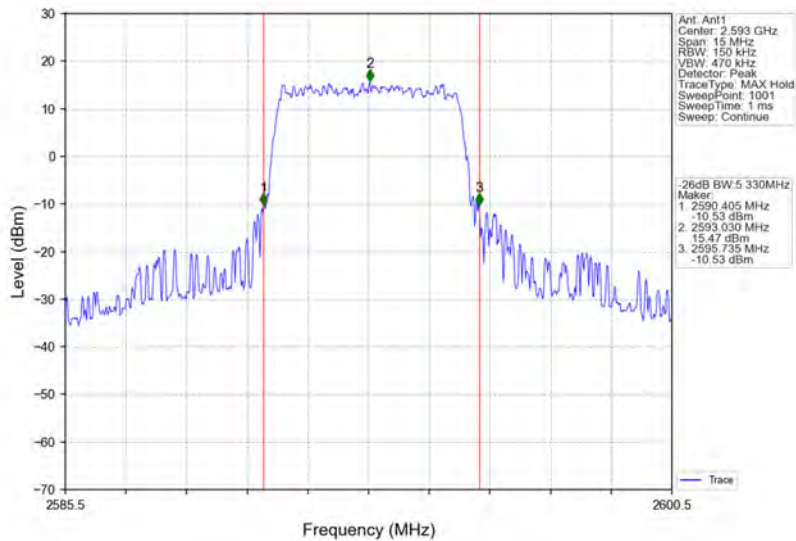
Band41_5MHz_64QAM_MCH_2593MHz_RB_25_0_NTNV
