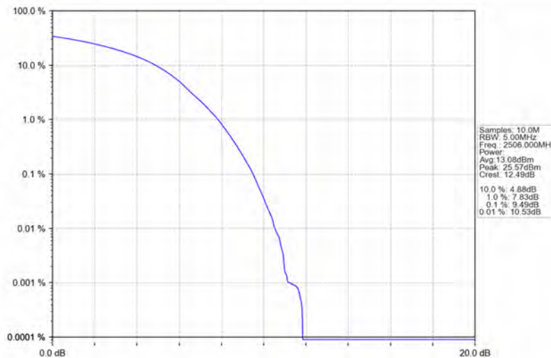
Band41_20MHz_16QAM_LCH_2506MHz_RB_100_0_NTNV
