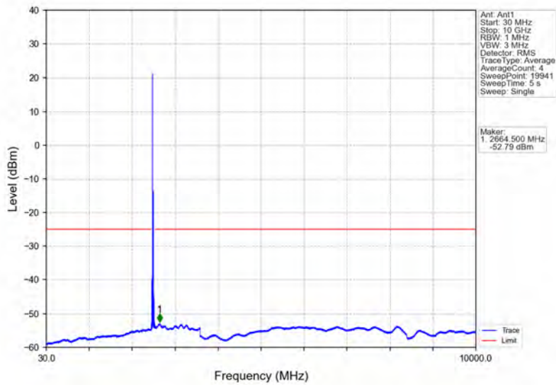
Band41_20MHz_16QAM_LCH_2506MHz_RB_1_0_NTNV
