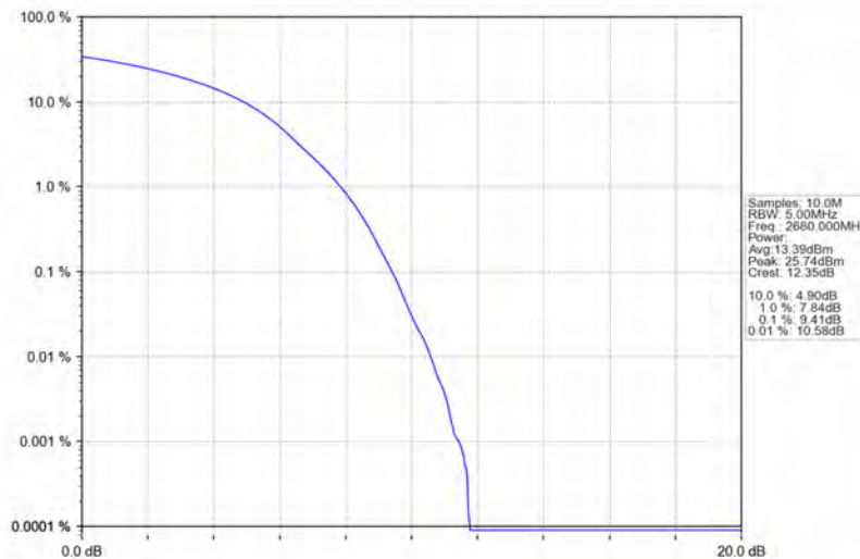
Band41_20MHz_16QAM_HCH_2680MHz_RB_100_0_NTNV
