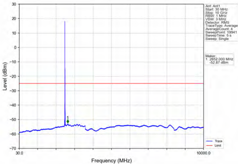
Band41_10MHz_64QAM_LCH_2501MHz_RB_1_0_NTNV
