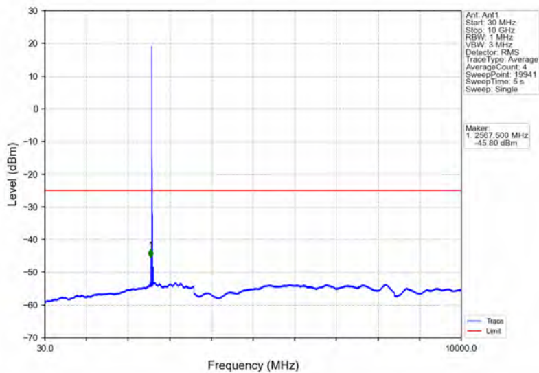
Band41_10MHz_64QAM_MCH_2593MHz_RB_1_0_NTNV
