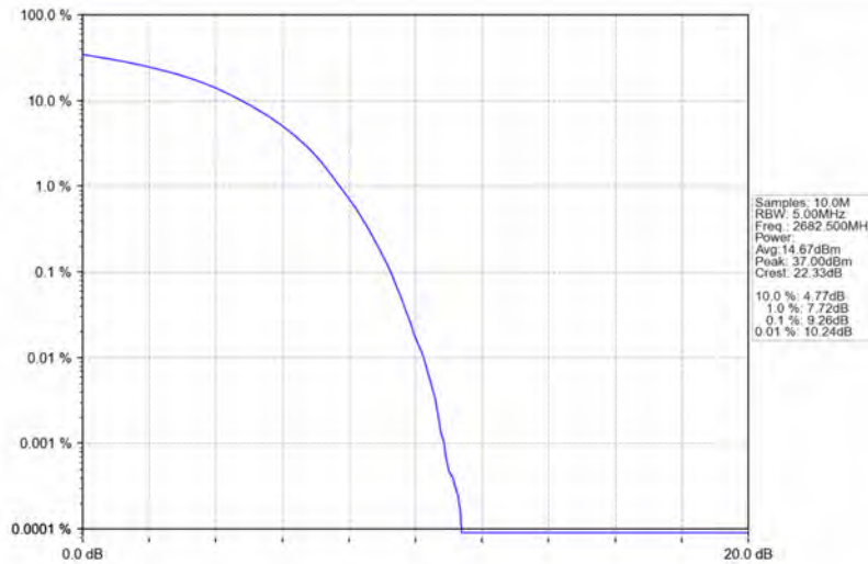
Band41_15MHz_16QAM_HCH_2682.5MHz_RB_75_0_NTNV
