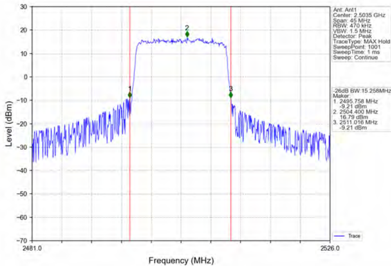
Band41_15MHz_16QAM_LCH_2503.5MHz_RB_75_0_NTNV
