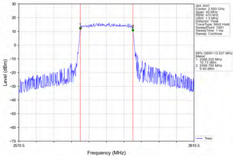
Band41_15MHz_64QAM_MCH_2593MHz_RB_75_0_NTNV
