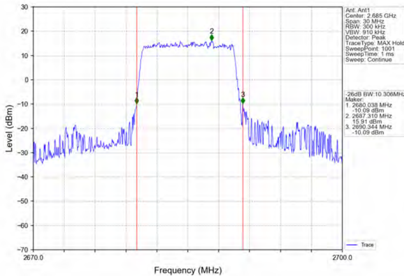
Band41_10MHz_64QAM_HCH_2685MHz_RB_50_0_NTNV
