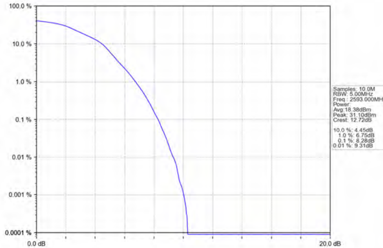
Band41_5MHz_16QAM_MCH_2593MHz_RB_25_0_NTNV
