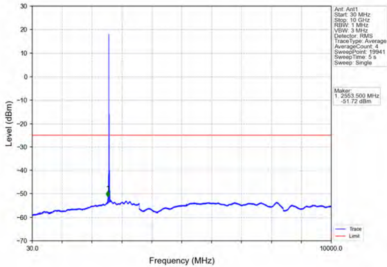
Band41_15MHz_16QAM_MCH_2593MHz_RB_1_0_NTNV
