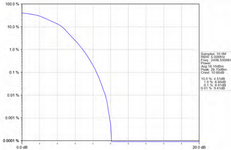
Band41_5MHz_16QAM_LCH_2498.5MHz_RB_25_0_NTNV
