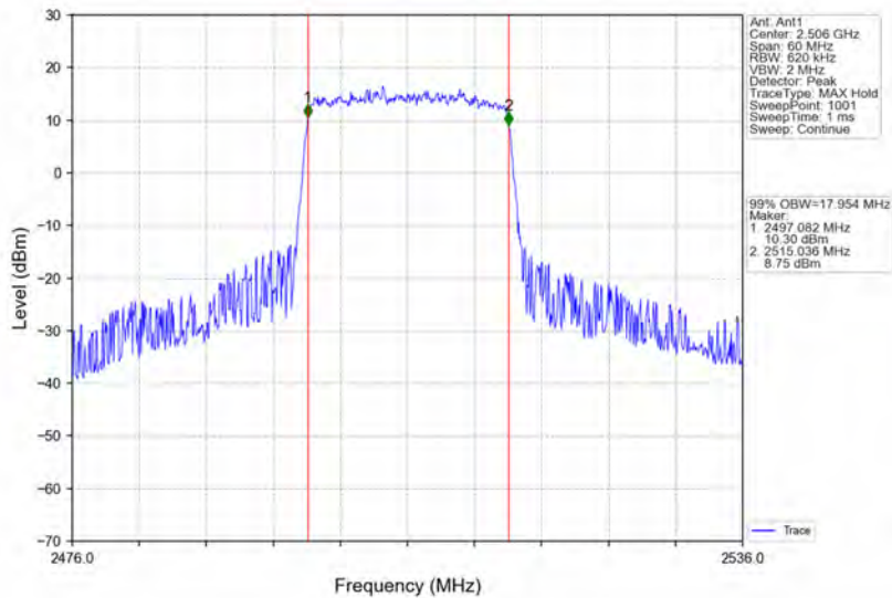
Band41_20MHz_64QAM_LCH_2506MHz_RB_100_0_NTNV
