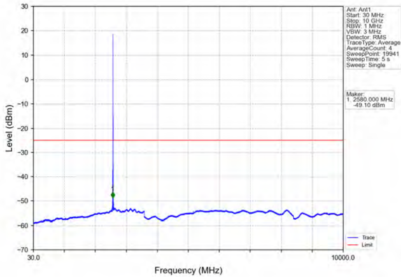
Band41_5MHz_16QAM_MCH_2593MHz_RB_1_0_NTNV
