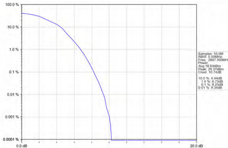
Band41_5MHz_16QAM_HCH_2687.5MHz_RB_25_0_NTNV
