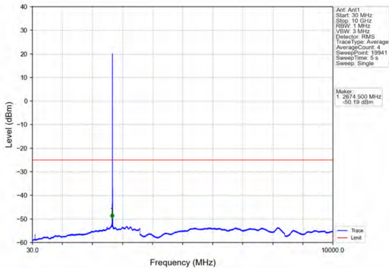
Band41_5MHz_16QAM_HCH_2687.5MHz_RB_1_0_NTNV
