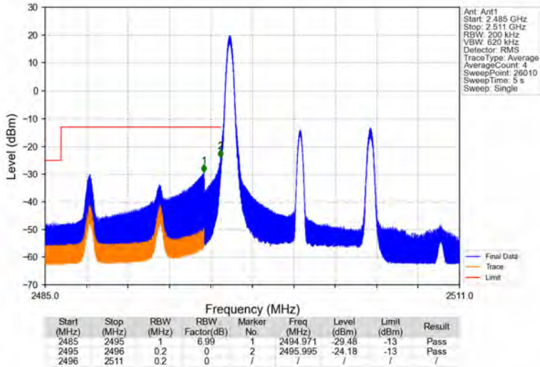
Band41_10MHz_64QAM_LCH_2501MHz_RB_1_0_NTNV
