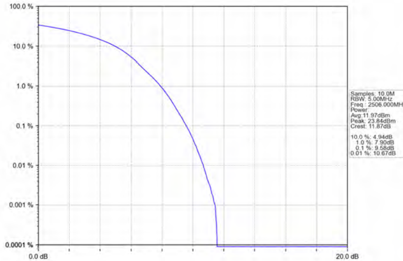
Band41_20MHz_64QAM_LCH_2506MHz_RB_100_0_NTNV
