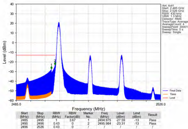
Band41_20MHz_16QAM_LCH_2506MHz_RB_1_0_NTNV
