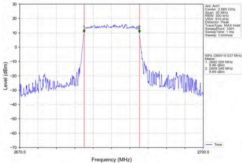
Band41_10MHz_64QAM_HCH_2685MHz_RB_50_0_NTNV
