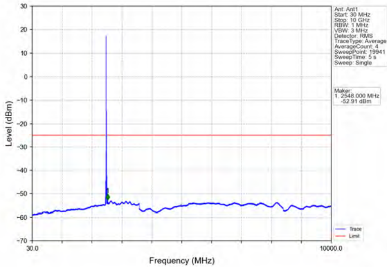
Band41_15MHz_16QAM_LCH_2503.5MHz_RB_1_0_NTNV
