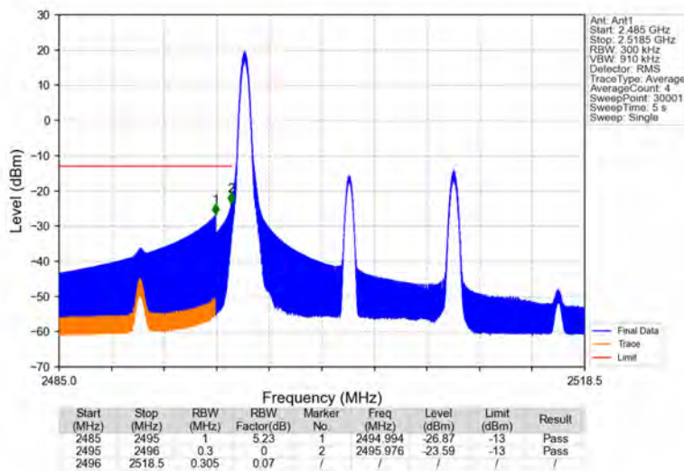
Band41_15MHz_16QAM_LCH_2503.5MHz_RB_1_0_NTNV
