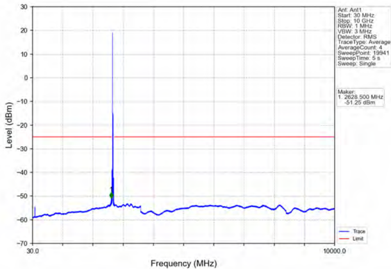
Band41_20MHz_16QAM_HCH_2680MHz_RB_1_0_NTNV
