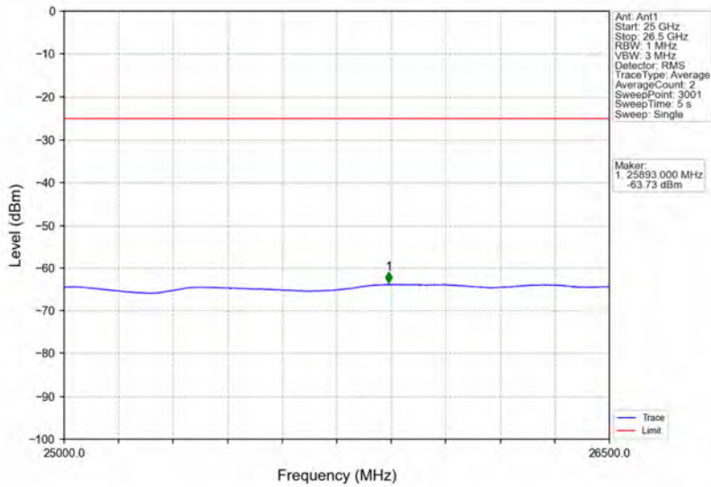
Band41_20MHz_64QAM_HCH_2680MHz_RB_1_99_NTNV
