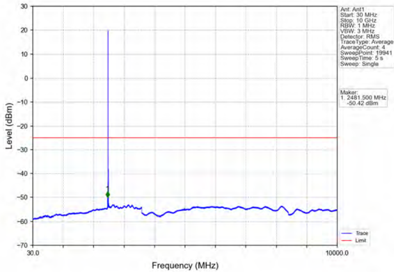
Band41_5MHz_16QAM_LCH_2498.5MHz_RB_1_0_NTNV
