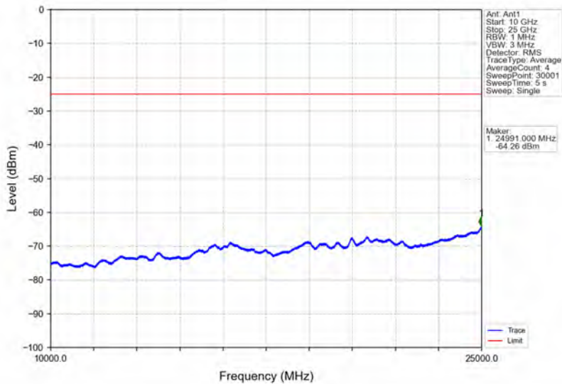
Band41_20MHz_16QAM_LCH_2506MHz_RB_1_0_NTNV
