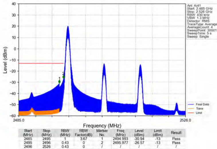
Band41_20MHz_64QAM_LCH_2506MHz_RB_1_0_NTNV
