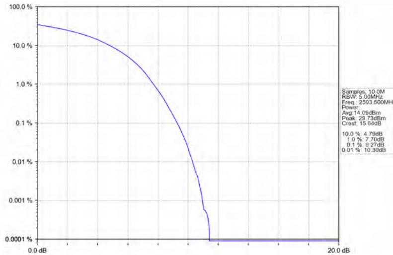
Band41_15MHz_16QAM_LCH_2503.5MHz_RB_75_0_NTNV
