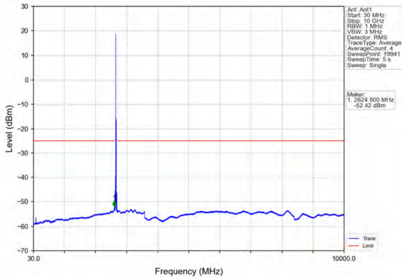
Band41_20MHz_64QAM_HCH_2680MHz_RB_1_0_NTNV
