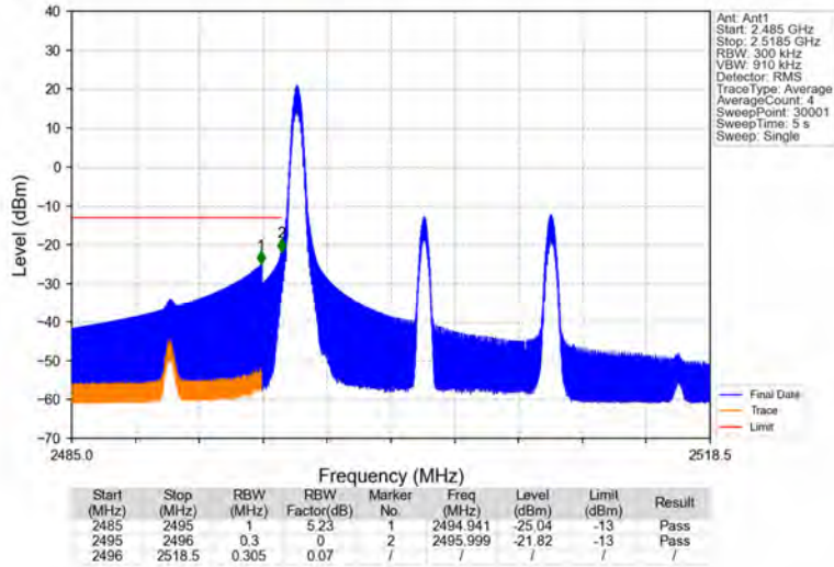
Band41_15MHz_64QAM_LCH_2503.5MHz_RB_1_0_NTNV
