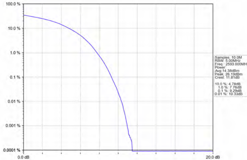
Band41_15MHz_16QAM_MCH_2593MHz_RB_75_0_NTNV
