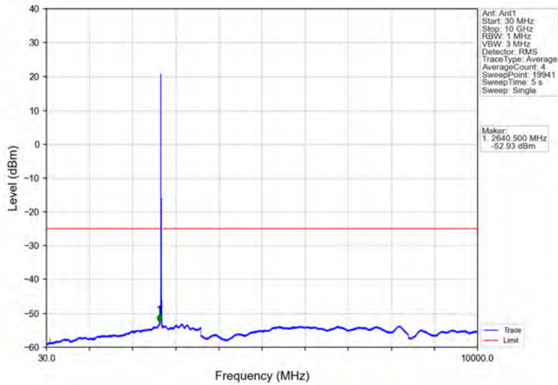
Band41_15MHz_64QAM_HCH_2682.5MHz_RB_1_0_NTNV
