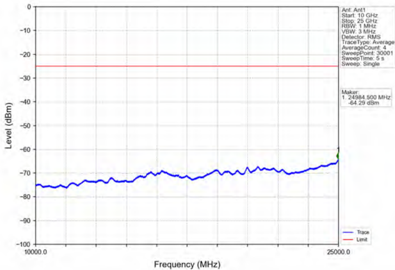
Band41_5MHz_64QAM_HCH_2687.5MHz_RB_1_0_NTNV
