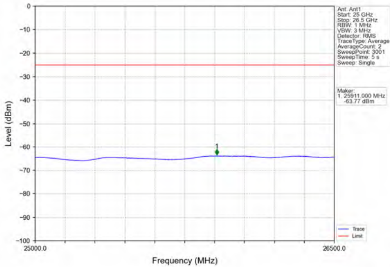
Band41_15MHz_64QAM_HCH_2682.5MHz_RB_1_74_NTNV
