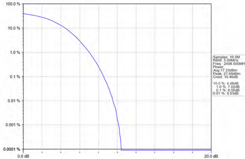
Band41_5MHz_64QAM_LCH_2498.5MHz_RB_25_0_NTNV
