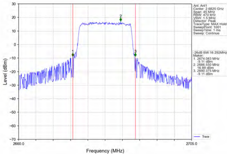
Band41_15MHz_16QAM_HCH_2682.5MHz_RB_75_0_NTNV
