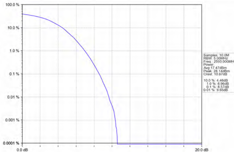
Band41_5MHz_64QAM_MCH_2593MHz_RB_25_0_NTNV
