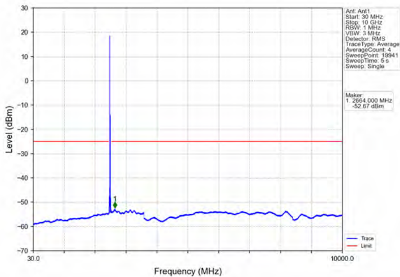
Band41_20MHz_64QAM_LCH_2506MHz_RB_1_0_NTNV
