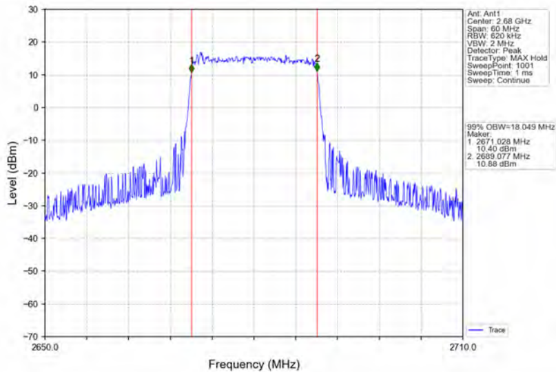
Band41_20MHz_64QAM_HCH_2680MHz_RB_100_0_NTNV
