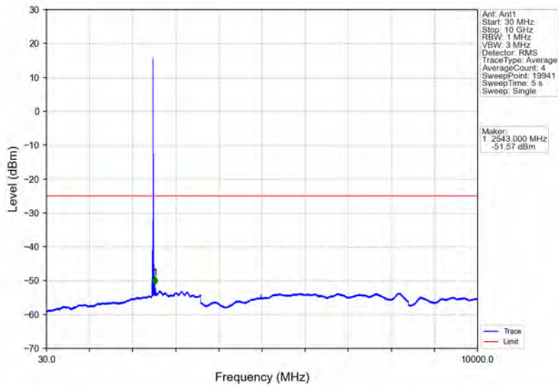
Band41_15MHz_64QAM_LCH_2503.5MHz_RB_1_0_NTNV
