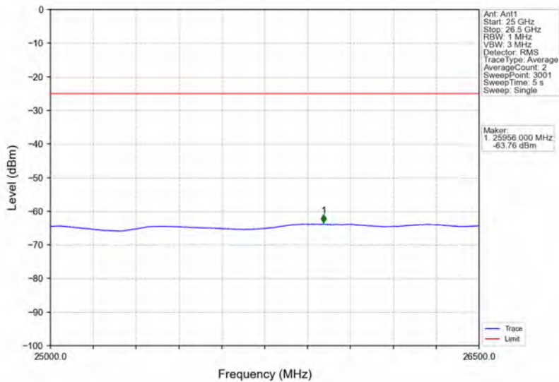
Band41_10MHz_64QAM_MCH_2593MHz_RB_1_0_NTNV
