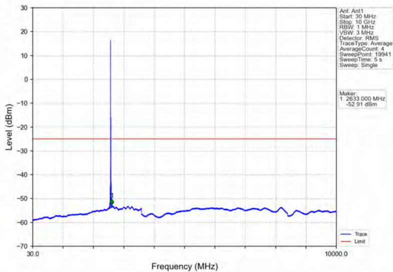
Band41_15MHz_64QAM_MCH_2593MHz_RB_1_0_NTNV
