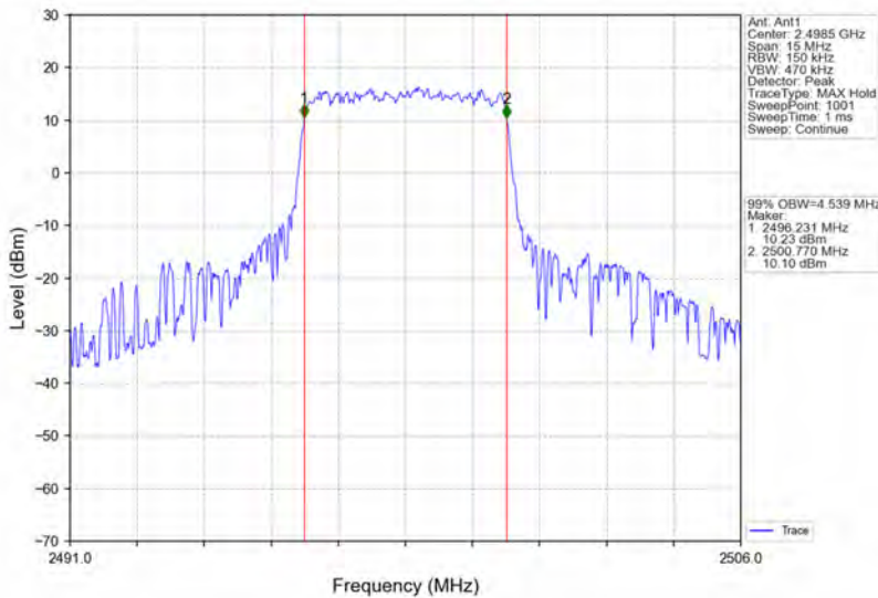
Band41_5MHz_16QAM_LCH_2498.5MHz_RB_25_0_NTNV
