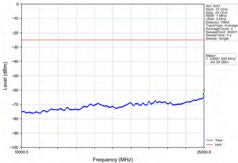
Band41_10MHz_64QAM_HCH_2685MHz_RB_1_0_NTNV
