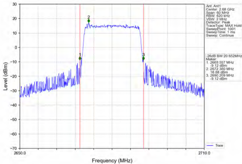
Band41_20MHz_64QAM_HCH_2680MHz_RB_100_0_NTNV
