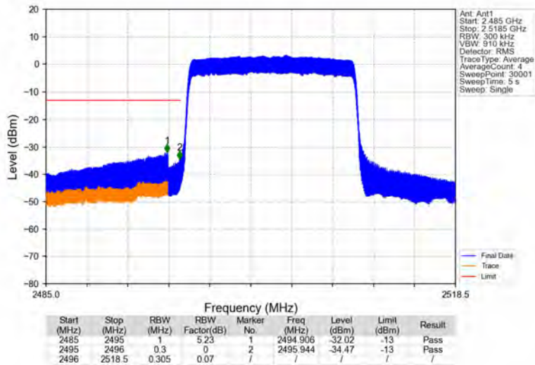
Band41_15MHz_64QAM_LCH_2503.5MHz_RB_75_0_NTNV
