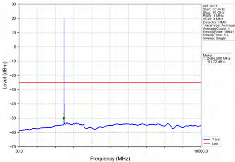
Band41_5MHz_64QAM_LCH_2498.5MHz_RB_1_0_NTNV
