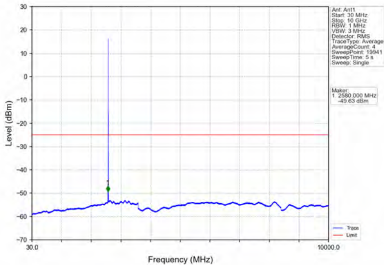
Band41_5MHz_64QAM_MCH_2593MHz_RB_1_0_NTNV
