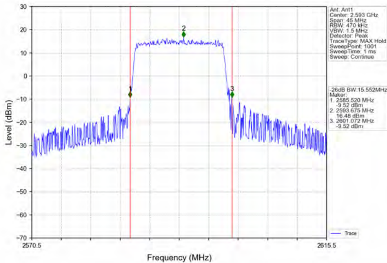
Band41_15MHz_64QAM_MCH_2593MHz_RB_75_0_NTNV
