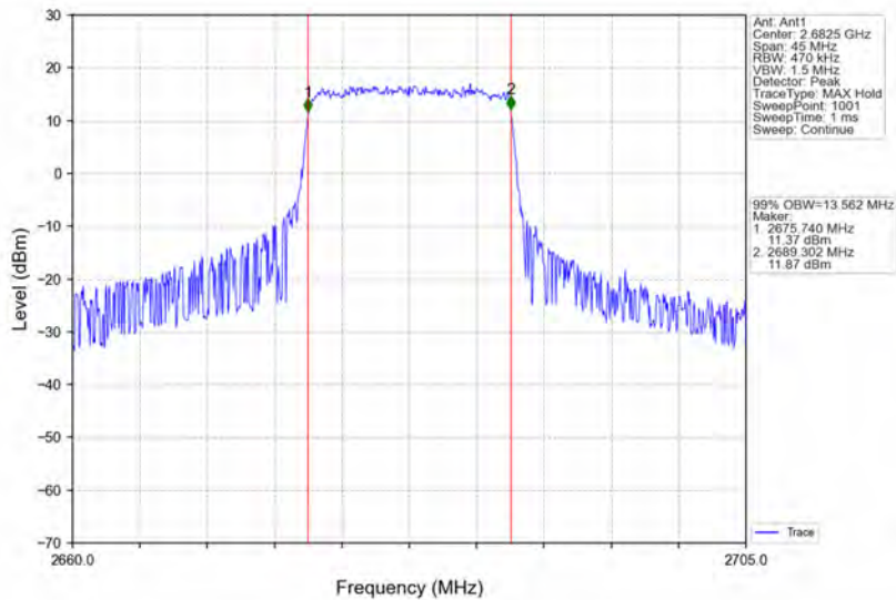
Band41_15MHz_16QAM_HCH_2682.5MHz_RB_75_0_NTNV
