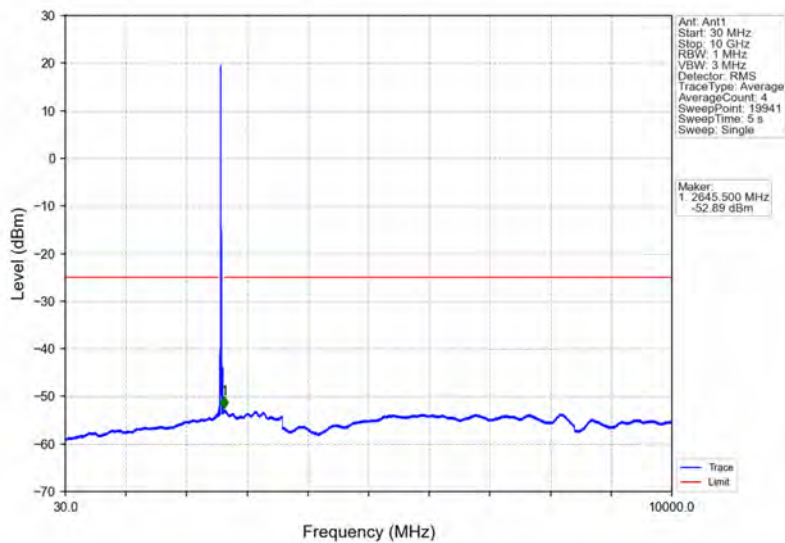
Band41_20MHz_64QAM_MCH_2593MHz_RB_1_0_NTNV
