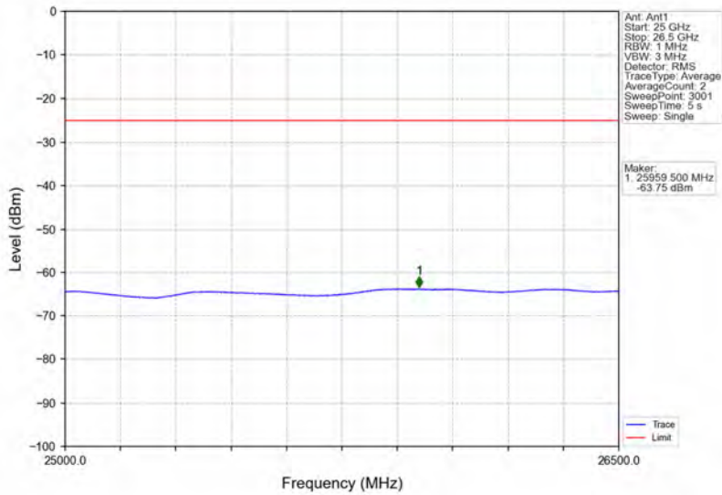
Band41_5MHz_64QAM_HCH_2687.5MHz_RB_1_24_NTNV
