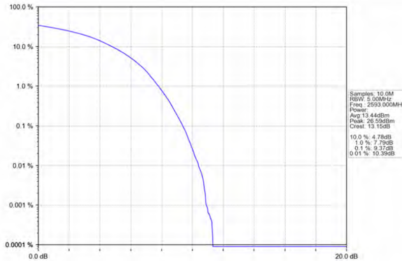
Band41_15MHz_64QAM_MCH_2593MHz_RB_75_0_NTNV
