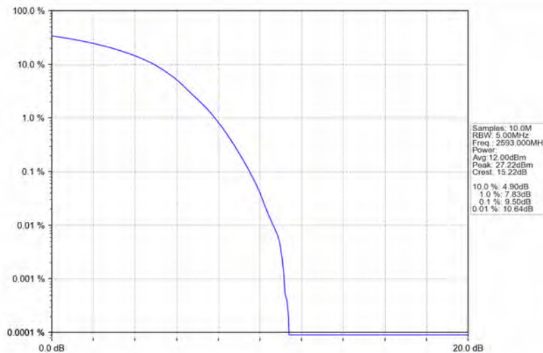
Band41_20MHz_64QAM_MCH_2593MHz_RB_100_0_NTNV
