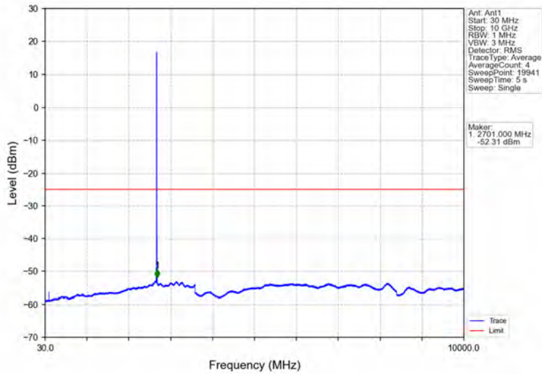
Band41_5MHz_64QAM_HCH_2687.5MHz_RB_1_0_NTNV
