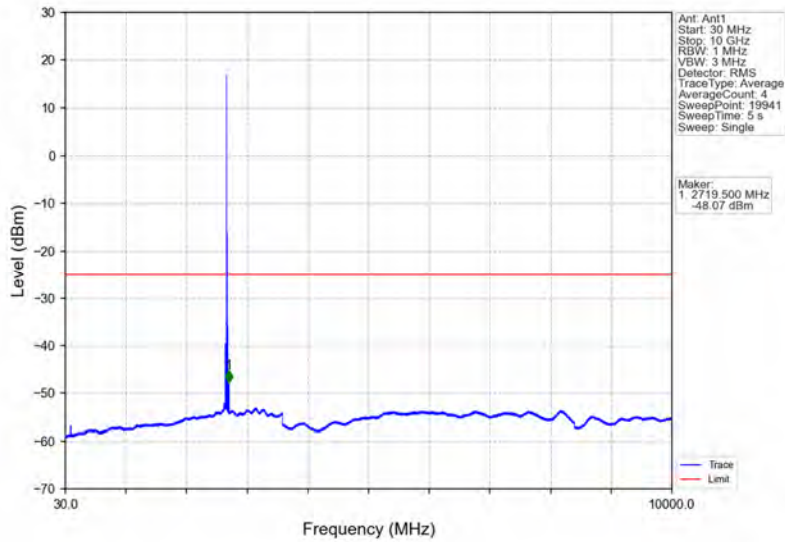
Band41_10MHz_64QAM_HCH_2685MHz_RB_1_0_NTNV
