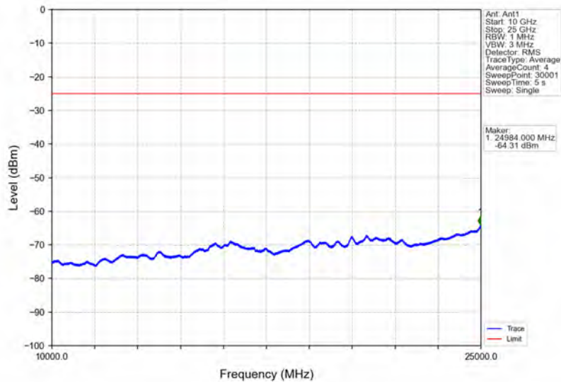
Band41_15MHz_64QAM_HCH_2682.5MHz_RB_1_0_NTNV
