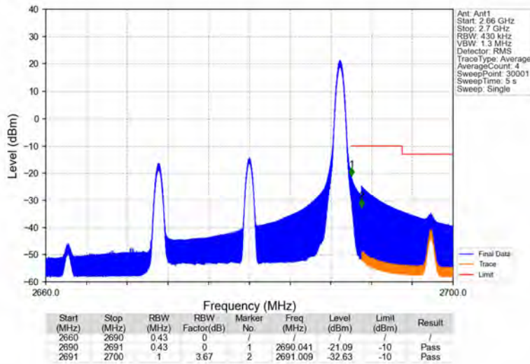
Band41_20MHz_16QAM_HCH_2680MHz_RB_1_99_NTNV
