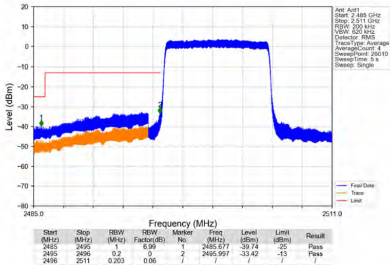
Band41_10MHz_64QAM_LCH_2501MHz_RB_50_0_NTNV
