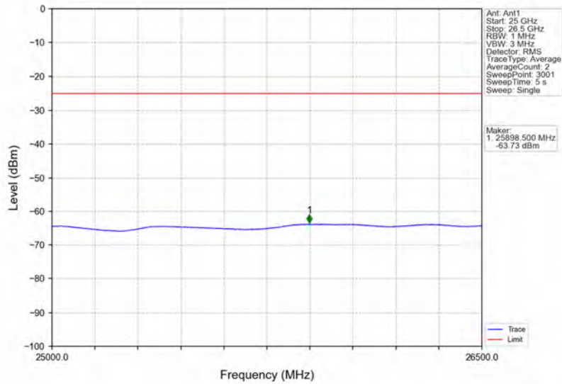
Band41_15MHz_16QAM_LCH_2503.5MHz_RB_75_0_NTNV
