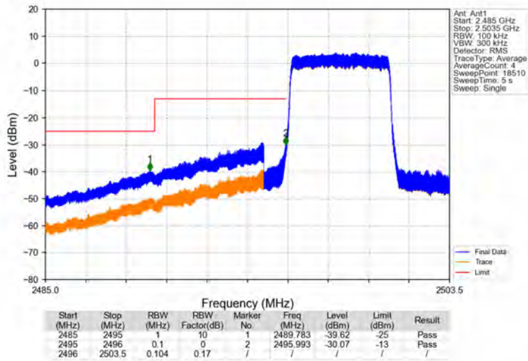
Band41_5MHz_64QAM_LCH_2498.5MHz_RB_25_0_NTNV
