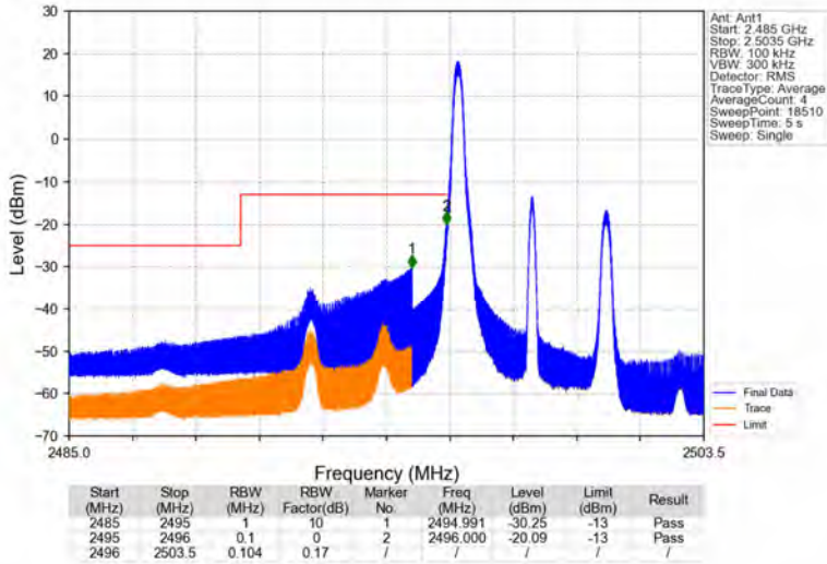
Band41_5MHz_64QAM_LCH_2498.5MHz_RB_1_0_NTNV
