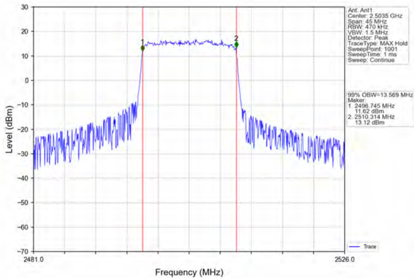
Band41_15MHz_16QAM_LCH_2503.5MHz_RB_75_0_NTNV
