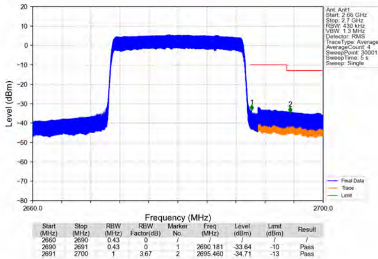
Band41_20MHz_16QAM_HCH_2680MHz_RB_100_0_NTNV
