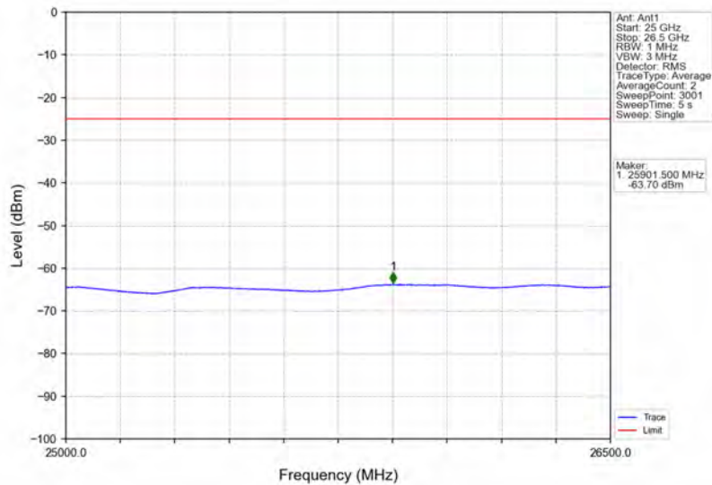
Band41_15MHz_16QAM_HCH_2682.5MHz_RB_1_0_NTNV
