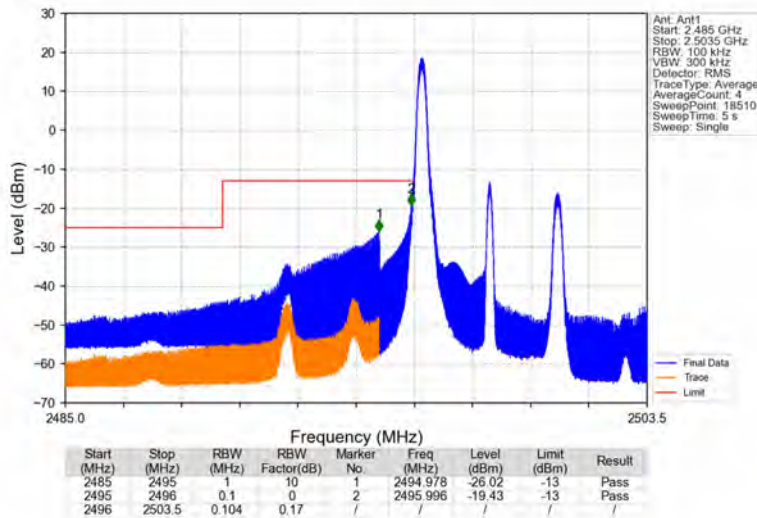
Band41_5MHz_16QAM_LCH_2498.5MHz_RB_1_0_NTNV
