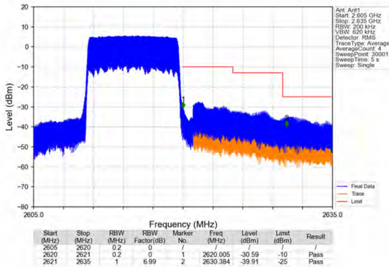
Band38_10MHz_16QAM_HCH_2615MHz_RB_50_0_NTNV
