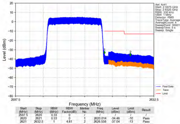
Band38_15MHz_64QAM_HCH_2612.5MHz_RB_75_0_NTNV
