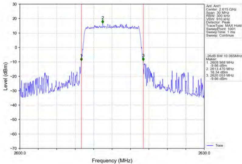
Band38_10MHz_64QAM_HCH_2615MHz_RB_50_0_NTNV
