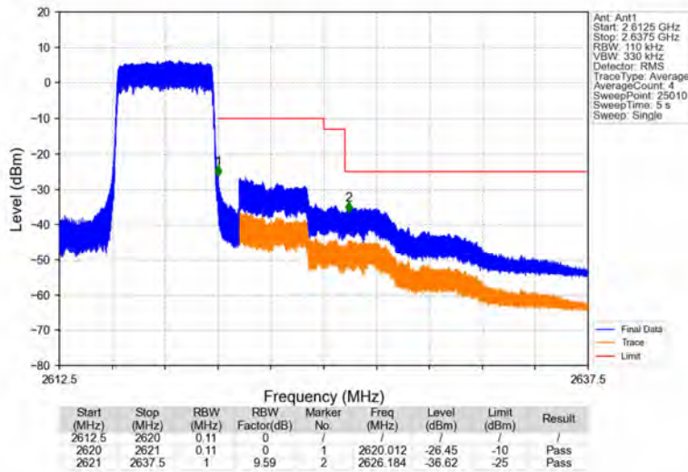
Band38_5MHz_QPSK_HCH_2617.5MHz_RB_25_0_NTNV
