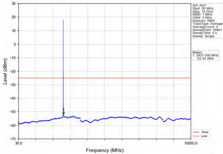
Band38_5MHz_64QAM_HCH_2617.5MHz_RB_1_0_NTNV
