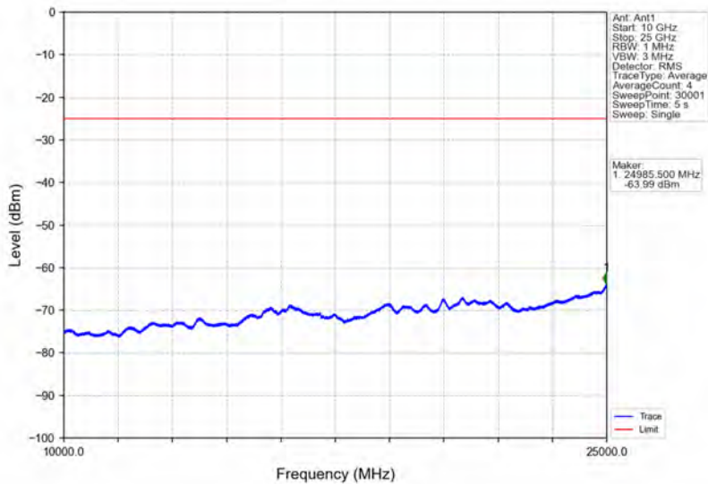
Band38_5MHz_16QAM_MCH_2595MHz_RB_1_0_NTNV
