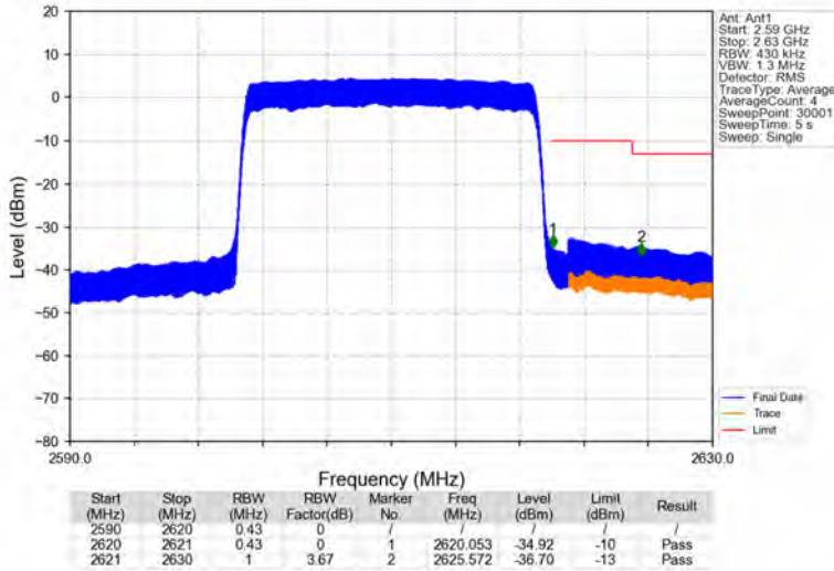
Band38_20MHz_64QAM_HCH_2610MHz_RB_100_0_NTNV
