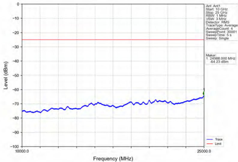
Band38_5MHz_16QAM_LCH_2572.5MHz_RB_1_0_NTNV
