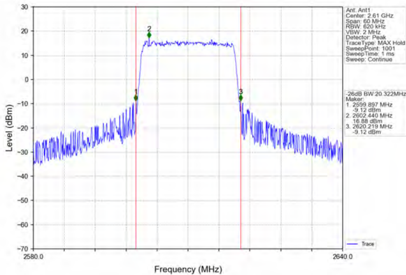
Band38_20MHz_64QAM_HCH_2610MHz_RB_100_0_NTNV
