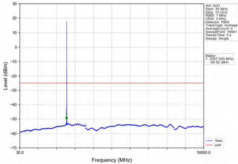
Band38_5MHz_16QAM_LCH_2572.5MHz_RB_1_0_NTNV
