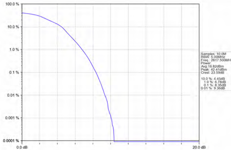
Band38_5MHz_16QAM_HCH_2617.5MHz_RB_25_0_NTNV
