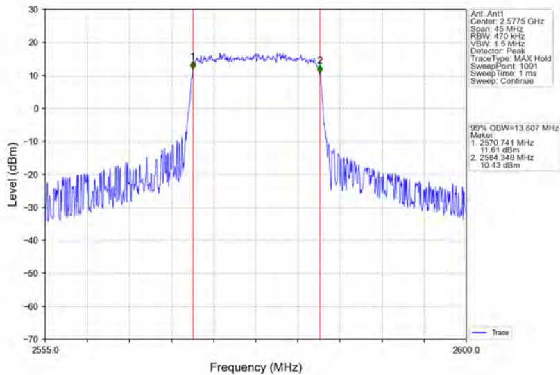
Band38_15MHz_16QAM_LCH_2577.5MHz_RB_75_0_NTNV
