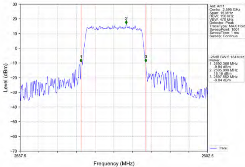
Band38_5MHz_64QAM_MCH_2595MHz_RB_25_0_NTNV
