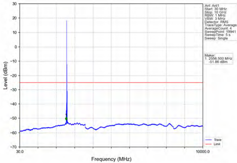
Band38_15MHz_16QAM_MCH_2595MHz_RB_1_0_NTNV
