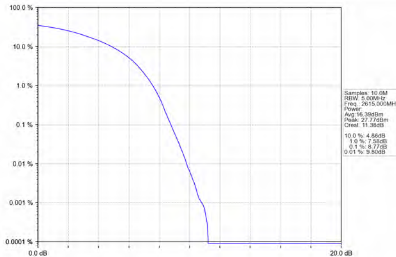
Band38_10MHz_16QAM_HCH_2615MHz_RB_50_0_NTNV
