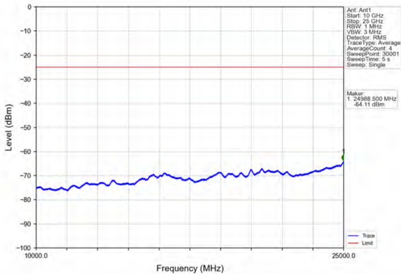
Band38_10MHz_16QAM_LCH_2575MHz_RB_1_0_NTNV
