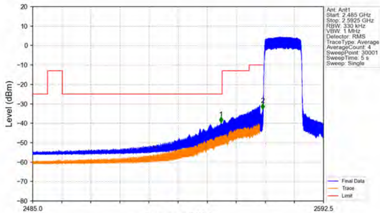
Band38_15MHz_16QAM_LCH_2577.5MHz_RB_75_0_NTNV
