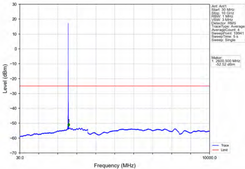
Band38_10MHz_64QAM_LCH_2575MHz_RB_1_0_NTNV
