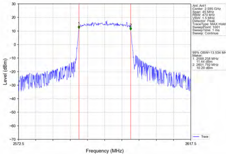
Band38_15MHz_64QAM_MCH_2595MHz_RB_75_0_NTNV
