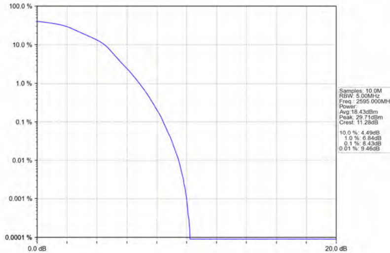
Band38_5MHz_16QAM_MCH_2595MHz_RB_25_0_NTNV
