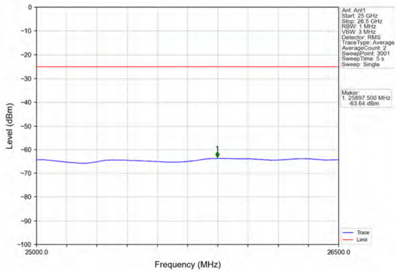
Band38_10MHz_16QAM_LCH_2575MHz_RB_50_0_NTNV
