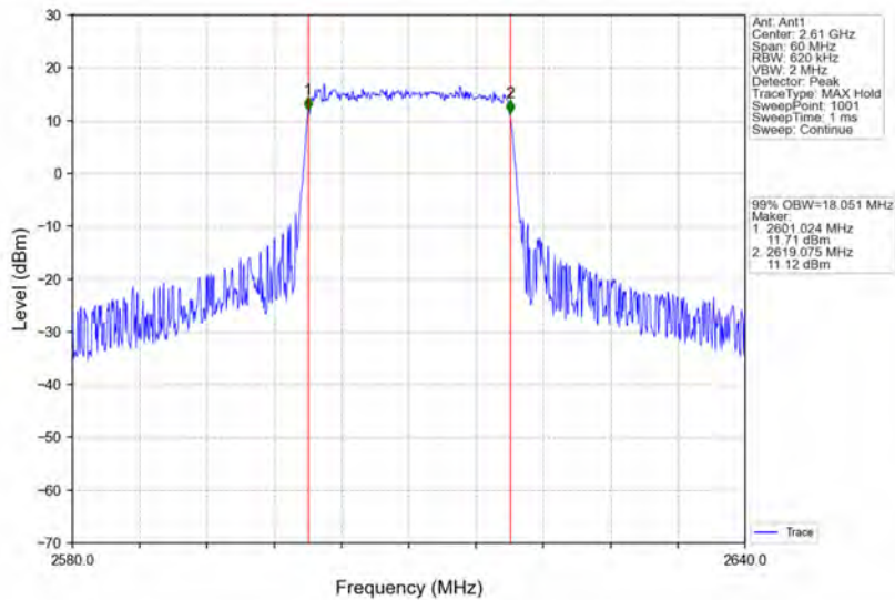
Band38_20MHz_64QAM_HCH_2610MHz_RB_100_0_NTNV
