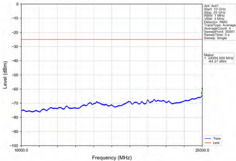
Band38_15MHz_16QAM_MCH_2595MHz_RB_1_0_NTNV
