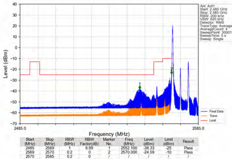
Band38_10MHz_16QAM_LCH_2575MHz_RB_1_0_NTNV
