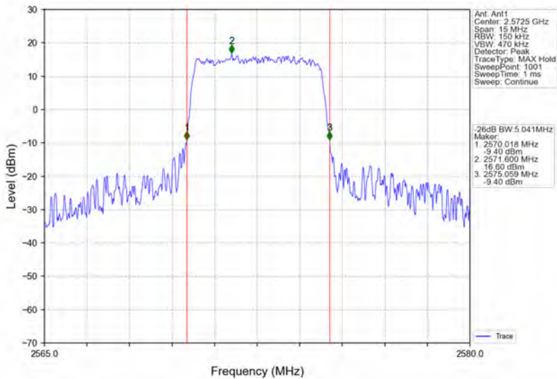
Band38_5MHz_16QAM_LCH_2572.5MHz_RB_25_0_NTNV
