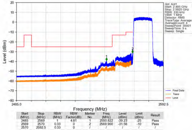
Band38_15MHz_QPSK_LCH_2577.5MHz_RB_75_0_NTNV
