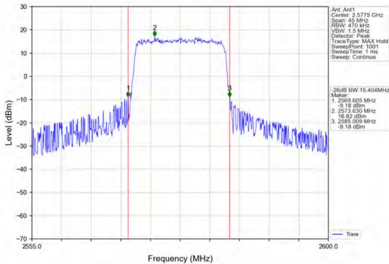
Band38_15MHz_16QAM_LCH_2577.5MHz_RB_75_0_NTNV
