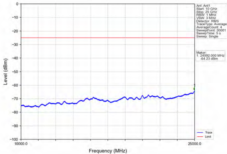
Band38_15MHz_16QAM_LCH_2577.5MHz_RB_1_0_NTNV
