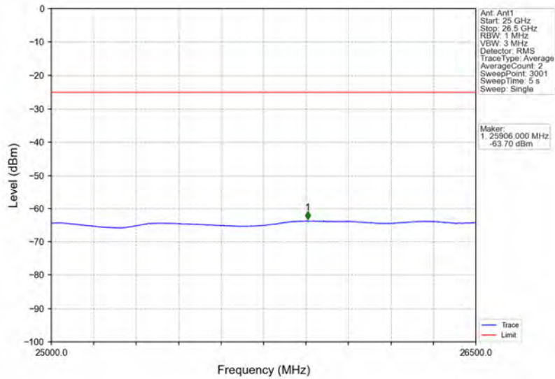
Band38_15MHz_16QAM_LCH_2577.5MHz_RB_75_0_NTNV
