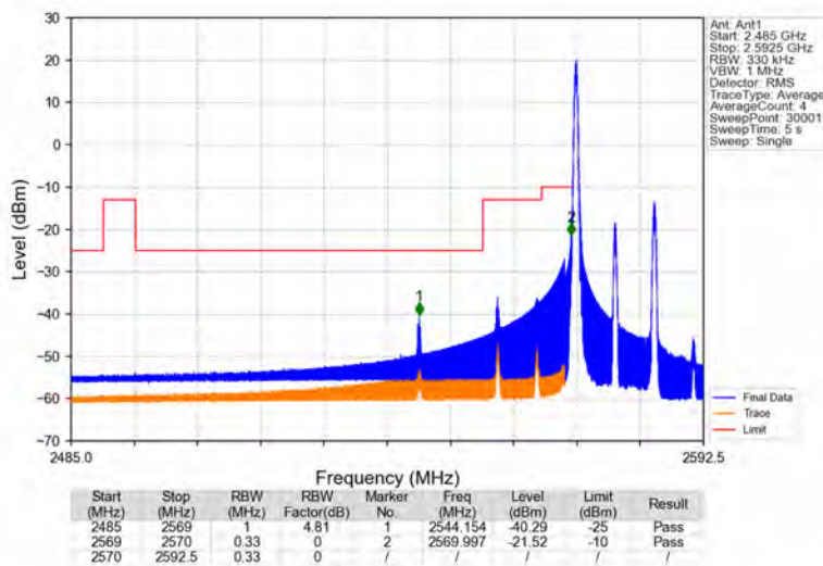
Band38_15MHz_16QAM_LCH_2577.5MHz_RB_1_0_NTNV
