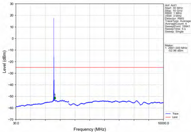
Band38_15MHz_64QAM_MCH_2595MHz_RB_1_0_NTNV
