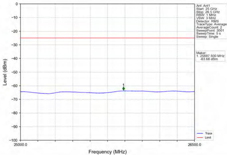
Band38_15MHz_16QAM_HCH_2612.5MHz_RB_1_0_NTNV
