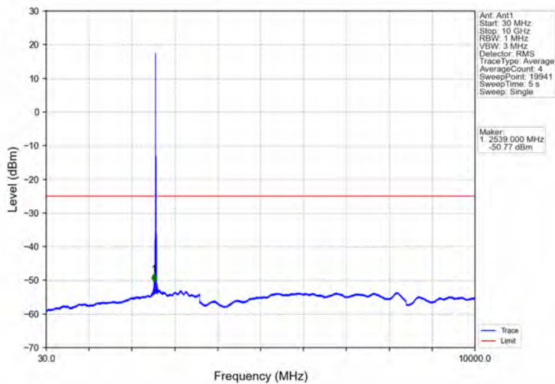
Band38_15MHz_64QAM_LCH_2577.5MHz_RB_1_0_NTNV
