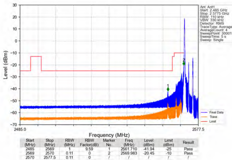
Band38_5MHz_16QAM_LCH_2572.5MHz_RB_1_0_NTNV
