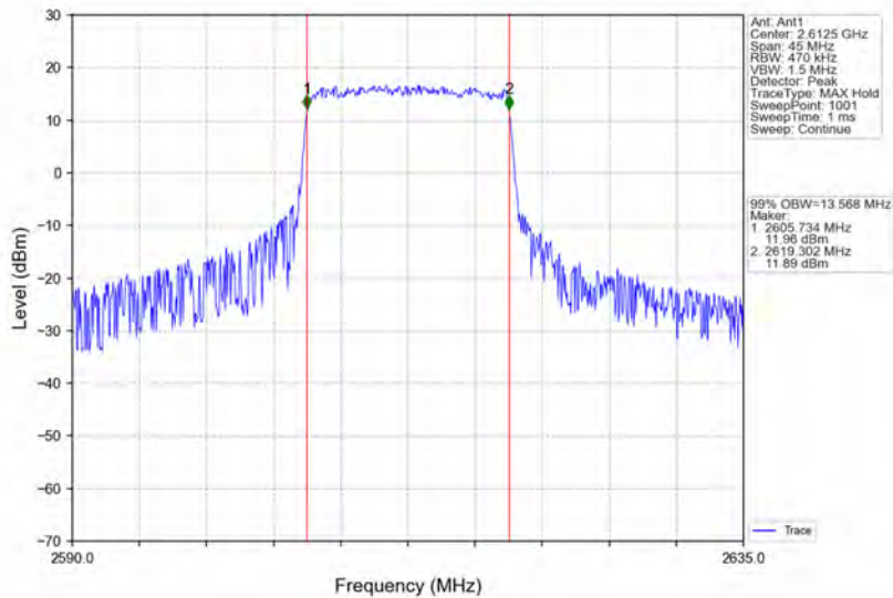
Band38_15MHz_16QAM_HCH_2612.5MHz_RB_75_0_NTNV
