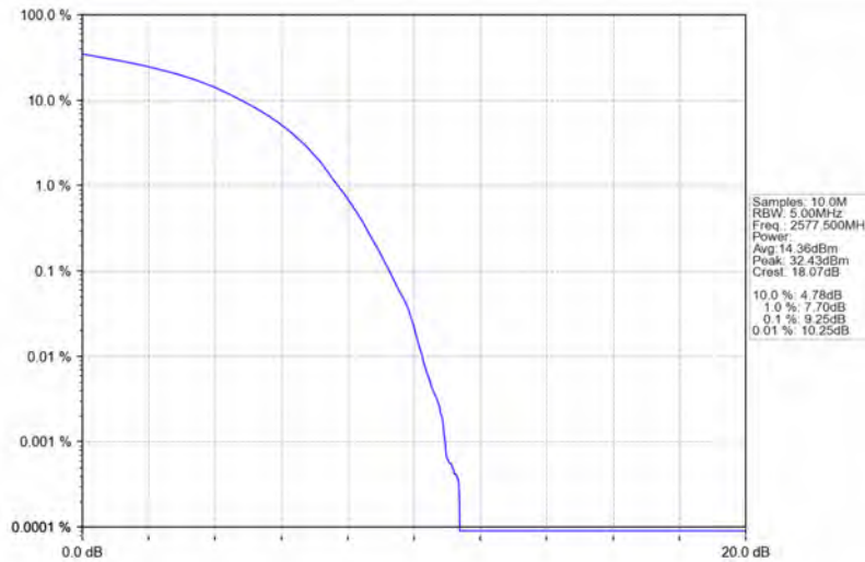
Band38_15MHz_16QAM_LCH_2577.5MHz_RB_75_0_NTNV
