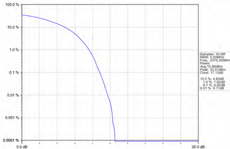
Band38_10MHz_16QAM_LCH_2575MHz_RB_50_0_NTNV
