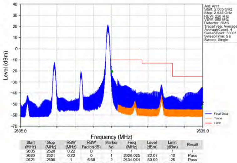
Band38_10MHz_16QAM_HCH_2615MHz_RB_1_49_NTNV
