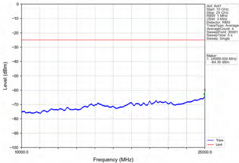
Band38_20MHz_64QAM_HCH_2610MHz_RB_1_0_NTNV
