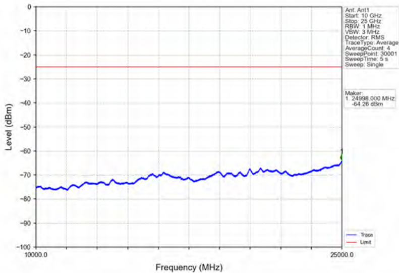
Band38_10MHz_64QAM_HCH_2615MHz_RB_1_0_NTNV
