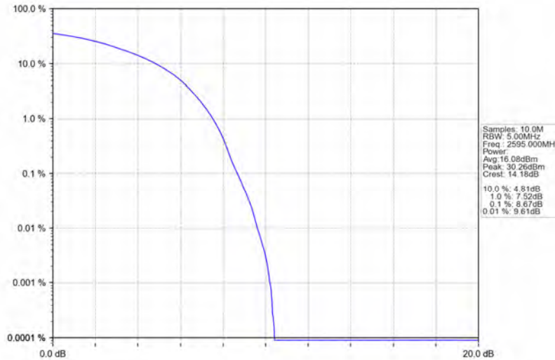
Band38_10MHz_16QAM_MCH_2595MHz_RB_50_0_NTNV
