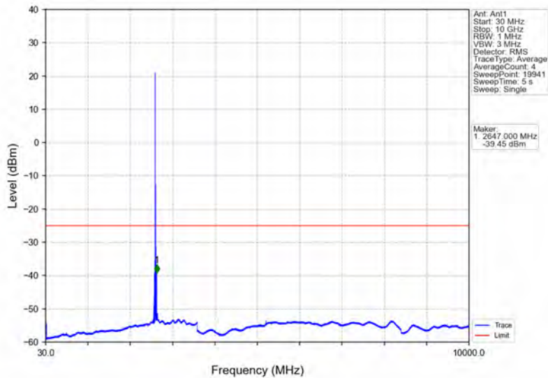
Band38_10MHz_16QAM_HCH_2615MHz_RB_1_0_NTNV
