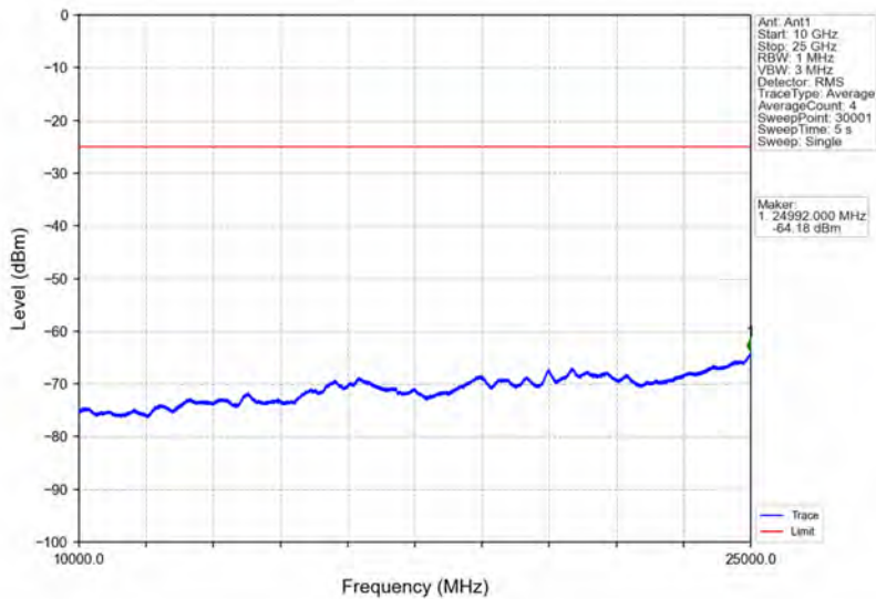
Band38_10MHz_16QAM_MCH_2595MHz_RB_1_0_NTNV
