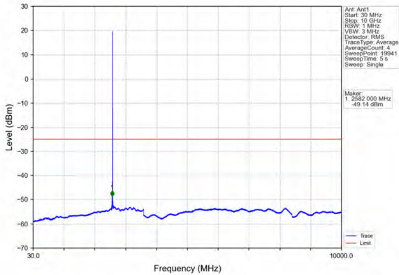
Band38_5MHz_16QAM_MCH_2595MHz_RB_1_0_NTNV
