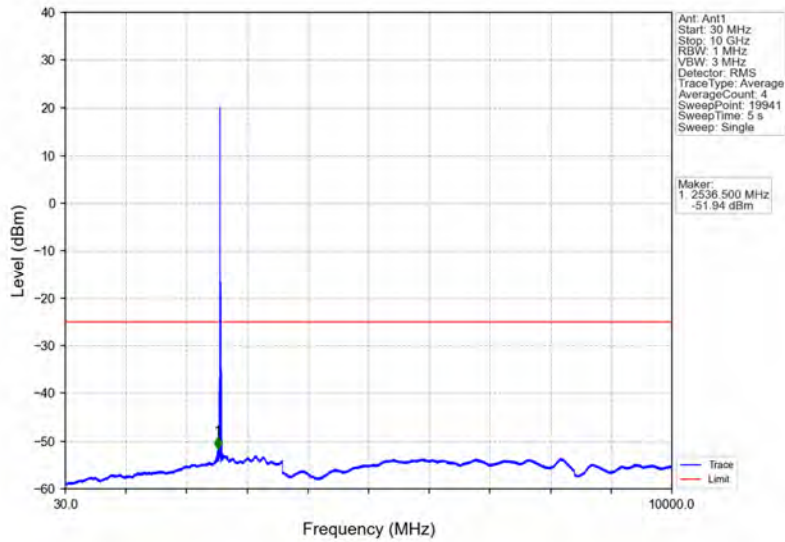
Band38_15MHz_16QAM_LCH_2577.5MHz_RB_1_0_NTNV
