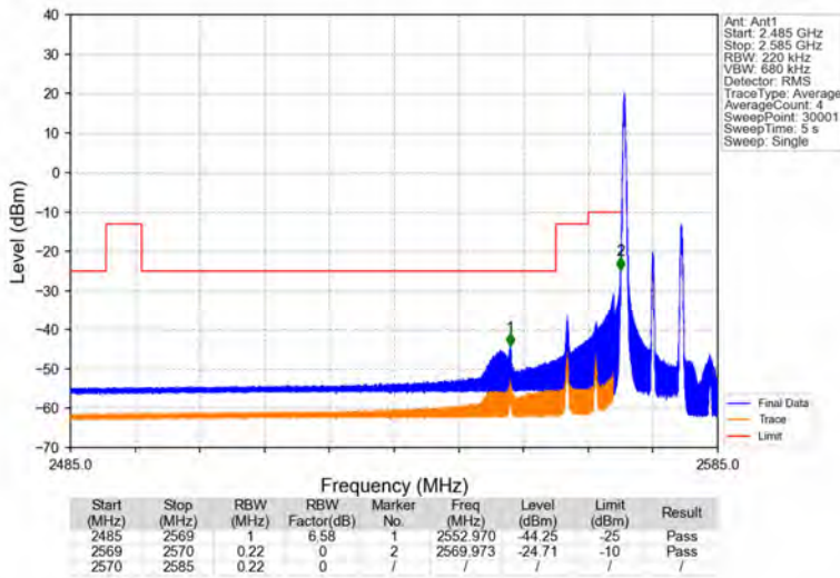
Band38_10MHz_64QAM_LCH_2575MHz_RB_1_0_NTNV
