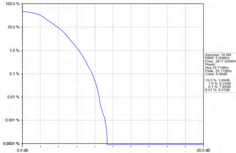
Band38_5MHz_QPSK_HCH_2617.5MHz_RB_25_0_NTNV
