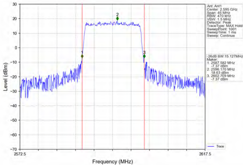
Band38_15MHz_QPSK_MCH_2595MHz_RB_75_0_NTNV
