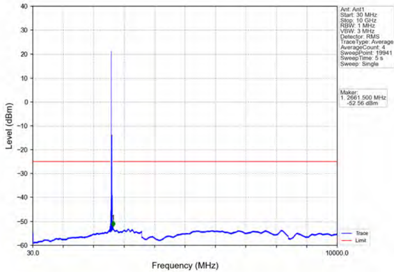
Band38_20MHz_64QAM_HCH_2610MHz_RB_1_0_NTNV
