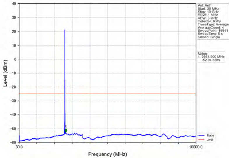
Band38_15MHz_64QAM_HCH_2612.5MHz_RB_1_0_NTNV
