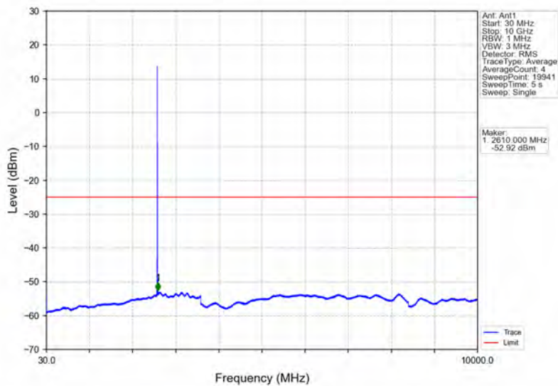
Band38_5MHz_64QAM_MCH_2595MHz_RB_1_0_NTNV
