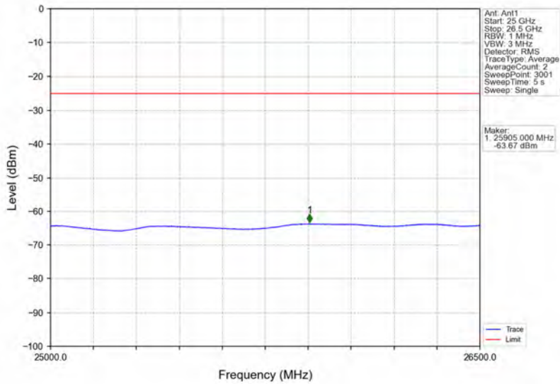
Band38_10MHz_64QAM_HCH_2615MHz_RB_1_49_NTNV
