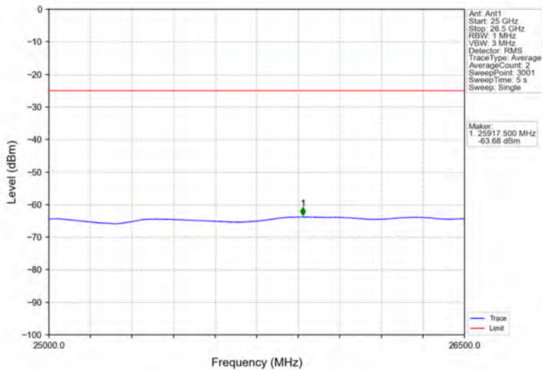
Band38_15MHz_64QAM_MCH_2595MHz_RB_1_0_NTNV
