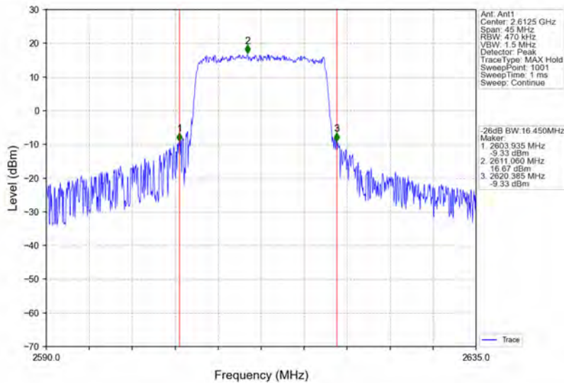
Band38_15MHz_16QAM_HCH_2612.5MHz_RB_75_0_NTNV
