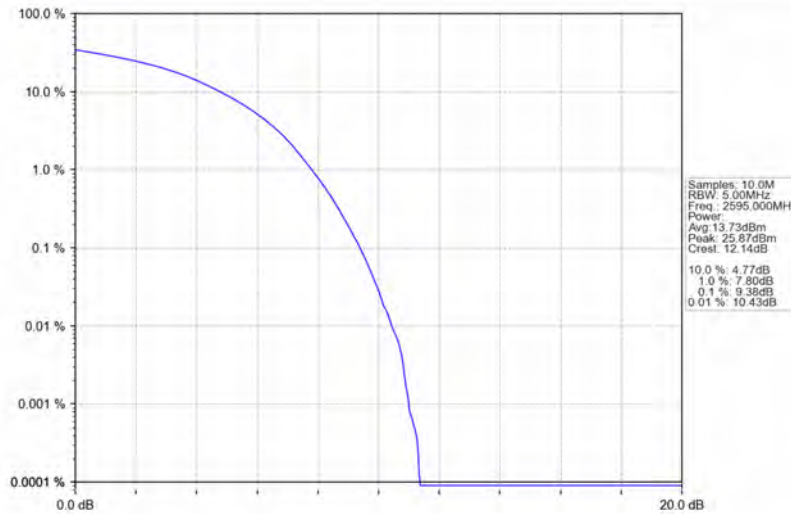
Band38_15MHz_64QAM_MCH_2595MHz_RB_75_0_NTNV
