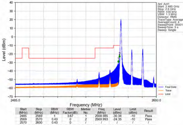
Band38_20MHz_64QAM_LCH_2580MHz_RB_1_0_NTNV
