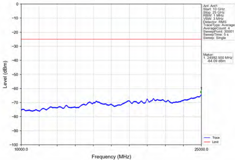
Band38_5MHz_64QAM_HCH_2617.5MHz_RB_1_0_NTNV
