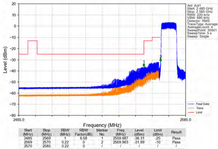
Band38_10MHz_64QAM_LCH_2575MHz_RB_50_0_NTNV
