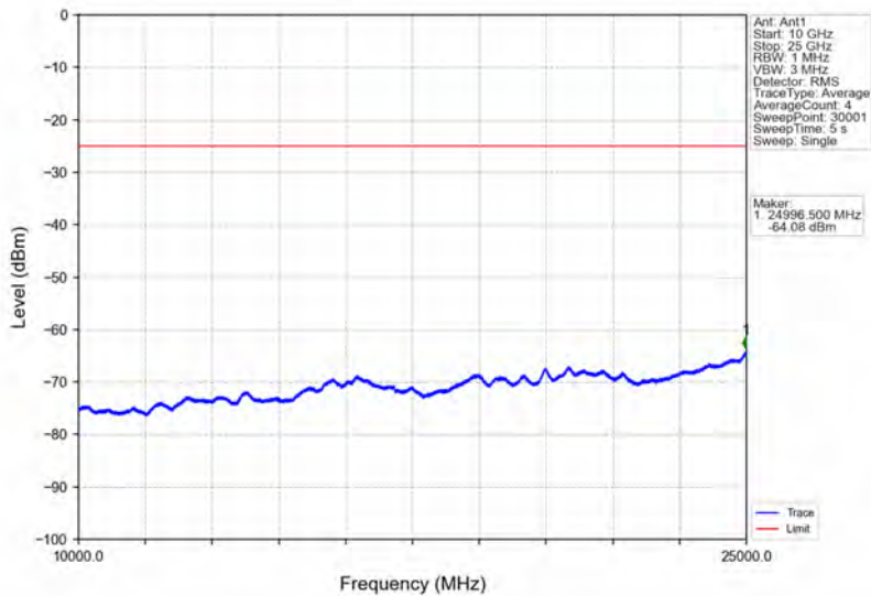
Band38_15MHz_64QAM_HCH_2612.5MHz_RB_1_0_NTNV
