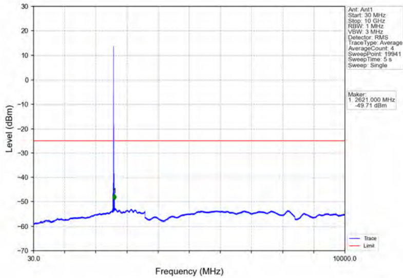
Band38_10MHz_16QAM_MCH_2595MHz_RB_1_0_NTNV
