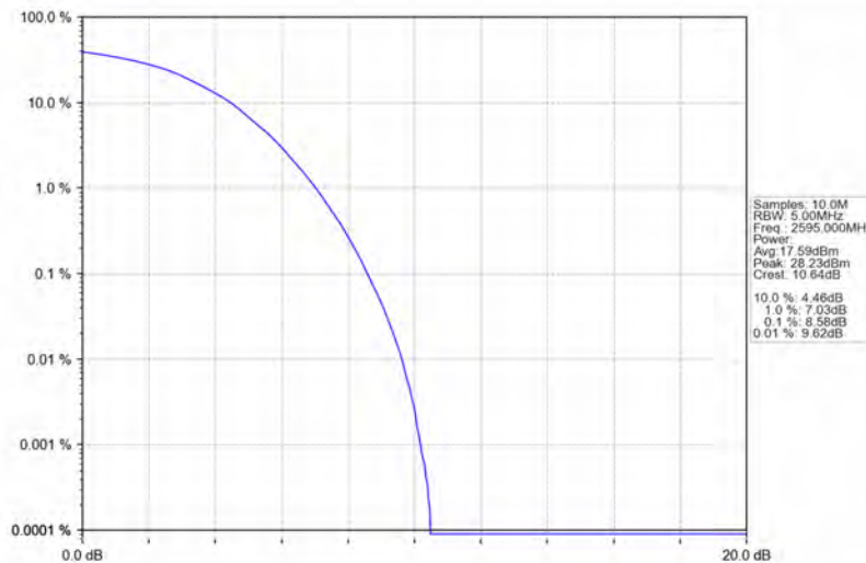
Band38_5MHz_64QAM_MCH_2595MHz_RB_25_0_NTNV
