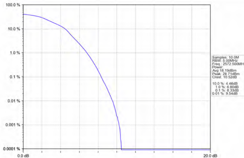
Band38_5MHz_16QAM_LCH_2572.5MHz_RB_25_0_NTNV
