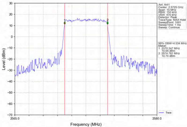
Band38_5MHz_16QAM_LCH_2572.5MHz_RB_25_0_NTNV
