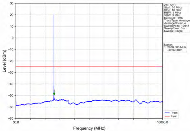
Band38_5MHz_16QAM_HCH_2617.5MHz_RB_1_0_NTNV
