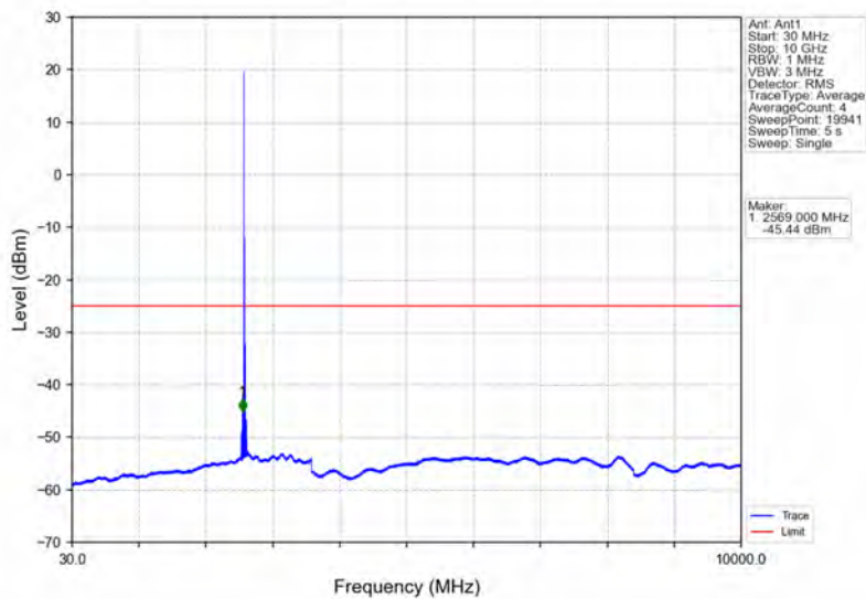
Band38_10MHz_64QAM_MCH_2595MHz_RB_1_0_NTNV
