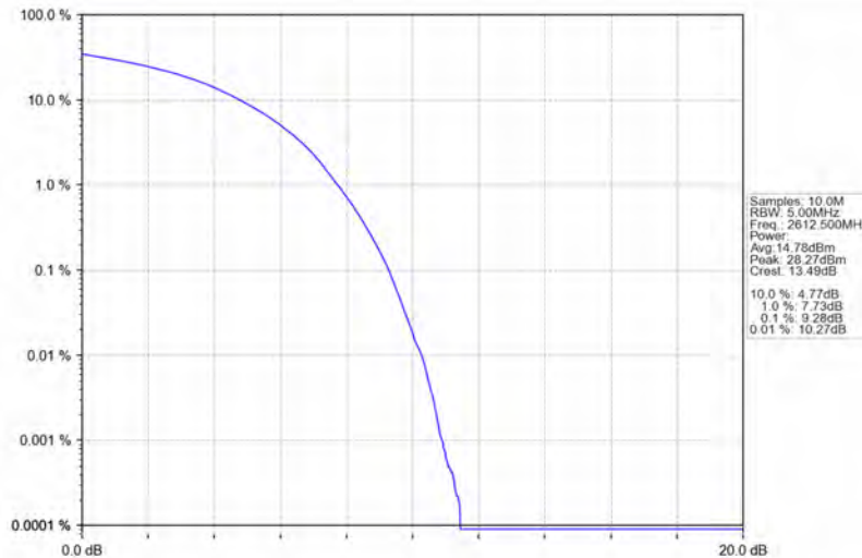
Band38_15MHz_16QAM_HCH_2612.5MHz_RB_75_0_NTNV
