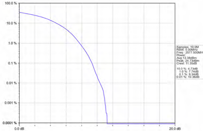
Band38_15MHz_64QAM_LCH_2577.5MHz_RB_75_0_NTNV
