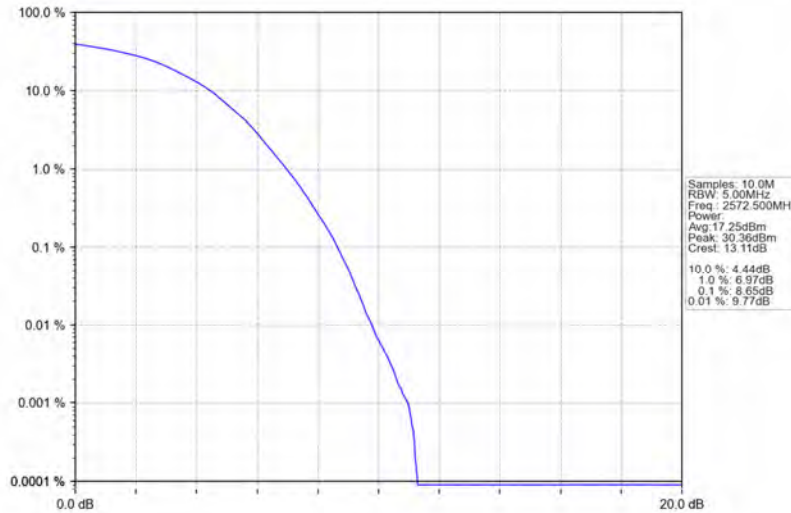
Band38_5MHz_64QAM_LCH_2572.5MHz_RB_25_0_NTNV
