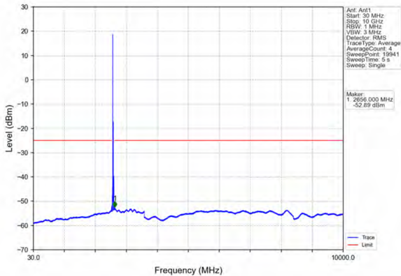
Band38_20MHz_64QAM_MCH_2595MHz_RB_1_0_NTNV
