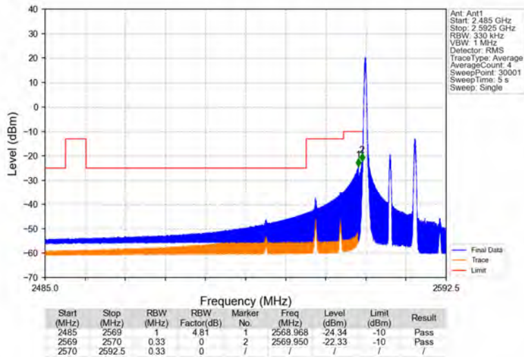
Band38_15MHz_64QAM_LCH_2577.5MHz_RB_1_0_NTNV
