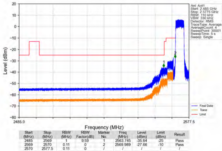
Band38_5MHz_QPSK_LCH_2572.5MHz_RB_25_0_NTNV
