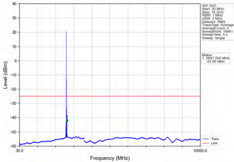
Band38_10MHz_64QAM_HCH_2615MHz_RB_1_0_NTNV
