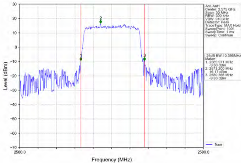
Band38_10MHz_64QAM_LCH_2575MHz_RB_50_0_NTNV
