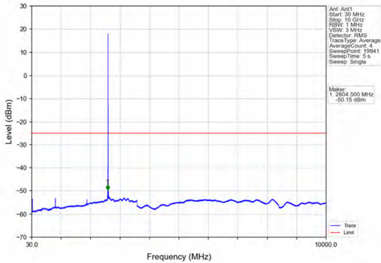
Band38_5MHz_QPSK_HCH_2617.5MHz_RB_1_0_NTNV
