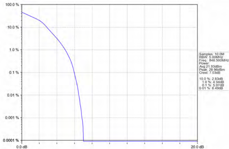
Band26b_5MHz_16QAM_HCH_846.5MHz_RB_25_0_NTNV
