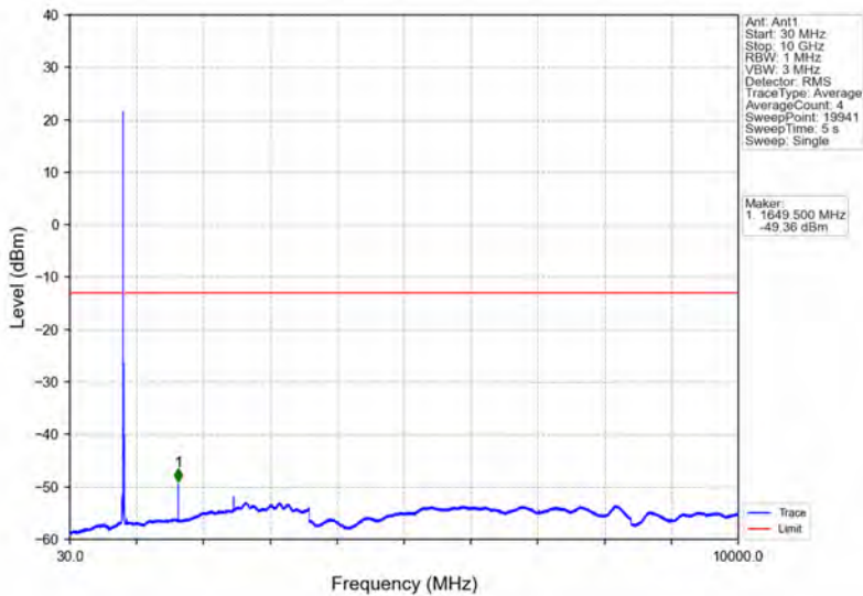
Band26b_10MHz_64QAM_LCH_829MHz_RB_1_0_NTNV
