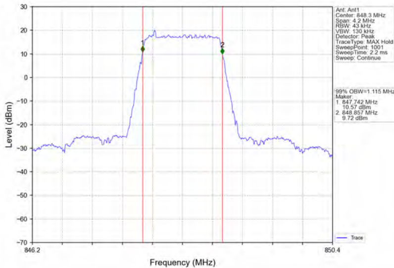
Band26b_1.4MHz_16QAM_HCH_848.3MHz_RB_6_0_NTNV
