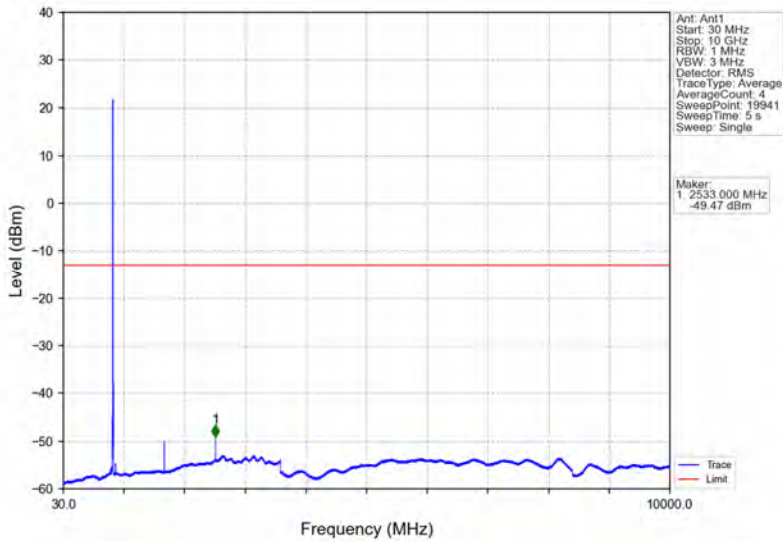
Band26b_5MHz_64QAM_HCH_846.5MHz_RB_1_24_NTNV
