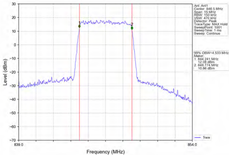
Band26b_5MHz_16QAM_HCH_846.5MHz_RB_25_0_NTNV
