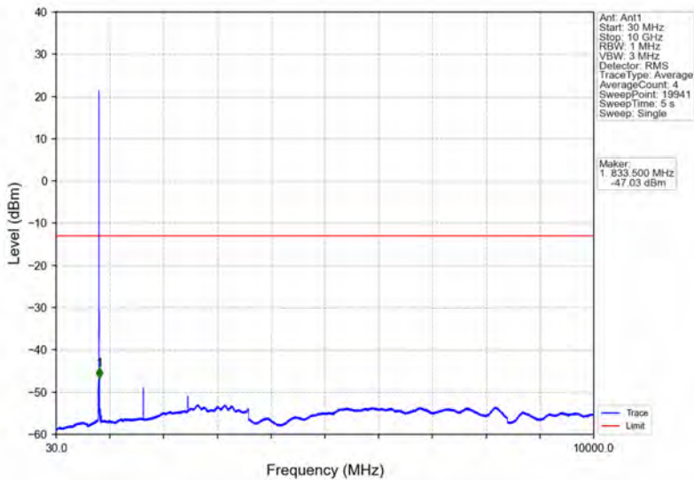
Band26b_3MHz_64QAM_LCH_825.5MHz_RB_1_0_NTNV
