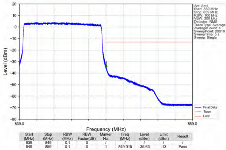
Band26b_10MHz_16QAM_HCH_844MHz_RB_50_0_NTNV
