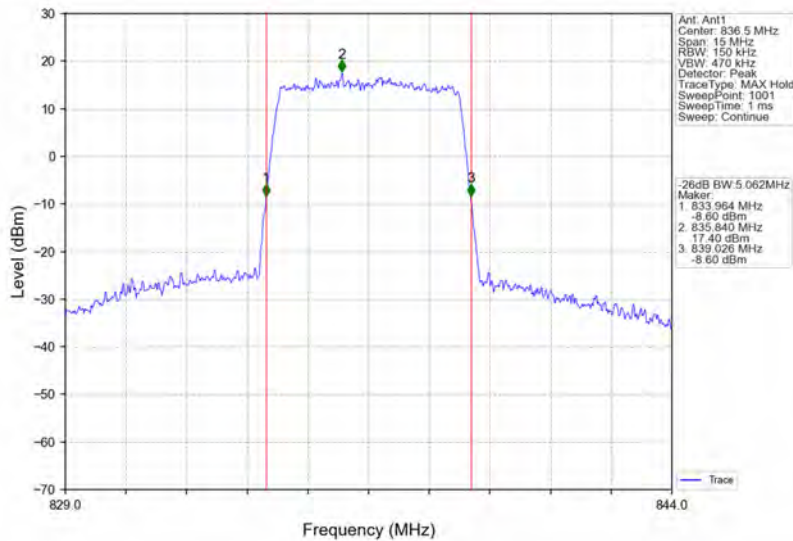
Band26b_5MHz_64QAM_MCH_836.5MHz_RB_25_0_NTNV
