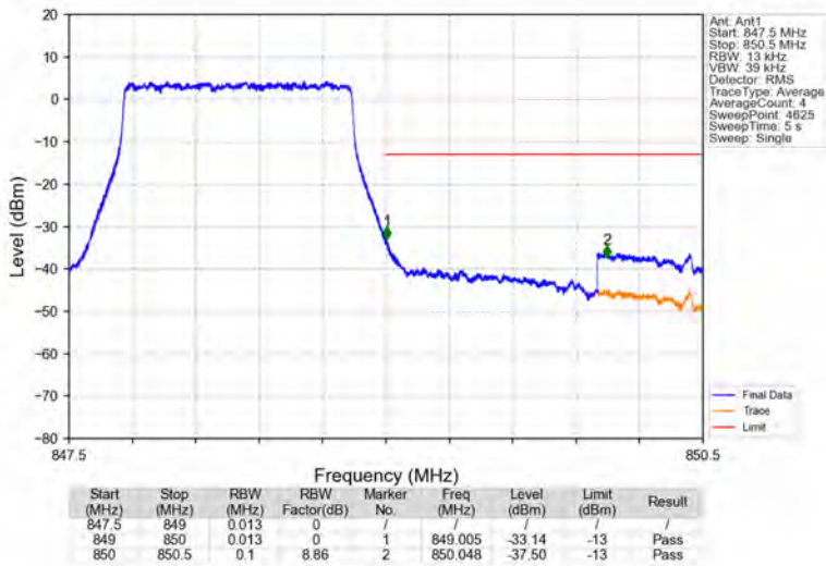
Band26b_1.4MHz_16QAM_HCH_848.3MHz_RB_6_0_NTNV
