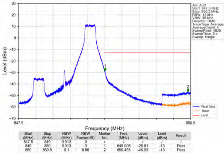
Band26b_1.4MHz_64QAM_HCH_848.3MHz_RB_1_5_NTNV
