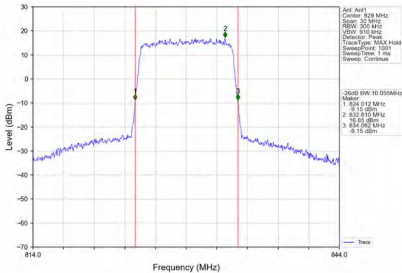
Band26b_10MHz_64QAM_LCH_829MHz_RB_50_0_NTNV
