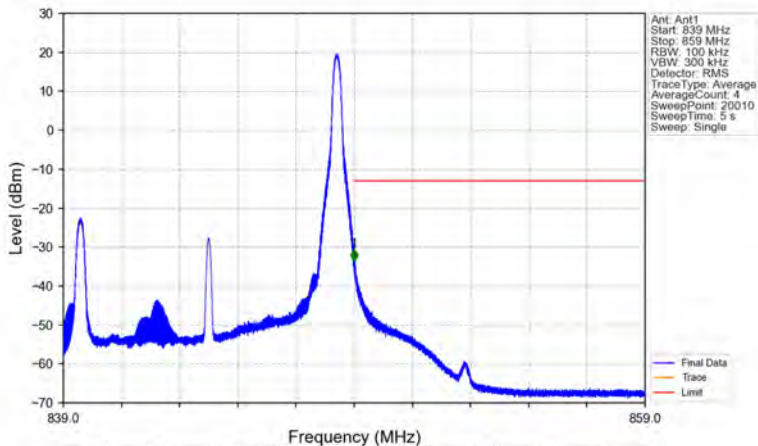
Band26b_10MHz_64QAM_HCH_844MHz_RB_1_49_NTNV
