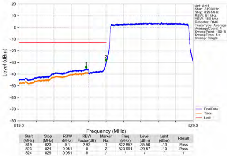
Band26b_5MHz_16QAM_LCH_826.5MHz_RB_25_0_NTNV
