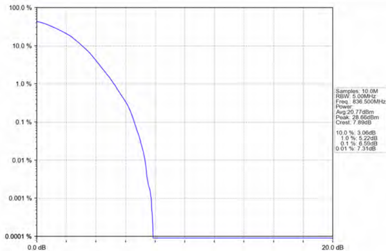
Band26b_1.4MHz_64QAM_MCH_836.5MHz_RB_6_0_NTNV
