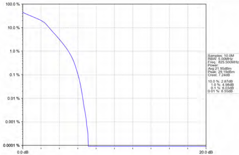
Band26b_3MHz_16QAM_LCH_825.5MHz_RB_15_0_NTNV
