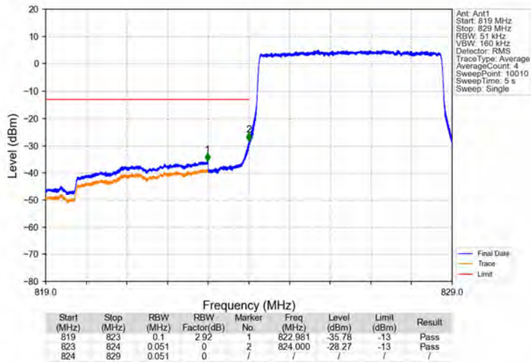
Band26b_5MHz_QPSK_LCH_826.5MHz_RB_25_0_NTNV
