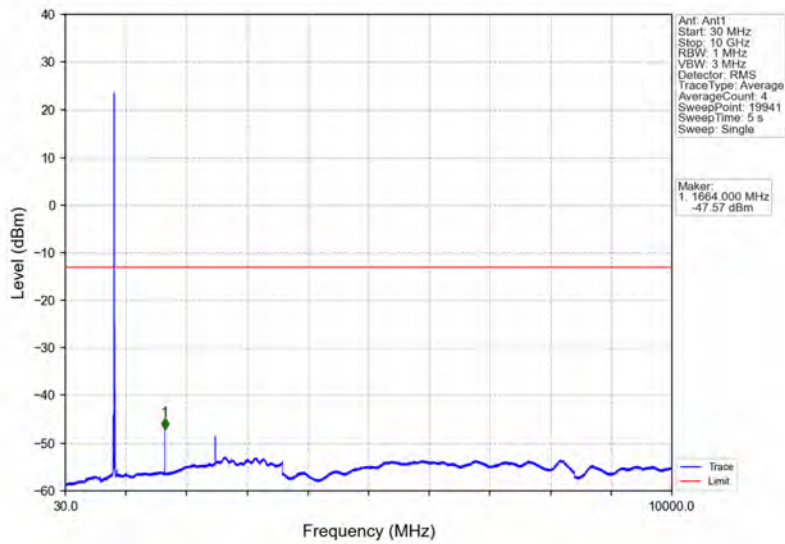
Band26b_10MHz_16QAM_HCH_844MHz_RB_1_0_NTNV
