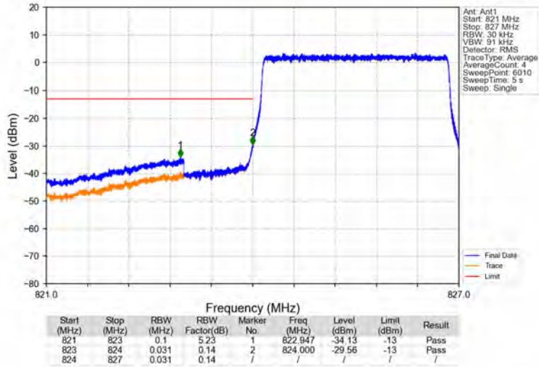
Band26b_3MHz_64QAM_LCH_825.5MHz_RB_15_0_NTNV
