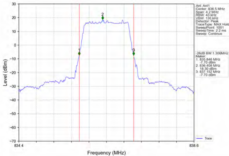
Band26b_1.4MHz_64QAM_MCH_836.5MHz_RB_6_0_NTNV
