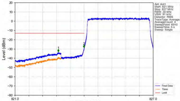
Band26b_3MHz_16QAM_LCH_825.5MHz_RB_15_0_NTNV
