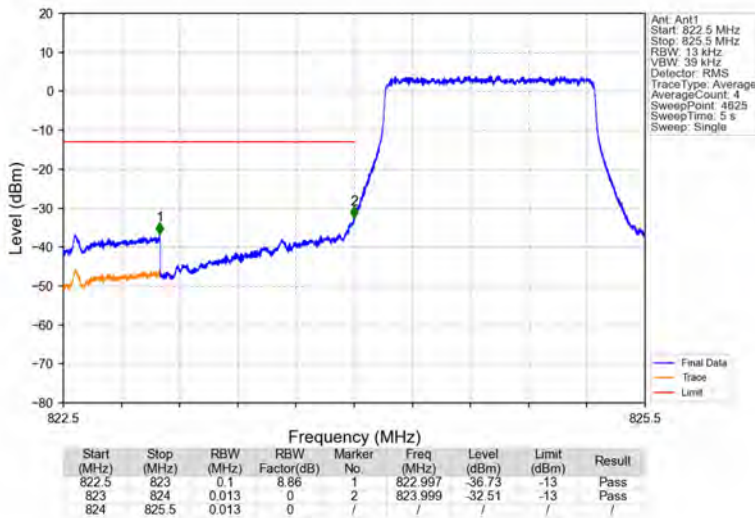
Band26b_1.4MHz_16QAM_LCH_824.7MHz_RB_6_0_NTNV
