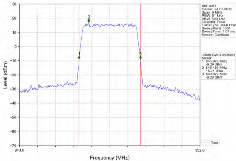
Band26b_3MHz_64QAM_HCH_847.5MHz_RB_15_0_NTNV
