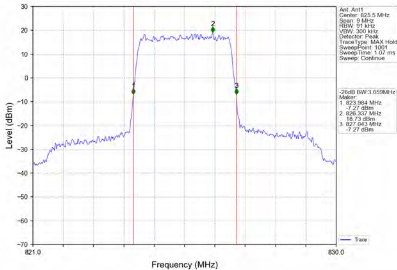
Band26b_3MHz_QPSK_LCH_825.5MHz_RB_15_0_NTNV
