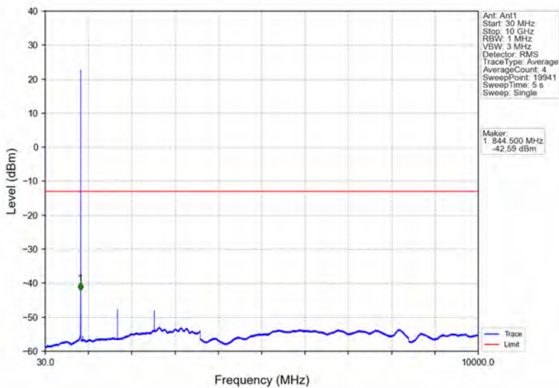
Band26b_1.4MHz_16QAM_HCH_848.3MHz_RB_1_0_NTNV
