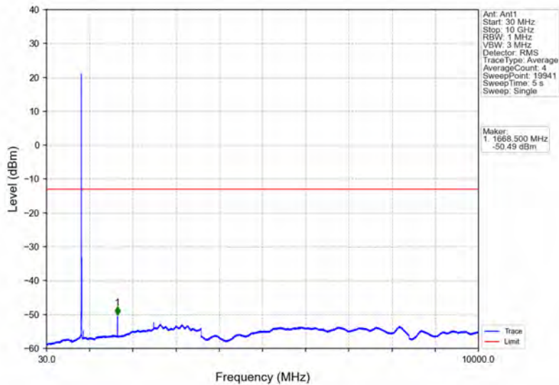
Band26b_5MHz_64QAM_MCH_836.5MHz_RB_1_0_NTNV
