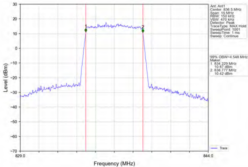
Band26b_5MHz_64QAM_MCH_836.5MHz_RB_25_0_NTNV
