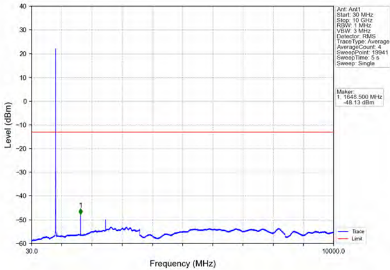
Band26b_3MHz_16QAM_LCH_825.5MHz_RB_15_0_NTNV
