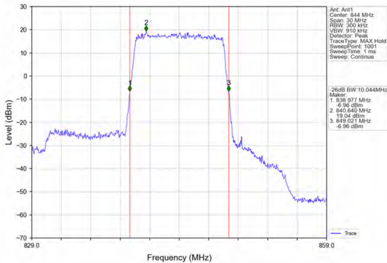
Band26b_10MHz_QPSK_HCH_844MHz_RB_50_0_NTNV
