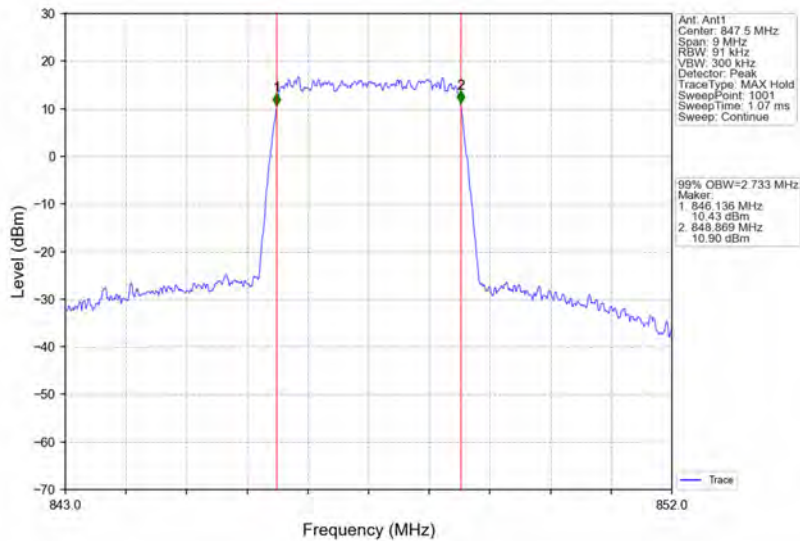
Band26b_3MHz_64QAM_HCH_847.5MHz_RB_15_0_NTNV
