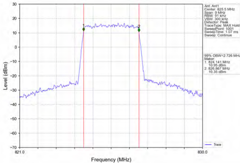
Band26b_3MHz_64QAM_LCH_825.5MHz_RB_15_0_NTNV
