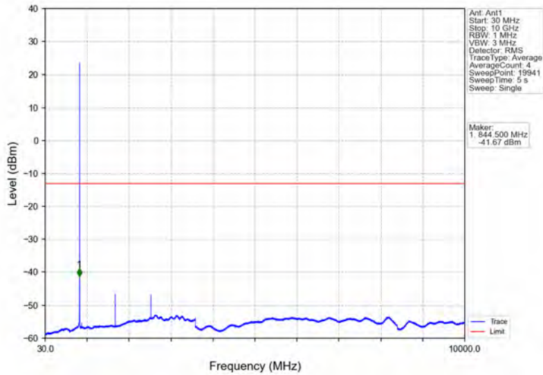
Band26b_1.4MHz_QPSK_HCH_848.3MHz_RB_1_5_NTNV
