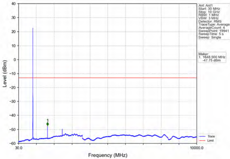
Band26b_5MHz_16QAM_LCH_826.5MHz_RB_25_0_NTNV
