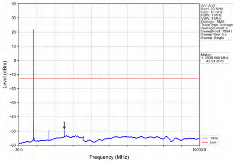
Band26b_3MHz_64QAM_HCH_847.5MHz_RB_1_14_NTNV
