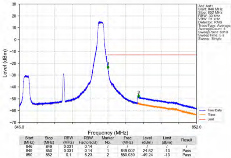
Band26b_3MHz_64QAM_HCH_847.5MHz_RB_1_14_NTNV
