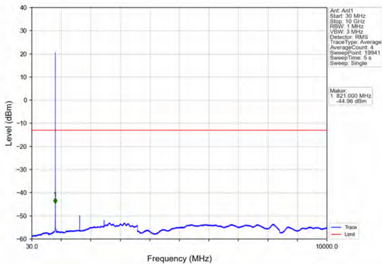
Band26b_1.4MHz_64QAM_LCH_824.7MHz_RB_1_0_NTNV
