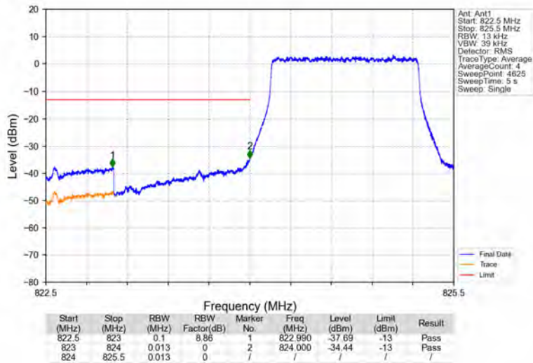
Band26b_1.4MHz_64QAM_LCH_824.7MHz_RB_6_0_NTNV
