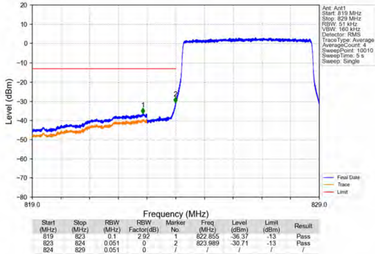
Band26b_5MHz_64QAM_LCH_826.5MHz_RB_25_0_NTNV
