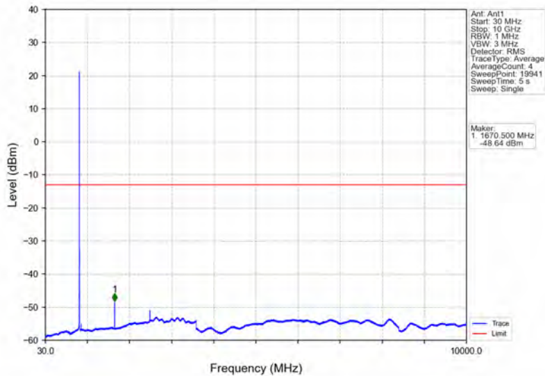
Band26b_3MHz_64QAM_MCH_836.5MHz_RB_1_0_NTNV
