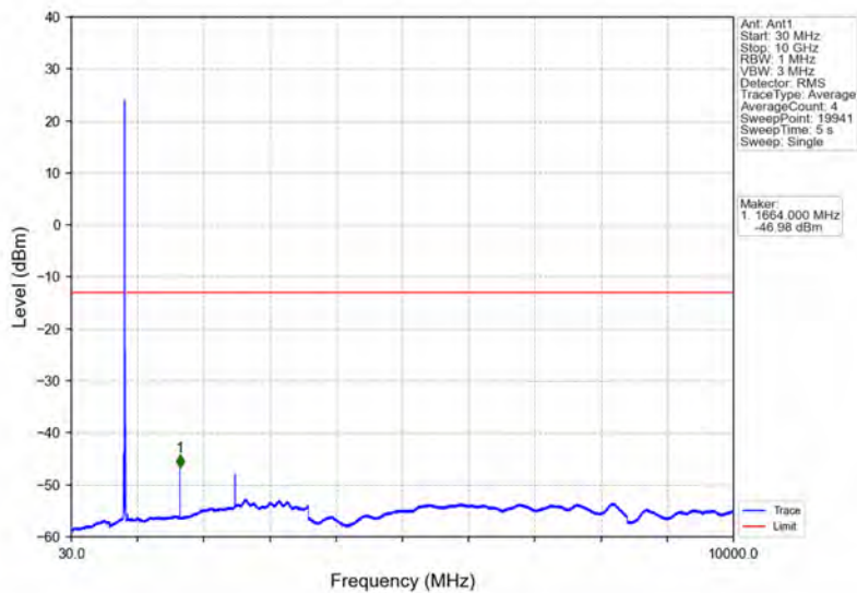
Band26b_10MHz_QPSK_MCH_836.5MHz_RB_1_0_NTNV
