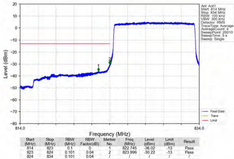
Band26b_10MHz_QPSK_LCH_829MHz_RB_50_0_NTNV
