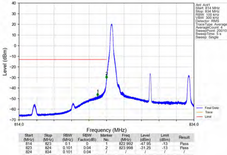
Band26b_10MHz_64QAM_LCH_829MHz_RB_1_0_NTNV
