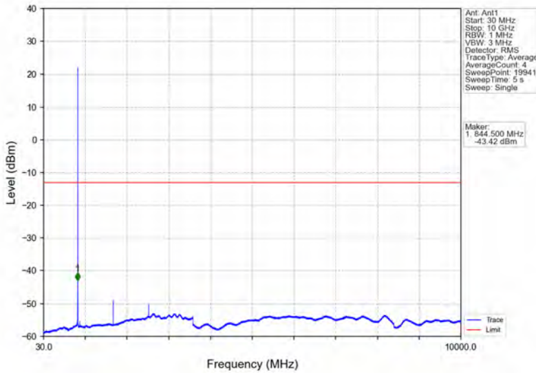
Band26b_1.4MHz_64QAM_HCH_848.3MHz_RB_1_5_NTNV
