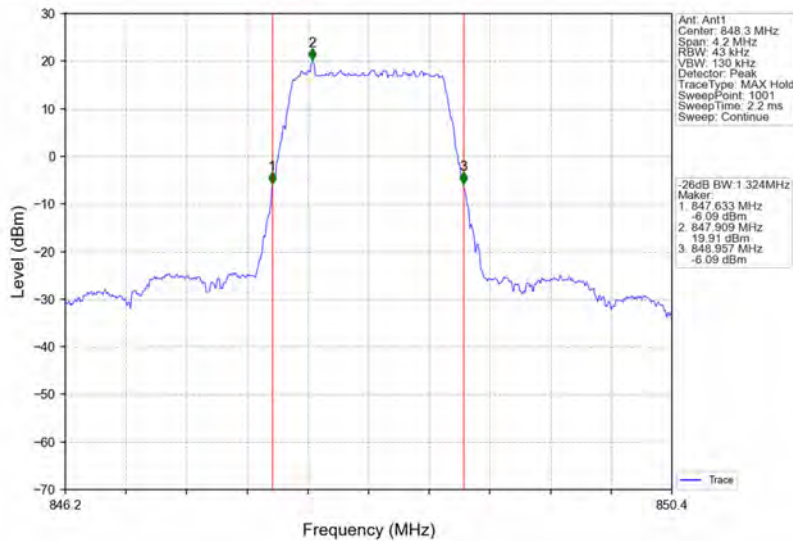
Band26b_1.4MHz_16QAM_HCH_848.3MHz_RB_6_0_NTNV
