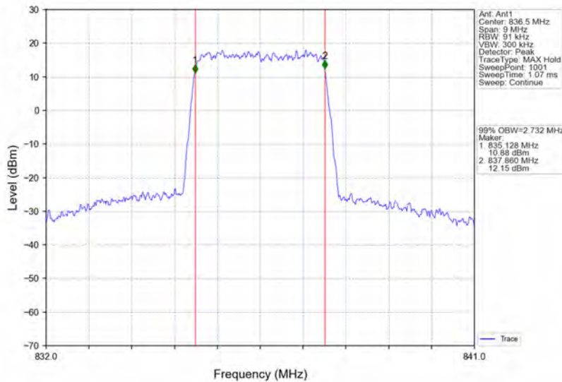
Band26b_3MHz_16QAM_MCH_836.5MHz_RB_15_0_NTNV
