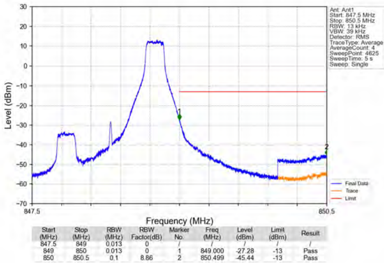
Band26b_1.4MHz_16QAM_HCH_848.3MHz_RB_1_5_NTNV
