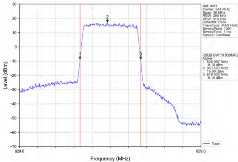
Band26b_10MHz_64QAM_HCH_844MHz_RB_50_0_NTNV
