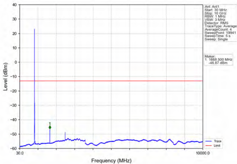
Band26b_5MHz_QPSK_MCH_836.5MHz_RB_1_0_NTNV
