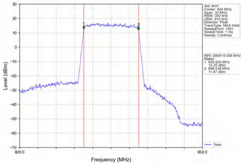
Band26b_10MHz_64QAM_HCH_844MHz_RB_50_0_NTNV
