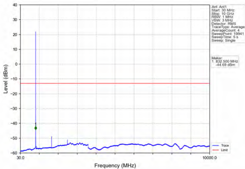
Band26b_1.4MHz_64QAM_MCH_836.5MHz_RB_1_0_NTNV
