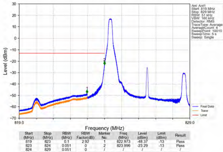
Band26b_5MHz_64QAM_LCH_826.5MHz_RB_1_0_NTNV
