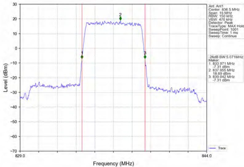
Band26b_5MHz_QPSK_MCH_836.5MHz_RB_25_0_NTNV
