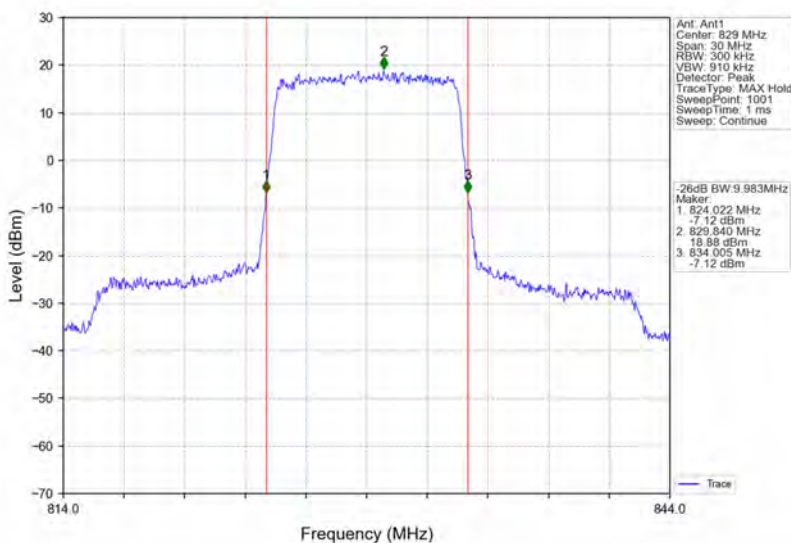
Band26b_10MHz_QPSK_LCH_829MHz_RB_50_0_NTNV
