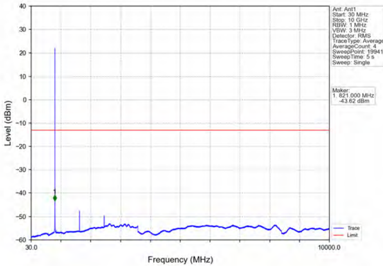
Band26b_1.4MHz_16QAM_LCH_824.7MHz_RB_6_0_NTNV
