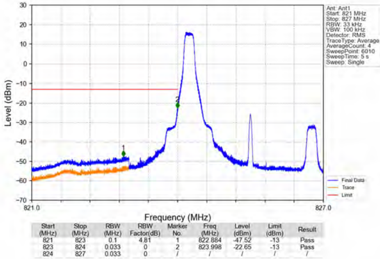
Band26b_3MHz_64QAM_LCH_825.5MHz_RB_1_0_NTNV
