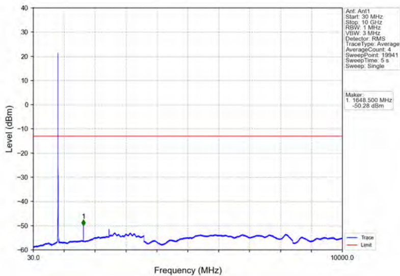
Band26b_5MHz_64QAM_LCH_826.5MHz_RB_1_0_NTNV
