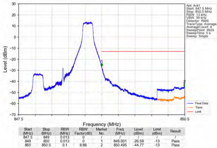
Band26b_1.4MHz_QPSK_HCH_848.3MHz_RB_1_5_NTNV
