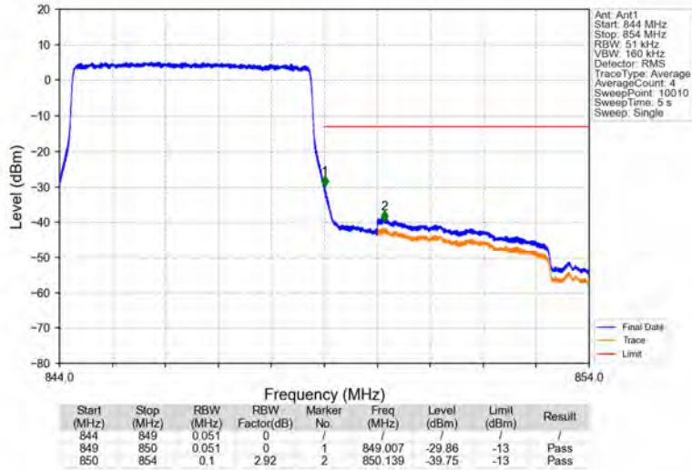
Band26b_5MHz_QPSK_HCH_846.5MHz_RB_25_0_NTNV
