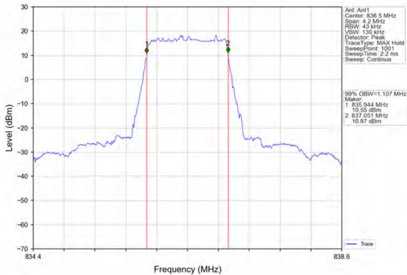
Band26b_1.4MHz_64QAM_MCH_836.5MHz_RB_6_0_NTNV
