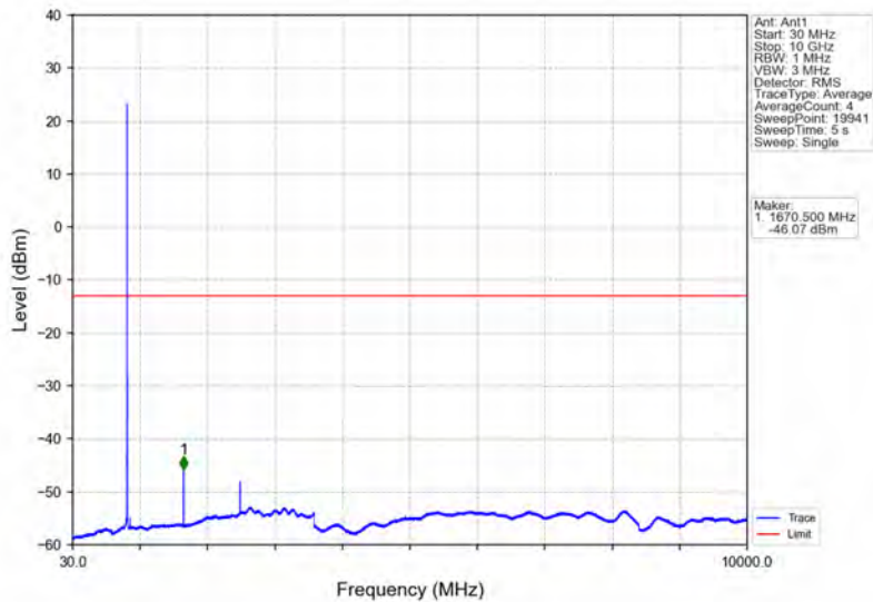
Band26b_3MHz_QPSK_MCH_836.5MHz_RB_1_0_NTNV
