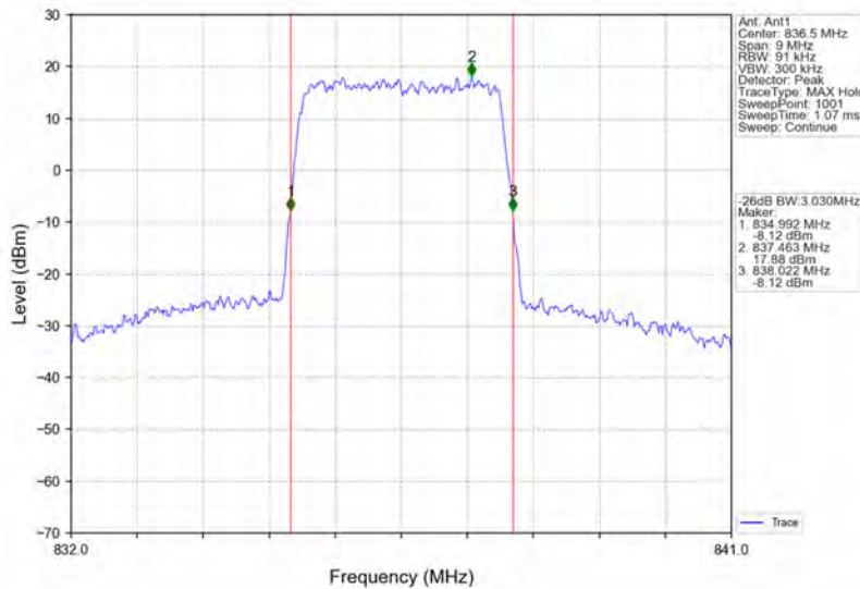
Band26b_3MHz_16QAM_MCH_836.5MHz_RB_15_0_NTNV
