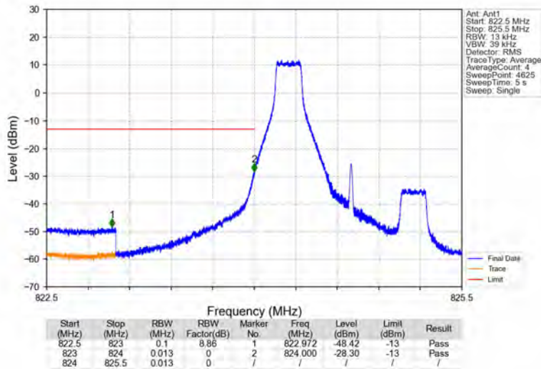
Band26b_1.4MHz_64QAM_LCH_824.7MHz_RB_1_0_NTNV
