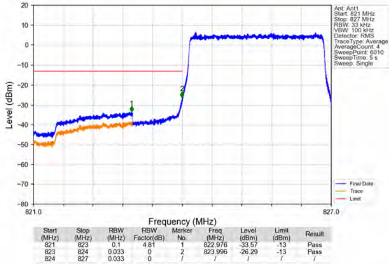
Band26b_3MHz_QPSK_LCH_825.5MHz_RB_15_0_NTNV
