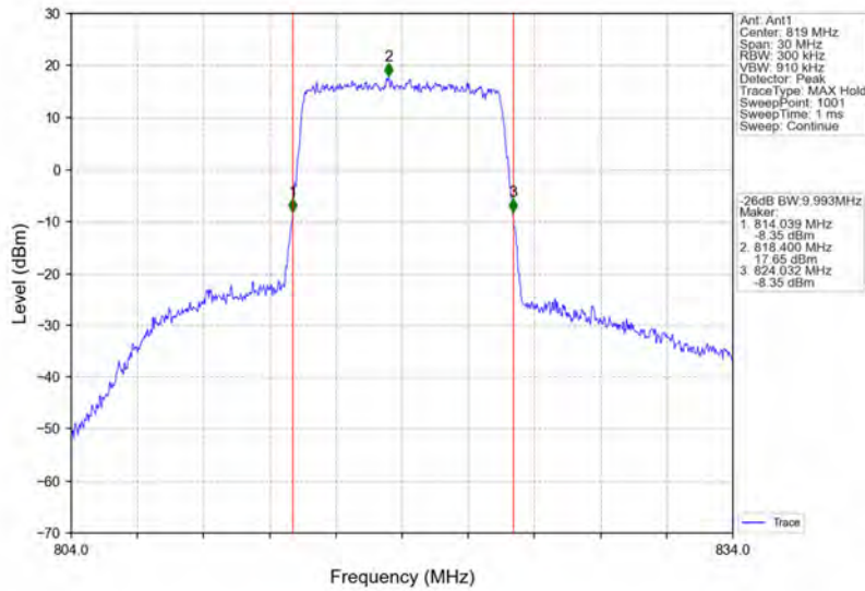
Band26a_10MHz_16QAM_MCH_819MHz_RB_50_0_NTNV
