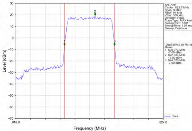
Band26a_3MHz_QPSK_HCH_822.5MHz_RB_15_0_NTNV
