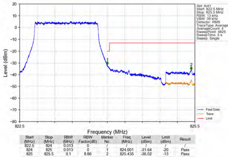
Band26a_1.4MHz_QPSK_HCH_823.3MHz_RB_6_0_NTNV
