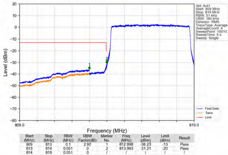
Band26a_5MHz_64QAM_LCH_816.5MHz_RB_25_0_NTNV
