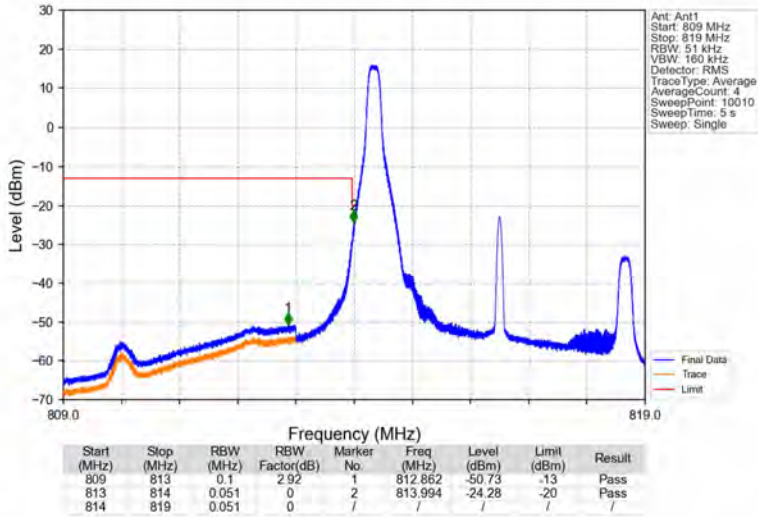
Band26a_5MHz_64QAM_LCH_816.5MHz_RB_1_0_NTNV
