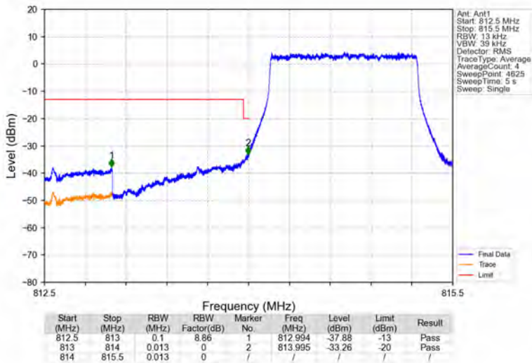
Band26a_1.4MHz_16QAM_LCH_814.7MHz_RB_6_0_NTNV
