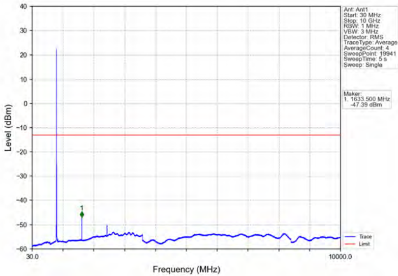
Band26a_5MHz_16QAM_HCH_821.5MHz_RB_1_0_NTNV
