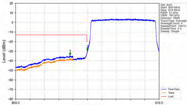
Band26a_5MHz_16QAM_LCH_816.5MHz_RB_25_0_NTNV
