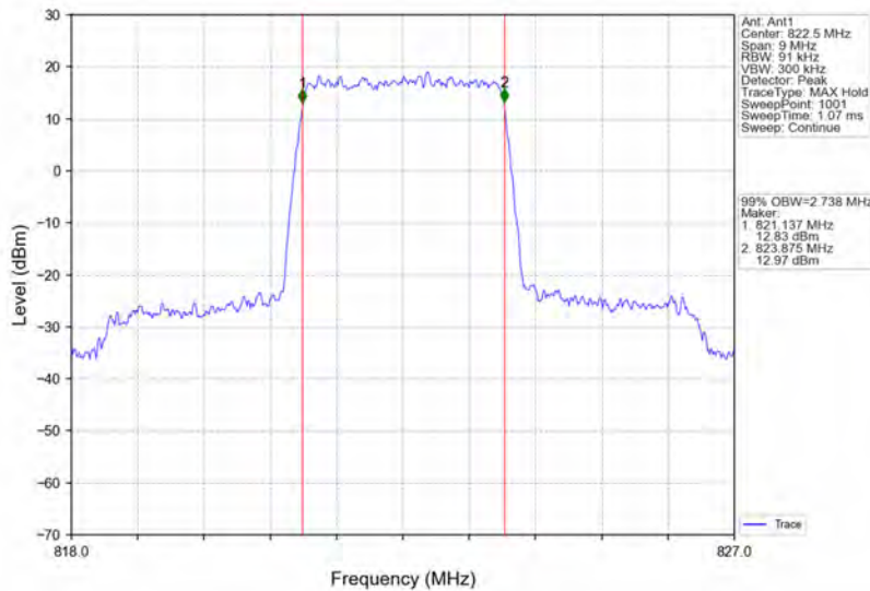
Band26a_3MHz_QPSK_HCH_822.5MHz_RB_15_0_NTNV
