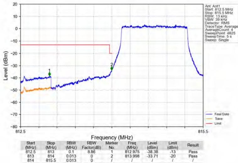
Band26a_1.4MHz_64QAM_LCH_814.7MHz_RB_6_0_NTNV
