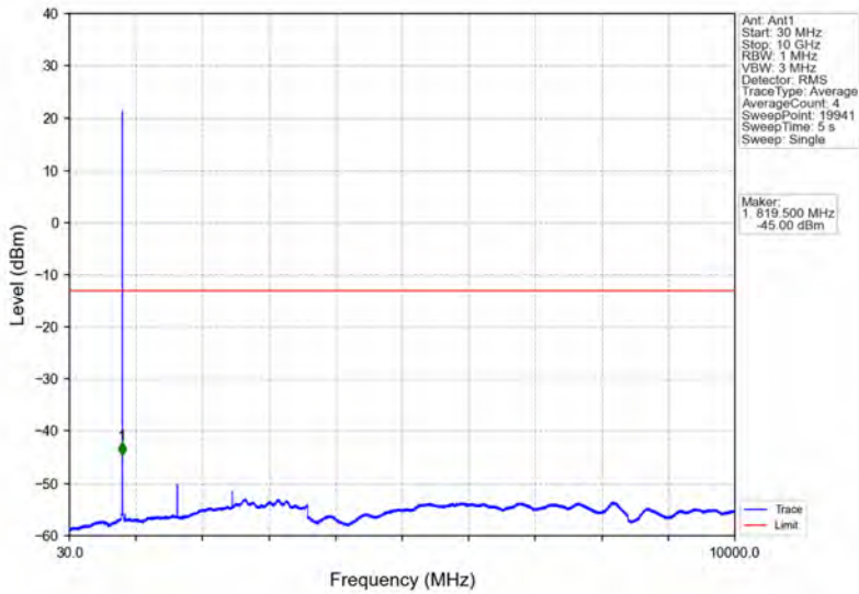
Band26a_1.4MHz_64QAM_HCH_823.3MHz_RB_1_5_NTNV
