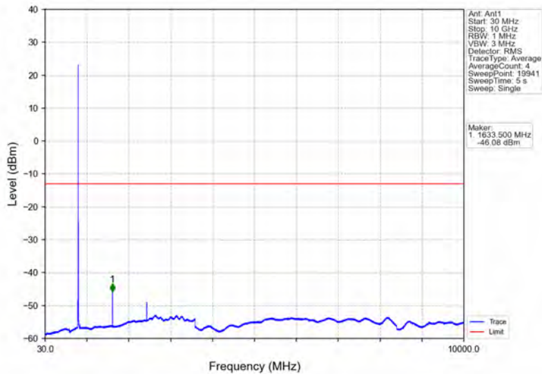
Band26a_5MHz_QPSK_MCH_819MHz_RB_1_0_NTNV
