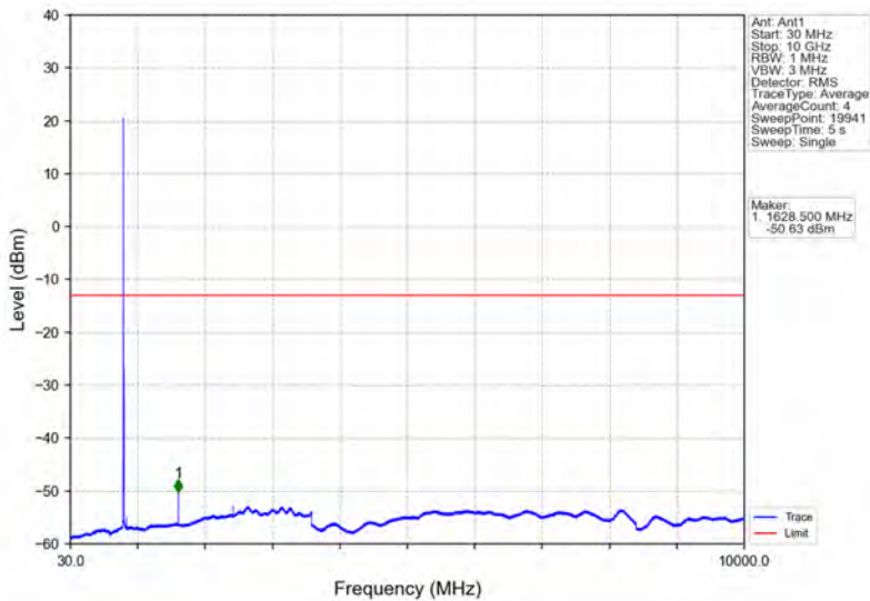
Band26a_5MHz_64QAM_LCH_816.5MHz_RB_1_0_NTNV
