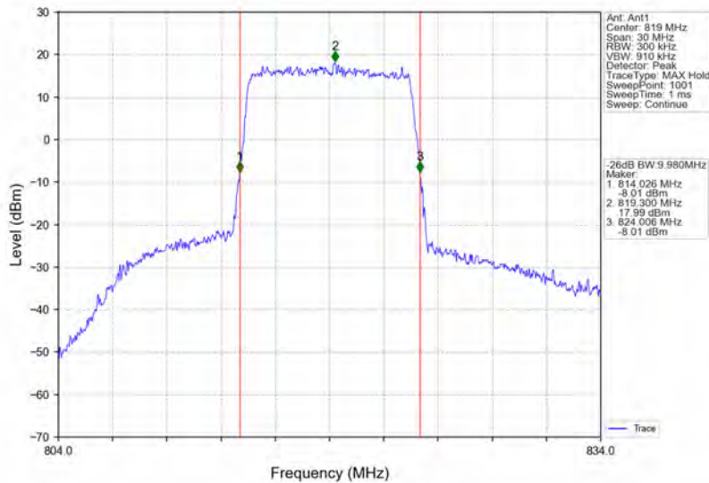
Band26a_10MHz_16QAM_MCH_819MHz_RB_50_0_NTNV
