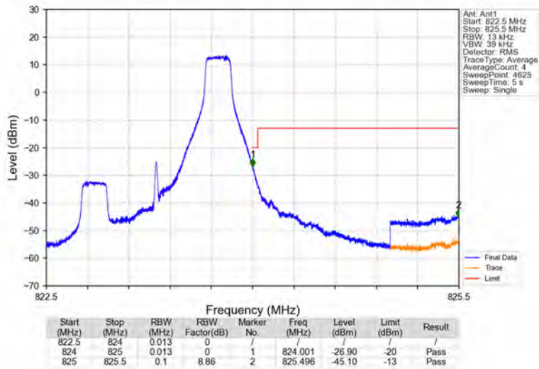
Band26a_1.4MHz_QPSK_HCH_823.3MHz_RB_1_5_NTNV
