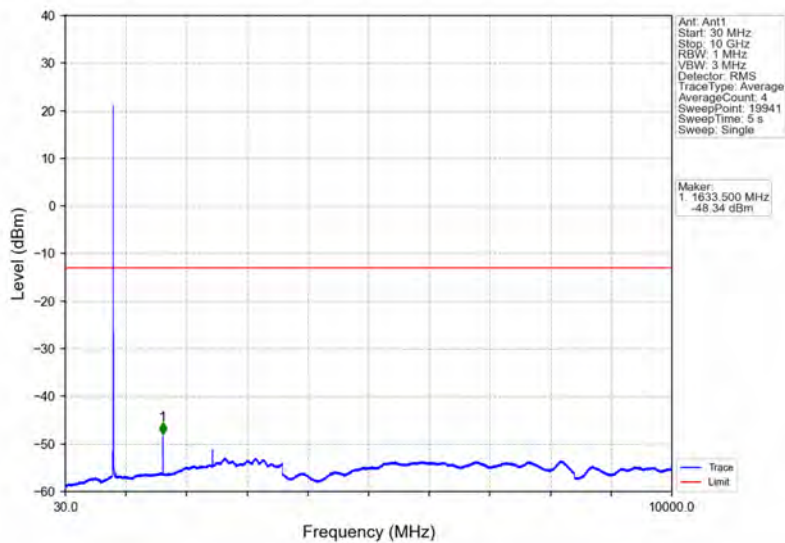
Band26a_5MHz_64QAM_MCH_819MHz_RB_1_0_NTNV
