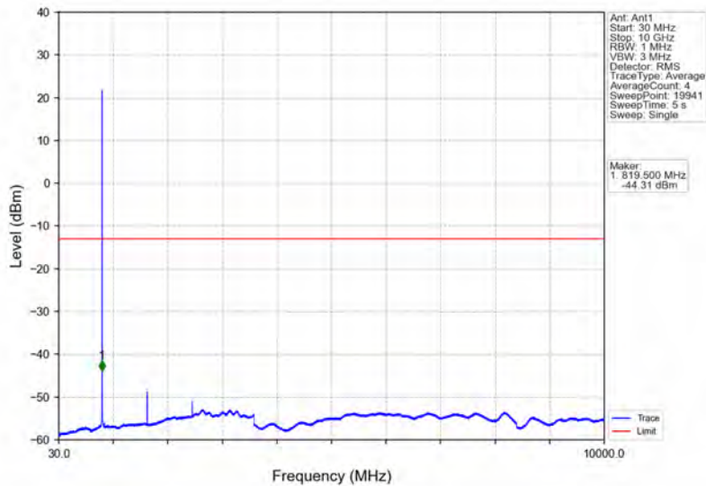
Band26a_1.4MHz_16QAM_HCH_823.3MHz_RB_1_0_NTNV
