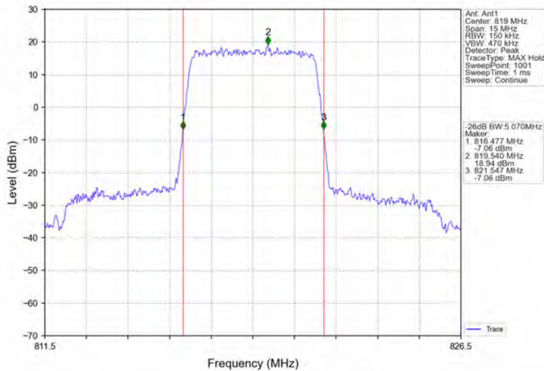
Band26a_5MHz_QPSK_MCH_819MHz_RB_25_0_NTNV
