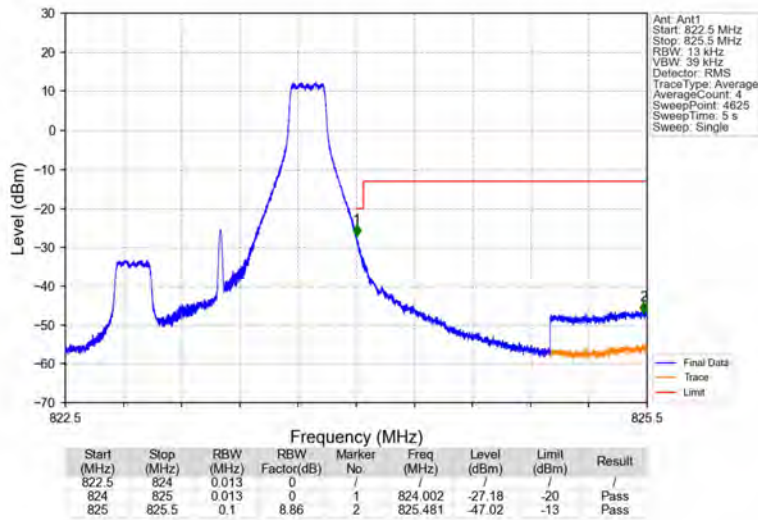
Band26a_1.4MHz_16QAM_HCH_823.3MHz_RB_1_5_NTNV
