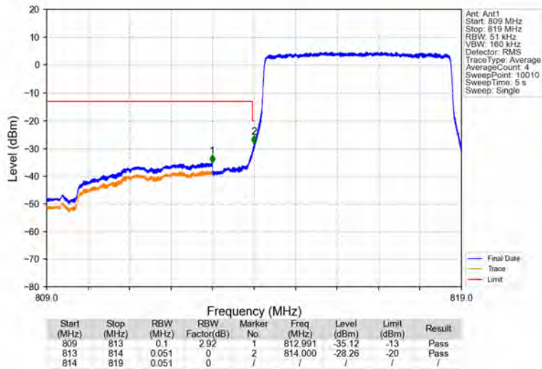
Band26a_5MHz_QPSK_LCH_816.5MHz_RB_25_0_NTNV
