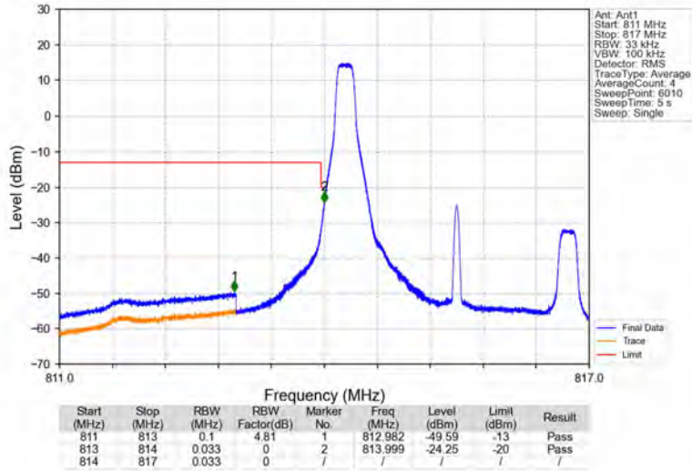
Band26a_3MHz_64QAM_LCH_815.5MHz_RB_1_0_NTNV
