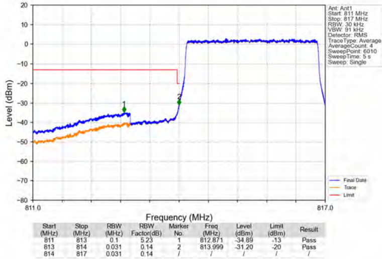
Band26a_3MHz_64QAM_LCH_815.5MHz_RB_15_0_NTNV
