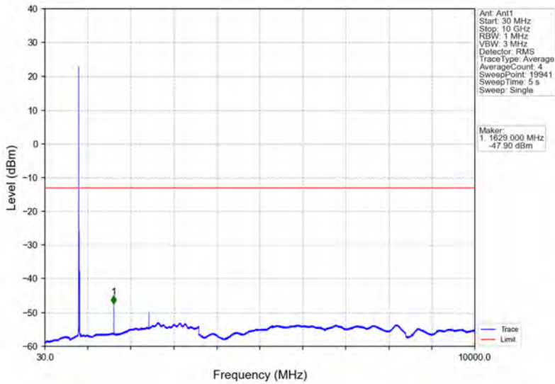
Band26a_10MHz_16QAM_LCH_819MHz_RB_50_0_NTNV
