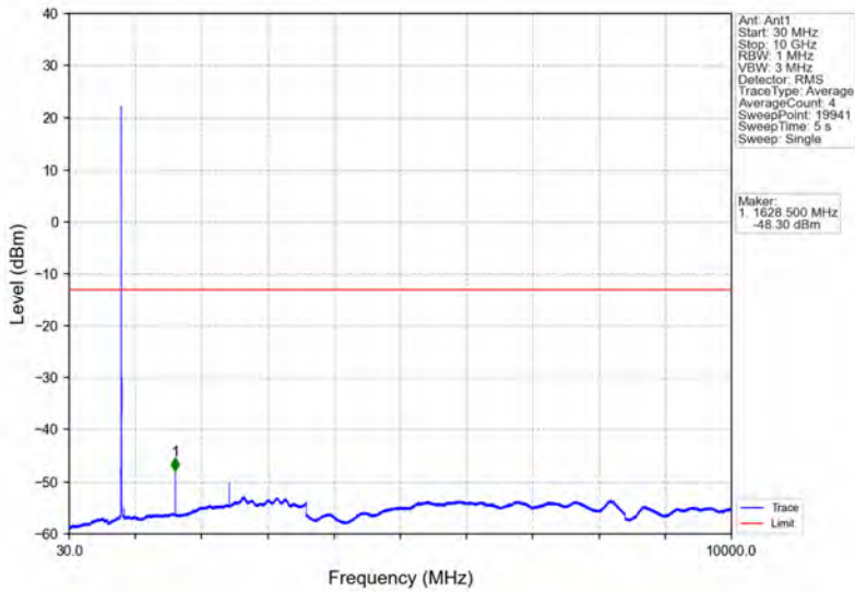
Band26a_3MHz_16QAM_LCH_815.5MHz_RB_15_0_NTNV
