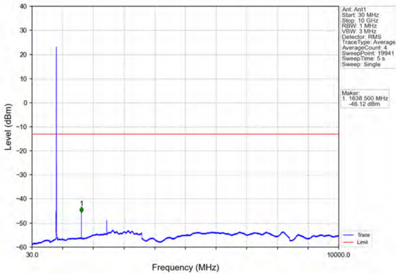
Band26a_5MHz_QPSK_HCH_821.5MHz_RB_1_24_NTNV
