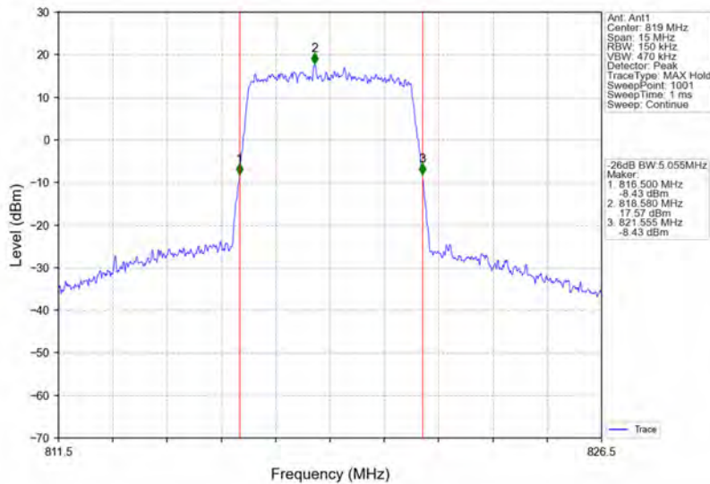
Band26a_5MHz_64QAM_MCH_819MHz_RB_25_0_NTNV
