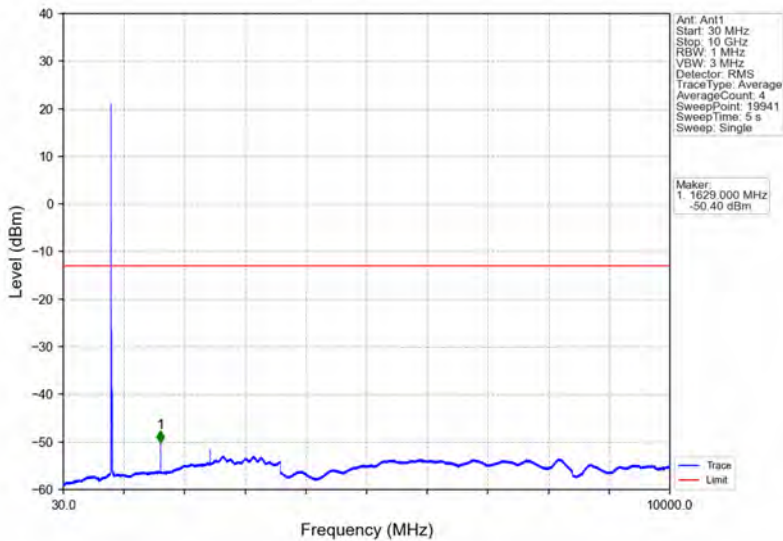
Band26a_10MHz_64QAM_LCH_819MHz_RB_1_0_NTNV
