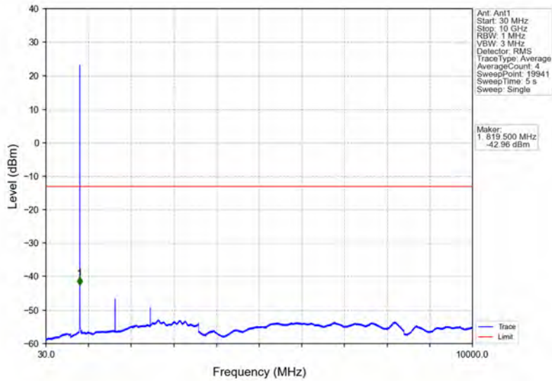
Band26a_1.4MHz_QPSK_HCH_823.3MHz_RB_1_5_NTNV
