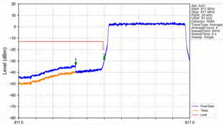
Band26a_3MHz_16QAM_LCH_815.5MHz_RB_15_0_NTNV
