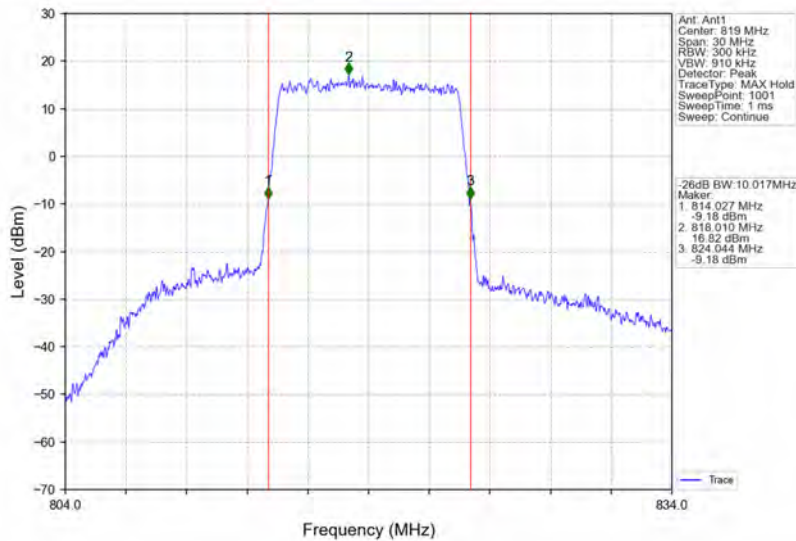
Band26a_10MHz_64QAM_LCH_819MHz_RB_50_0_NTNV
