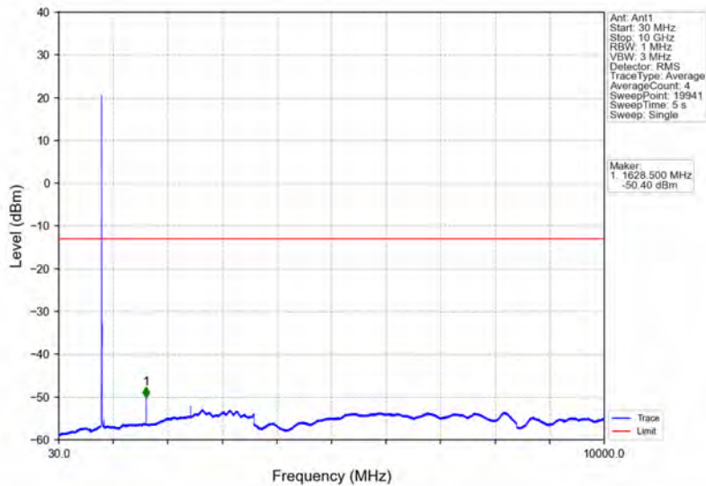
Band26a_3MHz_64QAM_LCH_815.5MHz_RB_1_0_NTNV
