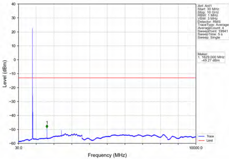
Band26a_10MHz_16QAM_HCH_819MHz_RB_1_0_NTNV
