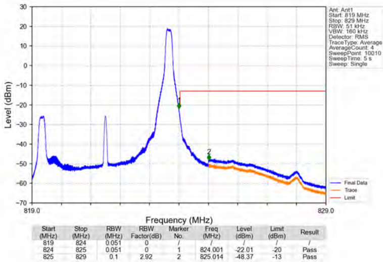
Band26a_5MHz_QPSK_HCH_821.5MHz_RB_1_24_NTNV
