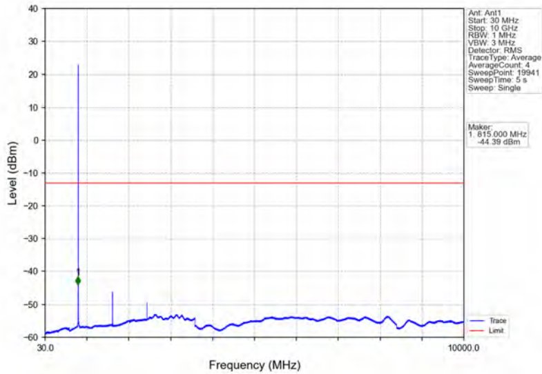
Band26a_1.4MHz_16QAM_HCH_823.3MHz_RB_1_0_NTNV
