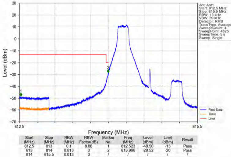
Band26a_1.4MHz_64QAM_LCH_814.7MHz_RB_1_0_NTNV
