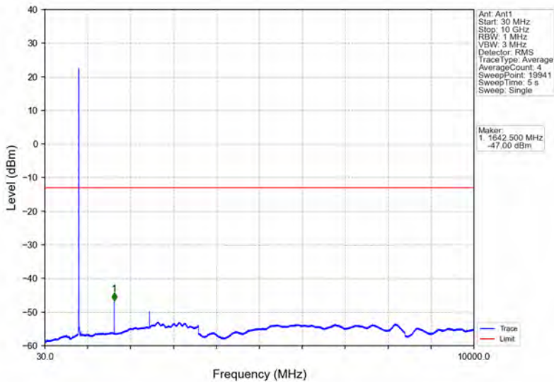
Band26a_3MHz_16QAM_HCH_822.5MHz_RB_1_0_NTNV
