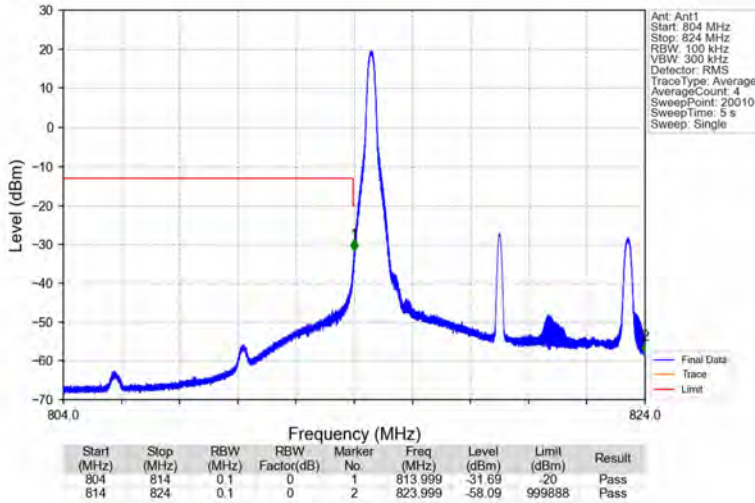
Band26a_10MHz_64QAM_LCH_819MHz_RB_1_0_NTNV
