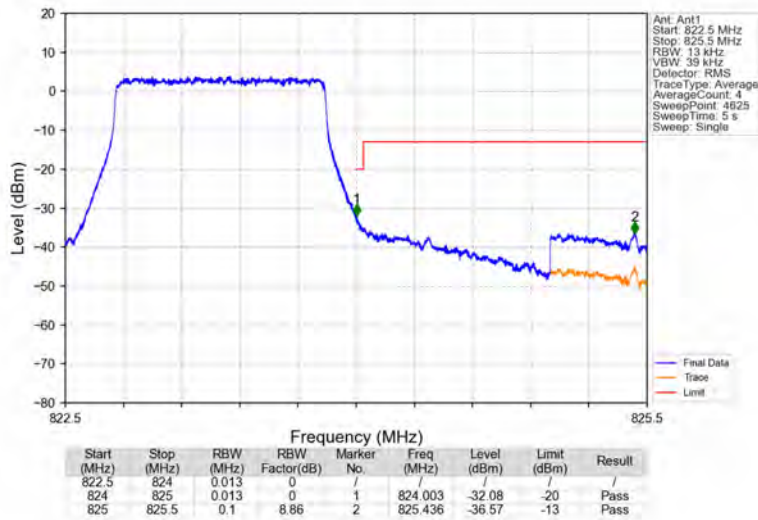
Band26a_1.4MHz_16QAM_HCH_823.3MHz_RB_6_0_NTNV
