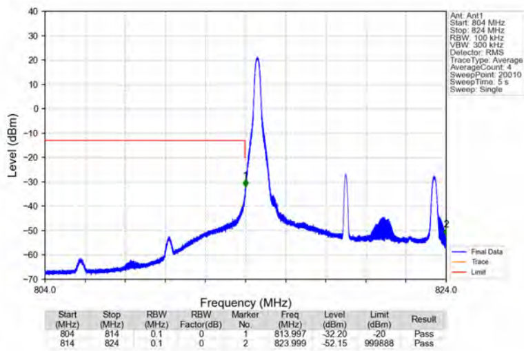
Band26a_10MHz_16QAM_LCH_819MHz_RB_1_0_NTNV
