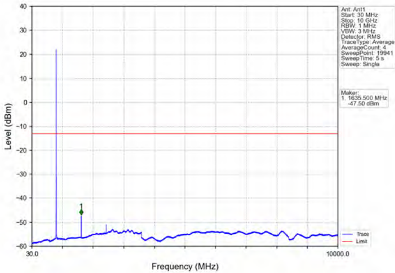
Band26a_3MHz_16QAM_HCH_822.5MHz_RB_1_0_NTNV
