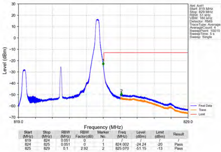
Band26a_5MHz_64QAM_HCH_821.5MHz_RB_1_24_NTNV
