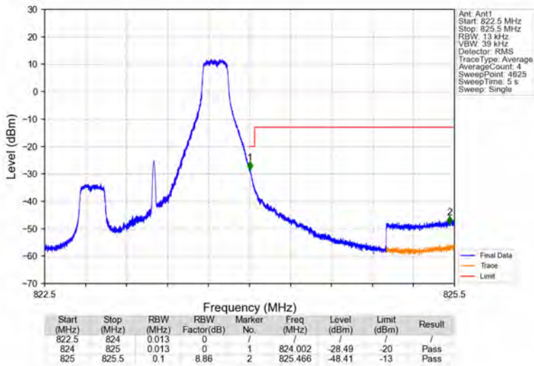
Band26a_1.4MHz_64QAM_HCH_823.3MHz_RB_1_5_NTNV
