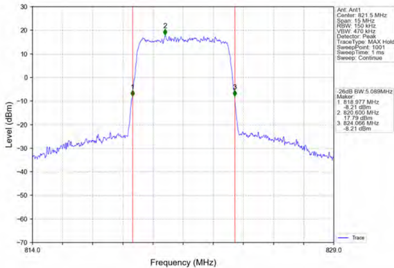
Band26a_5MHz_16QAM_HCH_821.5MHz_RB_25_0_NTNV
