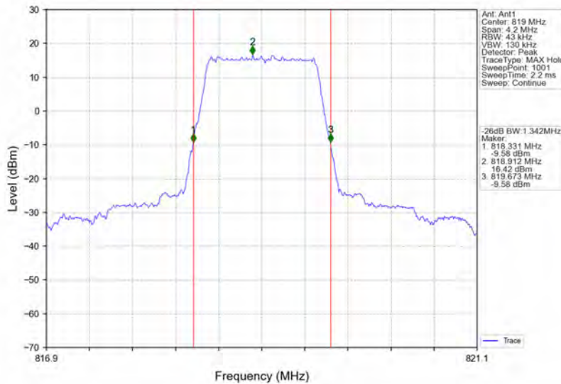
Band26a_1.4MHz_64QAM_MCH_819MHz_RB_6_0_NTNV
