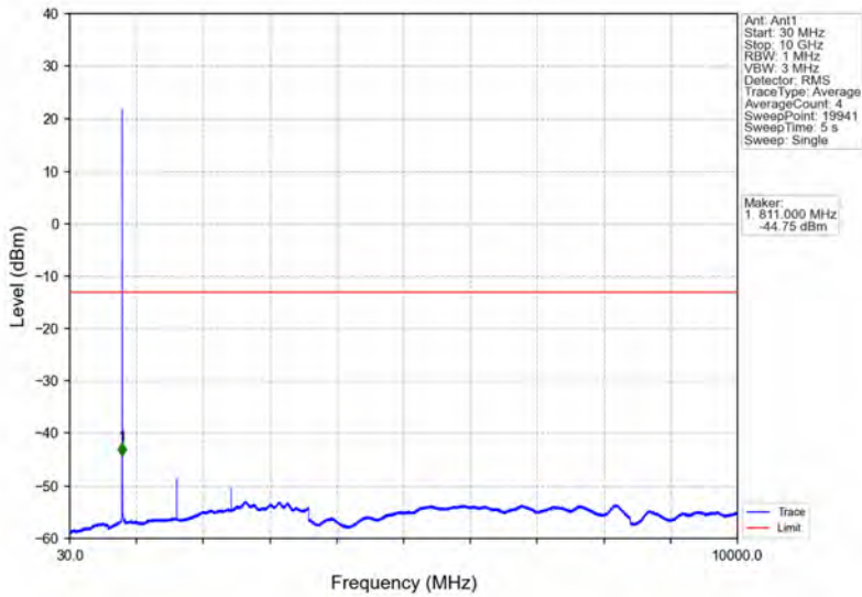
Band26a_1.4MHz_16QAM_LCH_814.7MHz_RB_6_0_NTNV
