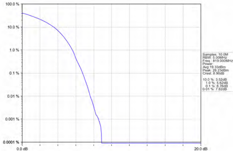
Band26a_10MHz_16QAM_LCH_819MHz_RB_50_0_NTNV
