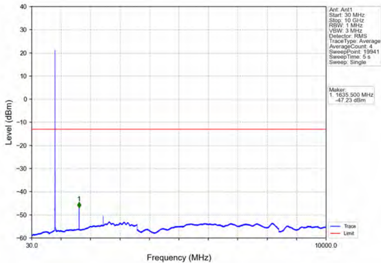
Band26a_3MHz_64QAM_MCH_819MHz_RB_1_0_NTNV
