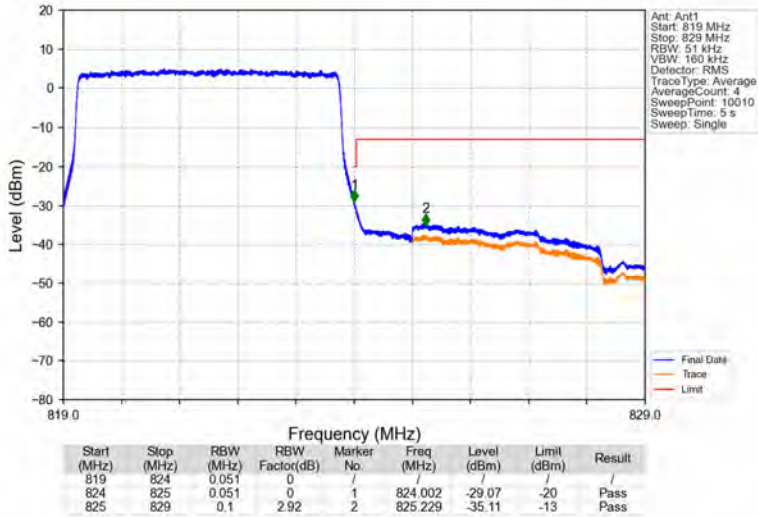
Band26a_5MHz_QPSK_HCH_821.5MHz_RB_25_0_NTNV
