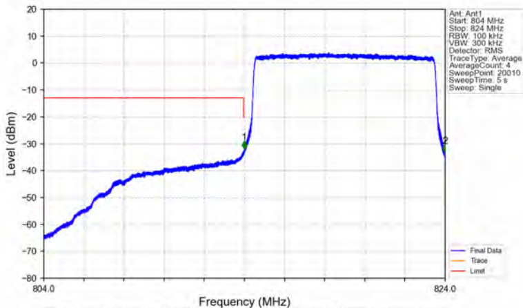
Band26a_10MHz_16QAM_LCH_819MHz_RB_50_0_NTNV
