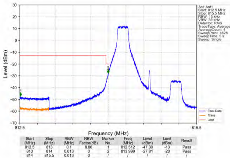
Band26a_1.4MHz_16QAM_LCH_814.7MHz_RB_1_0_NTNV
