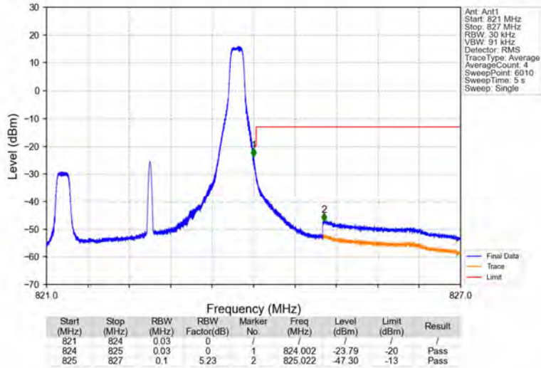
Band26a_3MHz_16QAM_HCH_822.5MHz_RB_1_14_NTNV
