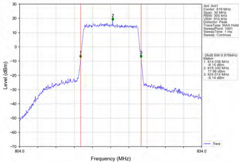
Band26a_10MHz_64QAM_HCH_819MHz_RB_50_0_NTNV
