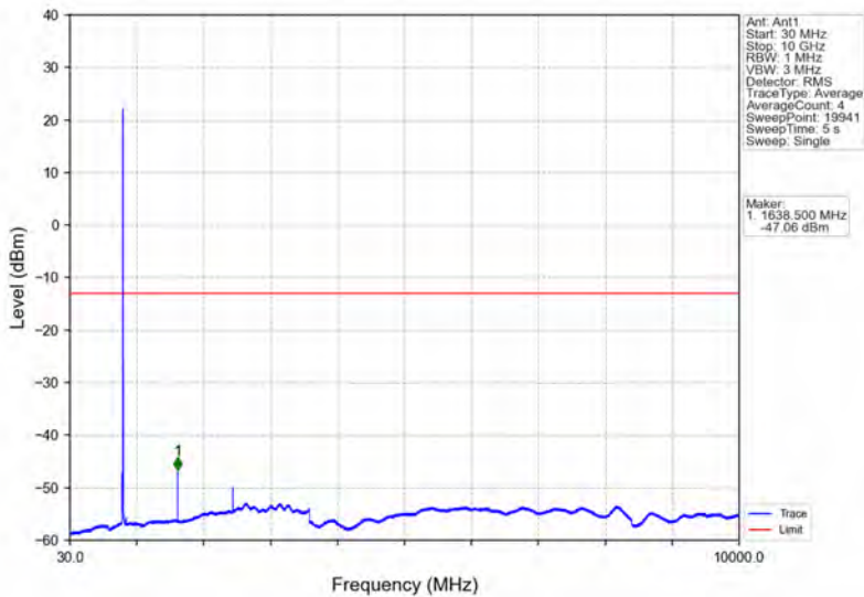
Band26a_5MHz_16QAM_HCH_821.5MHz_RB_1_0_NTNV
