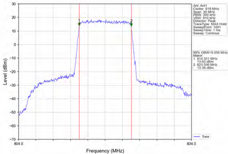
Band26a_10MHz_QPSK_HCH_819MHz_RB_50_0_NTNV
