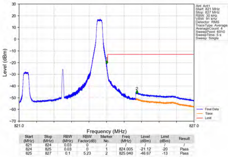
Band26a_3MHz_QPSK_HCH_822.5MHz_RB_1_14_NTNV
