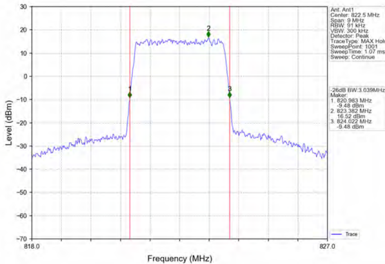
Band26a_3MHz_64QAM_HCH_822.5MHz_RB_15_0_NTNV
