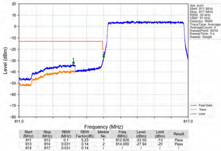
Band26a_3MHz_QPSK_LCH_815.5MHz_RB_15_0_NTNV
