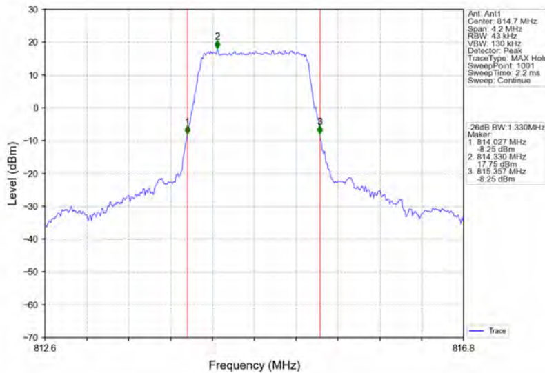
Band26a_1.4MHz_16QAM_LCH_814.7MHz_RB_6_0_NTNV
