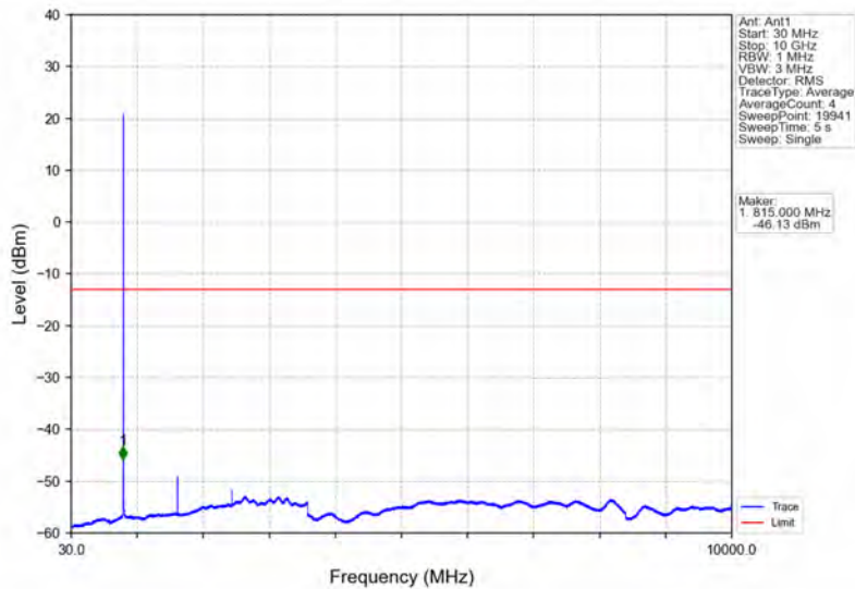
Band26a_1.4MHz_64QAM_MCH_819MHz_RB_1_0_NTNV
