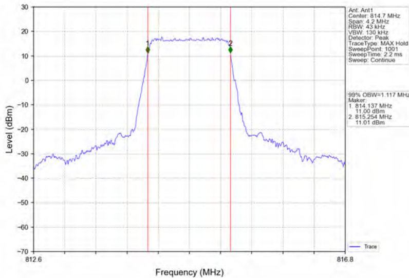
Band26a_1.4MHz_16QAM_LCH_814.7MHz_RB_6_0_NTNV
