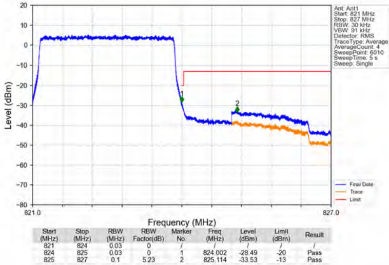
Band26a_3MHz_QPSK_HCH_822.5MHz_RB_15_0_NTNV
