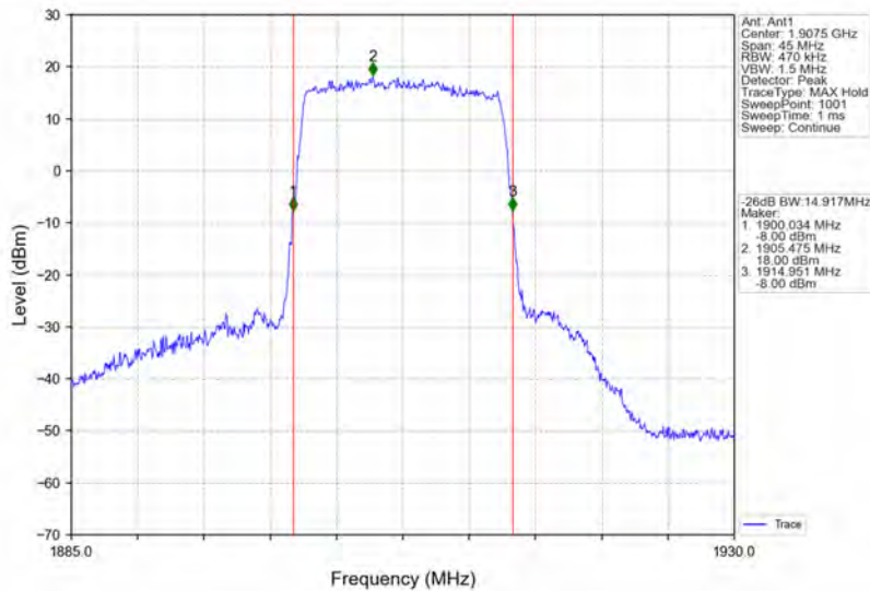
Band25_15MHz_16QAM_HCH_1907.5MHz_RB_75_0_NTNV
