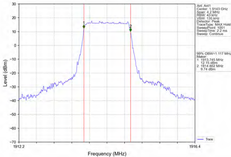
Band25_1.4MHz_16QAM_HCH_1914.3MHz_RB_6_0_NTNV
