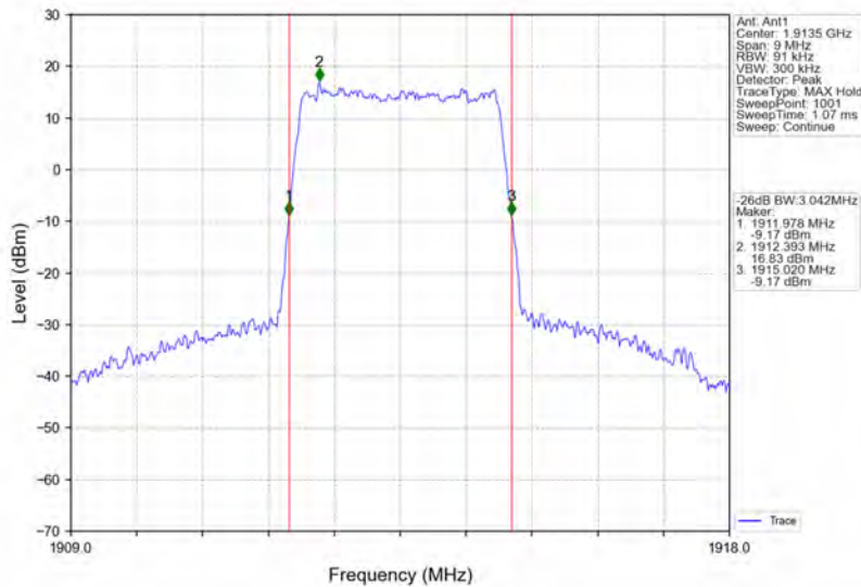
Band25_3MHz_64QAM_HCH_1913.5MHz_RB_15_0_NTNV
