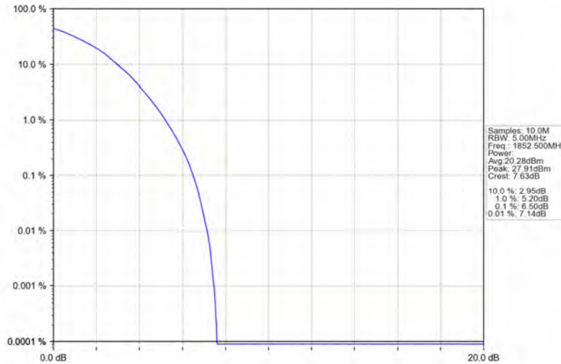
Band25_5MHz_64QAM_LCH_1852.5MHz_RB_25_0_NTNV
