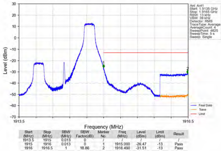
Band25_1.4MHz_QPSK_HCH_1914.3MHz_RB_1_5_NTNV
