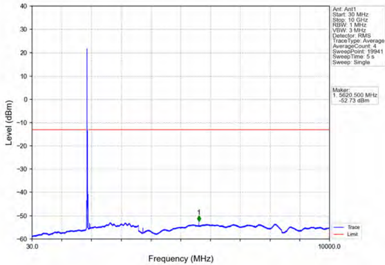
Band25_20MHz_16QAM_MCH_1882.5MHz_RB_1_0_NTNV
