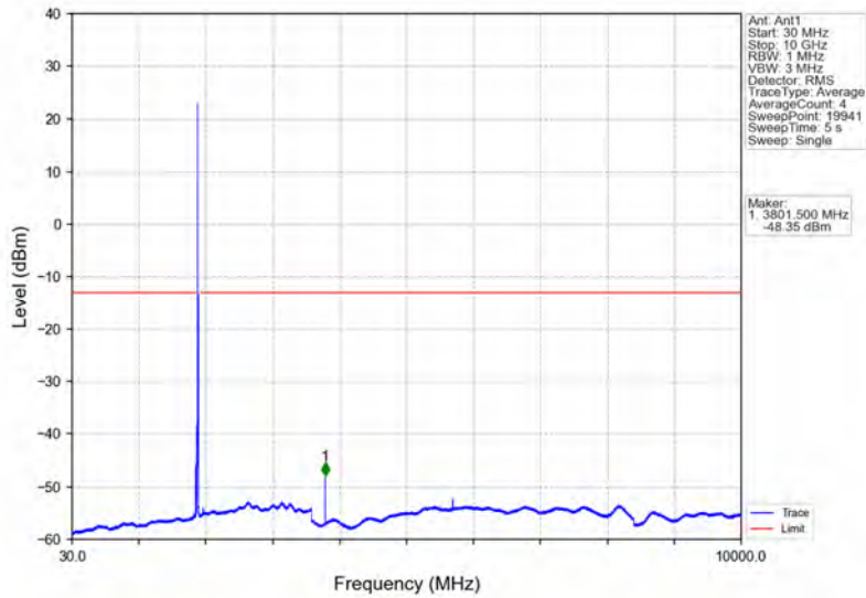
Band25_15MHz_QPSK_HCH_1907.5MHz_RB_1_0_NTNV
