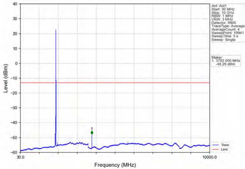
Band25_20MHz_16QAM_HCH_1905MHz_RB_1_0_NTNV
