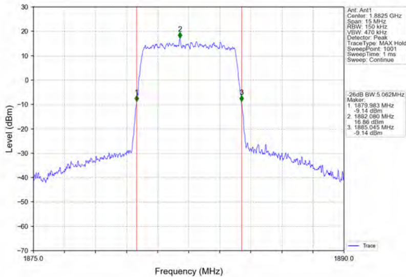
Band25_5MHz_64QAM_MCH_1882.5MHz_RB_25_0_NTNV
