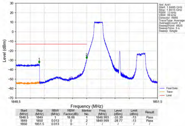
Band25_1.4MHz_64QAM_LCH_1850.7MHz_RB_1_0_NTNV
