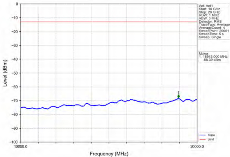
Band25_5MHz_QPSK_MCH_1882.5MHz_RB_1_0_NTNV
