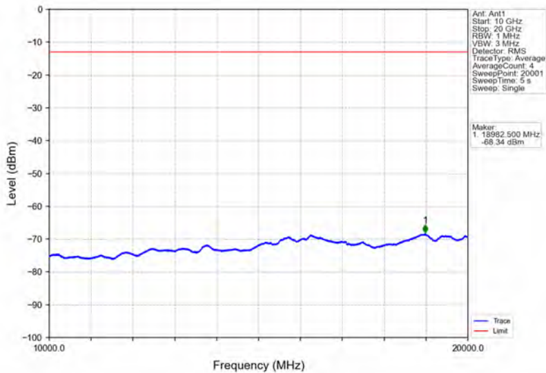
Band25_3MHz_QPSK_MCH_1882.5MHz_RB_1_0_NTNV
