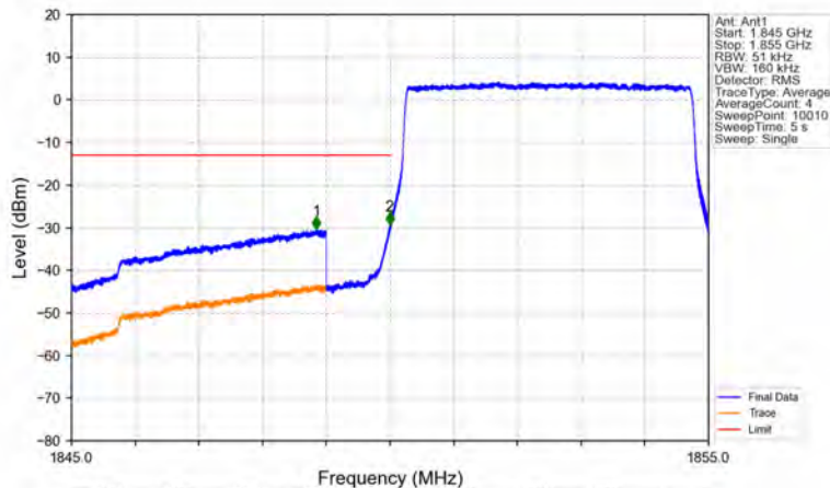
Band25_5MHz_QPSK_LCH_1852.5MHz_RB_25_0_NTNV
