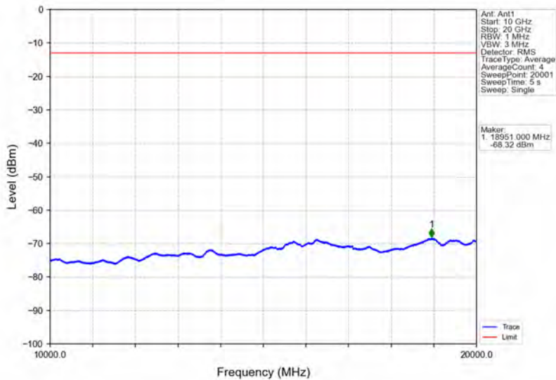
Band25_20MHz_16QAM_MCH_1882.5MHz_RB_1_0_NTNV
