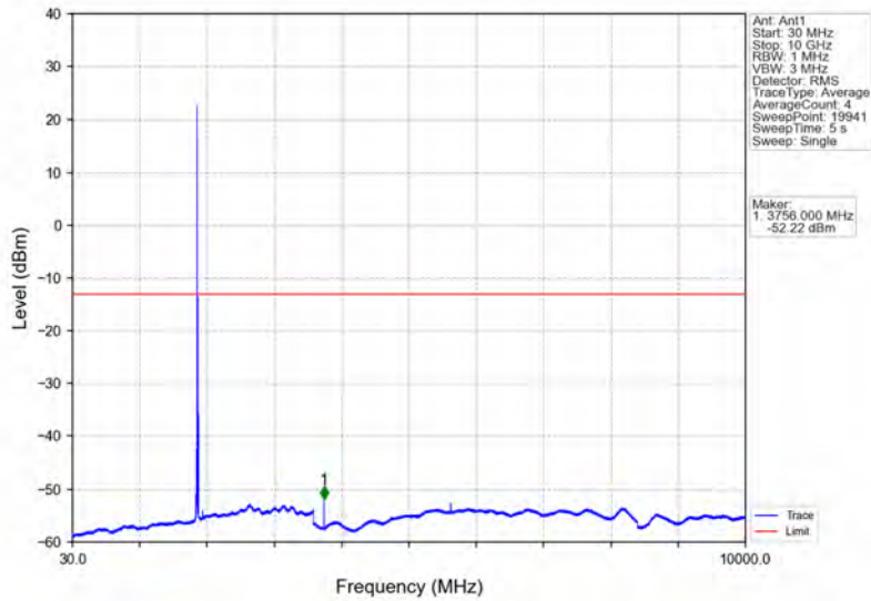
Band25_10MHz_16QAM_MCH_1882.5MHz_RB_1_0_NTNV
