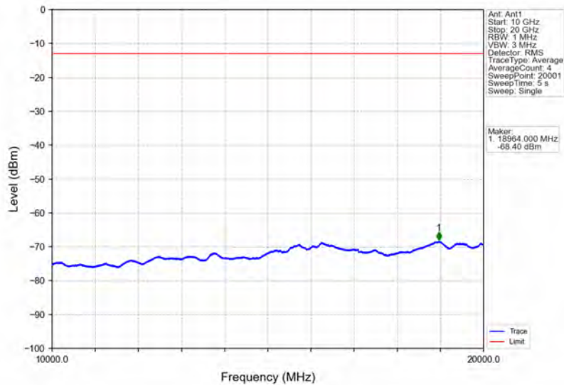
Band25_3MHz_QPSK_HCH_1913.5MHz_RB_1_0_NTNV
