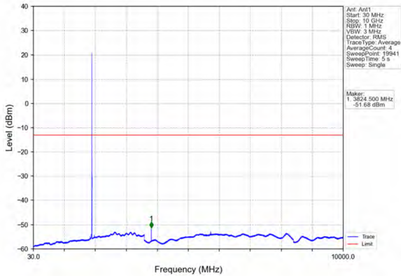
Band25_3MHz_64QAM_HCH_1913.5MHz_RB_1_0_NTNV
