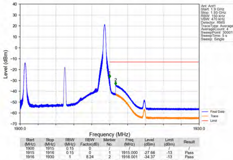
Band25_15MHz_QPSK_HCH_1907.5MHz_RB_1_74_NTNV
