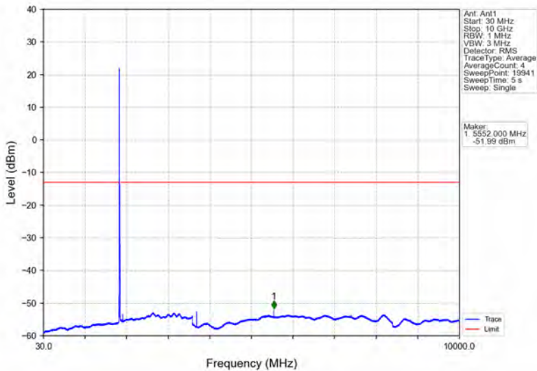
Band25_10MHz_16QAM_LCH_1855MHz_RB_1_0_NTNV
