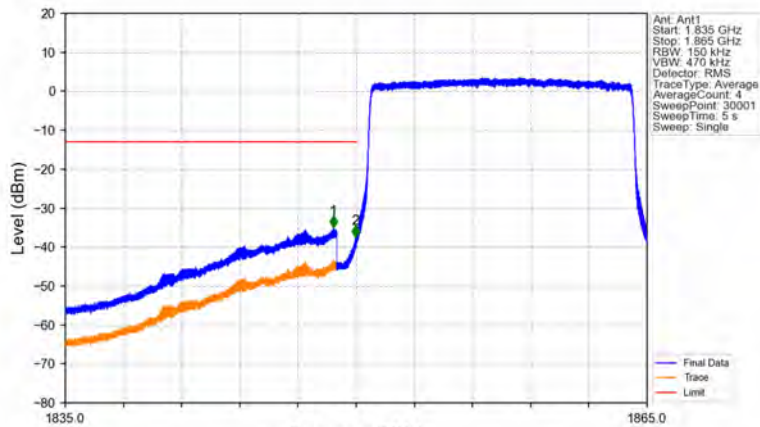
Band25_15MHz_16QAM_LCH_1857.5MHz_RB_75_0_NTNV
