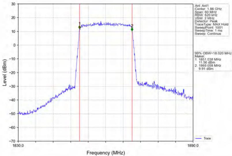
Band25_20MHz_64QAM_LCH_1860MHz_RB_100_0_NTNV
