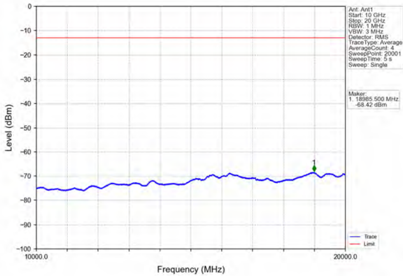
Band25_3MHz_64QAM_LCH_1851.5MHz_RB_15_0_NTNV
