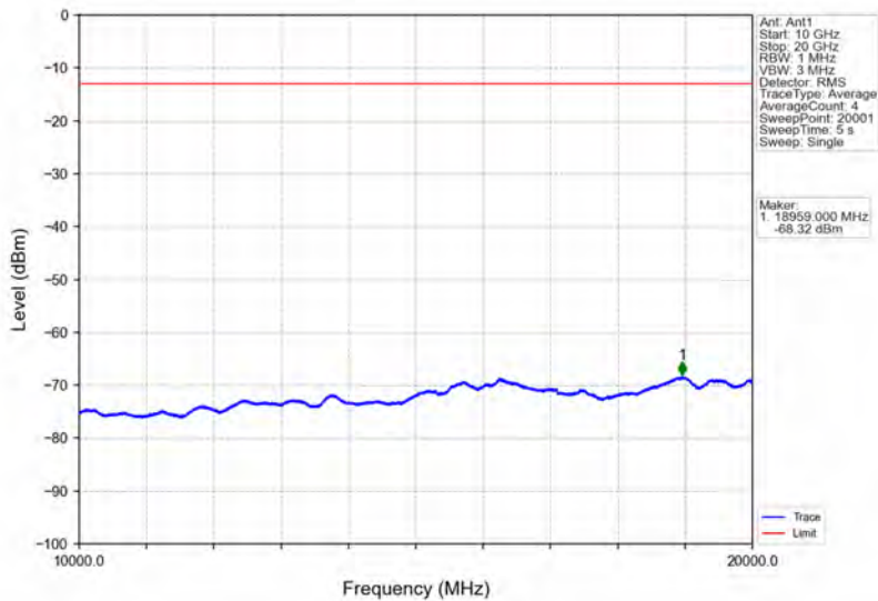
Band25_10MHz_16QAM_MCH_1882.5MHz_RB_1_0_NTNV
