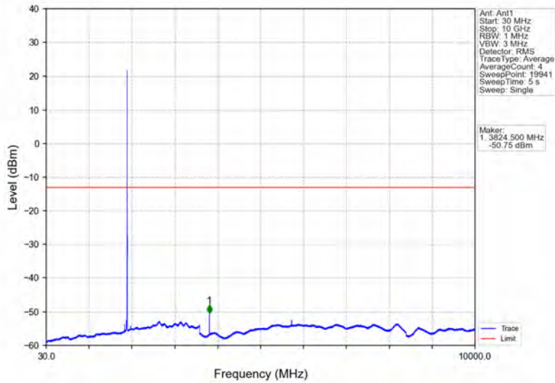
Band25_3MHz_16QAM_HCH_1913.5MHz_RB_1_0_NTNV
