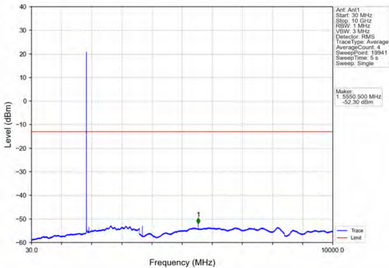
Band25_3MHz_64QAM_LCH_1851.5MHz_RB_1_0_NTNV
