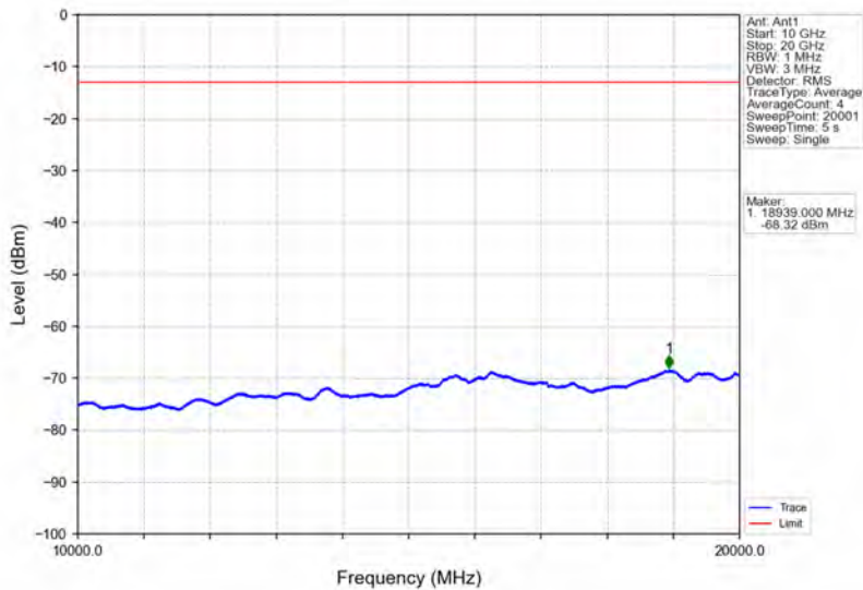
Band25_10MHz_64QAM_HCH_1910MHz_RB_1_0_NTNV
