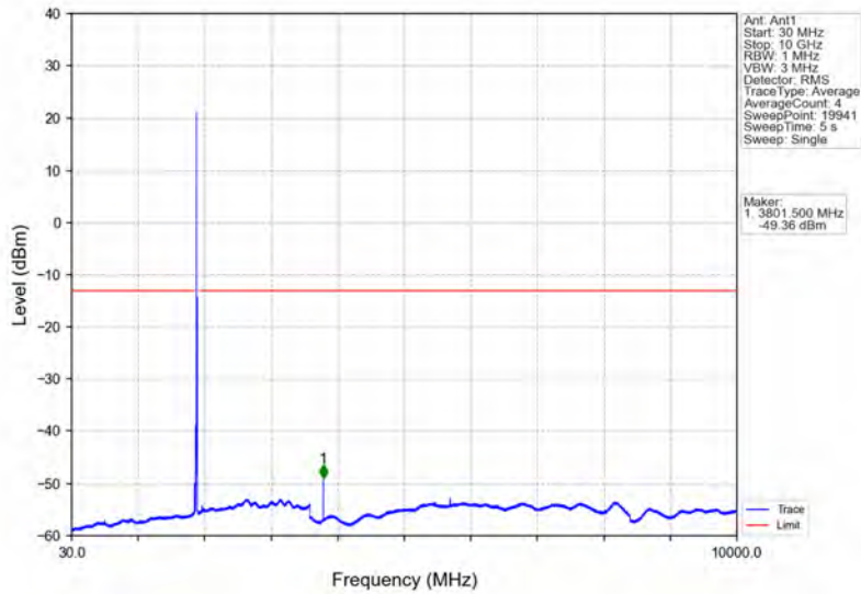
Band25_15MHz_64QAM_HCH_1907.5MHz_RB_1_0_NTNV
