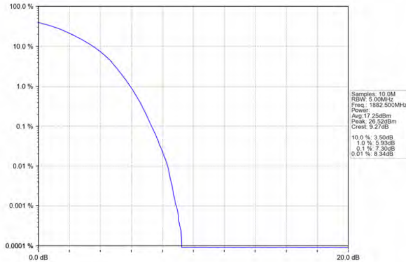
Band25_15MHz_16QAM_MCH_1882.5MHz_RB_75_0_NTNV
