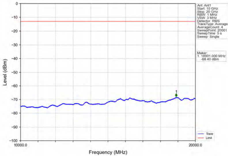
Band25_5MHz_64QAM_LCH_1852.5MHz_RB_25_0_NTNV
