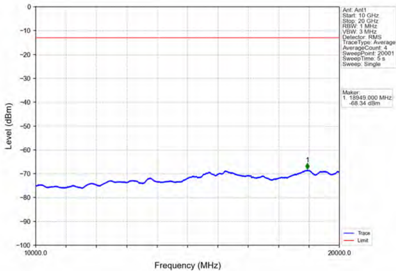
Band25_1.4MHz_16QAM_MCH_1882.5MHz_RB_1_0_NTNV
