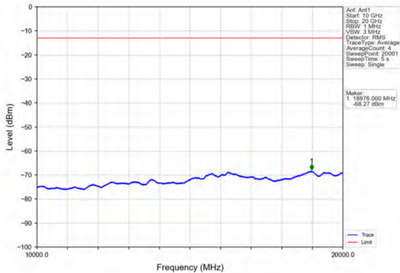
Band25_15MHz_QPSK_HCH_1907.5MHz_RB_1_0_NTNV
