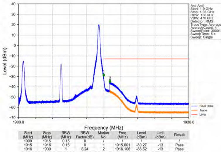
Band25_15MHz_64QAM_HCH_1907.5MHz_RB_1_74_NTNV
