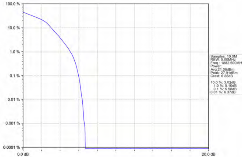
Band25_1.4MHz_16QAM_MCH_1882.5MHz_RB_6_0_NTNV
