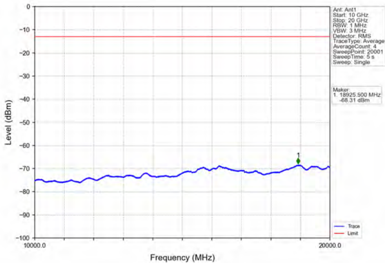
Band25_15MHz_16QAM_HCH_1907.5MHz_RB_1_0_NTNV
