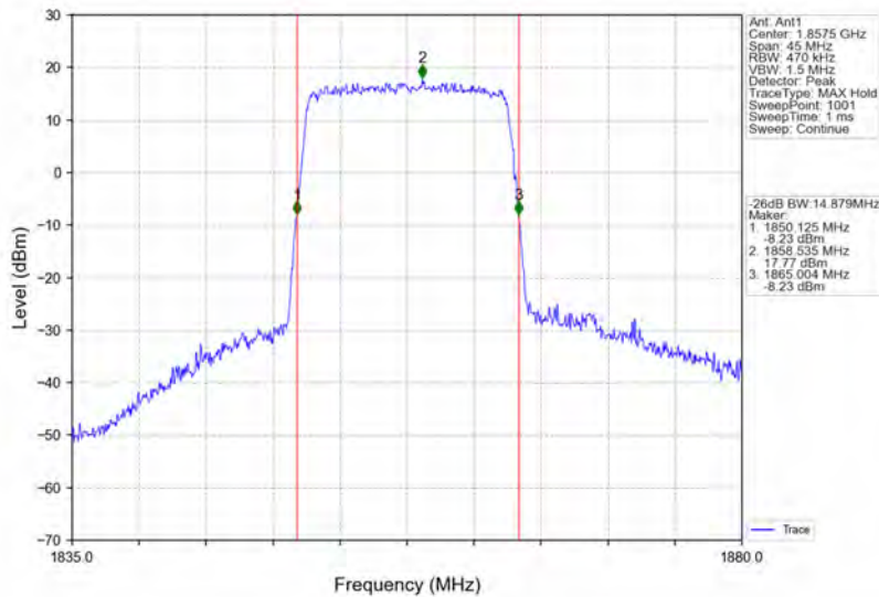
Band25_15MHz_16QAM_LCH_1857.5MHz_RB_75_0_NTNV
