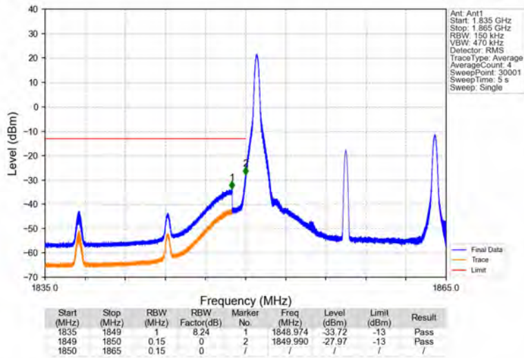
Band25_15MHz_16QAM_LCH_1857.5MHz_RB_1_0_NTNV
