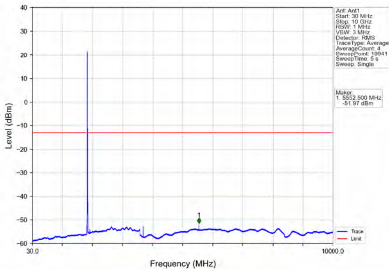
Band25_15MHz_64QAM_LCH_1857.5MHz_RB_1_0_NTNV
