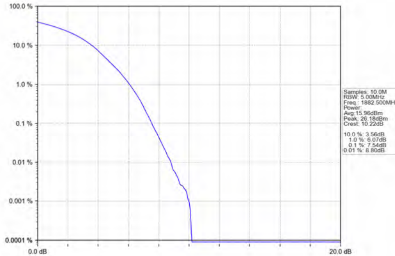
Band25_20MHz_16QAM_MCH_1882.5MHz_RB_100_0_NTNV
