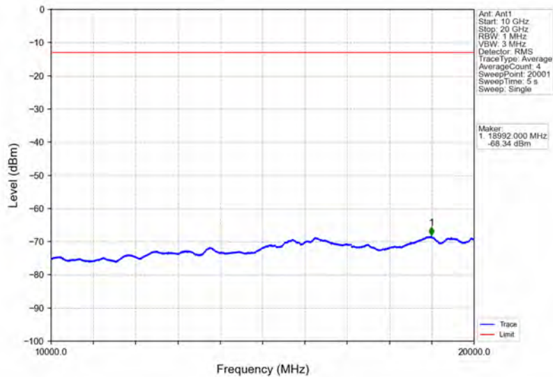
Band25_5MHz_QPSK_HCH_1912.5MHz_RB_1_0_NTNV
