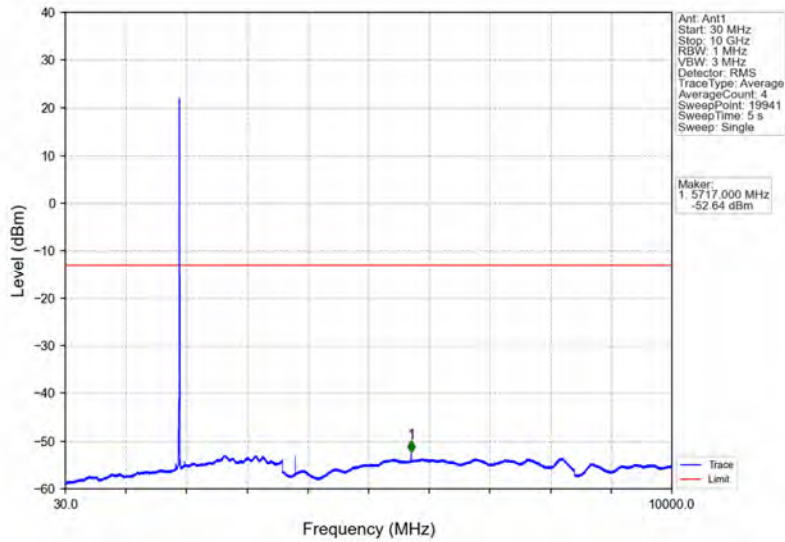
Band25_10MHz_16QAM_HCH_1910MHz_RB_1_0_NTNV
