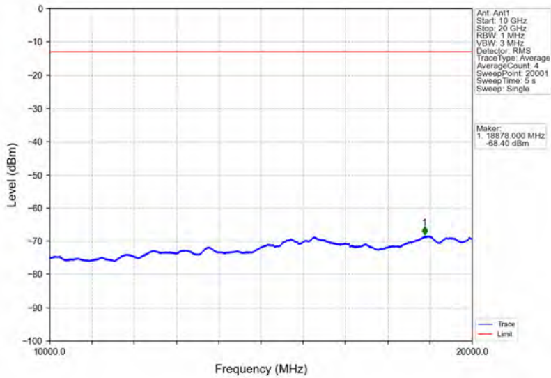
Band25_1.4MHz_16QAM_LCH_1850.7MHz_RB_6_0_NTNV
