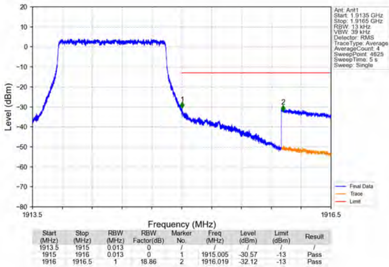
Band25_1.4MHz_16QAM_HCH_1914.3MHz_RB_6_0_NTNV
