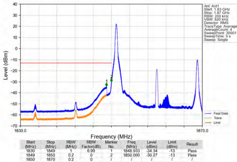
Band25_20MHz_16QAM_LCH_1860MHz_RB_1_0_NTNV
