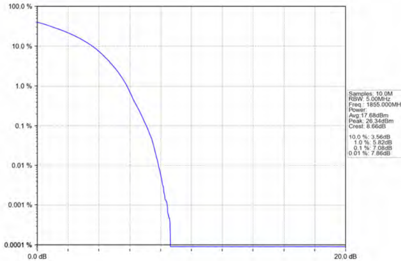
Band25_10MHz_64QAM_LCH_1855MHz_RB_50_0_NTNV
