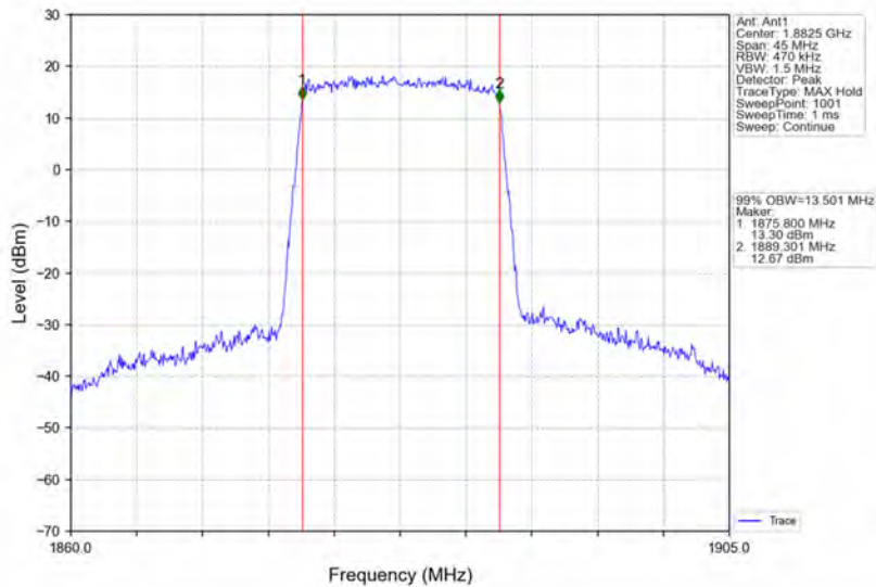
Band25_15MHz_QPSK_MCH_1882.5MHz_RB_75_0_NTNV
