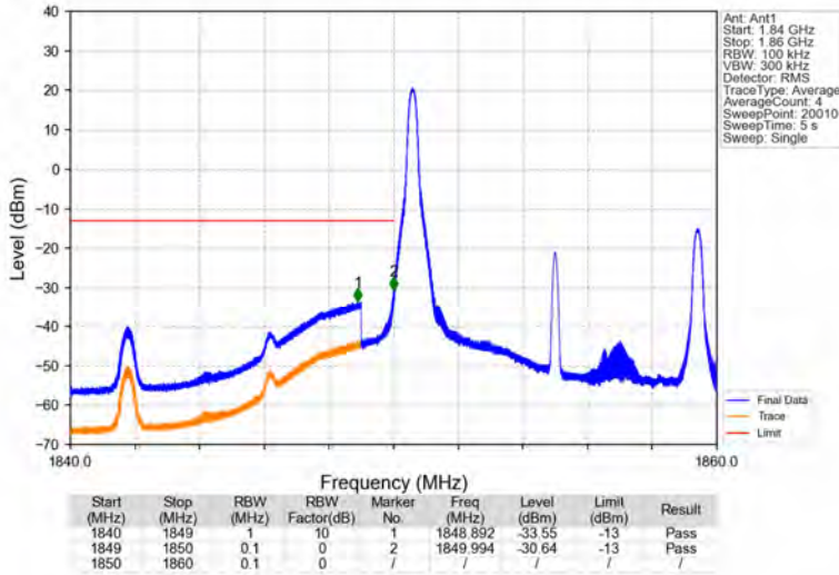
Band25_10MHz_16QAM_LCH_1855MHz_RB_1_0_NTNV
