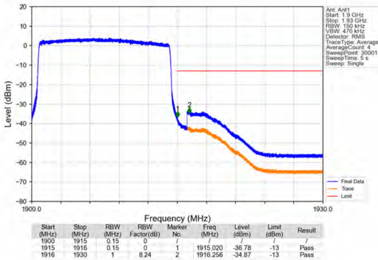
Band25_15MHz_16QAM_HCH_1907.5MHz_RB_75_0_NTNV
