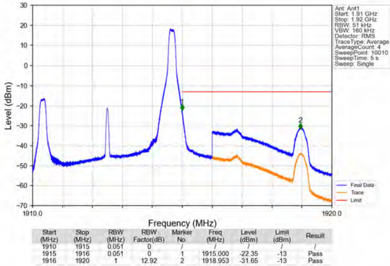
Band25_5MHz_QPSK_HCH_1912.5MHz_RB_1_24_NTNV
