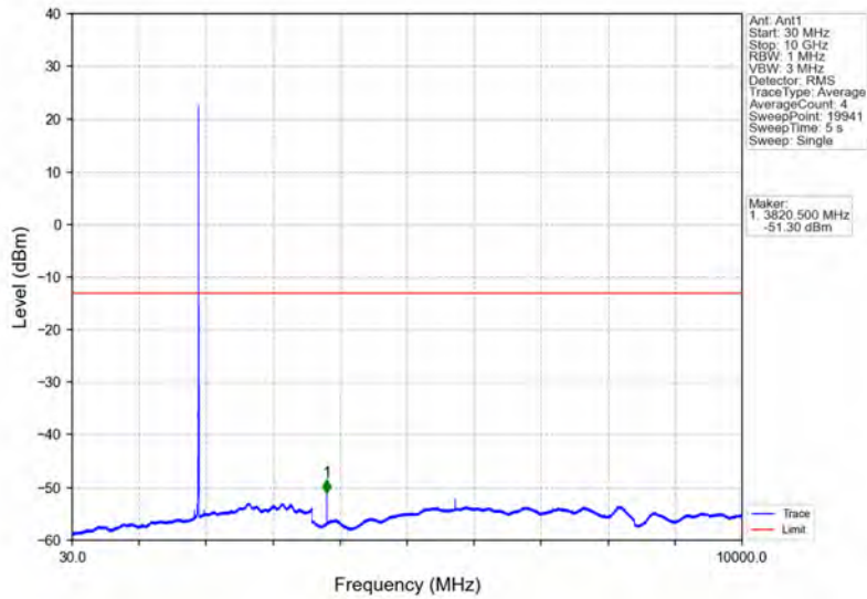
Band25_5MHz_QPSK_HCH_1912.5MHz_RB_1_0_NTNV
