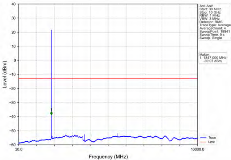
Band25_1.4MHz_16QAM_LCH_1850.7MHz_RB_1_0_NTNV
