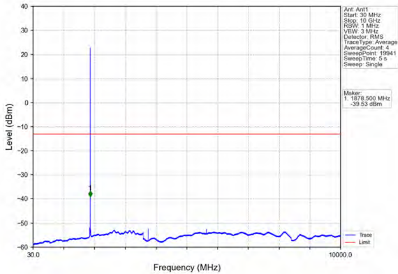
Band25_1.4MHz_QPSK_MCH_1882.5MHz_RB_1_0_NTNV
