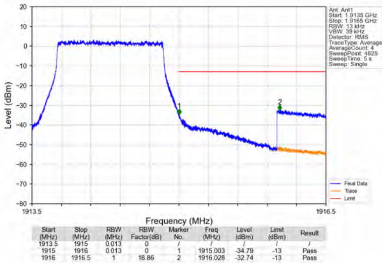
Band25_1.4MHz_64QAM_HCH_1914.3MHz_RB_6_0_NTNV
