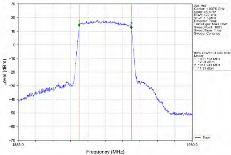
Band25_15MHz_16QAM_HCH_1907.5MHz_RB_75_0_NTNV
