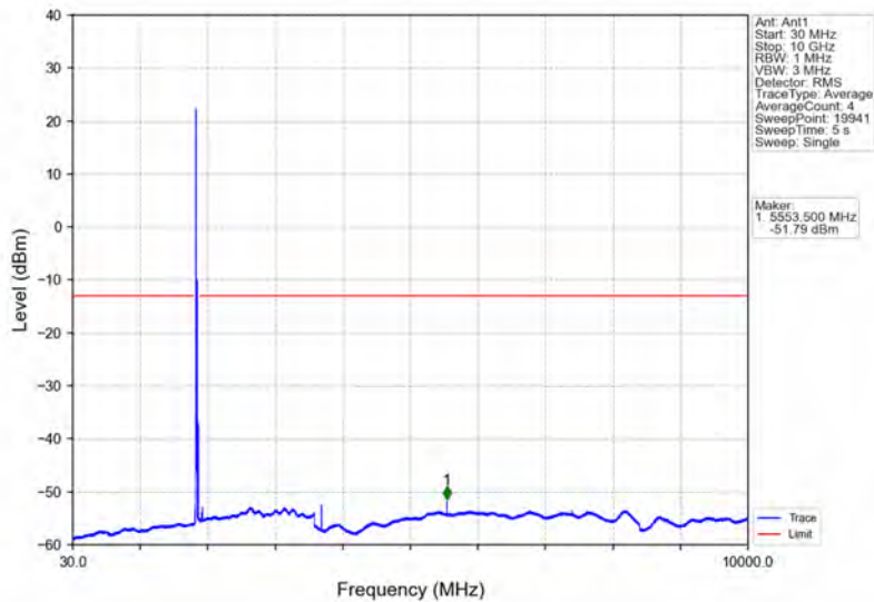
Band25_20MHz_16QAM_LCH_1860MHz_RB_1_0_NTNV
