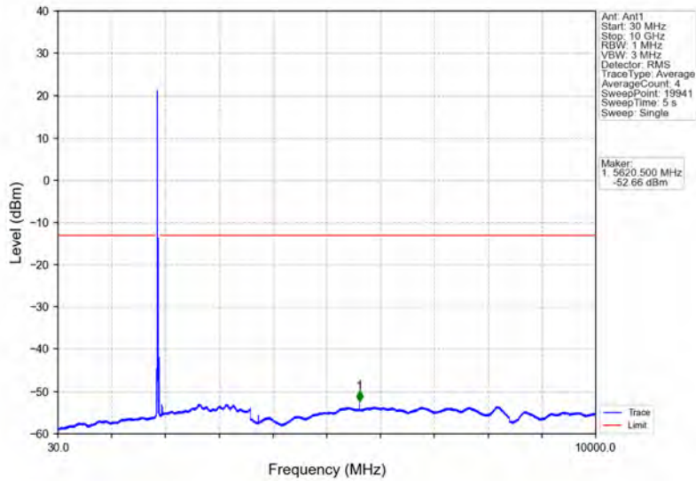
Band25_20MHz_64QAM_MCH_1882.5MHz_RB_1_0_NTNV
