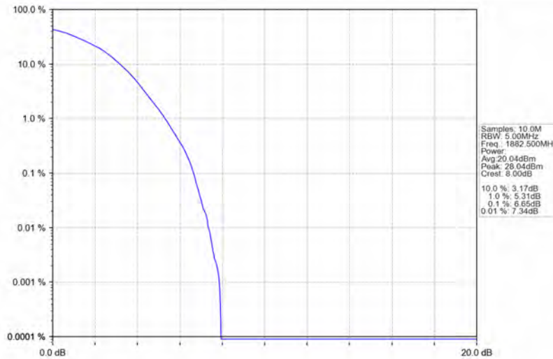
Band25_1.4MHz_64QAM_MCH_1882.5MHz_RB_6_0_NTNV
