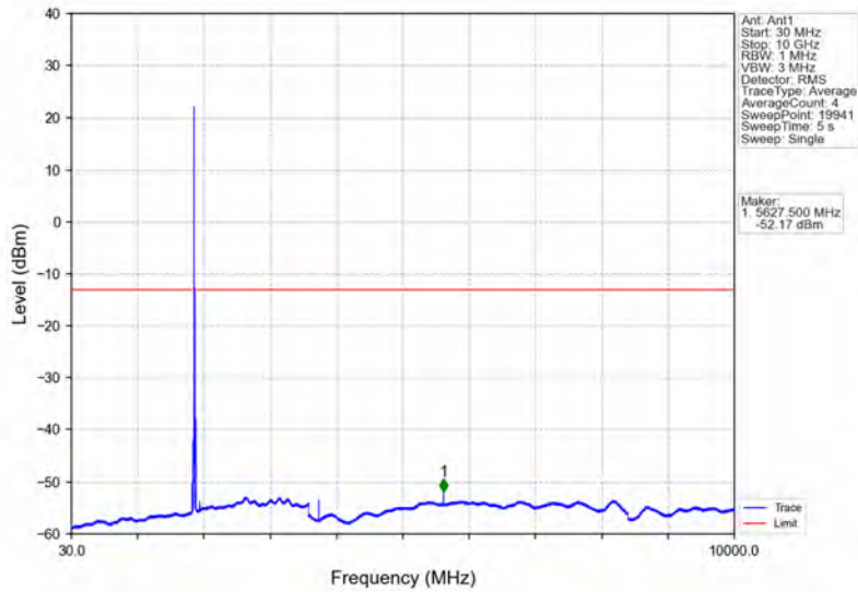
Band25_15MHz_16QAM_MCH_1882.5MHz_RB_1_0_NTNV
