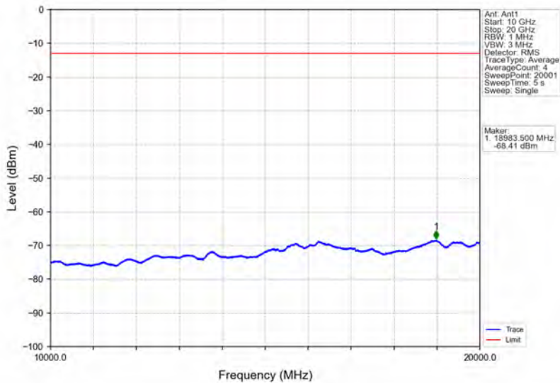
Band25_1.4MHz_QPSK_MCH_1882.5MHz_RB_1_0_NTNV
