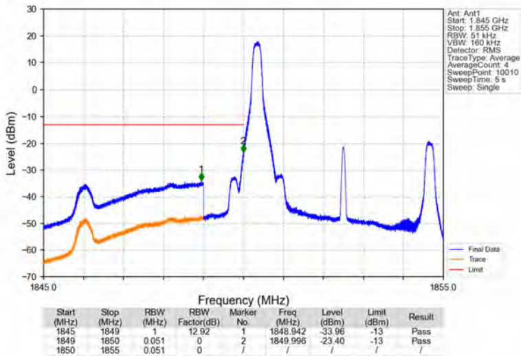
Band25_5MHz_16QAM_LCH_1852.5MHz_RB_1_0_NTNV
