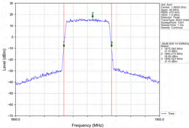
Band25_15MHz_64QAM_MCH_1882.5MHz_RB_75_0_NTNV
