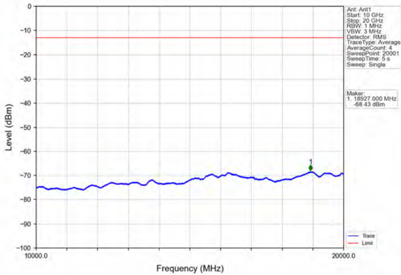
Band25_3MHz_16QAM_LCH_1851.5MHz_RB_15_0_NTNV
