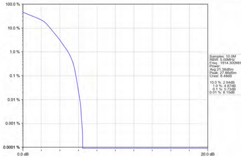
Band25_1.4MHz_16QAM_HCH_1914.3MHz_RB_6_0_NTNV
