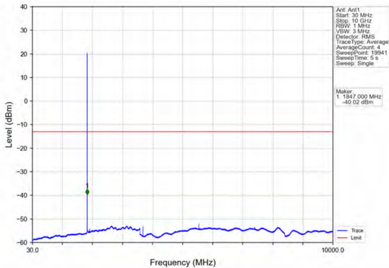
Band25_1.4MHz_64QAM_LCH_1850.7MHz_RB_1_0_NTNV
