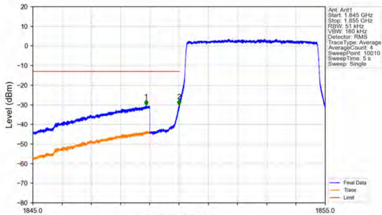
Band25_5MHz_16QAM_LCH_1852.5MHz_RB_25_0_NTNV
