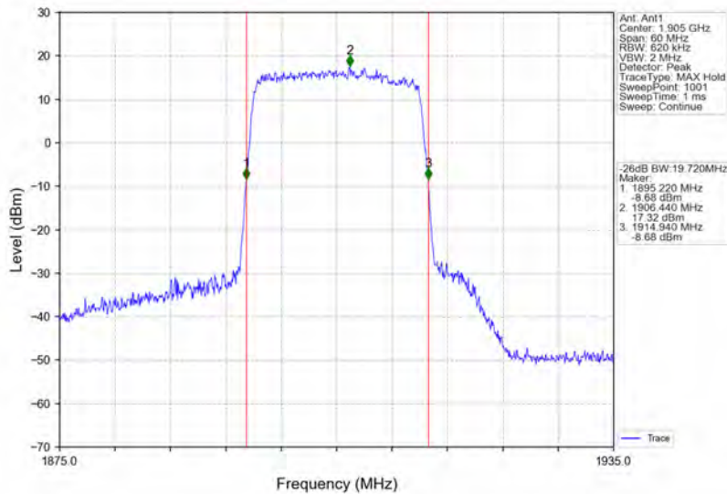
Band25_20MHz_64QAM_HCH_1905MHz_RB_100_0_NTNV
