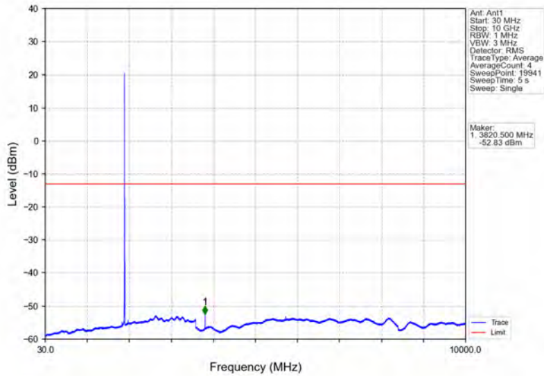
Band25_5MHz_64QAM_HCH_1912.5MHz_RB_1_0_NTNV
