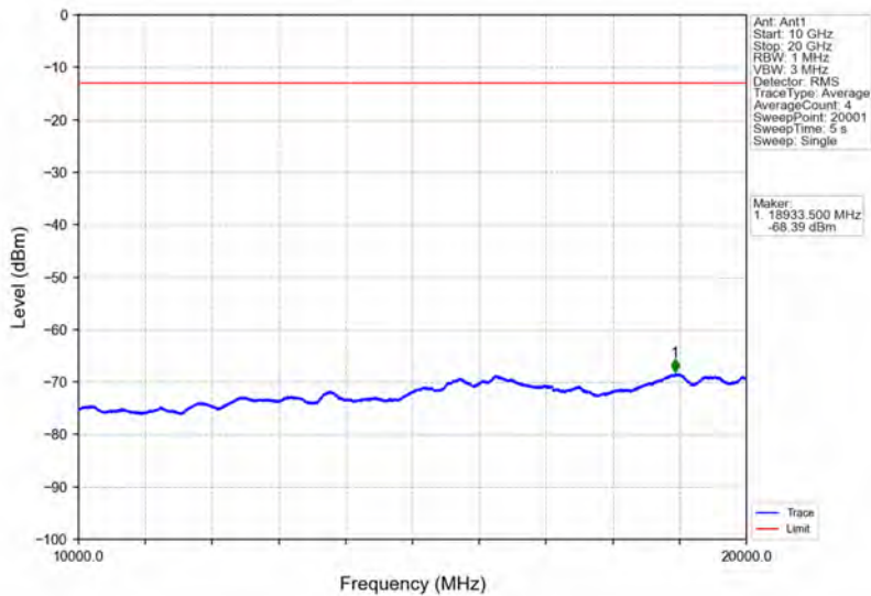
Band25_15MHz_64QAM_MCH_1882.5MHz_RB_1_0_NTNV
