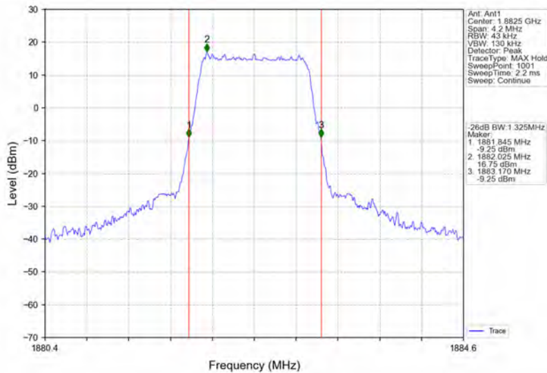
Band25_1.4MHz_64QAM_MCH_1882.5MHz_RB_6_0_NTNV
