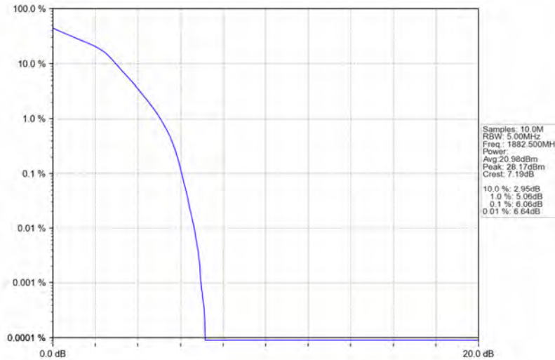
Band25_3MHz_16QAM_MCH_1882.5MHz_RB_15_0_NTNV
