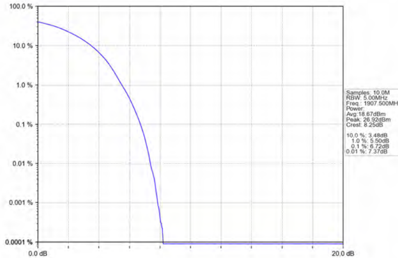
Band25_15MHz_QPSK_HCH_1907.5MHz_RB_75_0_NTNV
