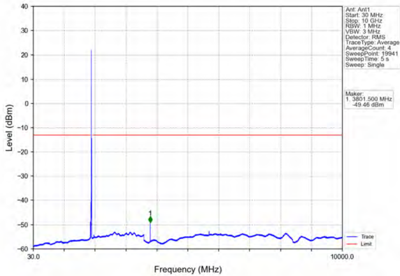
Band25_15MHz_16QAM_HCH_1907.5MHz_RB_1_0_NTNV
