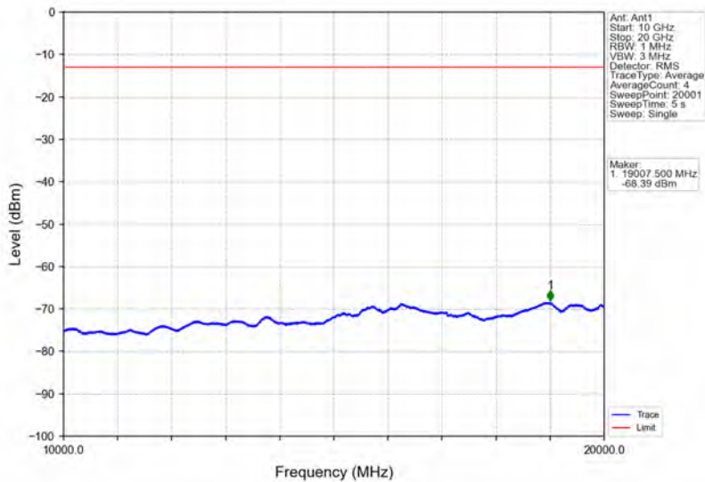
Band25_10MHz_64QAM_MCH_1882.5MHz_RB_1_0_NTNV
