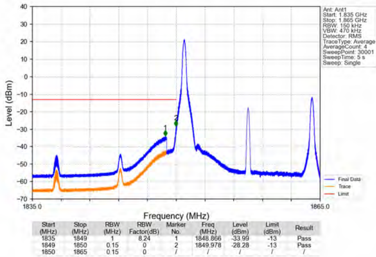
Band25_15MHz_64QAM_LCH_1857.5MHz_RB_1_0_NTNV
