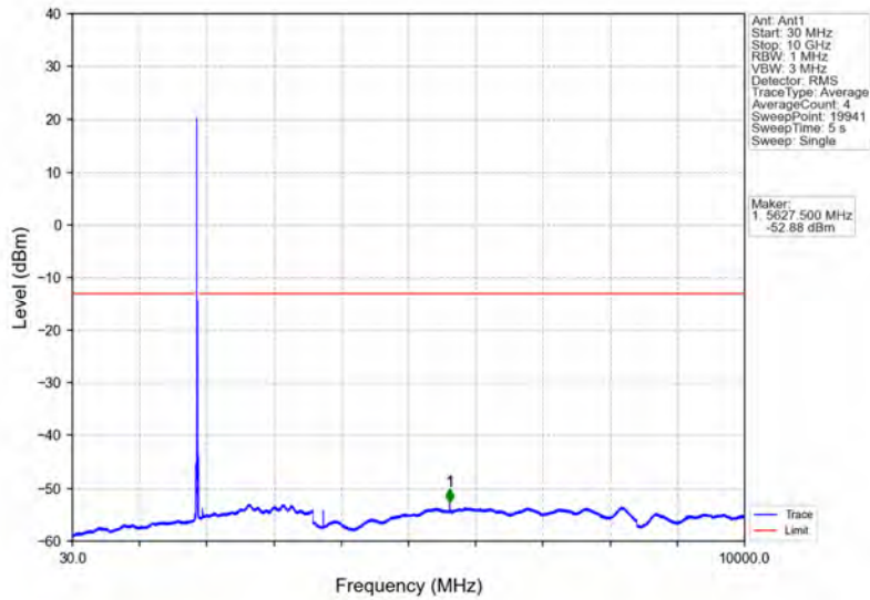
Band25_15MHz_64QAM_MCH_1882.5MHz_RB_1_0_NTNV
