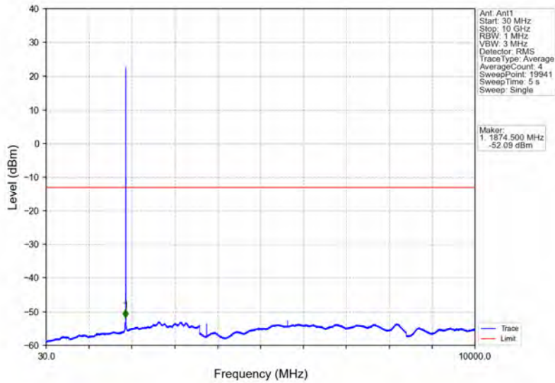
Band25_3MHz_QPSK_MCH_1882.5MHz_RB_1_0_NTNV
