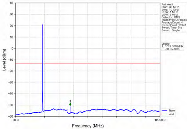
Band25_20MHz_64QAM_HCH_1905MHz_RB_1_0_NTNV
