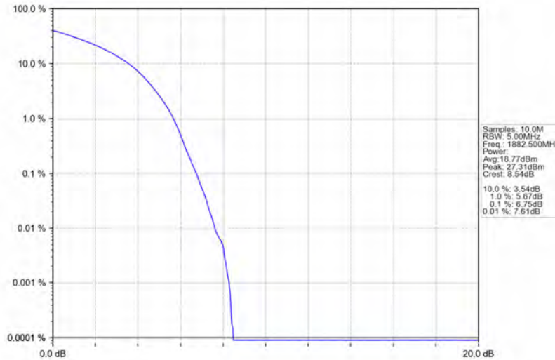
Band25_10MHz_16QAM_MCH_1882.5MHz_RB_50_0_NTNV
