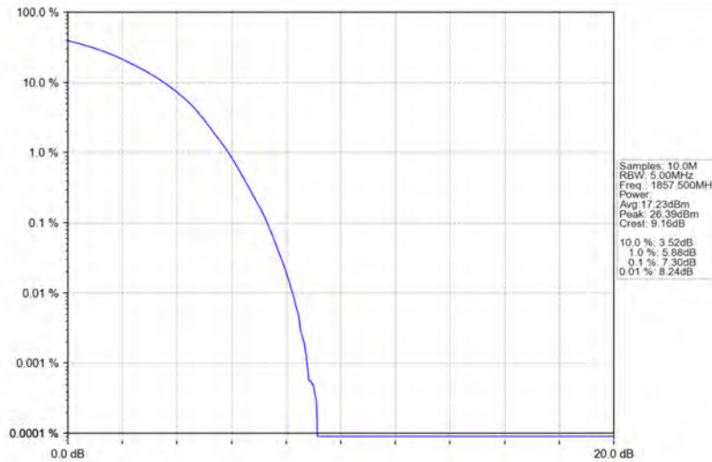
Band25_15MHz_16QAM_LCH_1857.5MHz_RB_75_0_NTNV
