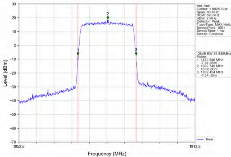
Band25_20MHz_16QAM_MCH_1882.5MHz_RB_100_0_NTNV
