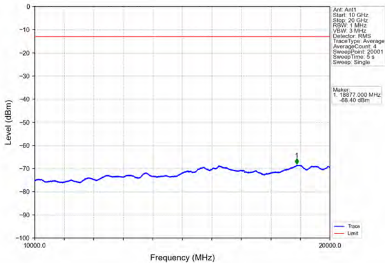
Band25_20MHz_64QAM_MCH_1882.5MHz_RB_1_0_NTNV
