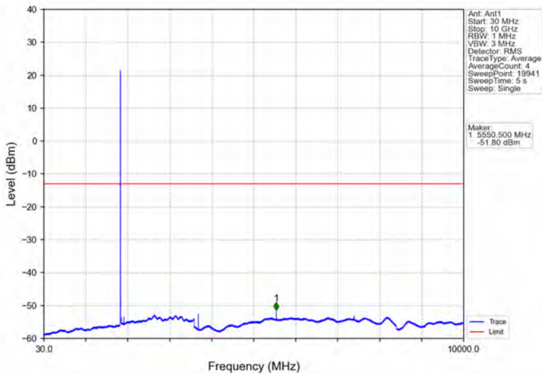
Band25_3MHz_16QAM_LCH_1851.5MHz_RB_1_0_NTNV
