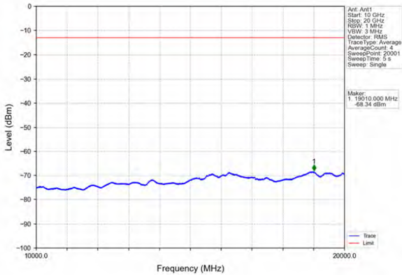
Band25_1.4MHz_64QAM_LCH_1850.7MHz_RB_6_0_NTNV
