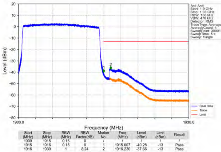
Band25_15MHz_64QAM_HCH_1907.5MHz_RB_75_0_NTNV
