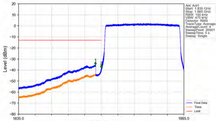
Band25_15MHz_64QAM_LCH_1857.5MHz_RB_75_0_NTNV
