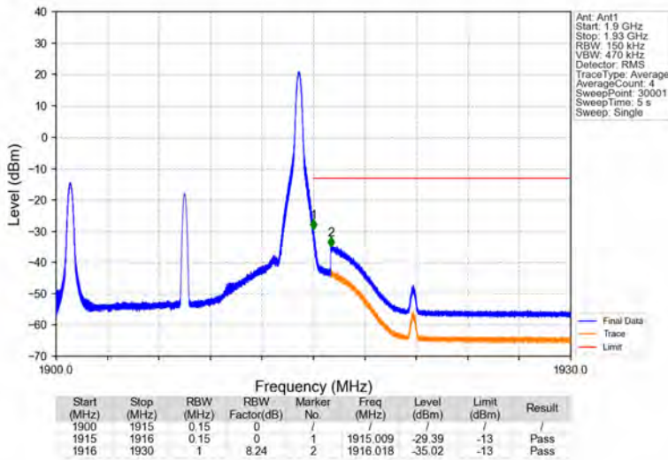
Band25_15MHz_16QAM_HCH_1907.5MHz_RB_1_74_NTNV
