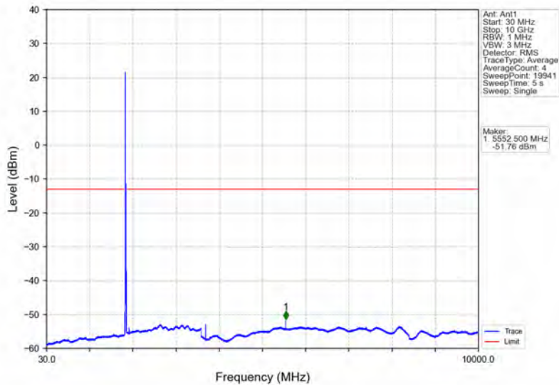
Band25_15MHz_16QAM_LCH_1857.5MHz_RB_1_0_NTNV
