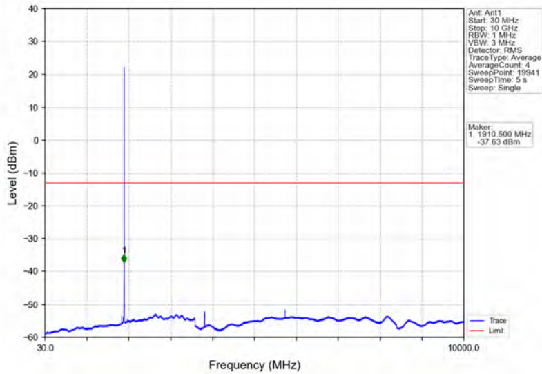
Band25_1.4MHz_16QAM_HCH_1914.3MHz_RB_1_0_NTNV
