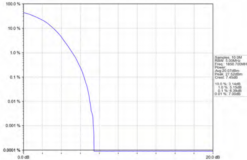
Band25_1.4MHz_64QAM_LCH_1850.7MHz_RB_6_0_NTNV
