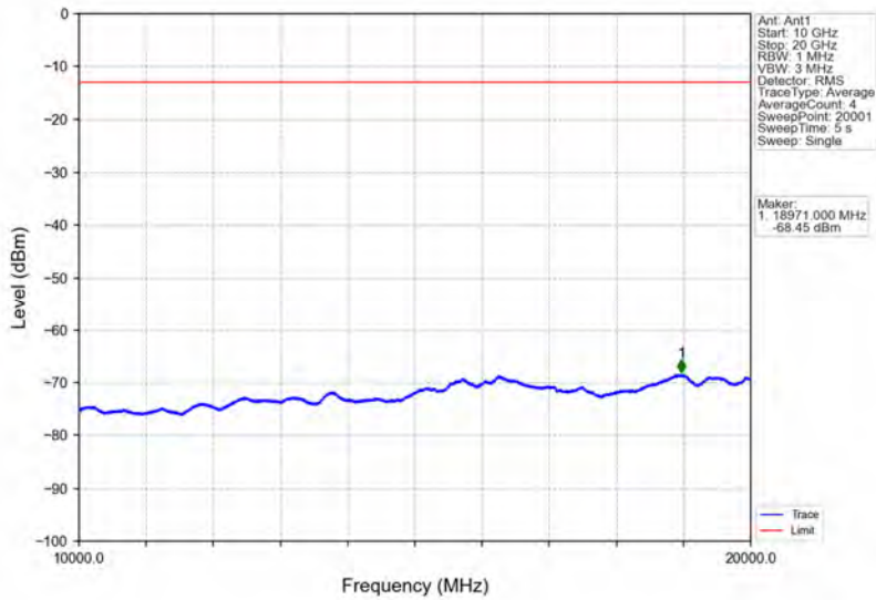
Band25_15MHz_QPSK_LCH_1857.5MHz_RB_75_0_NTNV
