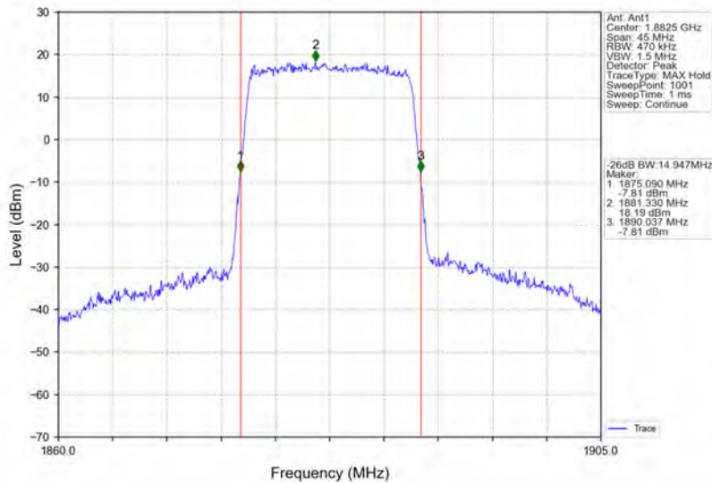
Band25_15MHz_QPSK_MCH_1882.5MHz_RB_75_0_NTNV
