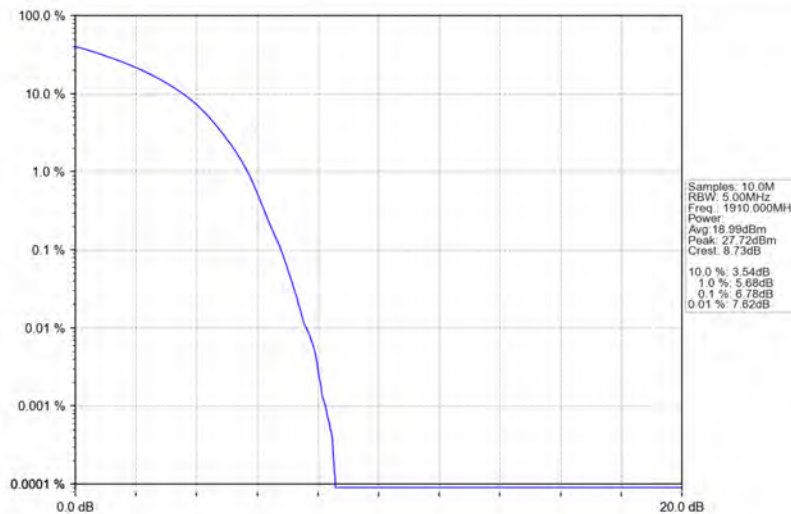
Band25_10MHz_16QAM_HCH_1910MHz_RB_50_0_NTNV
