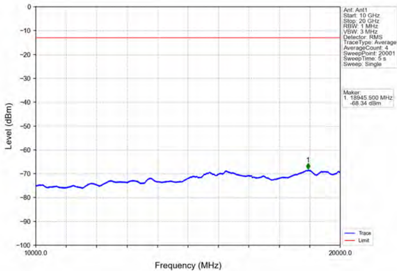
Band25_1.4MHz_64QAM_MCH_1882.5MHz_RB_1_0_NTNV
