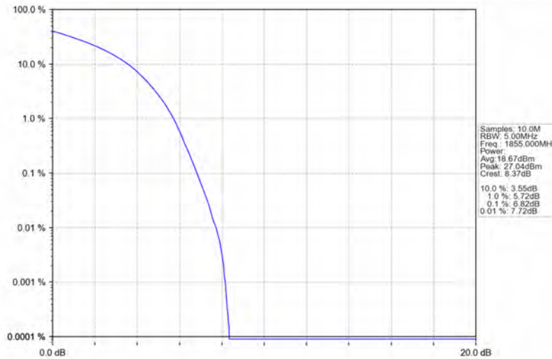
Band25_10MHz_16QAM_LCH_1855MHz_RB_50_0_NTNV
