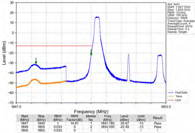
Band25_3MHz_16QAM_LCH_1851.5MHz_RB_1_0_NTNV
