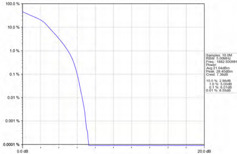
Band25_5MHz_16QAM_MCH_1882.5MHz_RB_25_0_NTNV
