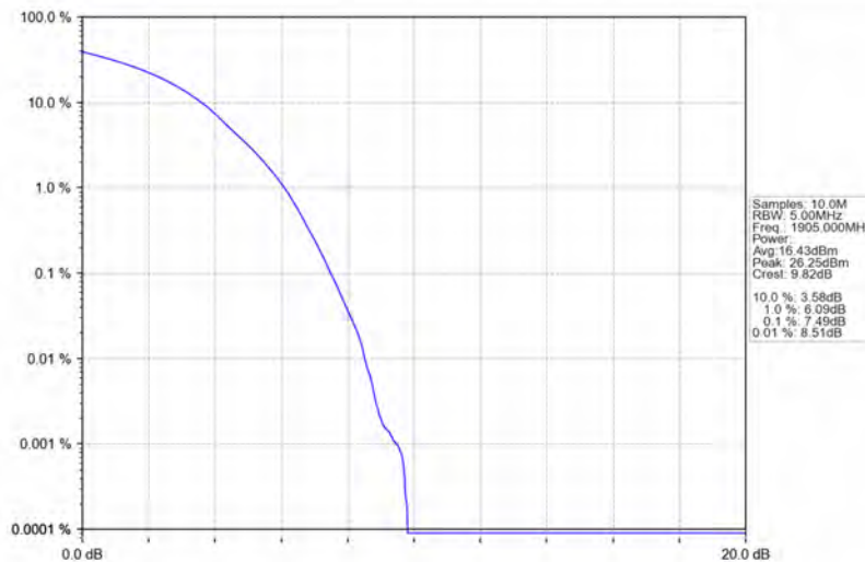
Band25_20MHz_16QAM_HCH_1905MHz_RB_100_0_NTNV
