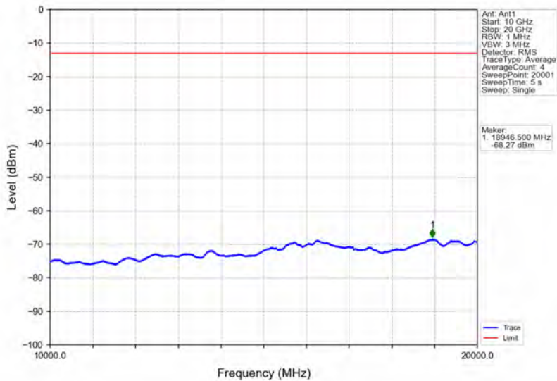
Band25_5MHz_64QAM_HCH_1912.5MHz_RB_1_0_NTNV
