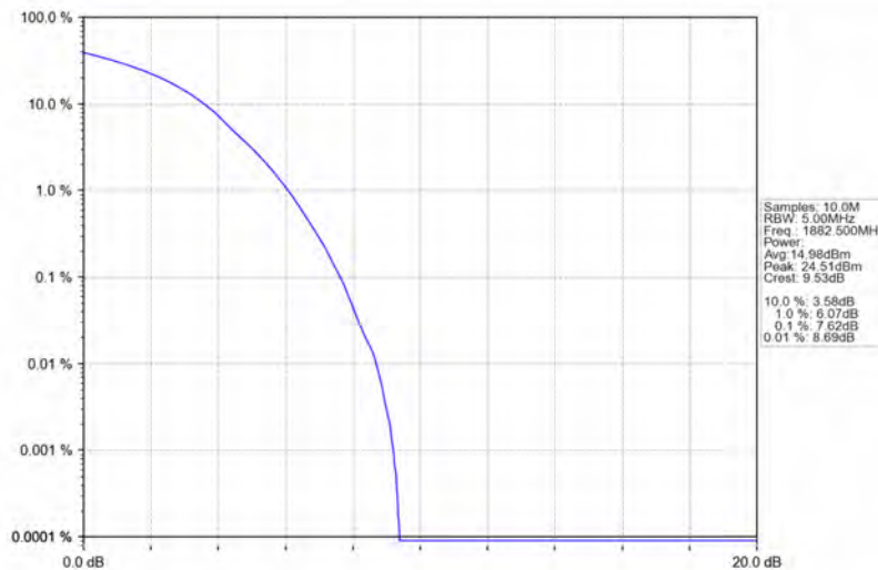
Band25_20MHz_64QAM_MCH_1882.5MHz_RB_100_0_NTNV
