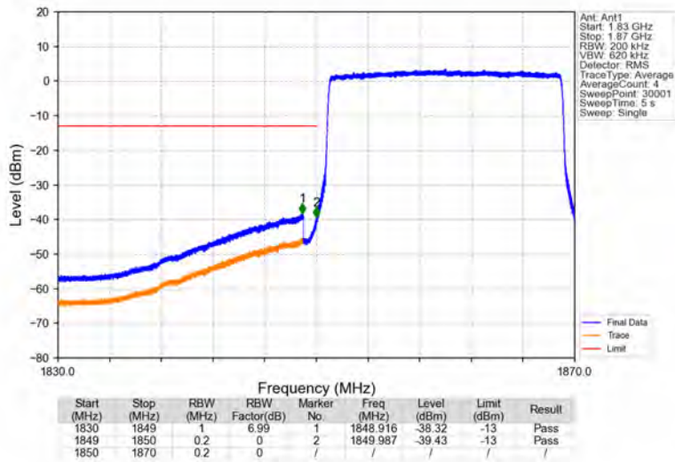
Band25_20MHz_16QAM_LCH_1860MHz_RB_100_0_NTNV
