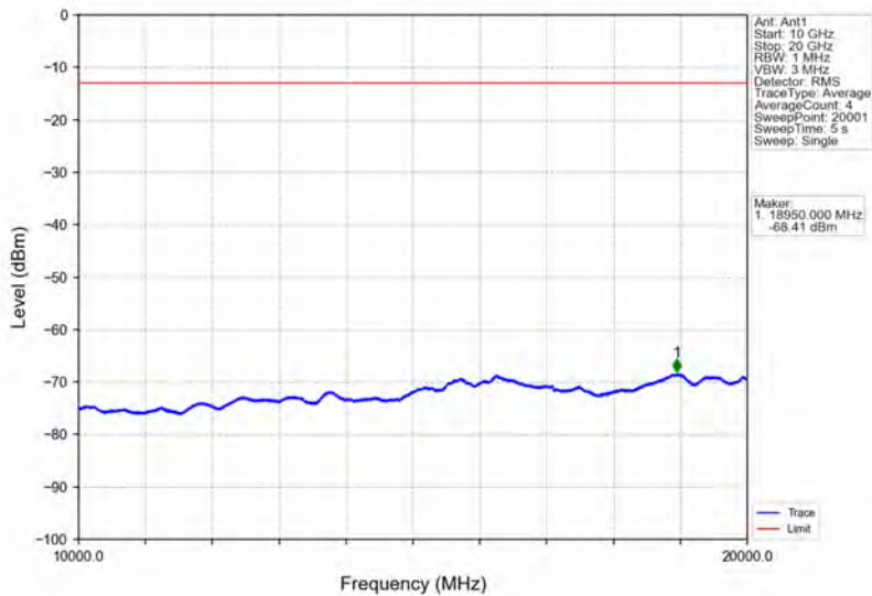
Band25_1.4MHz_16QAM_HCH_1914.3MHz_RB_1_0_NTNV
