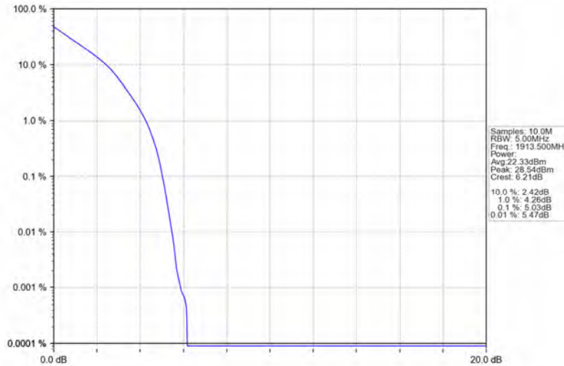
Band25_3MHz_QPSK_HCH_1913.5MHz_RB_15_0_NTNV
