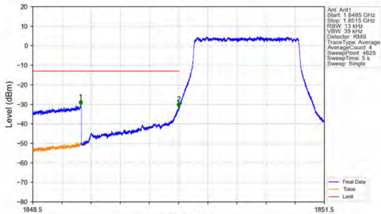
Band25_1.4MHz_QPSK_LCH_1850.7MHz_RB_6_0_NTNV
