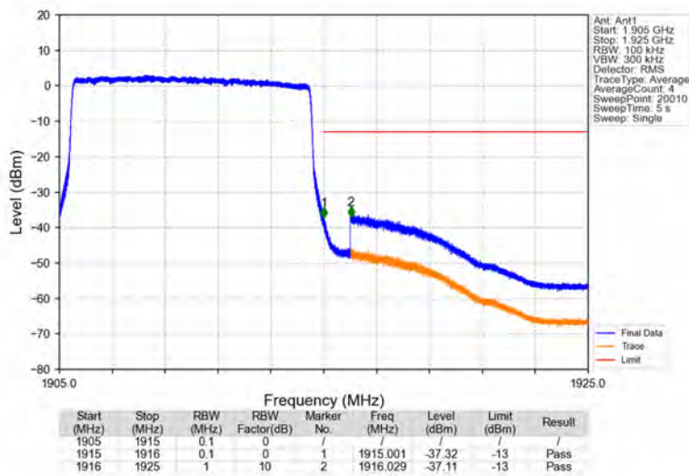
Band25_10MHz_64QAM_HCH_1910MHz_RB_50_0_NTNV
