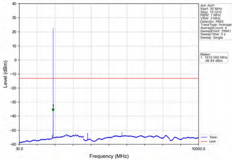
Band25_1.4MHz_QPSK_HCH_1914.3MHz_RB_1_0_NTNV
