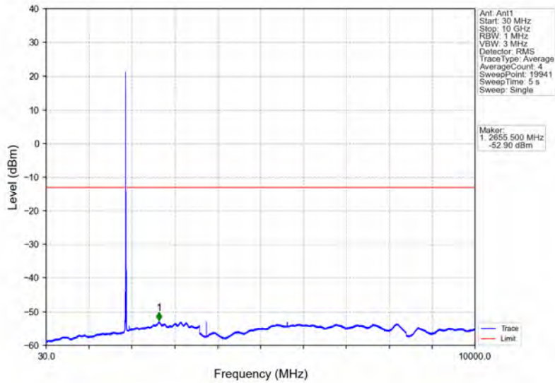
Band25_10MHz_64QAM_MCH_1882.5MHz_RB_1_0_NTNV
