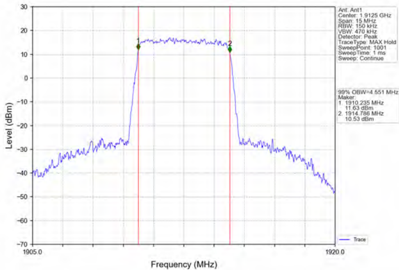
Band25_5MHz_16QAM_HCH_1912.5MHz_RB_25_0_NTNV
