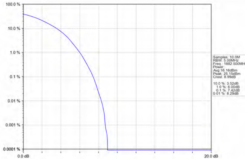
Band25_15MHz_64QAM_MCH_1882.5MHz_RB_75_0_NTNV
