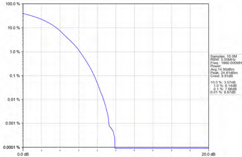
Band25_20MHz_64QAM_LCH_1860MHz_RB_100_0_NTNV
