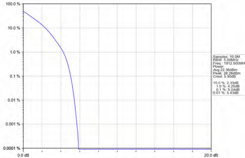
Band25_5MHz_QPSK_HCH_1912.5MHz_RB_25_0_NTNV
