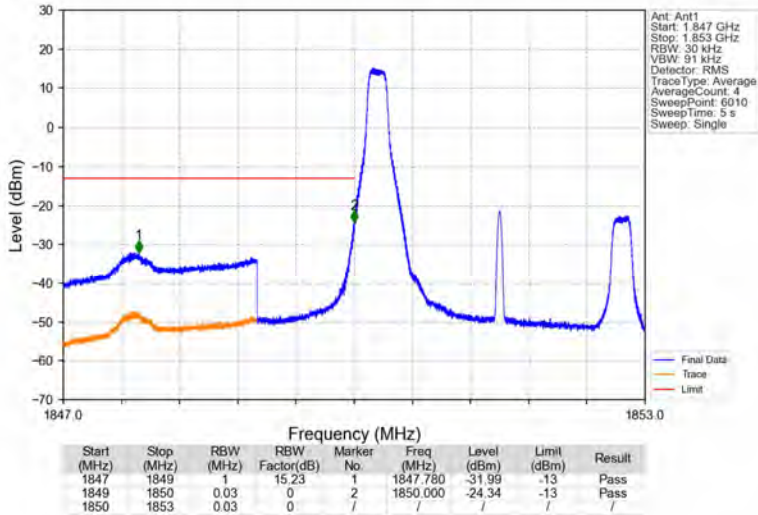
Band25_3MHz_64QAM_LCH_1851.5MHz_RB_1_0_NTNV
