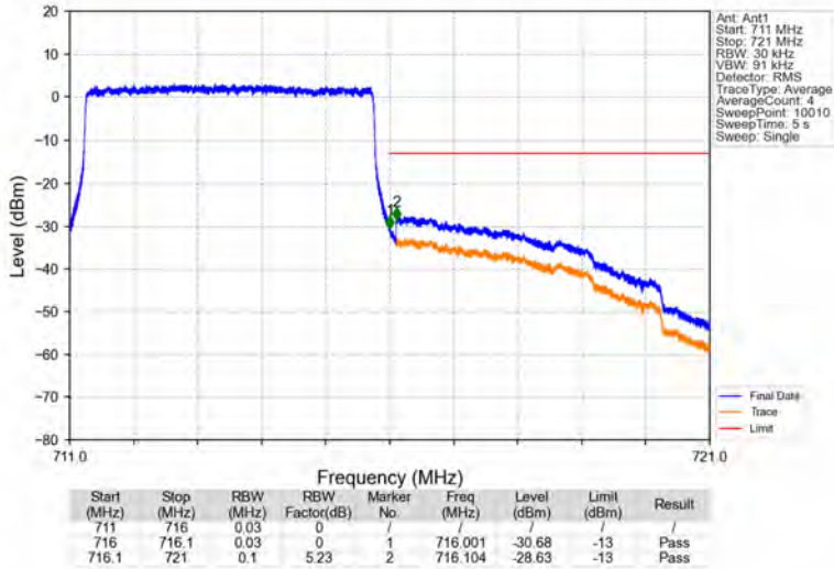
Band17_5MHz_QPSK_HCH_713.5MHz_RB_25_0_NTNV
