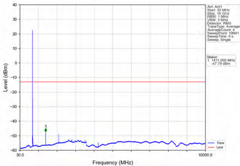
Band17_10MHz_64QAM_MCH_710MHz_RB_1_0_NTNV
