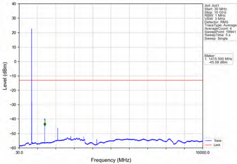
Band17_5MHz_16QAM_HCH_713.5MHz_RB_1_0_NTNV
