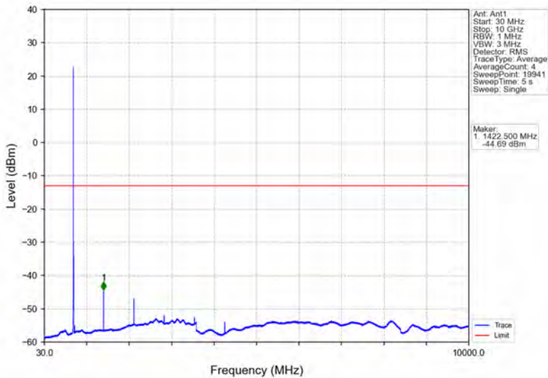
Band17_5MHz_16QAM_HCH_713.5MHz_RB_1_0_NTNV
