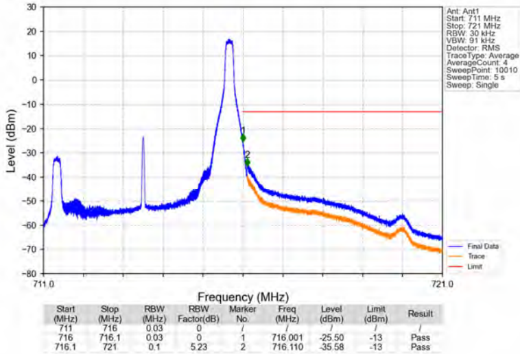
Band17_5MHz_16QAM_HCH_713.5MHz_RB_1_24_NTNV
