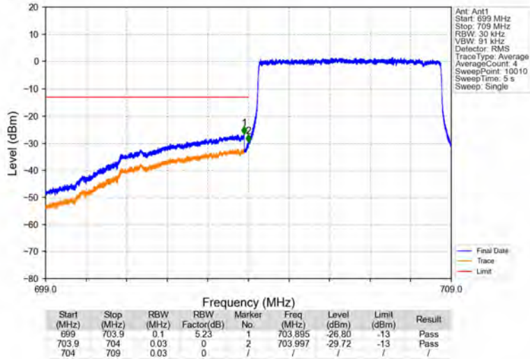
Band17_5MHz_64QAM_LCH_706.5MHz_RB_25_0_NTNV
