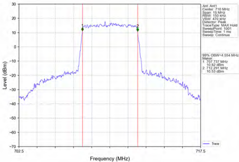
Band17_5MHz_64QAM_MCH_710MHz_RB_25_0_NTNV
