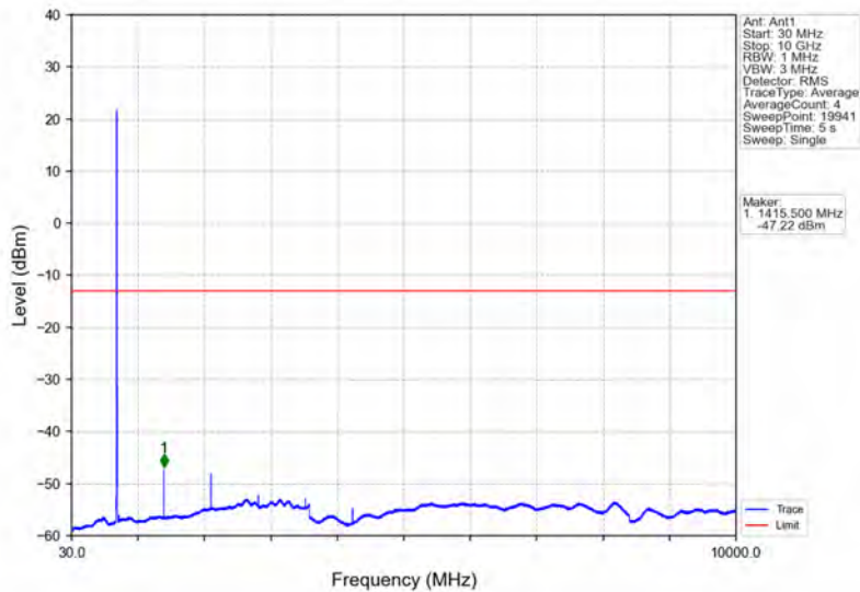
Band17_5MHz_64QAM_MCH_710MHz_RB_1_0_NTNV
