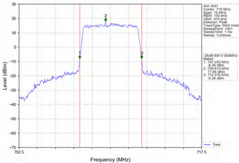
Band17_5MHz_64QAM_MCH_710MHz_RB_25_0_NTNV
