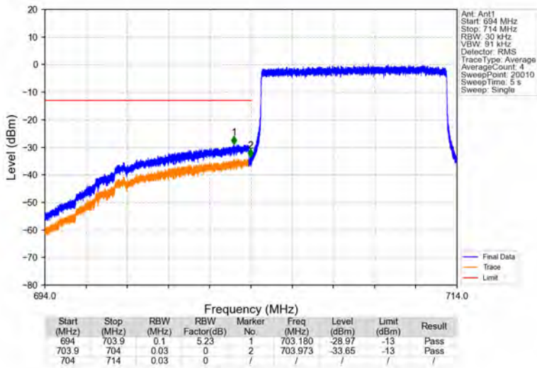
Band17_10MHz_16QAM_LCH_709MHz_RB_50_0_NTNV
