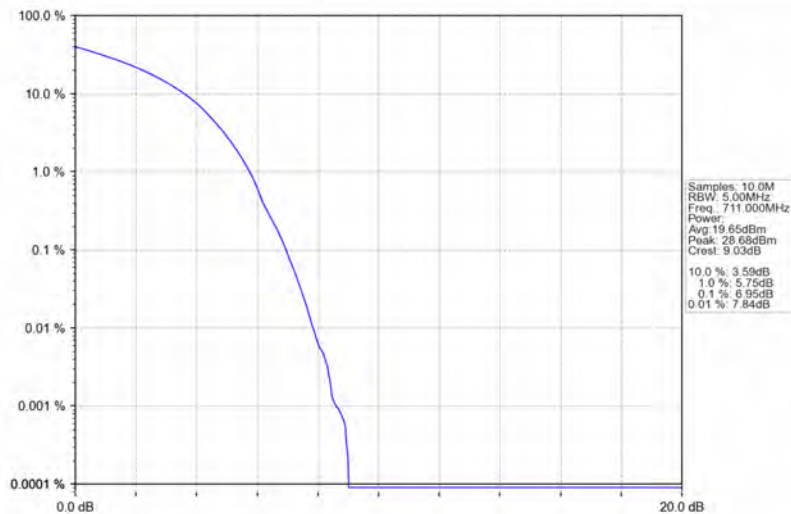
Band17_10MHz_16QAM_HCH_711MHz_RB_50_0_NTNV
