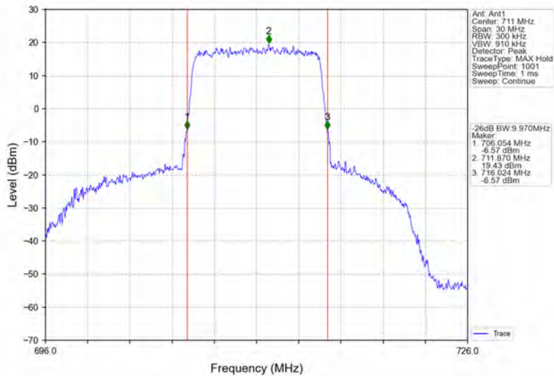
Band17_10MHz_QPSK_HCH_711MHz_RB_50_0_NTNV
