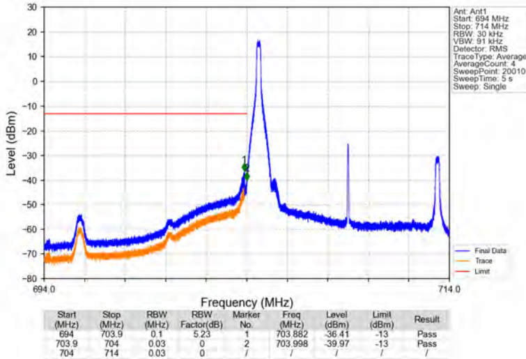
Band17_10MHz_64QAM_LCH_709MHz_RB_1_0_NTNV
