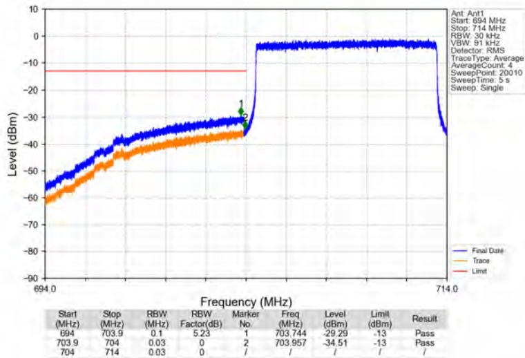
Band17_10MHz_64QAM_LCH_709MHz_RB_50_0_NTNV
