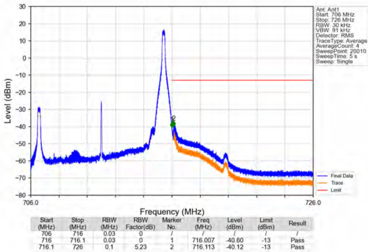
Band17_10MHz_64QAM_HCH_711MHz_RB_1_49_NTNV
