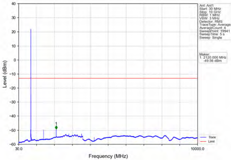
Band17_10MHz_64QAM_HCH_711MHz_RB_1_49_NTNV
