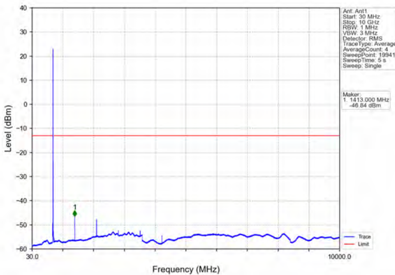
Band17_10MHz_16QAM_HCH_711MHz_RB_1_0_NTNV
