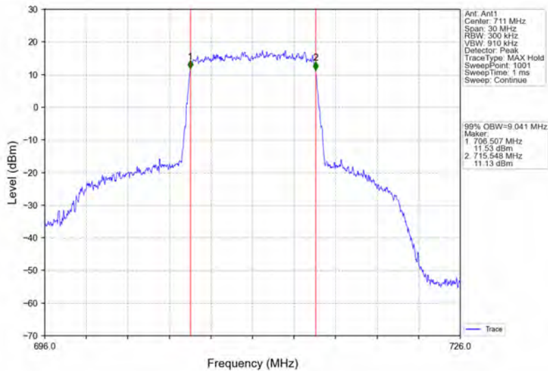
Band17_10MHz_64QAM_HCH_711MHz_RB_50_0_NTNV
