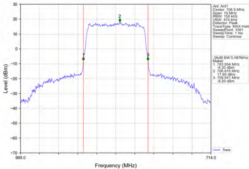
Band17_5MHz_16QAM_LCH_706.5MHz_RB_25_0_NTNV
