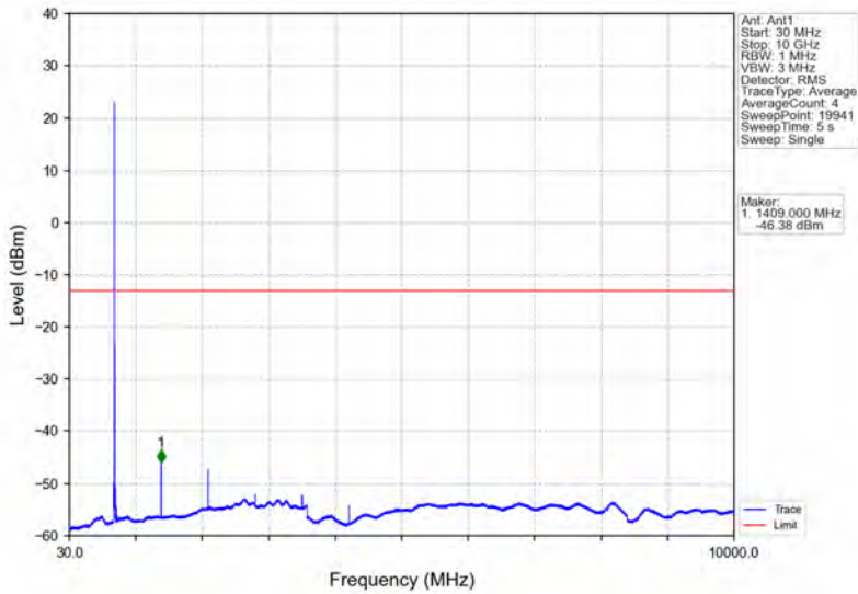
Band17_10MHz_16QAM_LCH_709MHz_RB_50_0_NTNV
