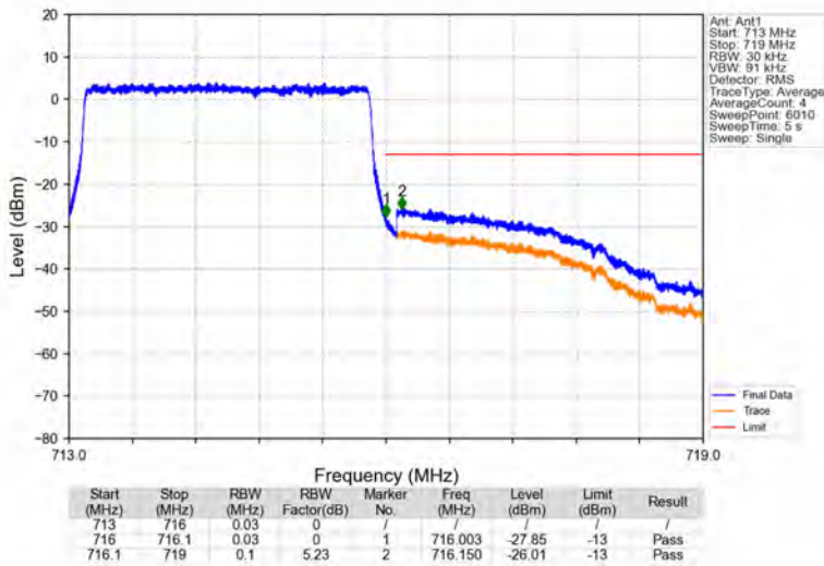
Band12_3MHz_16QAM_HCH_714.5MHz_RB_15_0_NTNV
