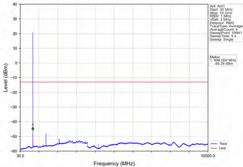
Band12_1.4MHz_64QAM_LCH_699.7MHz_RB_1_0_NTNV
