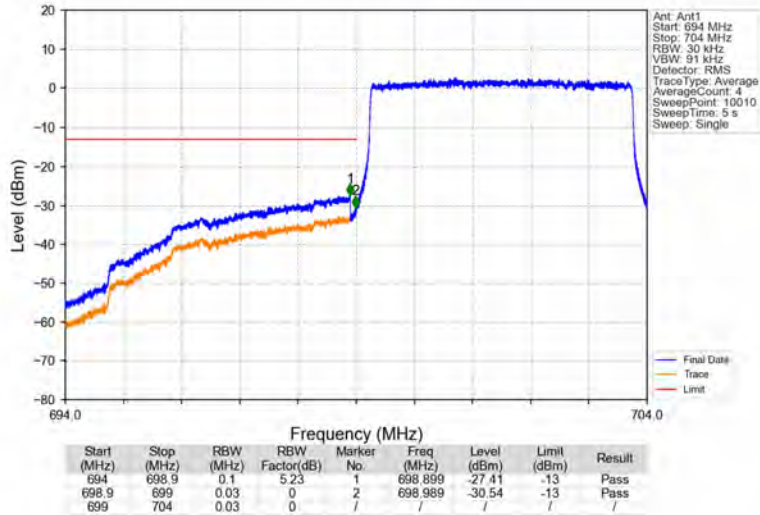
Band12_5MHz_QPSK_LCH_701.5MHz_RB_25_0_NTNV
