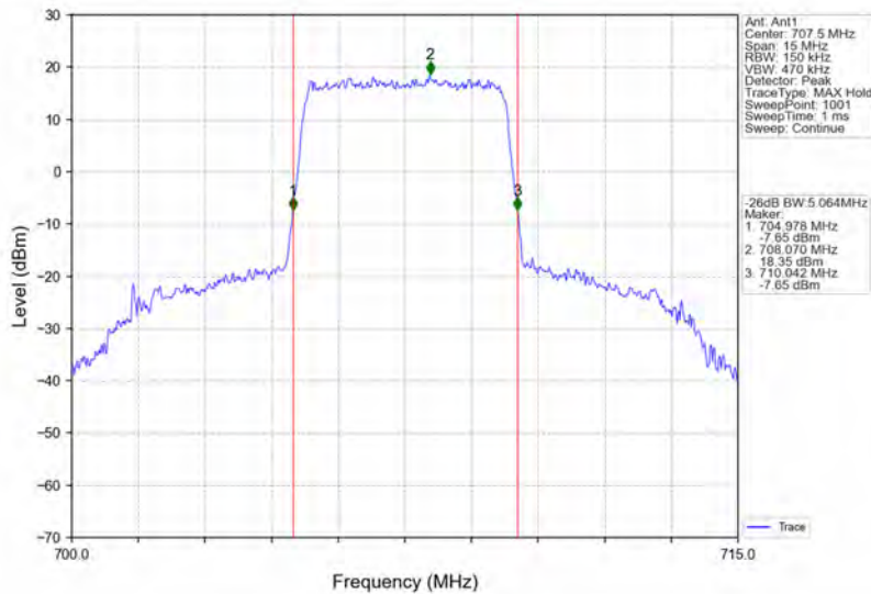
Band12_5MHz_QPSK_MCH_707.5MHz_RB_25_0_NTNV
