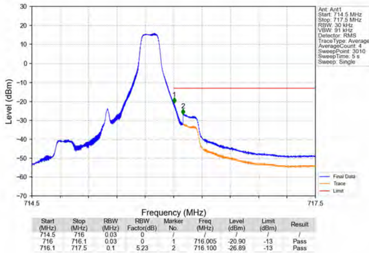
Band12_1.4MHz_16QAM_HCH_715.3MHz_RB_1_5_NTNV
