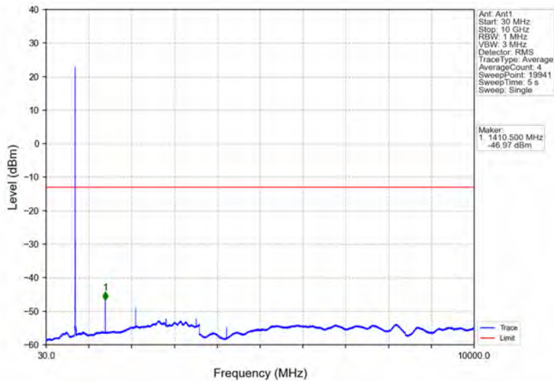
Band12_5MHz_QPSK_MCH_707.5MHz_RB_1_0_NTNV
