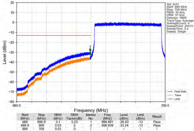
Band12_10MHz_QPSK_LCH_704MHz_RB_50_0_NTNV
