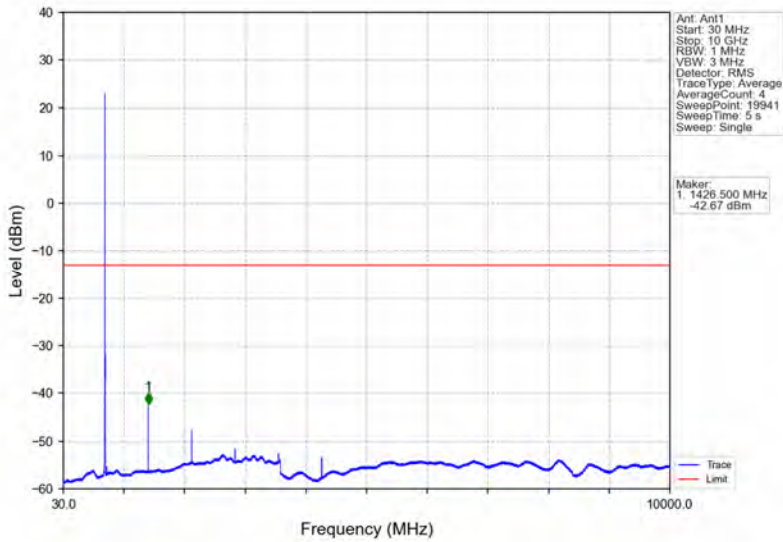
Band12_3MHz_QPSK_HCH_714.5MHz_RB_1_14_NTNV
