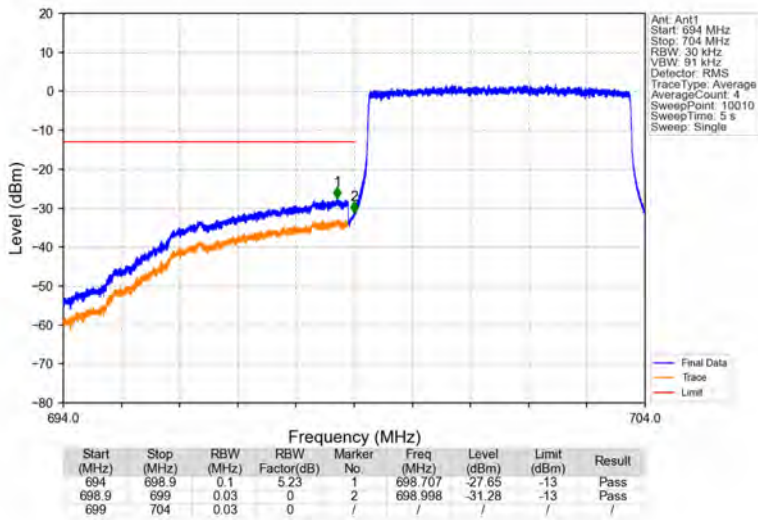
Band12_5MHz_16QAM_LCH_701.5MHz_RB_25_0_NTNV
