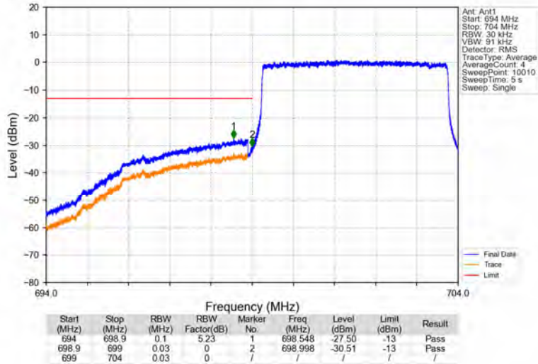
Band12_5MHz_64QAM_LCH_701.5MHz_RB_25_0_NTNV
