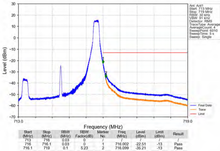
Band12_3MHz_16QAM_HCH_714.5MHz_RB_1_14_NTNV
