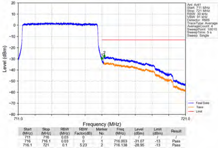
Band12_5MHz_QPSK_HCH_713.5MHz_RB_25_0_NTNV
