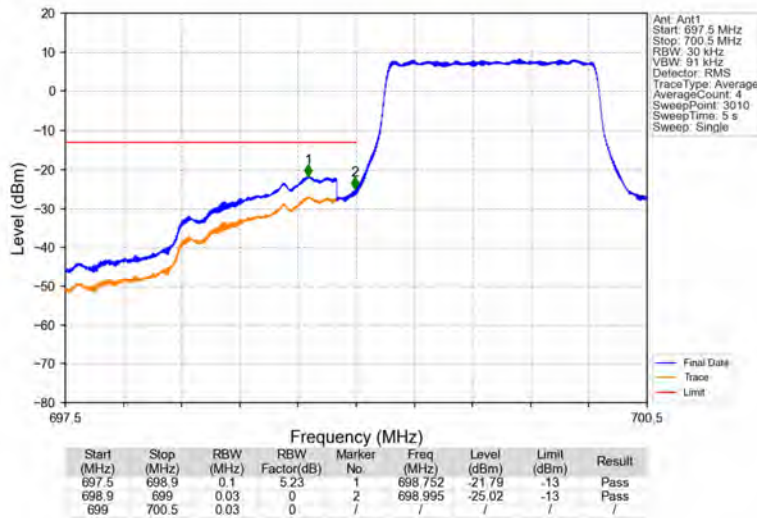
Band12_1.4MHz_QPSK_LCH_699.7MHz_RB_6_0_NTNV
