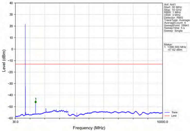
Band12_5MHz_16QAM_LCH_701.5MHz_RB_25_0_NTNV
