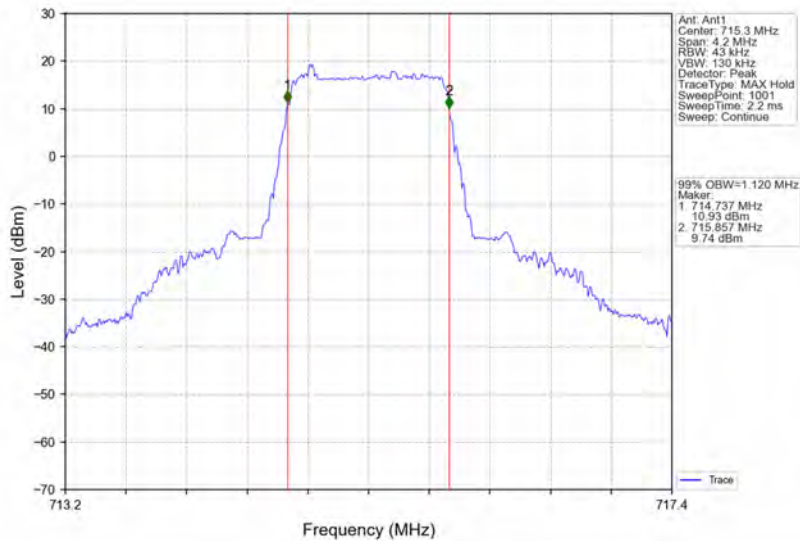
Band12_1.4MHz_16QAM_HCH_715.3MHz_RB_6_0_NTNV
