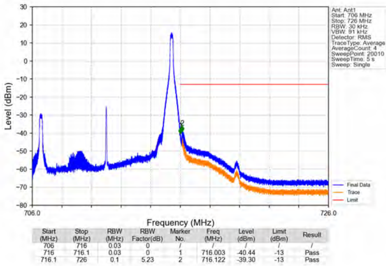
Band12_10MHz_64QAM_HCH_711MHz_RB_1_49_NTNV
