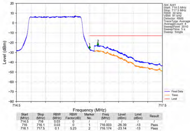
Band12_1.4MHz_16QAM_HCH_715.3MHz_RB_6_0_NTNV
