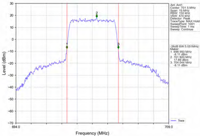
Band12_5MHz_16QAM_LCH_701.5MHz_RB_25_0_NTNV
