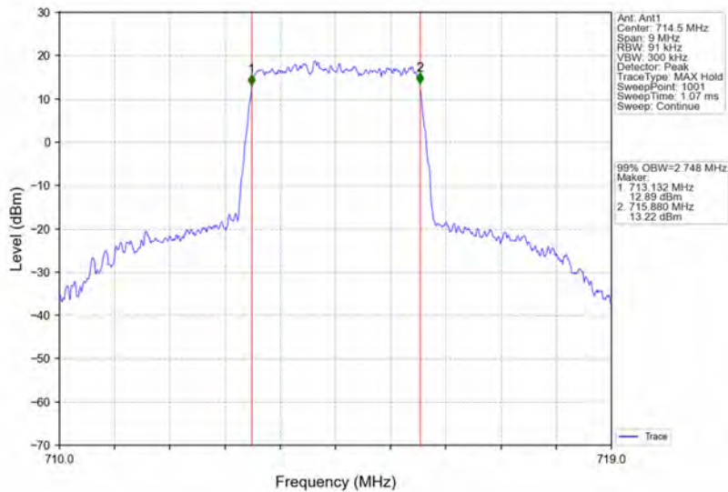
Band12_3MHz_QPSK_HCH_714.5MHz_RB_15_0_NTNV
