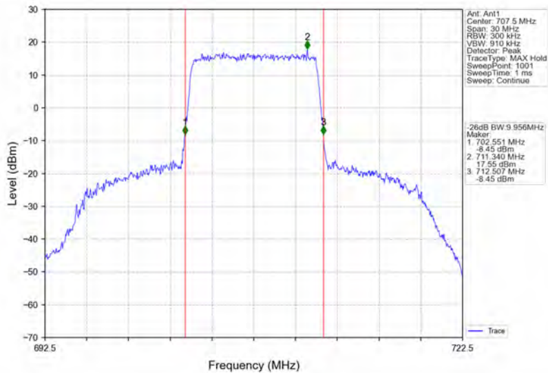
Band12_10MHz_16QAM_MCH_707.5MHz_RB_50_0_NTNV
