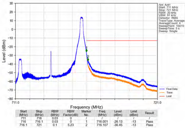
Band12_5MHz_64QAM_HCH_713.5MHz_RB_1_24_NTNV
