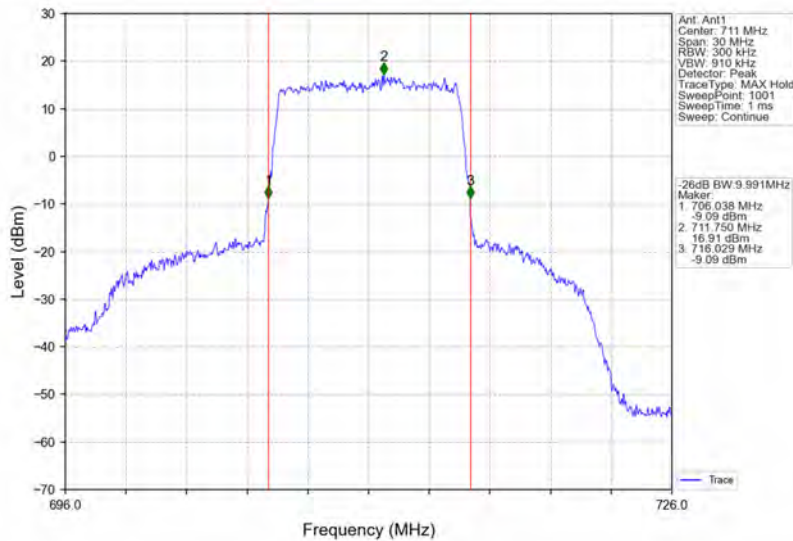
Band12_10MHz_64QAM_HCH_711MHz_RB_50_0_NTNV
