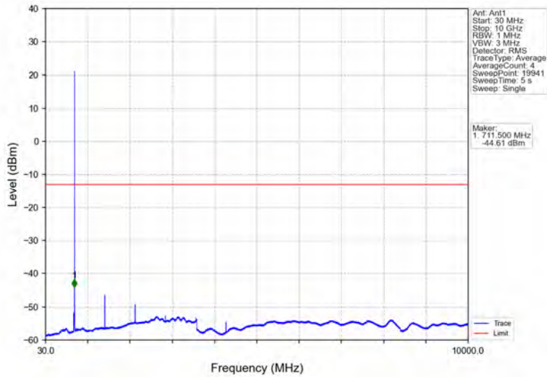
Band12_1.4MHz_64QAM_HCH_715.3MHz_RB_1_5_NTNV
