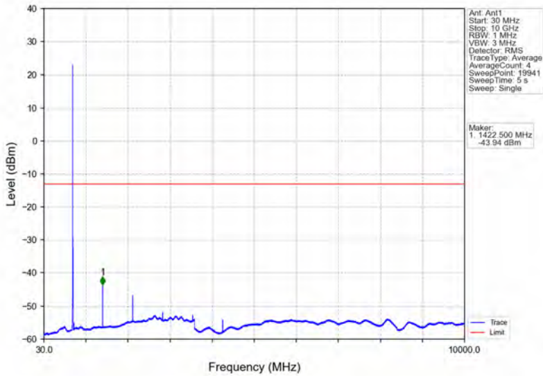
Band12_5MHz_QPSK_HCH_713.5MHz_RB_1_24_NTNV
