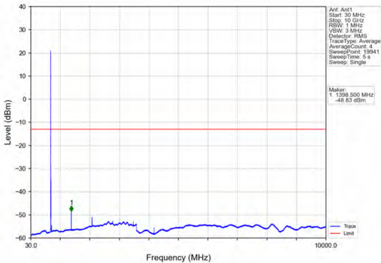
Band12_5MHz_64QAM_LCH_701.5MHz_RB_1_0_NTNV
