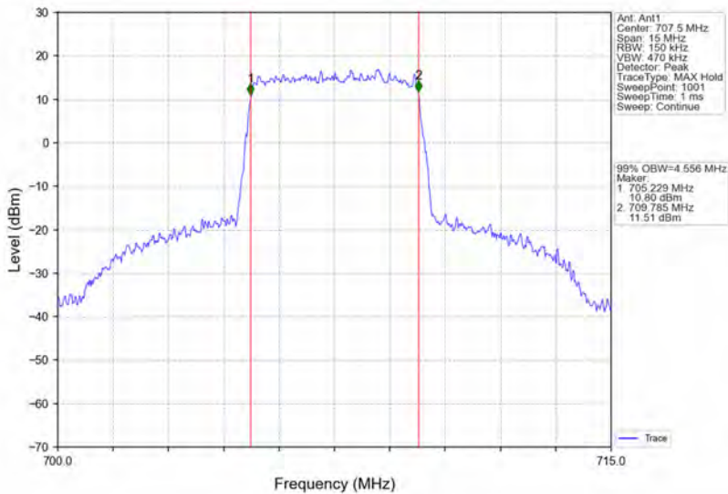
Band12_5MHz_64QAM_MCH_707.5MHz_RB_25_0_NTNV
