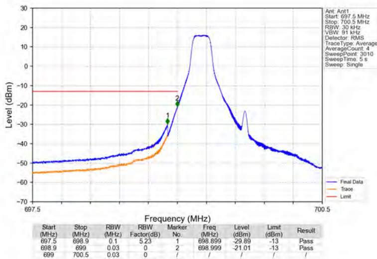
Band12_1.4MHz_16QAM_LCH_699.7MHz_RB_1_0_NTNV
