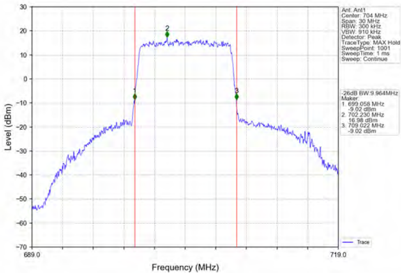
Band12_10MHz_64QAM_LCH_704MHz_RB_50_0_NTNV
