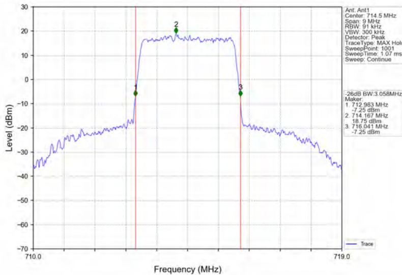
Band12_3MHz_QPSK_HCH_714.5MHz_RB_15_0_NTNV
