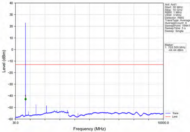
Band12_1.4MHz_16QAM_HCH_715.3MHz_RB_1_0_NTNV
