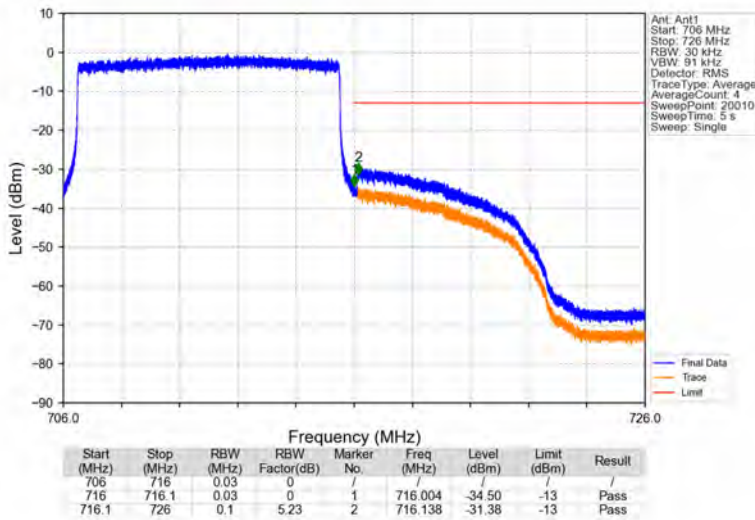
Band12_10MHz_16QAM_HCH_711MHz_RB_50_0_NTNV
