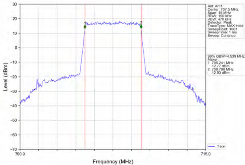
Band12_5MHz_QPSK_MCH_707.5MHz_RB_25_0_NTNV
