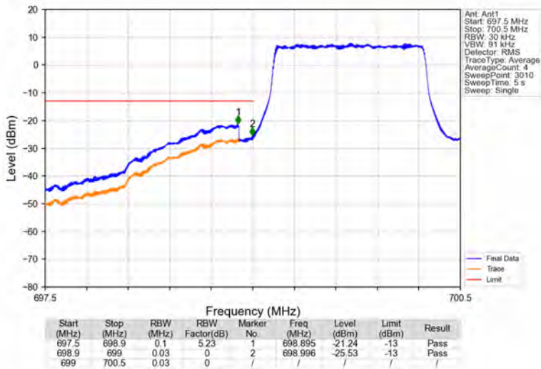
Band12_1.4MHz_16QAM_LCH_699.7MHz_RB_6_0_NTNV
