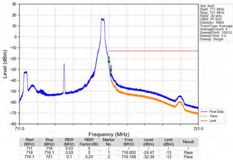
Band12_5MHz_QPSK_HCH_713.5MHz_RB_1_24_NTNV
