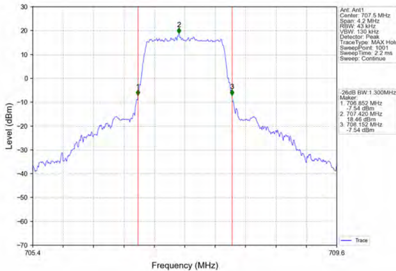
Band12_1.4MHz_64QAM_MCH_707.5MHz_RB_6_0_NTNV
