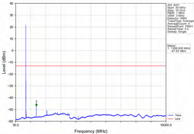
Band12_10MHz_64QAM_LCH_704MHz_RB_1_0_NTNV
