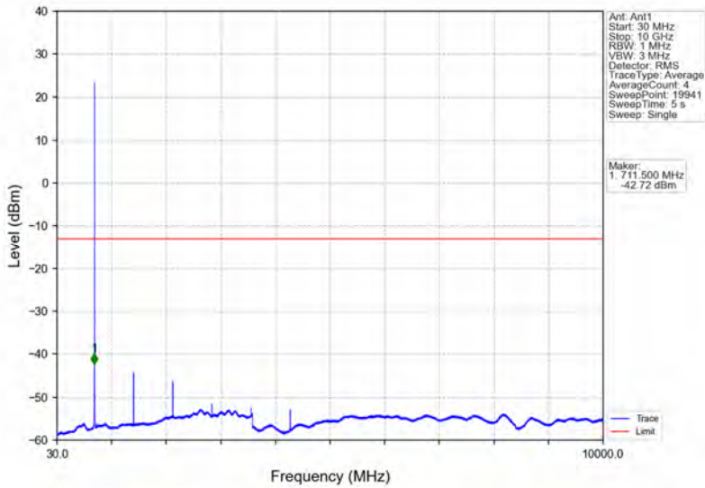
Band12_1.4MHz_QPSK_HCH_715.3MHz_RB_1_5_NTNV
