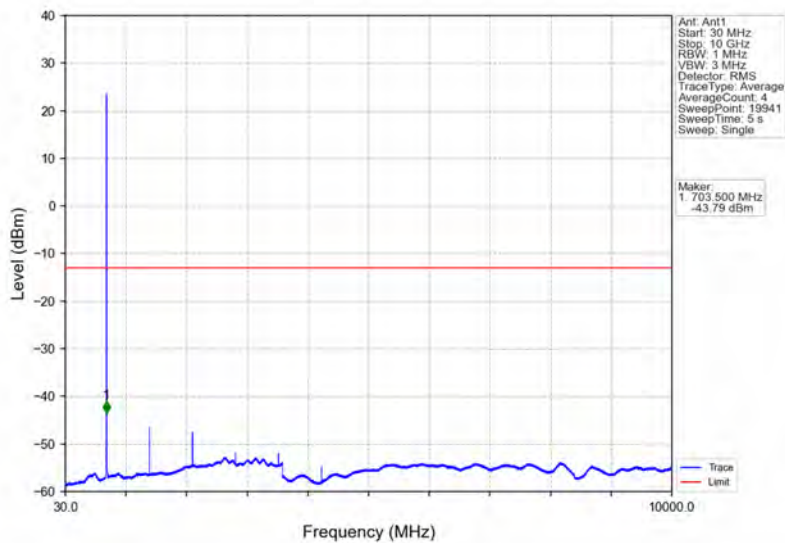
Band12_1.4MHz_QPSK_MCH_707.5MHz_RB_1_0_NTNV
