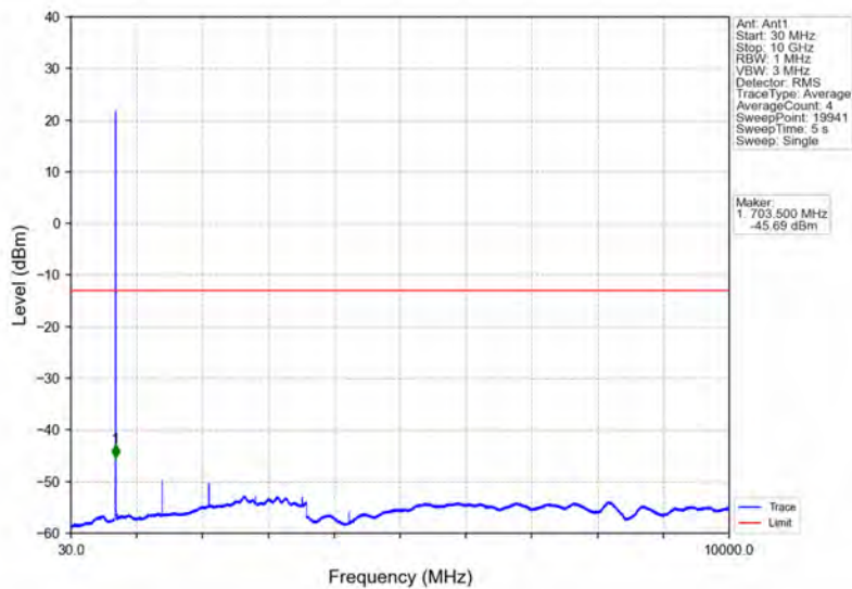
Band12_1.4MHz_64QAM_MCH_707.5MHz_RB_1_0_NTNV
