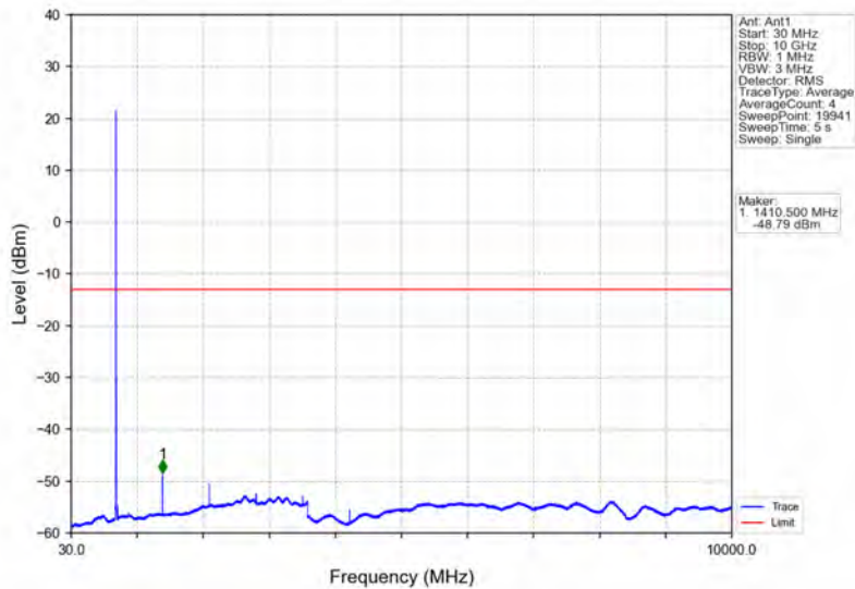
Band12_5MHz_64QAM_MCH_707.5MHz_RB_1_0_NTNV
