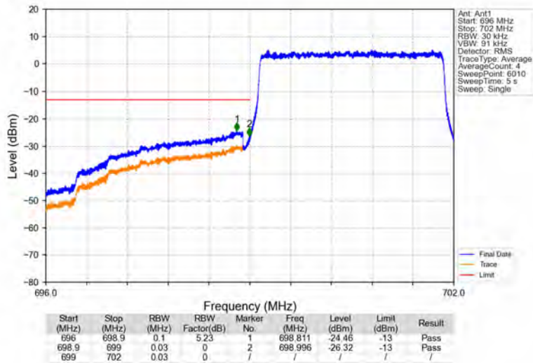
Band12_3MHz_QPSK_LCH_700.5MHz_RB_15_0_NTNV
