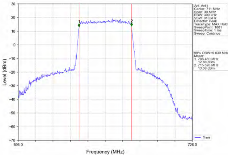
Band12_10MHz_QPSK_HCH_711MHz_RB_50_0_NTNV
