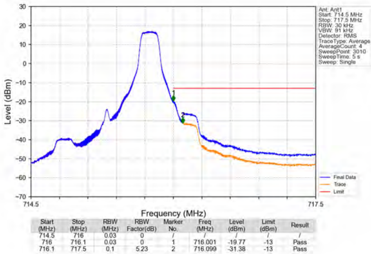
Band12_1.4MHz_QPSK_HCH_715.3MHz_RB_1_5_NTNV
