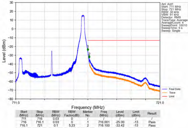
Band12_5MHz_16QAM_HCH_713.5MHz_RB_1_24_NTNV
