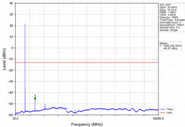
Band12_3MHz_64QAM_LCH_700.5MHz_RB_1_0_NTNV
