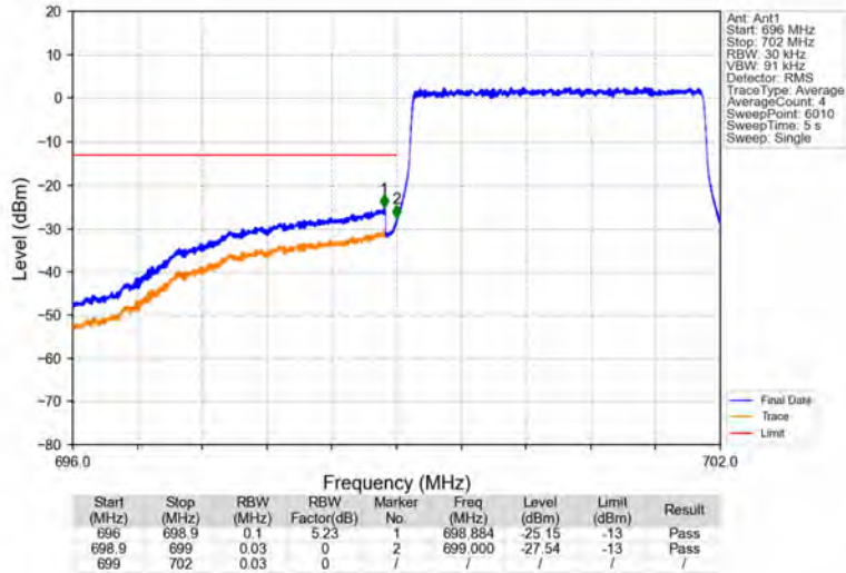
Band12_3MHz_64QAM_LCH_700.5MHz_RB_15_0_NTNV
