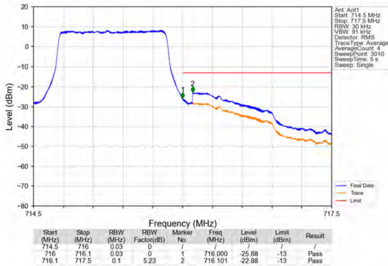
Band12_1.4MHz_QPSK_HCH_715.3MHz_RB_6_0_NTNV
