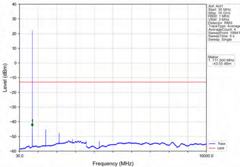
Band12_1.4MHz_16QAM_HCH_715.3MHz_RB_1_0_NTNV
