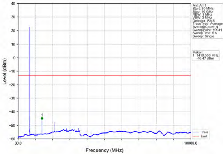
Band12_5MHz_16QAM_HCH_713.5MHz_RB_1_0_NTNV
