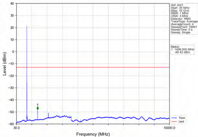
Band12_10MHz_64QAM_MCH_707.5MHz_RB_1_0_NTNV
