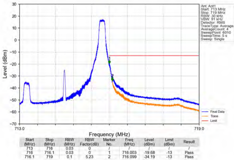
Band12_3MHz_QPSK_HCH_714.5MHz_RB_1_14_NTNV
