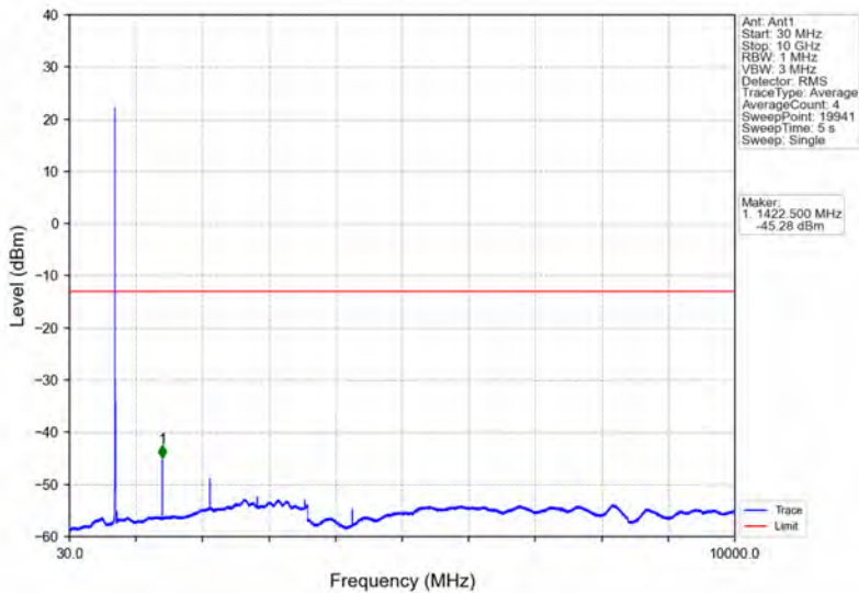
Band12_5MHz_16QAM_HCH_713.5MHz_RB_1_0_NTNV
