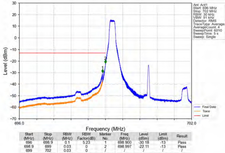
Band12_3MHz_64QAM_LCH_700.5MHz_RB_1_0_NTNV
