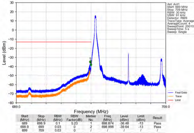
Band12_10MHz_64QAM_LCH_704MHz_RB_1_0_NTNV
