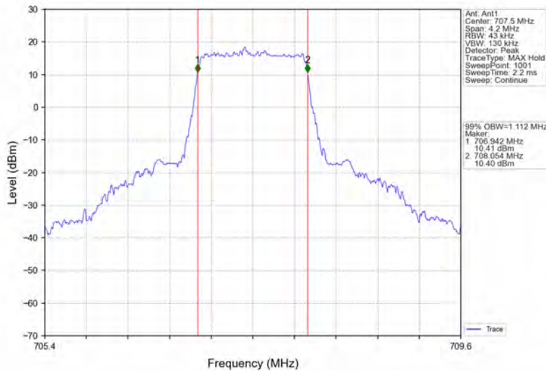
Band12_1.4MHz_64QAM_MCH_707.5MHz_RB_6_0_NTNV
