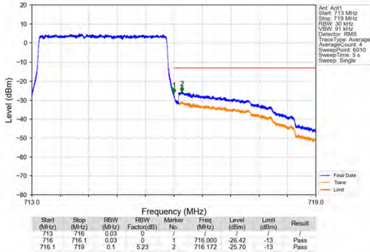
Band12_3MHz_QPSK_HCH_714.5MHz_RB_15_0_NTNV
