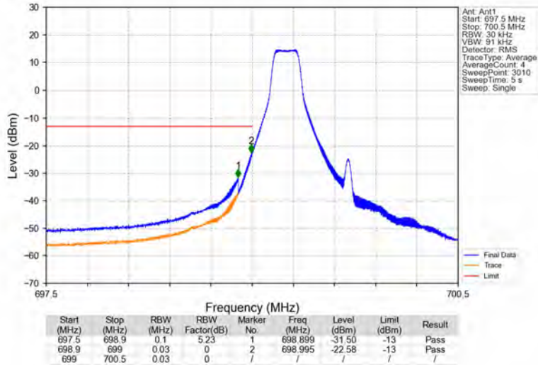
Band12_1.4MHz_64QAM_LCH_699.7MHz_RB_1_0_NTNV
