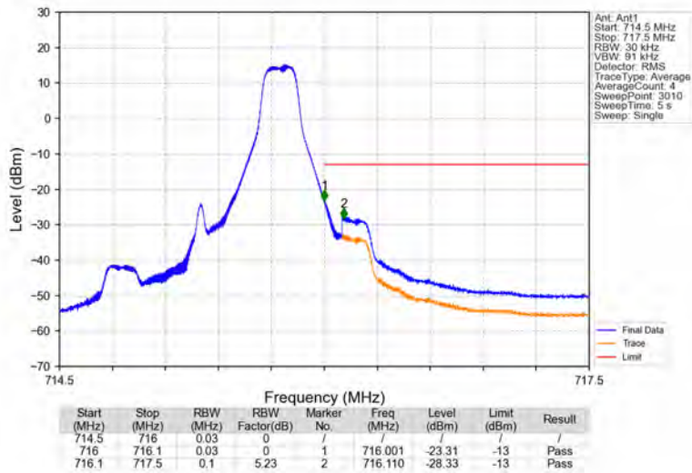
Band12_1.4MHz_64QAM_HCH_715.3MHz_RB_1_5_NTNV
