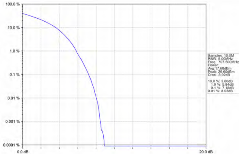
Band12_10MHz_64QAM_MCH_707.5MHz_RB_50_0_NTNV
