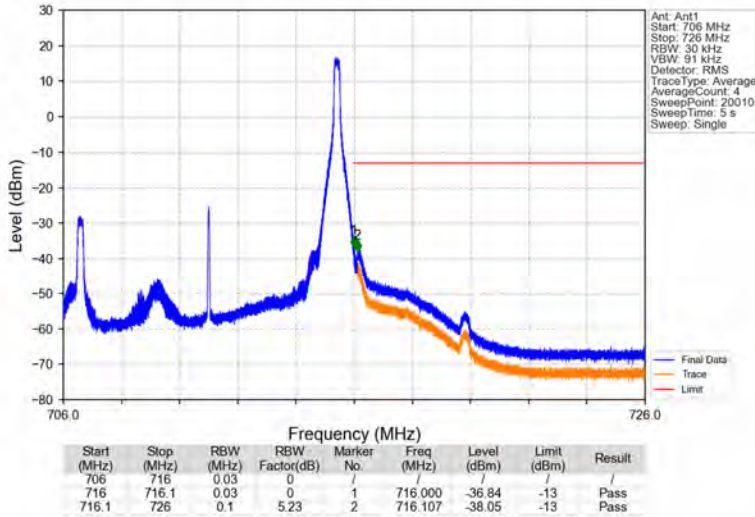
Band12_10MHz_16QAM_HCH_711MHz_RB_1_49_NTNV
