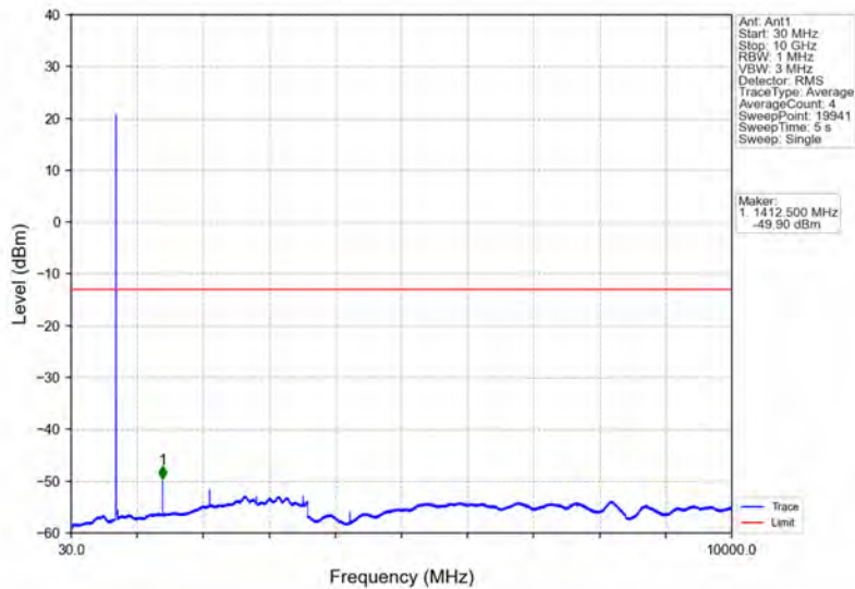
Band12_3MHz_64QAM_MCH_707.5MHz_RB_1_0_NTNV
