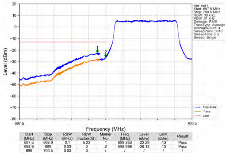
Band12_1.4MHz_64QAM_LCH_699.7MHz_RB_6_0_NTNV
