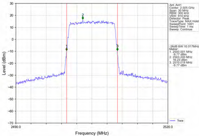
Band7_10MHz_64QAM_LCH_2505MHz_RB_50_0_NTNV
