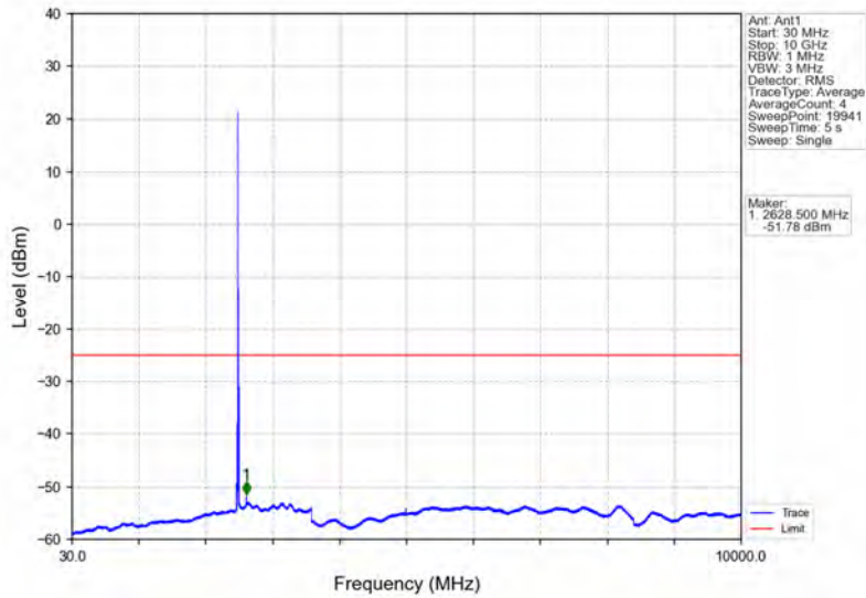
Band7_10MHz_16QAM_LCH_2505MHz_RB_1_0_NTNV
