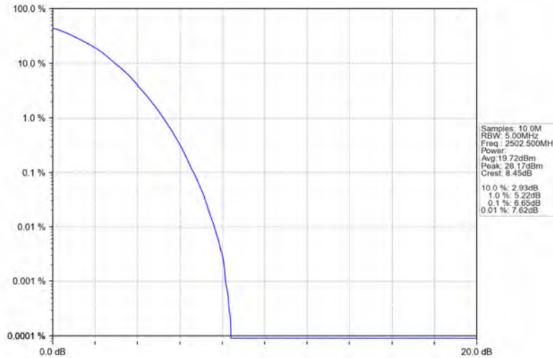
Band7_5MHz_64QAM_LCH_2502.5MHz_RB_25_0_NTNV
