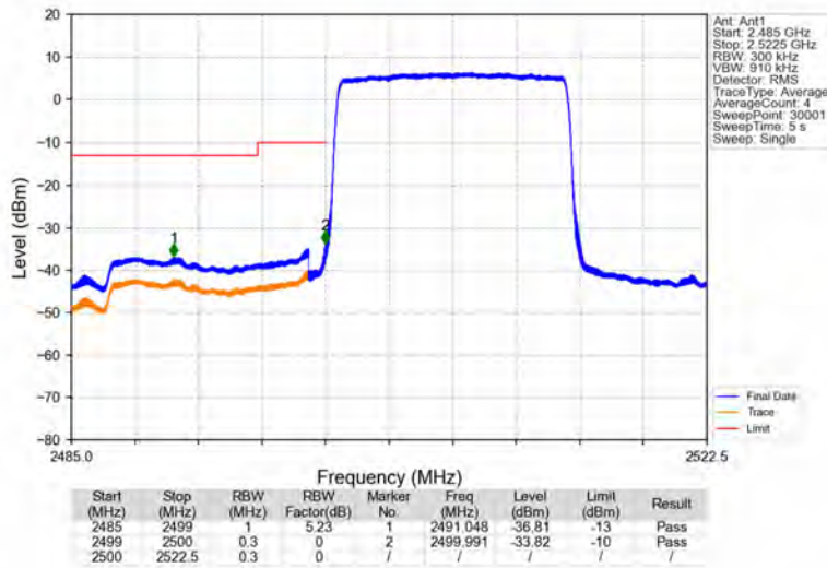
Band7_15MHz_QPSK_LCH_2507.5MHz_RB_75_0_NTNV
