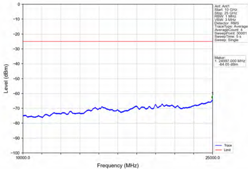
Band7_5MHz_64QAM_HCH_2567.5MHz_RB_1_0_NTNV
