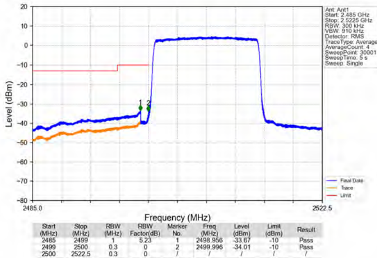
Band7_15MHz_64QAM_LCH_2507.5MHz_RB_75_0_NTNV
