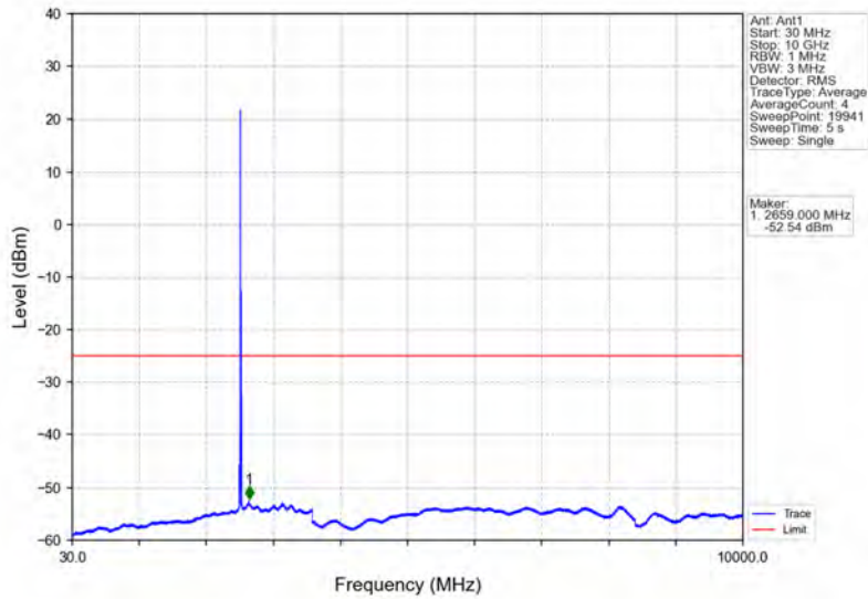
Band7_10MHz_16QAM_MCH_2535MHz_RB_1_0_NTNV
