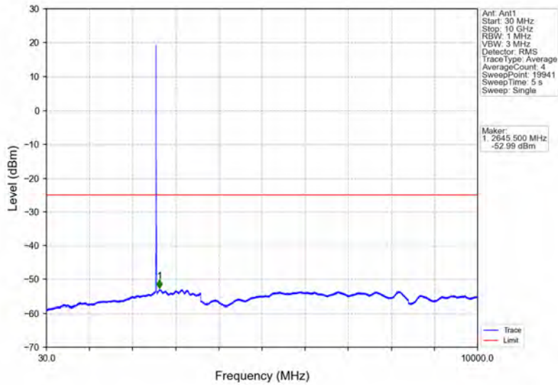
Band7_5MHz_64QAM_HCH_2567.5MHz_RB_1_0_NTNV
