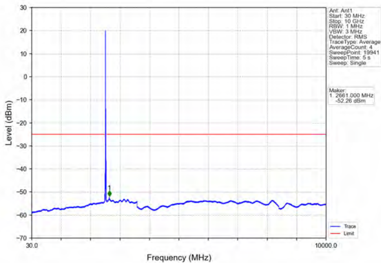
Band7_15MHz_64QAM_MCH_2535MHz_RB_1_0_NTNV
