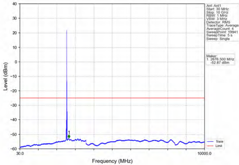
Band7_15MHz_QPSK_HCH_2562.5MHz_RB_1_0_NTNV
