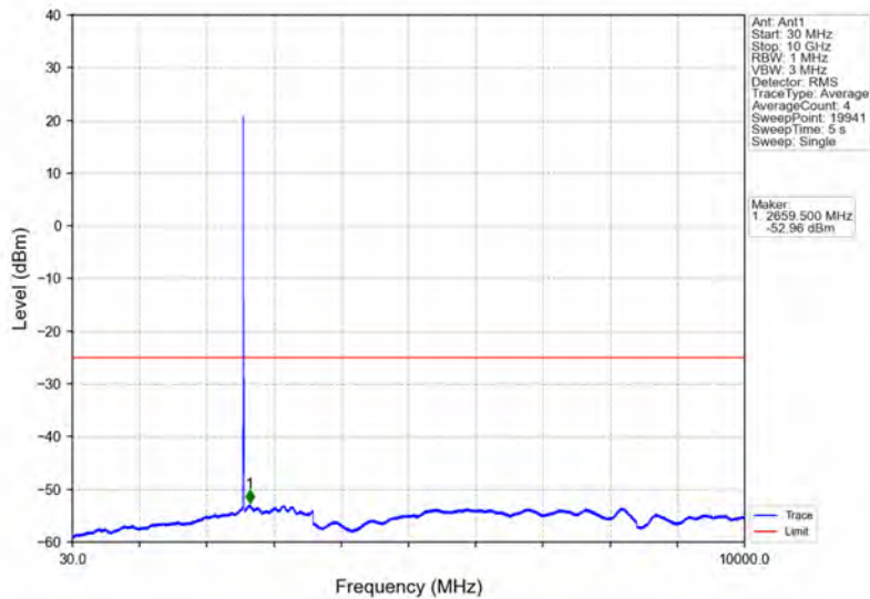
Band7_5MHz_16QAM_HCH_2567.5MHz_RB_1_0_NTNV
