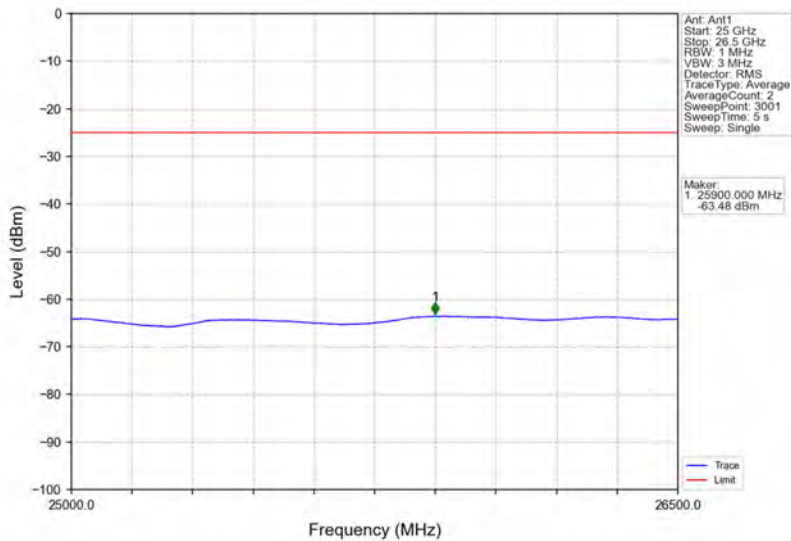
Band7_15MHz_QPSK_MCH_2535MHz_RB_1_0_NTNV
