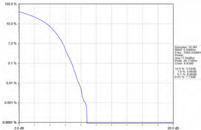
Band7_10MHz_16QAM_HCH_2565MHz_RB_50_0_NTNV
