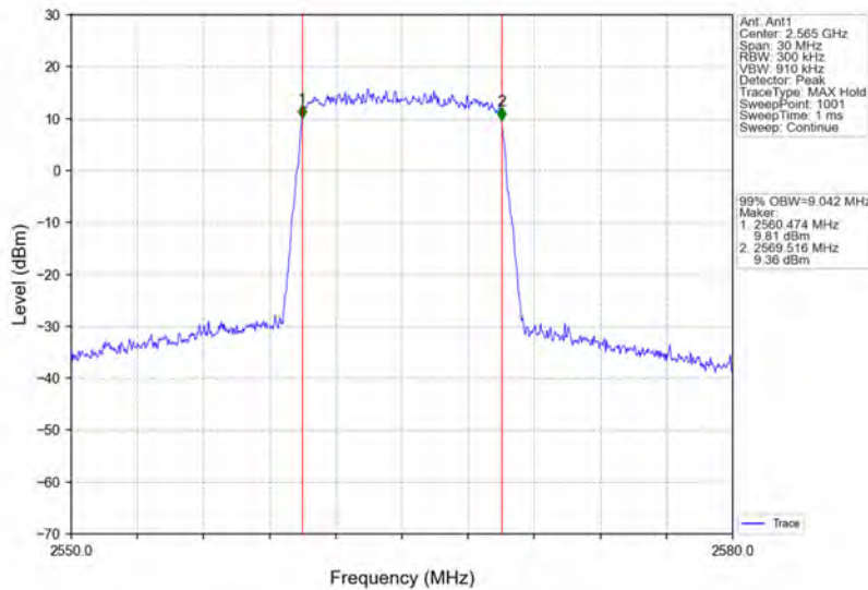
Band7_10MHz_64QAM_HCH_2565MHz_RB_50_0_NTNV
