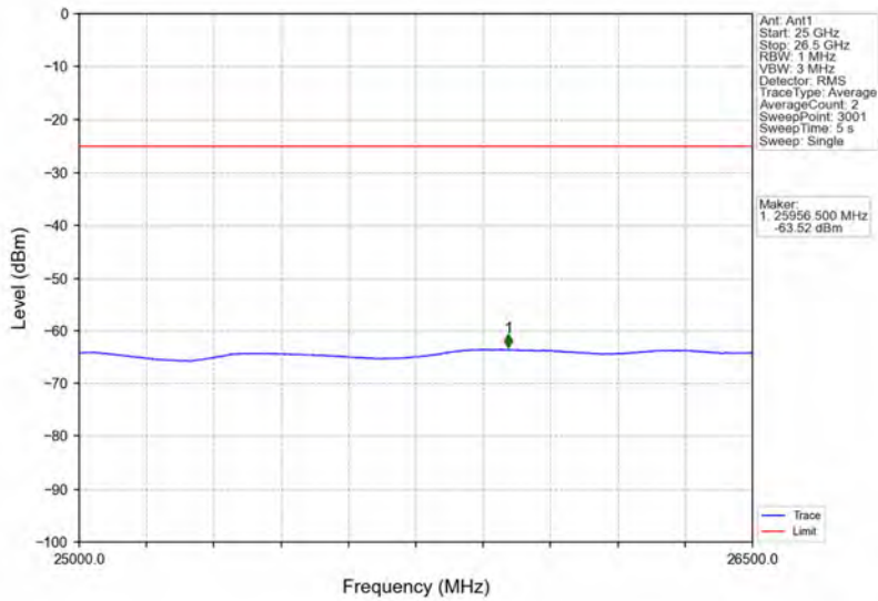
Band7_5MHz_64QAM_HCH_2567.5MHz_RB_1_24_NTNV
