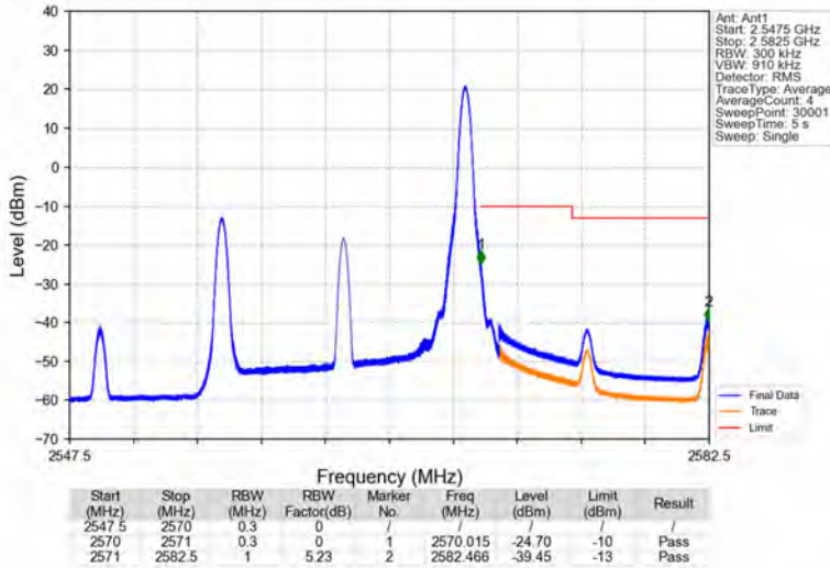
Band7_15MHz_16QAM_HCH_2562.5MHz_RB_1_74_NTNV
