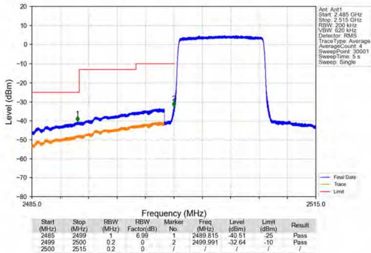
Band7_10MHz_64QAM_LCH_2505MHz_RB_50_0_NTNV
