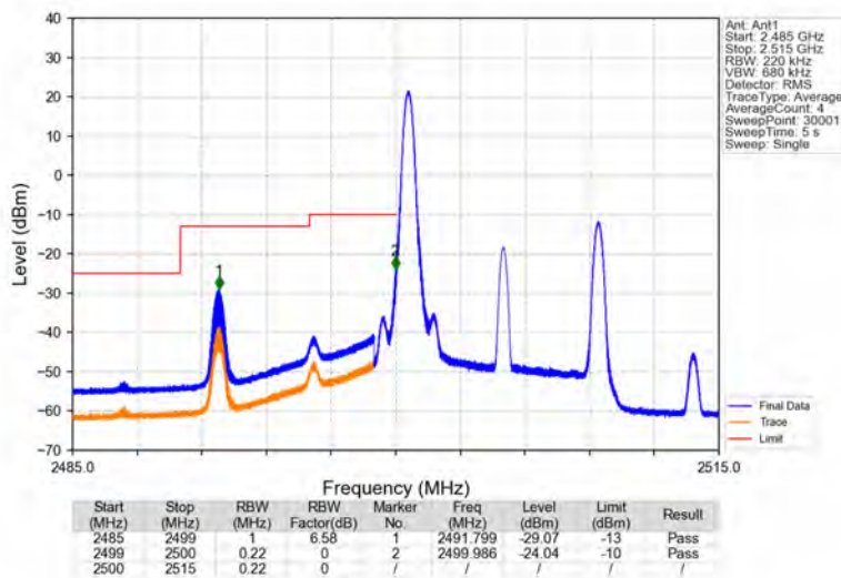
Band7_10MHz_16QAM_LCH_2505MHz_RB_1_0_NTNV
