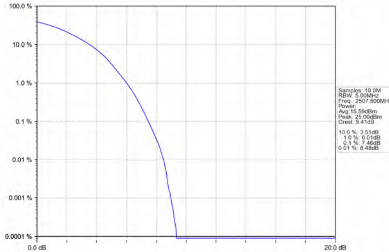
Band7_15MHz_64QAM_LCH_2507.5MHz_RB_75_0_NTNV
