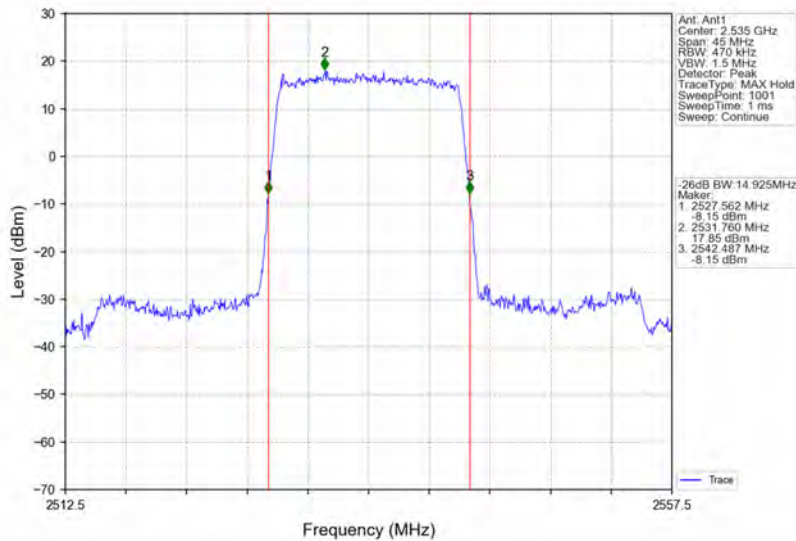
Band7_15MHz_QPSK_MCH_2535MHz_RB_75_0_NTNV
