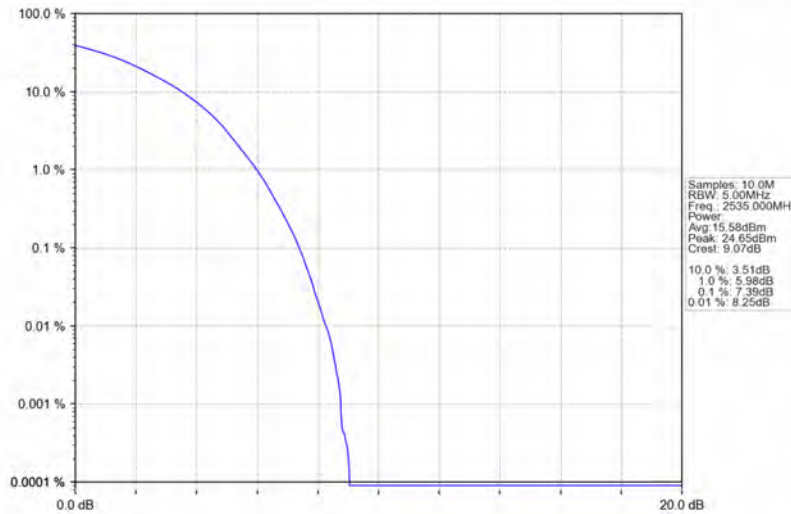
Band7_15MHz_64QAM_MCH_2535MHz_RB_75_0_NTNV
