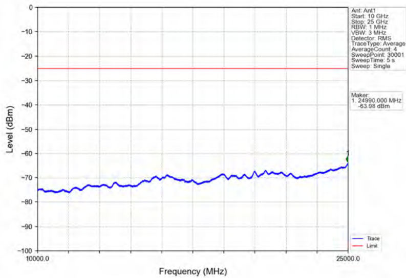
Band7_15MHz_64QAM_LCH_2507.5MHz_RB_1_0_NTNV
