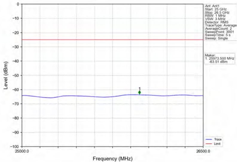
Band7_5MHz_16QAM_HCH_2567.5MHz_RB_1_0_NTNV
