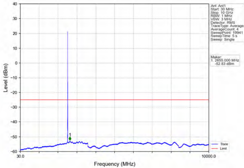
Band7_5MHz_16QAM_MCH_2535MHz_RB_1_0_NTNV
