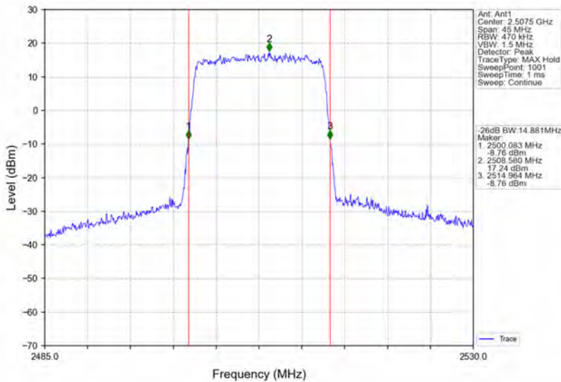
Band7_15MHz_16QAM_LCH_2507.5MHz_RB_75_0_NTNV
