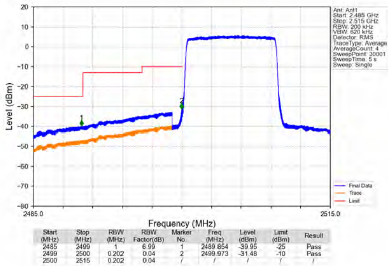
Band7_10MHz_16QAM_LCH_2505MHz_RB_50_0_NTNV
