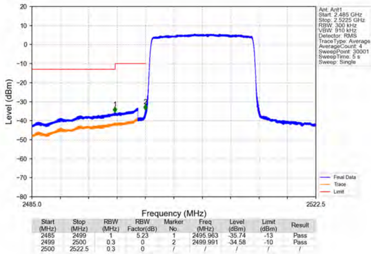
Band7_15MHz_16QAM_LCH_2507.5MHz_RB_75_0_NTNV
