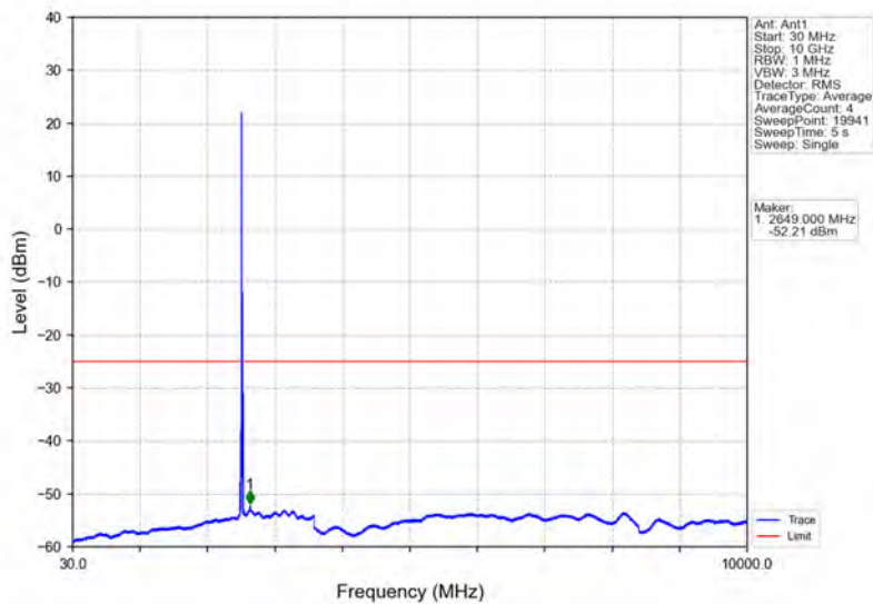
Band7_15MHz_QPSK_MCH_2535MHz_RB_1_0_NTNV
