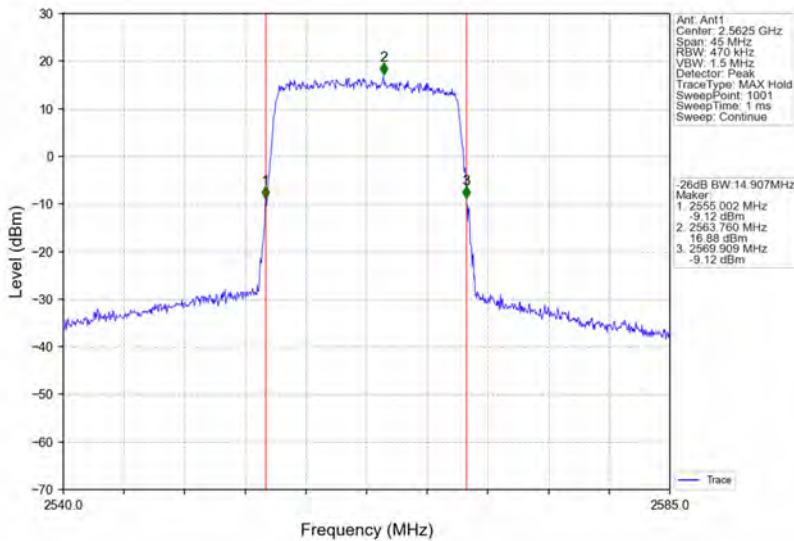
Band7_15MHz_16QAM_HCH_2562.5MHz_RB_75_0_NTNV
