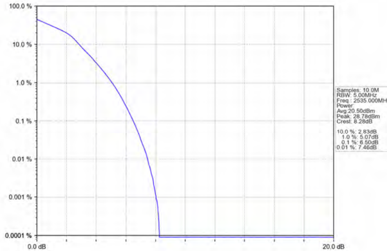
Band7_5MHz_16QAM_MCH_2535MHz_RB_25_0_NTNV
