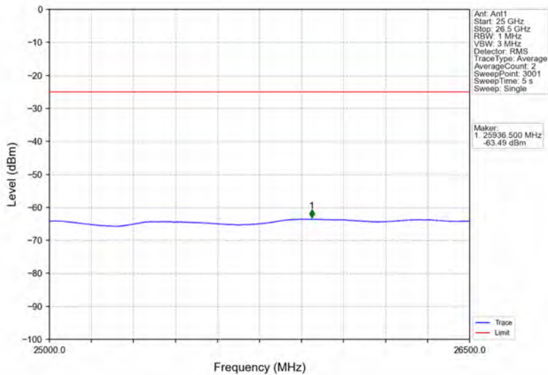
Band7_5MHz_64QAM_MCH_2535MHz_RB_1_0_NTNV
