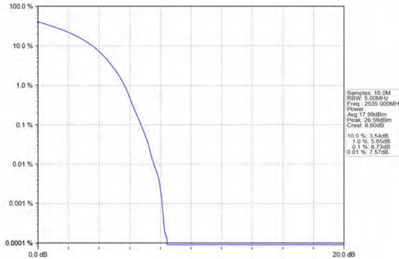
Band7_10MHz_16QAM_MCH_2535MHz_RB_50_0_NTNV
