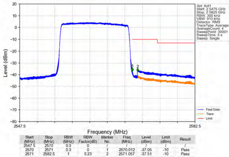
Band7_15MHz_64QAM_HCH_2562.5MHz_RB_75_0_NTNV
