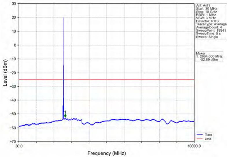
Band7_15MHz_64QAM_HCH_2562.5MHz_RB_1_0_NTNV
