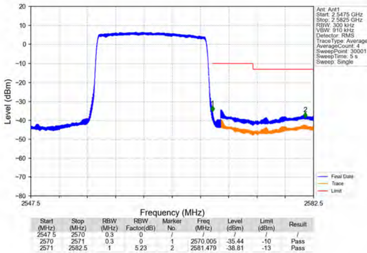
Band7_15MHz_QPSK_HCH_2562.5MHz_RB_75_0_NTNV
