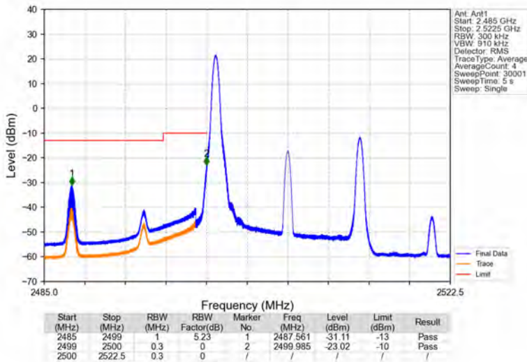
Band7_15MHz_16QAM_LCH_2507.5MHz_RB_1_0_NTNV
