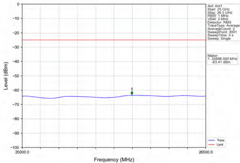
Band7_15MHz_QPSK_LCH_2507.5MHz_RB_1_0_NTNV
