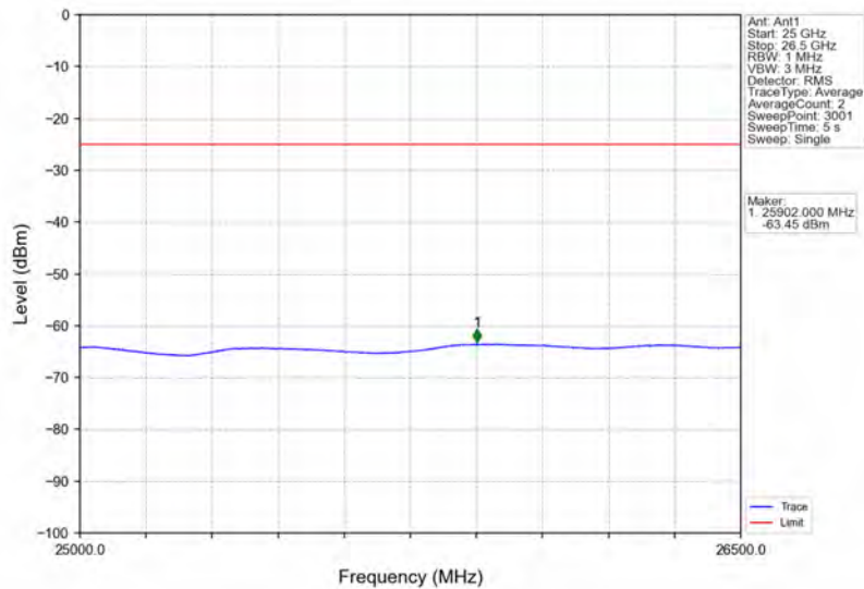
Band7_15MHz_64QAM_MCH_2535MHz_RB_1_0_NTNV
