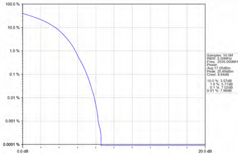
Band7_10MHz_64QAM_MCH_2535MHz_RB_50_0_NTNV
