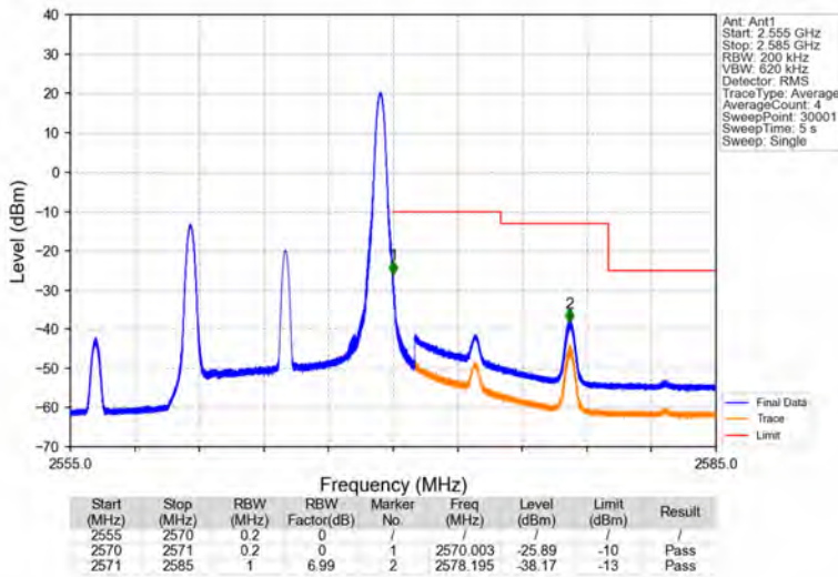
Band7_10MHz_16QAM_HCH_2565MHz_RB_1_49_NTNV
