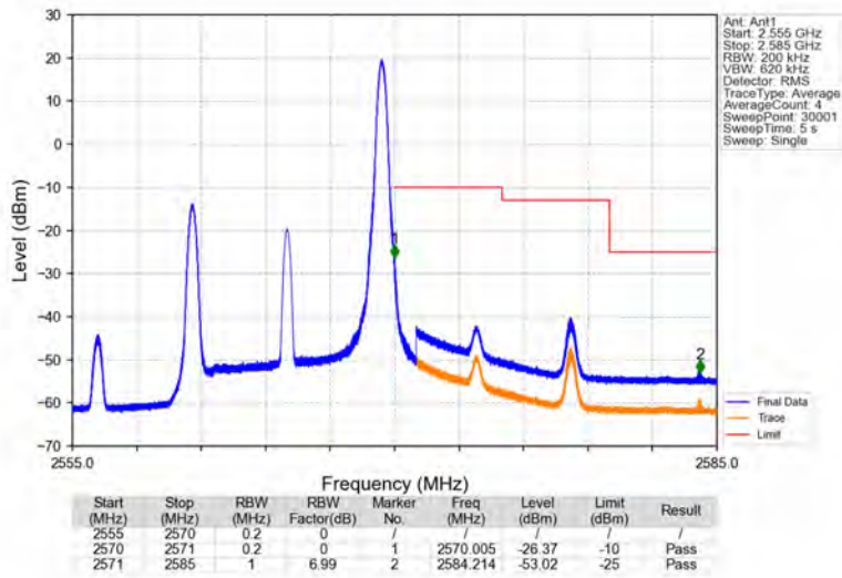
Band7_10MHz_64QAM_HCH_2565MHz_RB_1_49_NTNV
