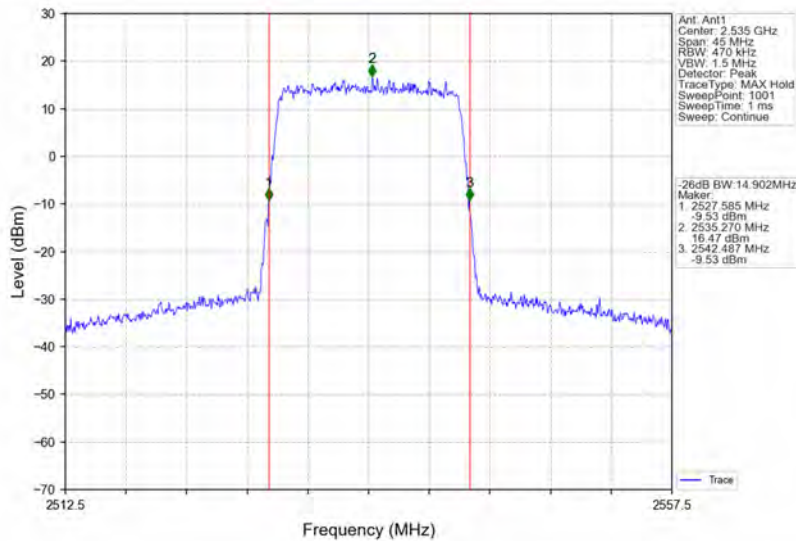
Band7_15MHz_64QAM_MCH_2535MHz_RB_75_0_NTNV
