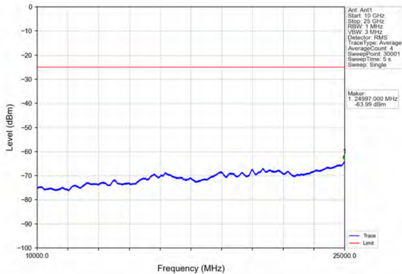
Band7_15MHz_16QAM_MCH_2535MHz_RB_1_0_NTNV
