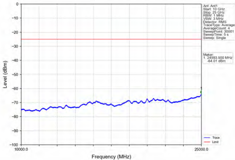
Band7_15MHz_16QAM_LCH_2507.5MHz_RB_1_0_NTNV
