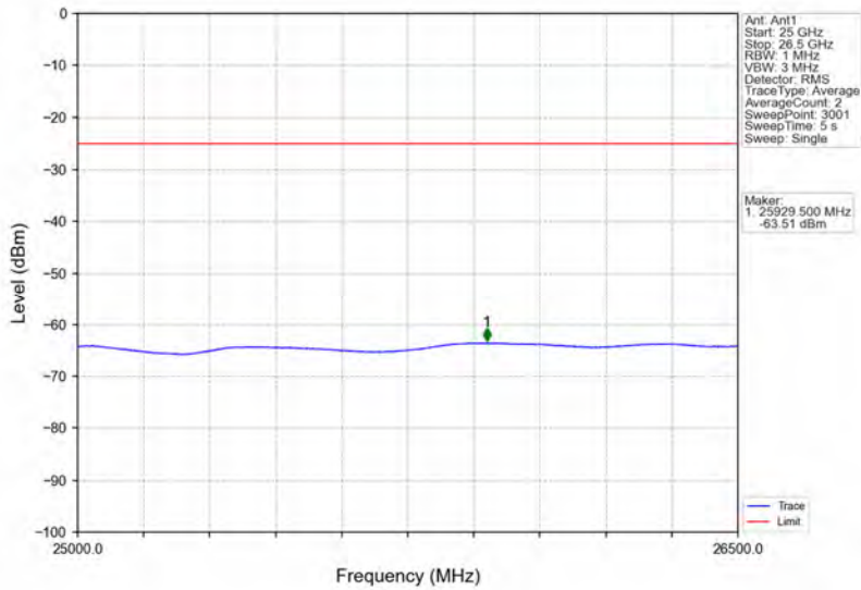
Band7_15MHz_16QAM_LCH_2507.5MHz_RB_75_0_NTNV
