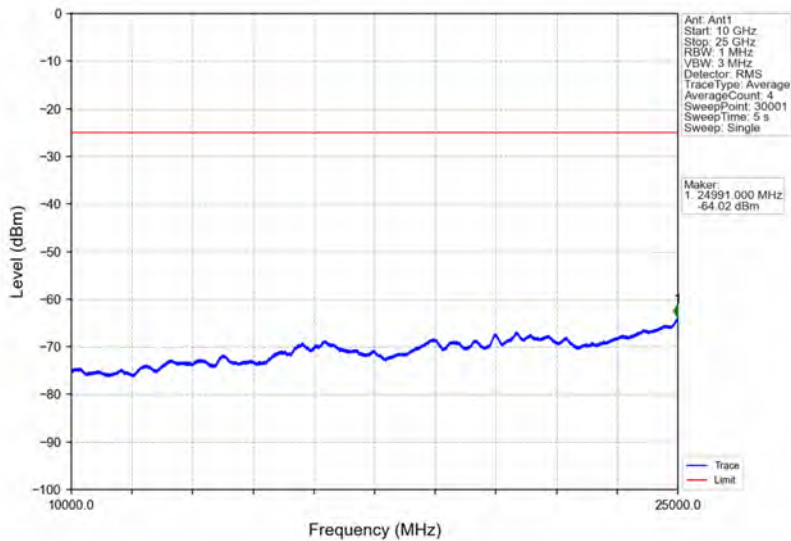
Band7_15MHz_64QAM_HCH_2562.5MHz_RB_1_0_NTNV
