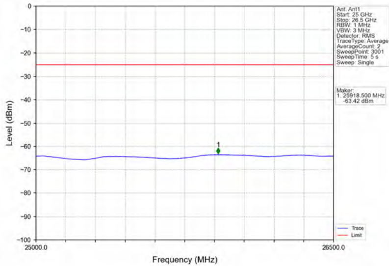
Band7_5MHz_16QAM_LCH_2502.5MHz_RB_25_0_NTNV
