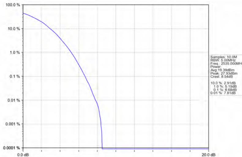
Band7_5MHz_64QAM_MCH_2535MHz_RB_25_0_NTNV
