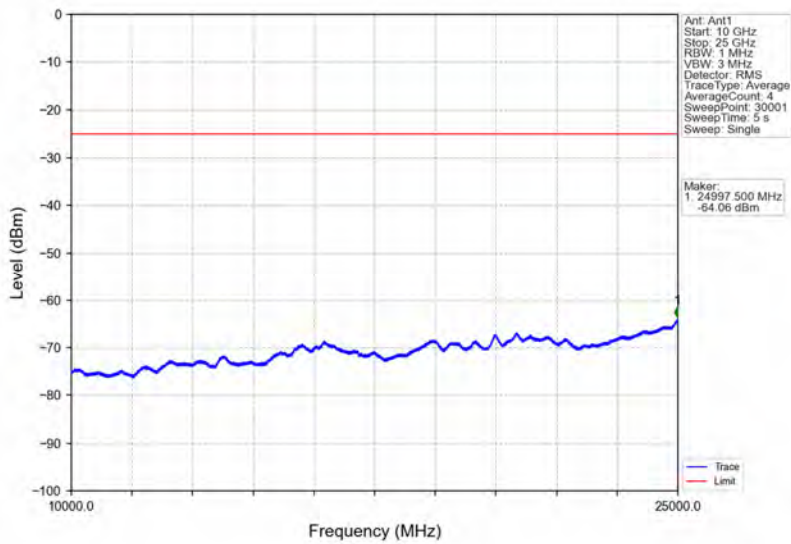
Band7_5MHz_64QAM_MCH_2535MHz_RB_1_0_NTNV
