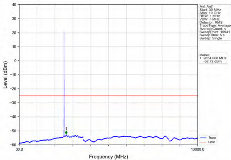
Band7_5MHz_64QAM_MCH_2535MHz_RB_1_0_NTNV
