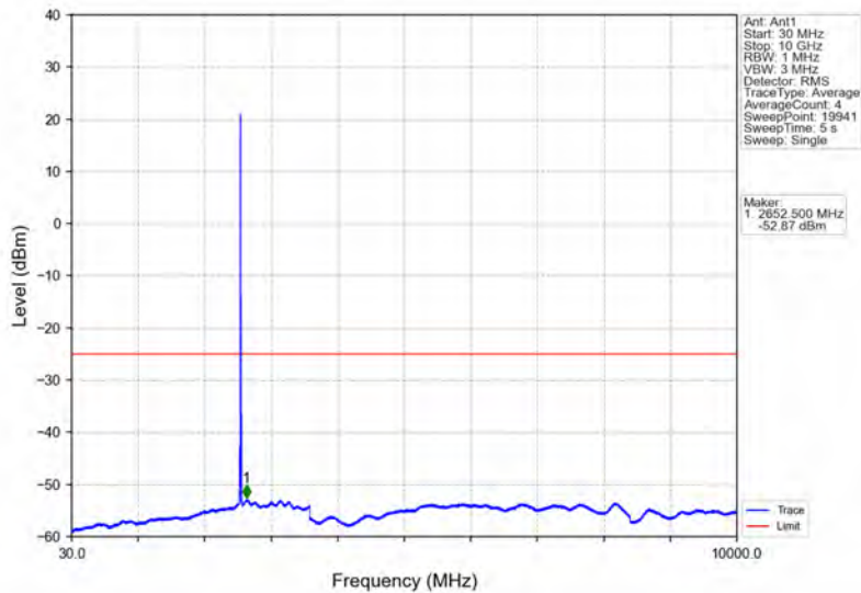
Band7_10MHz_16QAM_HCH_2565MHz_RB_1_0_NTNV
