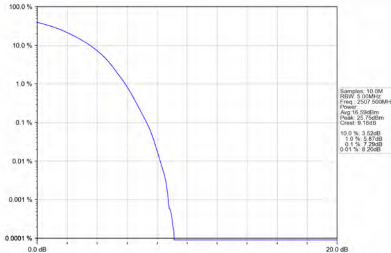
Band7_15MHz_16QAM_LCH_2507.5MHz_RB_75_0_NTNV
