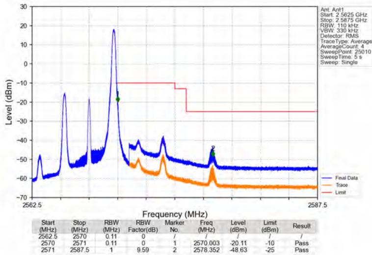
Band7_5MHz_64QAM_HCH_2567.5MHz_RB_1_24_NTNV
