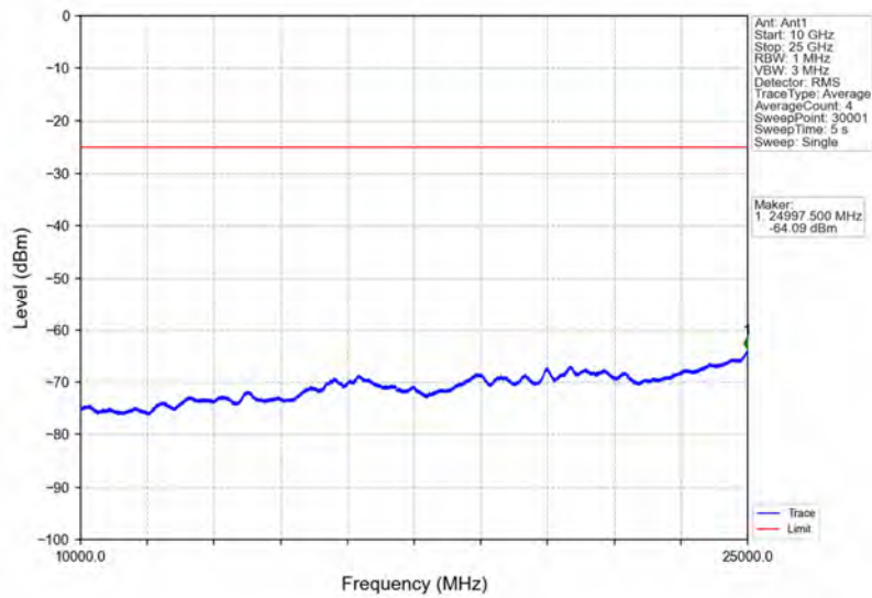
Band7_5MHz_16QAM_HCH_2567.5MHz_RB_1_0_NTNV
