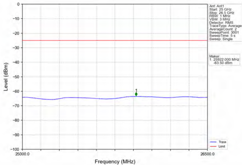
Band7_10MHz_64QAM_MCH_2535MHz_RB_1_0_NTNV
