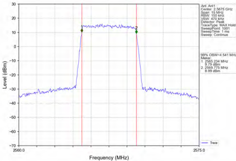
Band7_5MHz_16QAM_HCH_2567.5MHz_RB_25_0_NTNV
