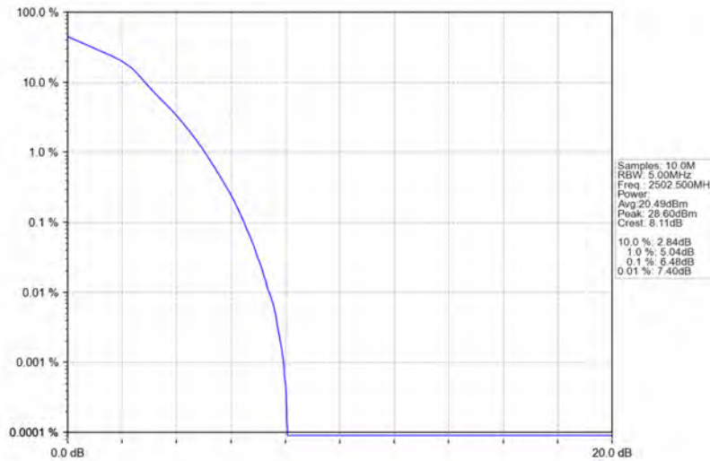
Band7_5MHz_16QAM_LCH_2502.5MHz_RB_25_0_NTNV
