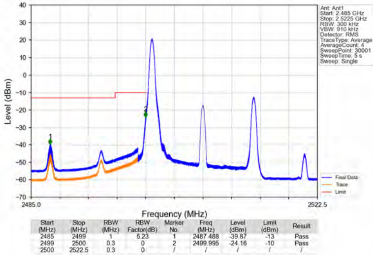
Band7_15MHz_64QAM_LCH_2507.5MHz_RB_1_0_NTNV
