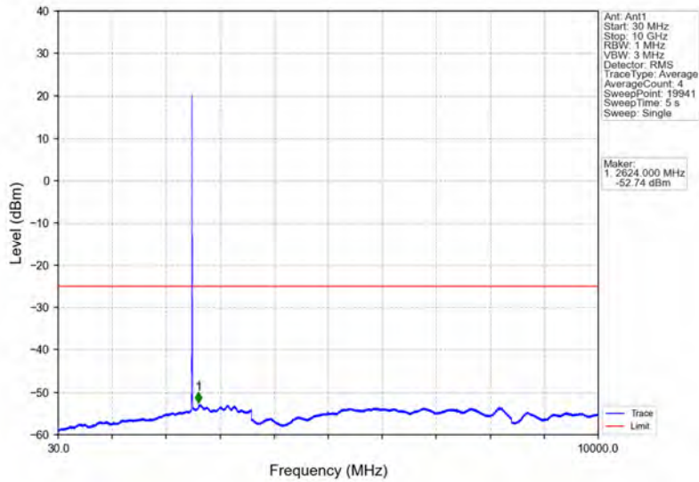
Band7_5MHz_16QAM_LCH_2502.5MHz_RB_1_0_NTNV
