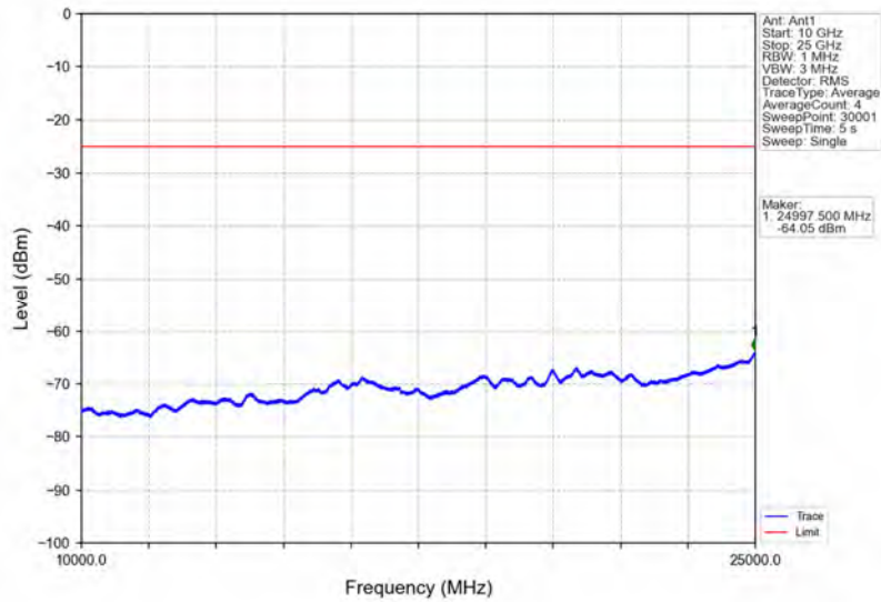
Band7_15MHz_64QAM_MCH_2535MHz_RB_1_0_NTNV
