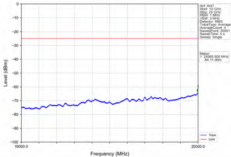
Band7_10MHz_16QAM_MCH_2535MHz_RB_1_0_NTNV
