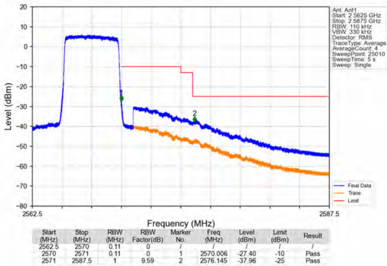
Band7_5MHz_16QAM_HCH_2567.5MHz_RB_25_0_NTNV
