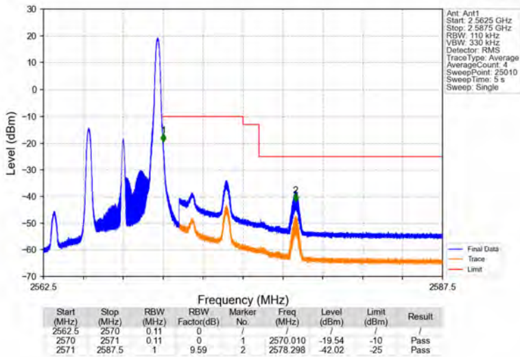
Band7_5MHz_16QAM_HCH_2567.5MHz_RB_1_24_NTNV
