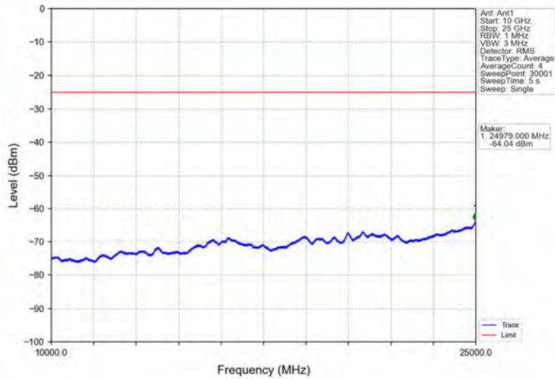
Band7_15MHz_QPSK_LCH_2507.5MHz_RB_1_0_NTNV
