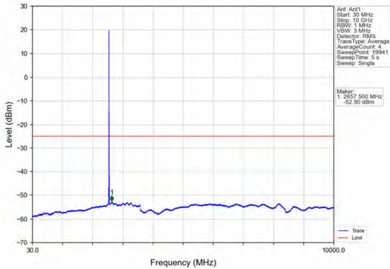
Band7_10MHz_64QAM_HCH_2565MHz_RB_1_0_NTNV
