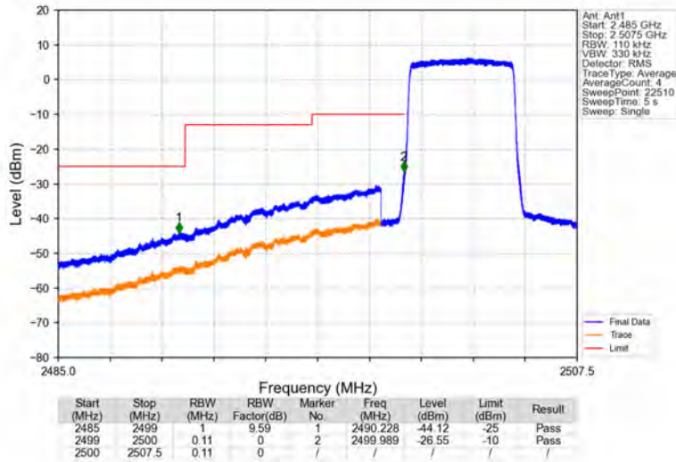
Band7_5MHz_16QAM_LCH_2502.5MHz_RB_25_0_NTNV
