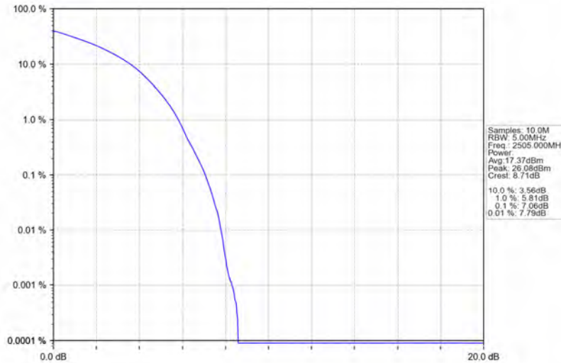
Band7_10MHz_64QAM_LCH_2505MHz_RB_50_0_NTNV
