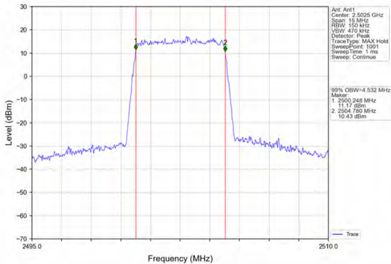
Band7_5MHz_16QAM_LCH_2502.5MHz_RB_25_0_NTNV
