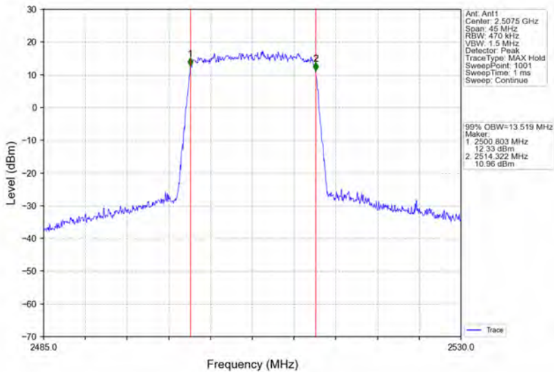
Band7_15MHz_16QAM_LCH_2507.5MHz_RB_75_0_NTNV
