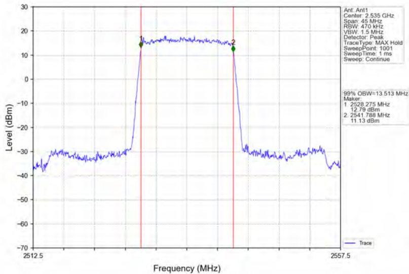
Band7_15MHz_QPSK_MCH_2535MHz_RB_75_0_NTNV
