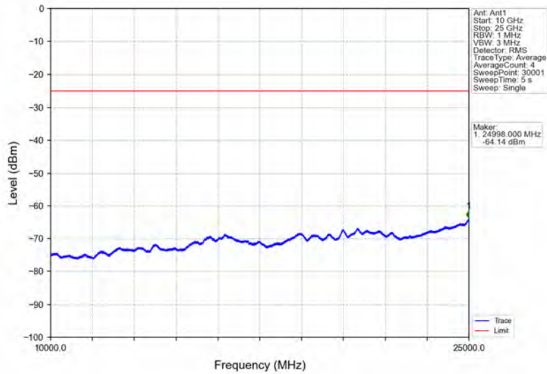
Band7_5MHz_64QAM_LCH_2502.5MHz_RB_1_0_NTNV
