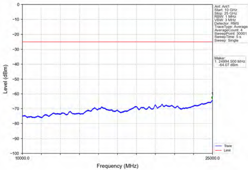
Band7_10MHz_16QAM_HCH_2565MHz_RB_1_0_NTNV
