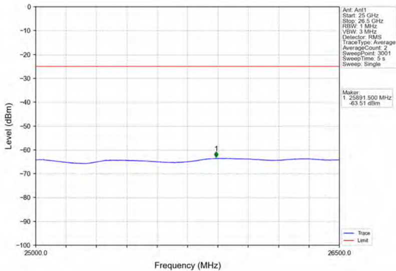
Band7_10MHz_16QAM_HCH_2565MHz_RB_1_0_NTNV
