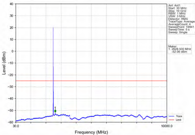
Band7_10MHz_64QAM_LCH_2505MHz_RB_1_0_NTNV
