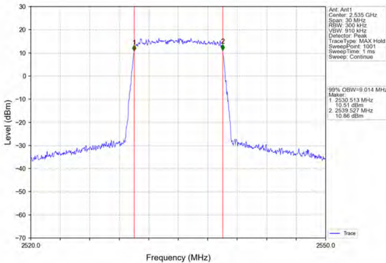
Band7_10MHz_16QAM_MCH_2535MHz_RB_50_0_NTNV
