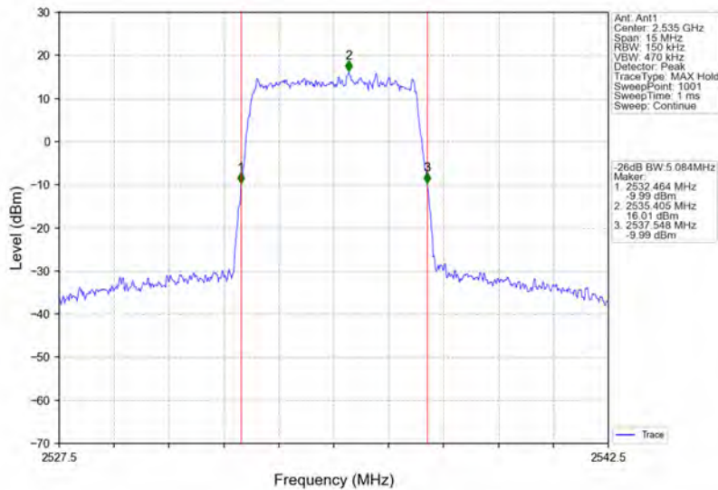
Band7_5MHz_64QAM_MCH_2535MHz_RB_25_0_NTNV
