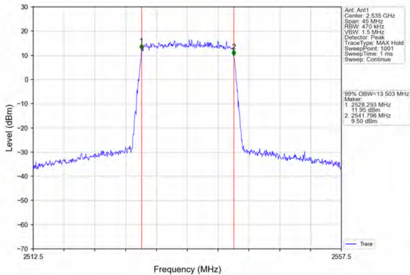
Band7_15MHz_64QAM_MCH_2535MHz_RB_75_0_NTNV
