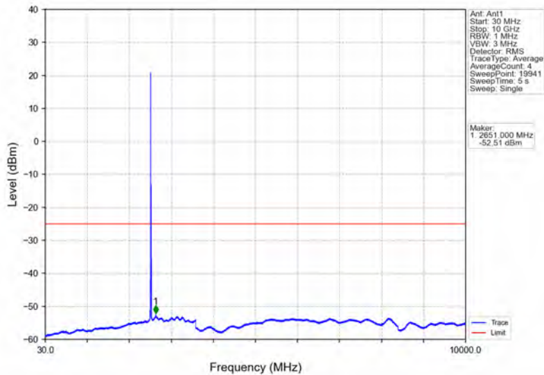
Band7_10MHz_64QAM_MCH_2535MHz_RB_1_0_NTNV
