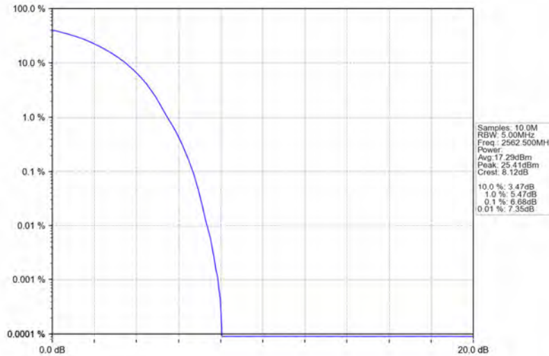
Band7_15MHz_QPSK_HCH_2562.5MHz_RB_75_0_NTNV
