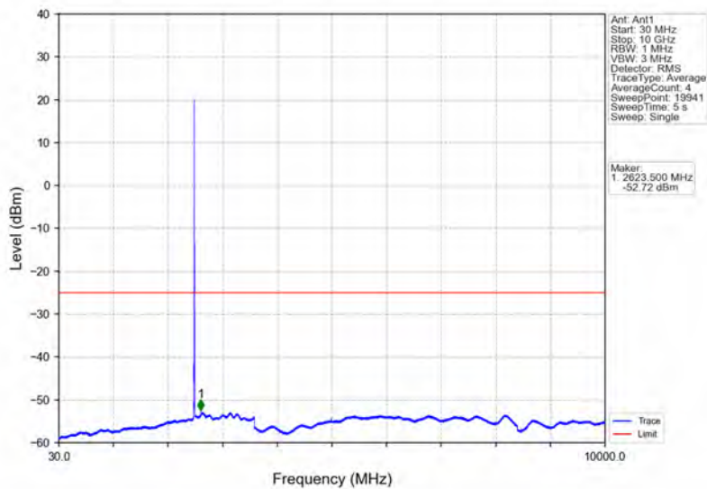
Band7_5MHz_64QAM_LCH_2502.5MHz_RB_1_0_NTNV
