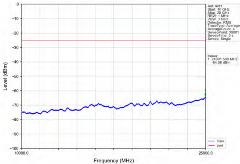
Band7_10MHz_64QAM_HCH_2565MHz_RB_1_0_NTNV
