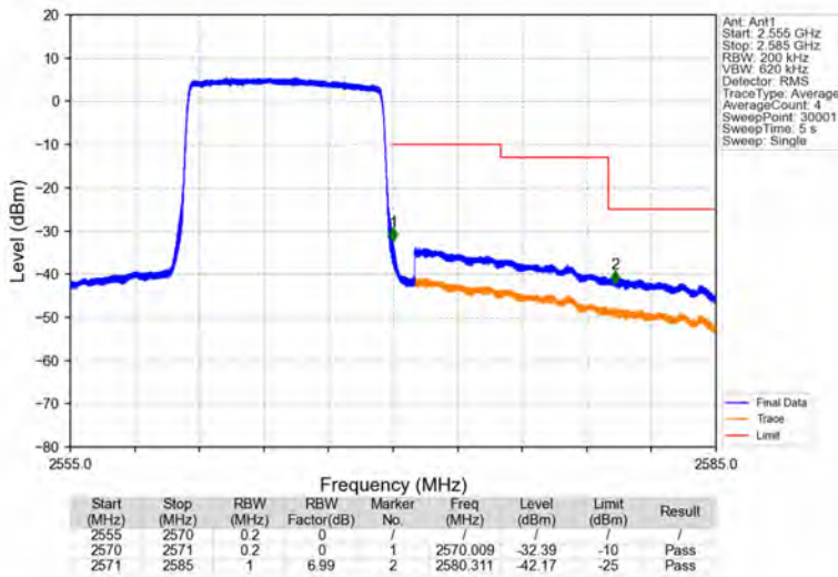
Band7_10MHz_16QAM_HCH_2565MHz_RB_50_0_NTNV
