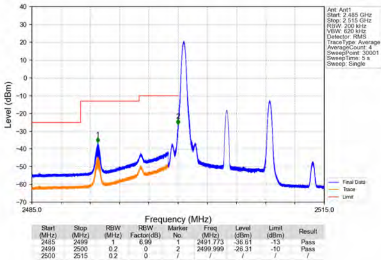
Band7_10MHz_64QAM_LCH_2505MHz_RB_1_0_NTNV
