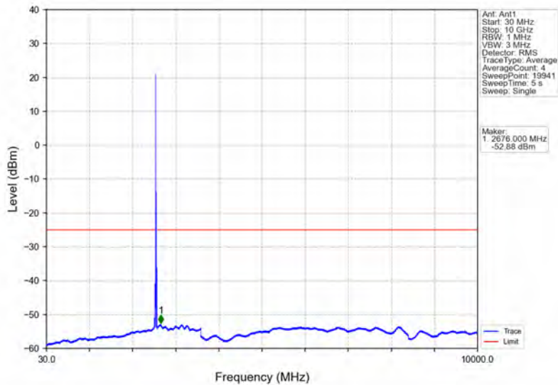
Band7_15MHz_16QAM_HCH_2562.5MHz_RB_1_0_NTNV
