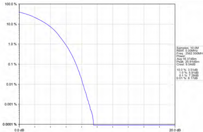
Band7_15MHz_16QAM_HCH_2562.5MHz_RB_75_0_NTNV
