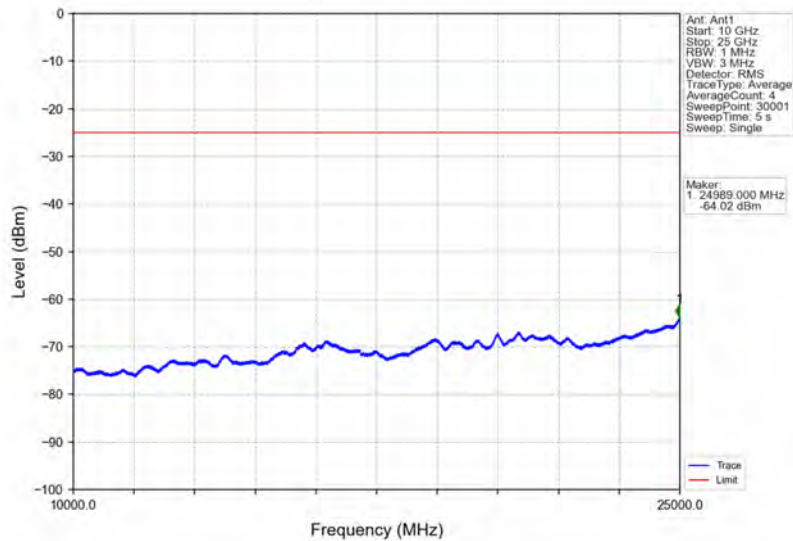
Band7_15MHz_QPSK_HCH_2562.5MHz_RB_1_0_NTNV
