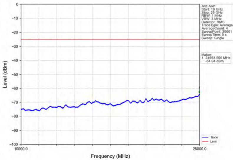
Band7_15MHz_QPSK_MCH_2535MHz_RB_1_0_NTNV
