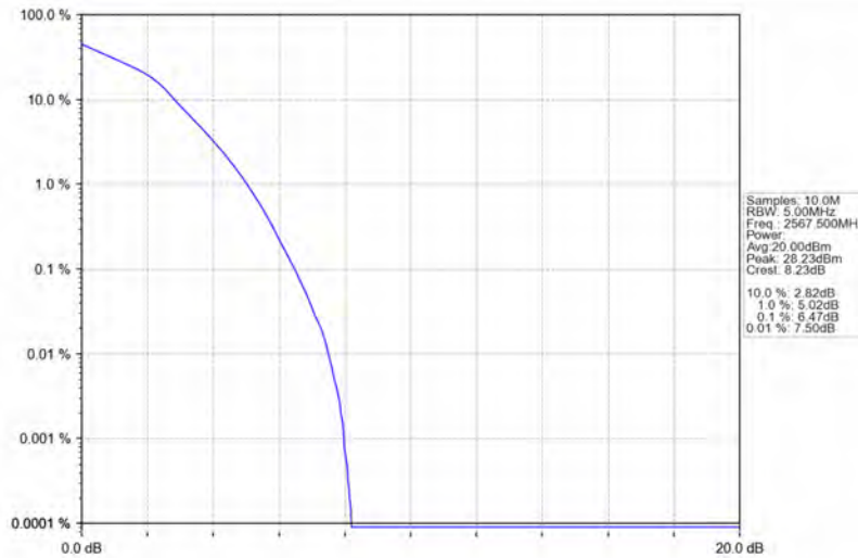
Band7_5MHz_16QAM_HCH_2567.5MHz_RB_25_0_NTNV
