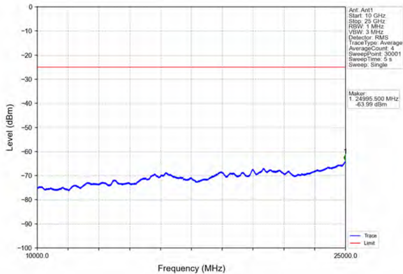
Band7_5MHz_16QAM_LCH_2502.5MHz_RB_1_0_NTNV
