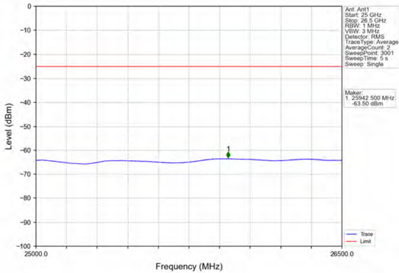
Band7_10MHz_16QAM_LCH_2505MHz_RB_50_0_NTNV
