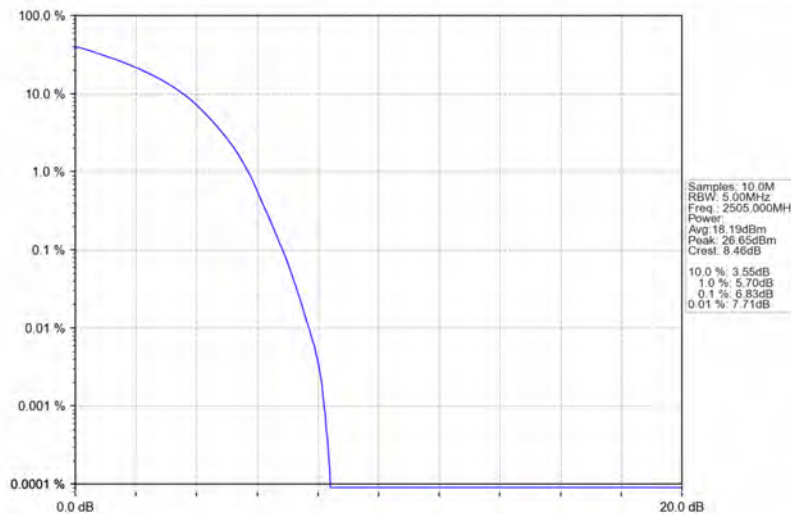
Band7_10MHz_16QAM_LCH_2505MHz_RB_50_0_NTNV
