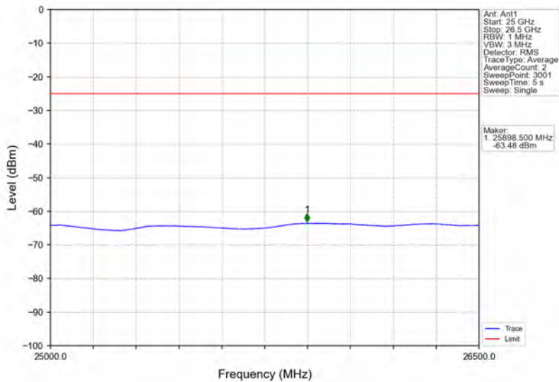
Band7_15MHz_16QAM_HCH_2562.5MHz_RB_1_0_NTNV
