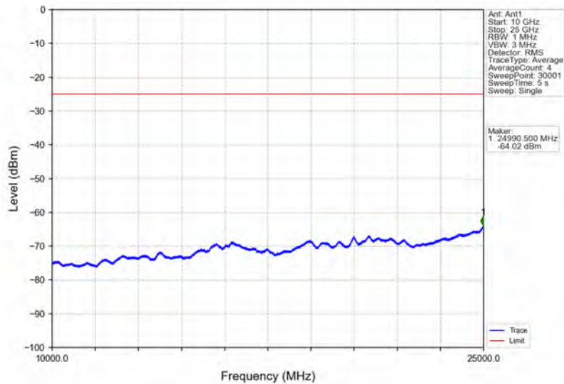
Band7_5MHz_16QAM_MCH_2535MHz_RB_1_0_NTNV
