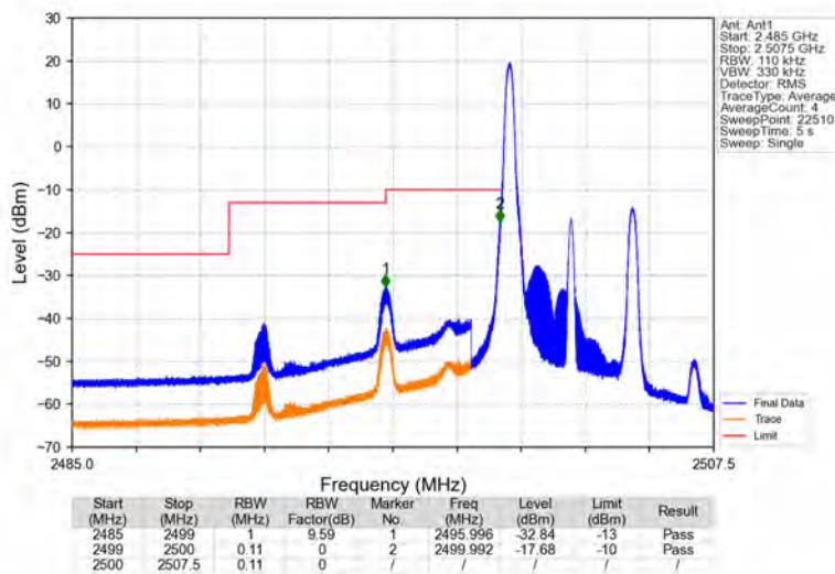
Band7_5MHz_16QAM_LCH_2502.5MHz_RB_1_0_NTNV
