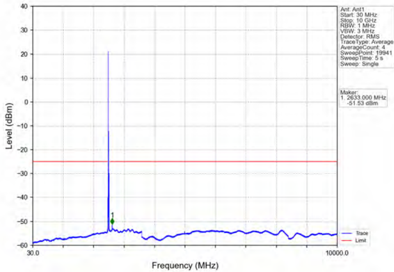
Band7_15MHz_16QAM_LCH_2507.5MHz_RB_1_0_NTNV
