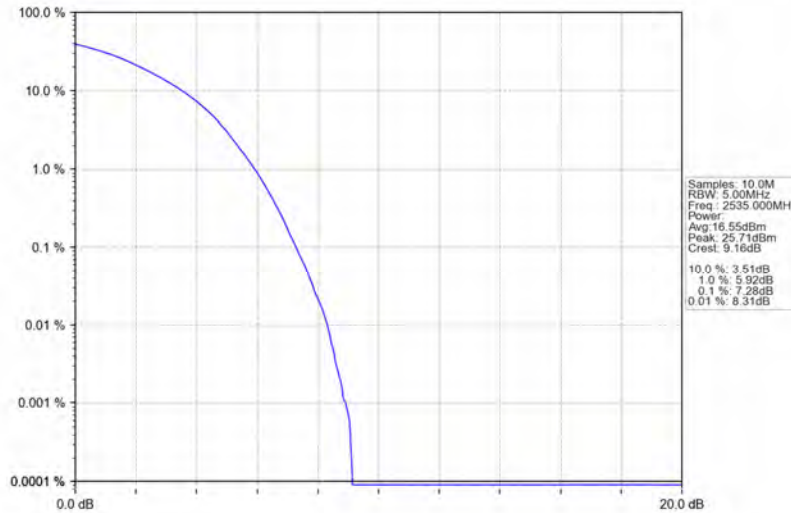
Band7_15MHz_16QAM_MCH_2535MHz_RB_75_0_NTNV
