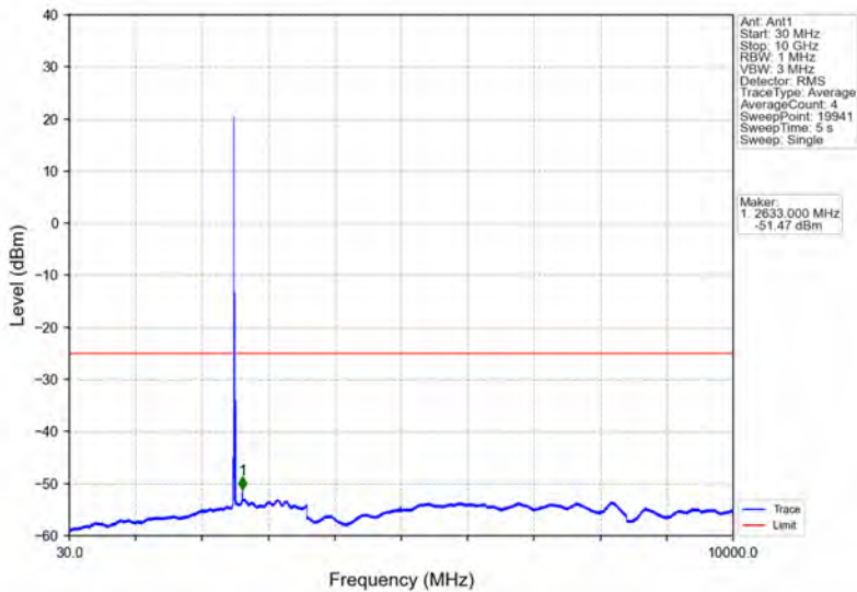
Band7_15MHz_64QAM_LCH_2507.5MHz_RB_1_0_NTNV
