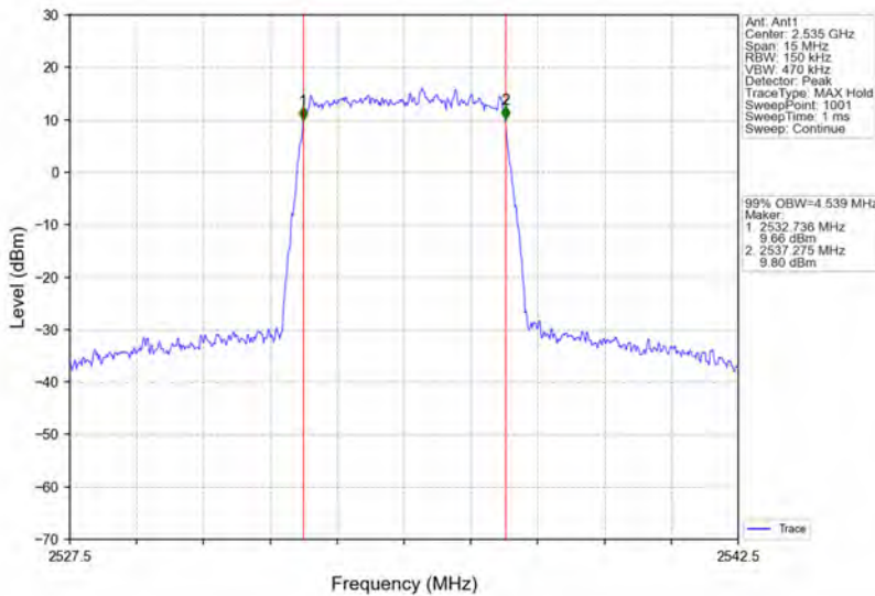
Band7_5MHz_64QAM_MCH_2535MHz_RB_25_0_NTNV
