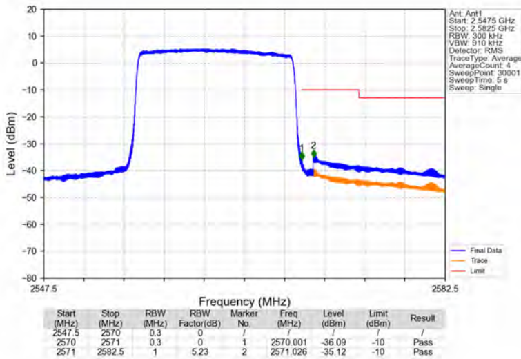
Band7_15MHz_16QAM_HCH_2562.5MHz_RB_75_0_NTNV
