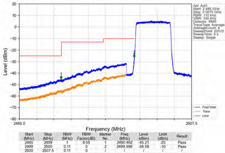
Band7_5MHz_64QAM_LCH_2502.5MHz_RB_25_0_NTNV
