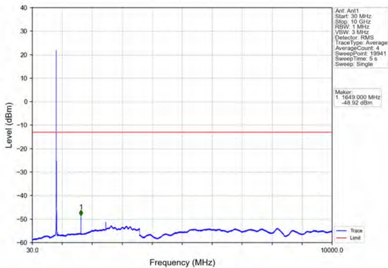
Band5_10MHz_64QAM_LCH_829MHz_RB_1_0_NTNV
