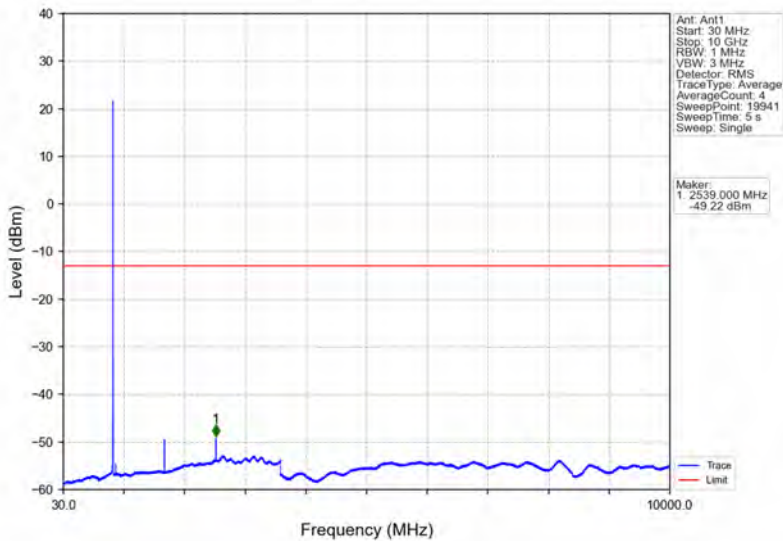
Band5_3MHz_16QAM_HCH_847.5MHz_RB_1_0_NTNV
