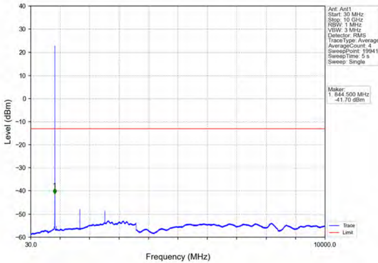
Band5_1.4MHz_QPSK_HCH_848.3MHz_RB_1_5_NTNV
