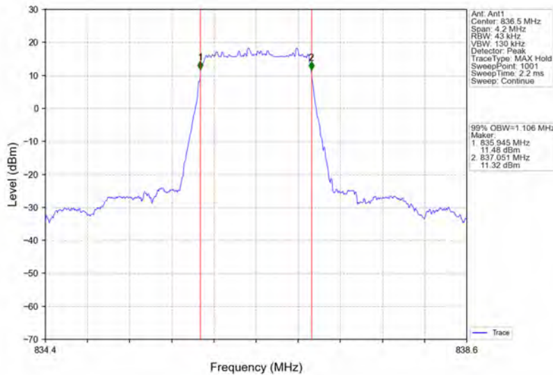
Band5_1.4MHz_64QAM_MCH_836.5MHz_RB_6_0_NTNV
