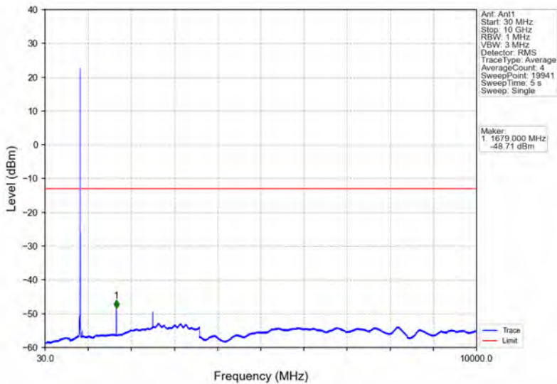
Band5_10MHz_16QAM_HCH_844MHz_RB_1_0_NTNV
