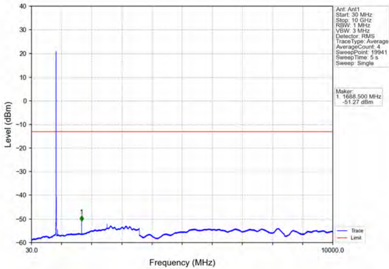
Band5_5MHz_64QAM_HCH_846.5MHz_RB_1_24_NTNV
