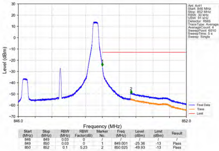
Band5_3MHz_64QAM_HCH_847.5MHz_RB_1_14_NTNV
