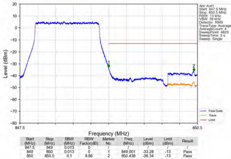
Band5_1.4MHz_QPSK_HCH_848.3MHz_RB_6_0_NTNV
