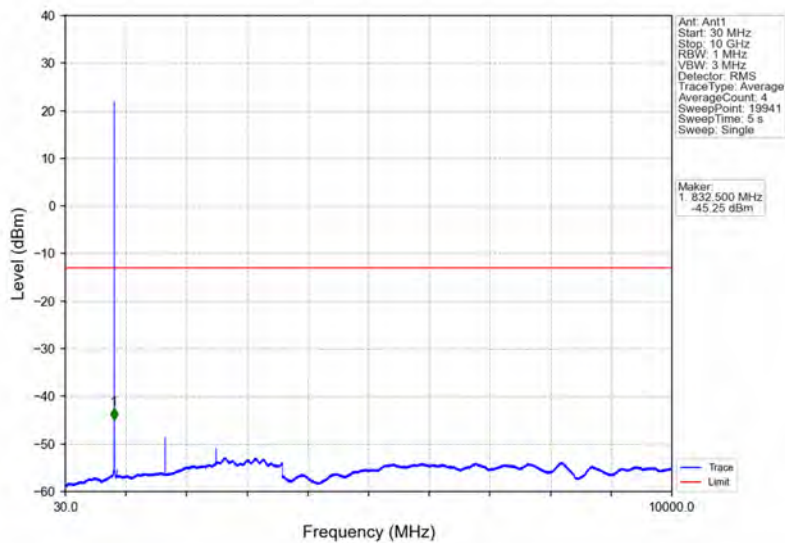
Band5_1.4MHz_64QAM_MCH_836.5MHz_RB_1_0_NTNV
