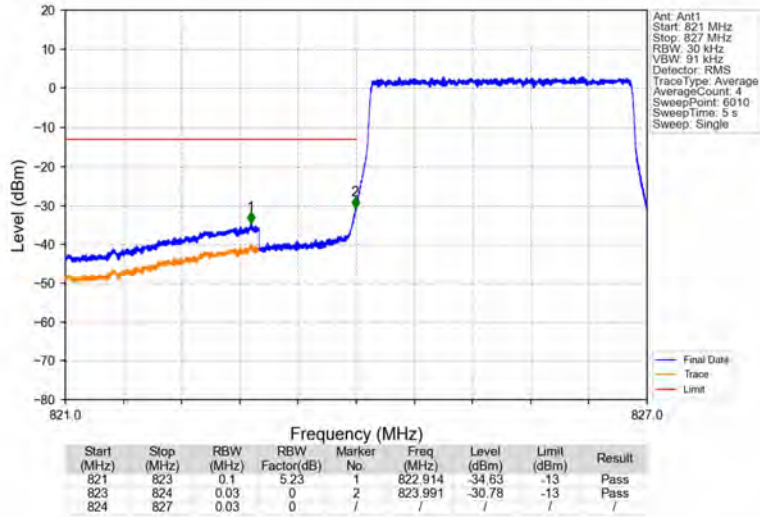
Band5_3MHz_64QAM_LCH_825.5MHz_RB_15_0_NTNV
