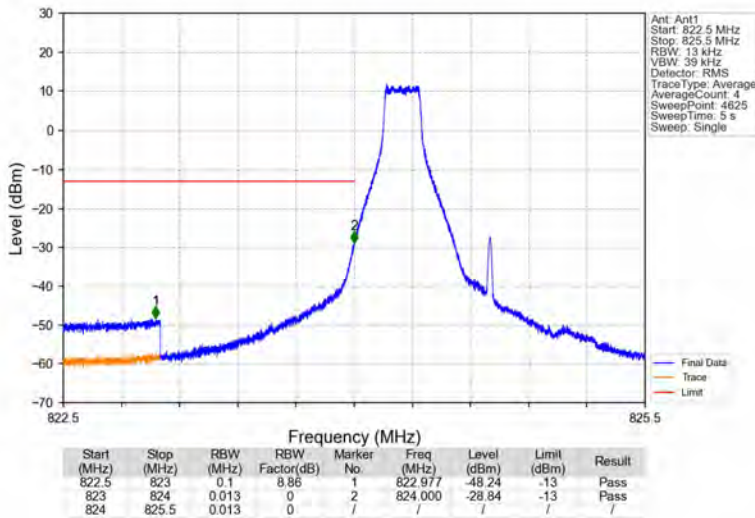
Band5_1.4MHz_64QAM_LCH_824.7MHz_RB_1_0_NTNV
