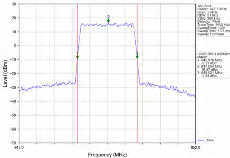
Band5_3MHz_64QAM_HCH_847.5MHz_RB_15_0_NTNV
