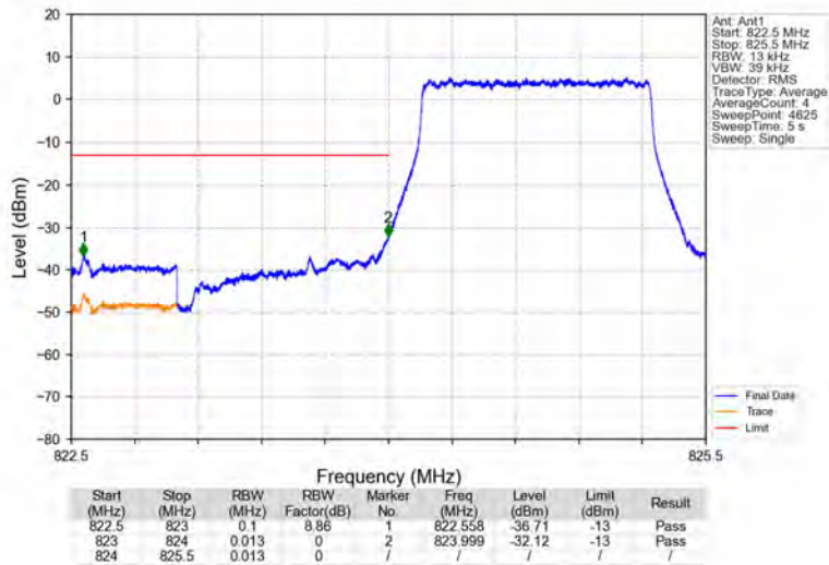
Band5_1.4MHz_QPSK_LCH_824.7MHz_RB_6_0_NTNV
