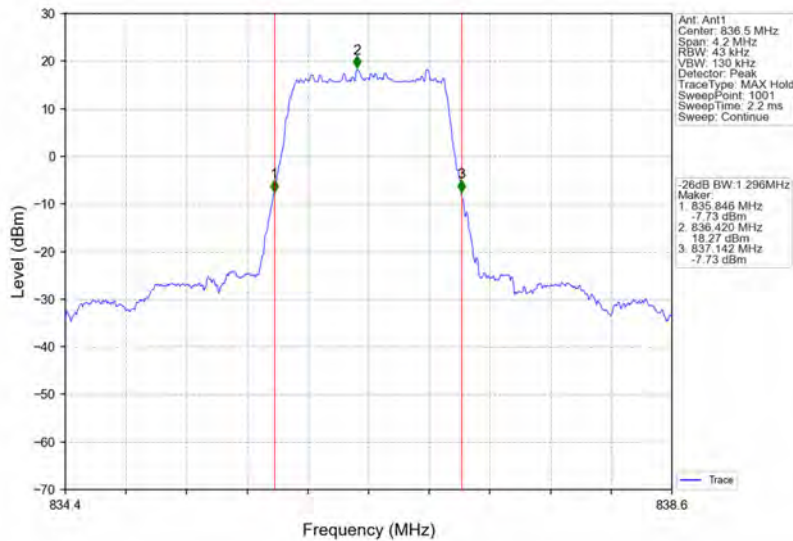
Band5_1.4MHz_64QAM_MCH_836.5MHz_RB_6_0_NTNV
