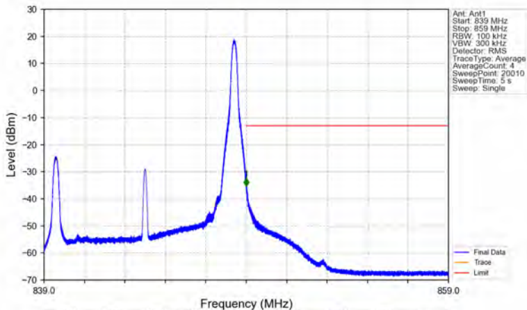
Band5_10MHz_64QAM_HCH_844MHz_RB_1_49_NTNV
