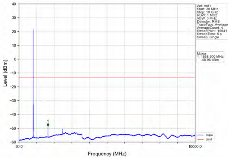
Band5_5MHz_64QAM_MCH_836.5MHz_RB_1_0_NTNV
