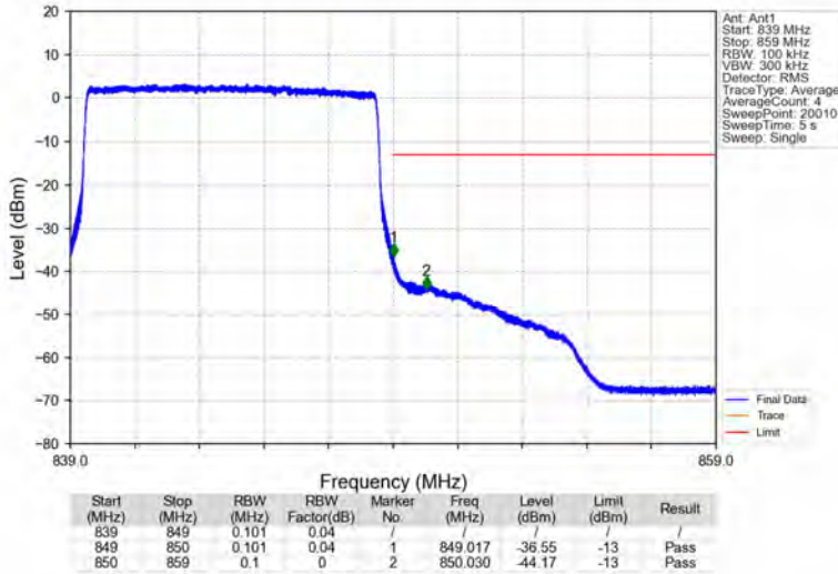
Band5_10MHz_64QAM_HCH_844MHz_RB_50_0_NTNV
