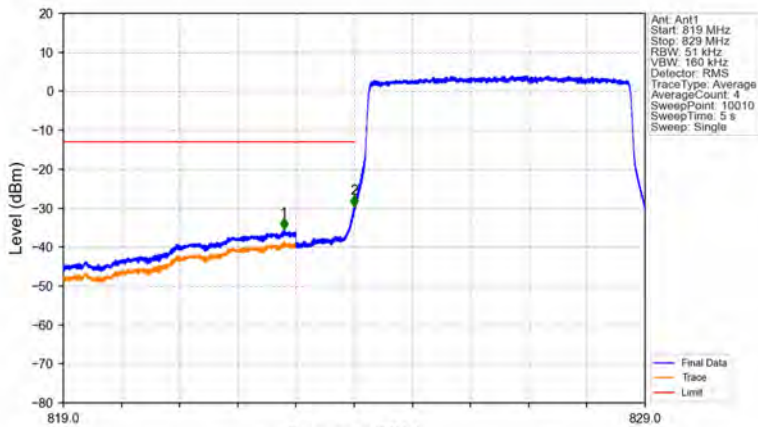
Band5_5MHz_16QAM_LCH_826.5MHz_RB_25_0_NTNV
