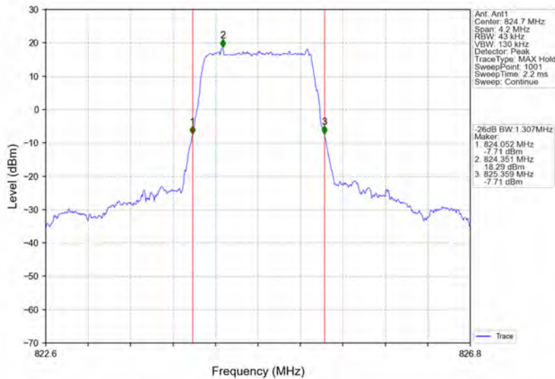
Band5_1.4MHz_16QAM_LCH_824.7MHz_RB_6_0_NTNV
