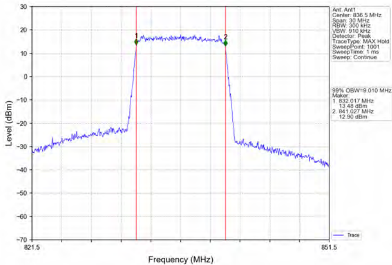
Band5_10MHz_16QAM_MCH_836.5MHz_RB_50_0_NTNV
