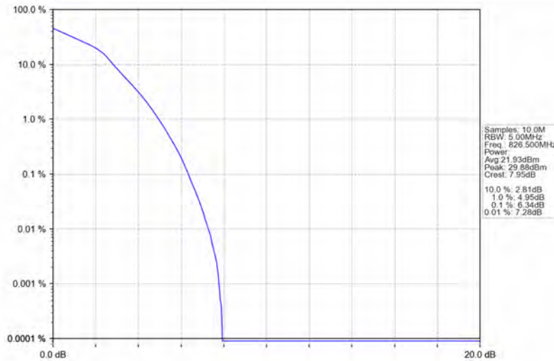
Band5_5MHz_16QAM_LCH_826.5MHz_RB_25_0_NTNV
