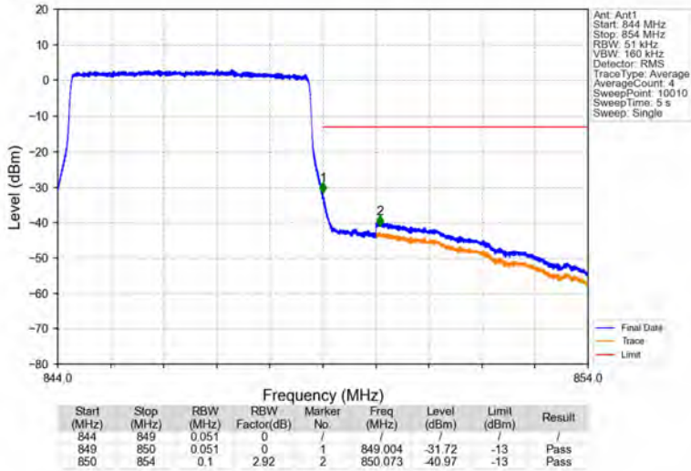
Band5_5MHz_64QAM_HCH_846.5MHz_RB_25_0_NTNV
