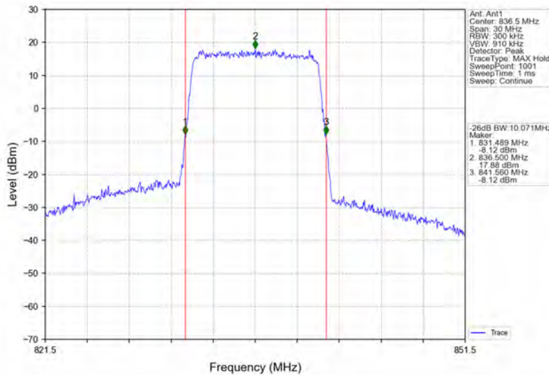
Band5_10MHz_16QAM_MCH_836.5MHz_RB_50_0_NTNV
