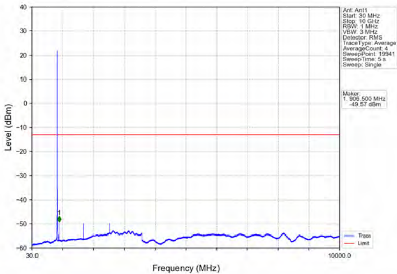
Band5_5MHz_16QAM_HCH_846.5MHz_RB_1_0_NTNV
