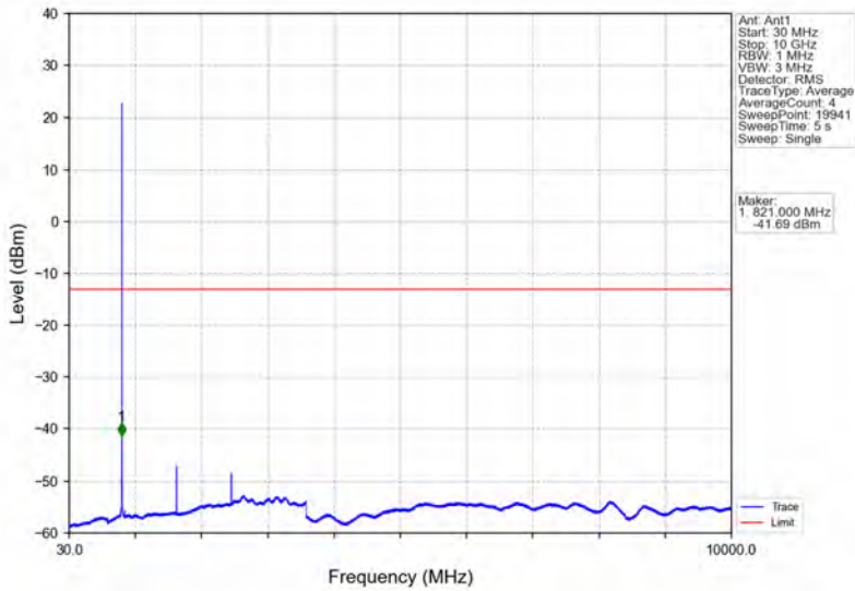
Band5_1.4MHz_16QAM_LCH_824.7MHz_RB_6_0_NTNV
