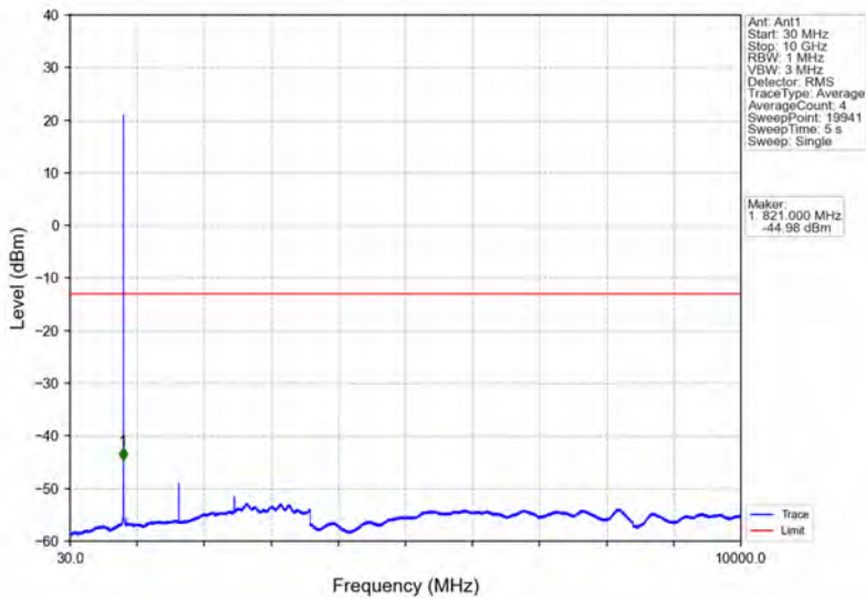
Band5_1.4MHz_64QAM_LCH_824.7MHz_RB_1_0_NTNV
