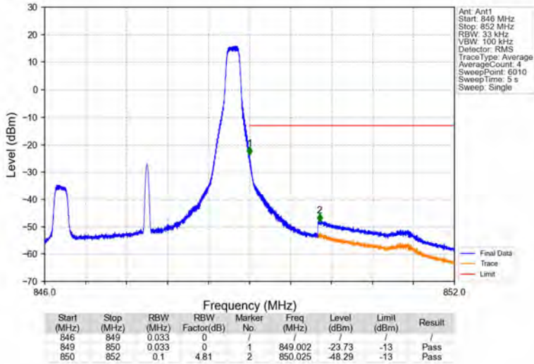
Band5_3MHz_16QAM_HCH_847.5MHz_RB_1_14_NTNV
