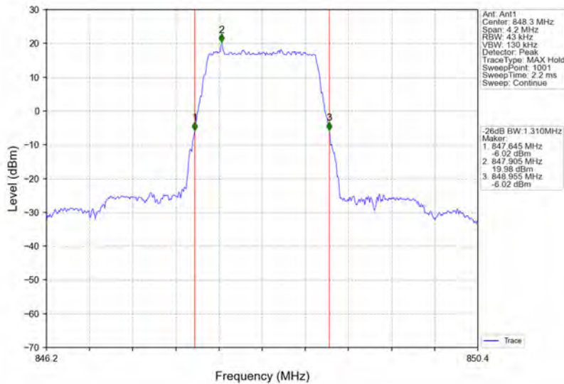
Band5_1.4MHz_16QAM_HCH_848.3MHz_RB_6_0_NTNV
