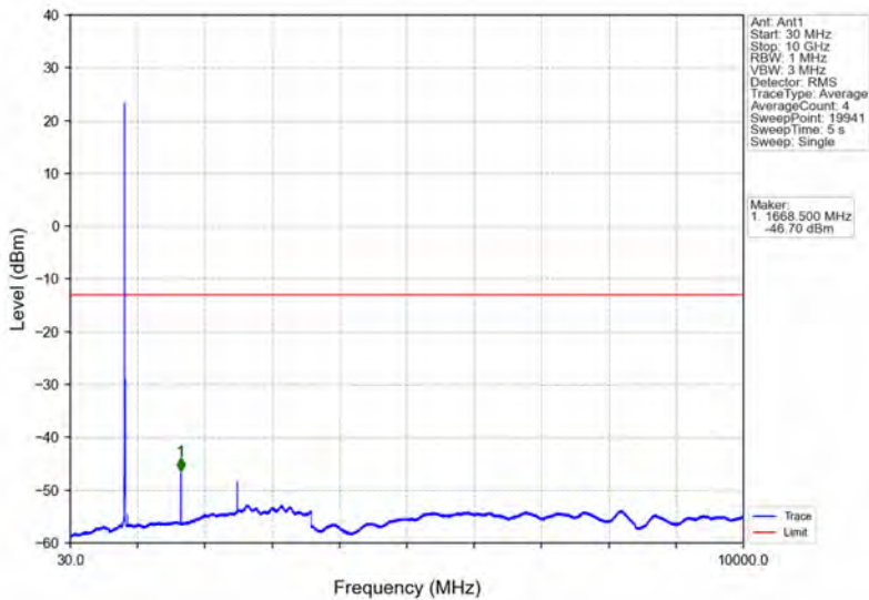
Band5_5MHz_QPSK_MCH_836.5MHz_RB_1_0_NTNV
