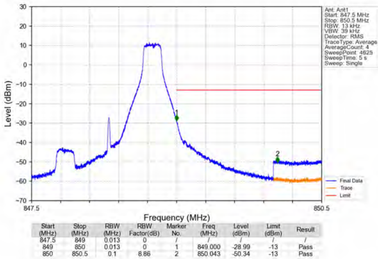
Band5_1.4MHz_64QAM_HCH_848.3MHz_RB_1_5_NTNV
