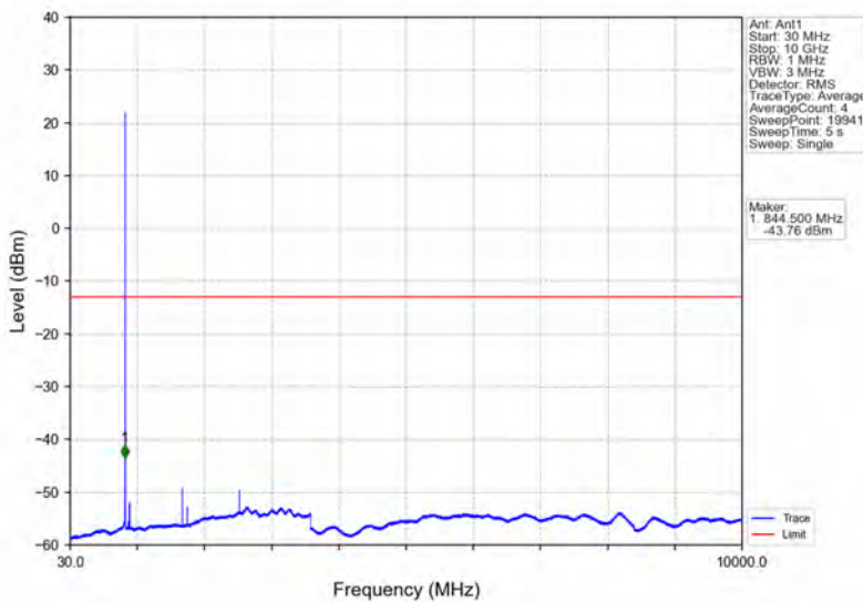
Band5_1.4MHz_16QAM_HCH_848.3MHz_RB_1_0_NTNV
