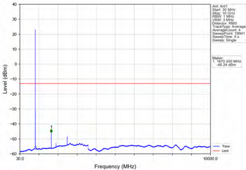
Band5_3MHz_QPSK_MCH_836.5MHz_RB_1_0_NTNV
