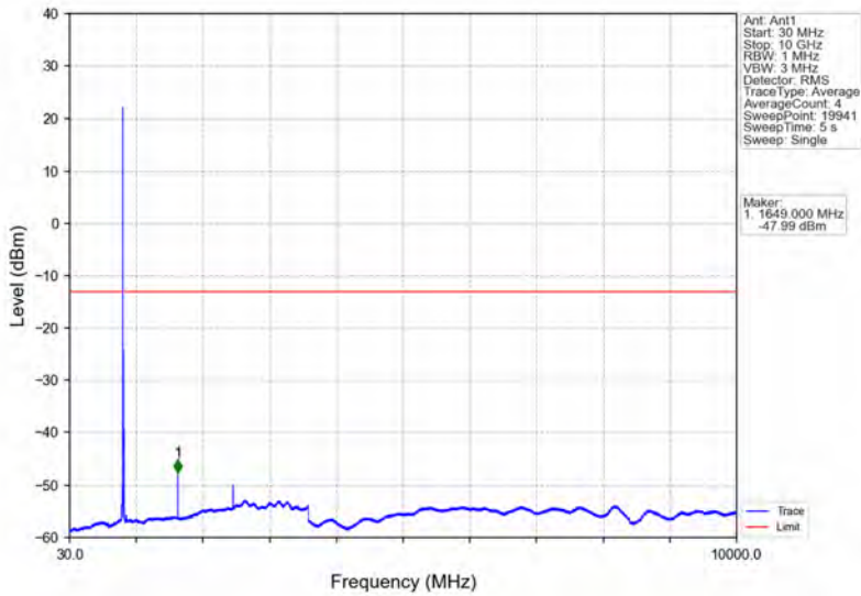
Band5_10MHz_16QAM_LCH_829MHz_RB_50_0_NTNV
