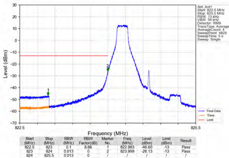
Band5_1.4MHz_16QAM_LCH_824.7MHz_RB_1_0_NTNV
