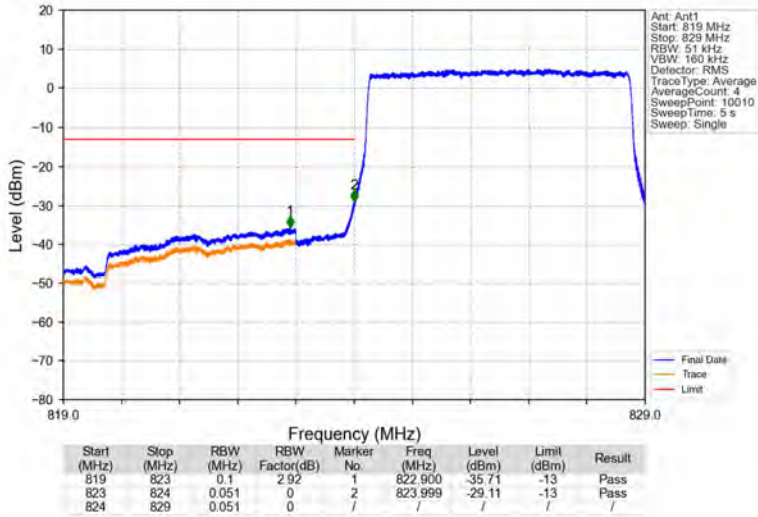
Band5_5MHz_QPSK_LCH_826.5MHz_RB_25_0_NTNV
