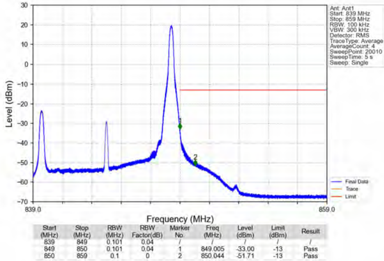
Band5_10MHz_16QAM_HCH_844MHz_RB_1_49_NTNV
