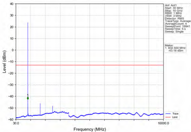
Band5_1.4MHz_QPSK_MCH_836.5MHz_RB_1_0_NTNV
