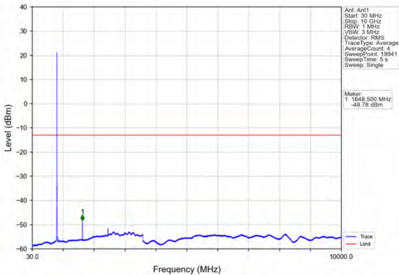
Band5_3MHz_64QAM_LCH_825.5MHz_RB_1_0_NTNV
