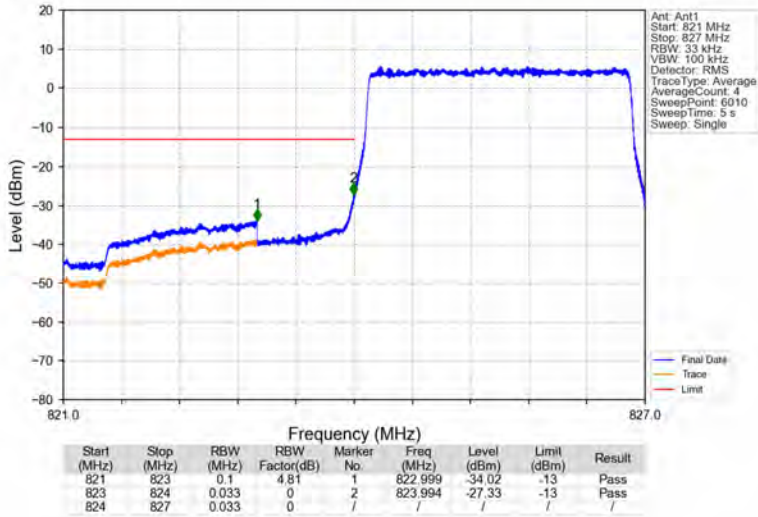
Band5_3MHz_QPSK_LCH_825.5MHz_RB_15_0_NTNV
