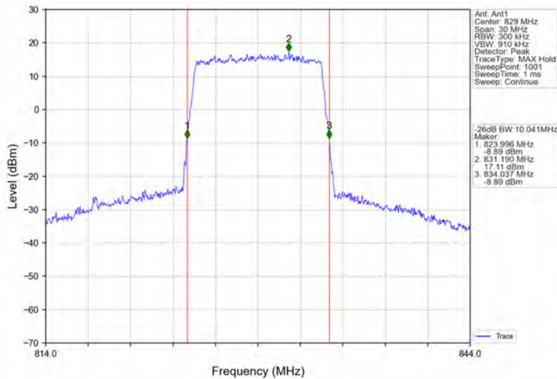
Band5_10MHz_64QAM_LCH_829MHz_RB_50_0_NTNV
