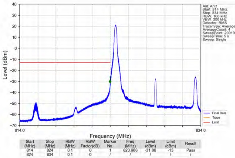
Band5_10MHz_16QAM_LCH_829MHz_RB_1_0_NTNV
