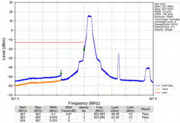
Band5_3MHz_64QAM_LCH_825.5MHz_RB_1_0_NTNV
