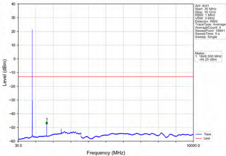
Band5_5MHz_64QAM_LCH_826.5MHz_RB_1_0_NTNV
