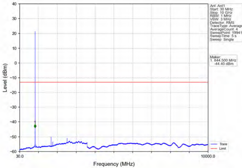
Band5_1.4MHz_64QAM_HCH_848.3MHz_RB_1_5_NTNV
