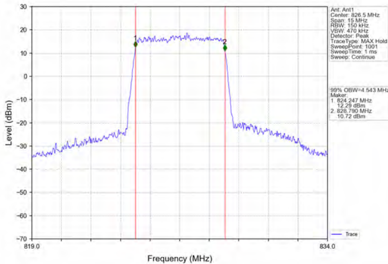
Band5_5MHz_16QAM_LCH_826.5MHz_RB_25_0_NTNV
