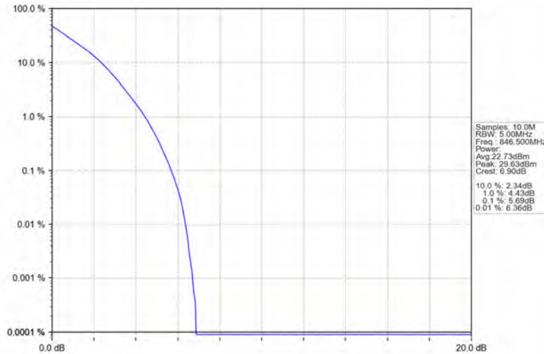
Band5_5MHz_QPSK_HCH_846.5MHz_RB_25_0_NTNV
