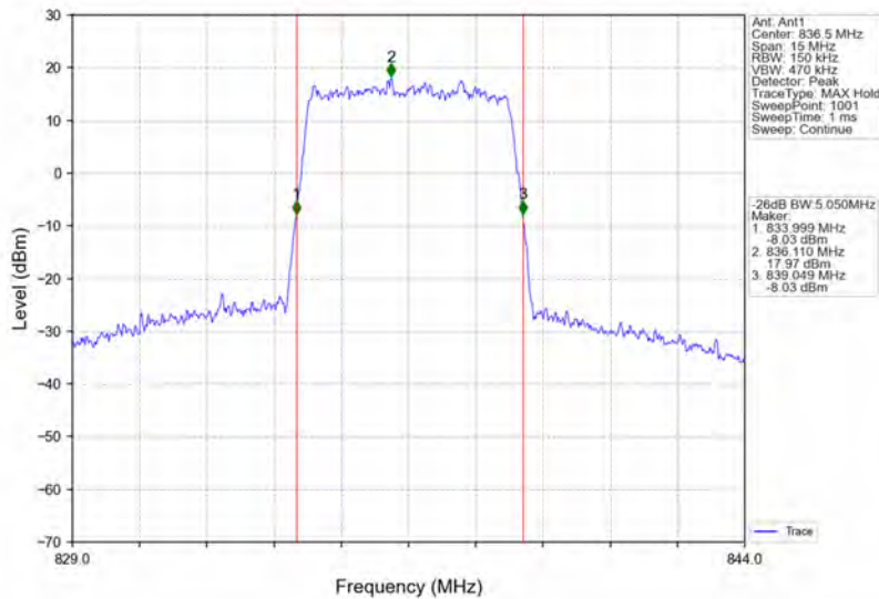
Band5_5MHz_64QAM_MCH_836.5MHz_RB_25_0_NTNV
