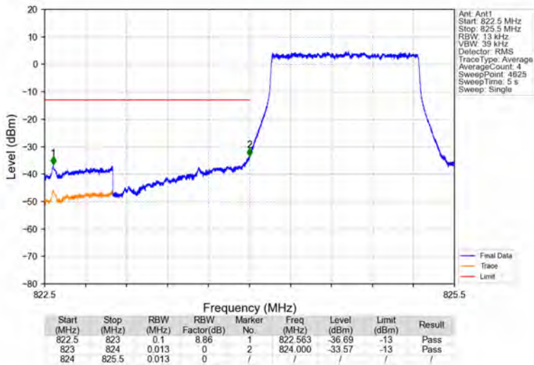
Band5_1.4MHz_16QAM_LCH_824.7MHz_RB_6_0_NTNV
