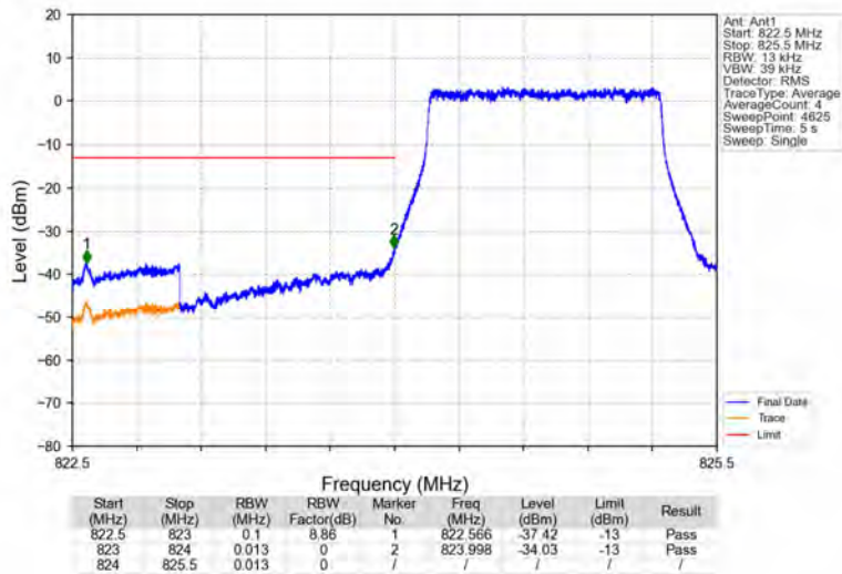
Band5_1.4MHz_64QAM_LCH_824.7MHz_RB_6_0_NTNV
