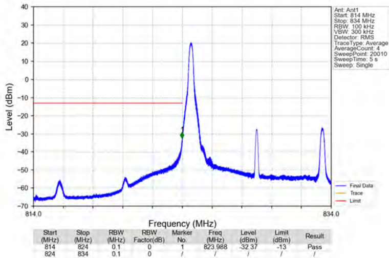
Band5_10MHz_64QAM_LCH_829MHz_RB_1_0_NTNV
