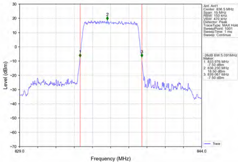
Band5_5MHz_QPSK_MCH_836.5MHz_RB_25_0_NTNV
