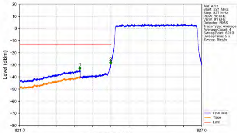
Band5_3MHz_16QAM_LCH_825.5MHz_RB_15_0_NTNV
