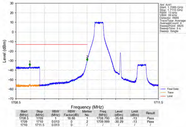
Band4_1.4MHz_64QAM_LCH_1710.7MHz_RB_1_0_NTNV
