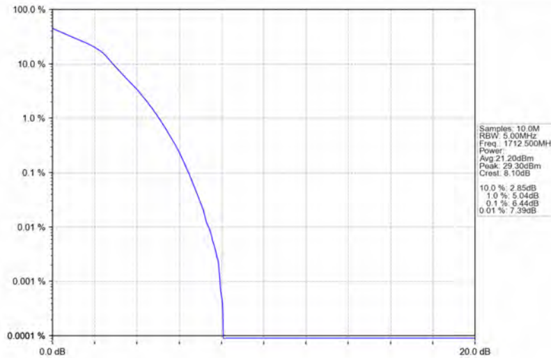
Band4_5MHz_16QAM_LCH_1712.5MHz_RB_25_0_NTNV
