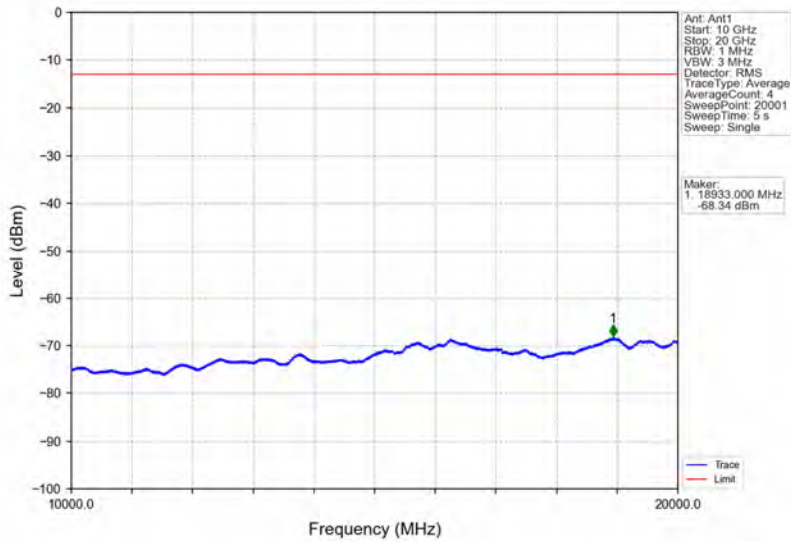
Band4_5MHz_QPSK_LCH_1712.5MHz_RB_25_0_NTNV
