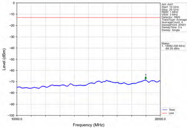
Band4_10MHz_64QAM_LCH_1715MHz_RB_50_0_NTNV
