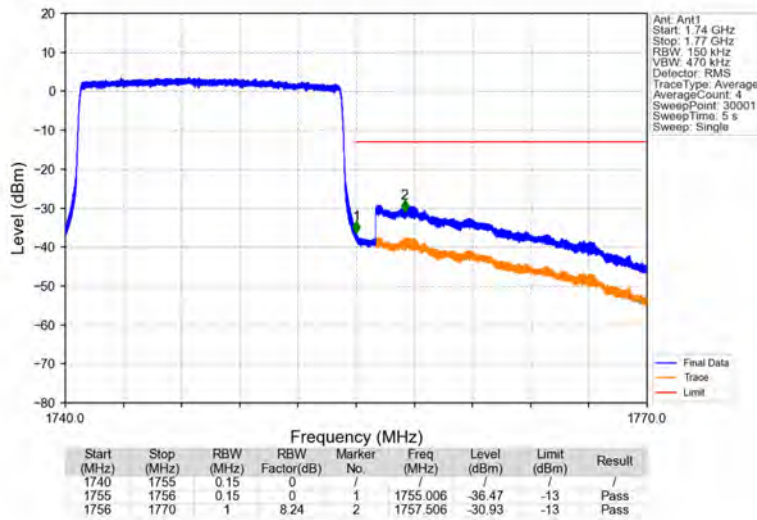
Band4_15MHz_16QAM_HCH_1747.5MHz_RB_75_0_NTNV
