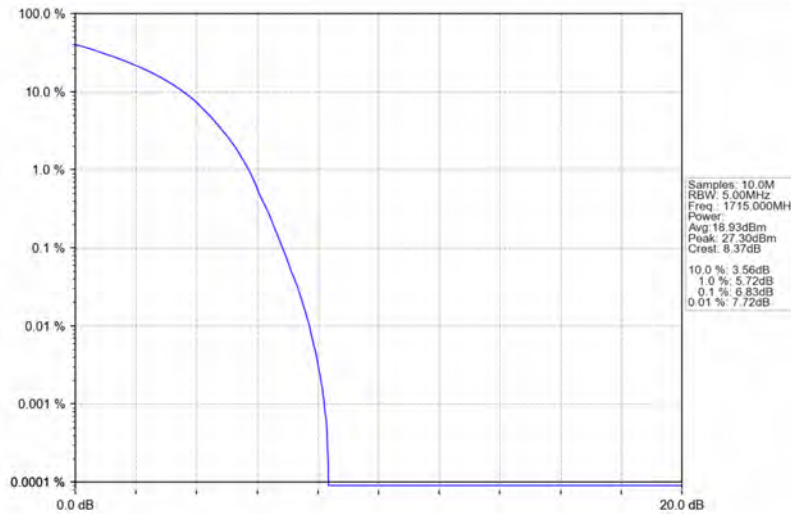
Band4_10MHz_16QAM_LCH_1715MHz_RB_50_0_NTNV
