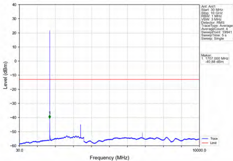
Band4_1.4MHz_16QAM_LCH_1710.7MHz_RB_1_0_NTNV
