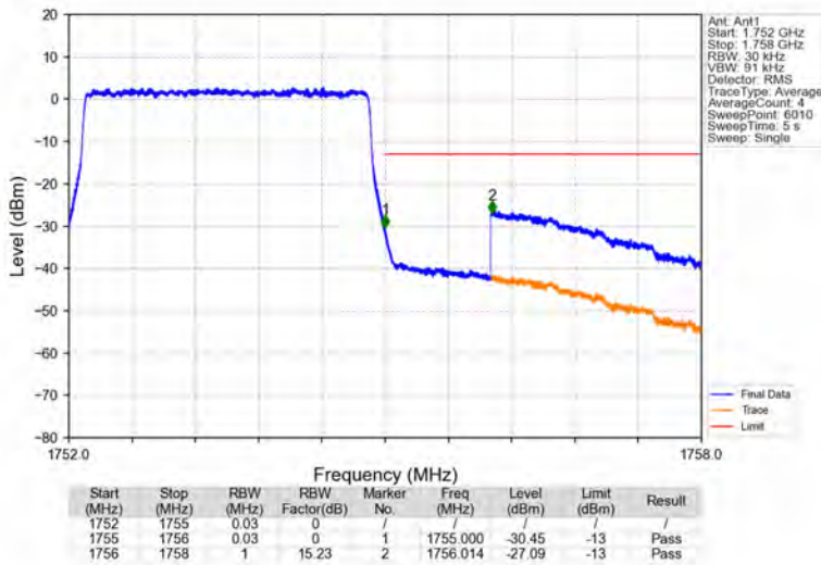
Band4_3MHz_16QAM_HCH_1753.5MHz_RB_15_0_NTNV
