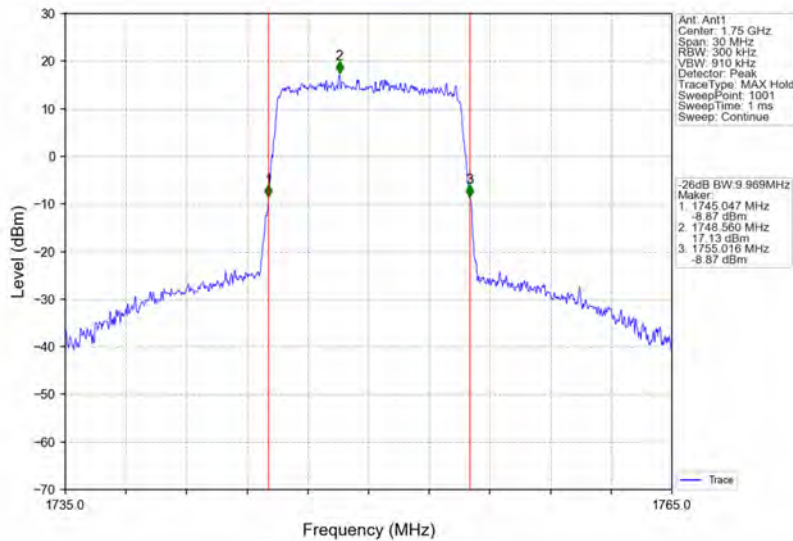
Band4_10MHz_64QAM_HCH_1750MHz_RB_50_0_NTNV
