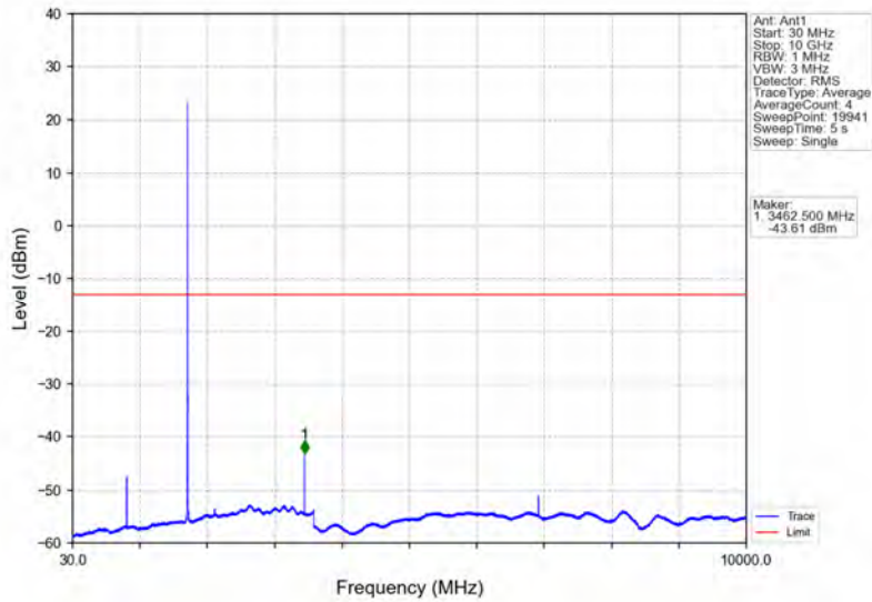
Band4_3MHz_QPSK_MCH_1732.5MHz_RB_1_0_NTNV
