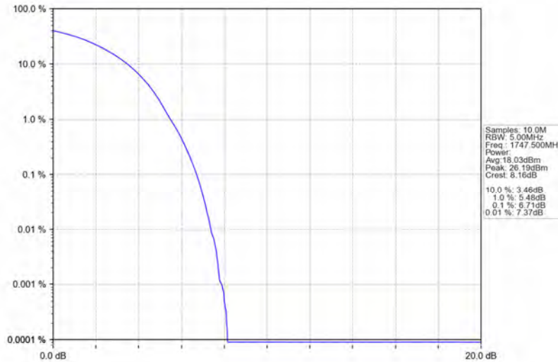
Band4_15MHz_QPSK_HCH_1747.5MHz_RB_75_0_NTNV
