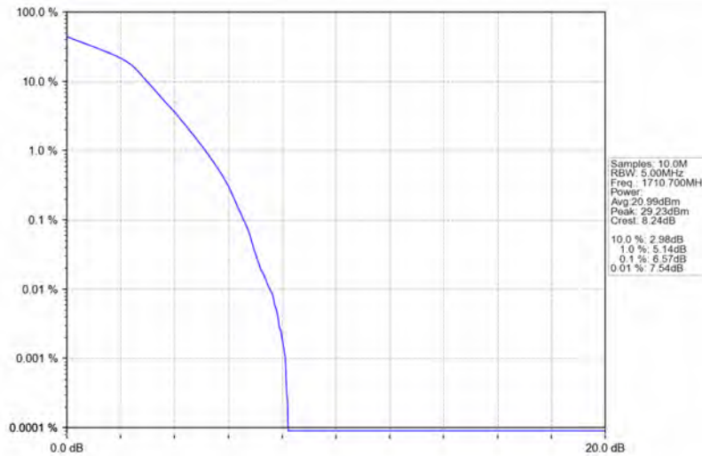
Band4_1.4MHz_16QAM_LCH_1710.7MHz_RB_6_0_NTNV
