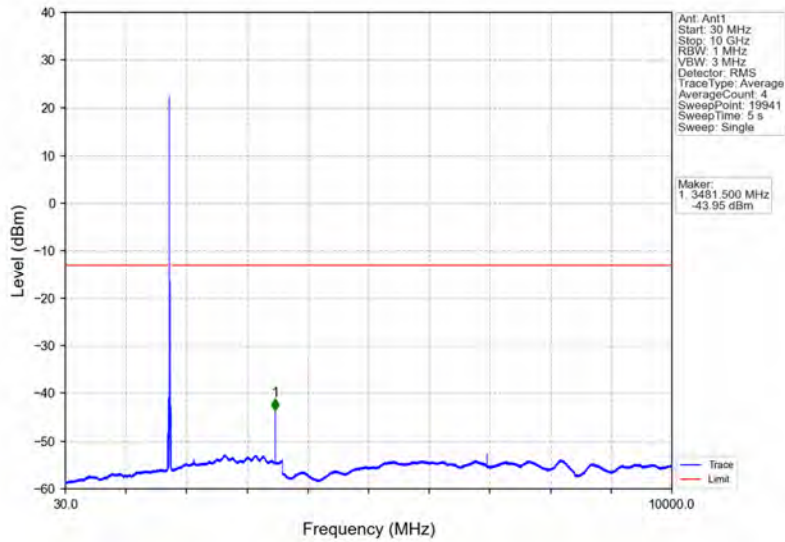
Band4_15MHz_16QAM_HCH_1747.5MHz_RB_1_0_NTNV
