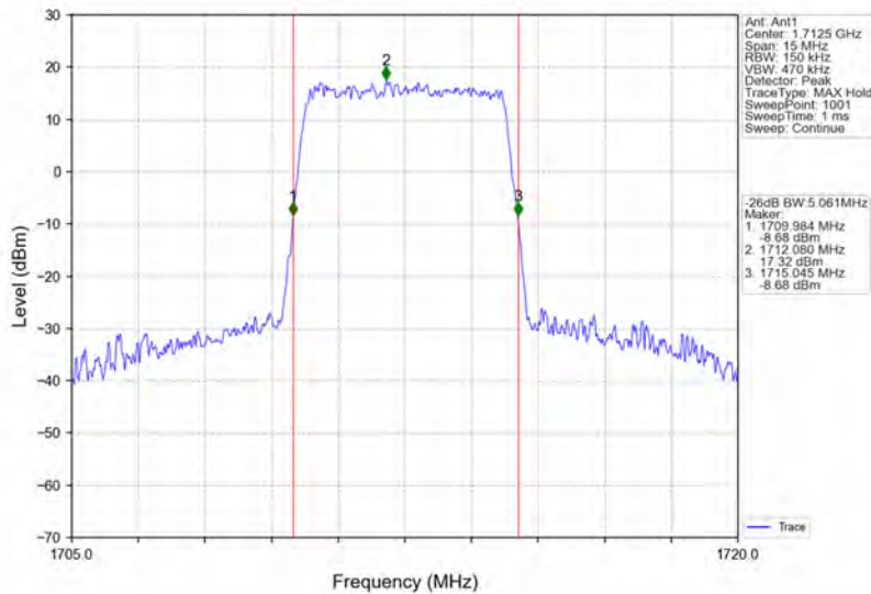
Band4_5MHz_16QAM_LCH_1712.5MHz_RB_25_0_NTNV
