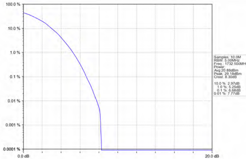
Band4_5MHz_64QAM_MCH_1732.5MHz_RB_25_0_NTNV
