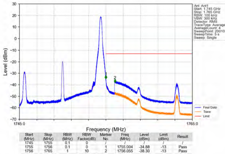
Band4_10MHz_64QAM_HCH_1750MHz_RB_1_49_NTNV
