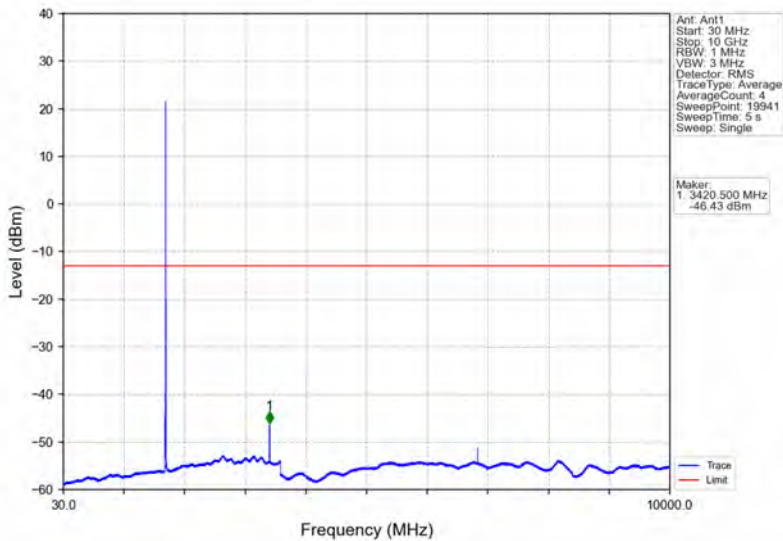
Band4_5MHz_16QAM_LCH_1712.5MHz_RB_1_0_NTNV
