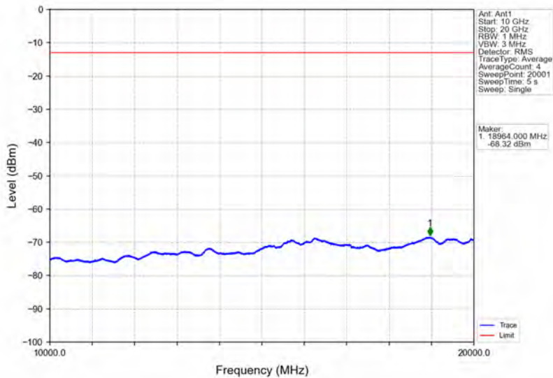
Band4_3MHz_64QAM_HCH_1753.5MHz_RB_1_0_NTNV
