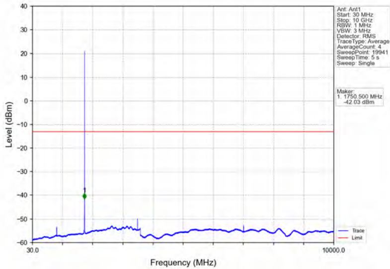
Band4_1.4MHz_16QAM_HCH_1754.3MHz_RB_1_0_NTNV
