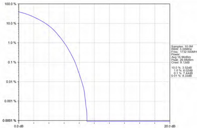
Band4_15MHz_64QAM_MCH_1732.5MHz_RB_75_0_NTNV
