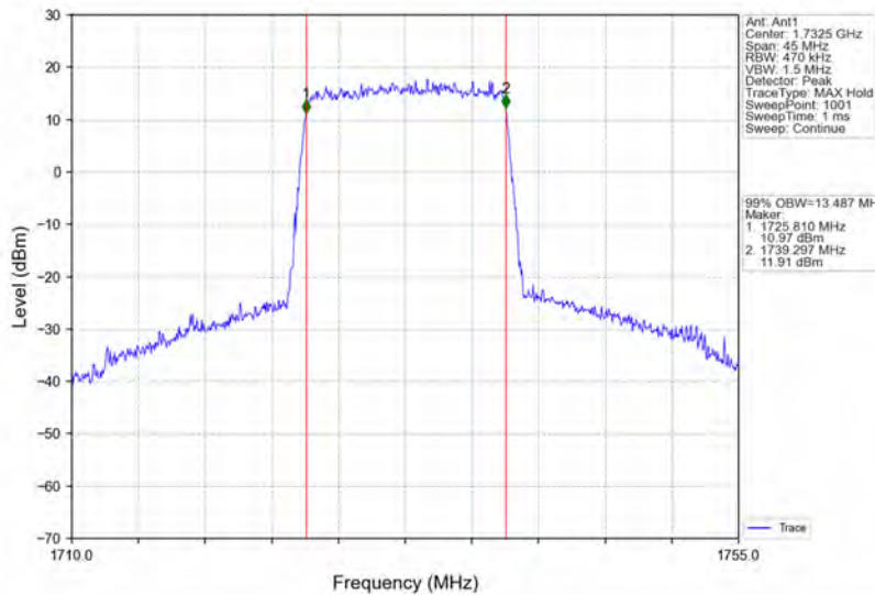
Band4_15MHz_64QAM_MCH_1732.5MHz_RB_75_0_NTNV
