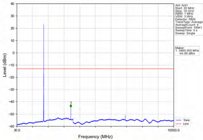
Band4_5MHz_QPSK_MCH_1732.5MHz_RB_1_0_NTNV
