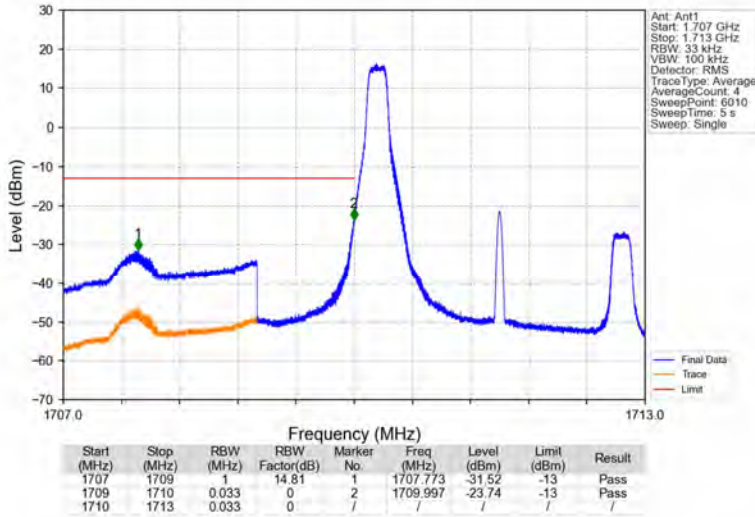
Band4_3MHz_16QAM_LCH_1711.5MHz_RB_1_0_NTNV
