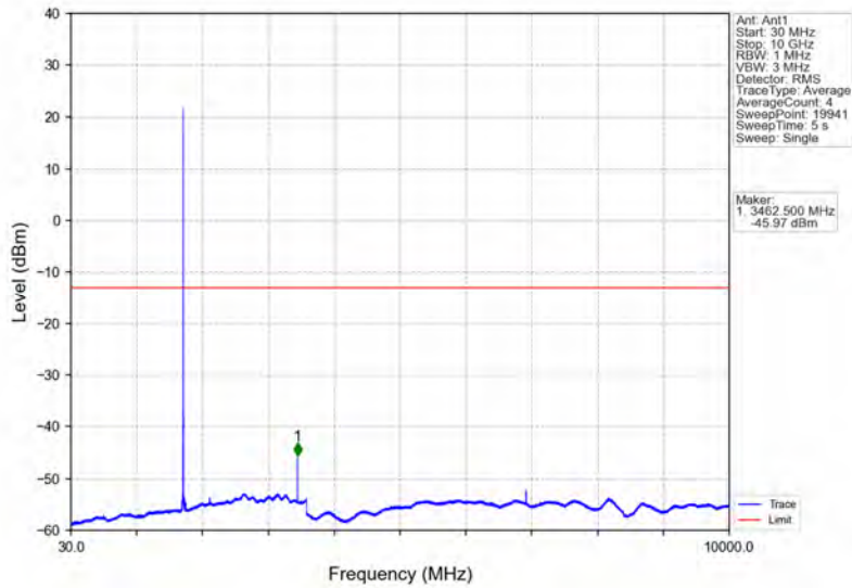
Band4_3MHz_64QAM_MCH_1732.5MHz_RB_1_0_NTNV
