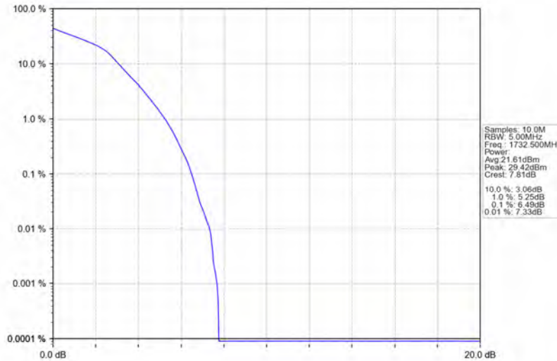
Band4_1.4MHz_16QAM_MCH_1732.5MHz_RB_6_0_NTNV
