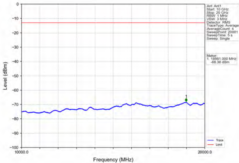
Band4_15MHz_64QAM_MCH_1732.5MHz_RB_1_0_NTNV
