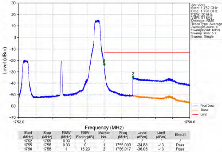
Band4_3MHz_16QAM_HCH_1753.5MHz_RB_1_14_NTNV
