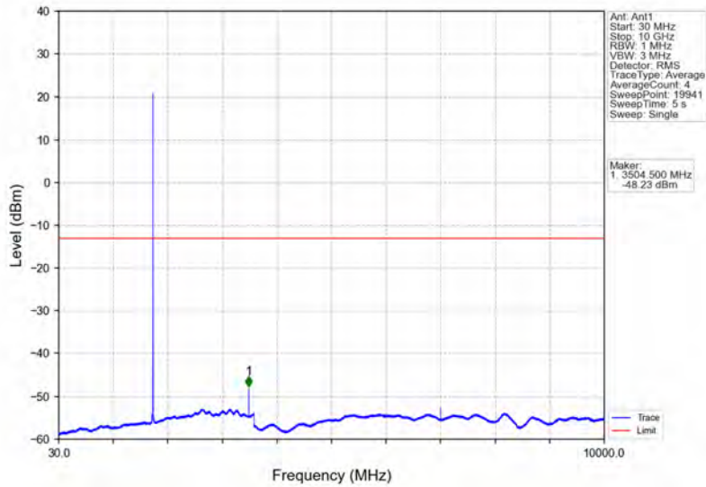
Band4_3MHz_16QAM_HCH_1753.5MHz_RB_1_0_NTNV
