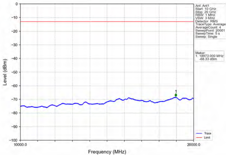
Band4_1.4MHz_64QAM_HCH_1754.3MHz_RB_1_0_NTNV
