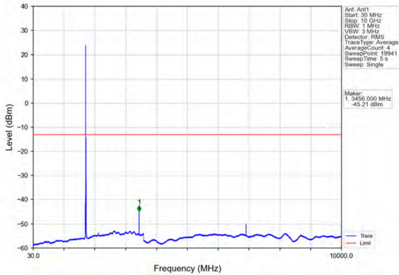
Band4_10MHz_QPSK_MCH_1732.5MHz_RB_1_0_NTNV
