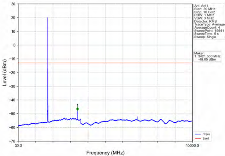
Band4_15MHz_64QAM_LCH_1717.5MHz_RB_1_0_NTNV
