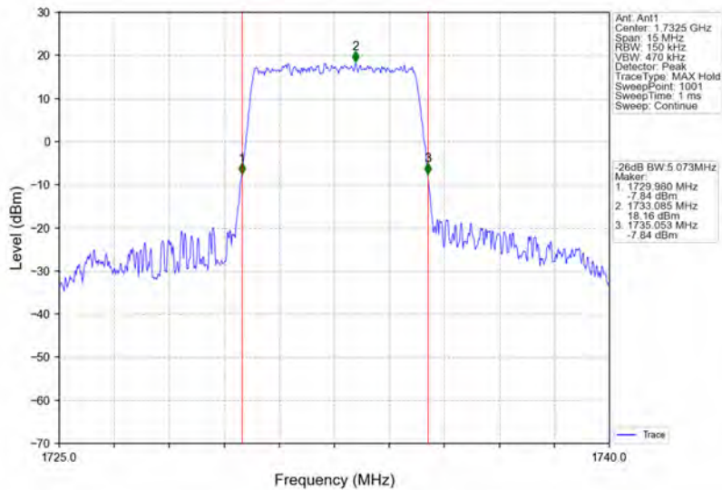
Band4_5MHz_QPSK_MCH_1732.5MHz_RB_25_0_NTNV
