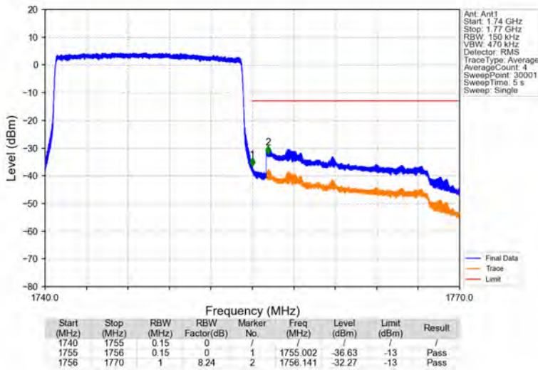
Band4_15MHz_QPSK_HCH_1747.5MHz_RB_75_0_NTNV
