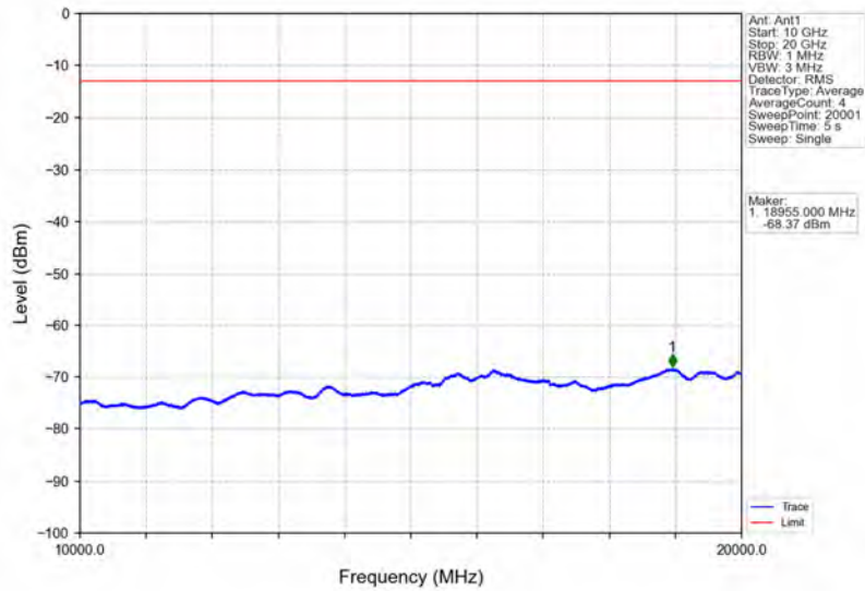
Band4_15MHz_QPSK_LCH_1717.5MHz_RB_75_0_NTNV
