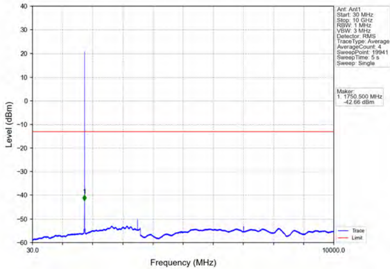
Band4_1.4MHz_64QAM_HCH_1754.3MHz_RB_1_0_NTNV
