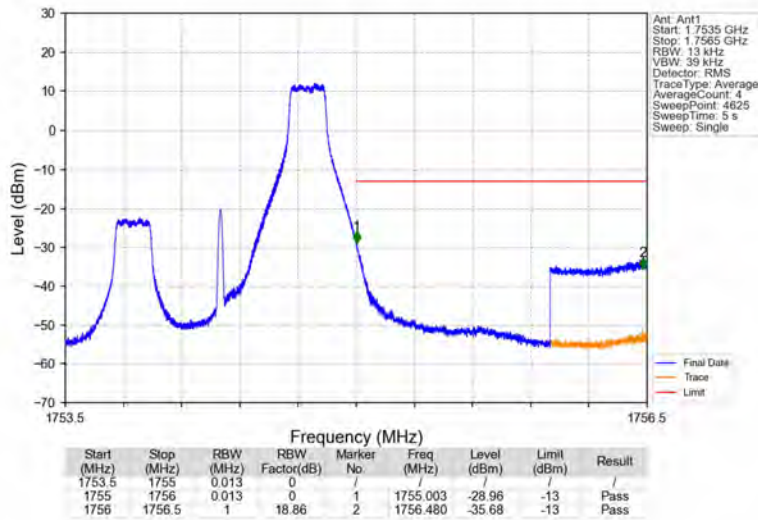
Band4_1.4MHz_16QAM_HCH_1754.3MHz_RB_1_5_NTNV
