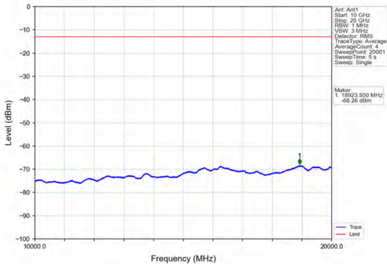
Band4_3MHz_QPSK_MCH_1732.5MHz_RB_1_0_NTNV
