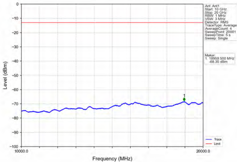
Band4_3MHz_16QAM_MCH_1732.5MHz_RB_1_0_NTNV
