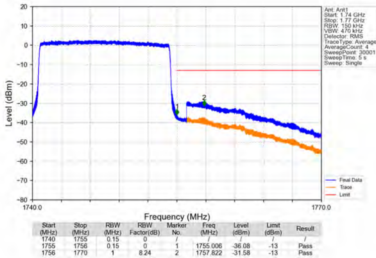
Band4_15MHz_64QAM_HCH_1747.5MHz_RB_75_0_NTNV
