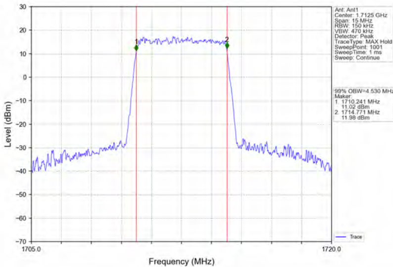
Band4_5MHz_16QAM_LCH_1712.5MHz_RB_25_0_NTNV
