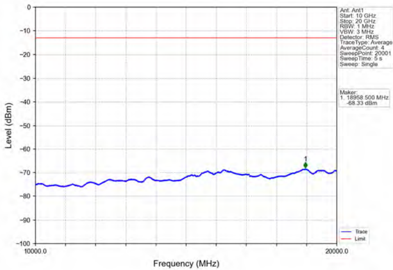
Band4_3MHz_QPSK_LCH_1711.5MHz_RB_15_0_NTNV
