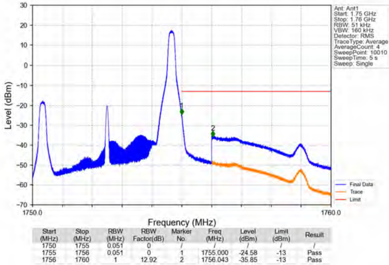
Band4_5MHz_16QAM_HCH_1752.5MHz_RB_1_24_NTNV
