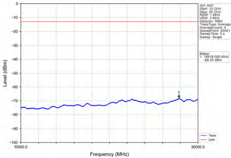
Band4_5MHz_64QAM_LCH_1712.5MHz_RB_25_0_NTNV
