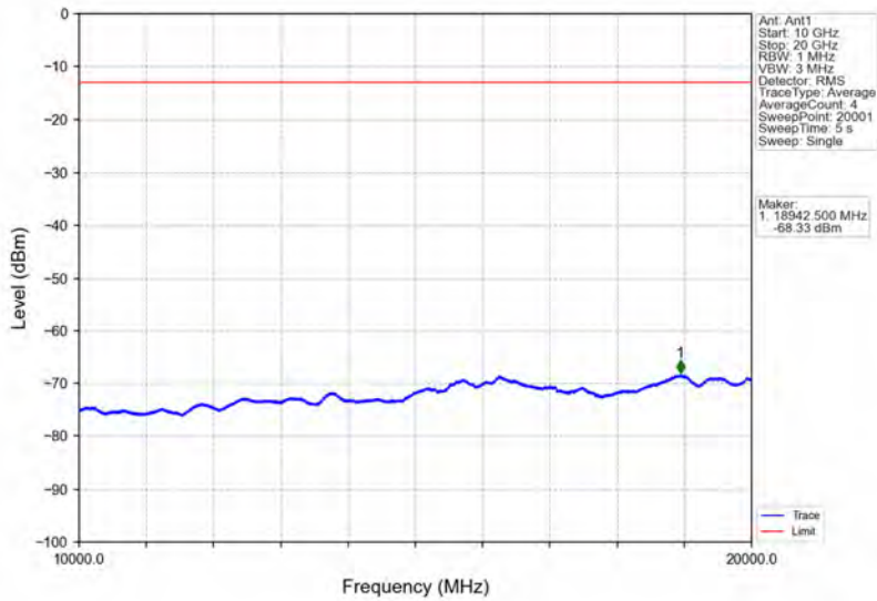
Band4_3MHz_16QAM_LCH_1711.5MHz_RB_15_0_NTNV
