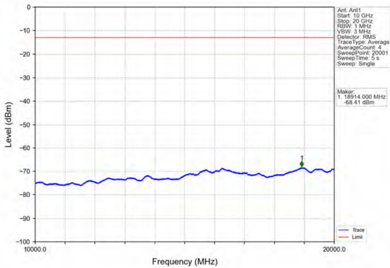
Band4_10MHz_16QAM_LCH_1715MHz_RB_50_0_NTNV
