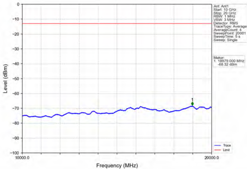
Band4_5MHz_QPSK_MCH_1732.5MHz_RB_1_0_NTNV
