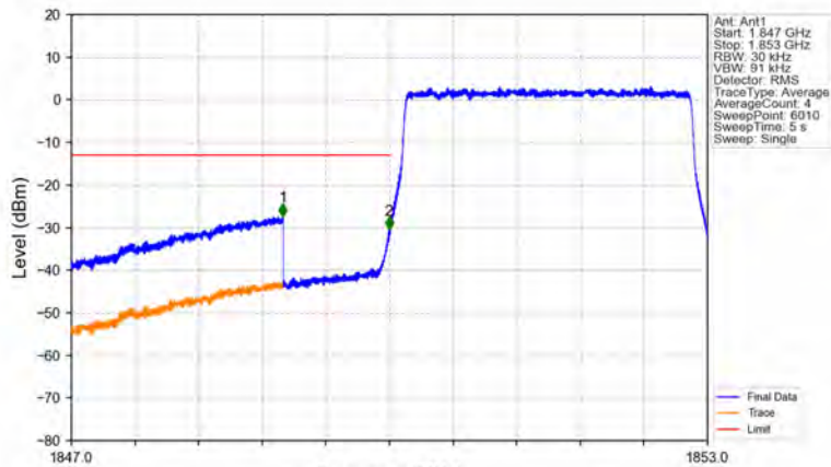
Band2_3MHz_16QAM_LCH_1851.5MHz_RB_15_0_NTNV
