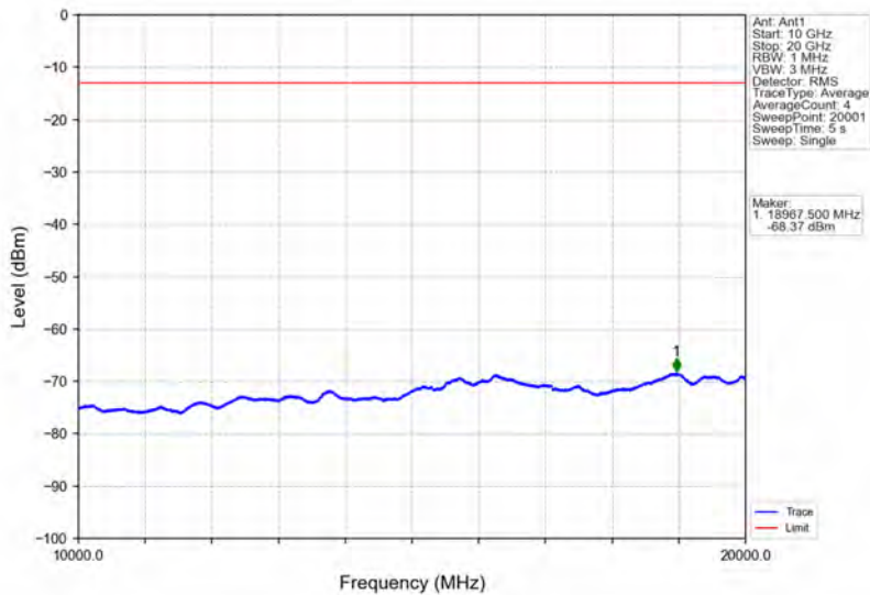
Band2_10MHz_64QAM_MCH_1880MHz_RB_1_0_NTNV
