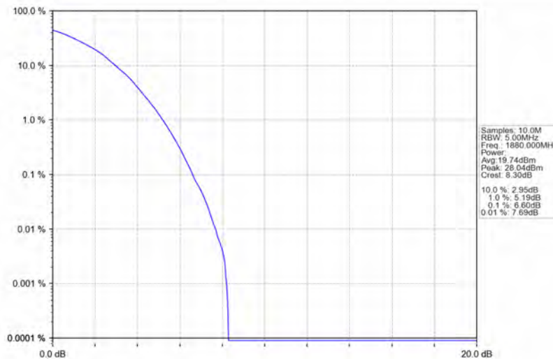
Band2_5MHz_64QAM_MCH_1880MHz_RB_25_0_NTNV
