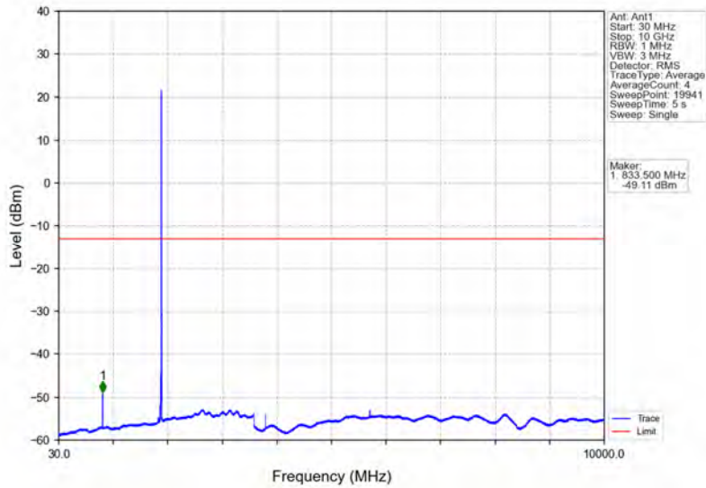
Band2_5MHz_16QAM_HCH_1907.5MHz_RB_1_0_NTNV
