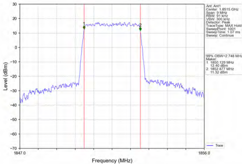
Band2_3MHz_QPSK_LCH_1851.5MHz_RB_15_0_NTNV
