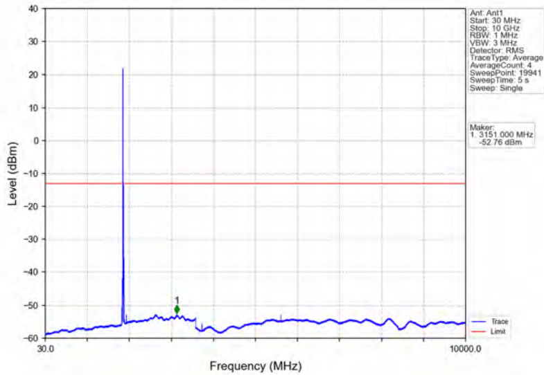
Band2_15MHz_16QAM_MCH_1880MHz_RB_1_0_NTNV
