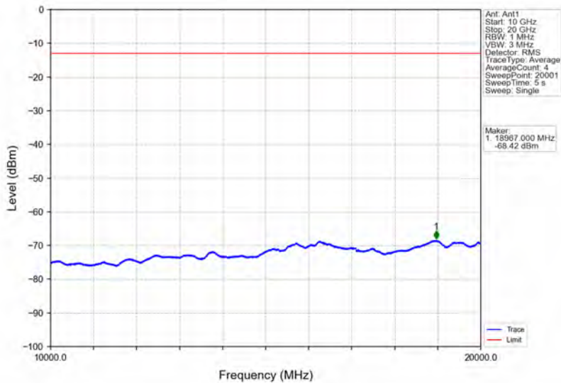
Band2_1.4MHz_64QAM_MCH_1880MHz_RB_1_0_NTNV
