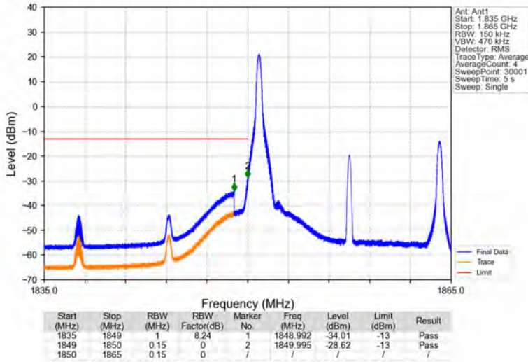
Band2_15MHz_16QAM_LCH_1857.5MHz_RB_1_0_NTNV
