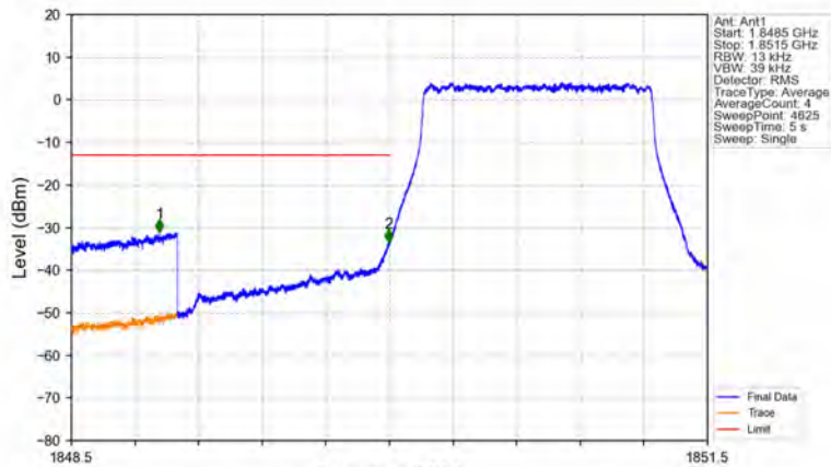
Band2_1.4MHz_QPSK_LCH_1850.7MHz_RB_6_0_NTNV
