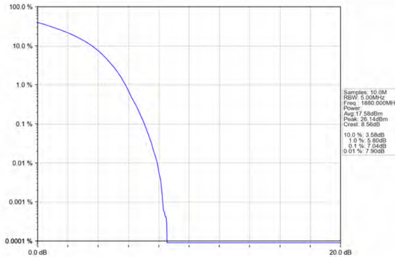
Band2_10MHz_64QAM_MCH_1880MHz_RB_50_0_NTNV
