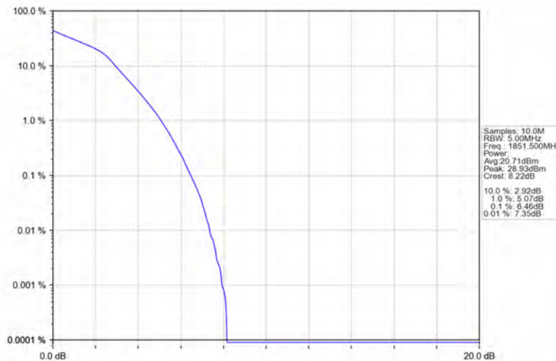
Band2_3MHz_16QAM_LCH_1851.5MHz_RB_15_0_NTNV
