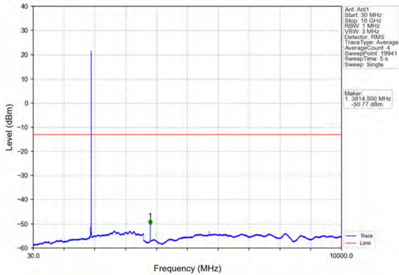
Band2_3MHz_16QAM_HCH_1908.5MHz_RB_1_0_NTNV
