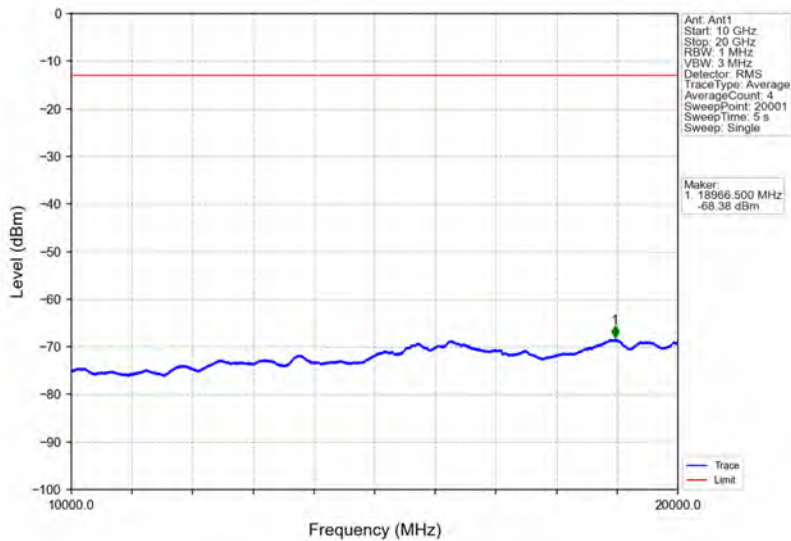
Band2_20MHz_64QAM_HCH_1900MHz_RB_1_0_NTNV
