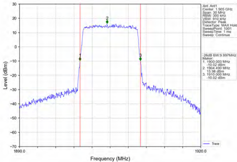
Band2_10MHz_64QAM_HCH_1905MHz_RB_50_0_NTNV
