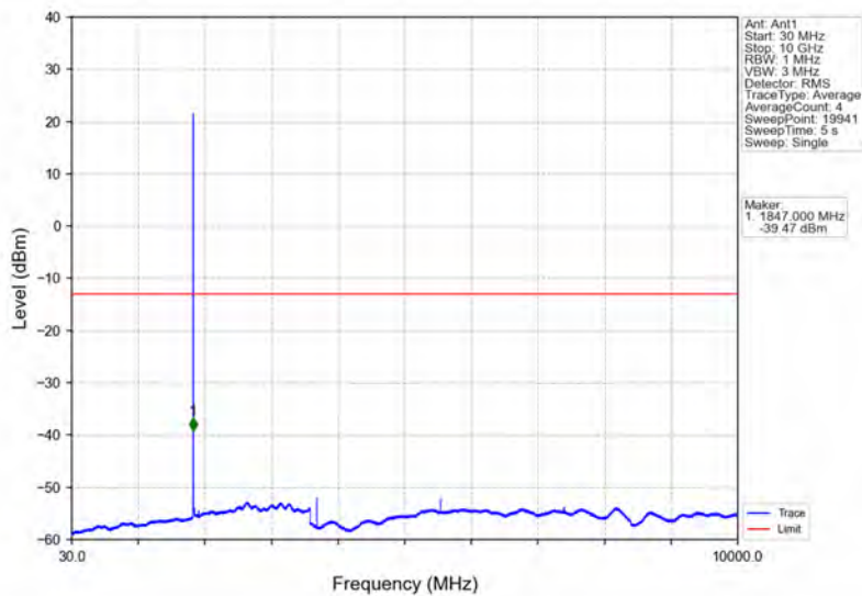
Band2_1.4MHz_16QAM_LCH_1850.7MHz_RB_1_0_NTNV
