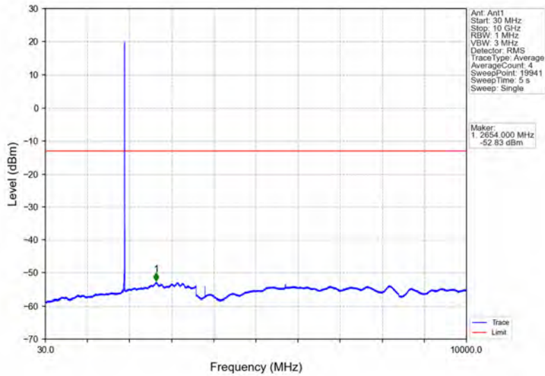
Band2_5MHz_64QAM_HCH_1907.5MHz_RB_1_0_NTNV
