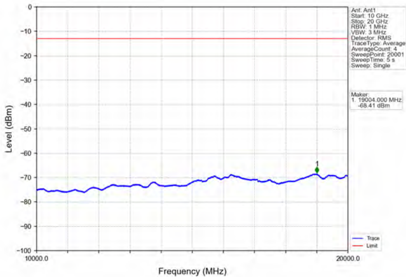
Band2_15MHz_64QAM_HCH_1902.5MHz_RB_1_0_NTNV
