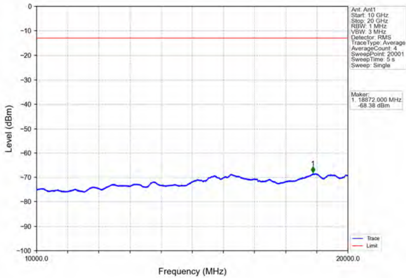
Band2_3MHz_16QAM_LCH_1851.5MHz_RB_15_0_NTNV
