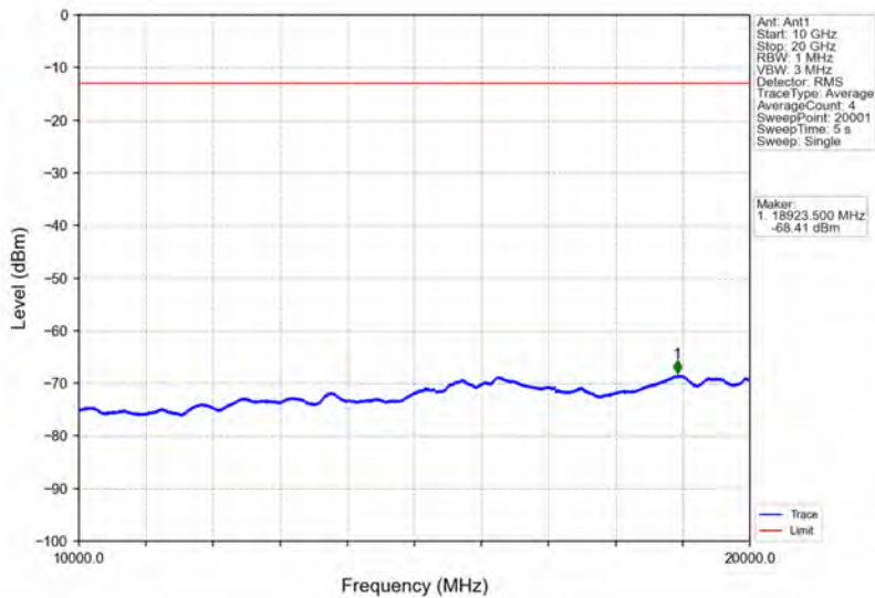
Band2_1.4MHz_16QAM_HCH_1909.3MHz_RB_1_0_NTNV
