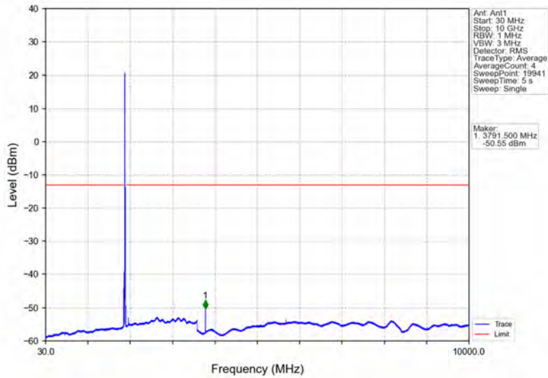
Band2_15MHz_64QAM_HCH_1902.5MHz_RB_1_0_NTNV
