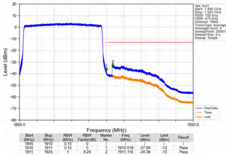
Band2_15MHz_16QAM_HCH_1902.5MHz_RB_75_0_NTNV
