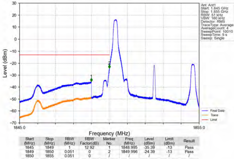
Band2_5MHz_64QAM_LCH_1852.5MHz_RB_1_0_NTNV
