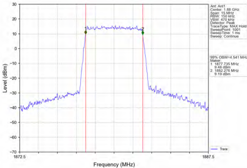
Band2_5MHz_64QAM_MCH_1880MHz_RB_25_0_NTNV
