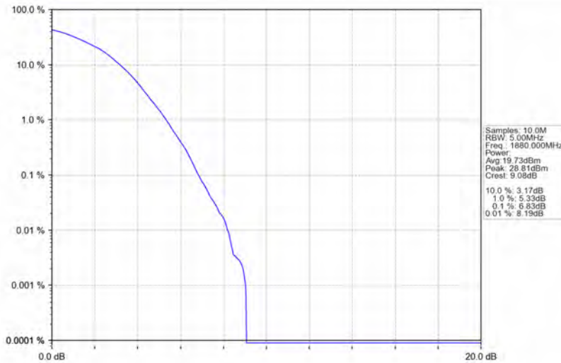
Band2_1.4MHz_64QAM_MCH_1880MHz_RB_6_0_NTNV
