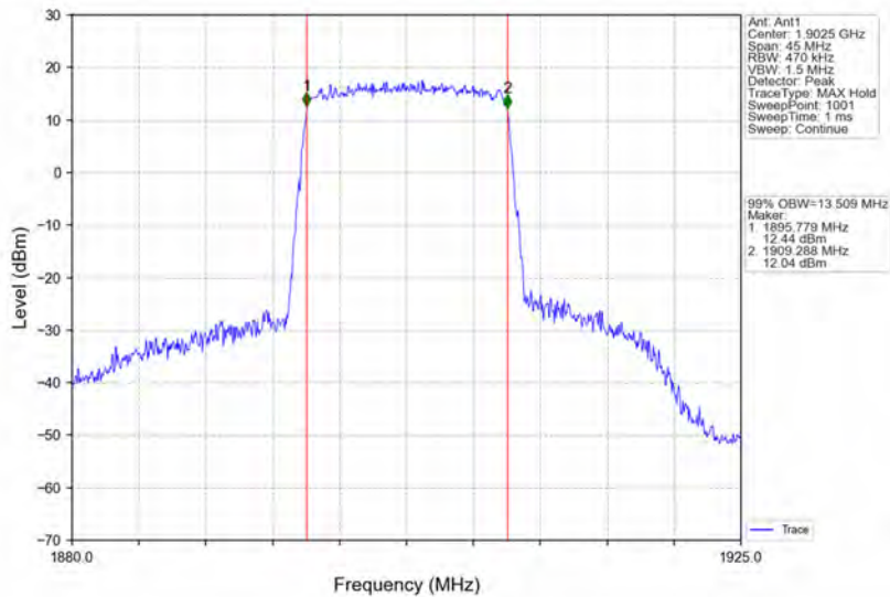
Band2_15MHz_16QAM_HCH_1902.5MHz_RB_75_0_NTNV
