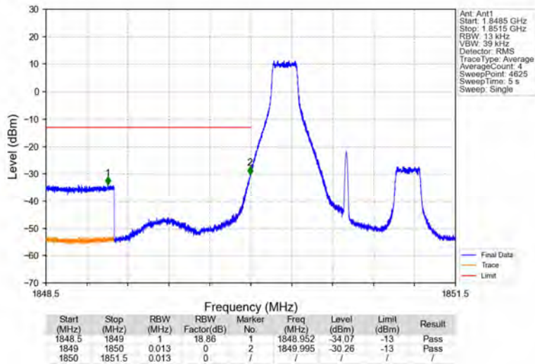
Band2_1.4MHz_64QAM_LCH_1850.7MHz_RB_1_0_NTNV
