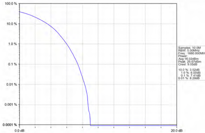
Band2_15MHz_64QAM_MCH_1880MHz_RB_75_0_NTNV
