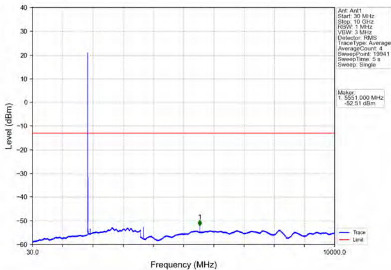
Band2_5MHz_16QAM_LCH_1852.5MHz_RB_1_0_NTNV
