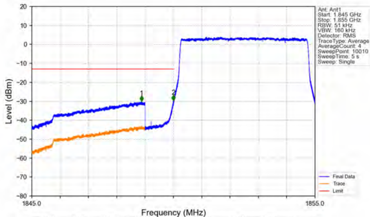
Band2_5MHz_QPSK_LCH_1852.5MHz_RB_25_0_NTNV
