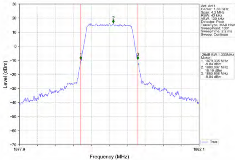
Band2_1.4MHz_64QAM_MCH_1880MHz_RB_6_0_NTNV
