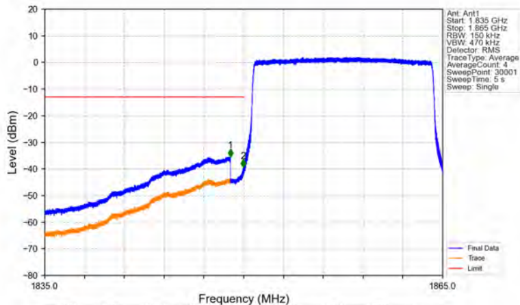
Band2_15MHz_64QAM_LCH_1857.5MHz_RB_75_0_NTNV
