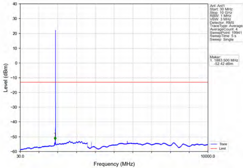
Band2_5MHz_QPSK_HCH_1907.5MHz_RB_1_0_NTNV
