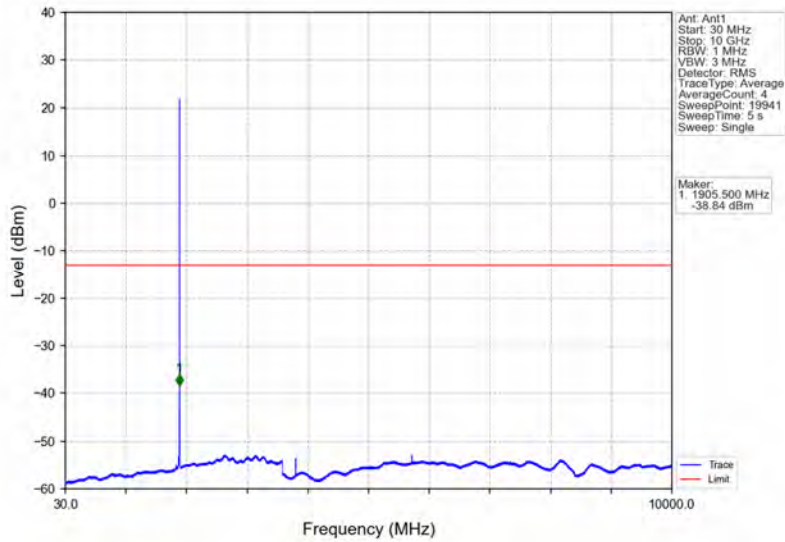
Band2_1.4MHz_16QAM_HCH_1909.3MHz_RB_1_0_NTNV
