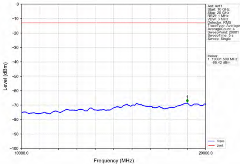
Band2_3MHz_16QAM_HCH_1908.5MHz_RB_1_0_NTNV
