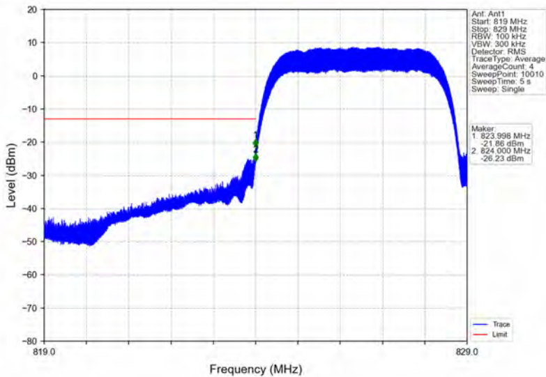
Band5_HSDPA_LCH_826.4MHz_Subtest 1_NTNV
