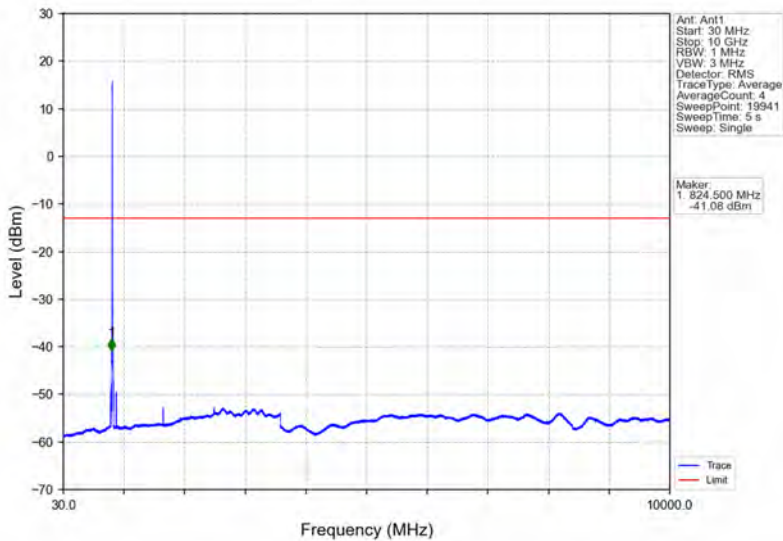
Band5_HSDPA_MCH_836.6MHz_Subtest 1_NTNV
