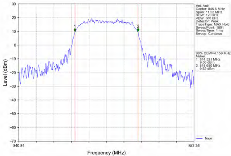
Band5_HSDPA_HCH_846.6MHz_Subtest 1_NTNV
