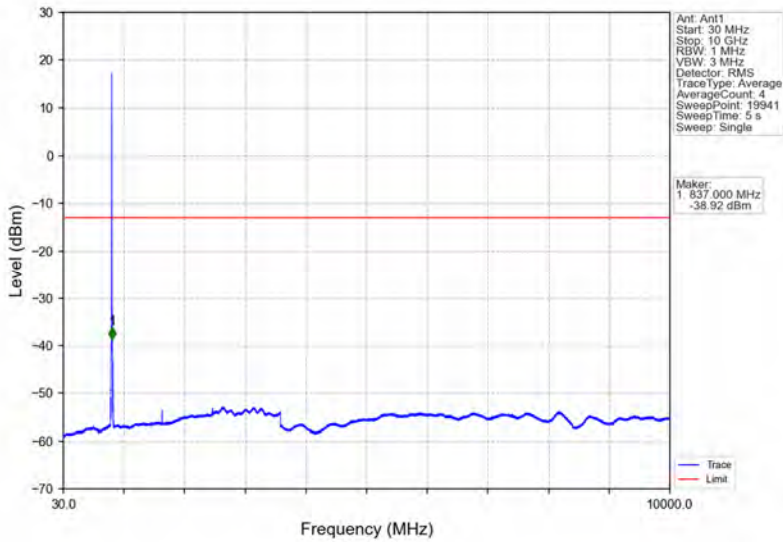
Band5_HSDPA_MCH_836.6MHz_Subtest 1_NTNV
