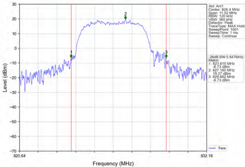
Band5_HSDPA_LCH_826.4MHz_Subtest 1_NTNV
