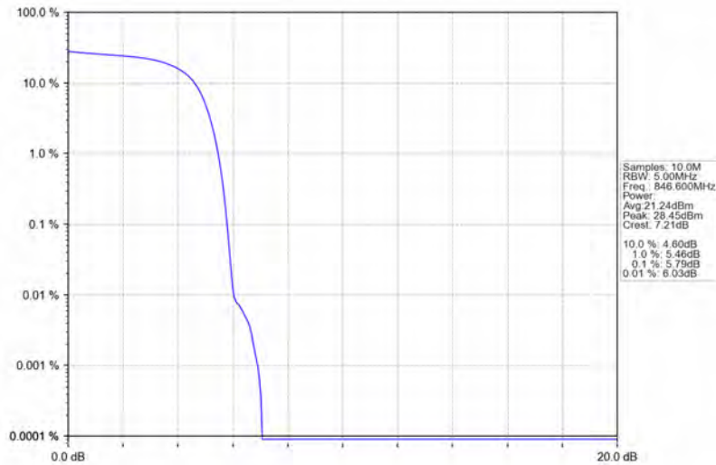
Band5_HSDPA_HCH_846.6MHz_Subtest 1_NTNV
