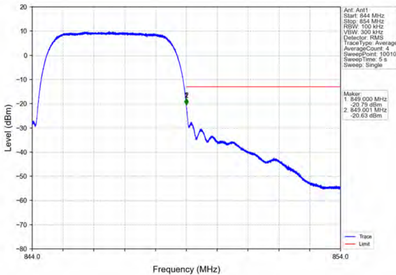
Band5_RMC_HCH_846.6MHz_12.2kbps RMC_NTNV
