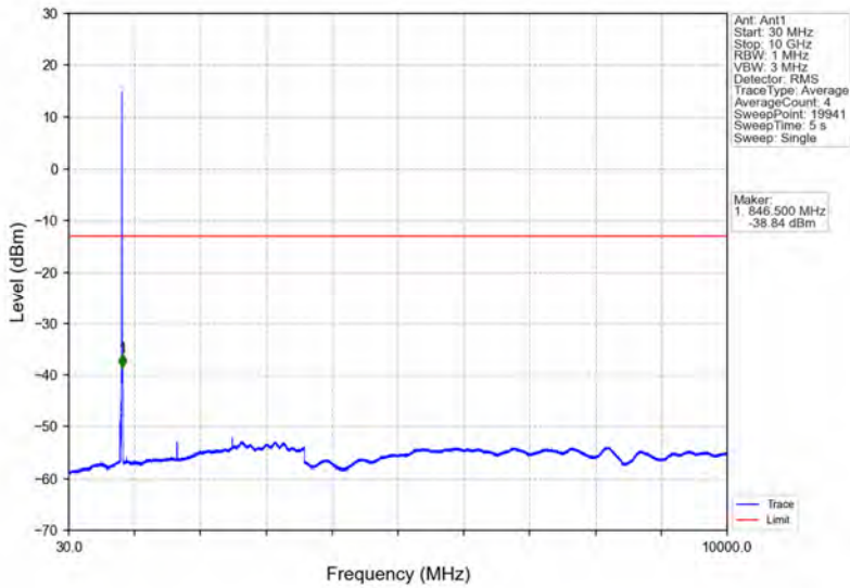
Band5_HSUPA_HCH_846.6MHz_Subtest 1_NTNV
