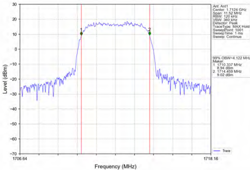
Band4_HSDPA_LCH_1712.4MHz_Subtest 1_NTNV
