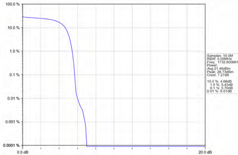
Band4_HSUPA_MCH_1732.6MHz_Subtest 1_NTNV
