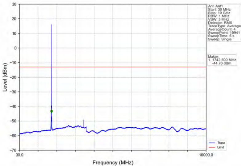
Band4_HSDPA_MCH_1732.6MHz_Subtest 1_NTNV
