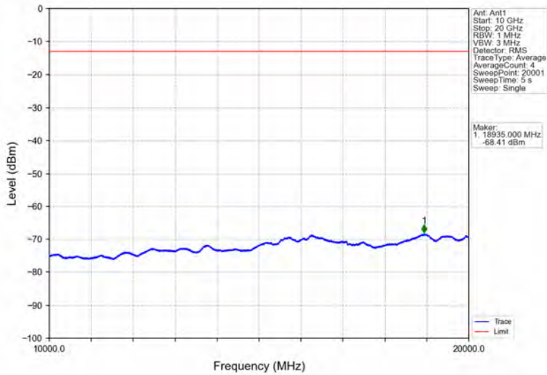
Band4_HSDPA_MCH_1732.6MHz_Subtest 1_NTNV
