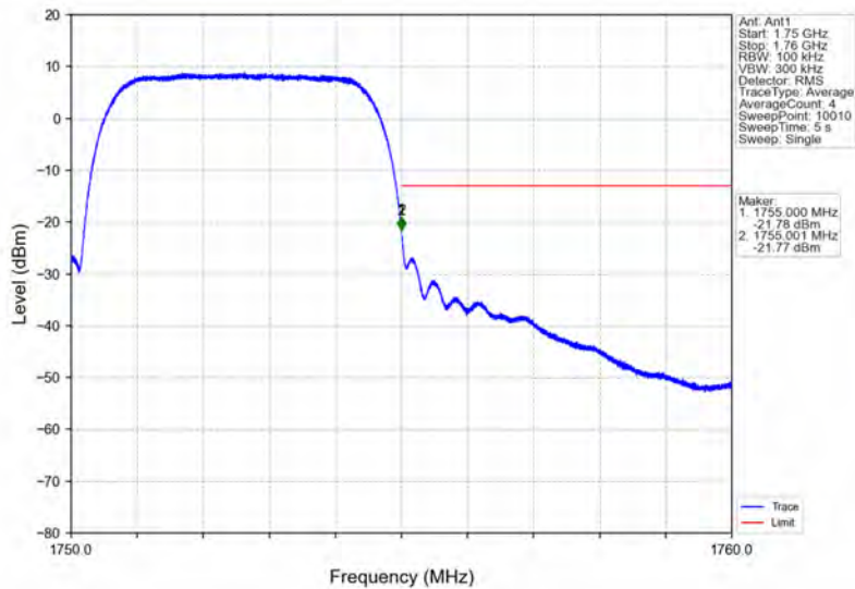
Band4_RMC_HCH_1752.6MHz_12.2kbps RMC_NTNV
