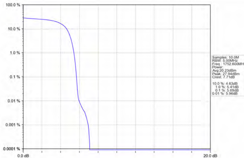
Band4_HSDPA_HCH_1752.6MHz_Subtest 1_NTNV
