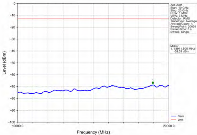
Band4_HSUPA_HCH_1752.6MHz_Subtest 1_NTNV
