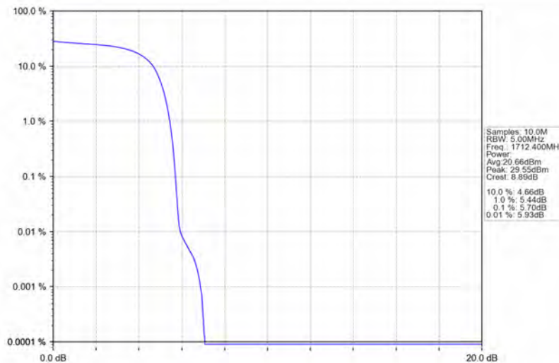
Band4_HSDPA_LCH_1712.4MHz_Subtest 1_NTNV
