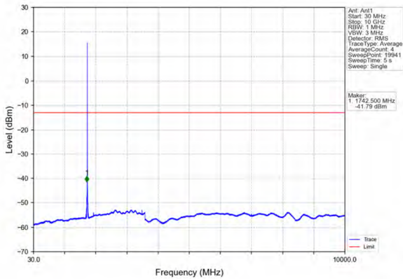
Band4_HSDPA_HCH_1752.6MHz_Subtest 1_NTNV
