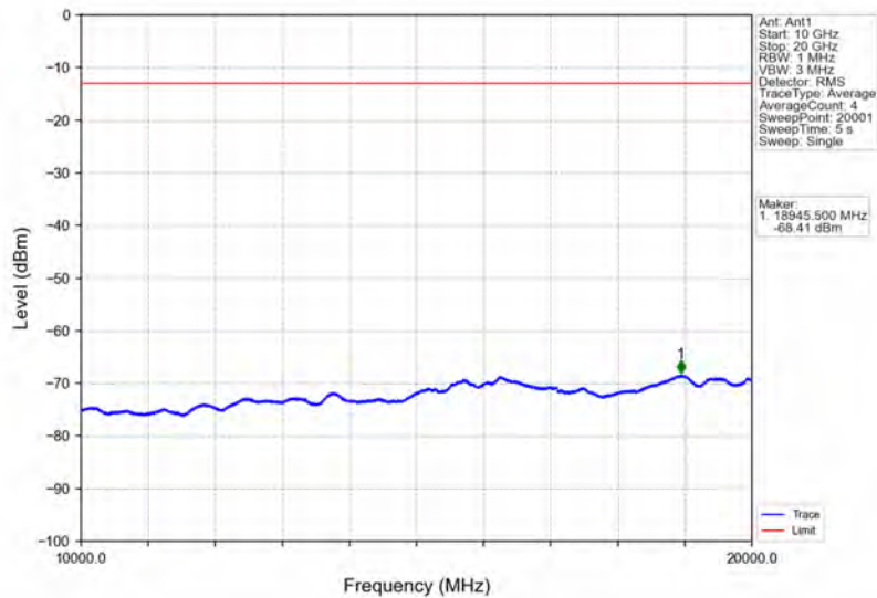
Band2_RMC_HCH_1907.6MHz_12.2kbps RMC_NTNV
