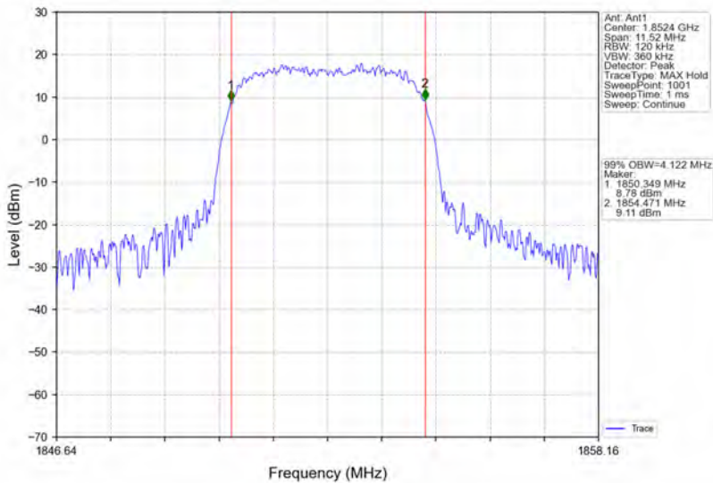
Band2_HSDPA_LCH_1852.4MHz_Subtest 1_NTNV
