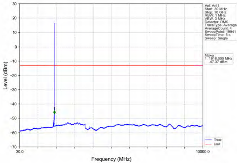
Band2_HSDPA_HCH_1907.6MHz_Subtest 1_NTNV
