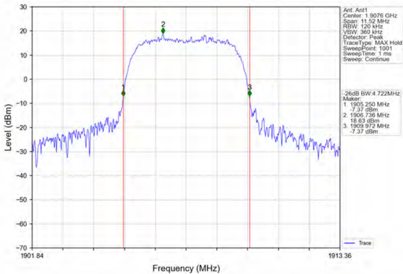
Band2_HSDPA_HCH_1907.6MHz_Subtest 1_NTNV
