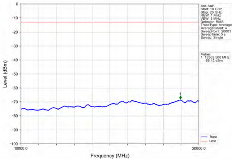
Band2_HSUPA_HCH_1907.6MHz_Subtest 1_NTNV
