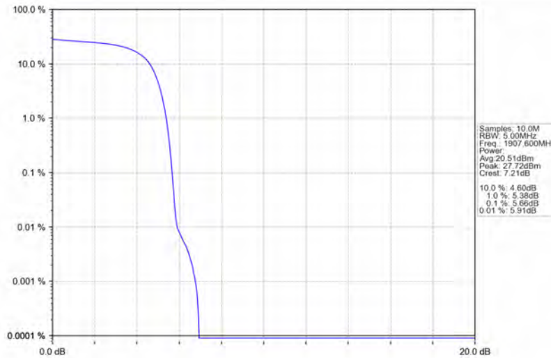
Band2_HSDPA_HCH_1907.6MHz_Subtest 1_NTNV
