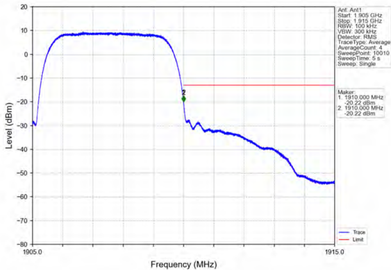
Band2_RMC_HCH_1907.6MHz_12.2kbps RMC_NTNV
