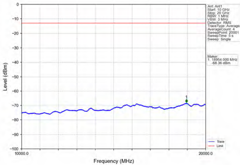
Band2_HSDPA_MCH_1880MHz_Subtest 1_NTNV
