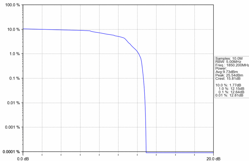
PCS1900_EGPRS_LCH_1850.2MHz_4 TX Slots_NTNV
