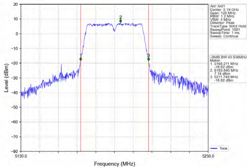
802.11ac(VHT40)_LCH_5190MHz_Ant1_NTNV
