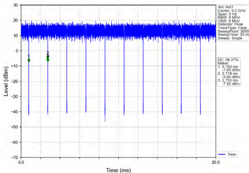
802.11n(HT20)_MCH_5200MHz_Ant1_NTNV
