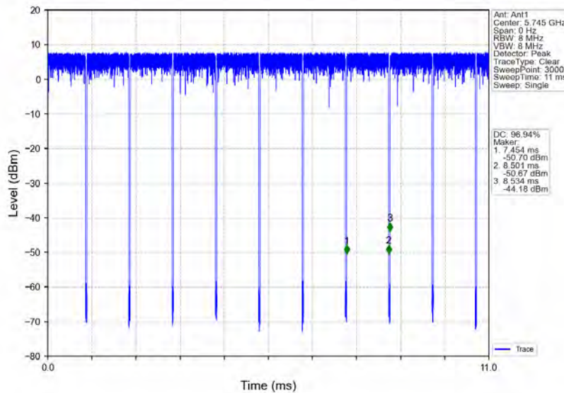
802.11a_LCH_5745MHz_Ant1_NTNV
