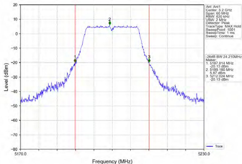
802.11ac(VHT20)_MCH_5200MHz_Ant1_NTNV
