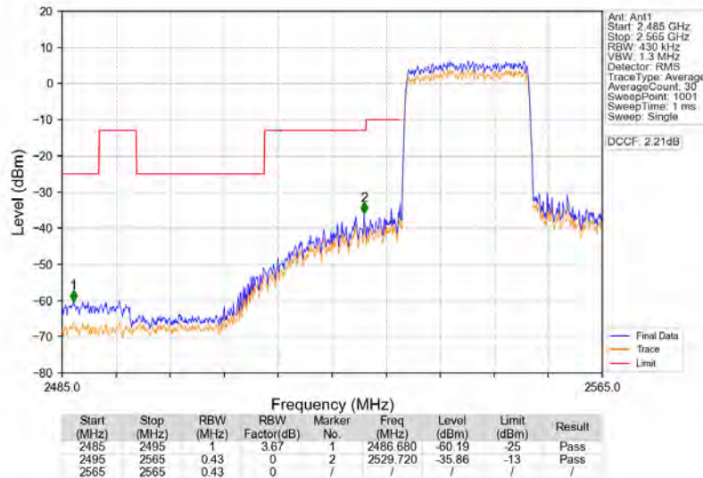
Band41_20MHz_16QAM_LCH_2545MHz_RB_100_0_NTNV
