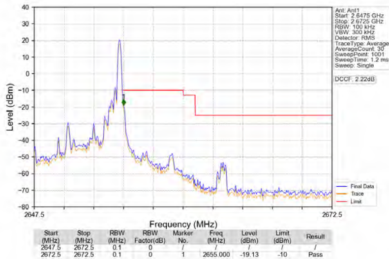
Band41_5MHz_16QAM_HCH_2652.5MHz_RB_1_24_NTNV
