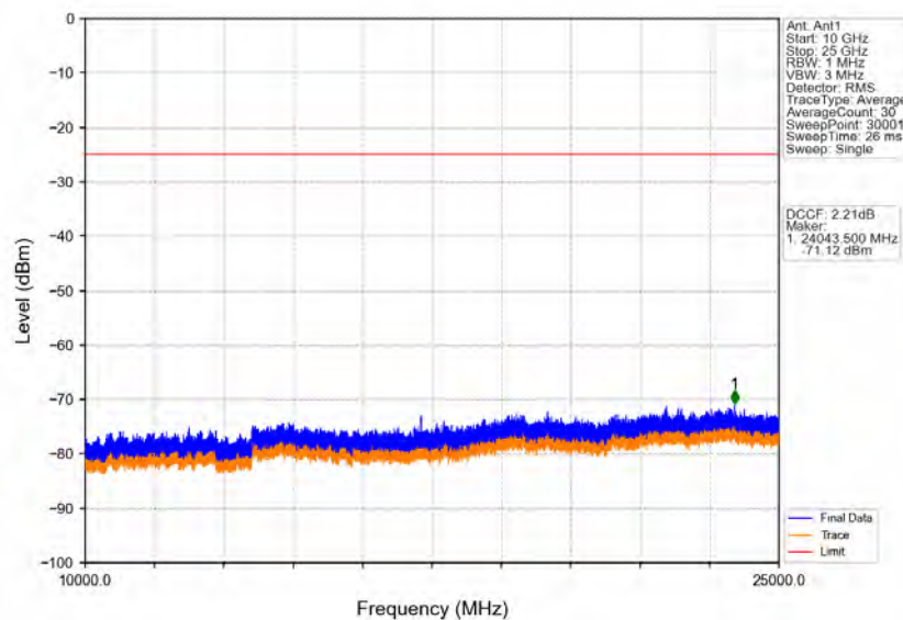
Band41_5MHz_16QAM_LCH_2537.5MHz_RB_1_0_NTNV
