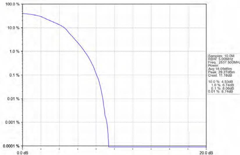
Band41_5MHz_16QAM_LCH_2537.5MHz_RB_25_0_NTNV
