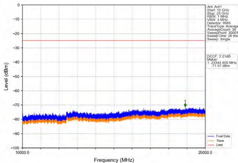
Band41_15MHz_16QAM_MCH_2595MHz_RB_1_0_NTNV
