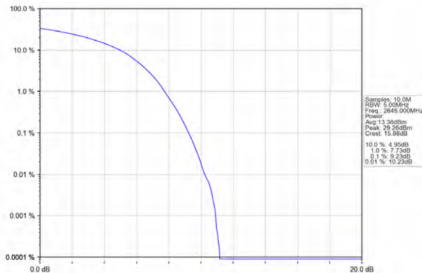
Band41_20MHz_16QAM_HCH_2645MHz_RB_100_0_NTNV
