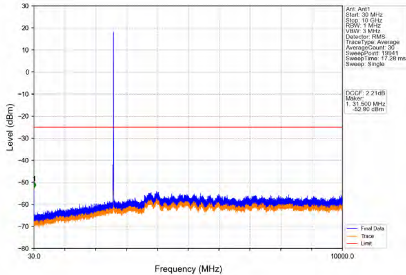
Band41_5MHz_16QAM_MCH_2595MHz_RB_1_0_NTNV
