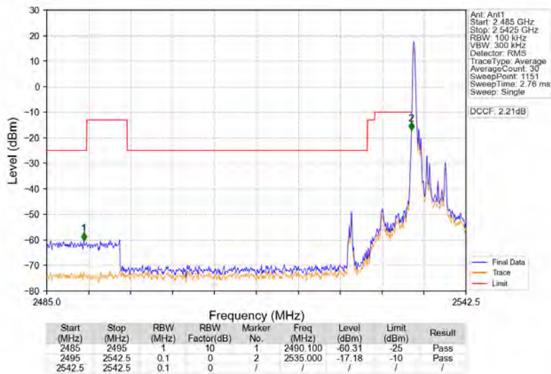
Band41_5MHz_16QAM_LCH_2537.5MHz_RB_1_0_NTNV
