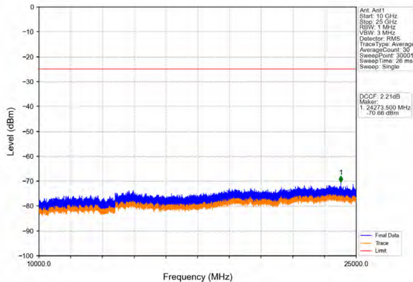
Band41_5MHz_16QAM_MCH_2595MHz_RB_1_0_NTNV
