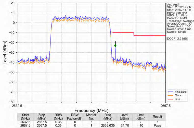
Band41_15MHz_16QAM_HCH_2647.5MHz_RB_75_0_NTNV
