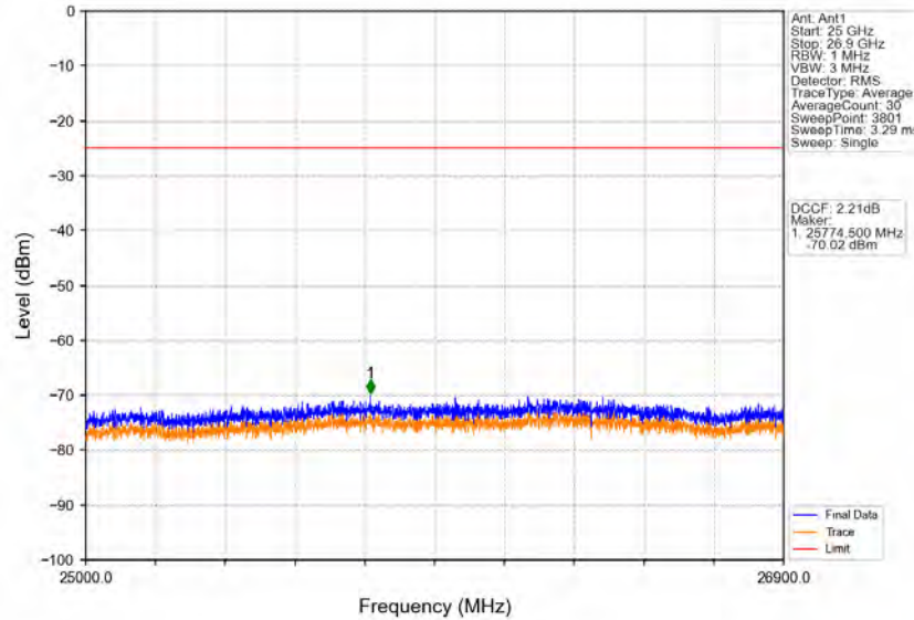
Band41_20MHz_16QAM_LCH_2545MHz_RB_100_0_NTNV
