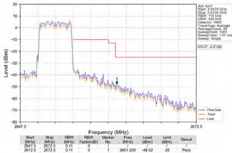
Band41_5MHz_16QAM_HCH_2652.5MHz_RB_25_0_NTNV
