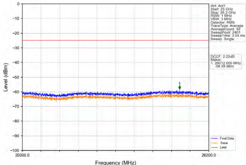
Band38_15MHz_16QAM_HCH_2612.5MHz_RB_1_0_NTNV
