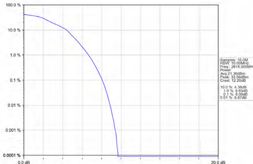
Band38_10MHz_16QAM_HCH_2615MHz_RB_50_0_NTNV
