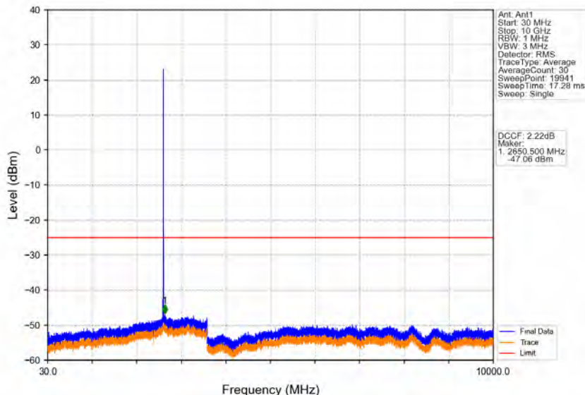
Band38_5MHz_16QAM_HCH_2617.5MHz_RB_1_0_NTNV
