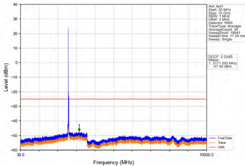
Band38_15MHz_16QAM_MCH_2595MHz_RB_1_0_NTNV
