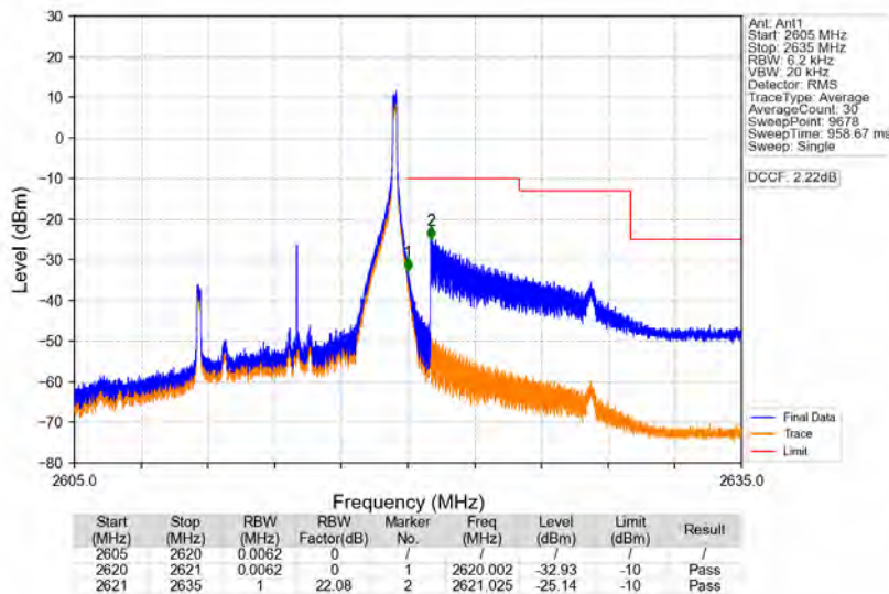
Band38_10MHz_16QAM_HCH_2615MHz_RB_1_49_NTNV
