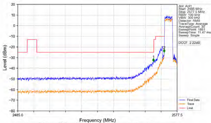
Band38_5MHz_16QAM_LCH_2572.5MHz_RB_25_0_NTNV
