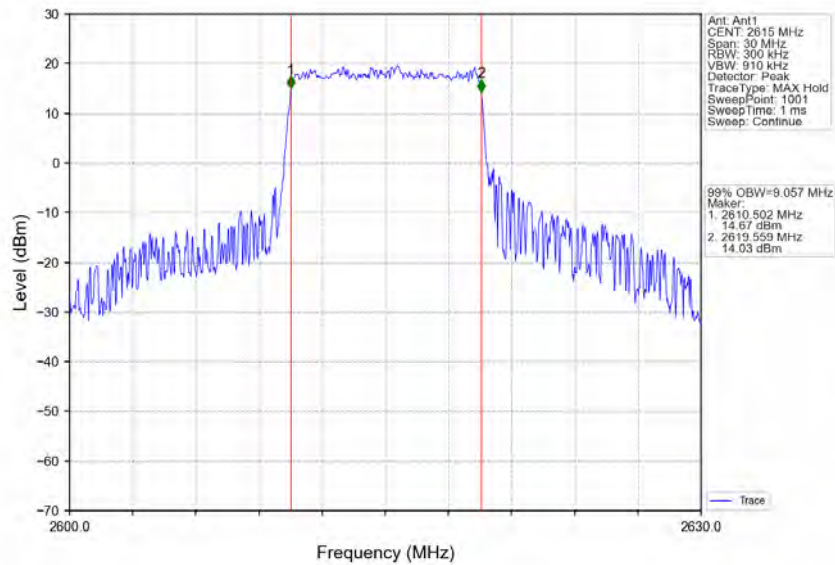
Band38_10MHz_16QAM_HCH_2615MHz_RB_50_0_NTNV
