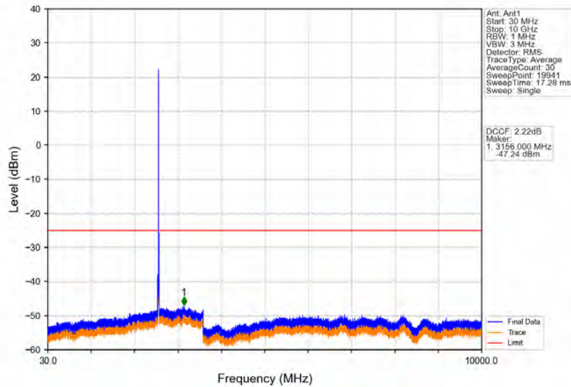
Band38_10MHz_16QAM_LCH_2575MHz_RB_1_0_NTV
