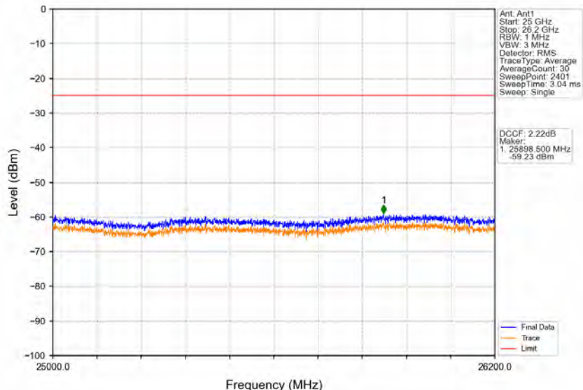
Band38_5MHz_16QAM_HCH_2617.5MHz_RB_1_0_NTNV
