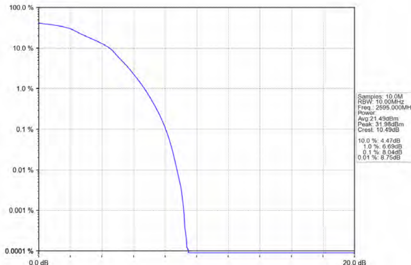
Band38_10MHz_16QAM_MCH_2595MHz_RB_50_0_NTNV
