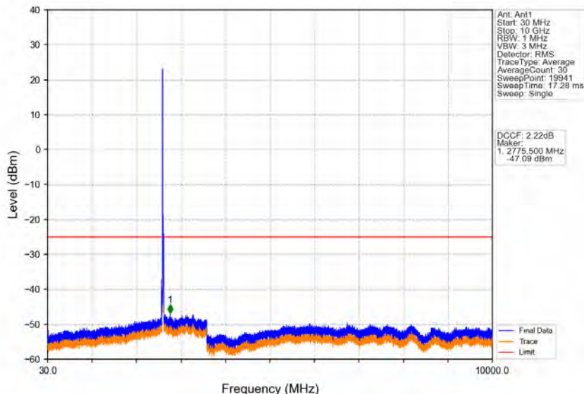
Band38_15MHz_16QAM_HCH_2612.5MHz_RB_1_0_NTNV
