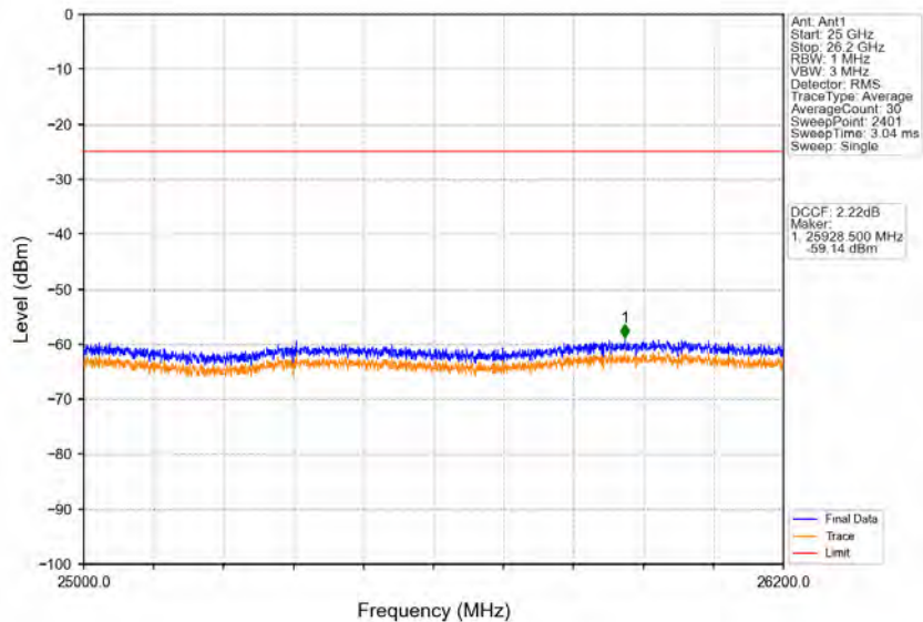
Band38_10MHz_16QAM_LCH_2575MHz_RB_50_0_NTNV
