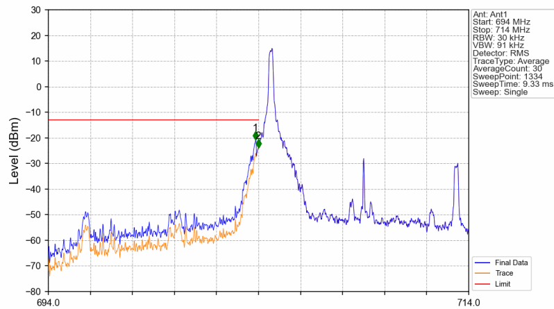
Band17_10MHz_16QAM_LCH_709MHz_RB_1_0_NTNV
