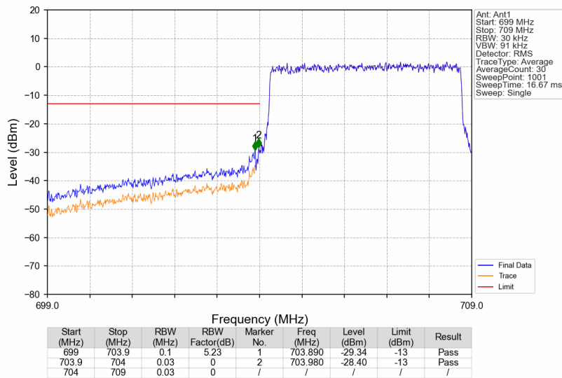
Band17_5MHz_QPSK_LCH_706.5MHz_RB_25_0_NTNV
