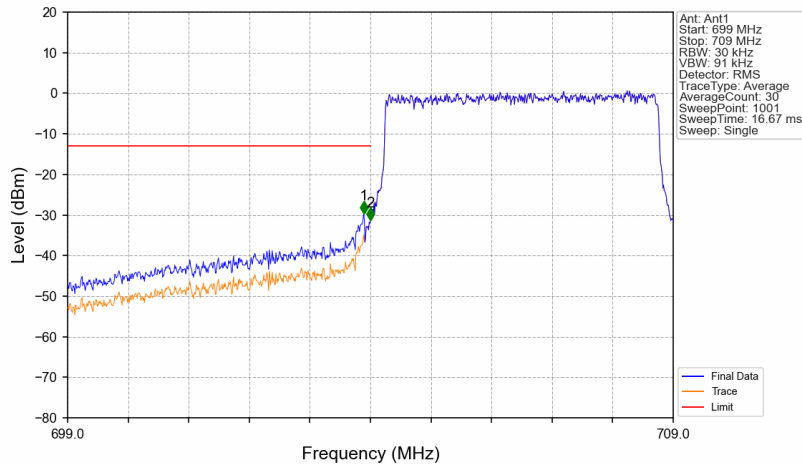
Band17_5MHz_16QAM_LCH_706.5MHz_RB_25_0_NTNV
