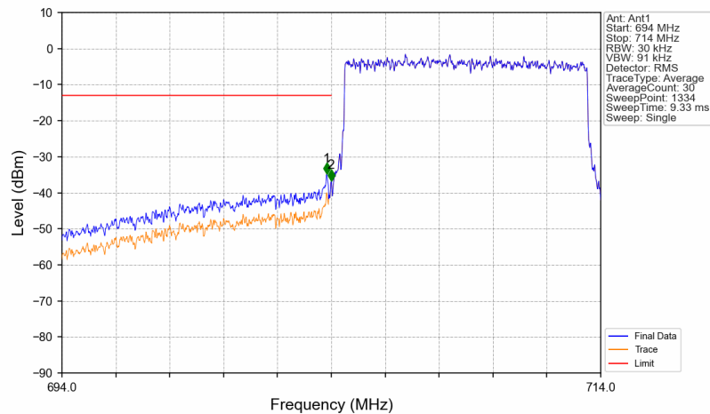
Band17_10MHz_16QAM_LCH_709MHz_RB_50_0_NTNV
