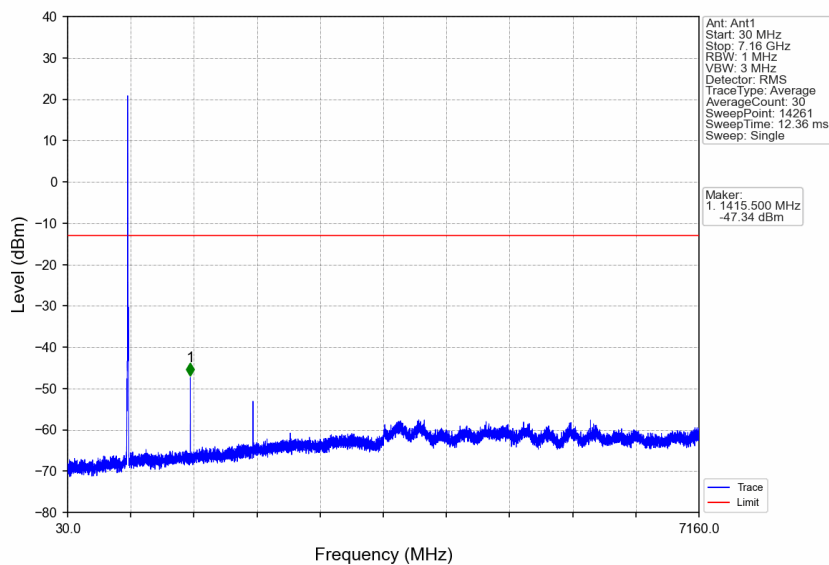
Band17_5MHz_QPSK_MCH_710MHz_RB_1_0_NTNV
