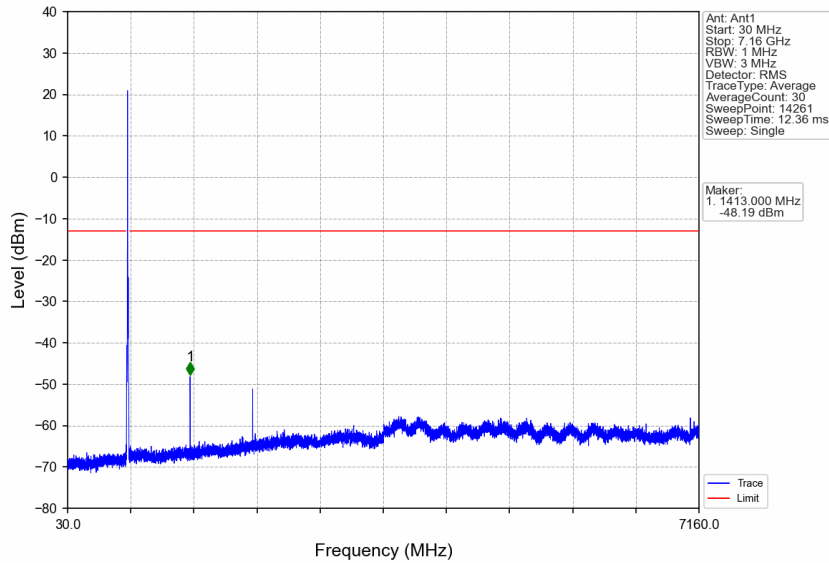
Band17_10MHz_QPSK_HCH_711MHz_RB_1_49_NTNV
