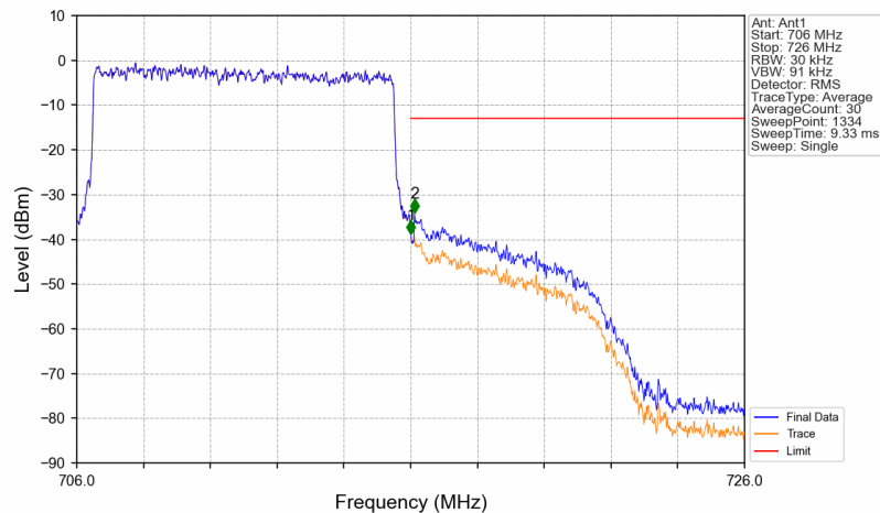
Band17_10MHz_QPSK_HCH_711MHz_RB_50_0_NTNV
