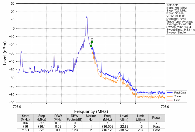
Band17_10MHz_16QAM_HCH_711MHz_RB_1_49_NTNV
