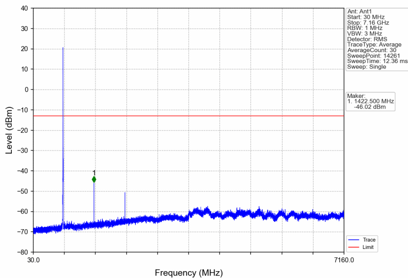
Band17_5MHz_16QAM_HCH_713.5MHz_RB_1_0_NTNV
