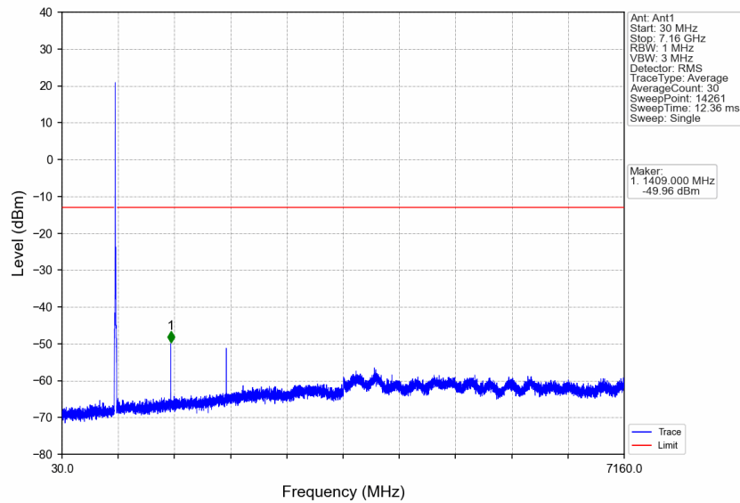
Band17_10MHz_16QAM_LCH_709MHz_RB_50_0_NTNV
