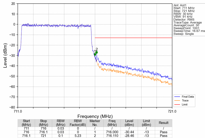
Band17_5MHz_16QAM_HCH_713.5MHz_RB_25_0_NTNV
