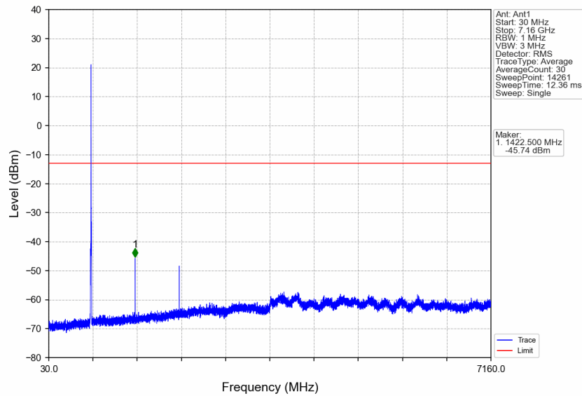
Band17_5MHz_QPSK_HCH_713.5MHz_RB_1_24_NTNV
