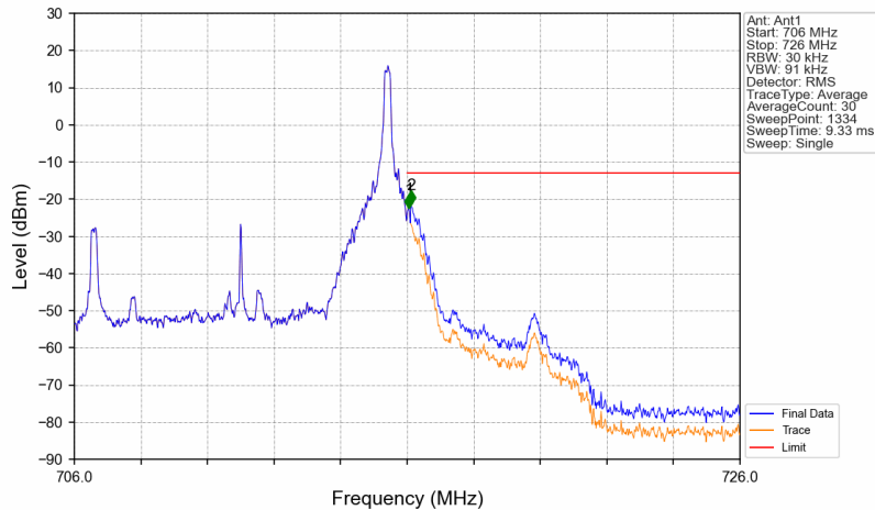
Band17_10MHz_QPSK_HCH_711MHz_RB_1_49_NTNV
