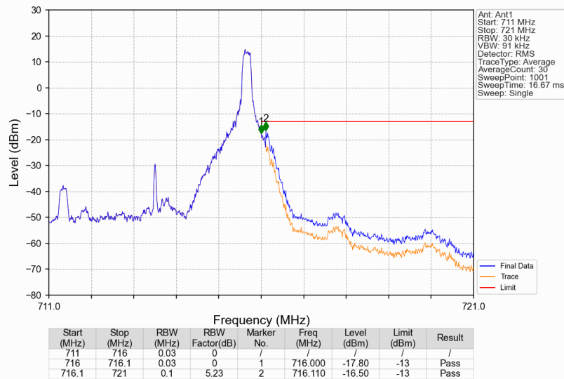
Band17_5MHz_16QAM_HCH_713.5MHz_RB_1_24_NTNV
