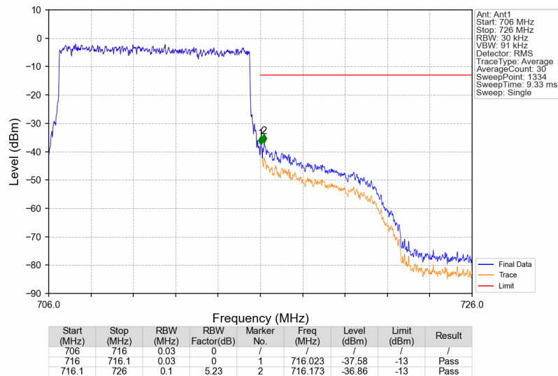
Band17_10MHz_16QAM_HCH_711MHz_RB_50_0_NTNV
