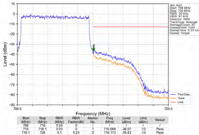
Band12_10MHz_QPSK_HCH_711MHz_RB_50_0_NTNV
