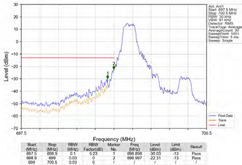
Band12_1.4MHz_16QAM_LCH_699.7MHz_RB_1_0_NTNV
