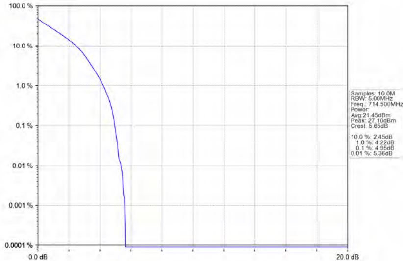
Band12_3MHz_QPSK_HCH_714.5MHz_RB_15_0_NTNV
