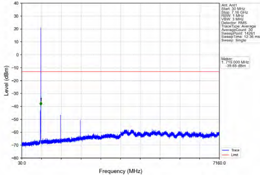
Band12_1.4MHz_QPSK_HCH_715.3MHz_RB_1_5_NTV
