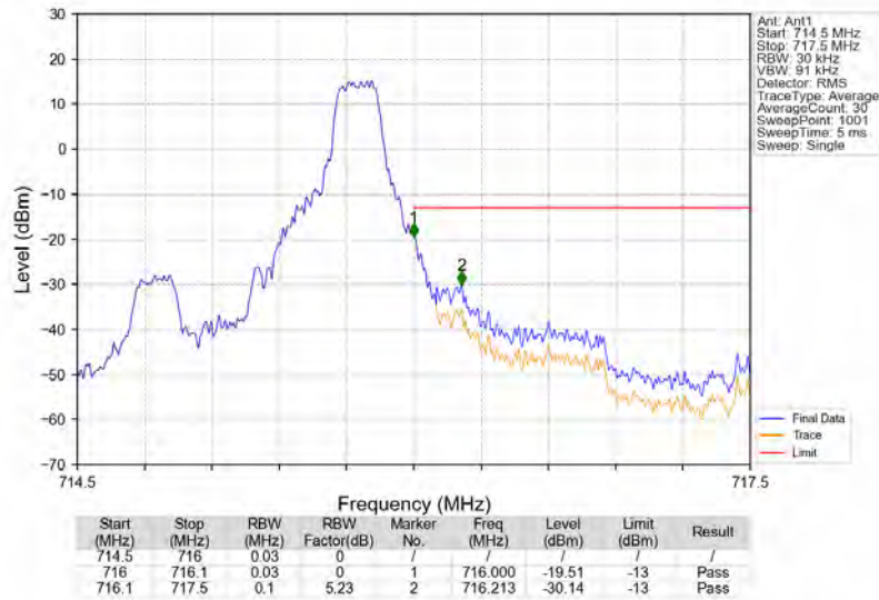
Band12_1.4MHz_QPSK_HCH_715.3MHz_RB_1_5_NTV
