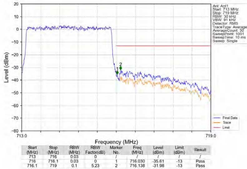
Band12_3MHz_16QAM_HCH_714.5MHz_RB_15_0_NTNV
