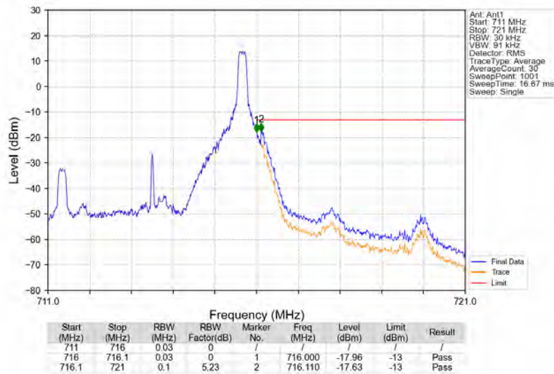
Band12_5MHz_16QAM_HCH_713.5MHz_RB_1_24_NTNV
