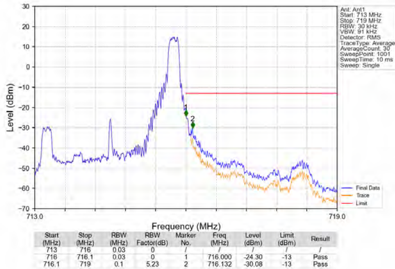
Band12_3MHz_16QAM_HCH_714.5MHz_RB_1_14_NTNV
