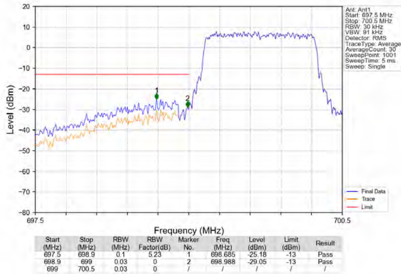
Band12_1.4MHz_QPSK_LCH_699.7MHz_RB_6_0_NTV
