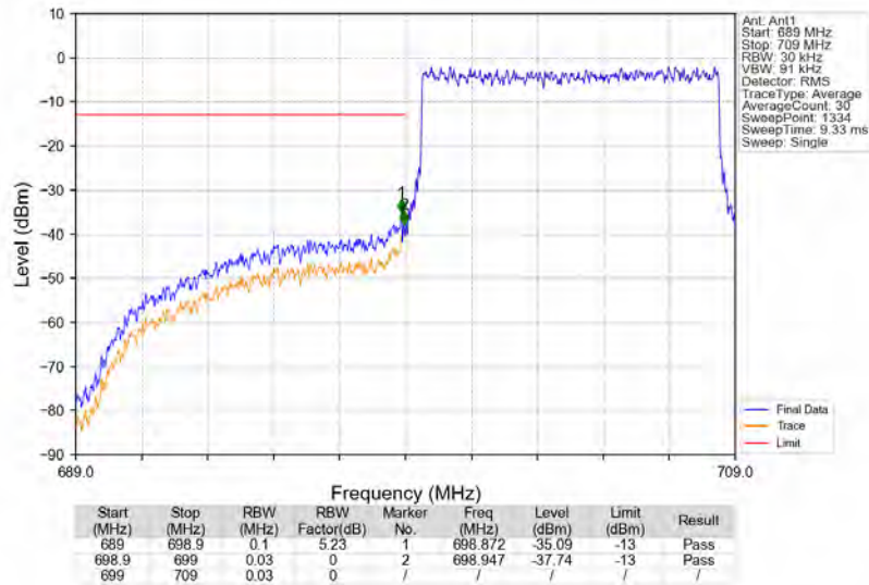
Band12_10MHz_16QAM_LCH_704MHz_RB_50_0_NTNV
