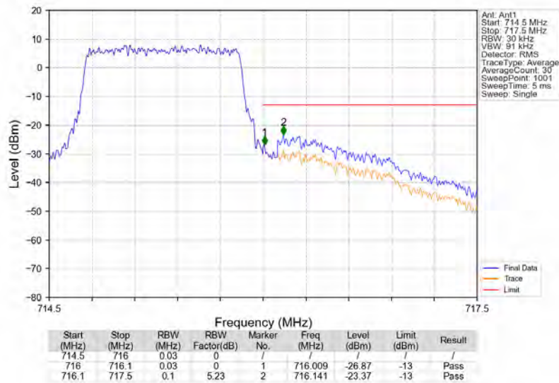
Band12_1.4MHz_QPSK_HCH_715.3MHz_RB_6_0_NTNV
