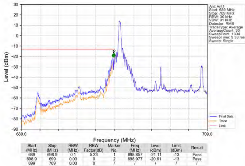
Band12_10MHz_16QAM_LCH_704MHz_RB_1_0_NTNV
