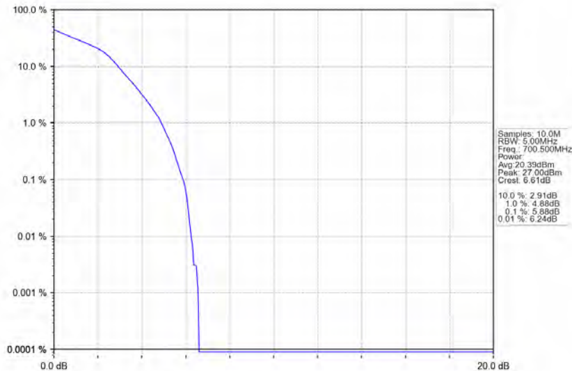
Band12_3MHz_16QAM_LCH_700.5MHz_RB_15_0_NTNV
