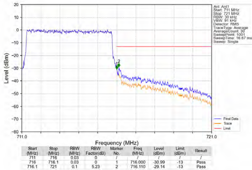
Band12_5MHz_16QAM_HCH_713.5MHz_RB_25_0_NTNV
