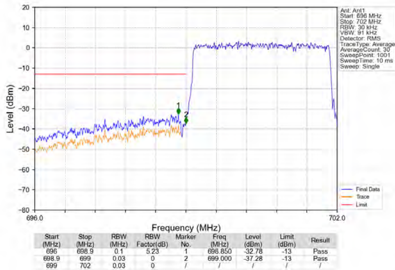
Band12_3MHz_16QAM_LCH_700.5MHz_RB_15_0_NTNV
