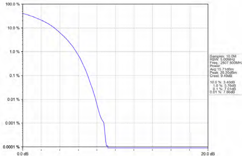
Band7_15MHz_16QAM_LCH_2507.5MHz_RB_75_0_NTNV
