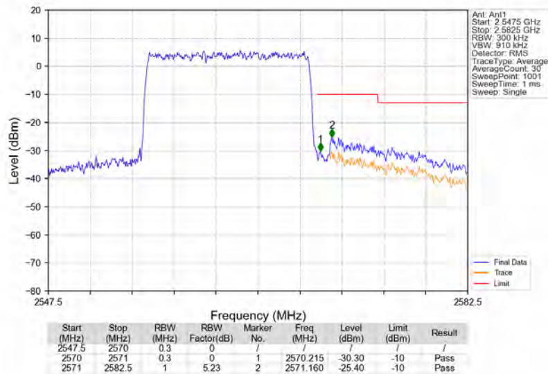
Band7_15MHz_16QAM_HCH_2562.5MHz_RB_75_0_NTNV
