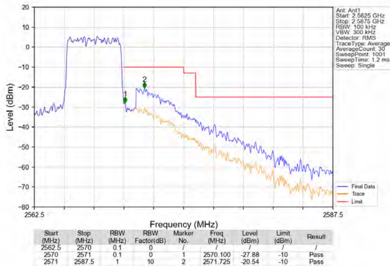
Band7_5MHz_16QAM_HCH_2567.5MHz_RB_25_0_NTNV
