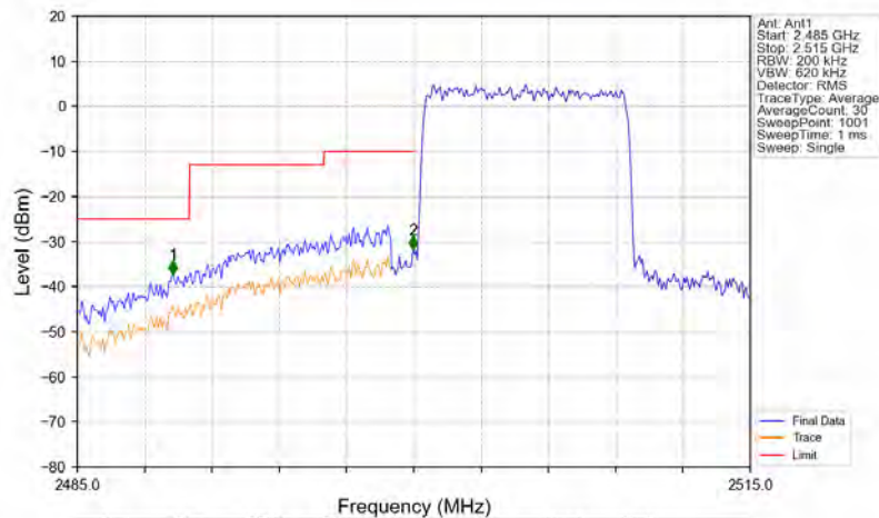
Band7_10MHz_16QAM_LCH_2505MHz_RB_50_0_NTNV
