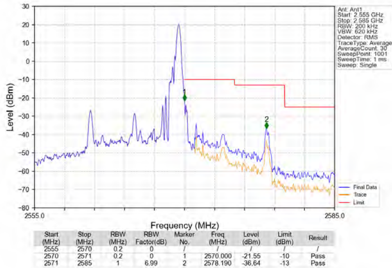
Band7_10MHz_16QAM_HCH_2565MHz_RB_1_49_NTNV
