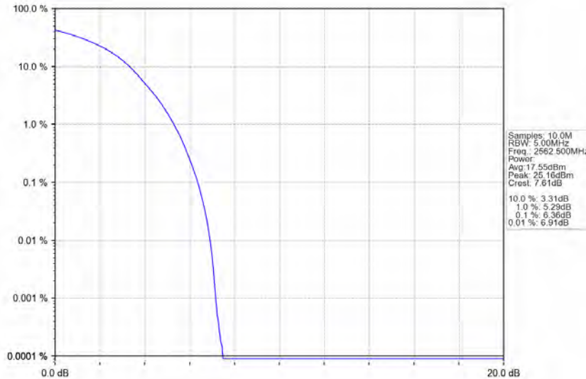
Band7_15MHz_QPSK_HCH_2562.5MHz_RB_75_0_NTNV
