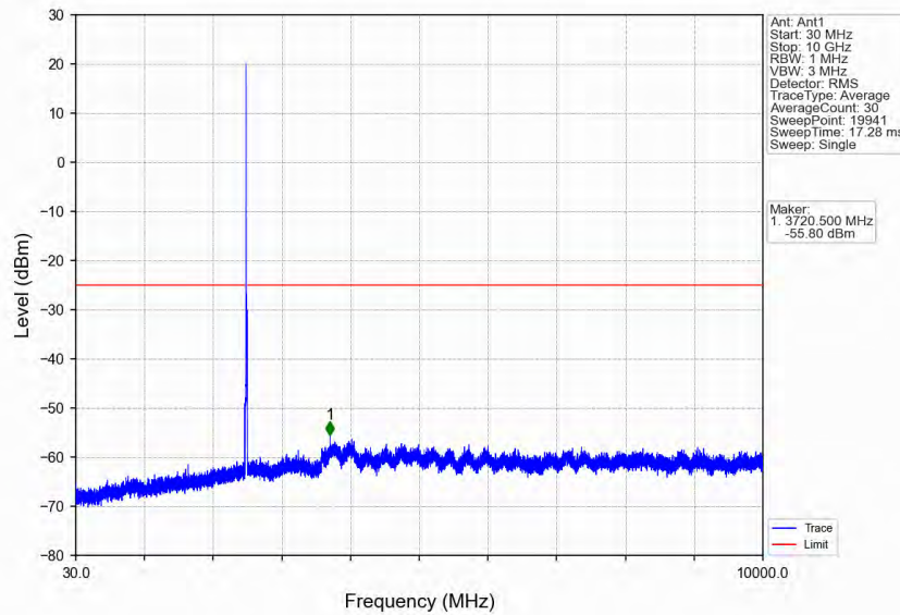
Band7_10MHz_16QAM_LCH_2505MHz_RB_1_0_NTNV
