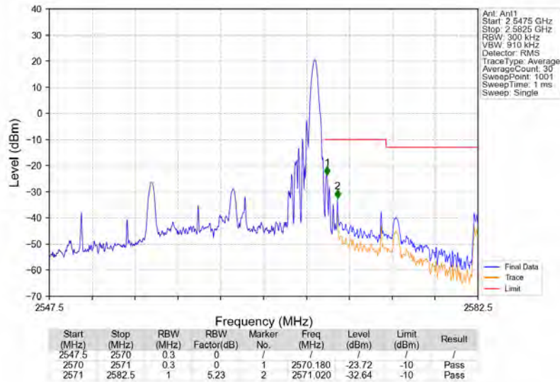
Band7_15MHz_16QAM_HCH_2562.5MHz_RB_1_74_NTNV
