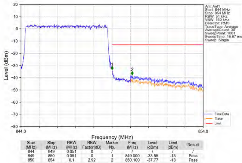
Band5_5MHz_QPSK_HCH_846.5MHz_RB_25_0_NTNV
