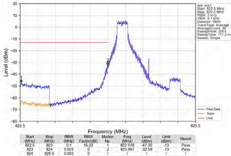
Band5_1.4MHz_16QAM_LCH_824.7MHz_RB_1_0_NTNV
