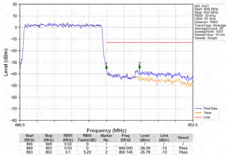
Band5_3MHz_QPSK_HCH_847.5MHz_RB_15_0_NTNV
