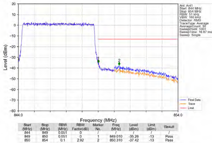
Band5_5MHz_16QAM_HCH_846.5MHz_RB_25_0_NTNV
