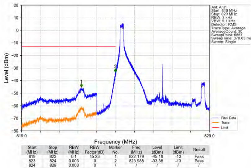
Band5_5MHz_16QAM_LCH_826.5MHz_RB_1_0_NTNV
