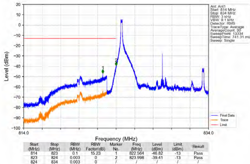
Band5_10MHz_16QAM_LCH_829MHz_RB_1_0_NTNV
