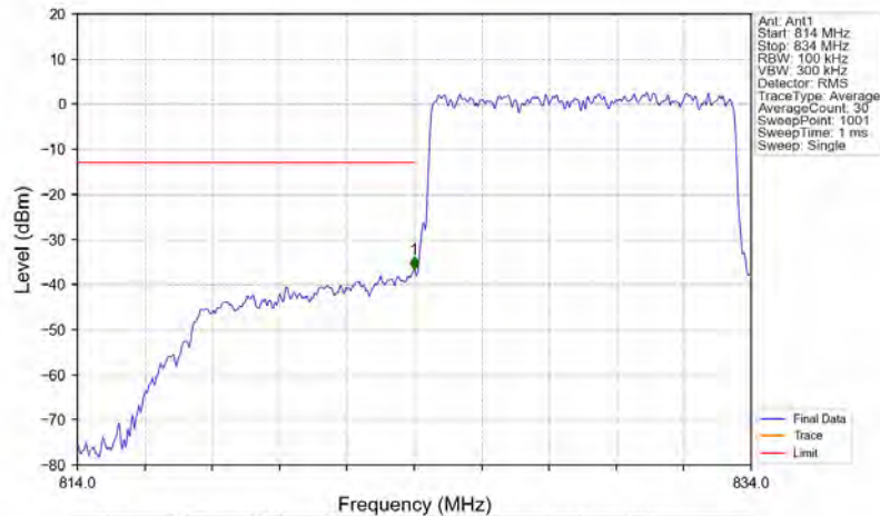
Band5_10MHz_16QAM_LCH_829MHz_RB_50_0_NTNV
