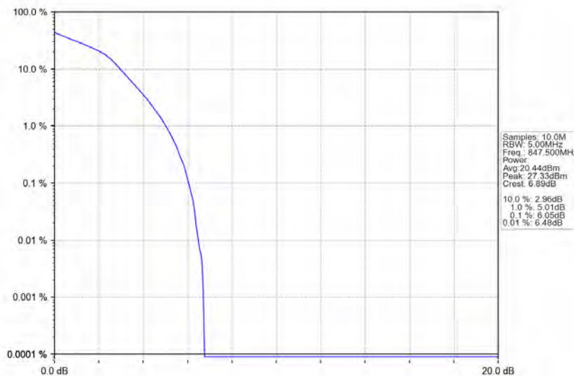
Band5_3MHz_16QAM_HCH_847.5MHz_RB_15_0_NTNV
