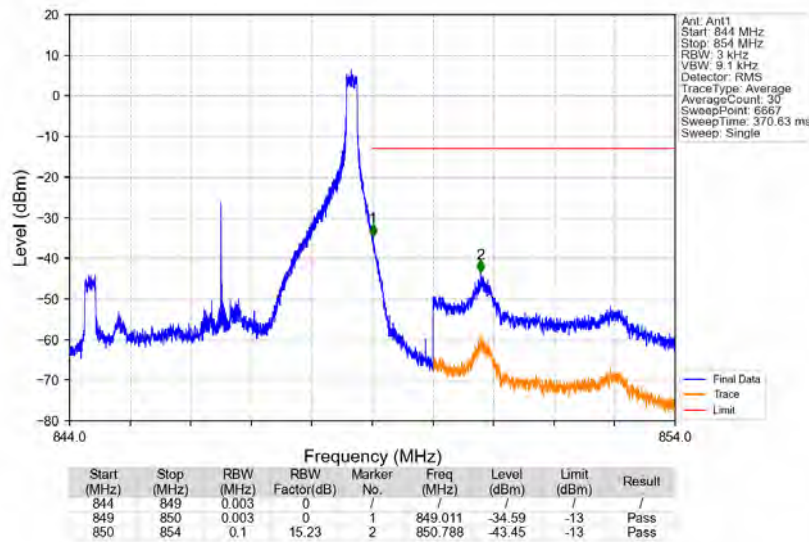
Band5_5MHz_16QAM_HCH_846.5MHz_RB_1_24_NTNV
