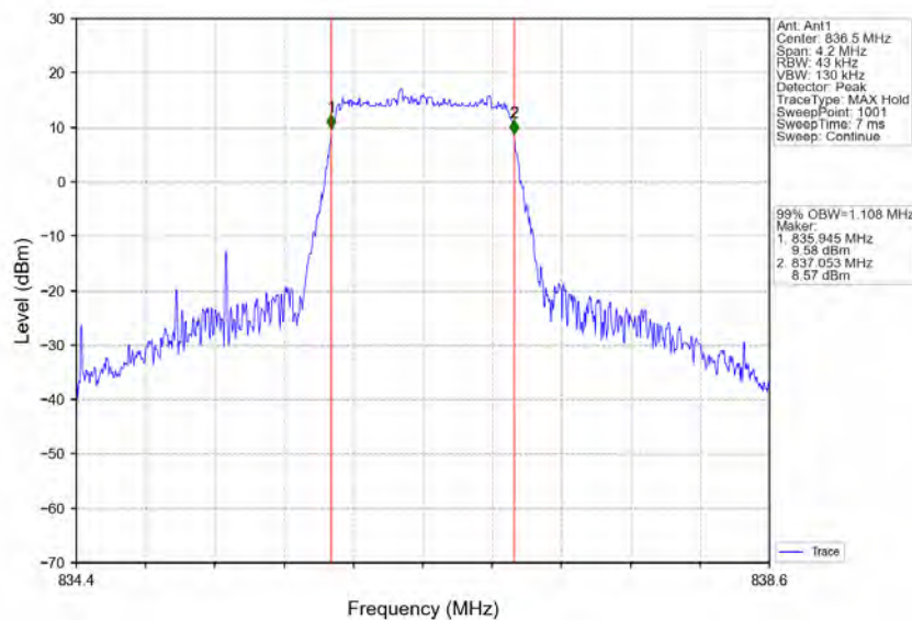
Band5_1.4MHz_16QAM_MCH_836.5MHz_RB_6_0_NTNV
