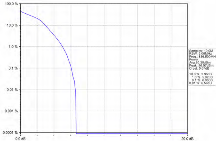
Band5_3MHz_16QAM_MCH_836.5MHz_RB_15_0_NTNV
