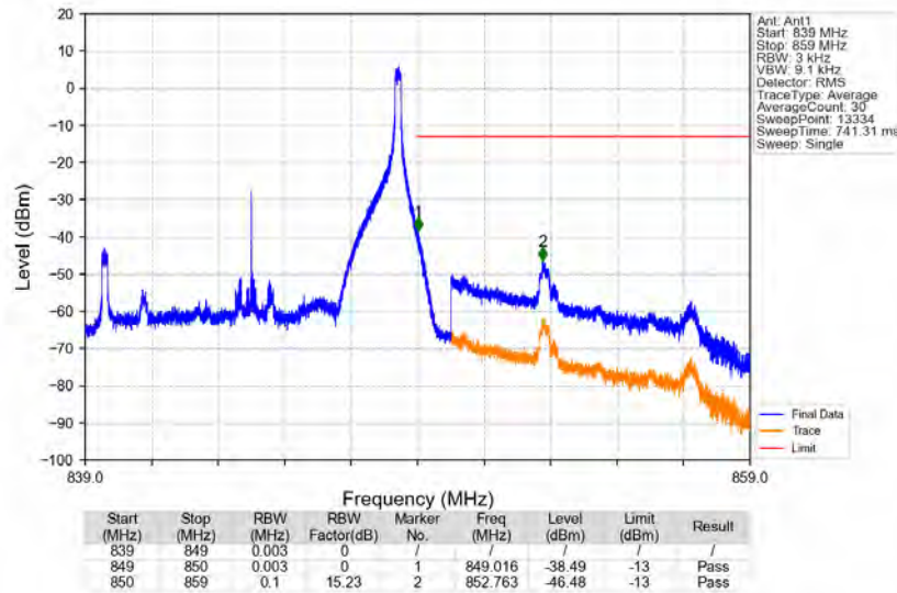
Band5_10MHz_16QAM_HCH_844MHz_RB_1_49_NTNV
