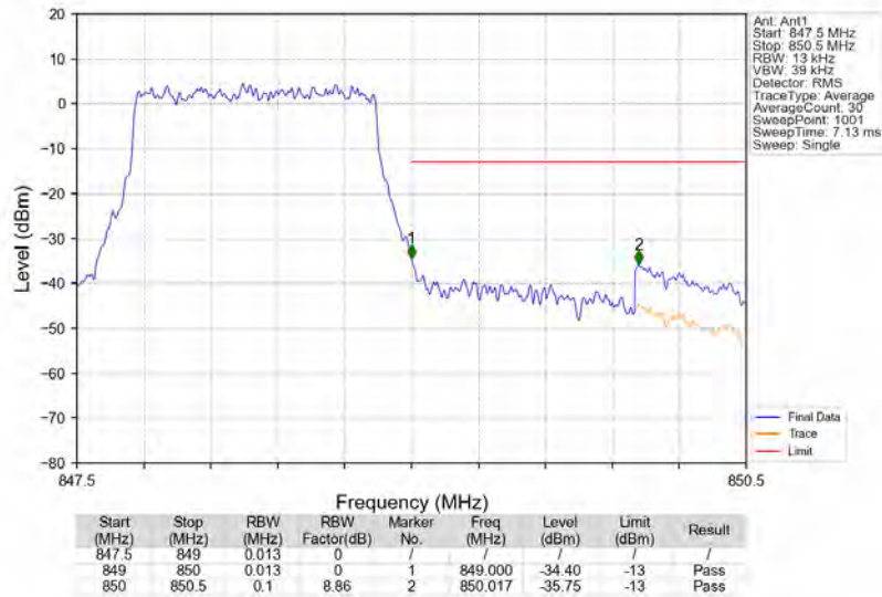
Band5_1.4MHz_QPSK_HCH_848.3MHz_RB_6_0_NTNV
