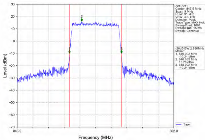
Band5_3MHz_16QAM_HCH_847.5MHz_RB_15_0_NTNV
