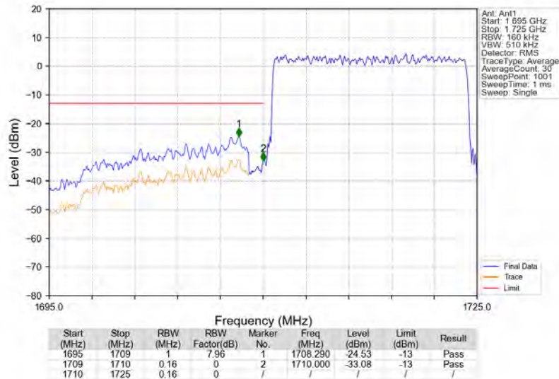
Band4_15MHz_QPSK_LCH_1717.5MHz_RB_75_0_NTNV
