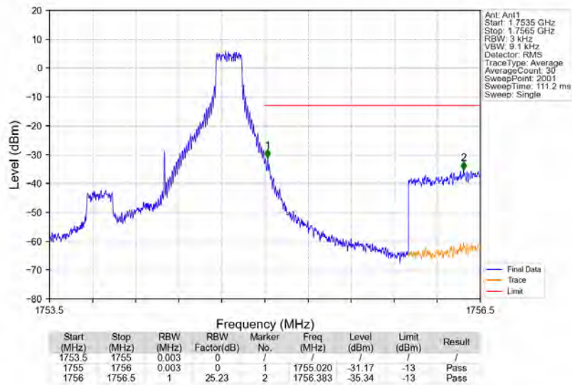
Band4_1.4MHz_16QAM_HCH_1754.3MHz_RB_1_5_NTNV
