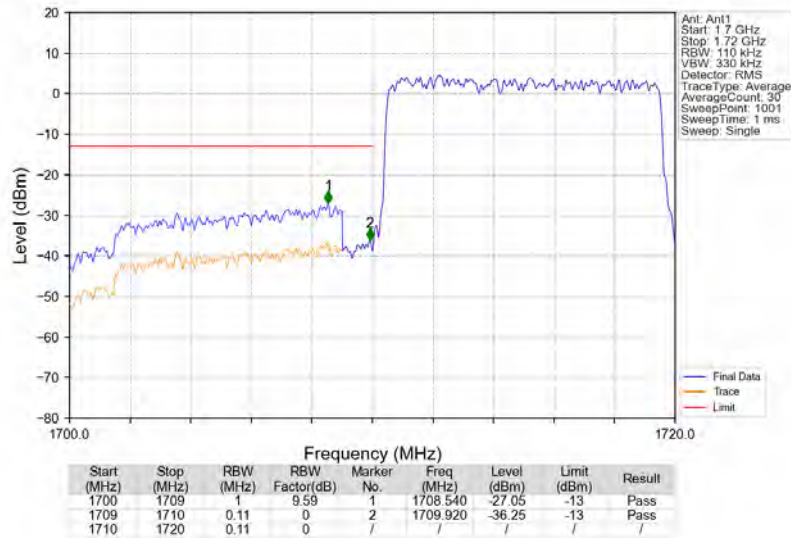
Band4_10MHz_QPSK_LCH_1715MHz_RB_50_0_NTNV
