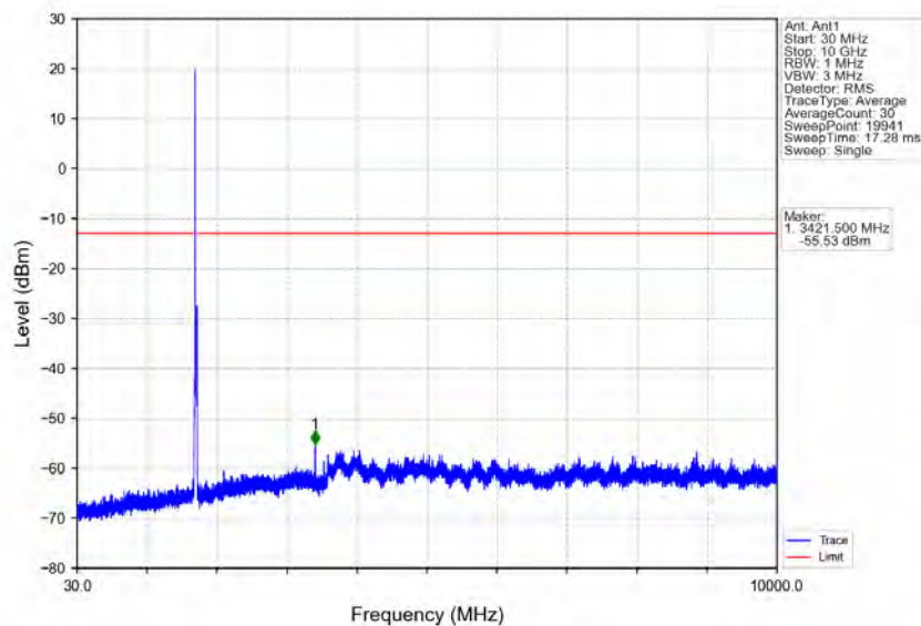
Band4_15MHz_16QAM_LCH_1717.5MHz_RB_1_0_NTNV
