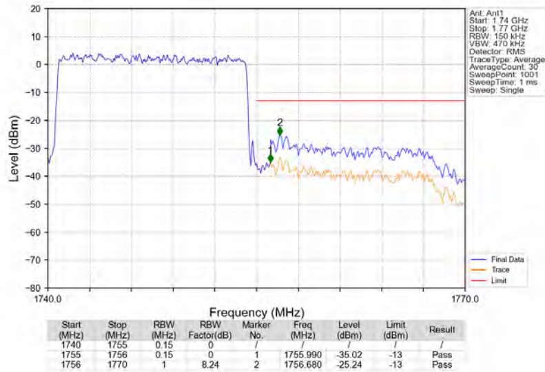
Band4_15MHz_QPSK_HCH_1747.5MHz_RB_75_0_NTNV
