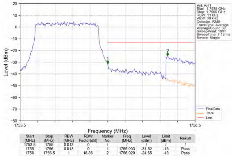
Band4_1.4MHz_QPSK_HCH_1754.3MHz_RB_6_0_NTV
