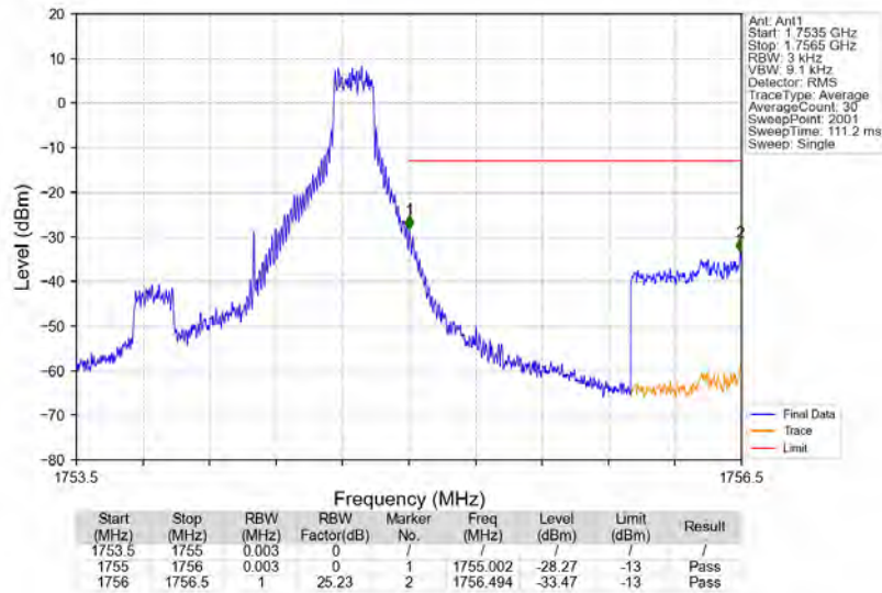
Band4_1.4MHz_QPSK_HCH_1754.3MHz_RB_1_5_NTV
