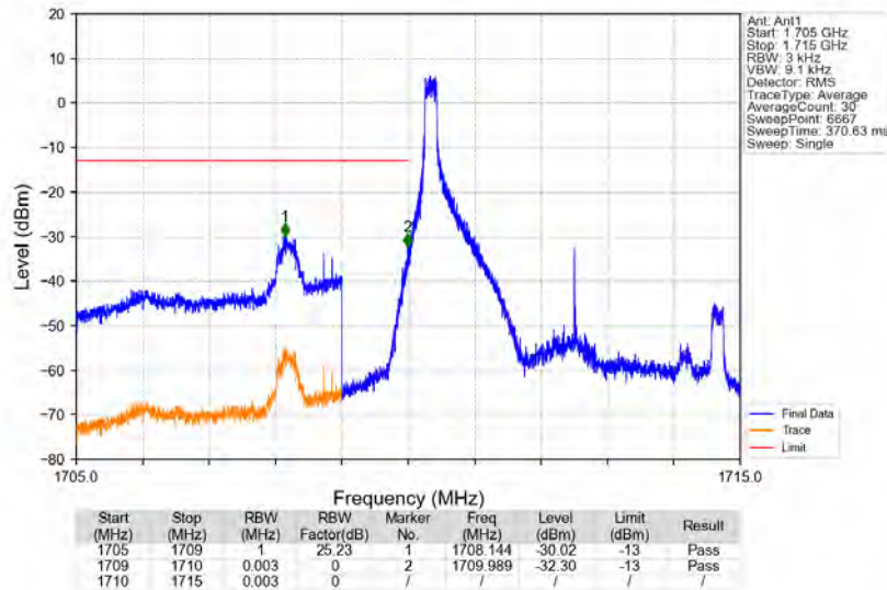
Band4_5MHz_16QAM_LCH_1712.5MHz_RB_1_0_NTNV
