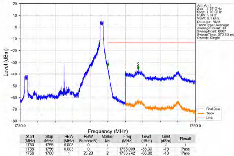
Band4_5MHz_16QAM_HCH_1752.5MHz_RB_1_24_NTNV
