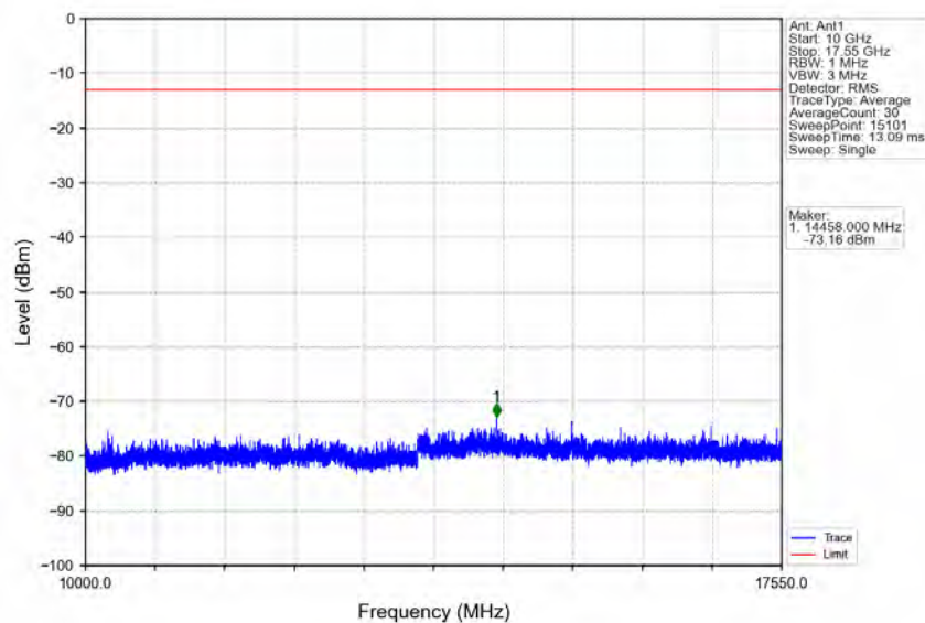
Band4_3MHz_QPSK_HCH_1753.5MHz_RB_1_0_NTNV
