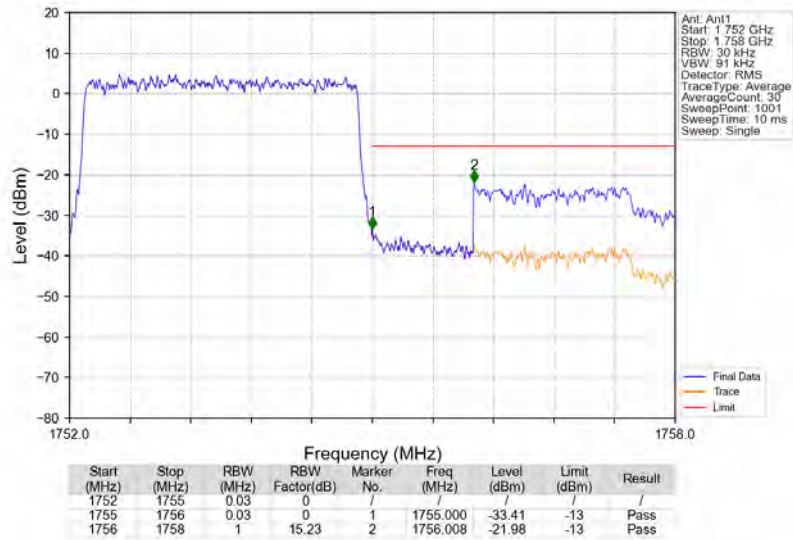
Band4_3MHz_QPSK_HCH_1753.5MHz_RB_15_0_NTNV
