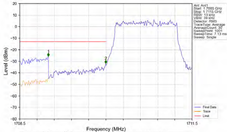
Band4_1.4MHz_QPSK_LCH_1710.7MHz_RB_6_0_NTNV
