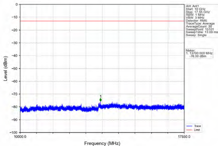
Band4_10MHz_QPSK_MCH_1732.5MHz_RB_1_0_NTV
