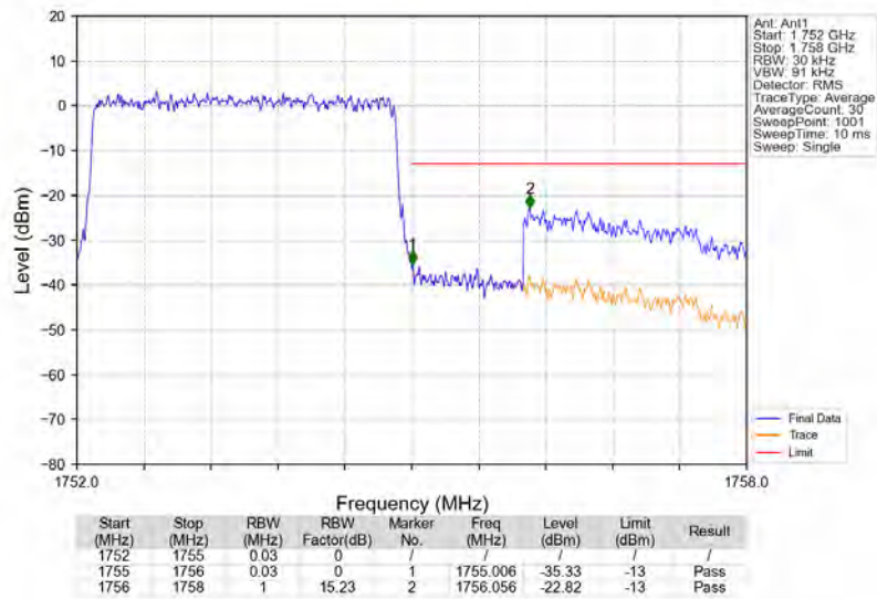
Band4_3MHz_16QAM_HCH_1753.5MHz_RB_15_0_NTNV
