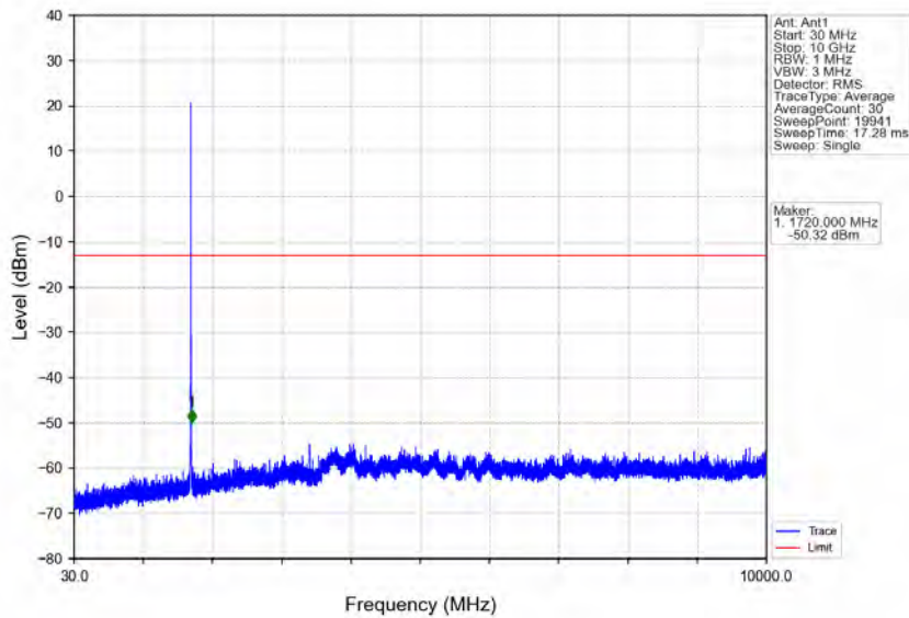
Band4_3MHz_16QAM_LCH_1711.5MHz_RB_1_0_NTNV
