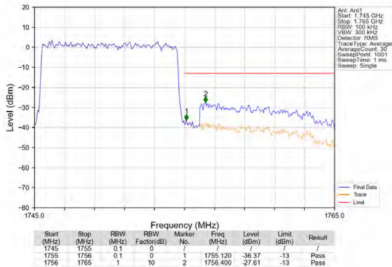
Band4_10MHz_16QAM_HCH_1750MHz_RB_50_0_NTV
