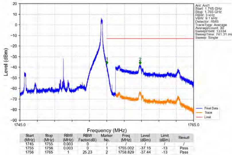
Band4_10MHz_16QAM_HCH_1750MHz_RB_1_49_NTV
