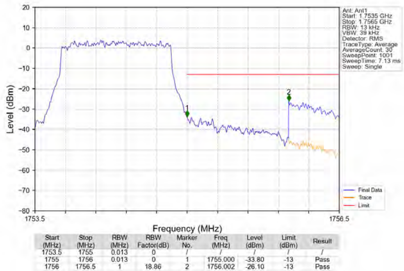
Band4_1.4MHz_16QAM_HCH_1754.3MHz_RB_6_0_NTNV
