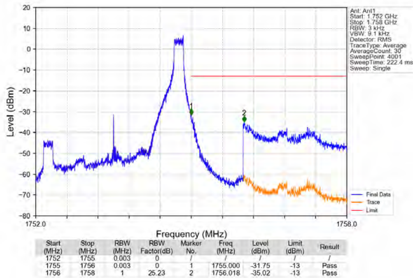
Band4_3MHz_16QAM_HCH_1753.5MHz_RB_1_14_NTNV
