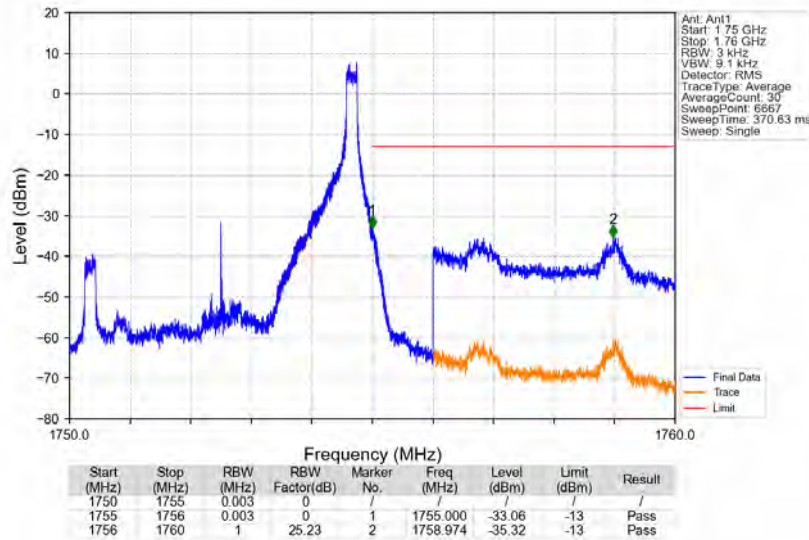
Band4_5MHz_QPSK_HCH_1752.5MHz_RB_1_24_NTNV
