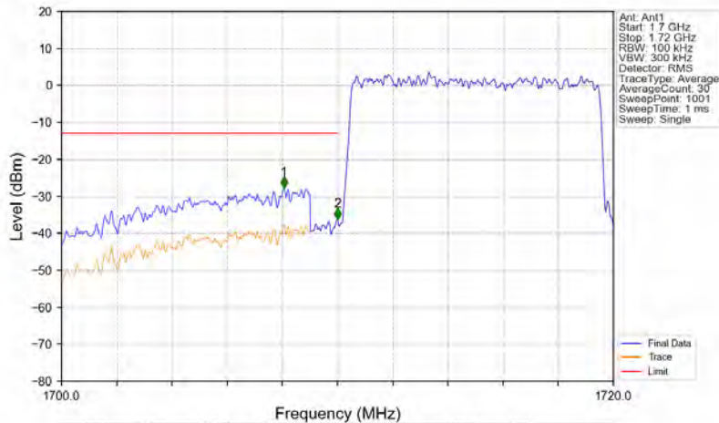
Band4_10MHz_16QAM_LCH_1715MHz_RB_50_0_NTNV
