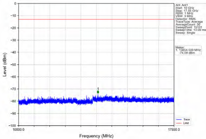
Band4_1.4MHz_QPSK_LCH_1710.7MHz_RB_6_0_NTNV
