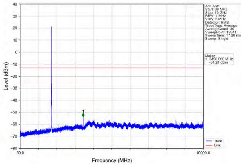
Band4_10MHz_QPSK_MCH_1732.5MHz_RB_1_0_NTV
