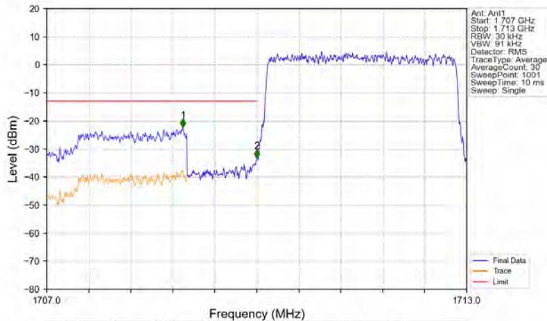
Band4_3MHz_QPSK_LCH_1711.5MHz_RB_15_0_NTNV
