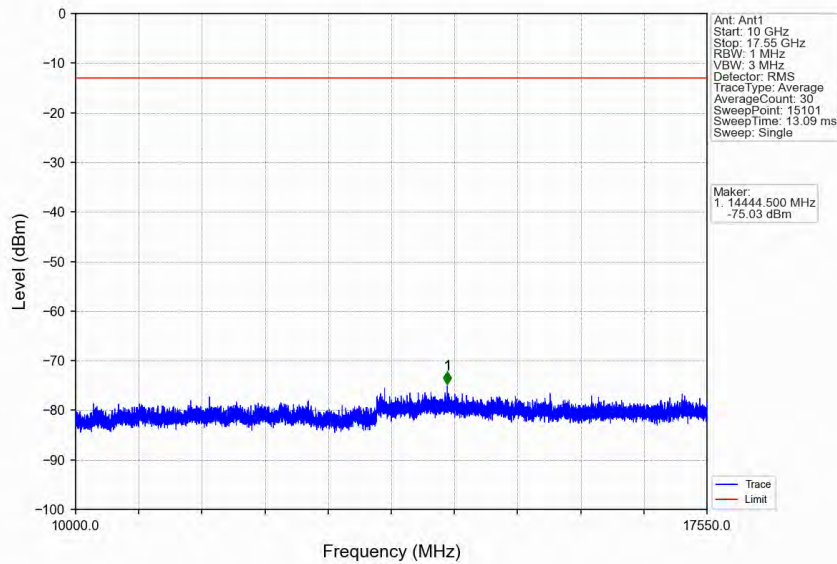
Band4_20MHz_16QAM_HCH_1745MHz_RB_1_0_NTNV
