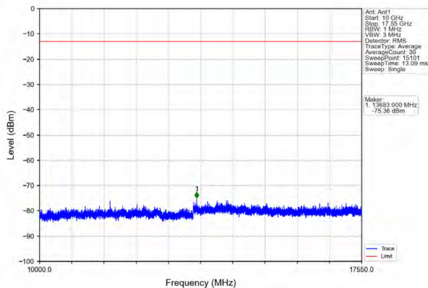
Band4_15MHz_QPSK_HCH_1747.5MHz_RB_1_0_NTNV
