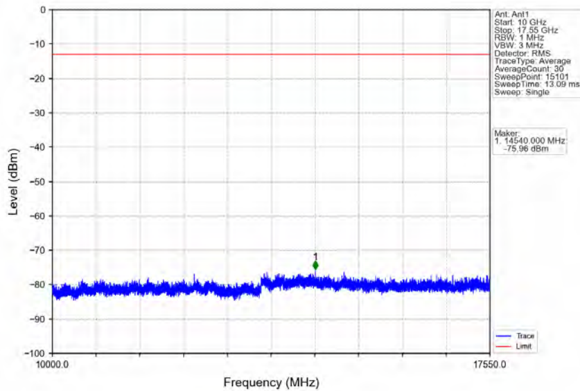
Band4_10MHz_16QAM_LCH_1715MHz_RB_50_0_NTNV
