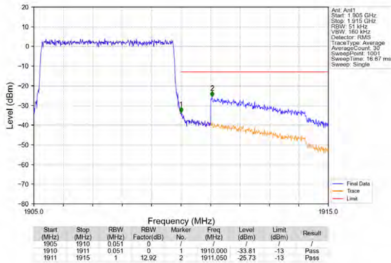
Band2_5MHz_QPSK_HCH_1907.5MHz_RB_25_0_NTNV
