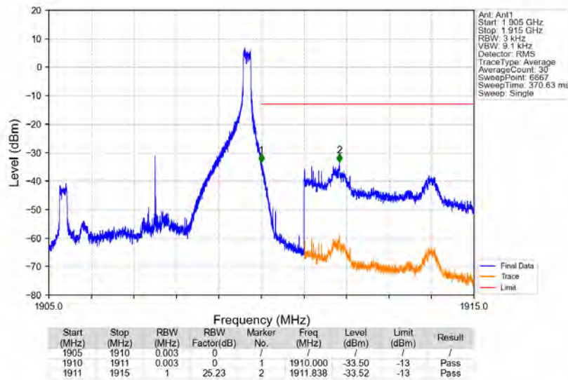
Band2_5MHz_QPSK_HCH_1907.5MHz_RB_1_24_NTNV
