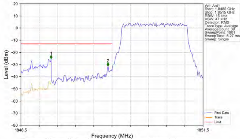
Band2_1.4MHz_QPSK_LCH_1850.7MHz_RB_6_0_NTNV
