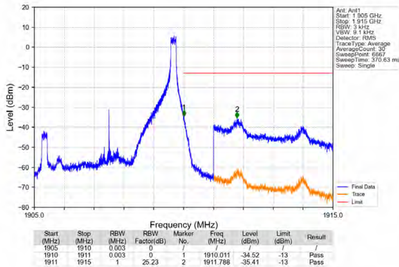
Band2_5MHz_16QAM_HCH_1907.5MHz_RB_1_24_NTNV
