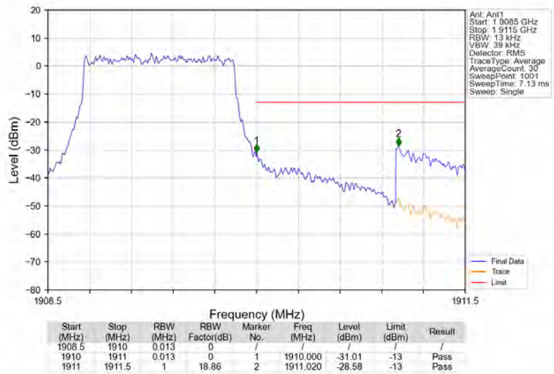
Band2_1.4MHz_QPSK_HCH_1909.3MHz_RB_6_0_NTV
