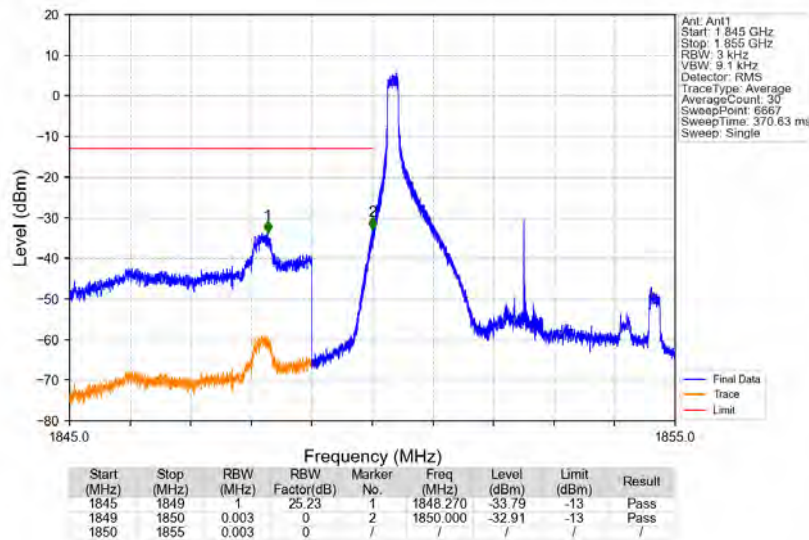
Band2_5MHz_16QAM_LCH_1852.5MHz_RB_1_0_NTNV
