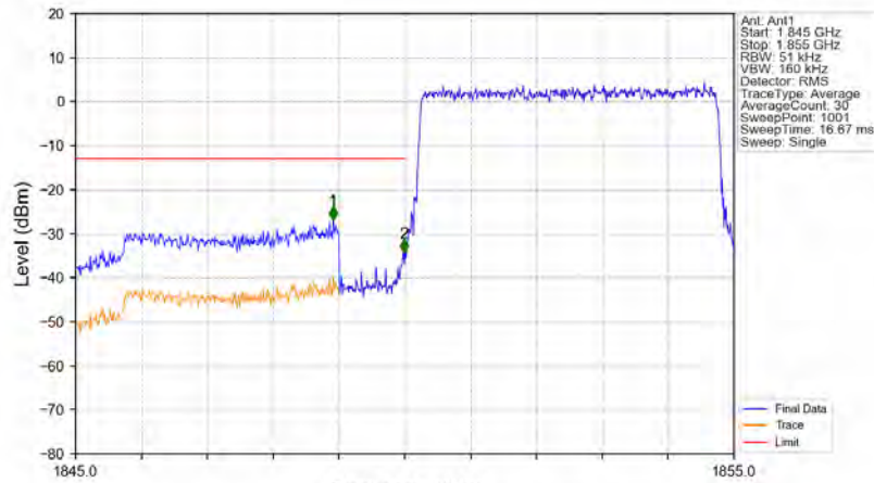
Band2_5MHz_QPSK_LCH_1852.5MHz_RB_25_0_NTNV
