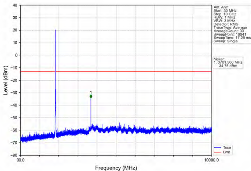
Band2_15MHz_16QAM_LCH_1857.5MHz_RB_1_0_NTNV
