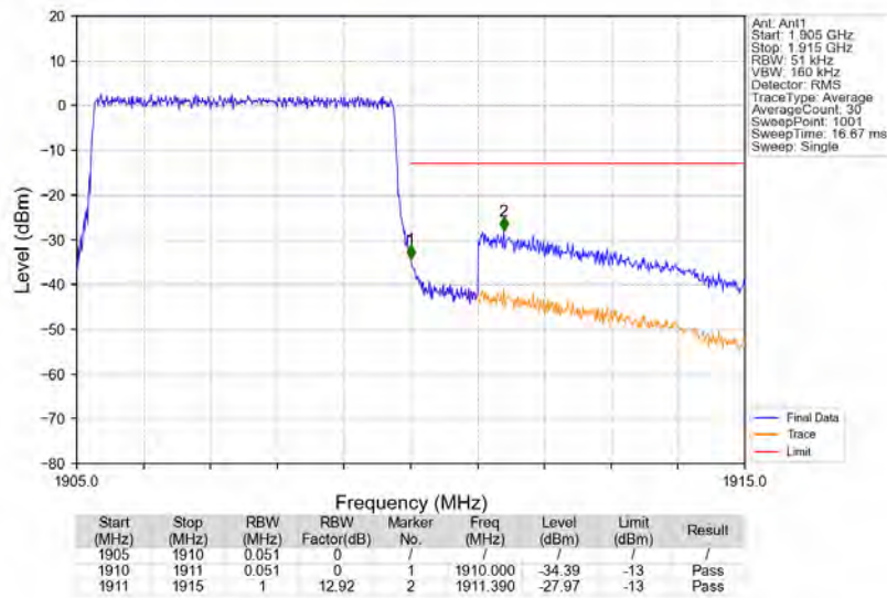
Band2_5MHz_16QAM_HCH_1907.5MHz_RB_25_0_NTNV
