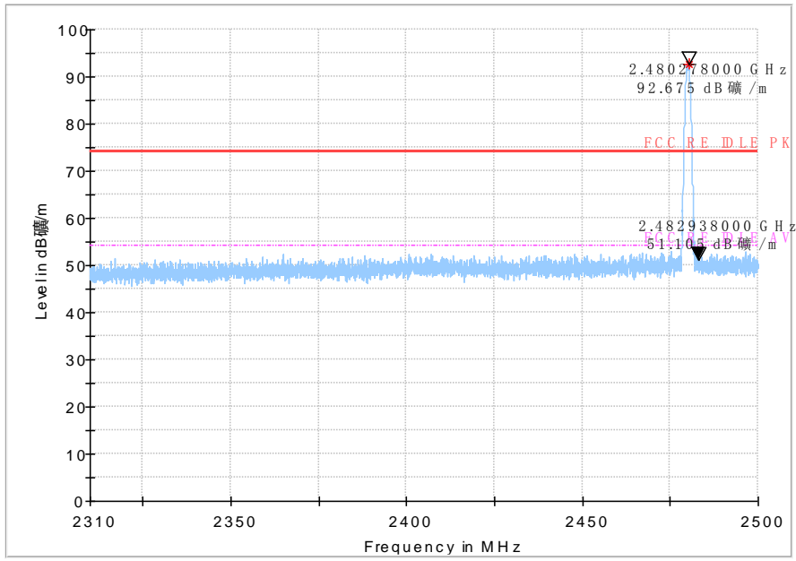
Fig.25 Bandedge:Ch39
