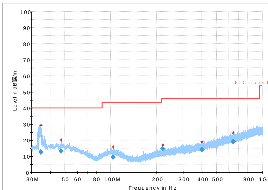
Fig. 19 Radiated Spurious Emission (802.11a, Ch157, 30 MHz-1 GHz)
